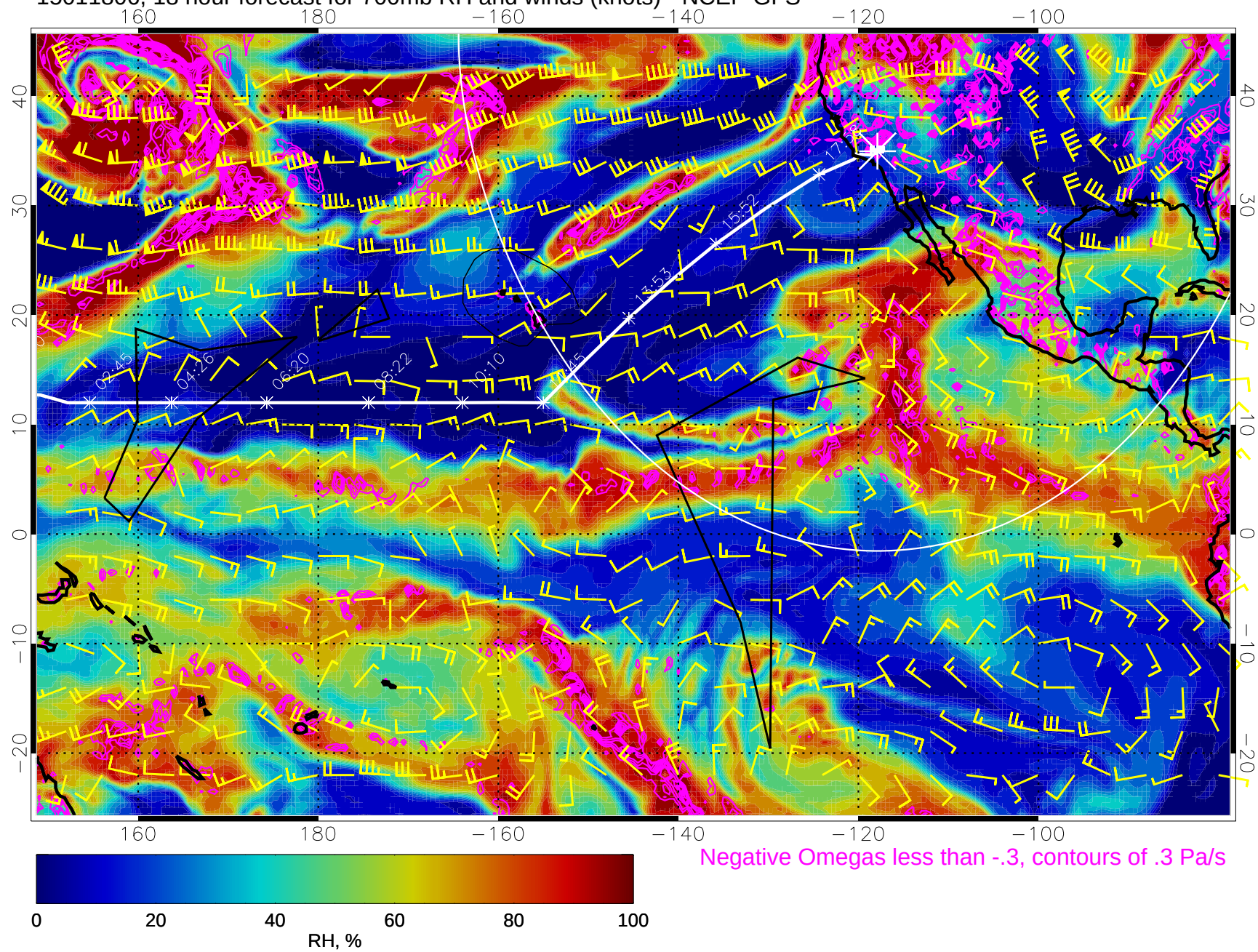
15011806, 18 hour forecast for 700mb RH and winds (knots) - NCEP GFS
