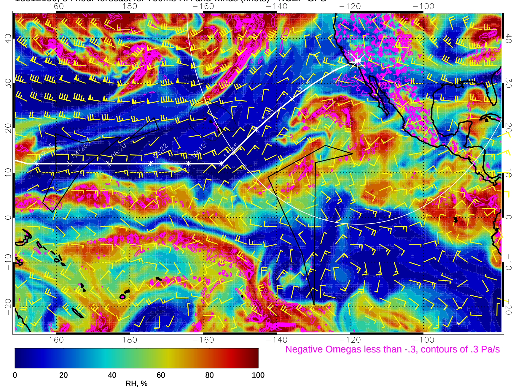
15012100, 84 hour forecast for 700mb RH and winds (knots) - NCEP GFS
