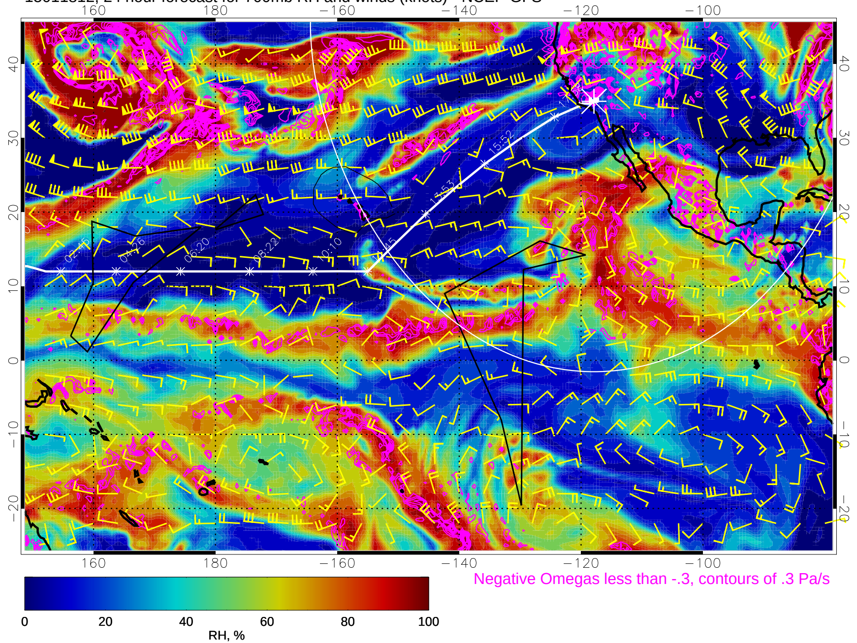
15011812, 24 hour forecast for 700mb RH and winds (knots) - NCEP GFS
