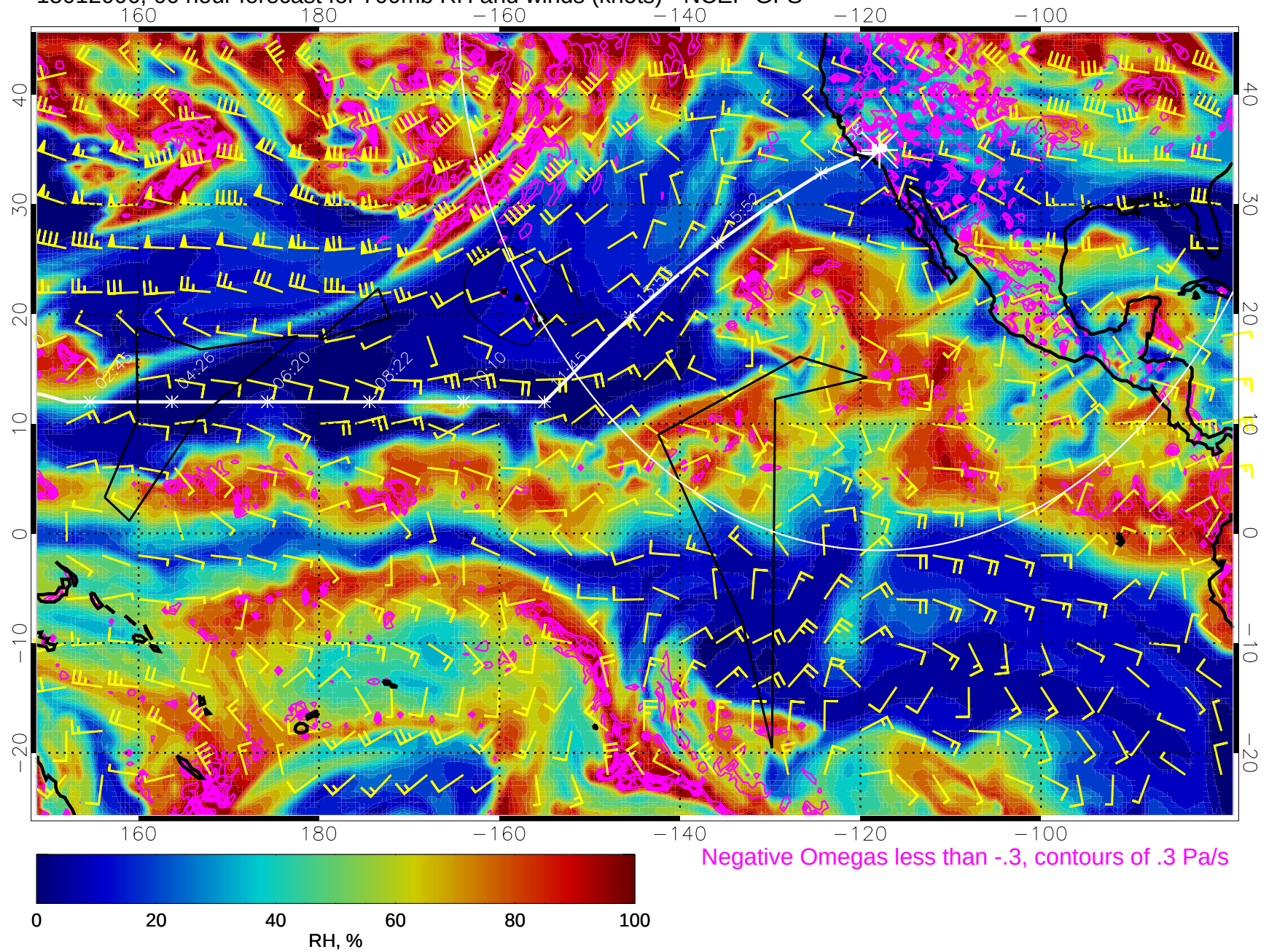
15012006, 66 hour forecast for 700mb RH and winds (knots) - NCEP GFS
