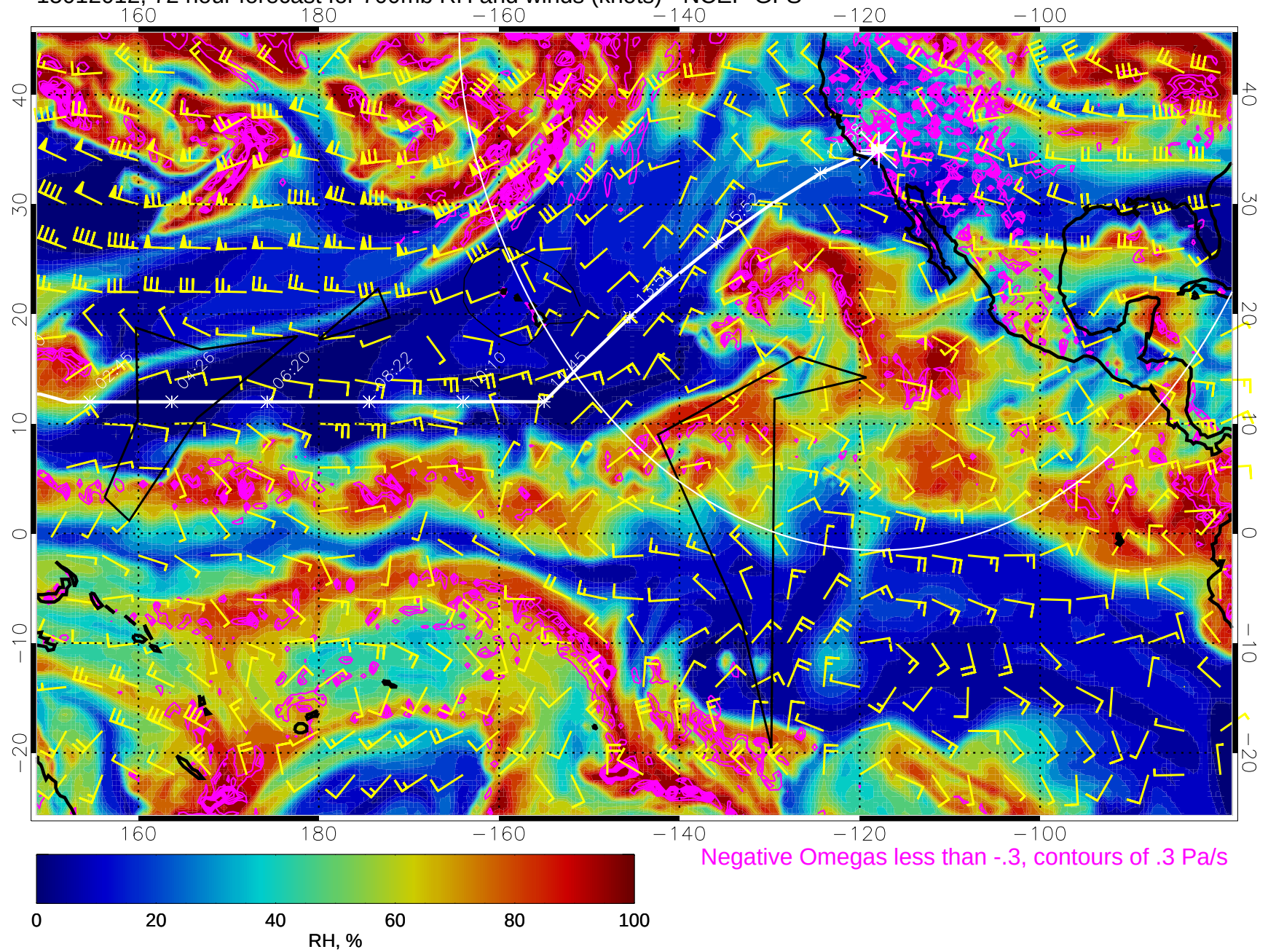
15012012, 72 hour forecast for 700mb RH and winds (knots) - NCEP GFS
