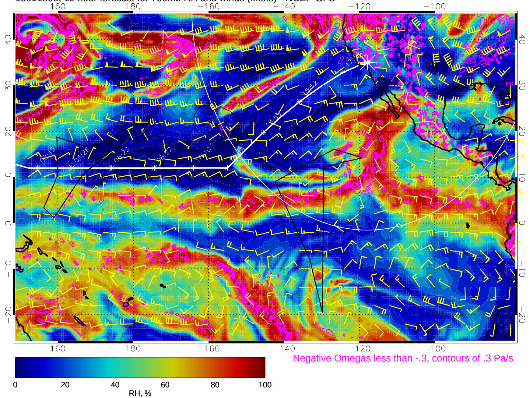
15011800, 12 hour forecast for 700mb RH and winds (knots) - NCEP GFS
