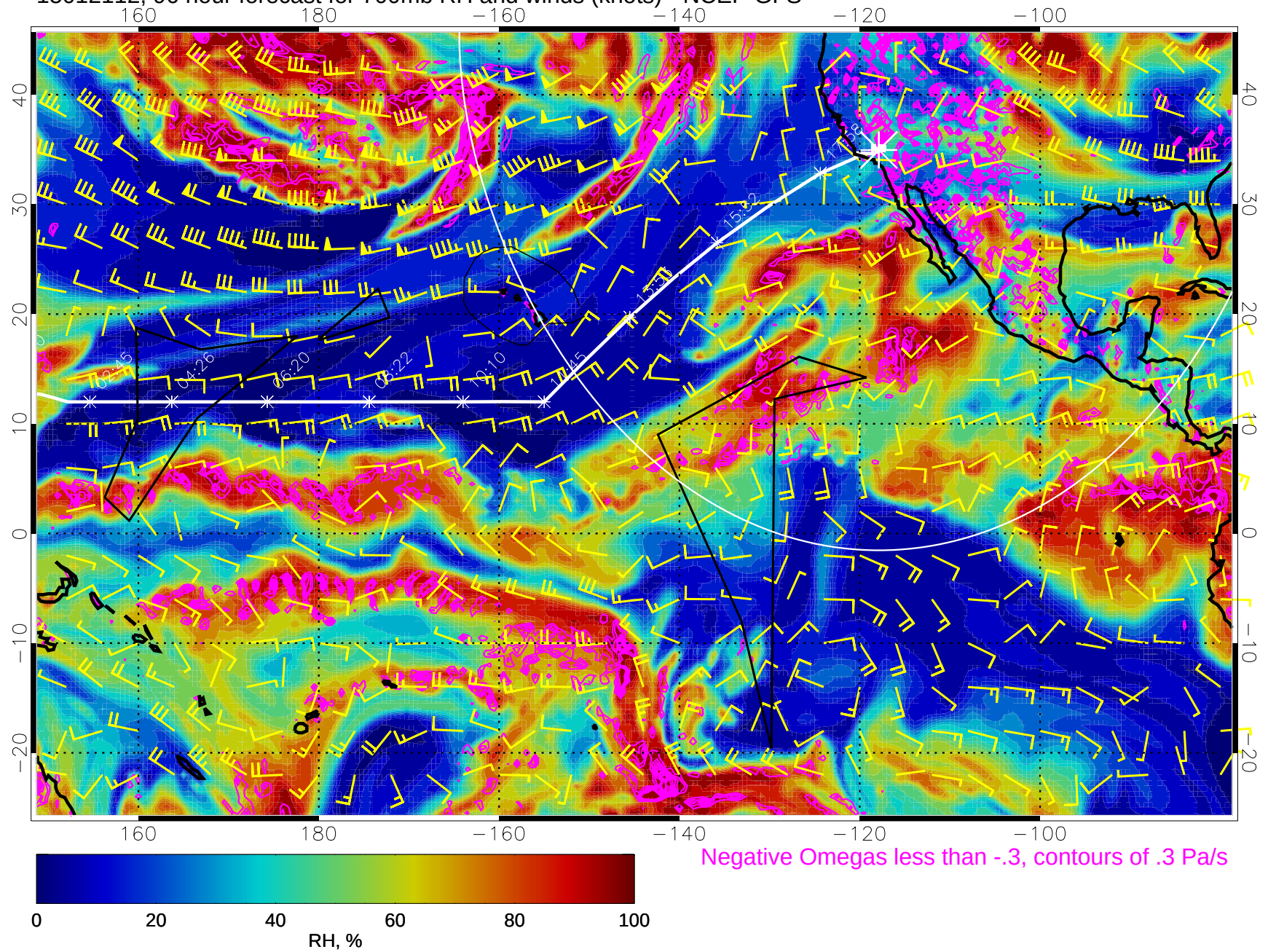
15012112, 96 hour forecast for 700mb RH and winds (knots) - NCEP GFS
