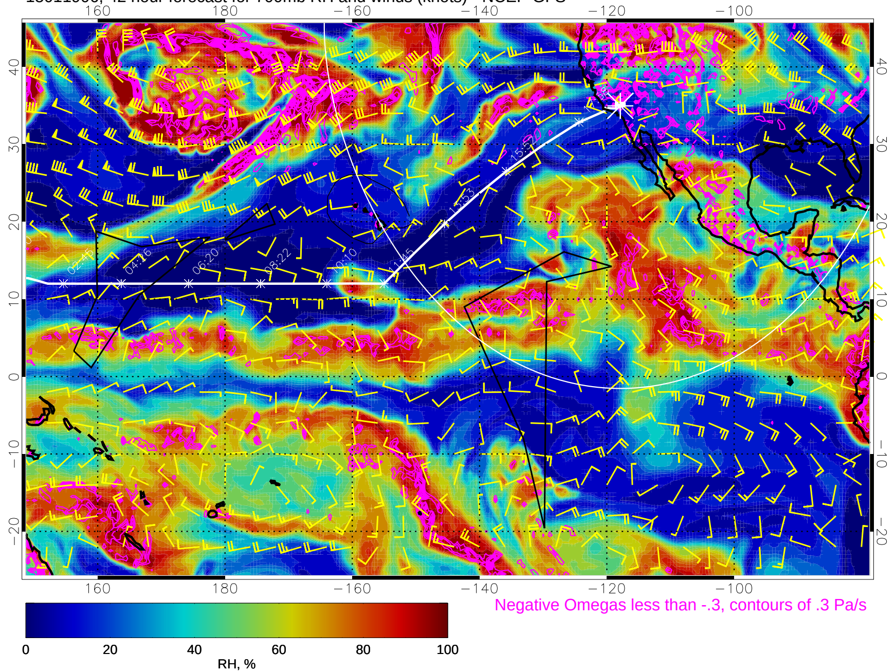
15011906, 42 hour forecast for 700mb RH and winds (knots) - NCEP GFS
