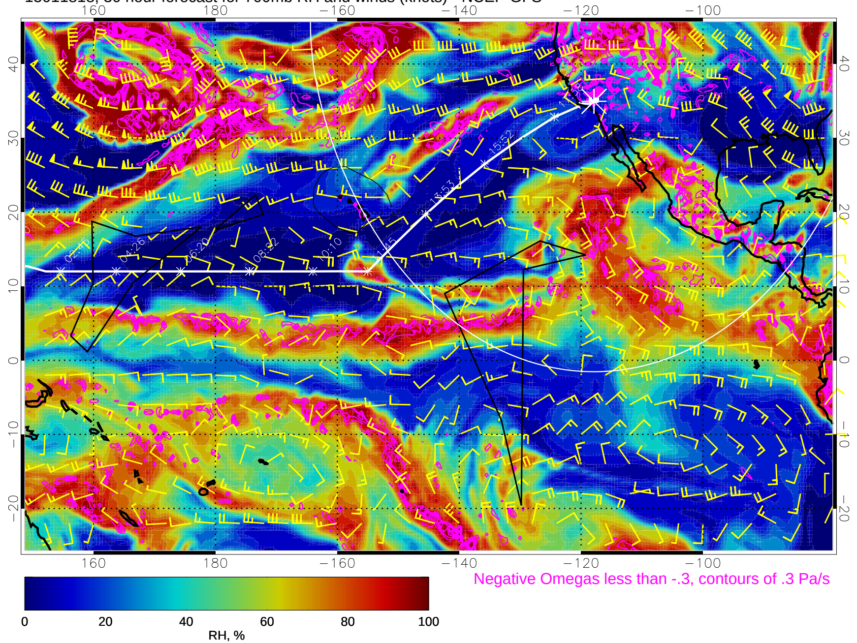
15011818, 30 hour forecast for 700mb RH and winds (knots) - NCEP GFS
