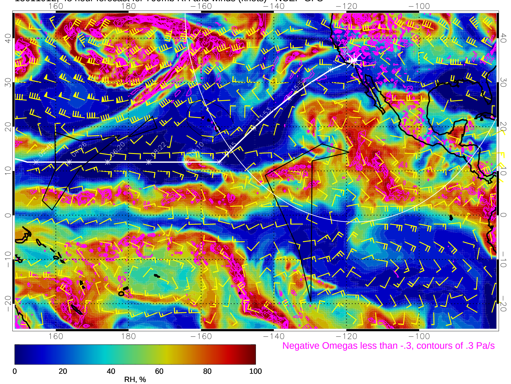
15011912, 48 hour forecast for 700mb RH and winds (knots) - NCEP GFS
