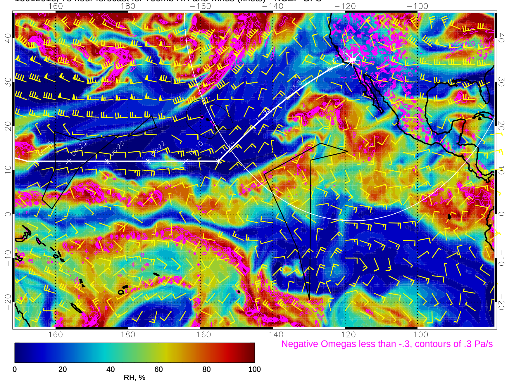
15012018, 78 hour forecast for 700mb RH and winds (knots) - NCEP GFS
