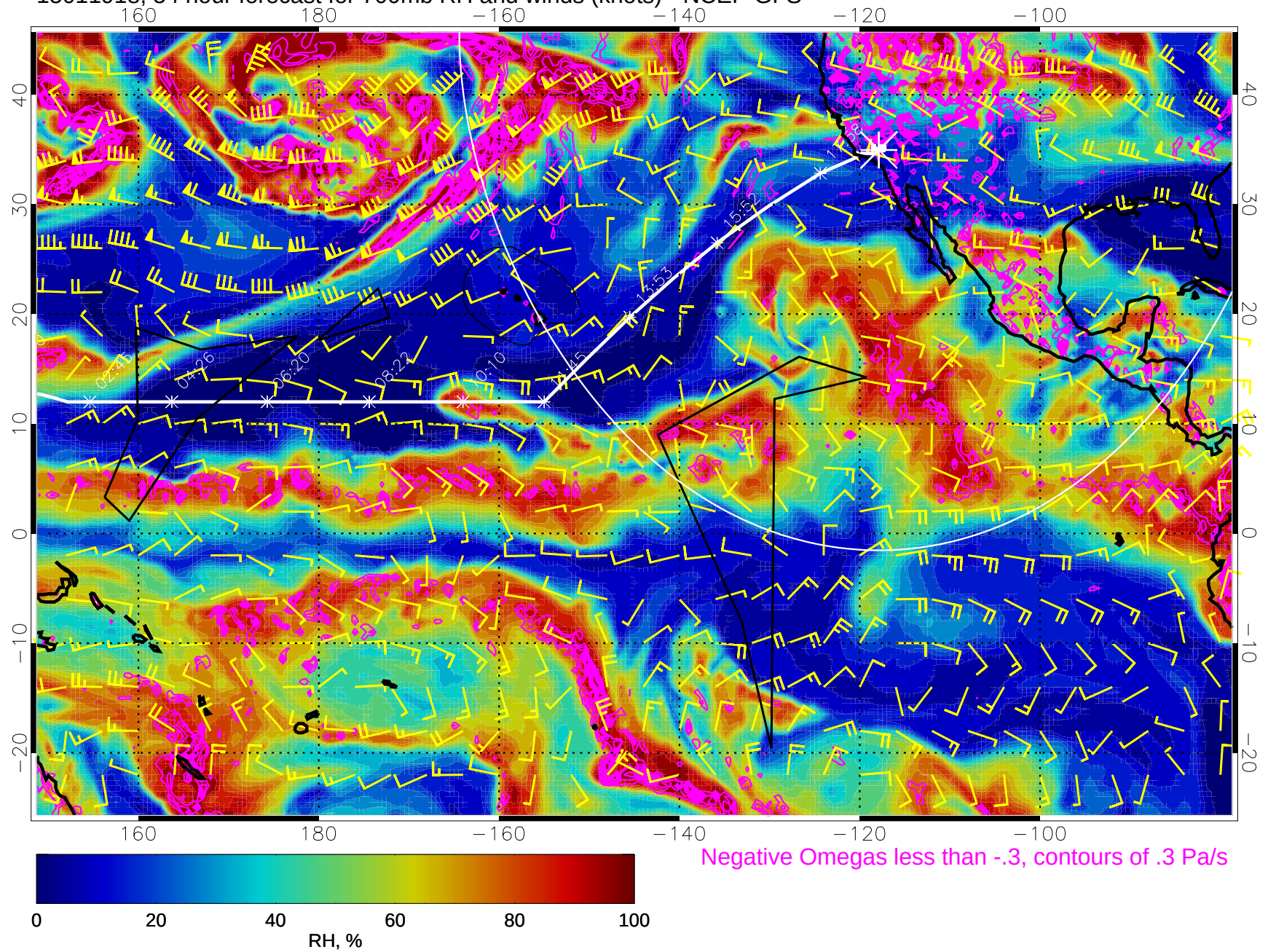
15011918, 54 hour forecast for 700mb RH and winds (knots) - NCEP GFS
