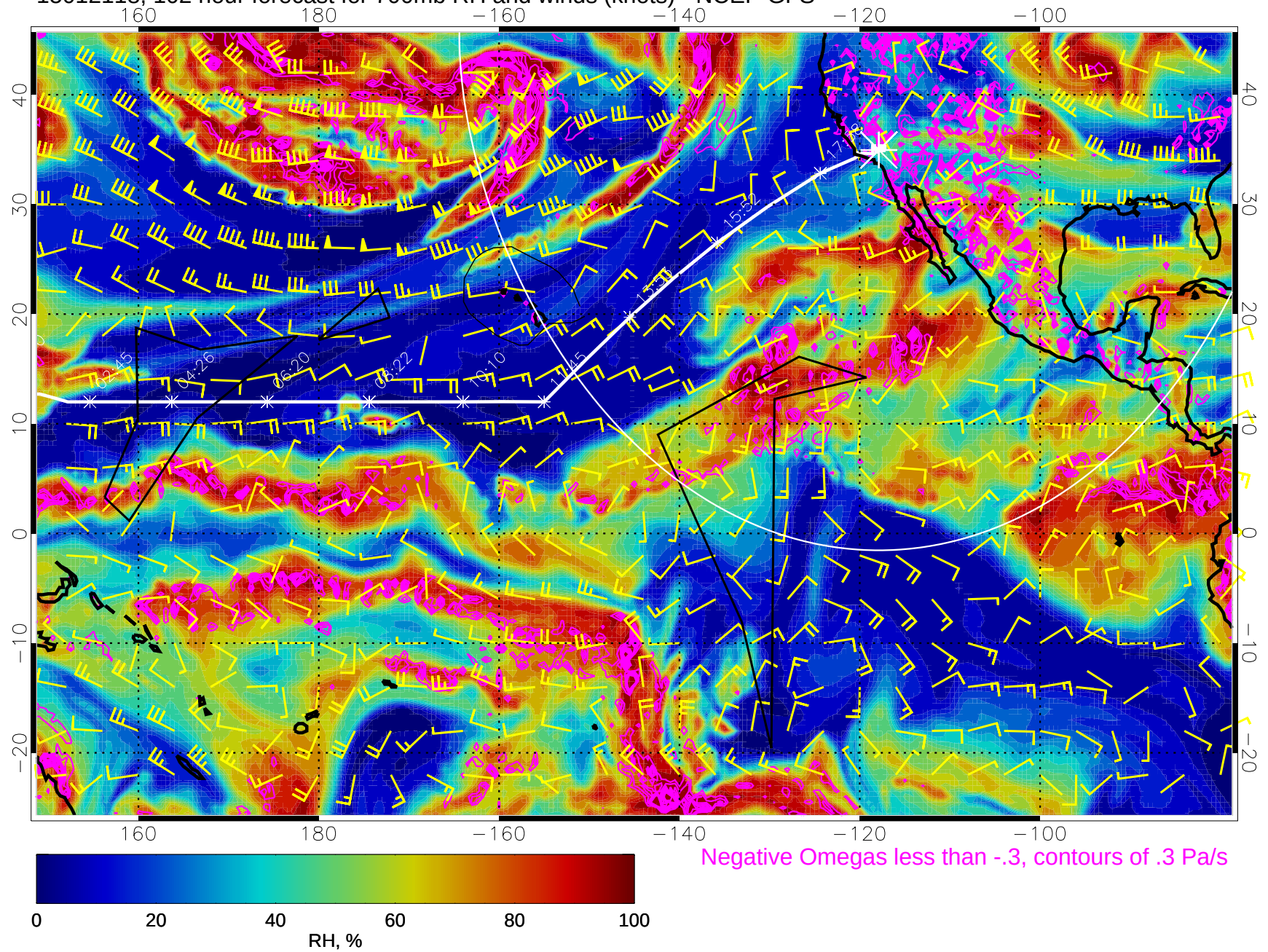
15012118, 102 hour forecast for 700mb RH and winds (knots) - NCEP GFS
