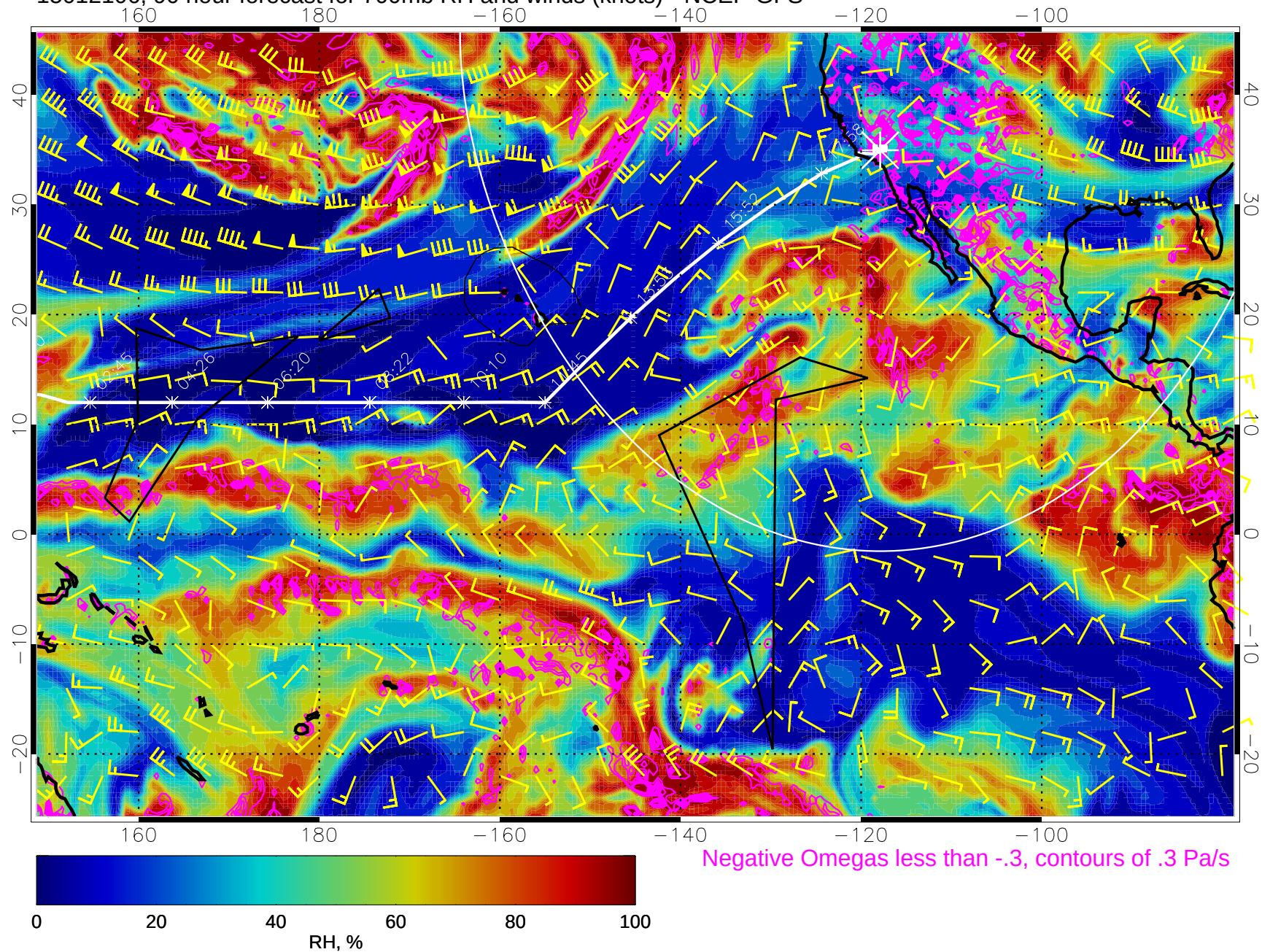
15012106, 90 hour forecast for 700mb RH and winds (knots) - NCEP GFS
