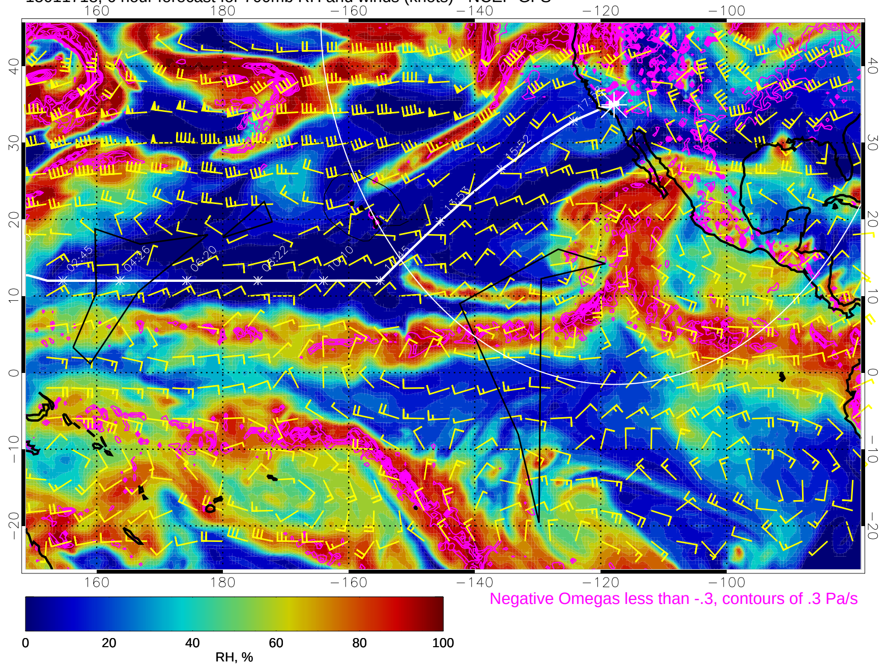
15011718, 6 hour forecast for 700mb RH and winds (knots) - NCEP GFS
