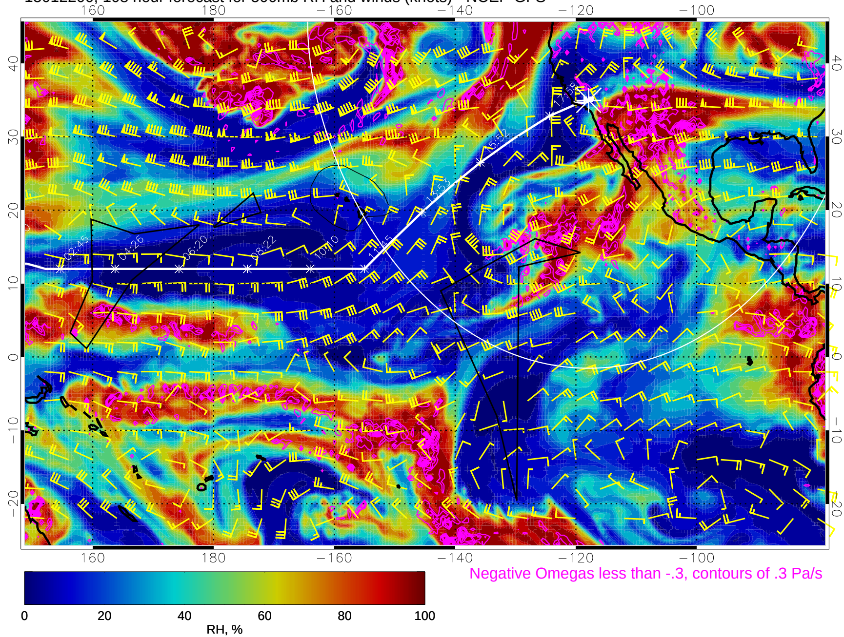
15012200, 108 hour forecast for 500mb RH and winds (knots) - NCEP GFS
