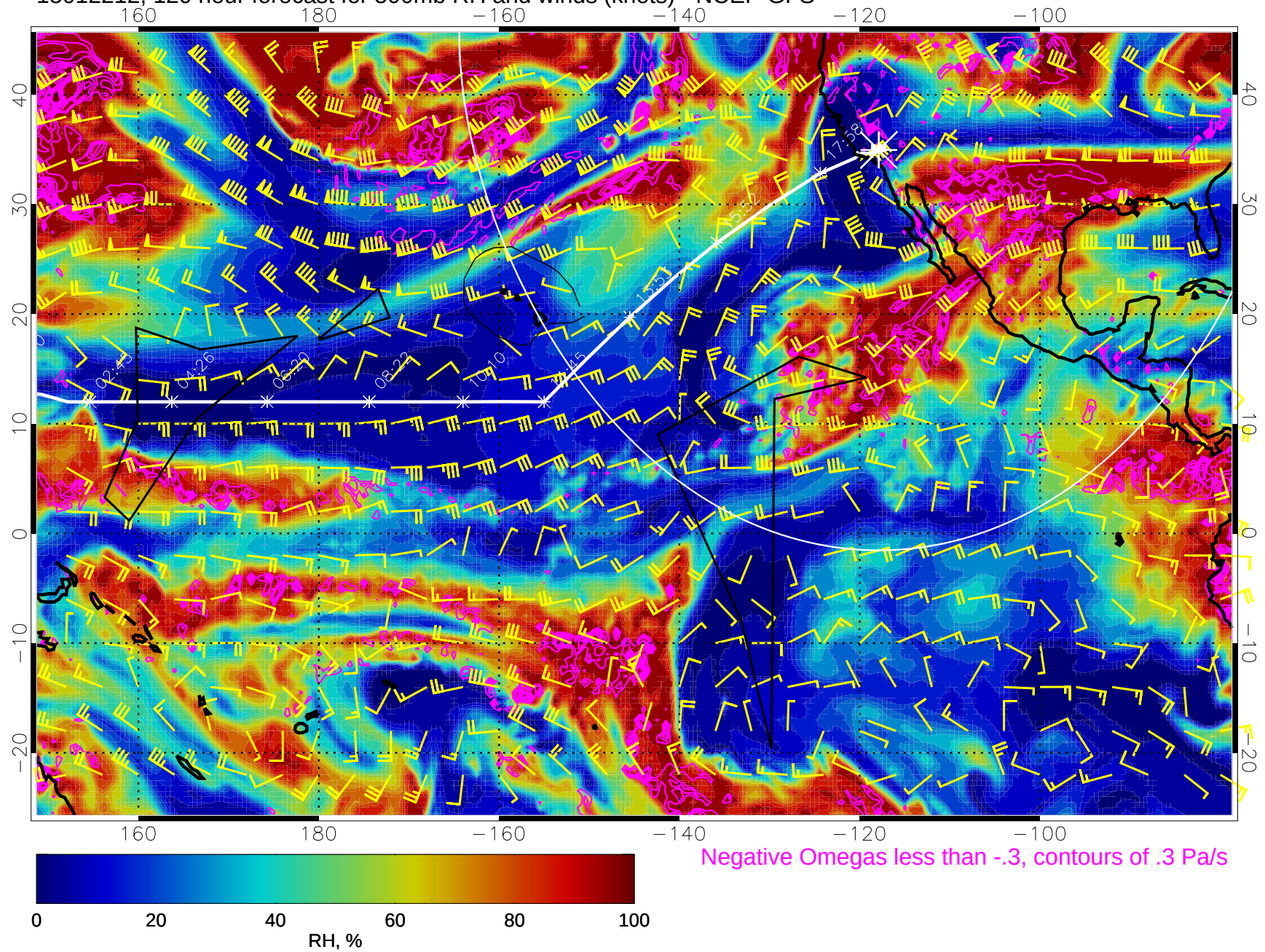
15012212, 120 hour forecast for 500mb RH and winds (knots) - NCEP GFS
