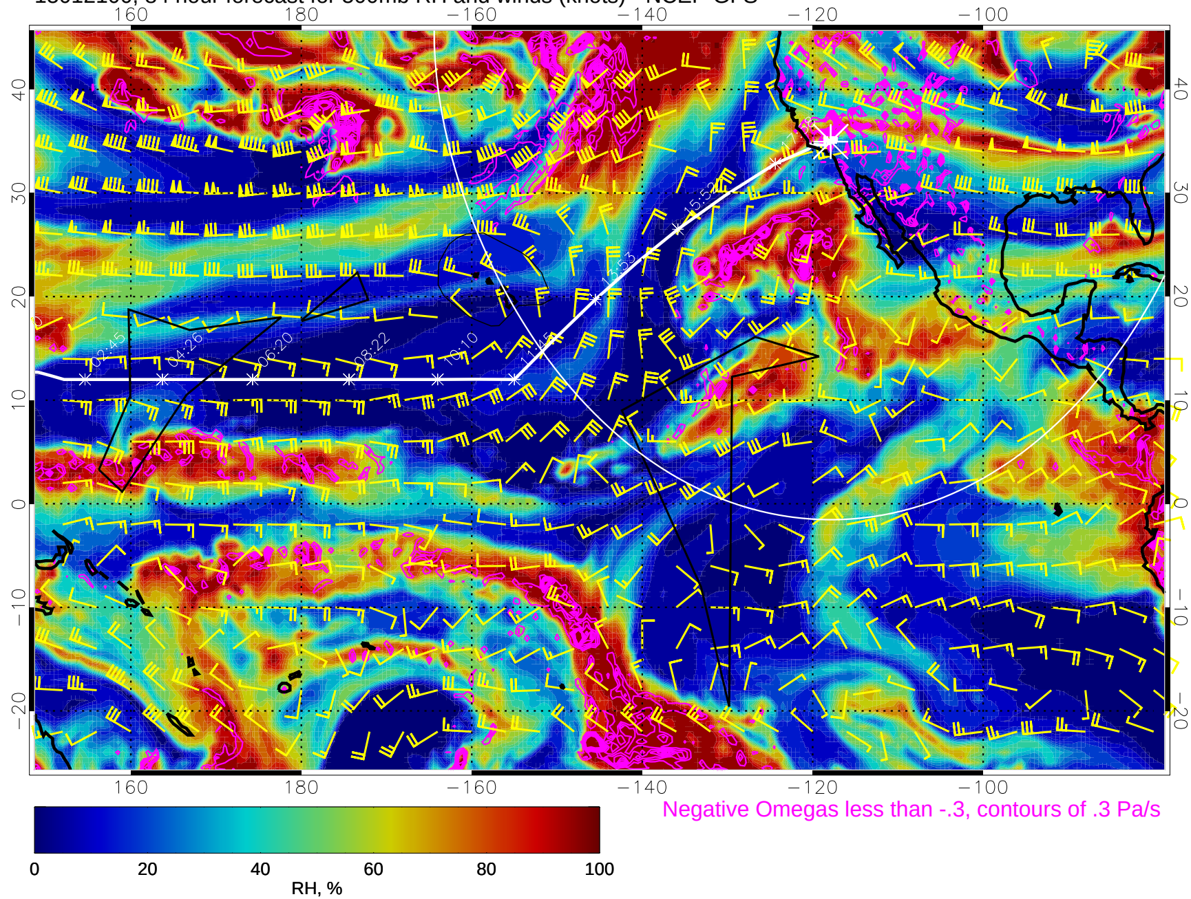
15012100, 84 hour forecast for 500mb RH and winds (knots) - NCEP GFS
