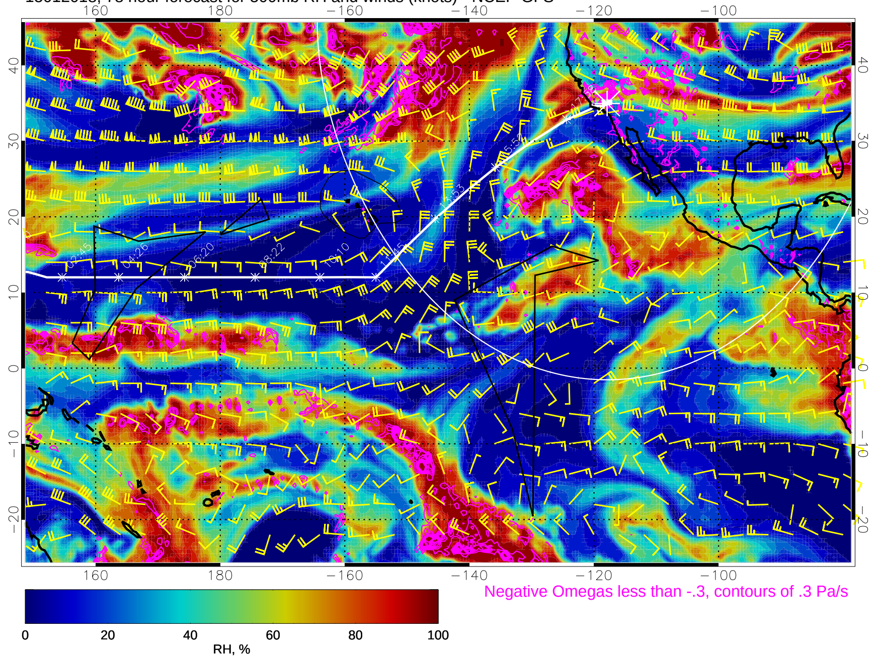
15012018, 78 hour forecast for 500mb RH and winds (knots) - NCEP GFS
