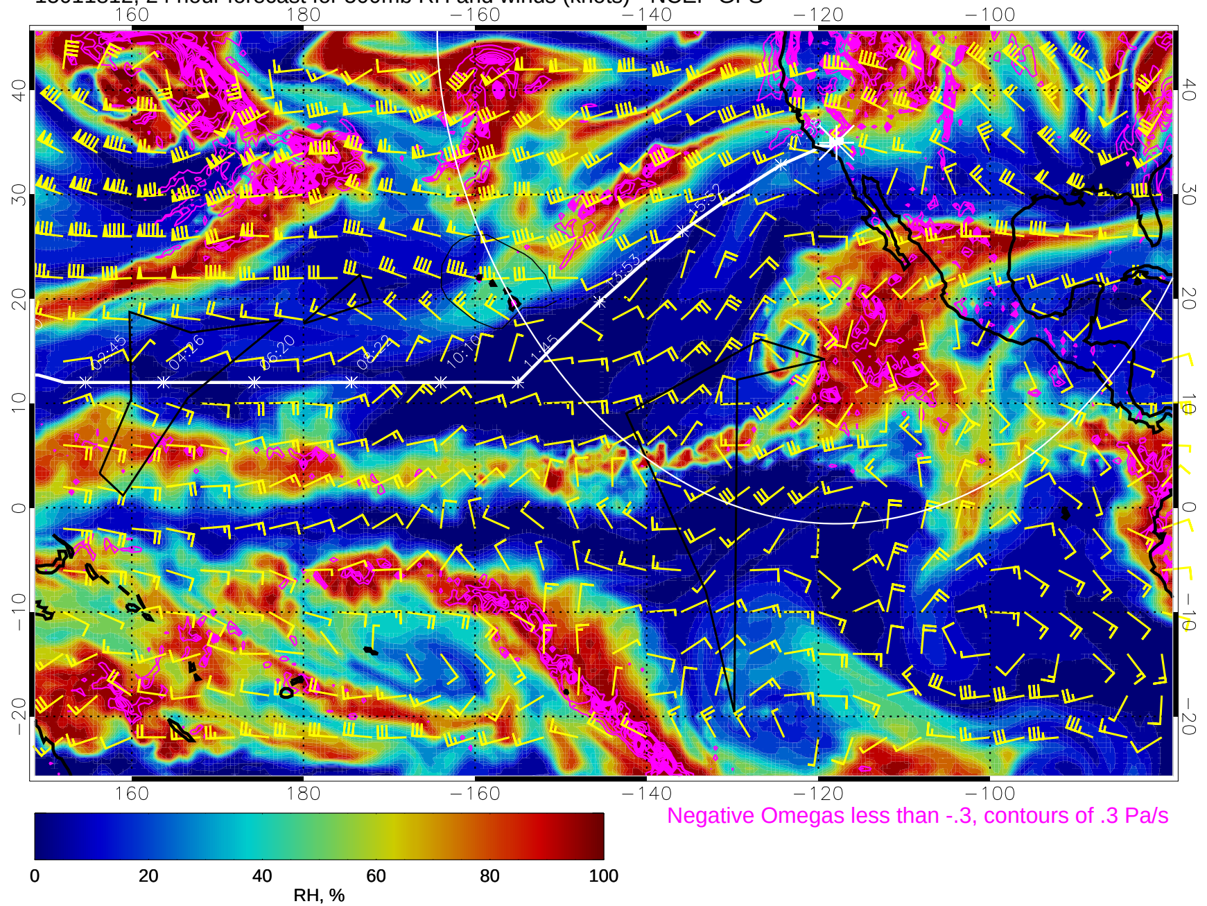
15011812, 24 hour forecast for 500mb RH and winds (knots) - NCEP GFS
