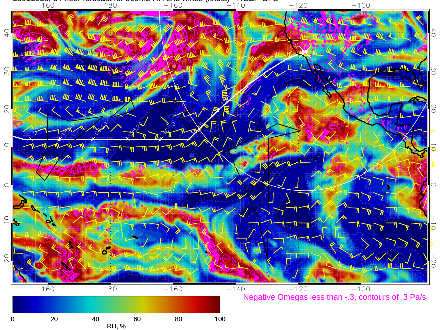
15011918, 54 hour forecast for 500mb RH and winds (knots) - NCEP GFS
