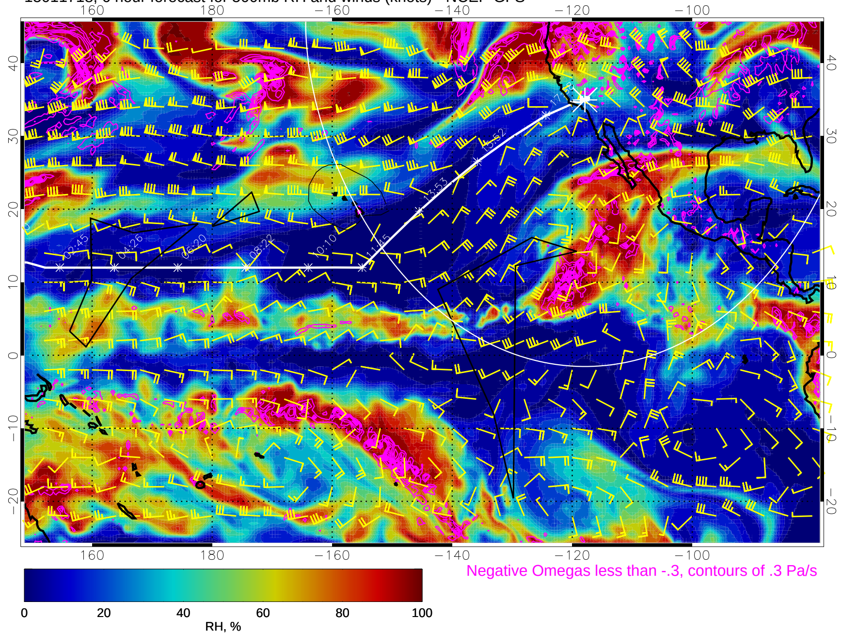
15011718, 6 hour forecast for 500mb RH and winds (knots) - NCEP GFS
