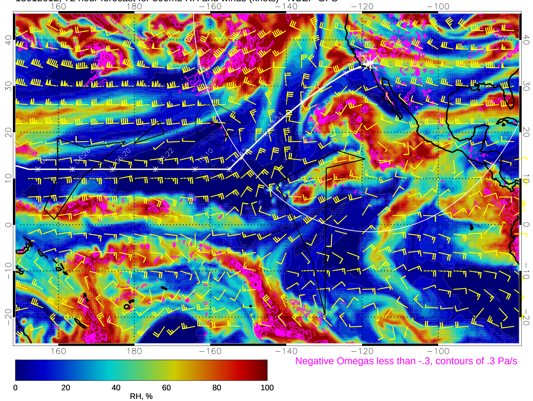
15012012, 72 hour forecast for 500mb RH and winds (knots) - NCEP GFS
