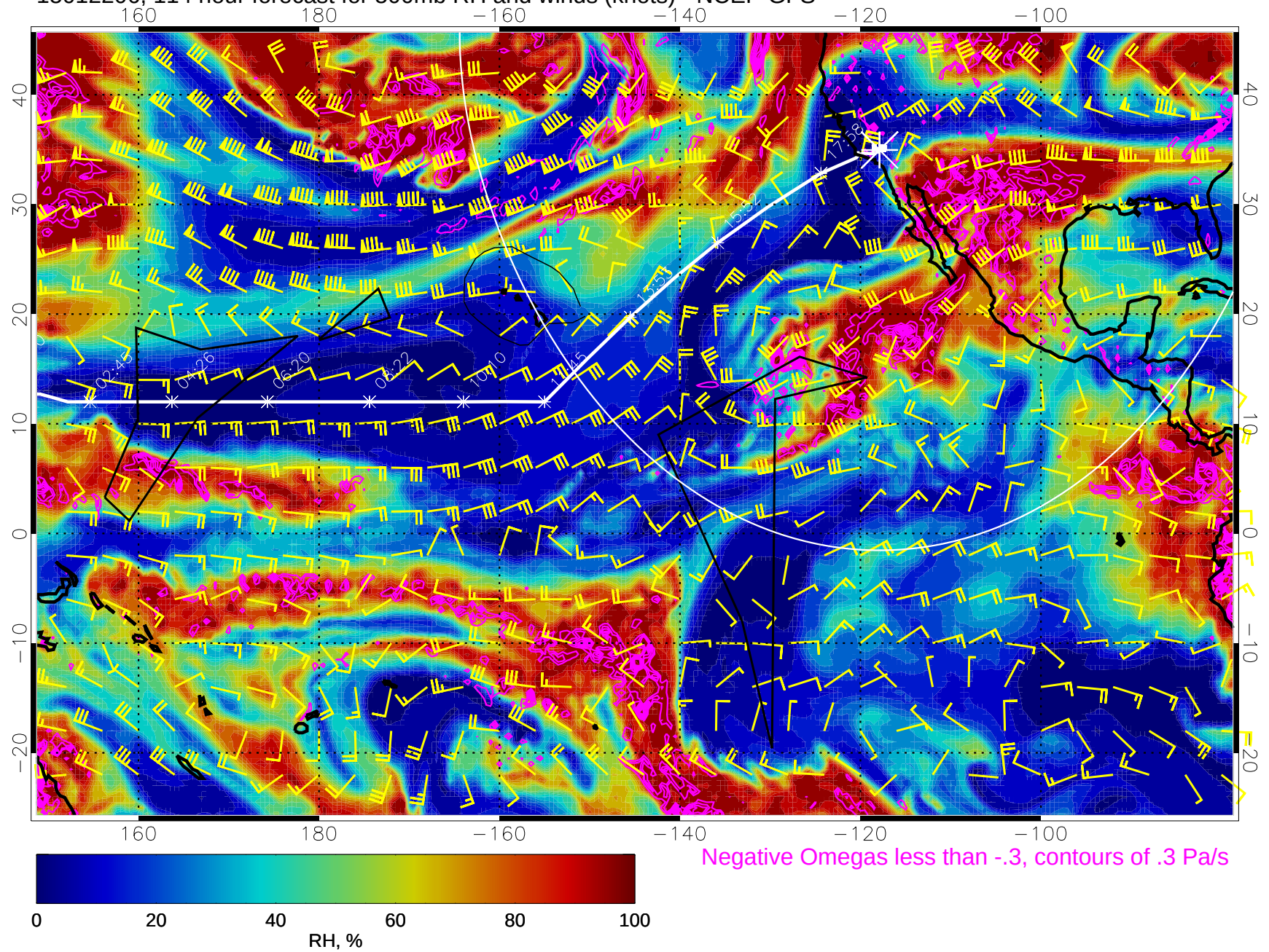
15012206, 114 hour forecast for 500mb RH and winds (knots) - NCEP GFS
