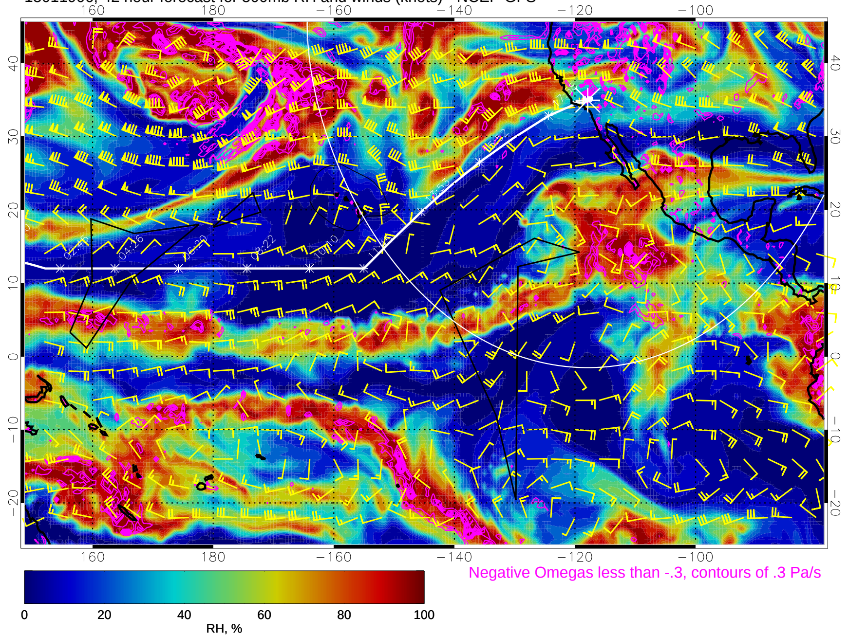
15011906, 42 hour forecast for 500mb RH and winds (knots) - NCEP GFS
