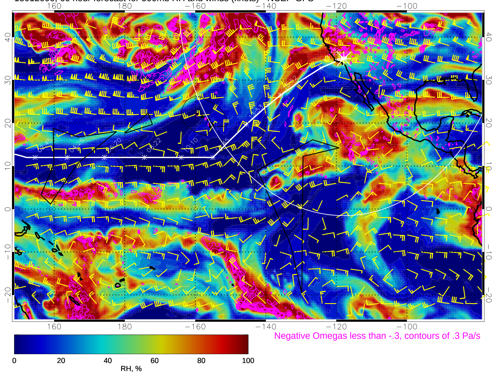
15012000, 60 hour forecast for 500mb RH and winds (knots) - NCEP GFS
