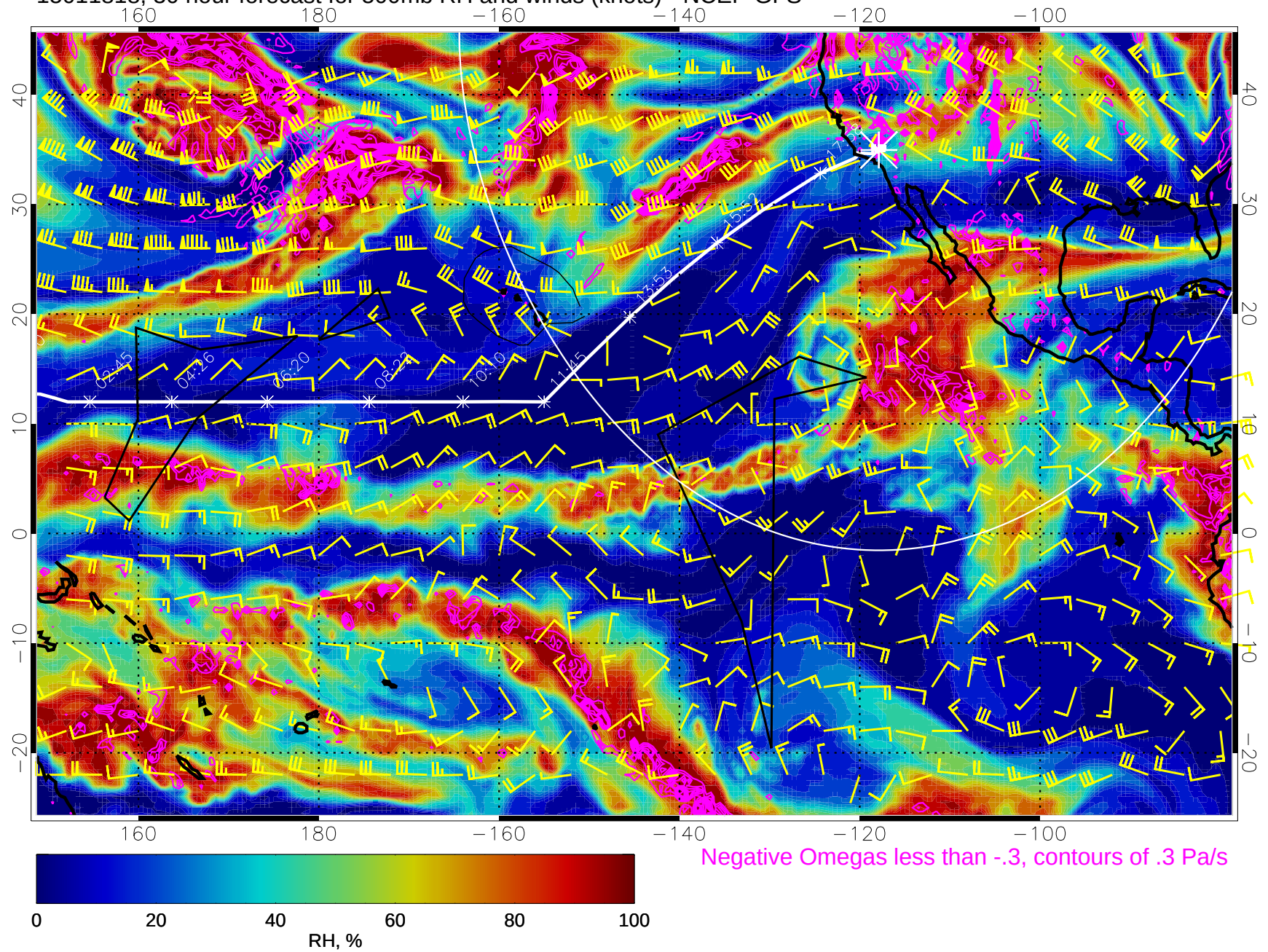
15011818, 30 hour forecast for 500mb RH and winds (knots) - NCEP GFS
