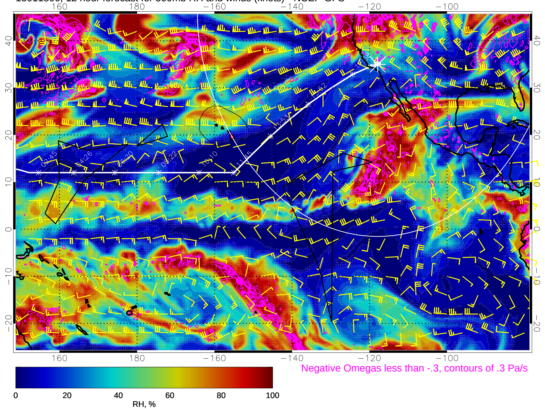
15011800, 12 hour forecast for 500mb RH and winds (knots) - NCEP GFS
