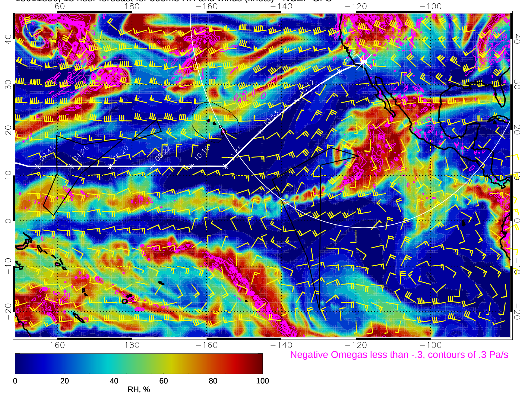
15011806, 18 hour forecast for 500mb RH and winds (knots) - NCEP GFS
