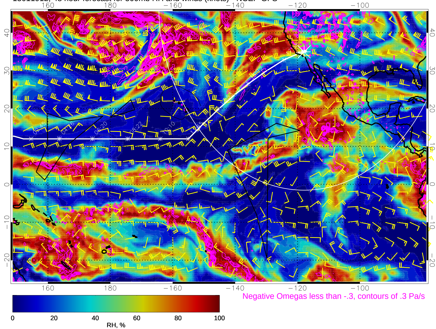
15011912, 48 hour forecast for 500mb RH and winds (knots) - NCEP GFS
