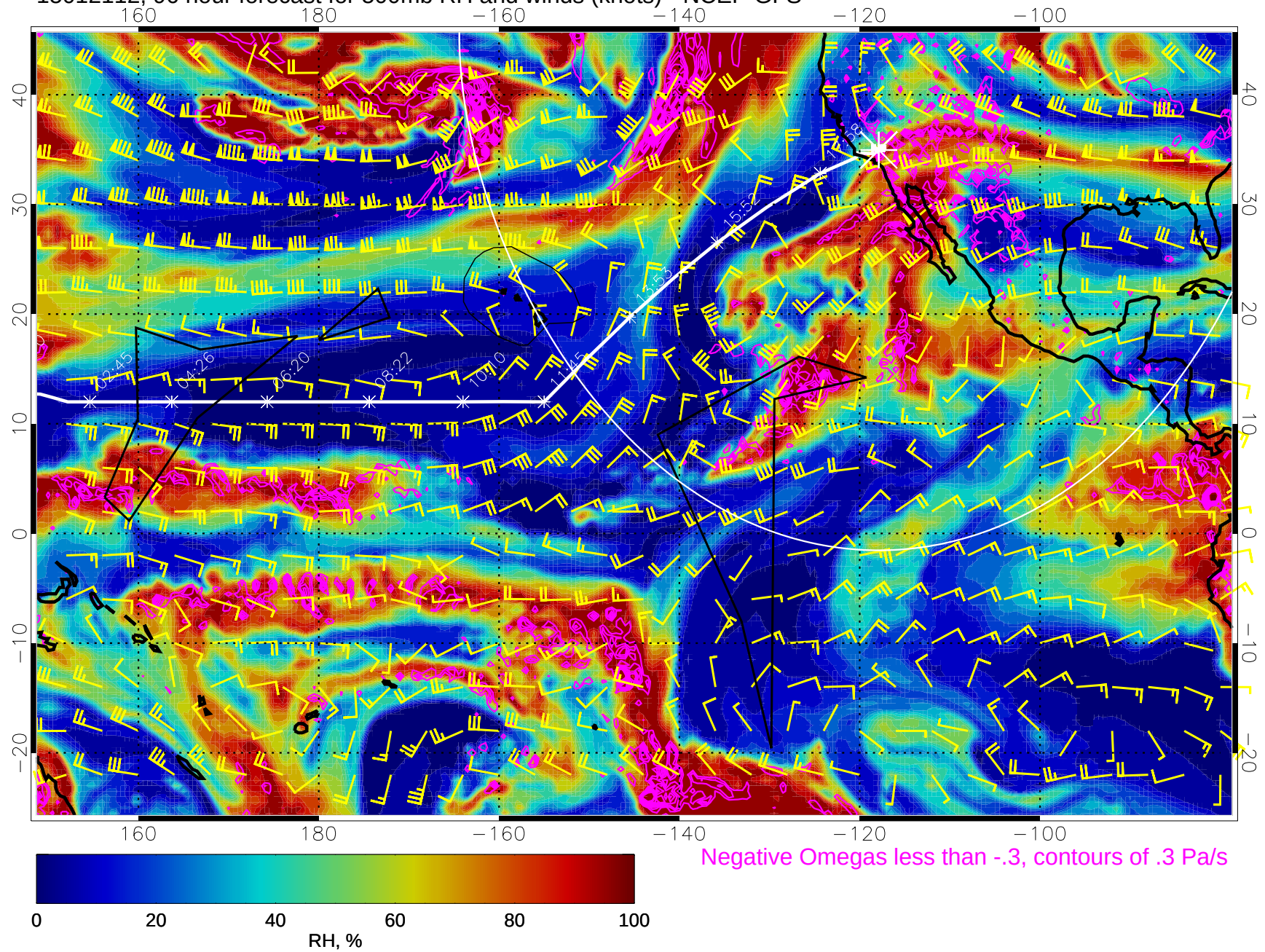
15012112, 96 hour forecast for 500mb RH and winds (knots) - NCEP GFS
