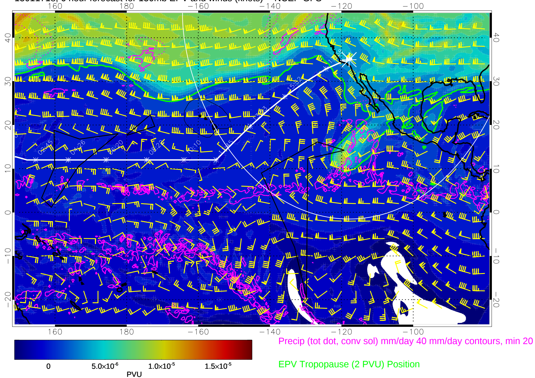
15011718, 6 hour forecast for 150mb EPV and winds (knots) -- NCEP GFS
