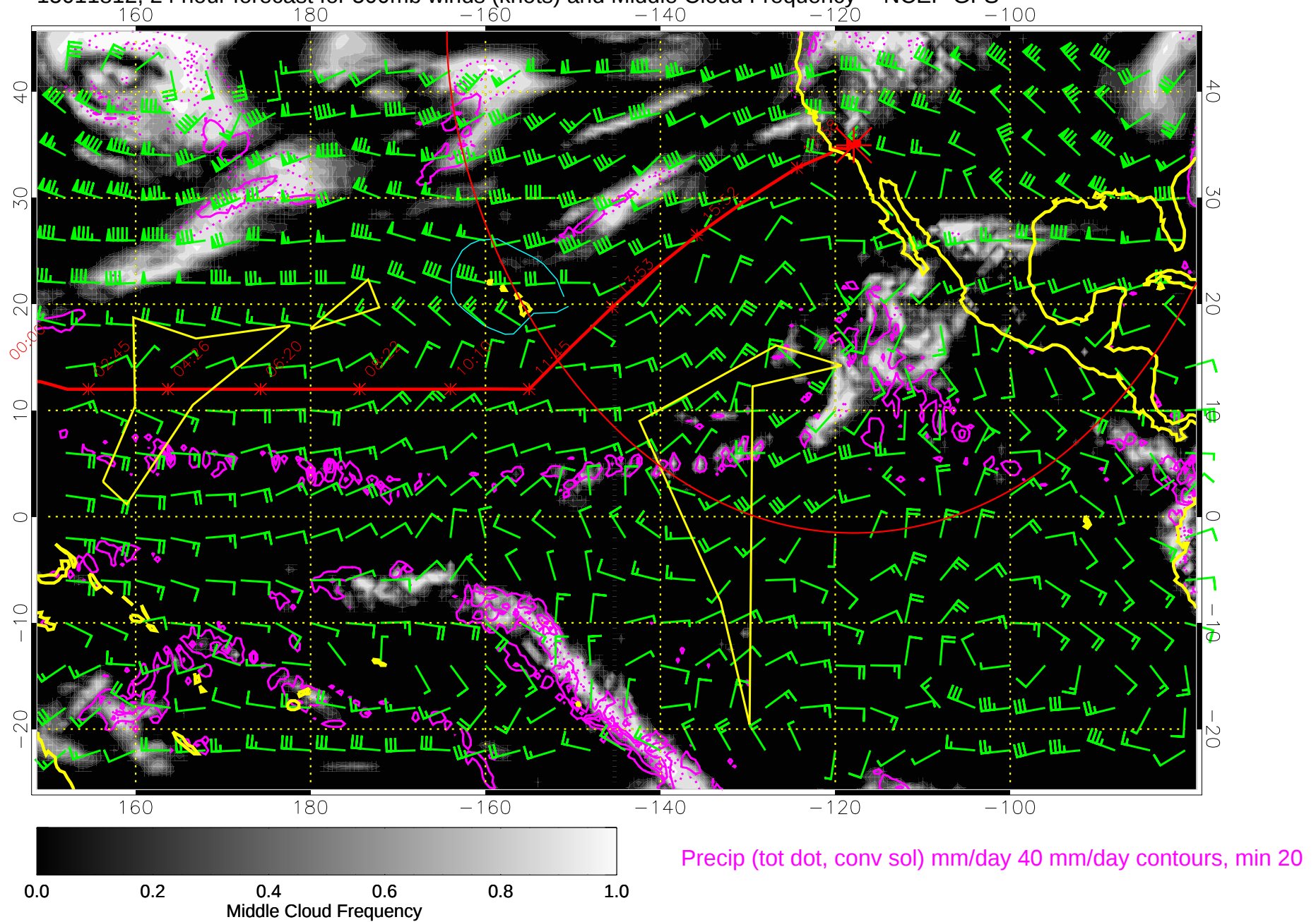
15011812, 24 hour forecast for 500mb winds (knots) and Middle Cloud Frequency -- NCEP GFS
