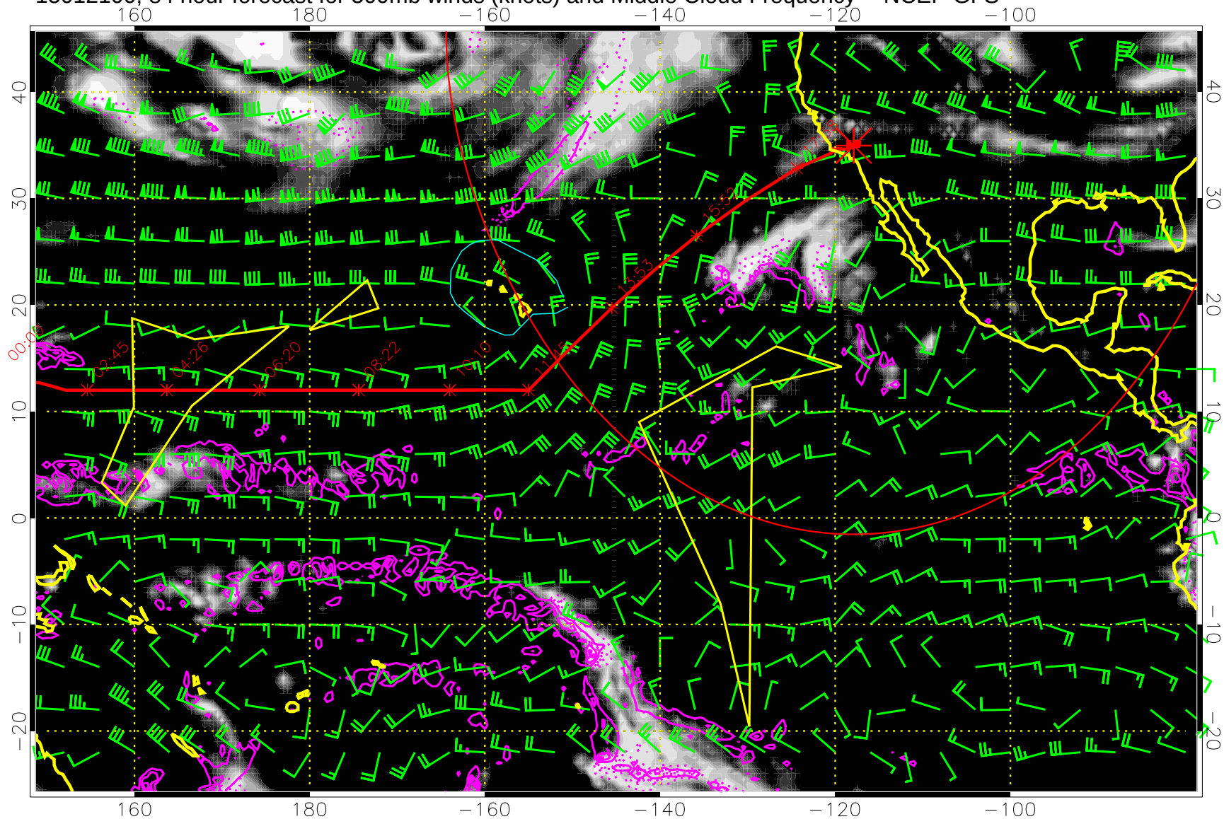
15012100, 84 hour forecast for 500mb winds (knots) and Middle Cloud Frequency -- NCEP GFS
