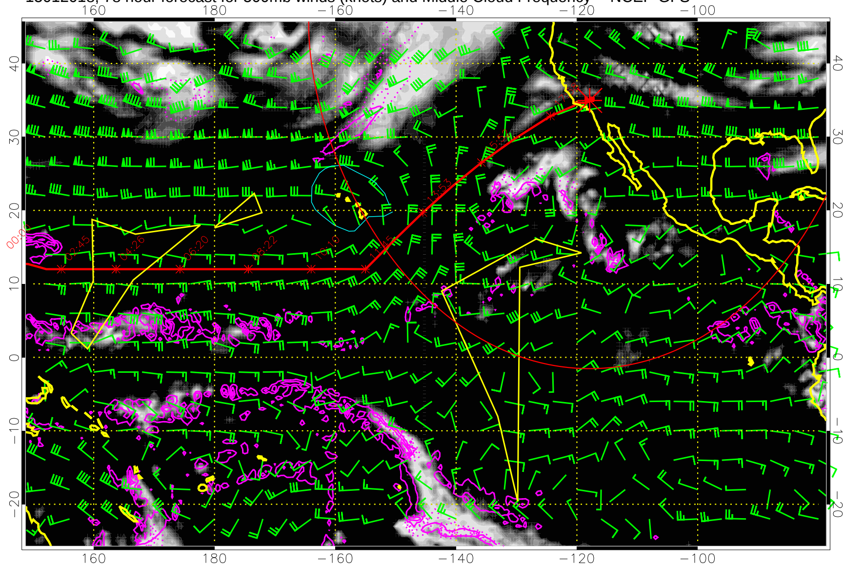
15012018, 78 hour forecast for 500mb winds (knots) and Middle Cloud Frequency -- NCEP GFS
