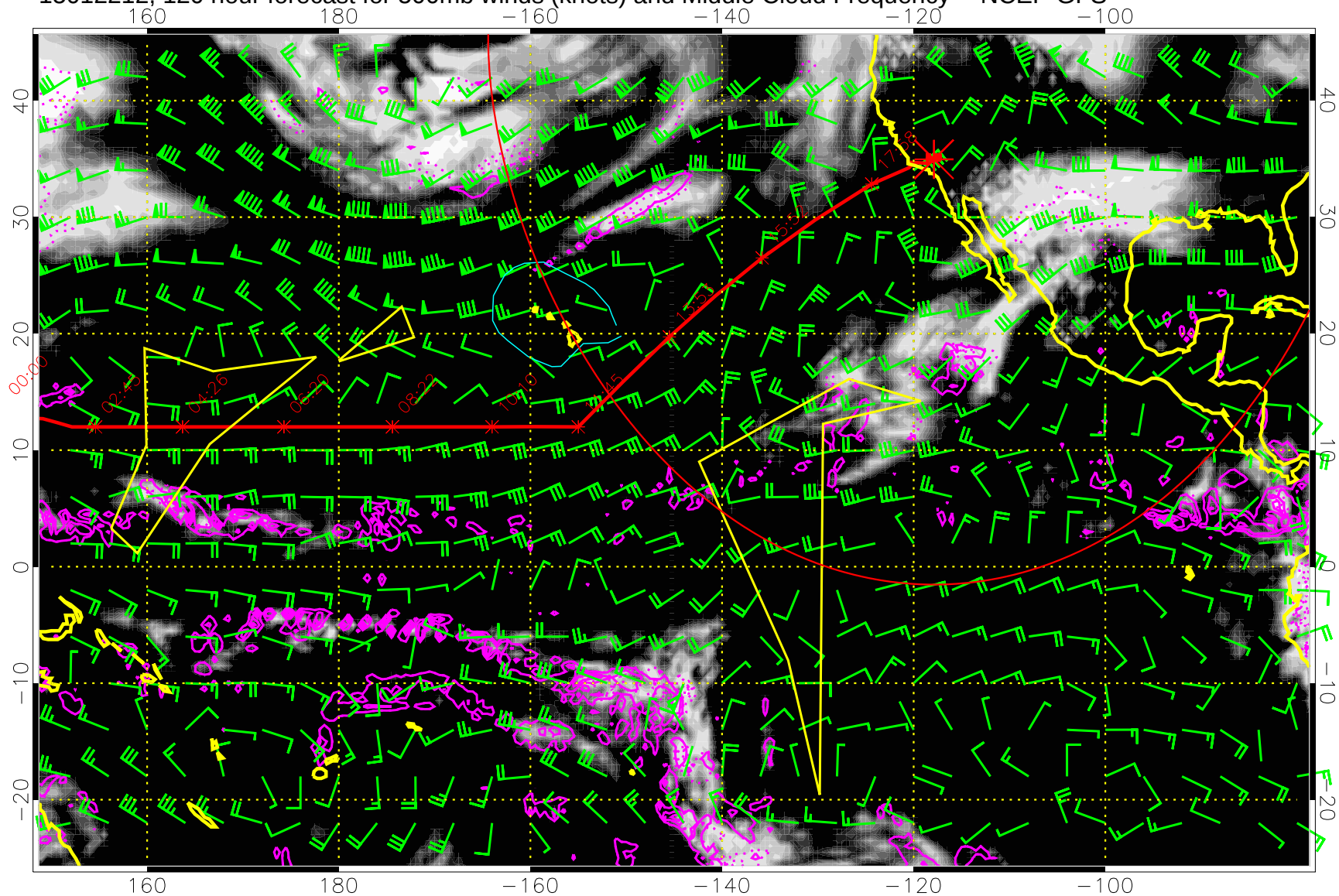
15012212, 120 hour forecast for 500mb winds (knots) and Middle Cloud Frequency -- NCEP GFS
