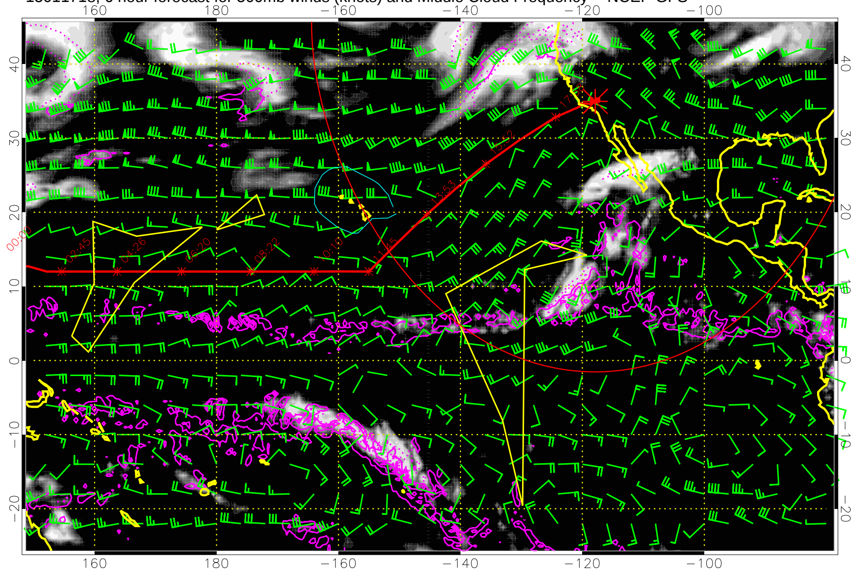
15011718, 6 hour forecast for 500mb winds (knots) and Middle Cloud Frequency -- NCEP GFS
