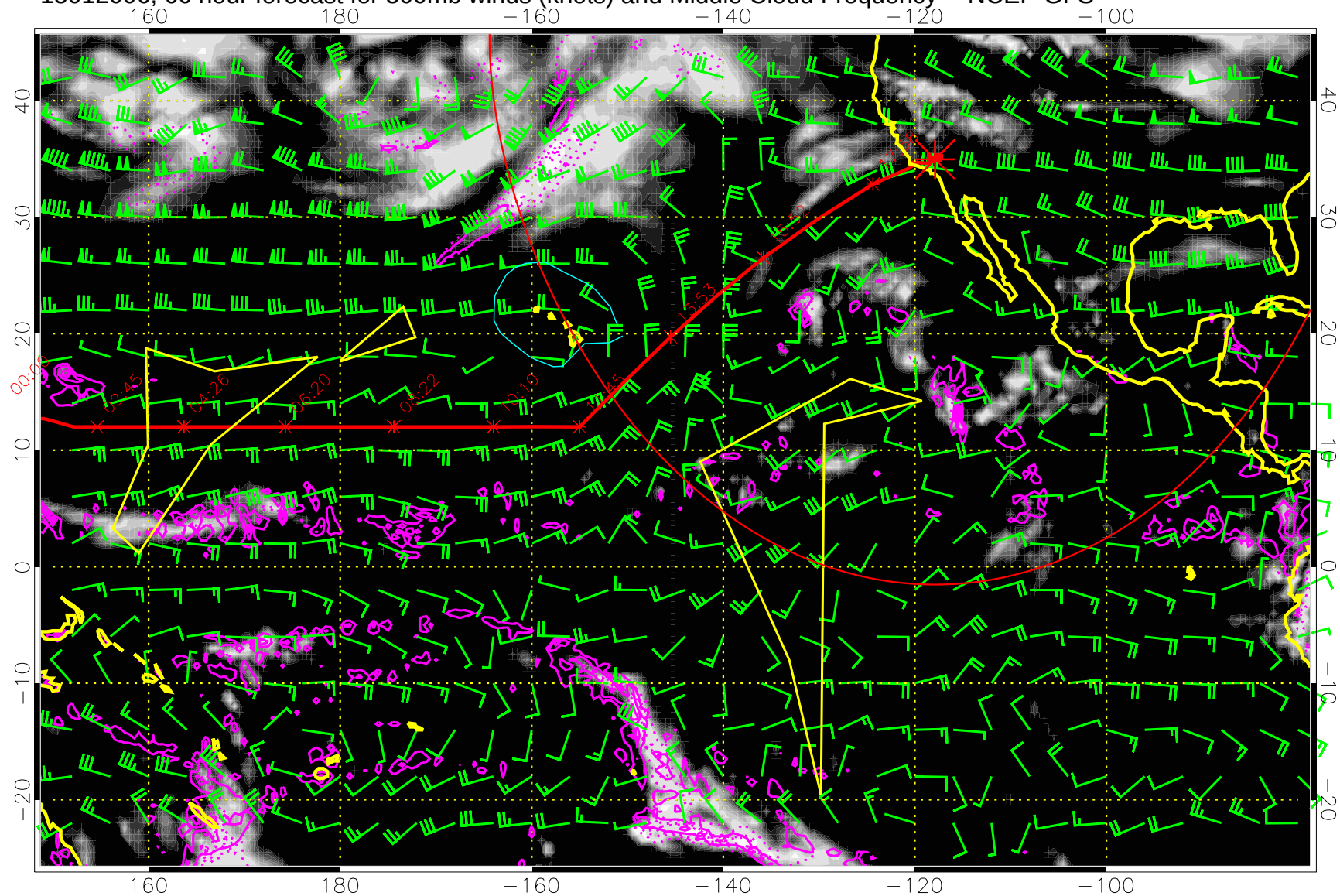
15012006, 66 hour forecast for 500mb winds (knots) and Middle Cloud Frequency -- NCEP GFS
