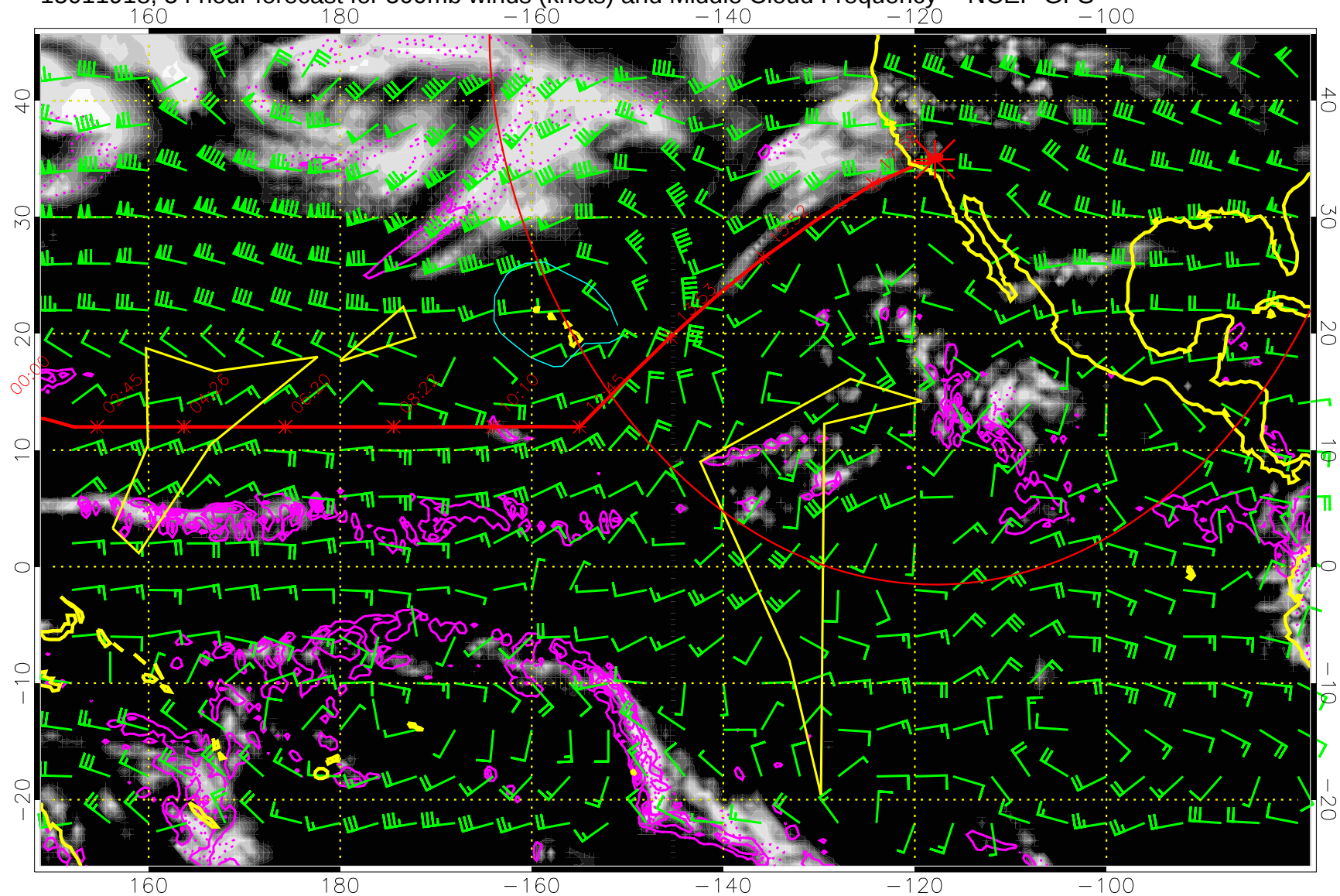
15011918, 54 hour forecast for 500mb winds (knots) and Middle Cloud Frequency -- NCEP GFS
