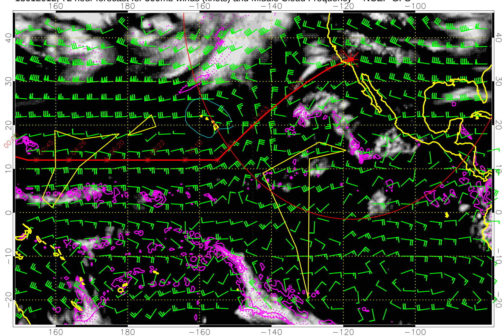
15012012, 72 hour forecast for 500mb winds (knots) and Middle Cloud Frequency -- NCEP GFS
