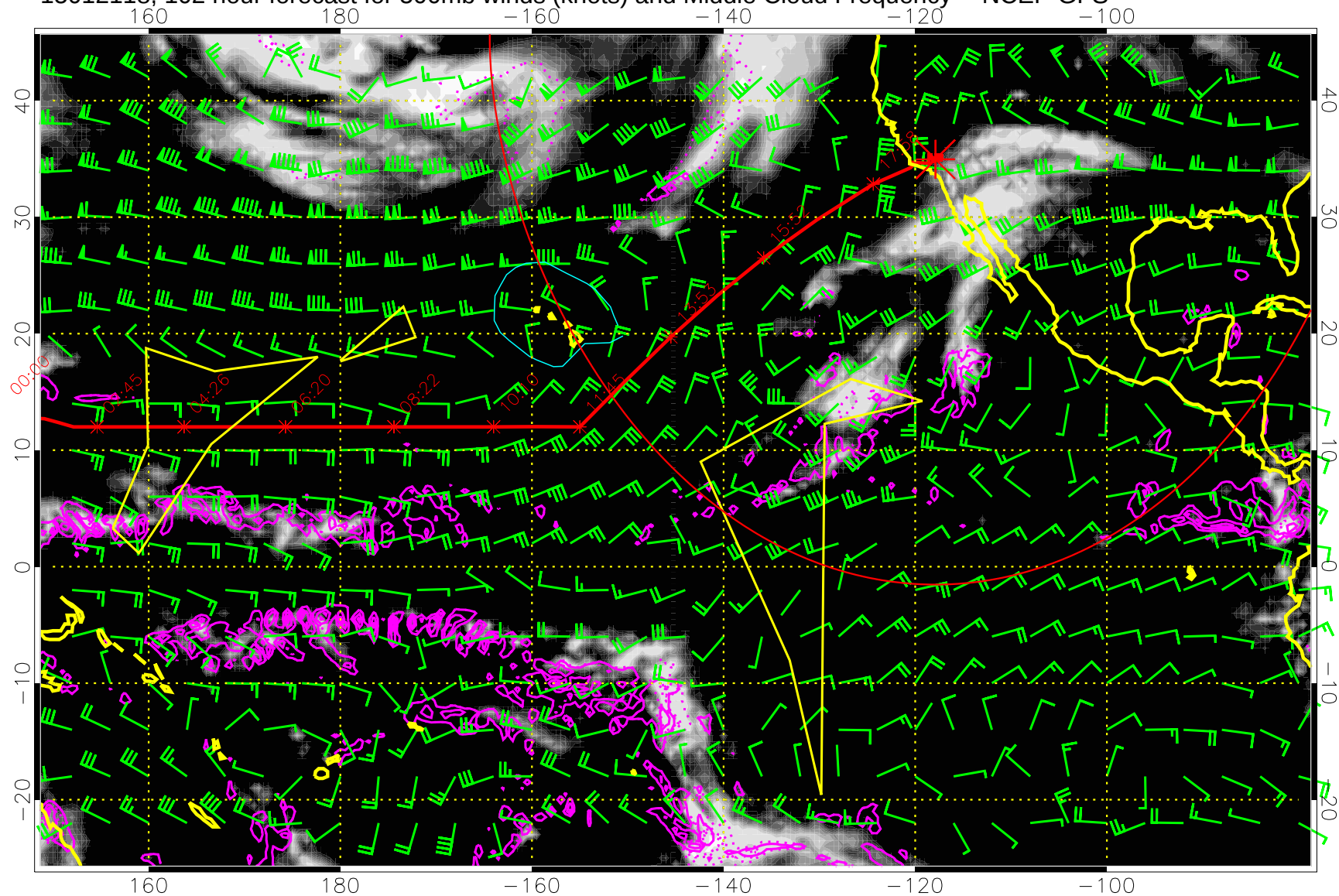
15012118, 102 hour forecast for 500mb winds (knots) and Middle Cloud Frequency -- NCEP GFS
