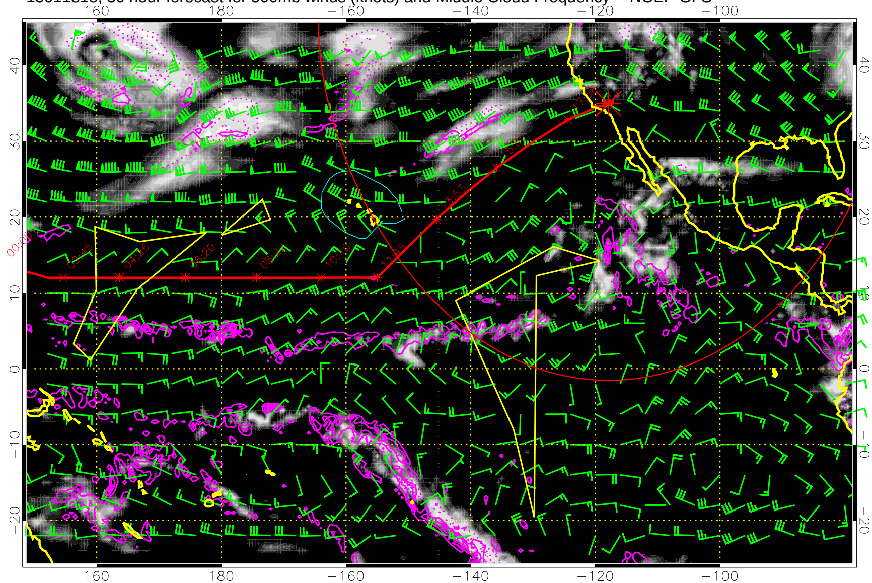
15011818, 30 hour forecast for 500mb winds (knots) and Middle Cloud Frequency -- NCEP GFS
