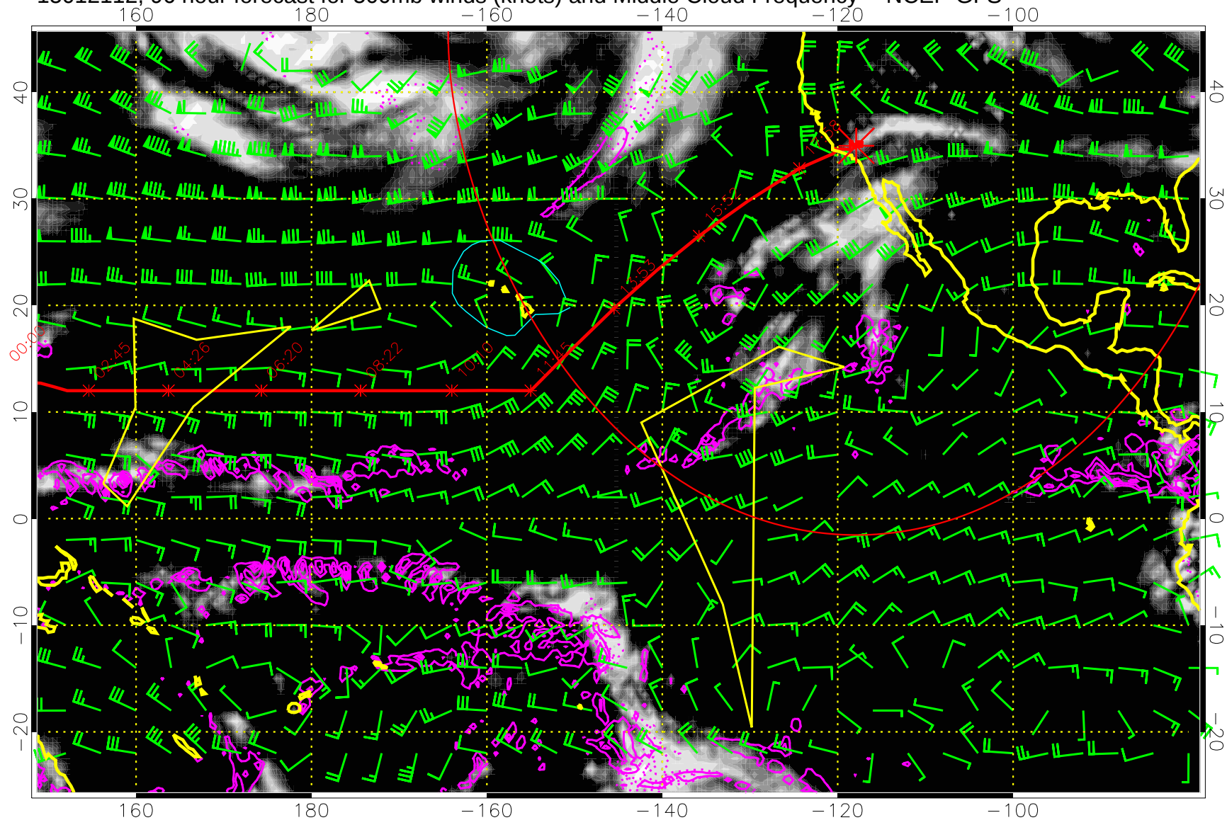
15012112, 96 hour forecast for 500mb winds (knots) and Middle Cloud Frequency -- NCEP GFS
