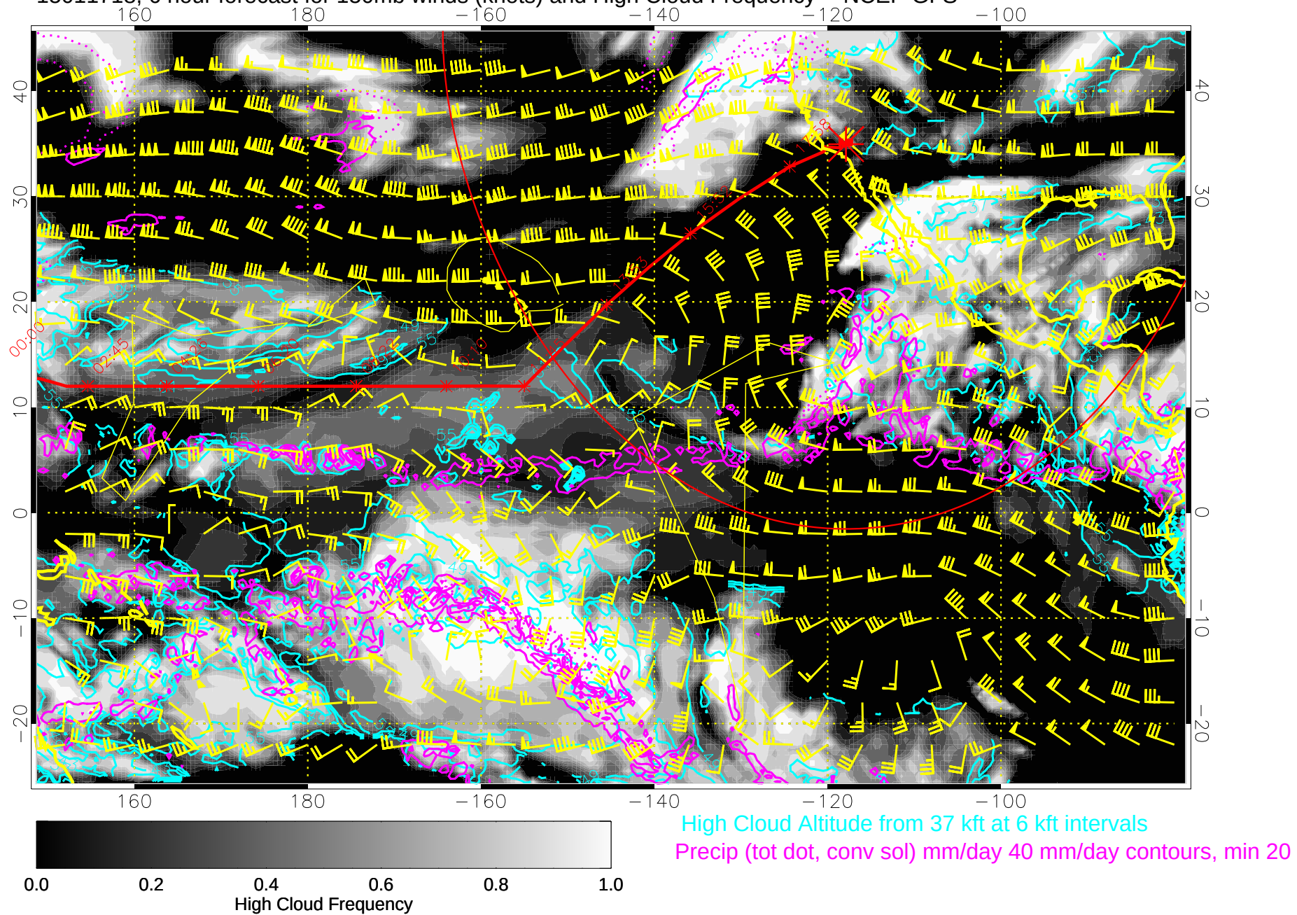
15011718, 6 hour forecast for 150mb winds (knots) and High Cloud Frequency -- NCEP GFS
