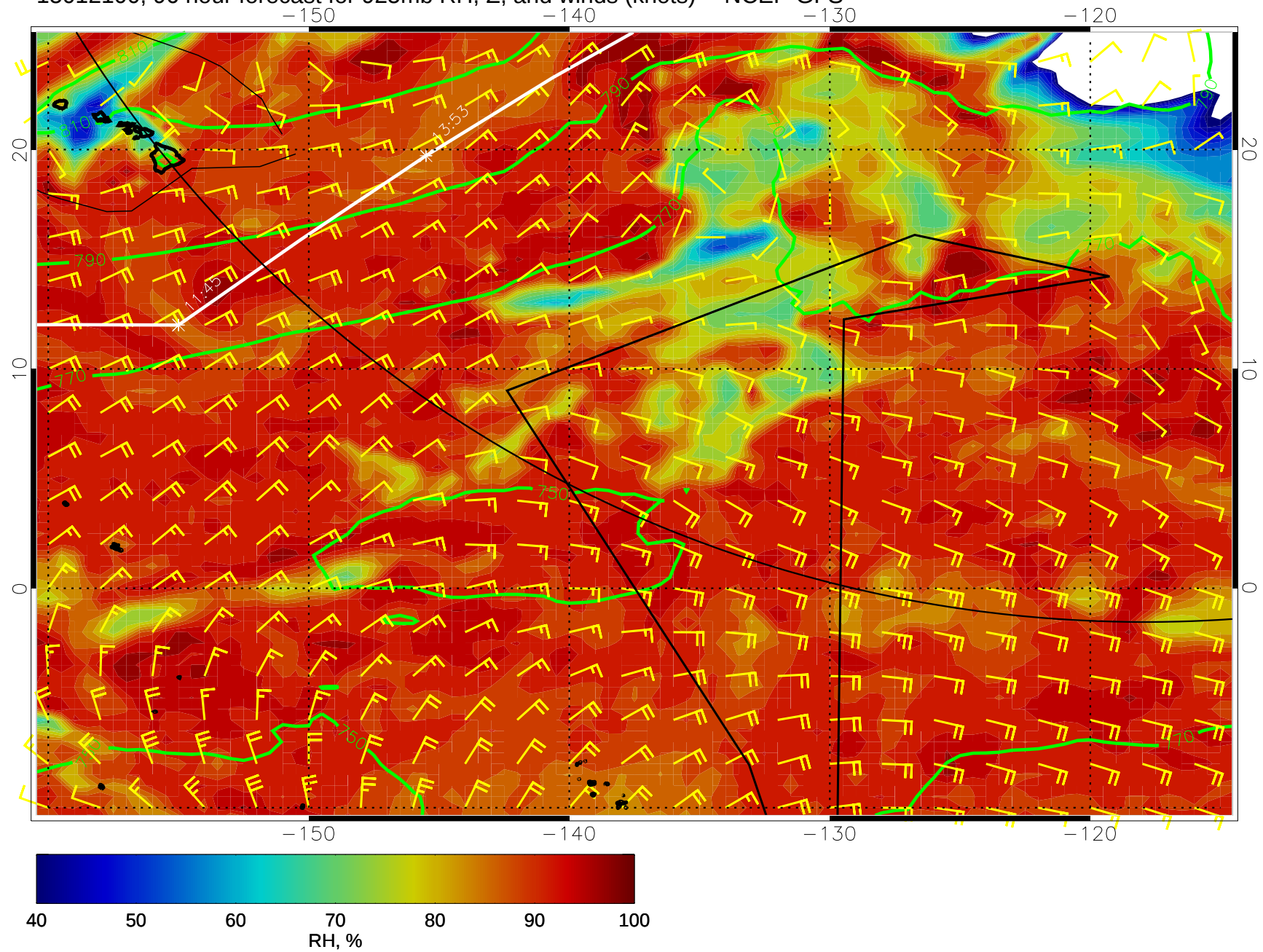
15012100, 96 hour forecast for 925mb RH, Z, and winds (knots) -- NCEP GFS
