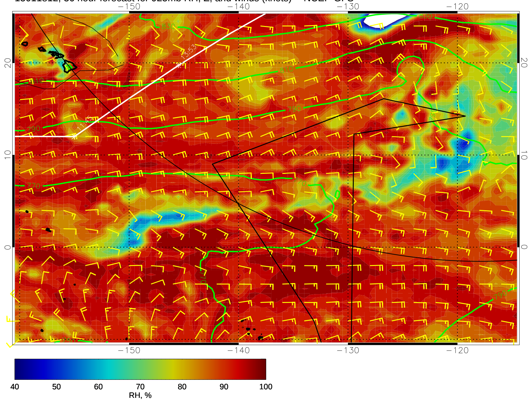
15011812, 36 hour forecast for 925mb RH, Z, and winds (knots) -- NCEP GFS
