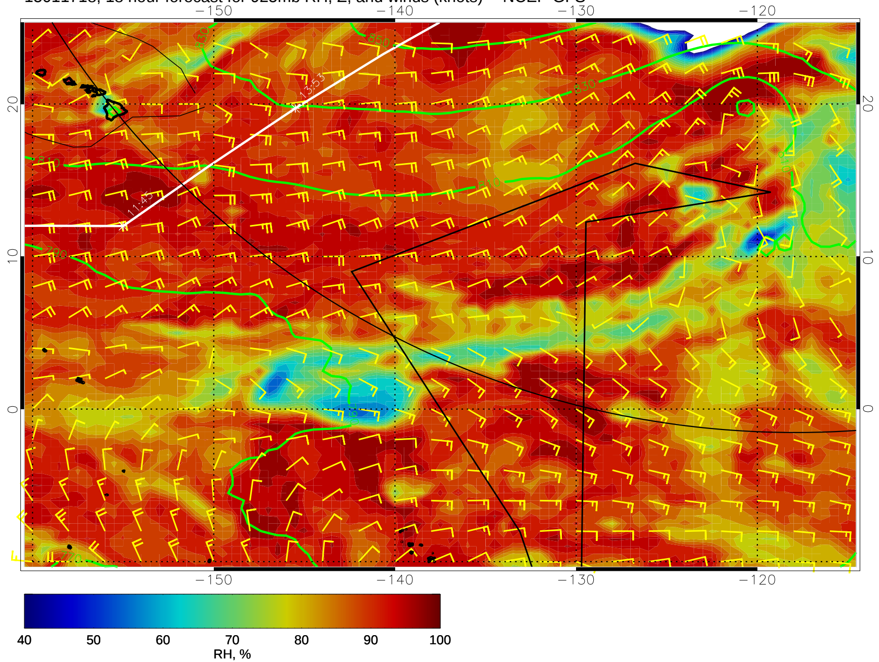
15011718, 18 hour forecast for 925mb RH, Z, and winds (knots) -- NCEP GFS
