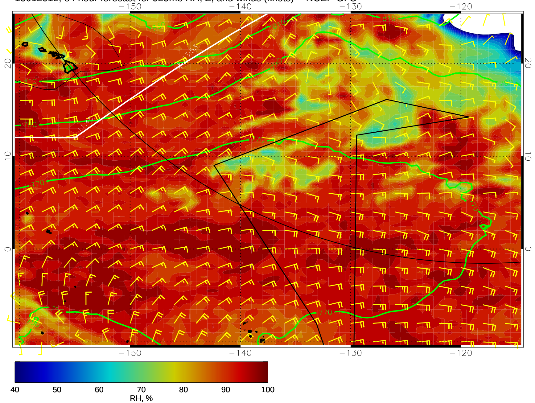
15012012, 84 hour forecast for 925mb RH, Z, and winds (knots) -- NCEP GFS
