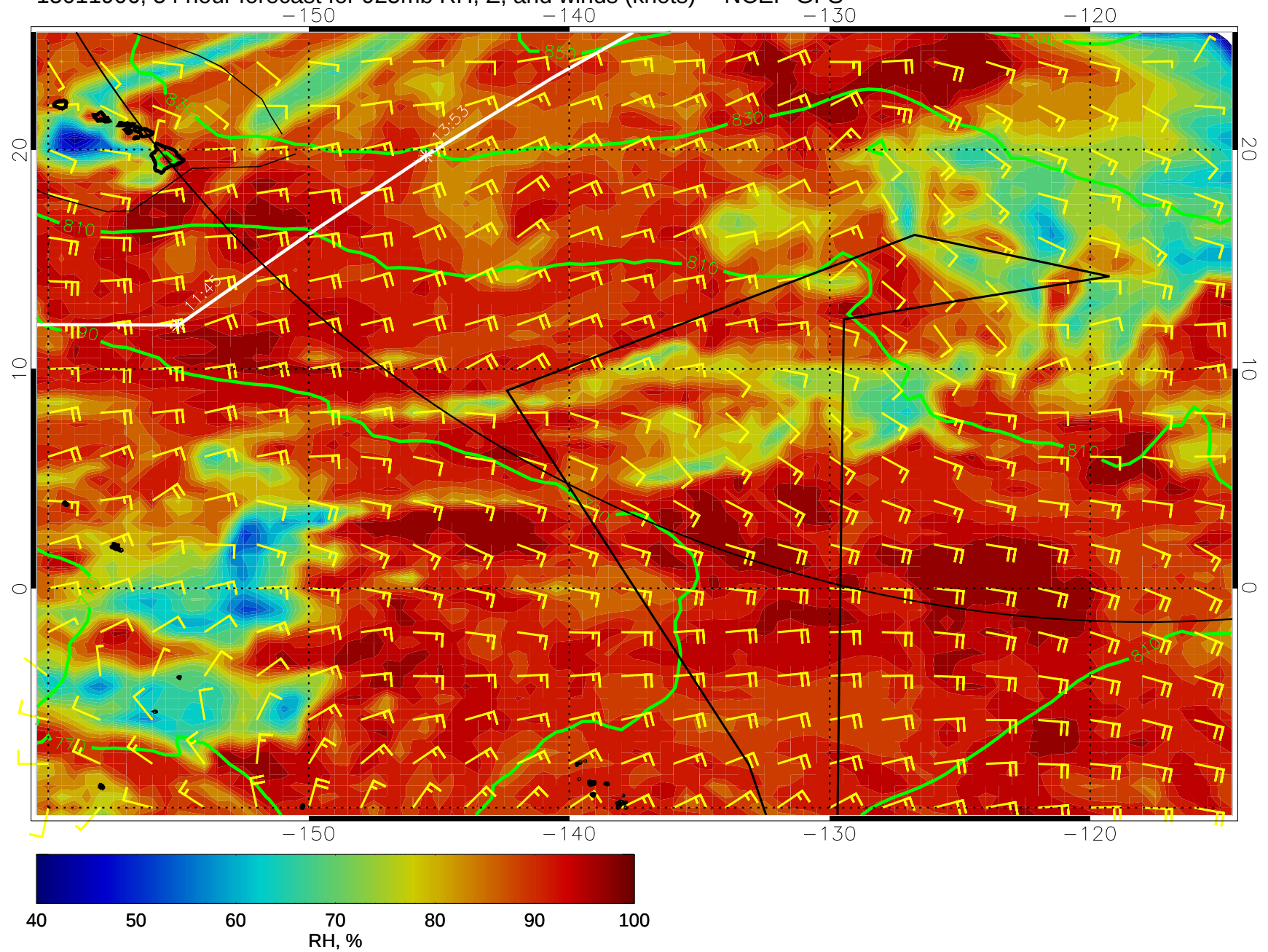
15011906, 54 hour forecast for 925mb RH, Z, and winds (knots) -- NCEP GFS
