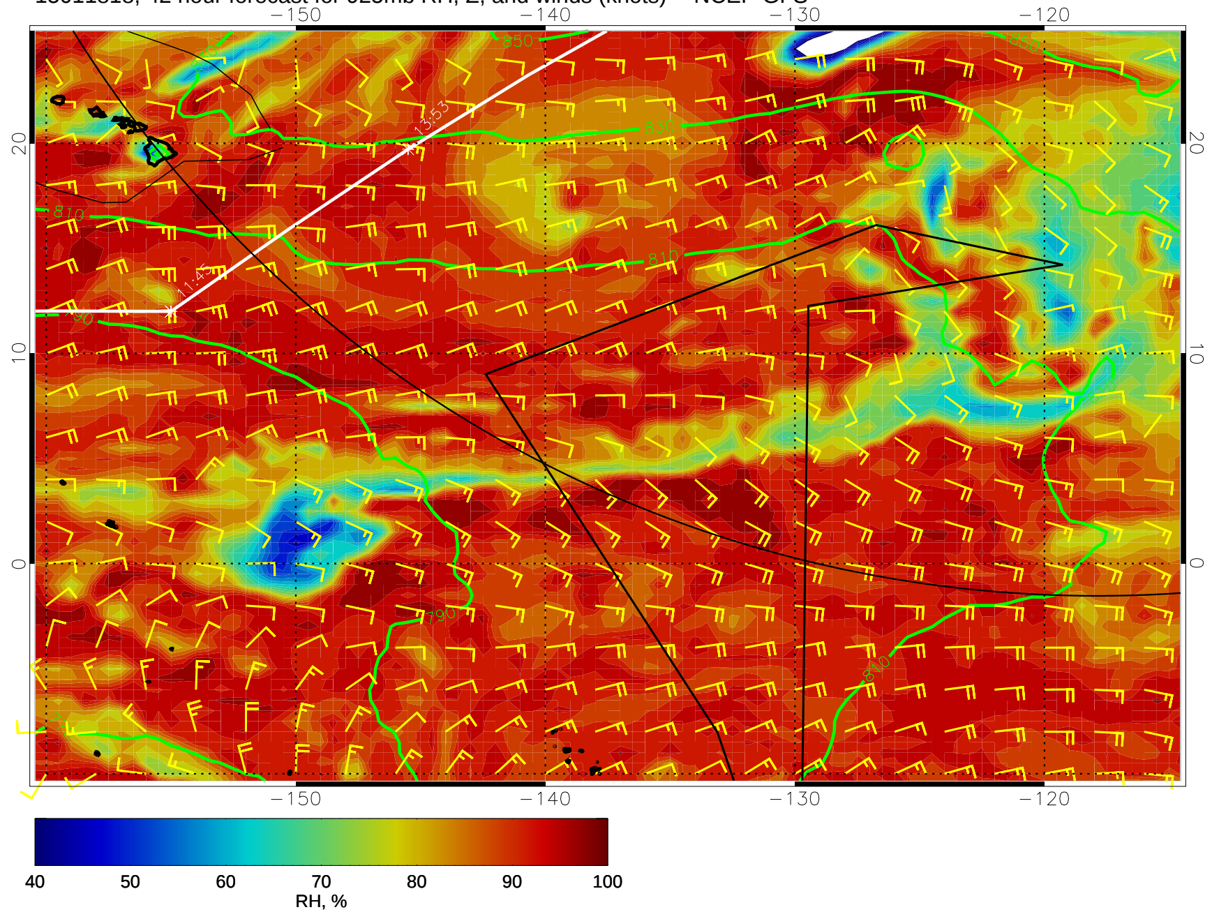
15011818, 42 hour forecast for 925mb RH, Z, and winds (knots) -- NCEP GFS
