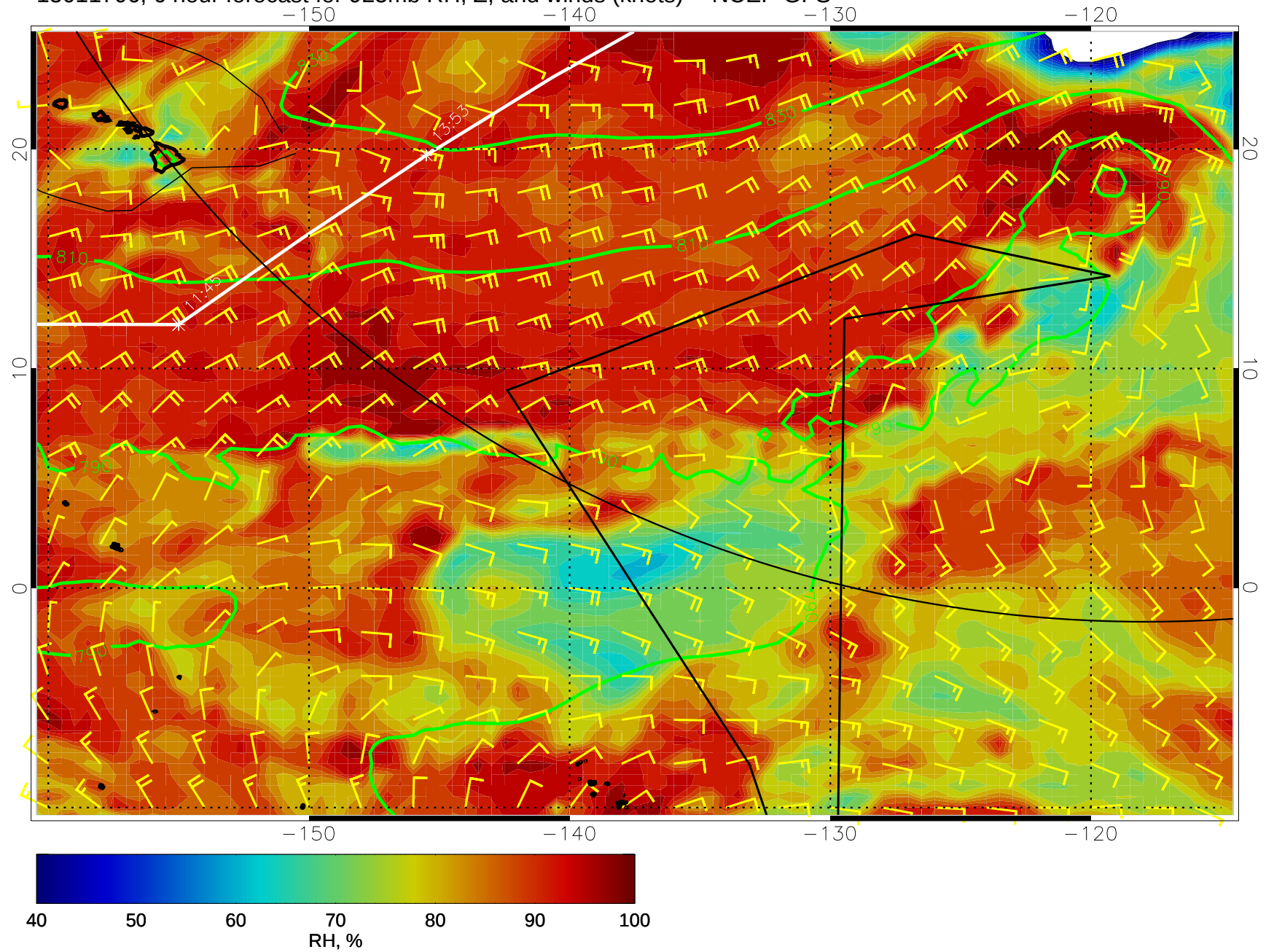
15011706, 6 hour forecast for 925mb RH, Z, and winds (knots) -- NCEP GFS
