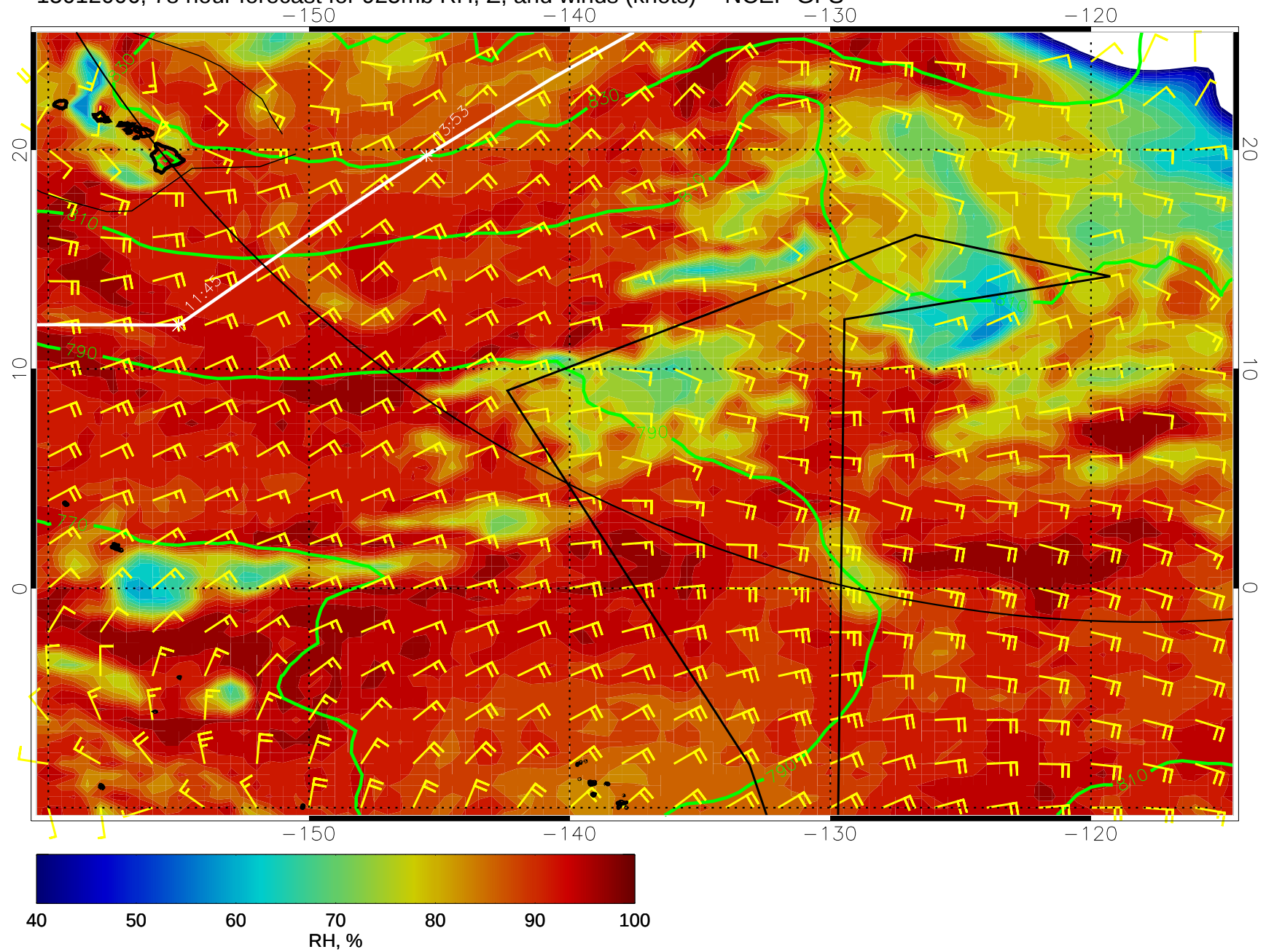
15012006, 78 hour forecast for 925mb RH, Z, and winds (knots) -- NCEP GFS
