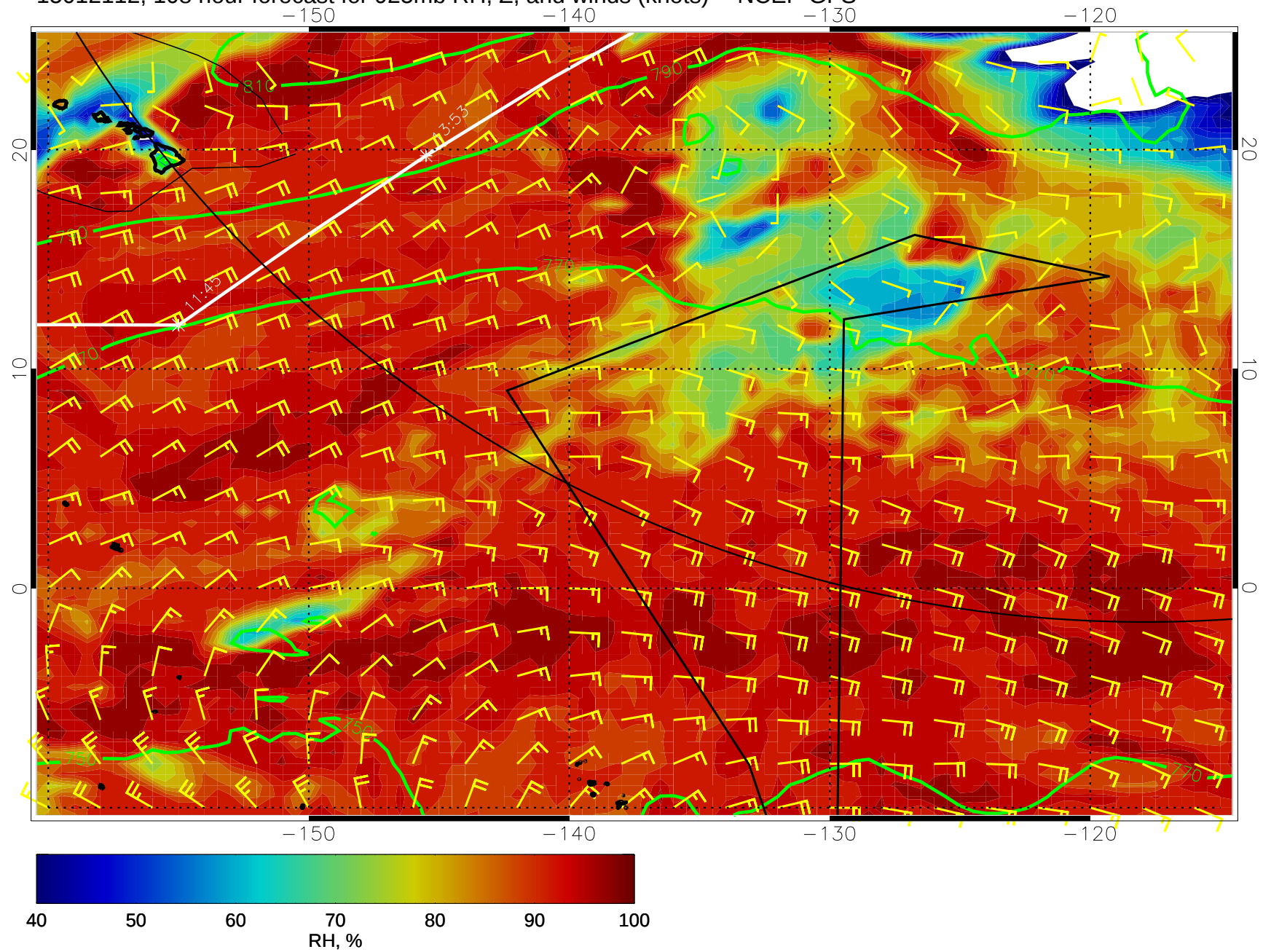
15012112, 108 hour forecast for 925mb RH, Z, and winds (knots) -- NCEP GFS
