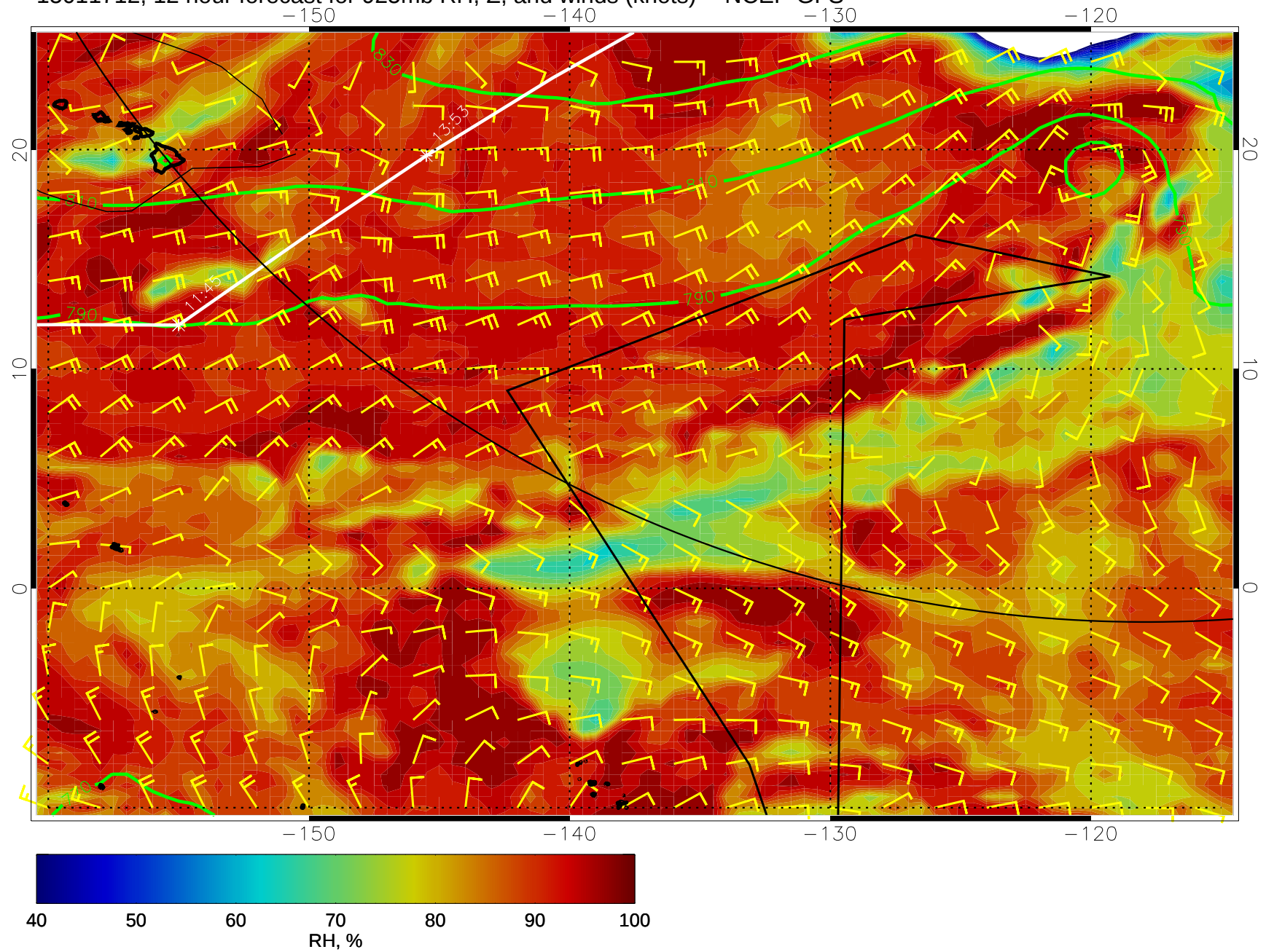
15011712, 12 hour forecast for 925mb RH, Z, and winds (knots) -- NCEP GFS
