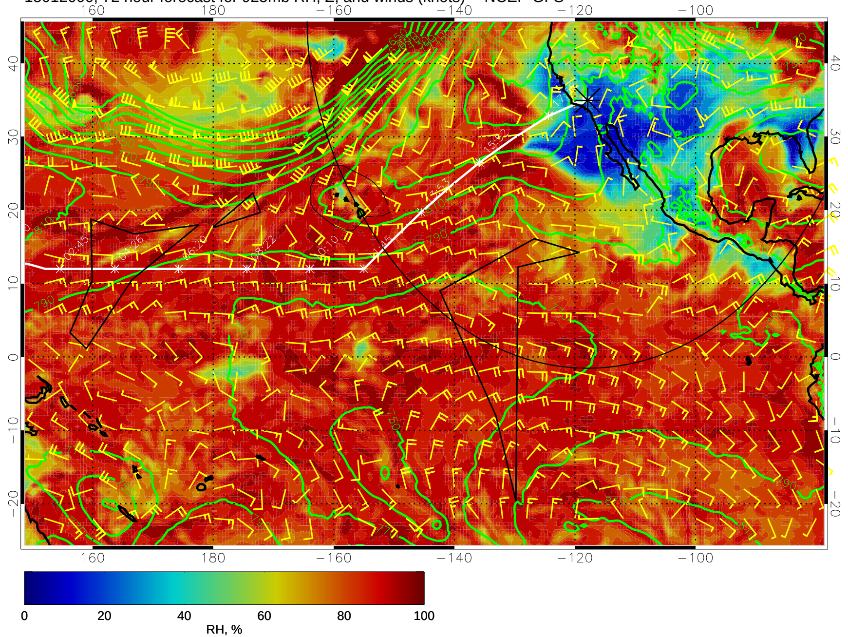
15012000, 72 hour forecast for 925mb RH, Z, and winds (knots) -- NCEP GFS
