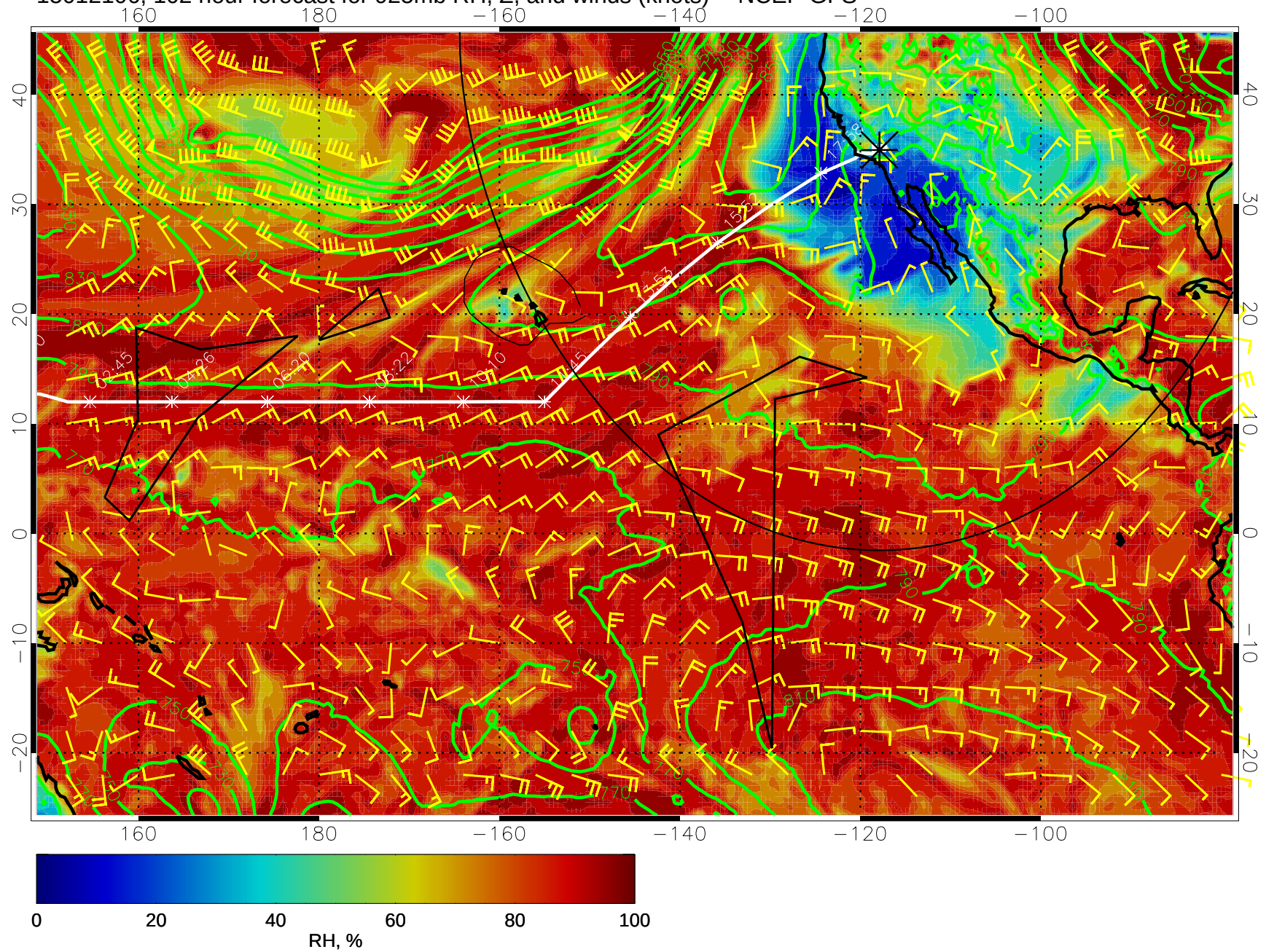
15012106, 102 hour forecast for 925mb RH, Z, and winds (knots) -- NCEP GFS
