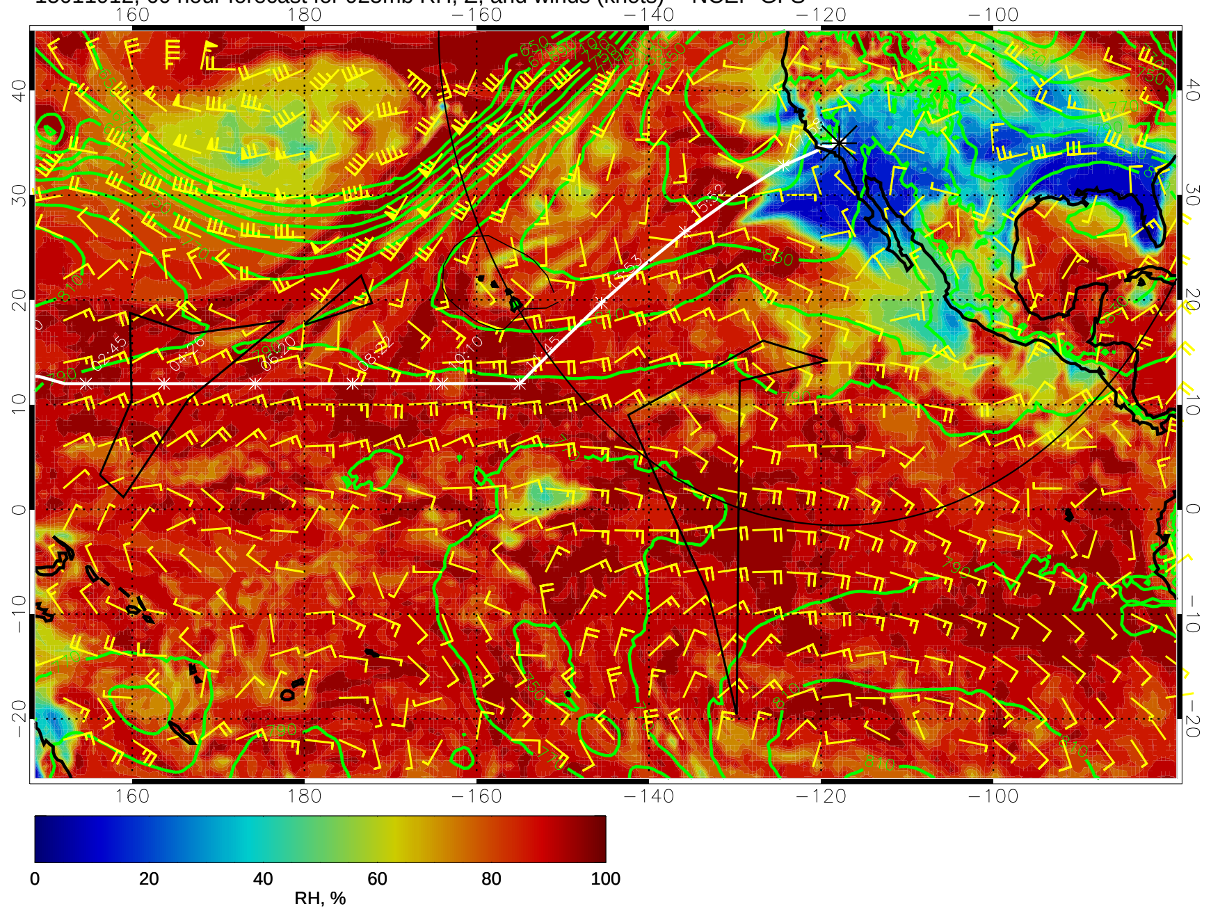
15011912, 60 hour forecast for 925mb RH, Z, and winds (knots) -- NCEP GFS
