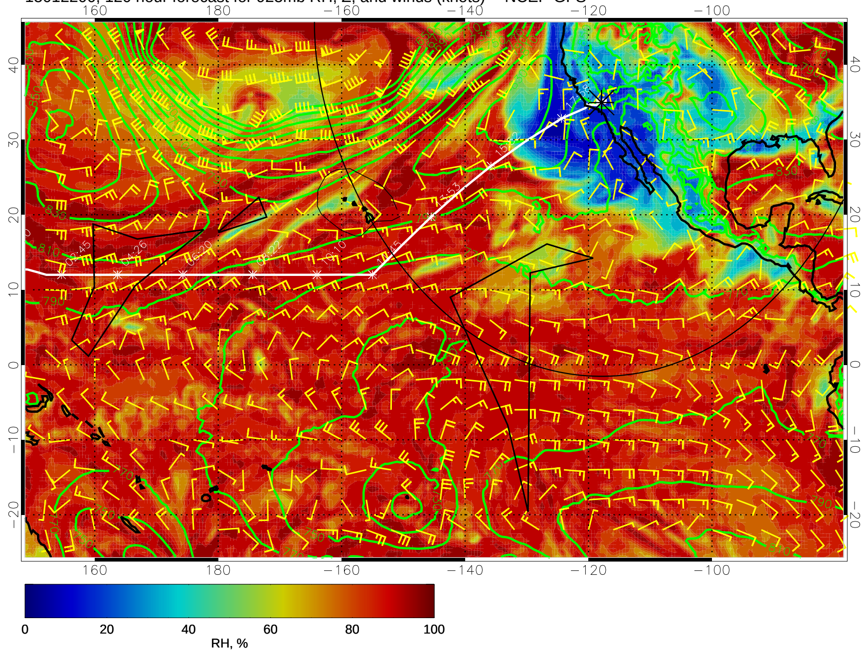
15012200, 120 hour forecast for 925mb RH, Z, and winds (knots) -- NCEP GFS
