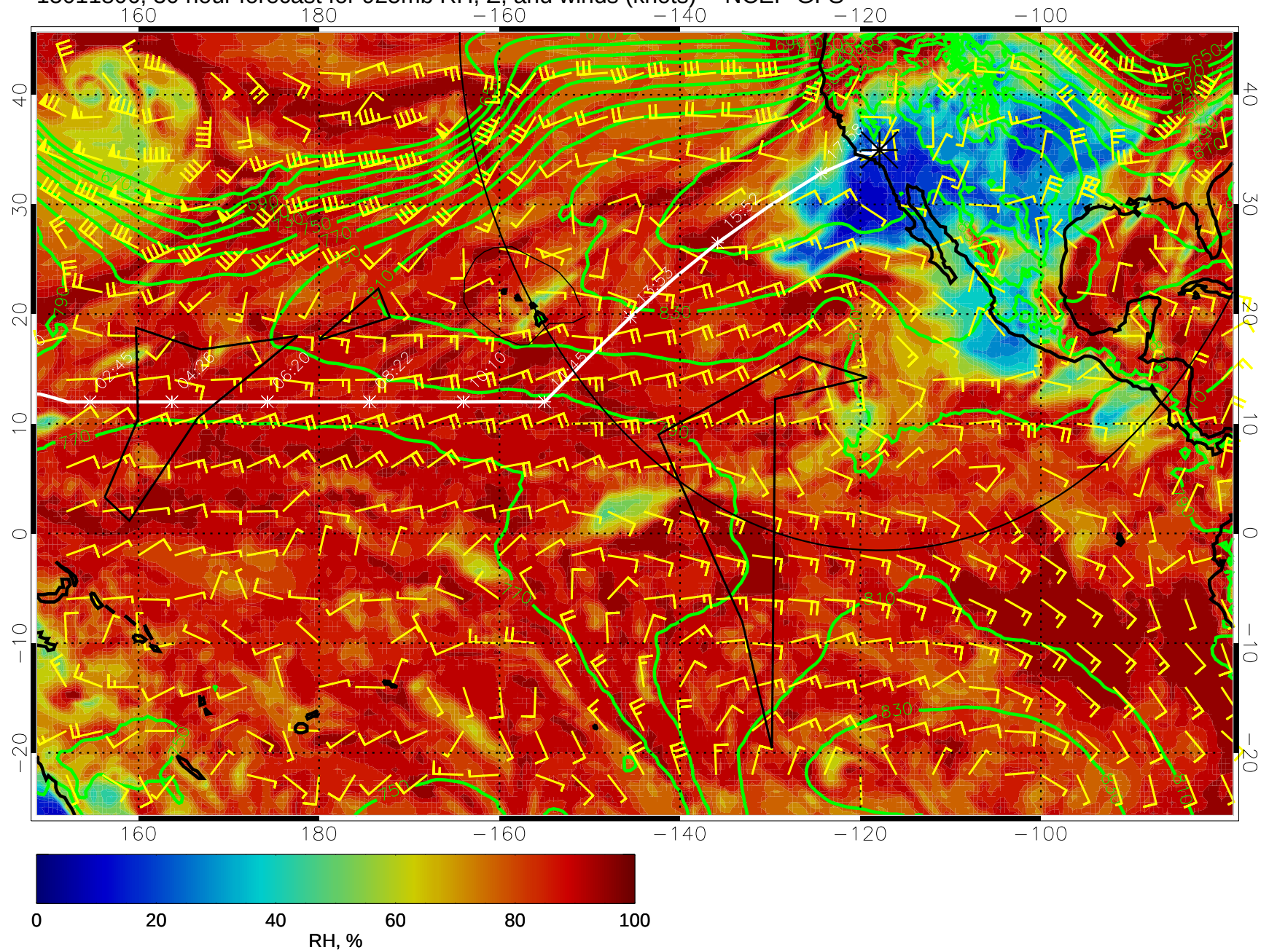
15011806, 30 hour forecast for 925mb RH, Z, and winds (knots) -- NCEP GFS
