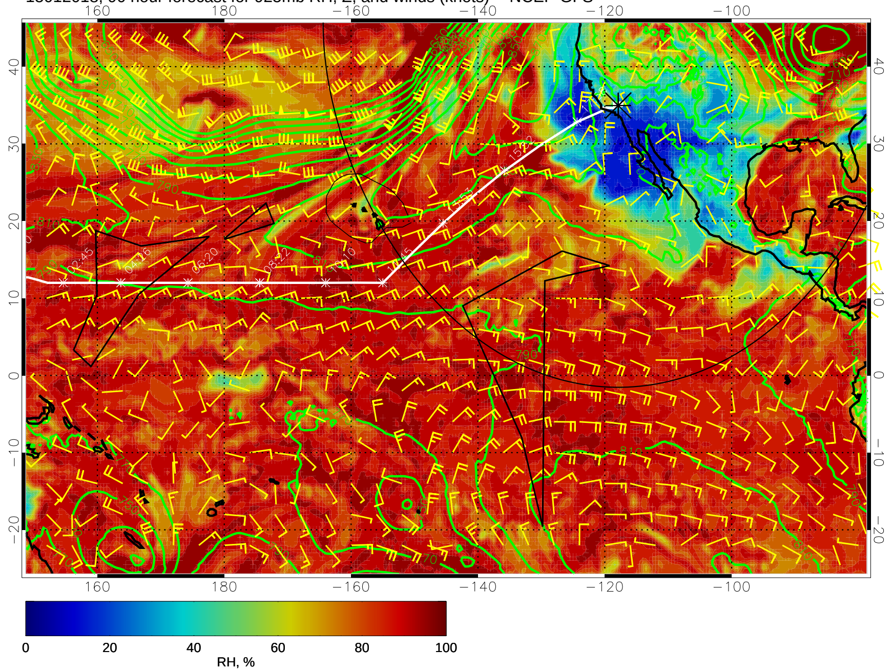
15012018, 90 hour forecast for 925mb RH, Z, and winds (knots) -- NCEP GFS
