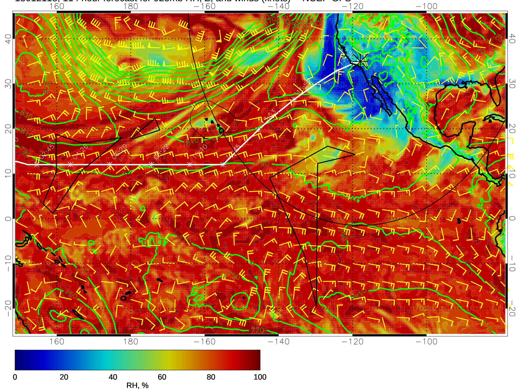
15012118, 114 hour forecast for 925mb RH, Z, and winds (knots) -- NCEP GFS
