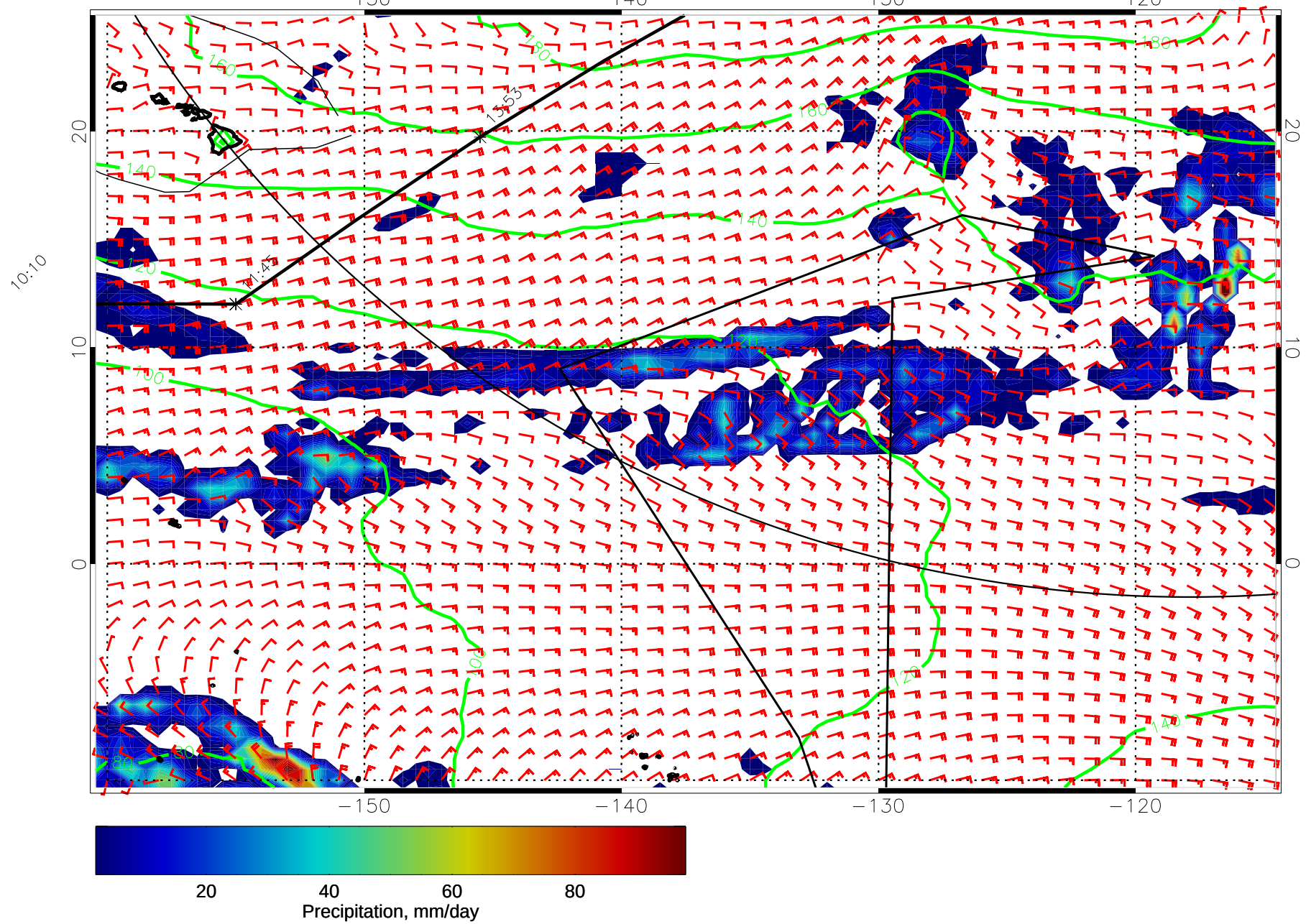
15011906, 54 hour forecast for precip, 1000mb Z, and winds (knots) -- NCEP GFS
