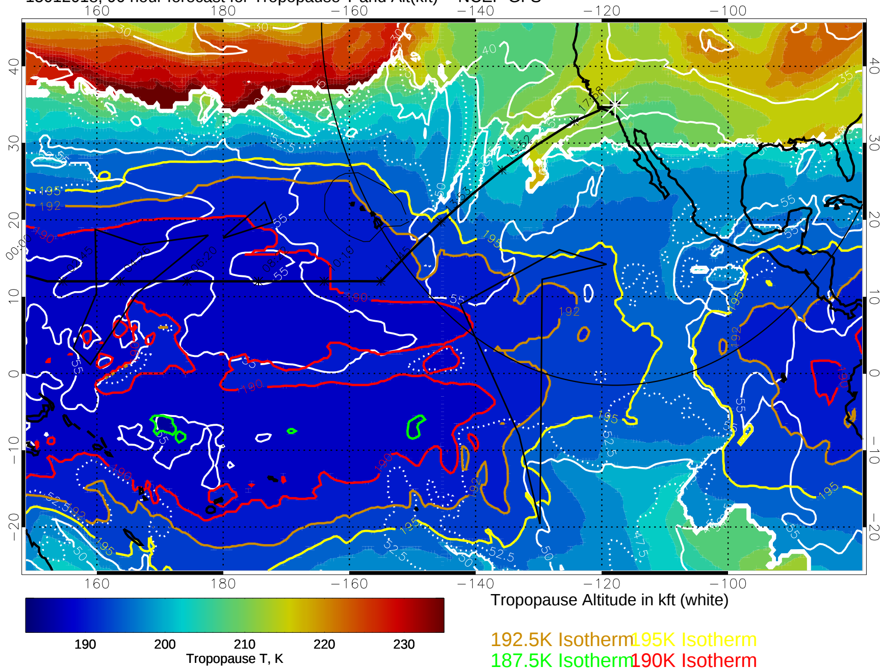
15012018, 90 hour forecast for Tropopause T and Alt(kft) -- NCEP GFS
