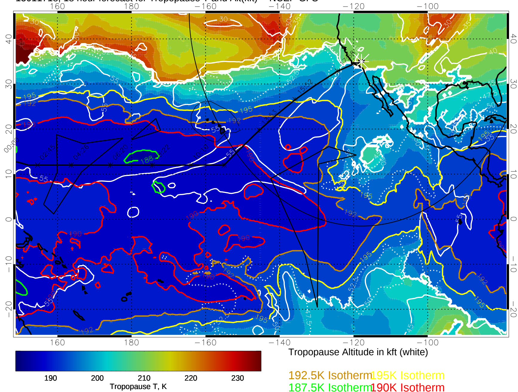
15011718, 18 hour forecast for Tropopause T and Alt(kft) -- NCEP GFS
