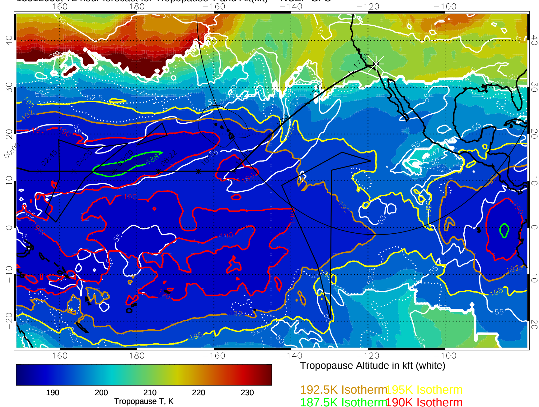
15012000, 72 hour forecast for Tropopause T and Alt(kft) -- NCEP GFS
