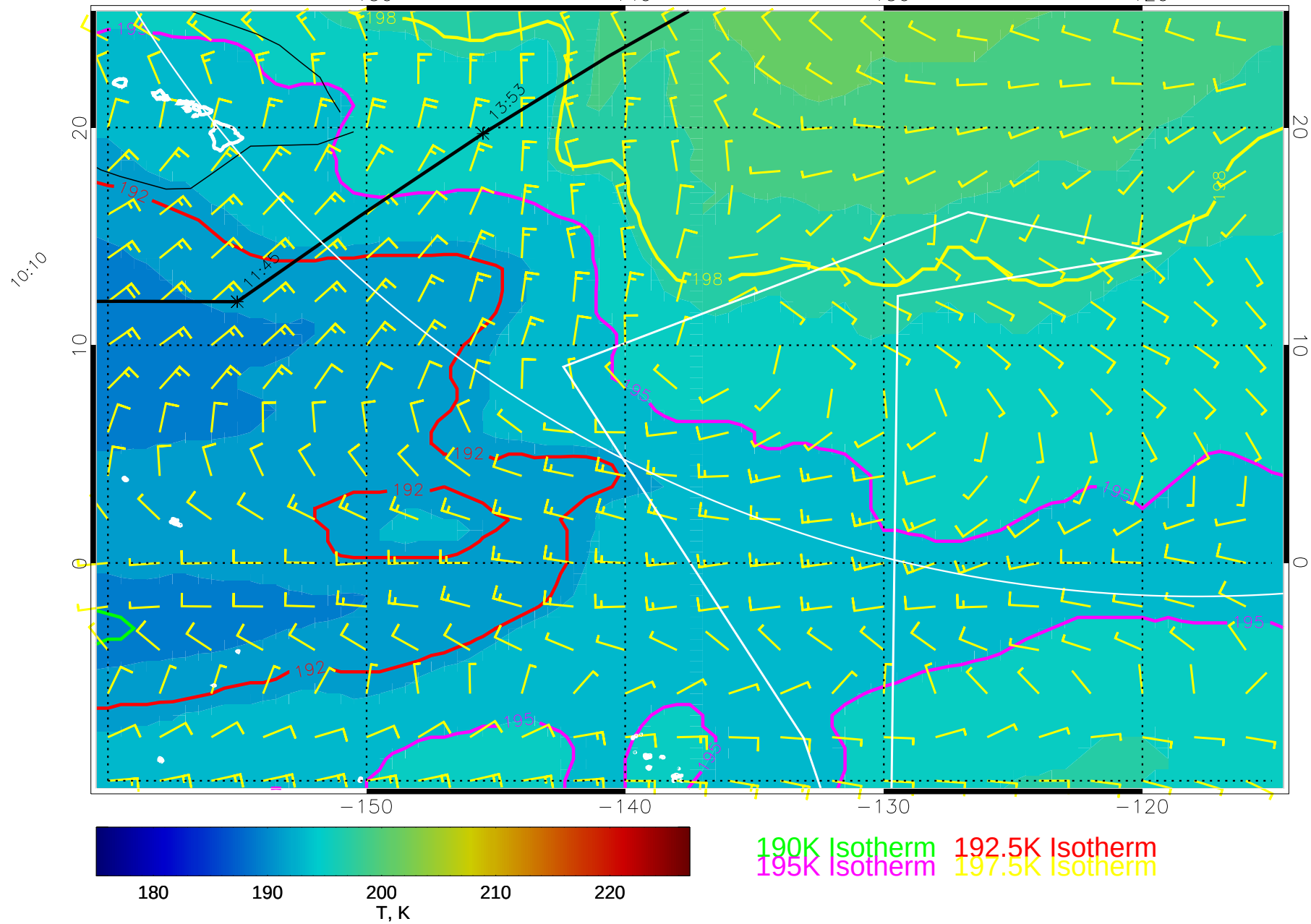
15012106, 102 hour forecast for 70mb T and winds (knots) -- NCEP GFS
