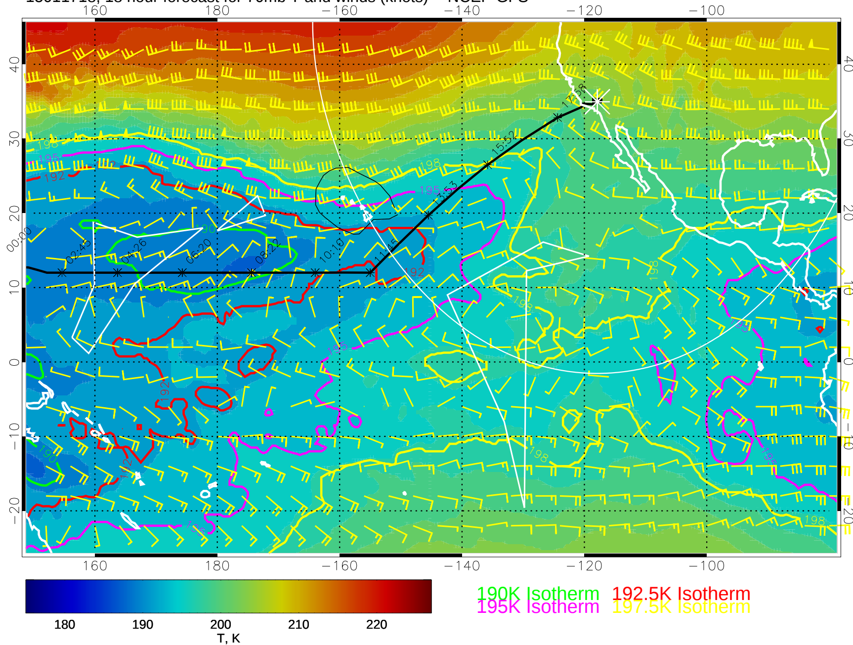
15011718, 18 hour forecast for 70mb T and winds (knots) -- NCEP GFS
