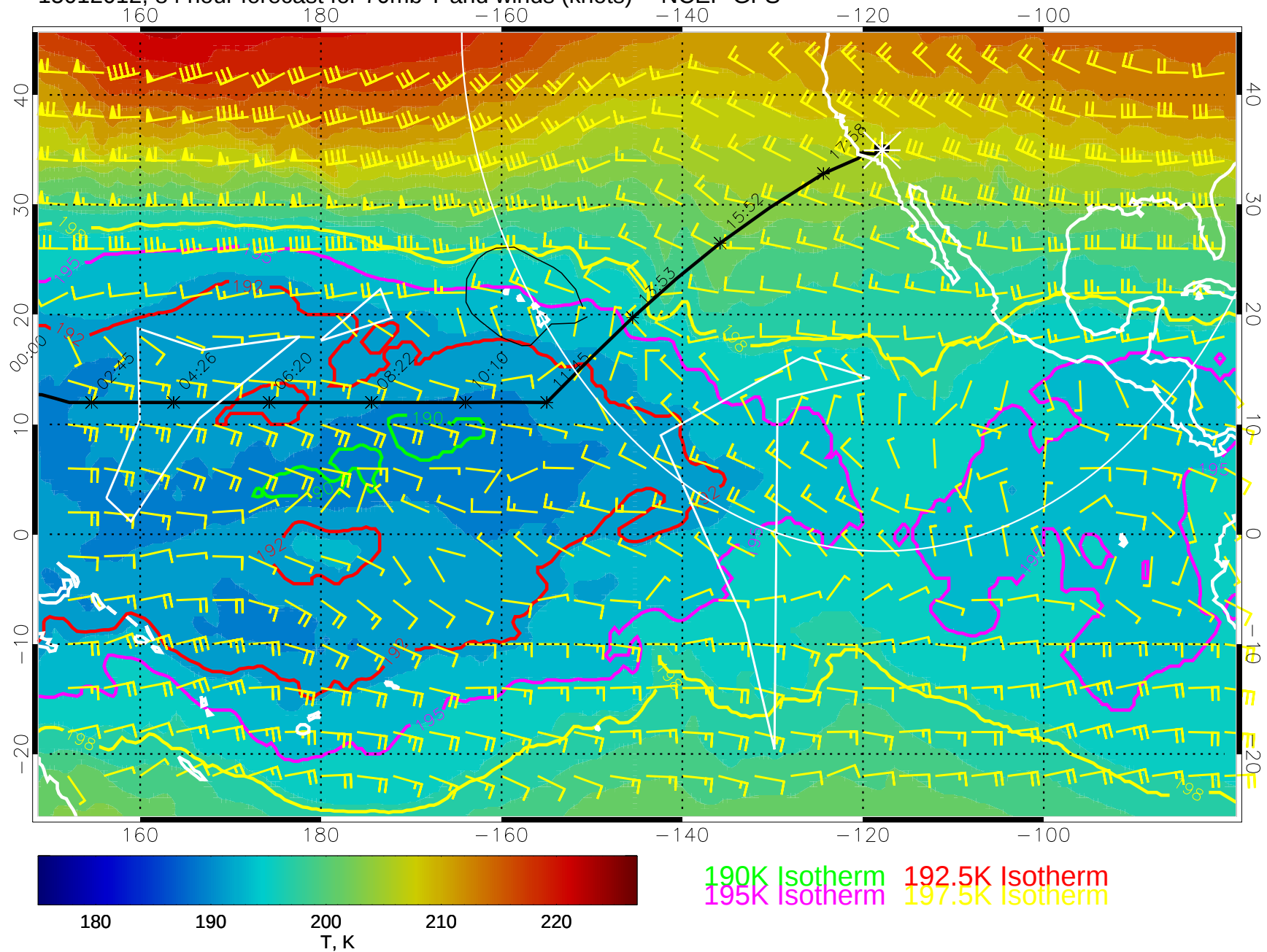
15012012, 84 hour forecast for 70mb T and winds (knots) -- NCEP GFS
