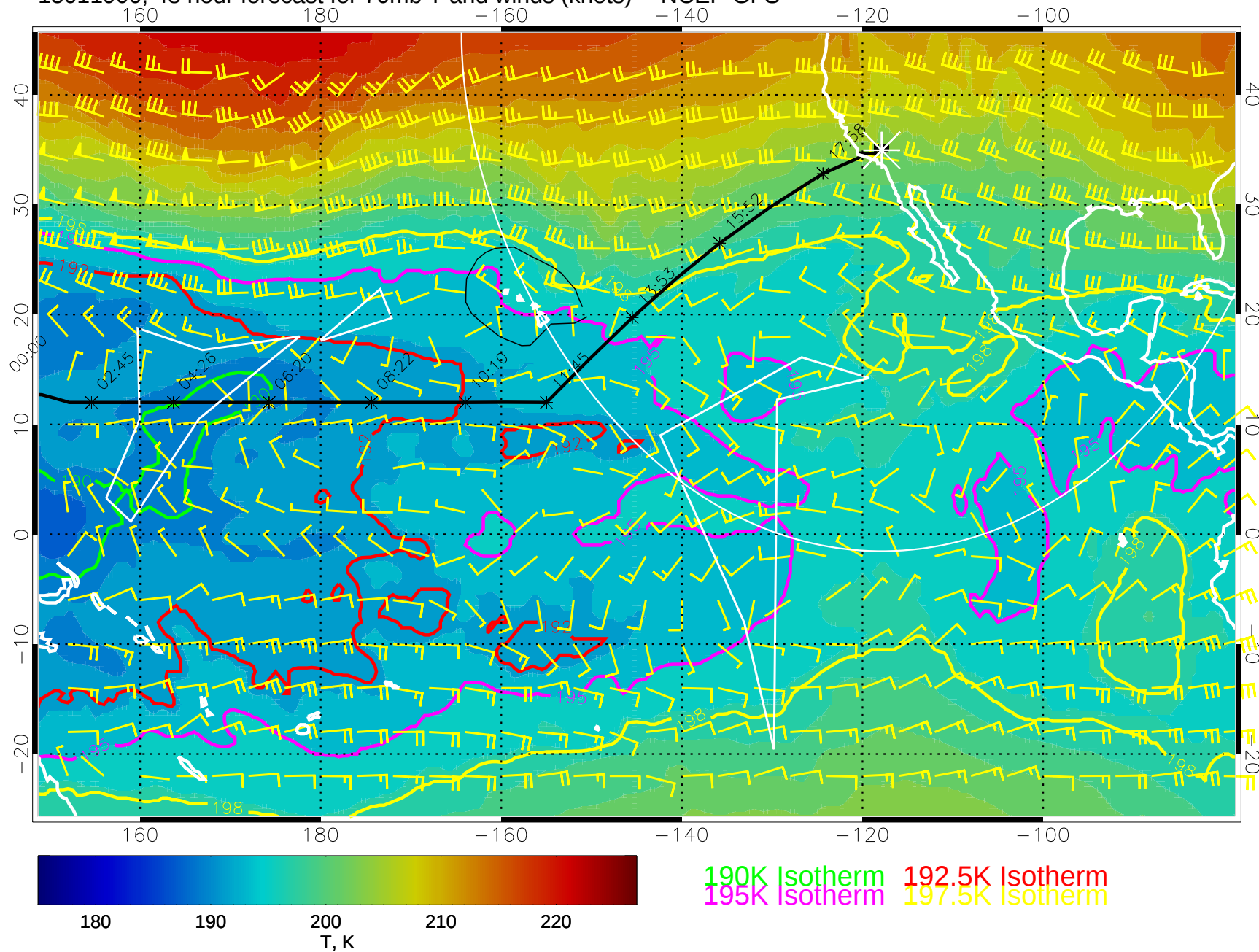
15011900, 48 hour forecast for 70mb T and winds (knots) -- NCEP GFS
