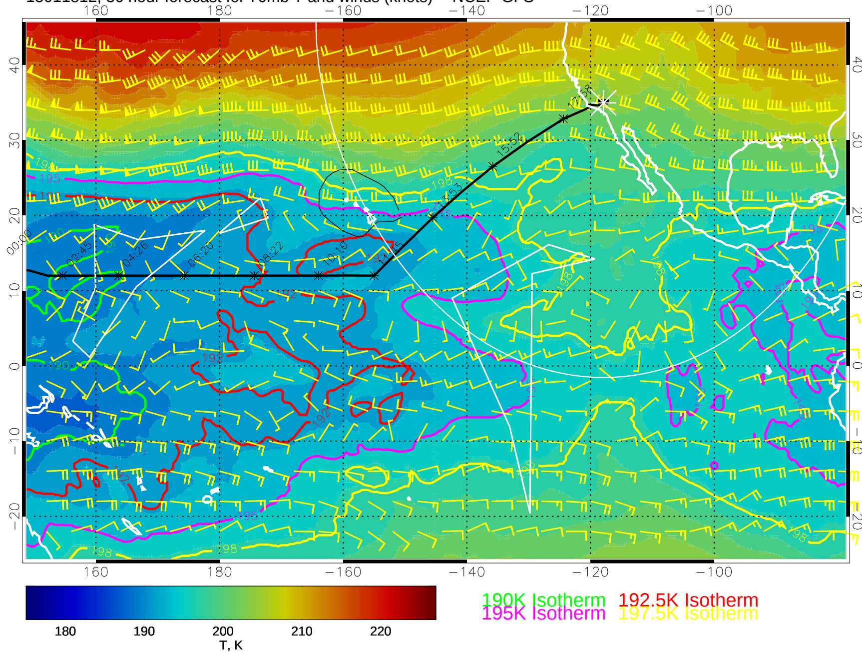
15011812, 36 hour forecast for 70mb T and winds (knots) -- NCEP GFS
