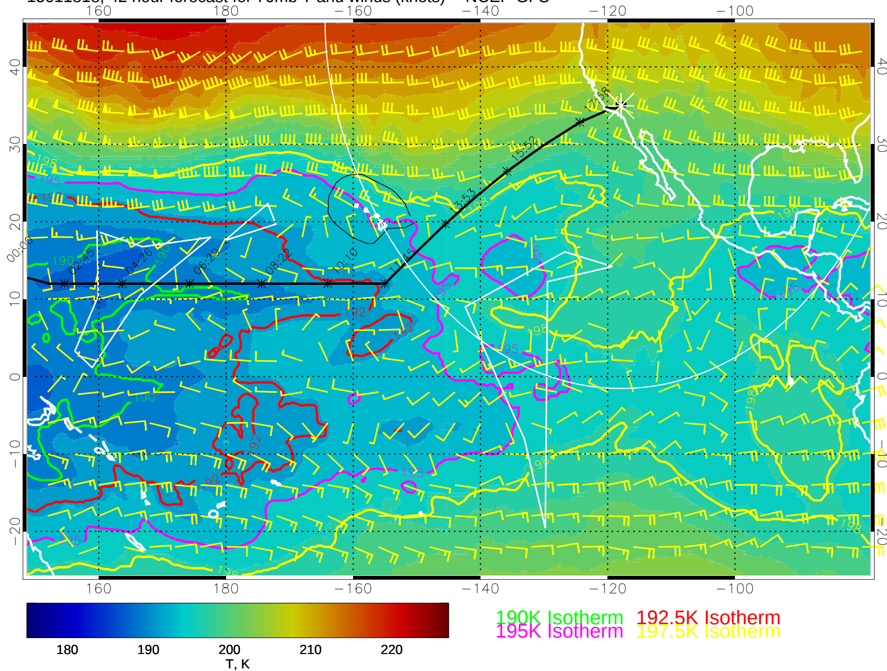
15011818, 42 hour forecast for 70mb T and winds (knots) -- NCEP GFS
