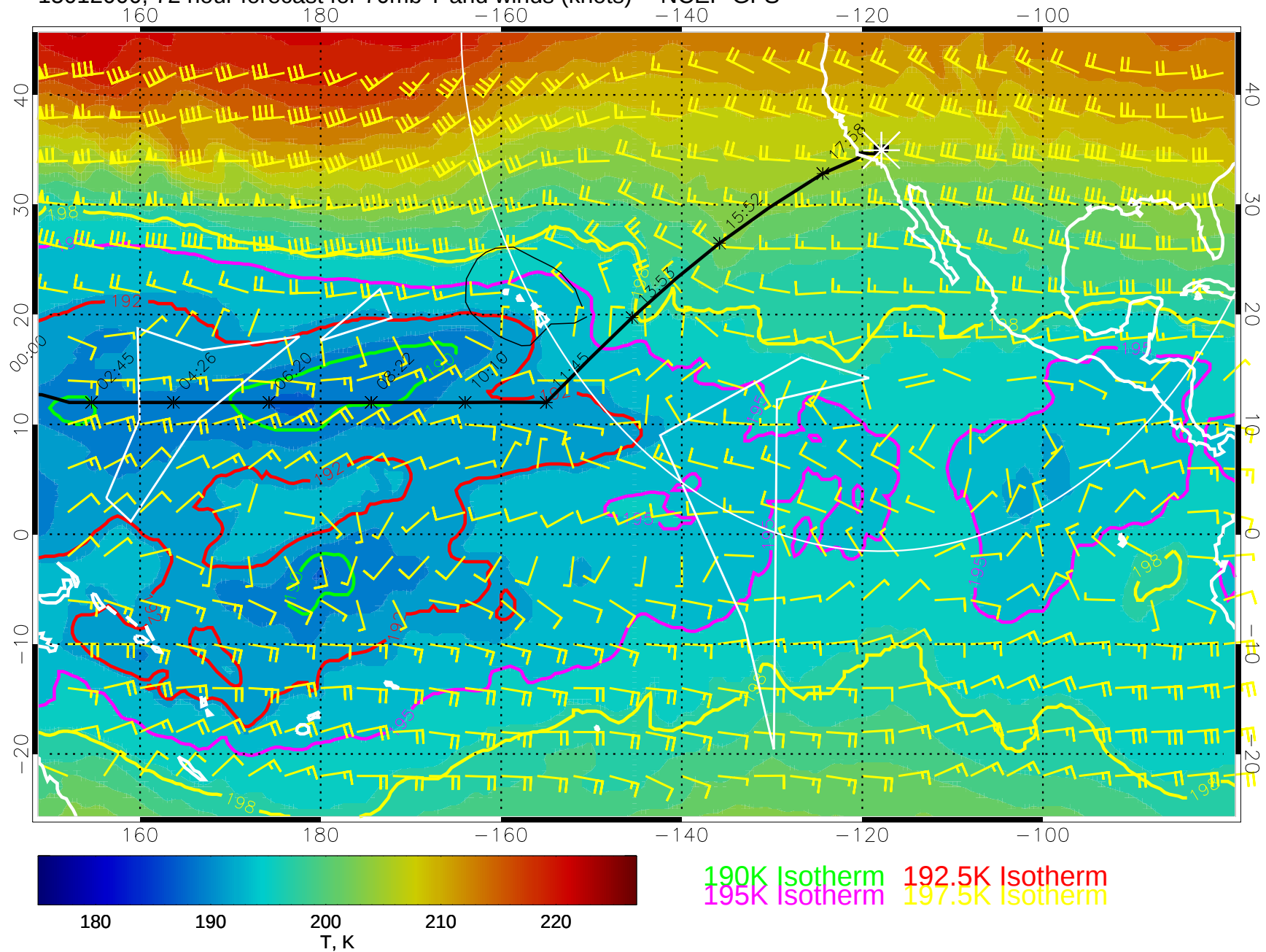
15012000, 72 hour forecast for 70mb T and winds (knots) -- NCEP GFS
