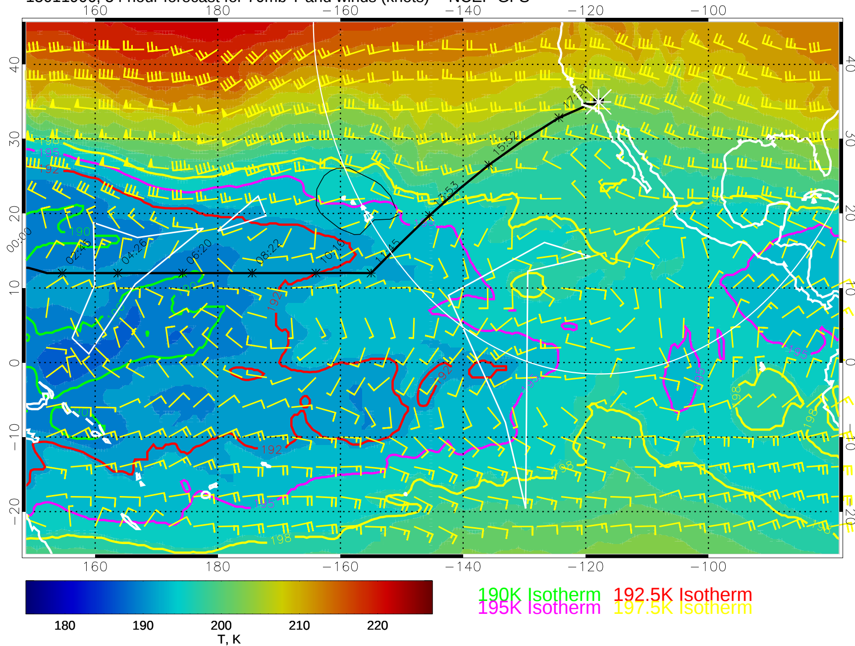
15011906, 54 hour forecast for 70mb T and winds (knots) -- NCEP GFS
