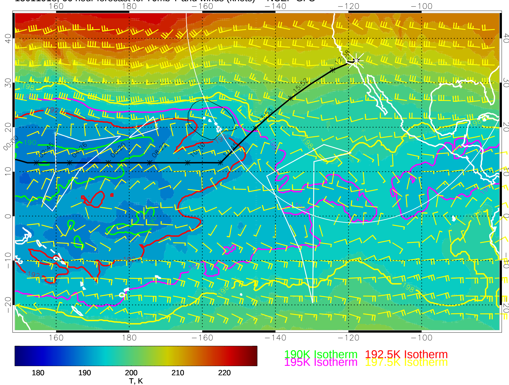
15011918, 66 hour forecast for 70mb T and winds (knots) -- NCEP GFS
