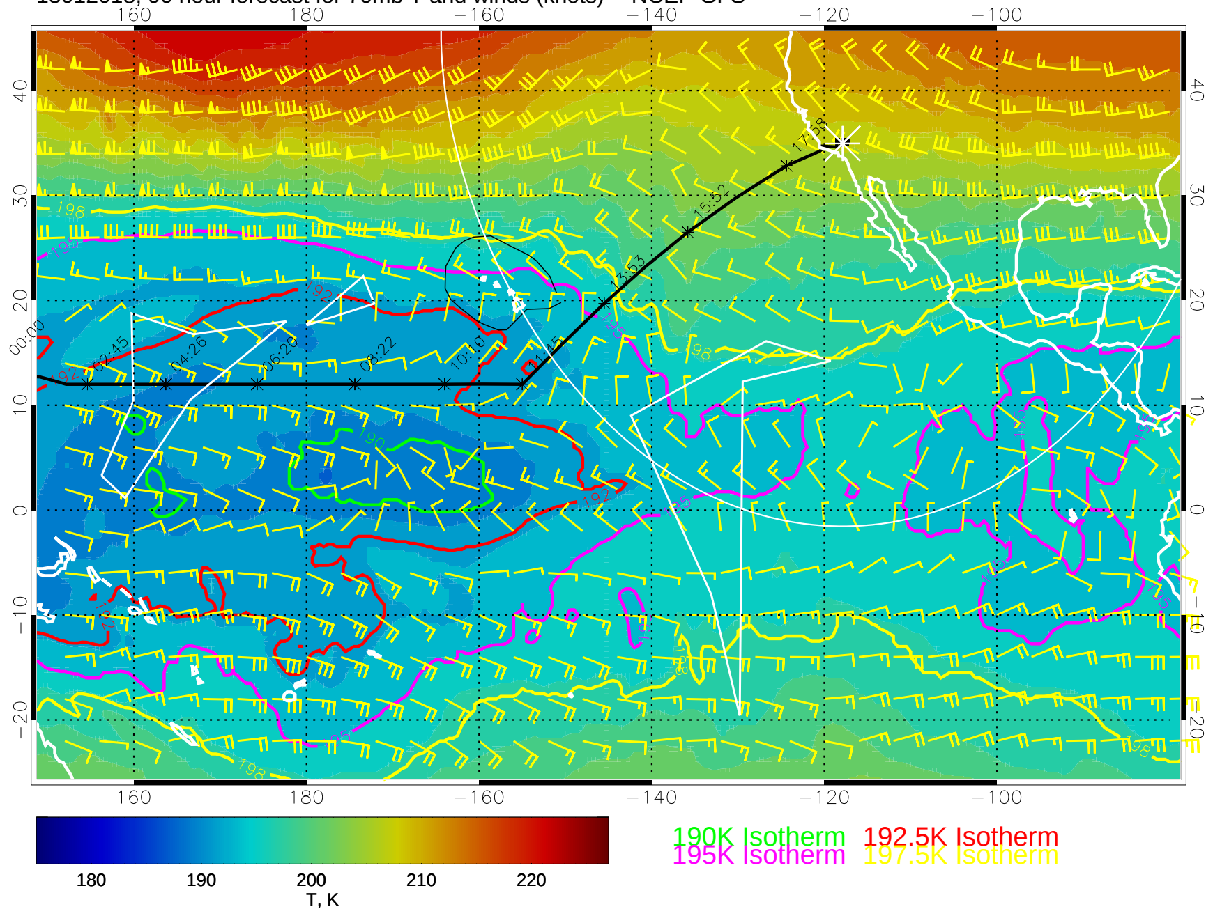
15012018, 90 hour forecast for 70mb T and winds (knots) -- NCEP GFS
