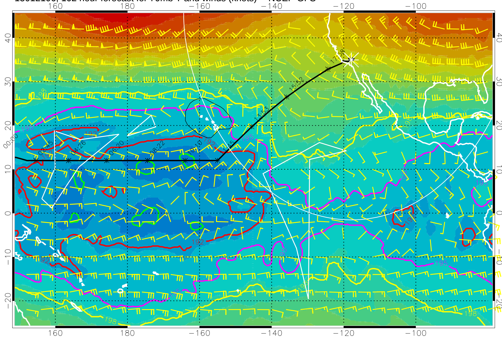
15012106, 102 hour forecast for 70mb T and winds (knots) -- NCEP GFS
