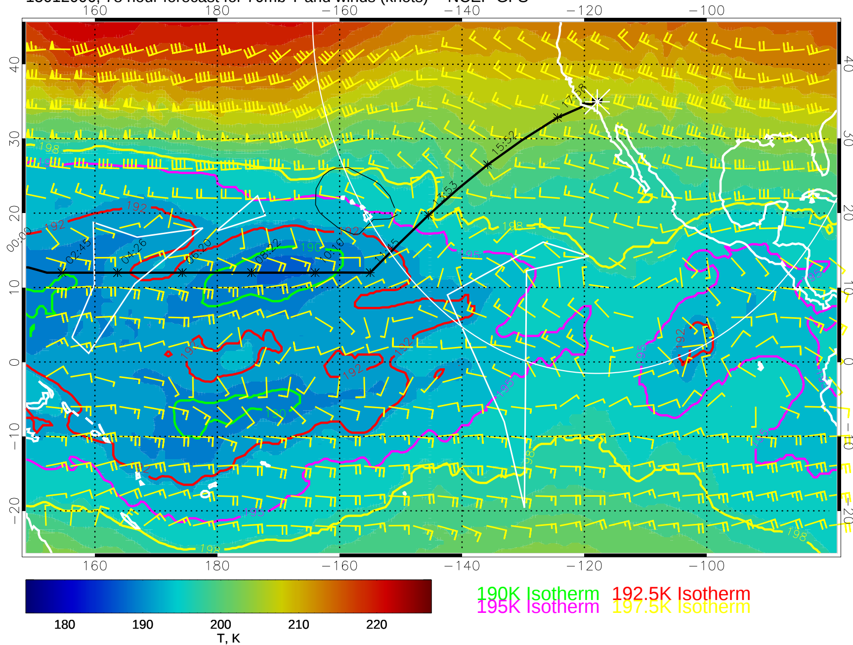
15012006, 78 hour forecast for 70mb T and winds (knots) -- NCEP GFS
