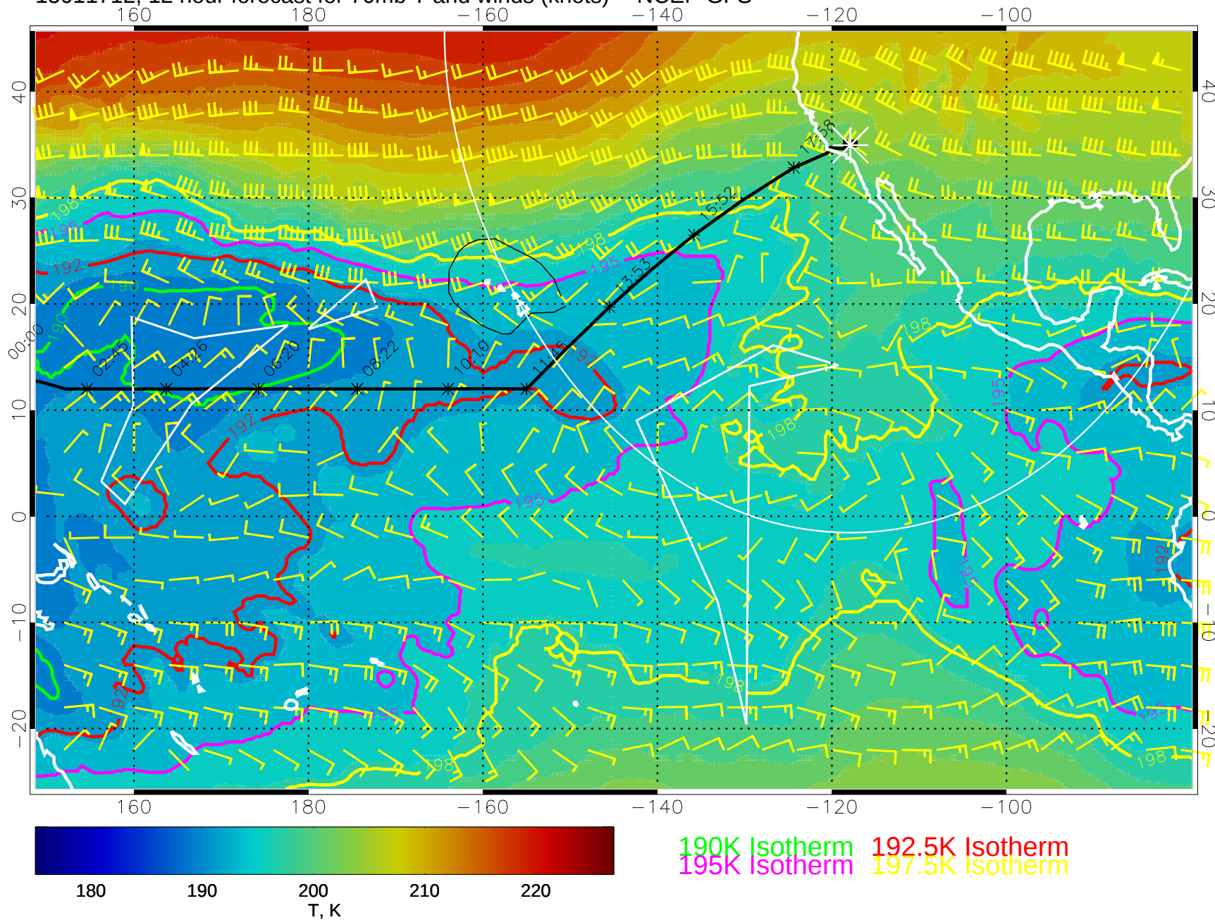
15011712, 12 hour forecast for 70mb T and winds (knots) -- NCEP GFS
