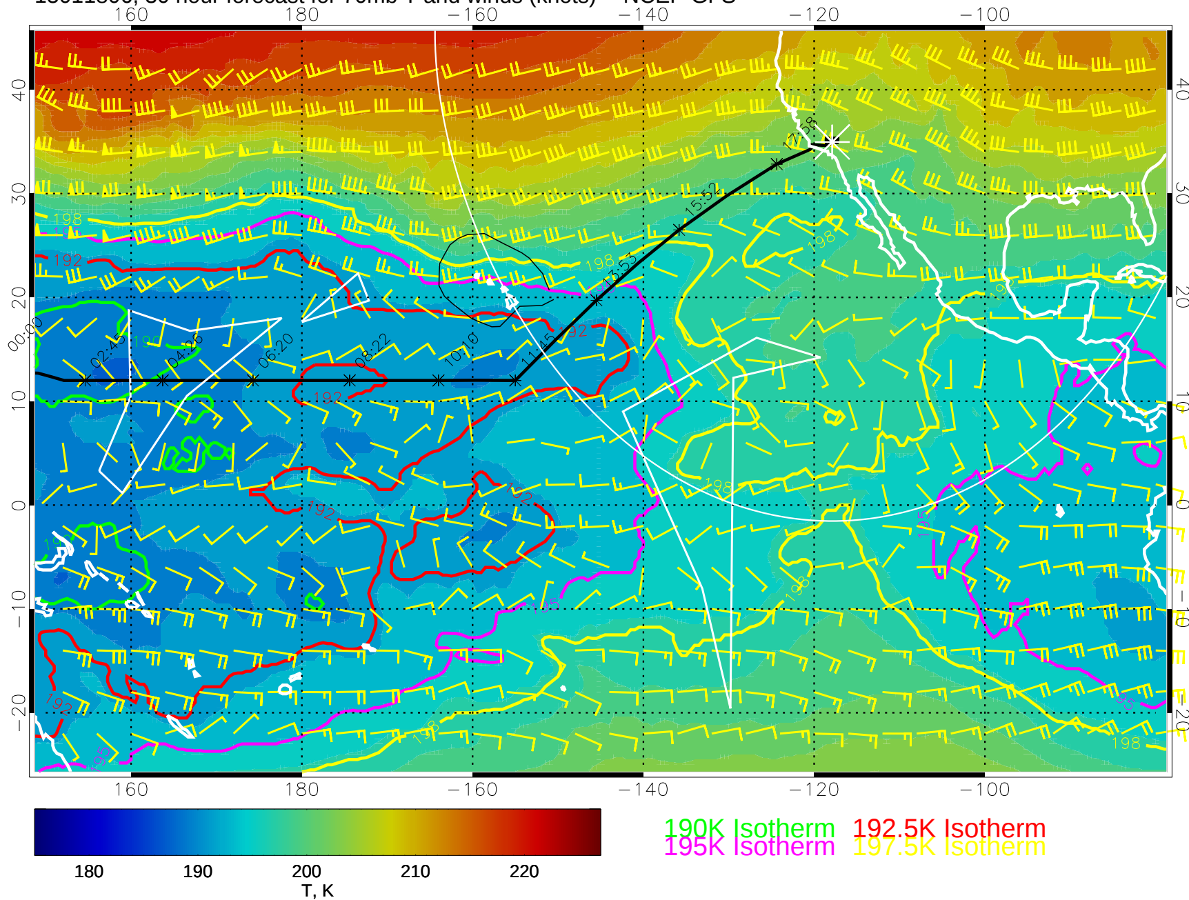
15011806, 30 hour forecast for 70mb T and winds (knots) -- NCEP GFS
