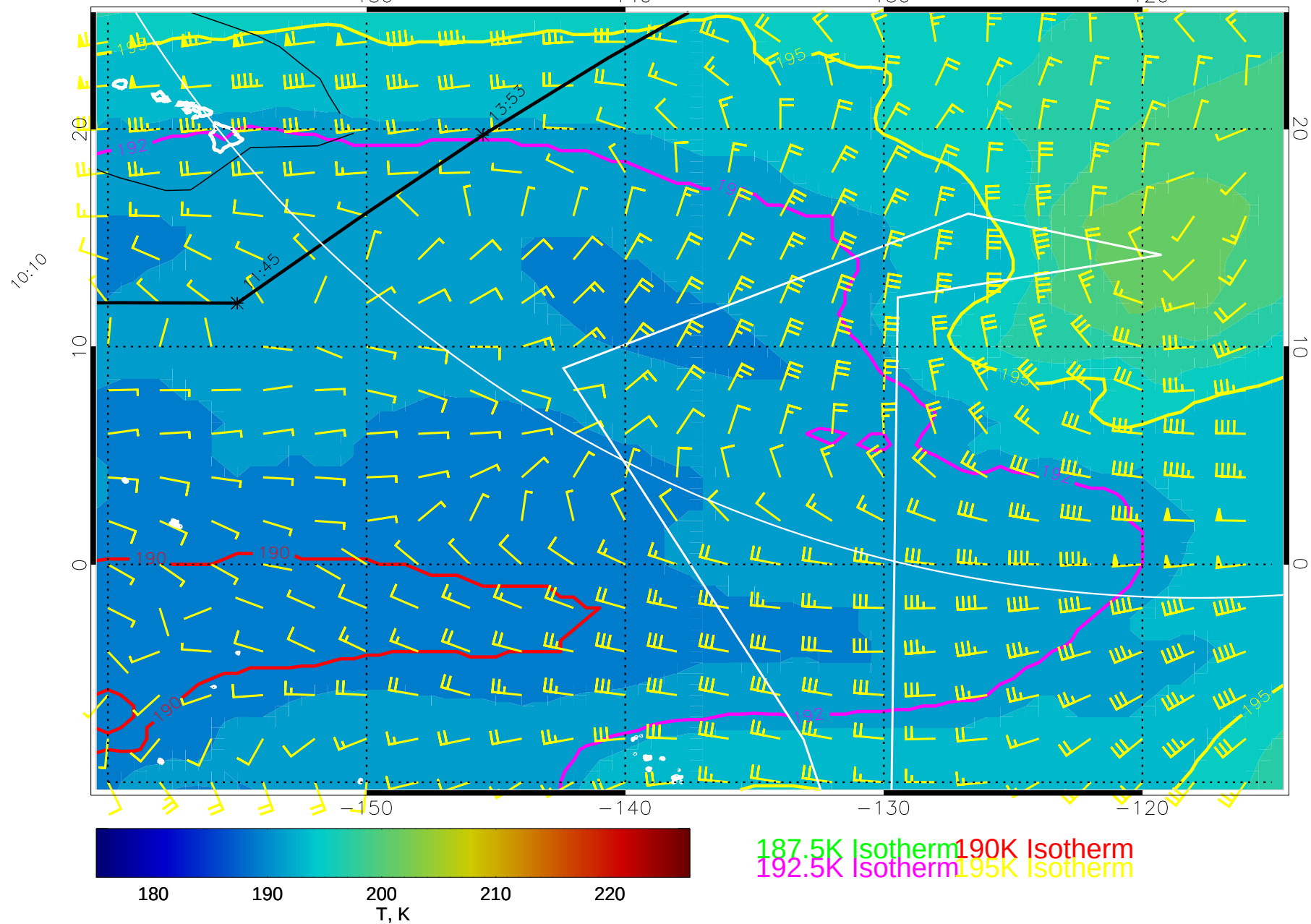
15011712, 12 hour forecast for 100mb T and winds (knots) -- NCEP GFS
