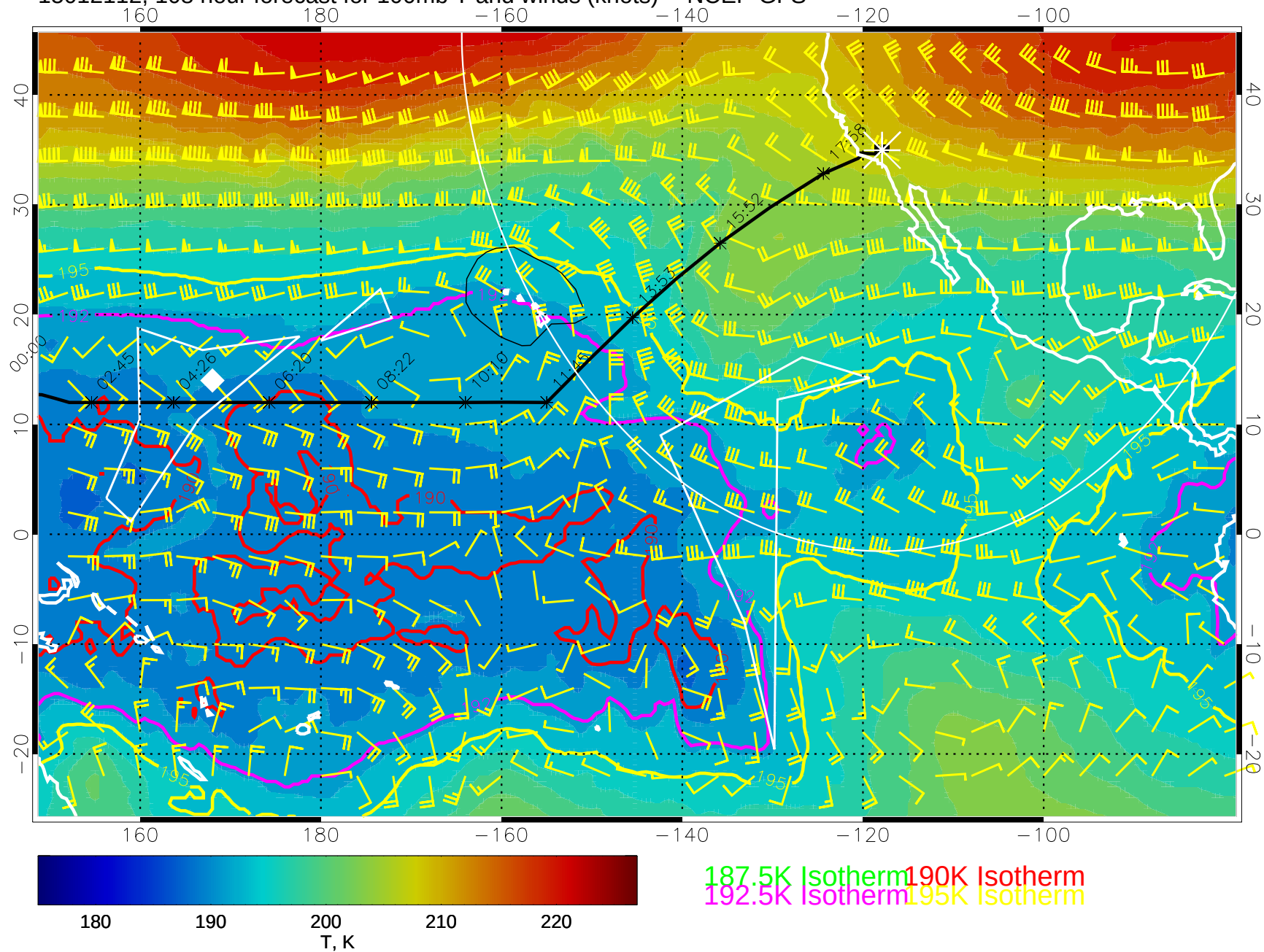
15012112, 108 hour forecast for 100mb T and winds (knots) -- NCEP GFS
