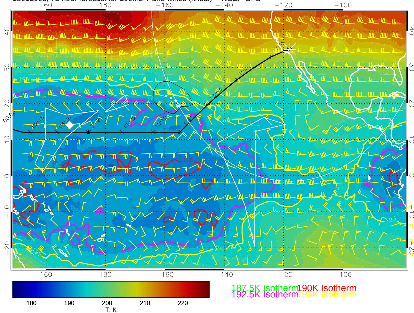
15012000, 72 hour forecast for 100mb T and winds (knots) -- NCEP GFS
