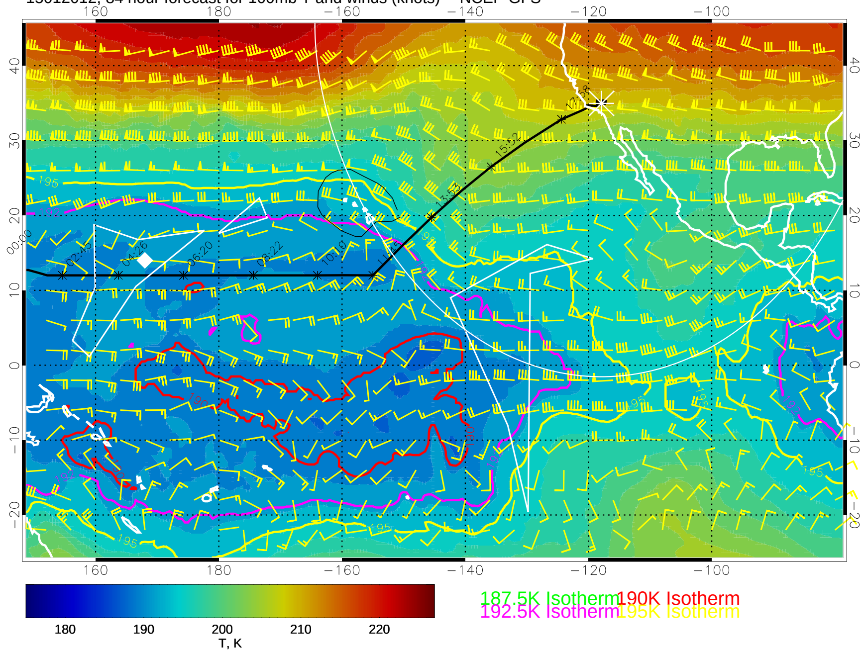
15012012, 84 hour forecast for 100mb T and winds (knots) -- NCEP GFS
