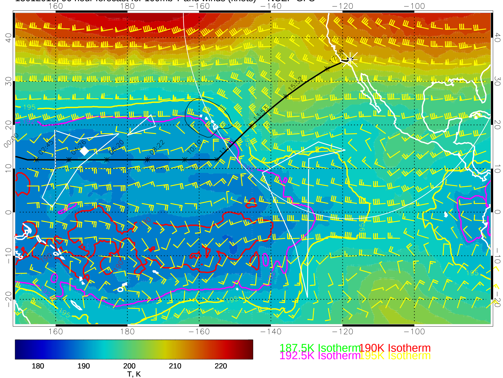
15012018, 90 hour forecast for 100mb T and winds (knots) -- NCEP GFS
