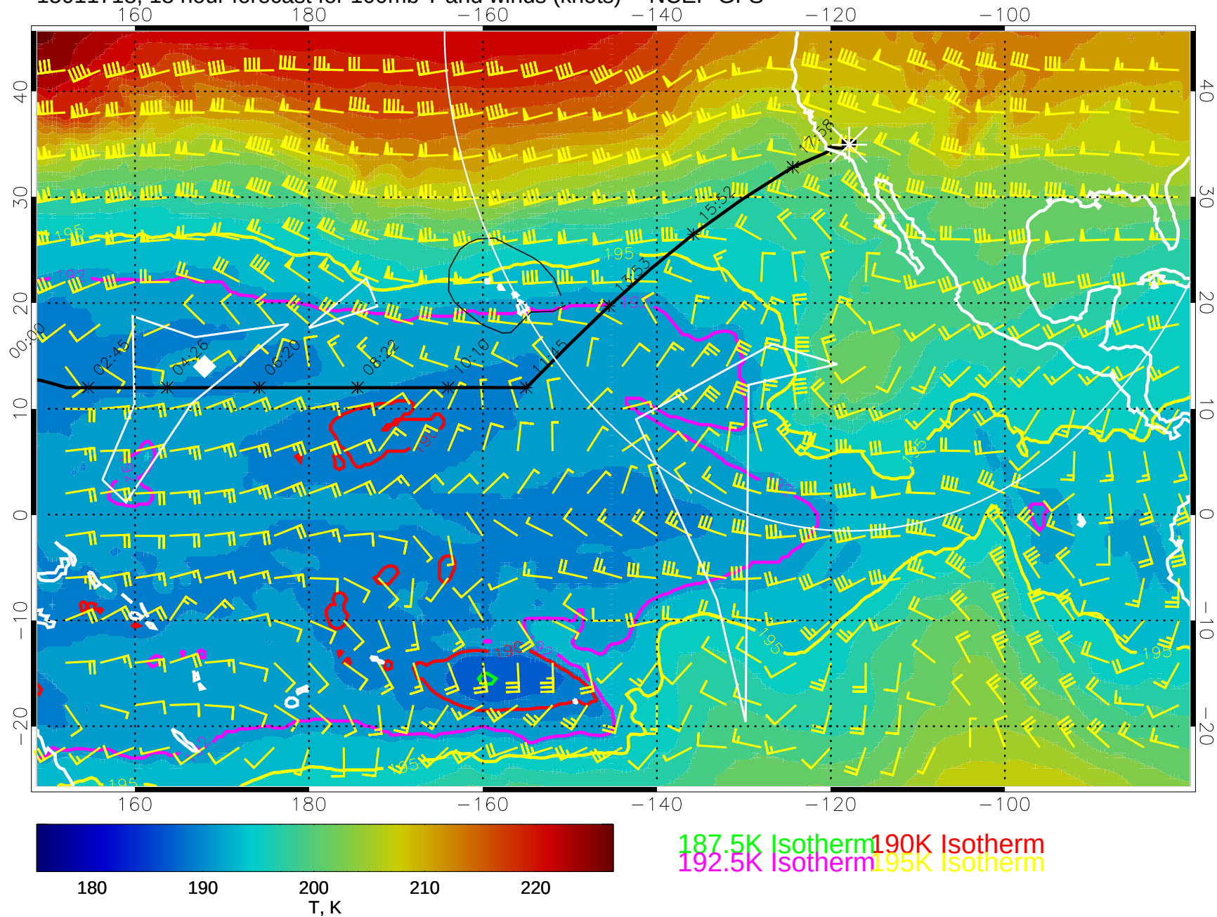
15011718, 18 hour forecast for 100mb T and winds (knots) -- NCEP GFS
