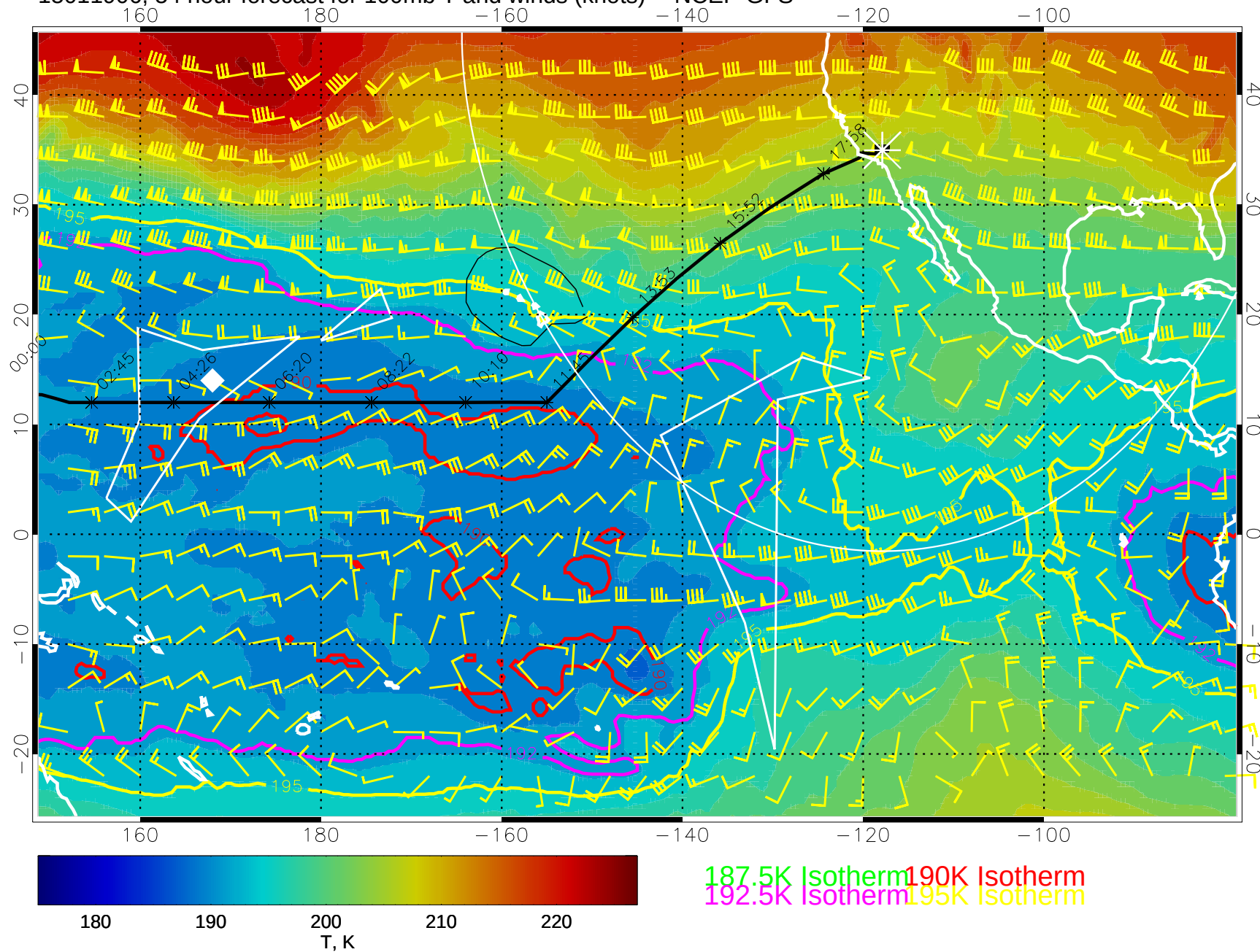
15011906, 54 hour forecast for 100mb T and winds (knots) -- NCEP GFS
