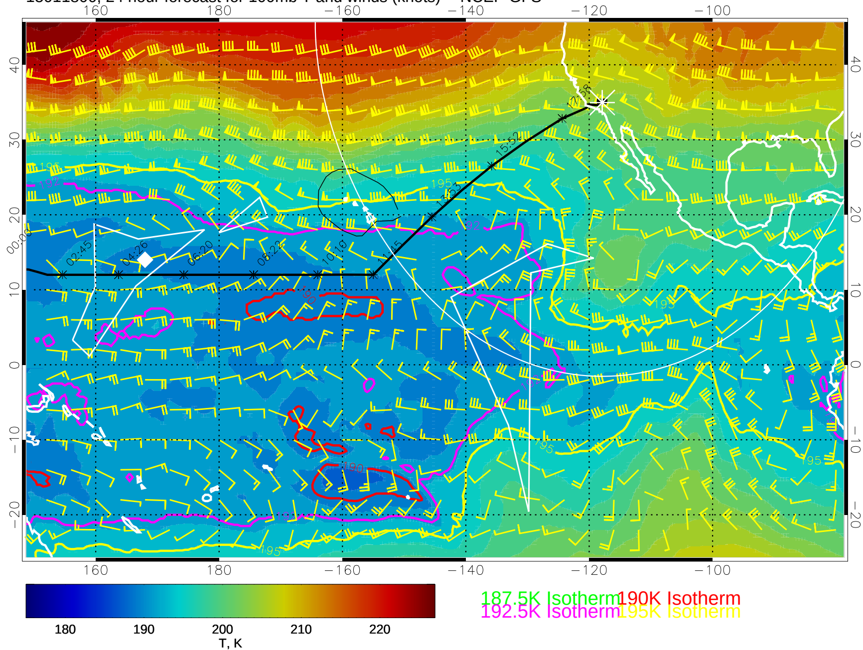
15011800, 24 hour forecast for 100mb T and winds (knots) -- NCEP GFS
