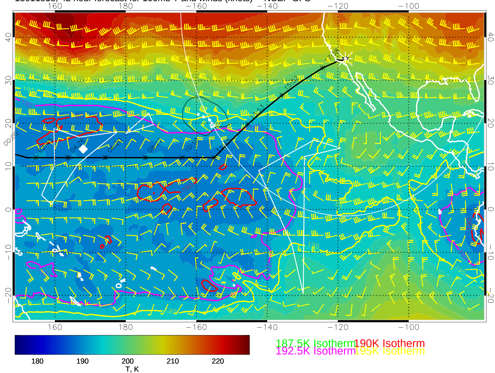
15011818, 42 hour forecast for 100mb T and winds (knots) -- NCEP GFS
