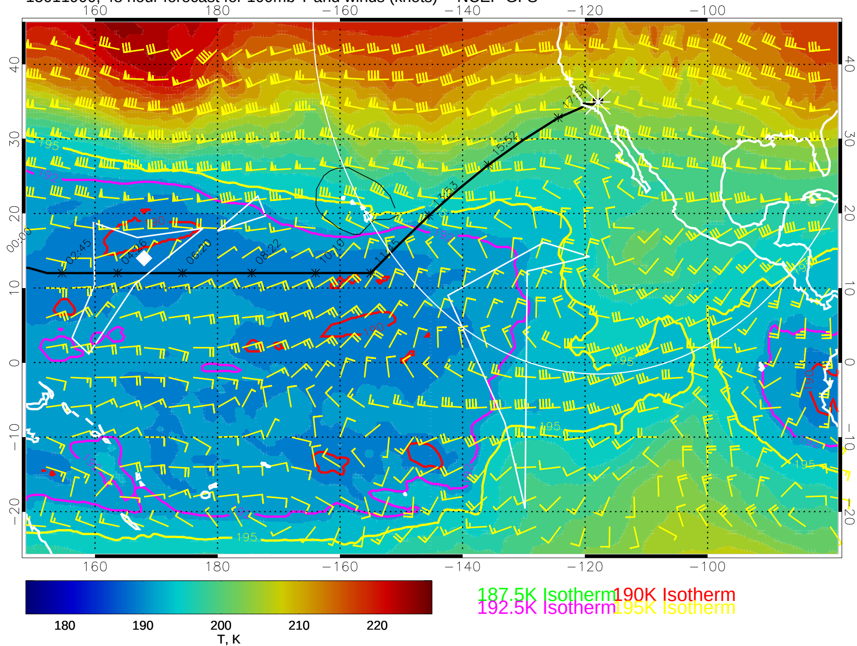
15011900, 48 hour forecast for 100mb T and winds (knots) -- NCEP GFS
