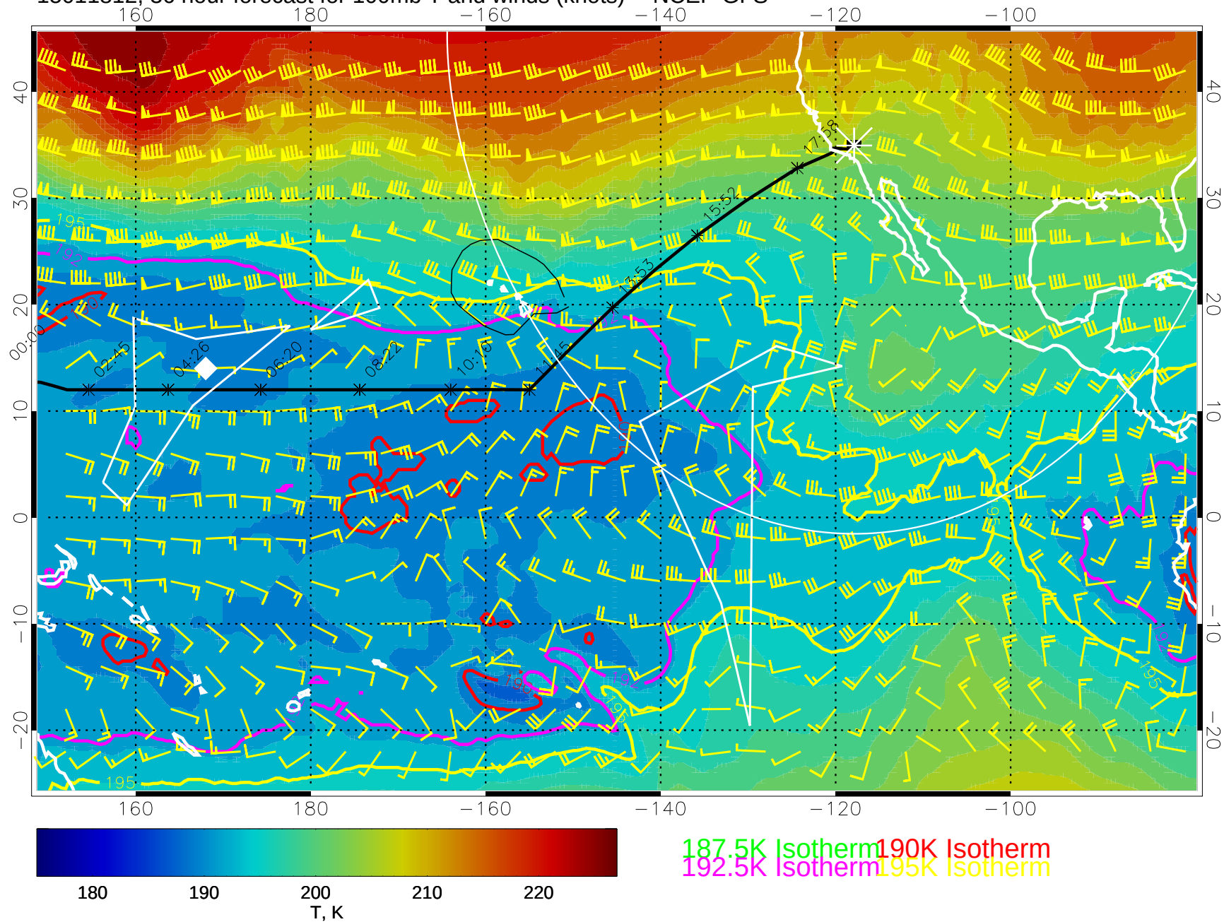
15011812, 36 hour forecast for 100mb T and winds (knots) -- NCEP GFS
