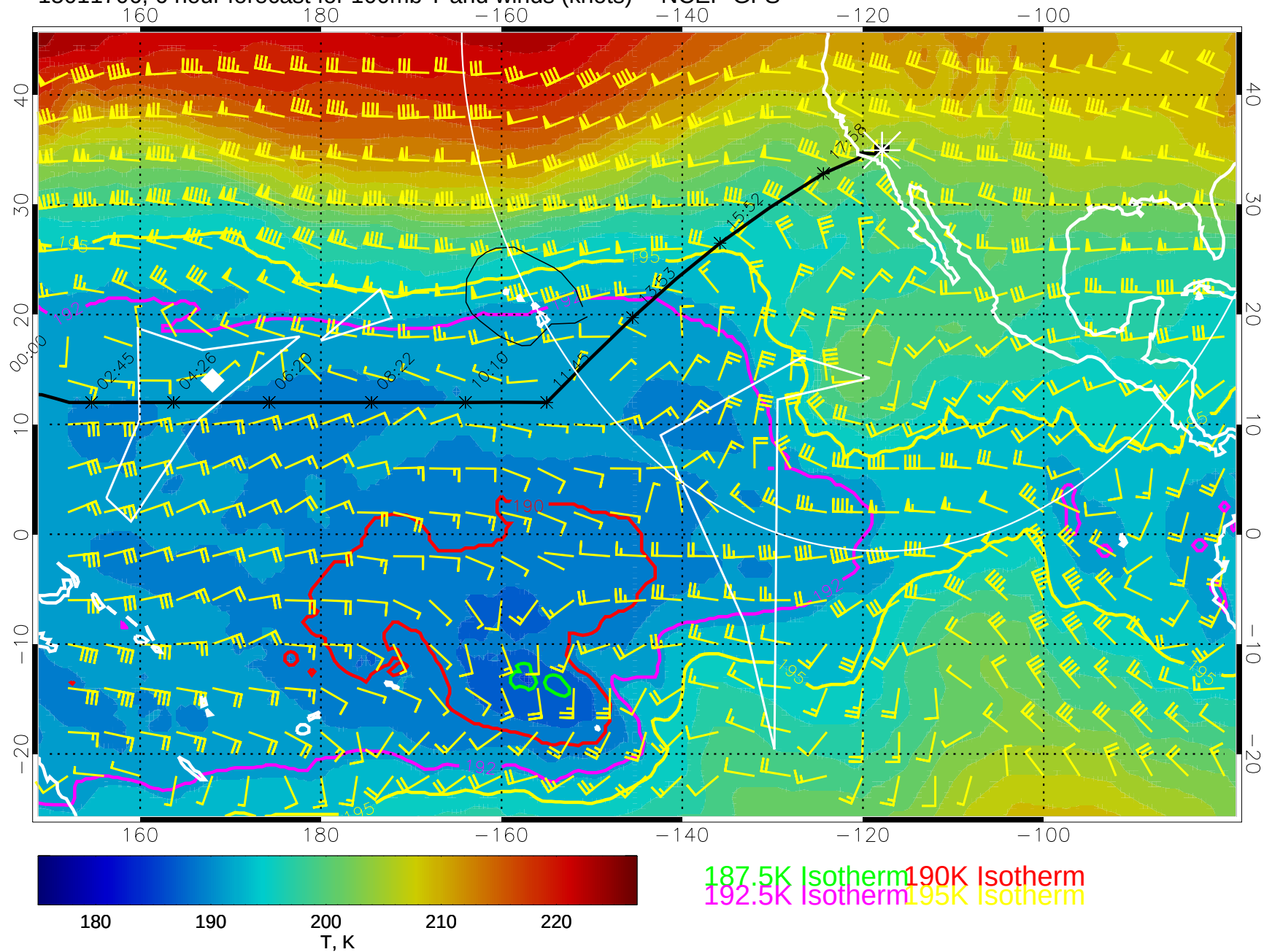
15011706, 6 hour forecast for 100mb T and winds (knots) -- NCEP GFS
