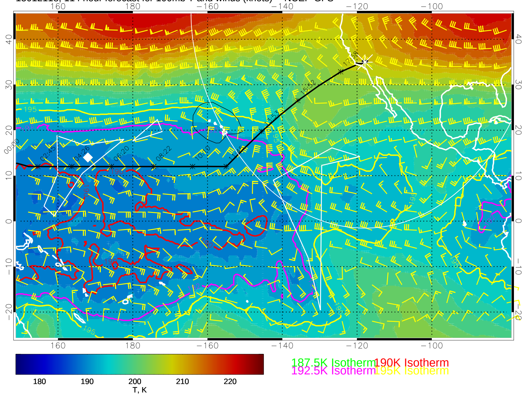
15012118, 114 hour forecast for 100mb T and winds (knots) -- NCEP GFS
