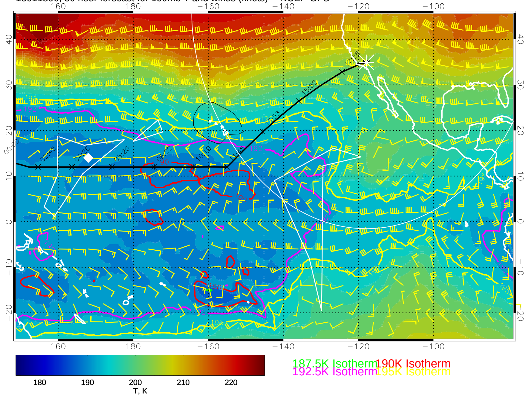
15011806, 30 hour forecast for 100mb T and winds (knots) -- NCEP GFS
