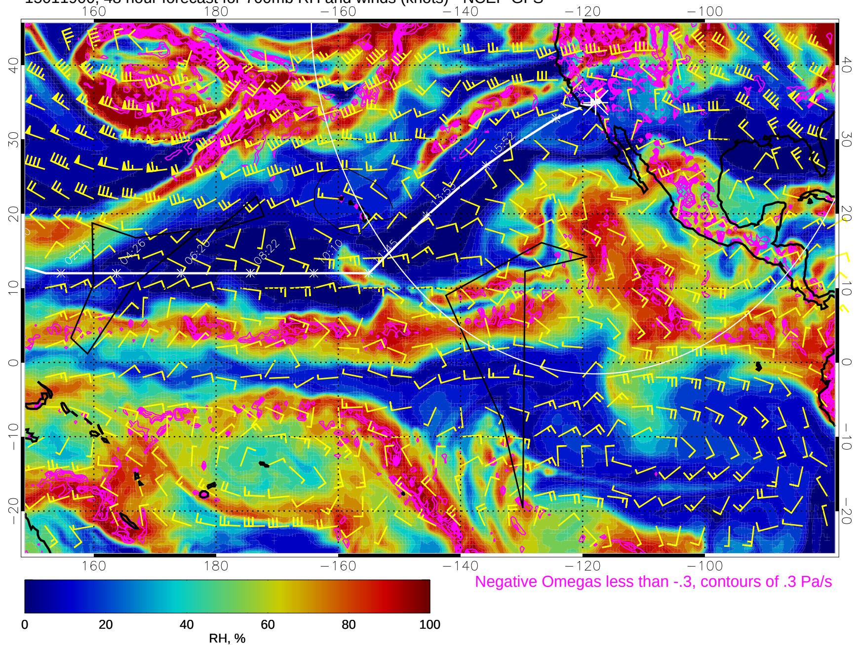
15011900, 48 hour forecast for 700mb RH and winds (knots) - NCEP GFS
