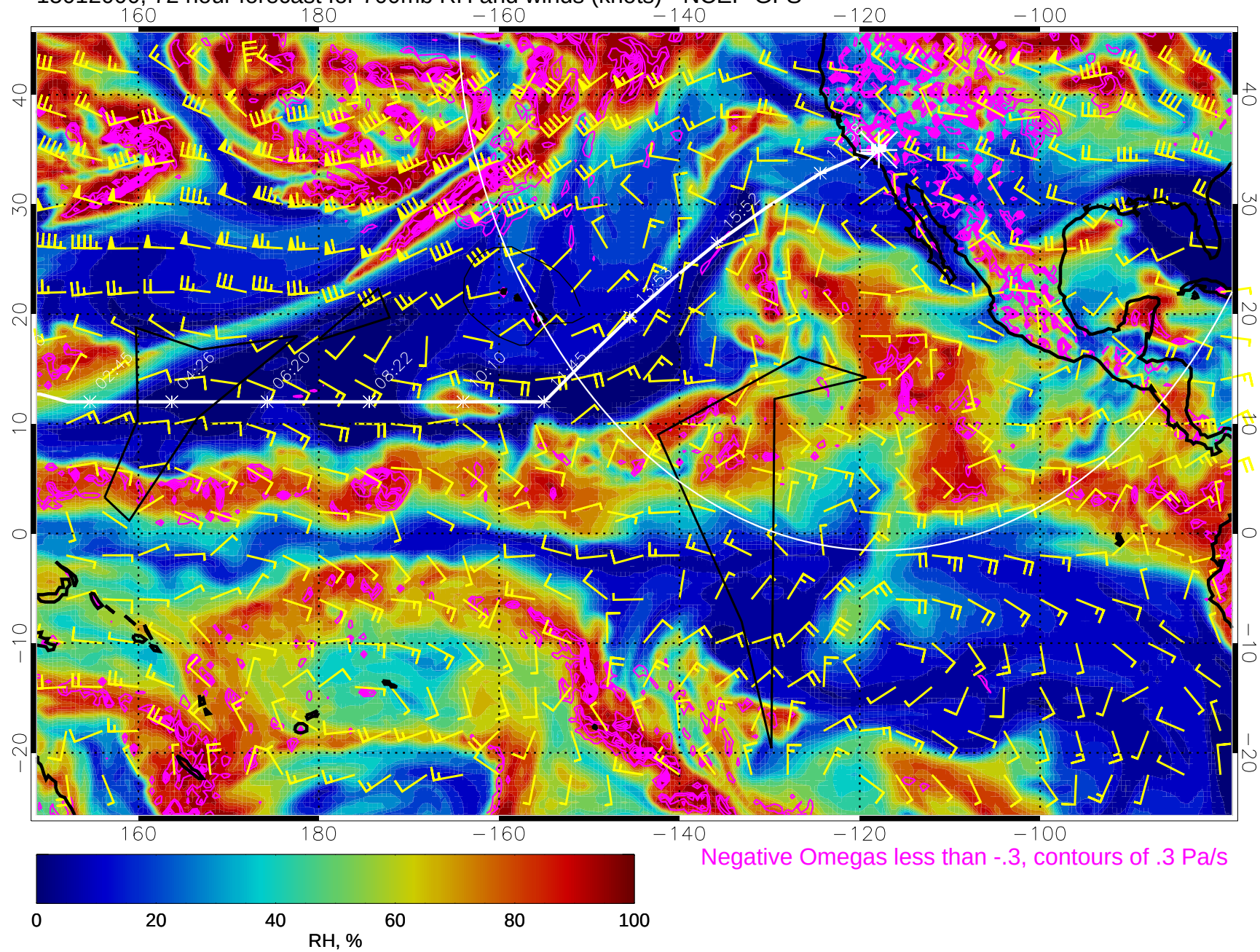
15012000, 72 hour forecast for 700mb RH and winds (knots) - NCEP GFS
