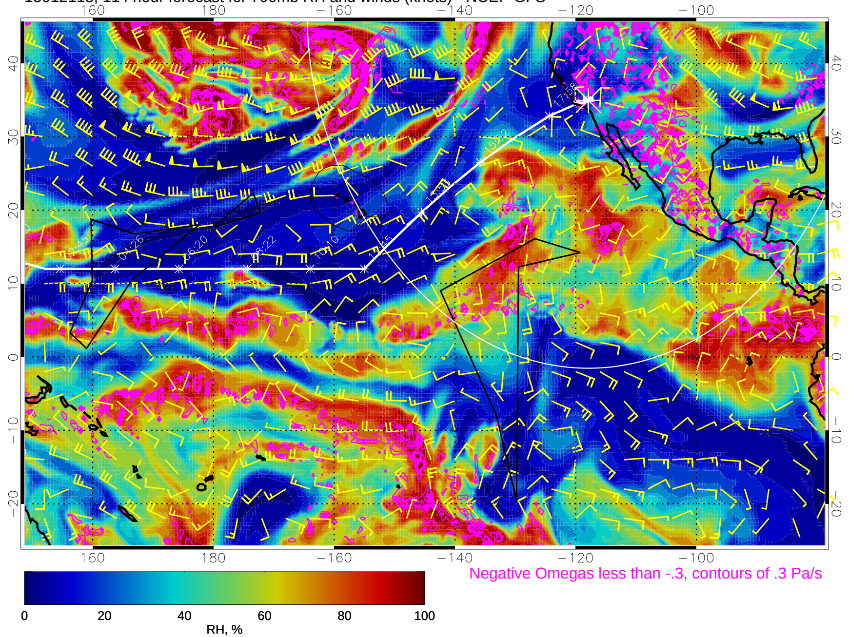
15012118, 114 hour forecast for 700mb RH and winds (knots) - NCEP GFS
