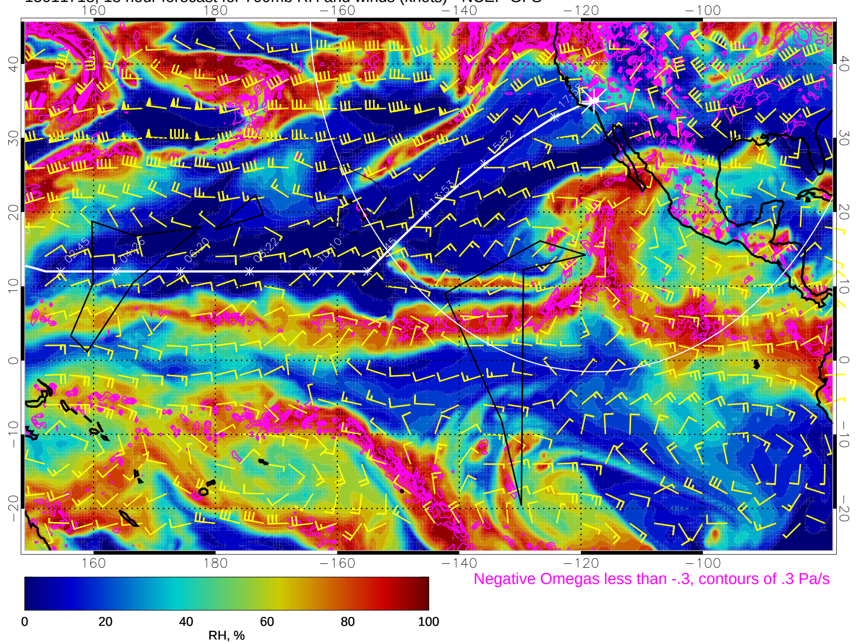
15011718, 18 hour forecast for 700mb RH and winds (knots) - NCEP GFS
