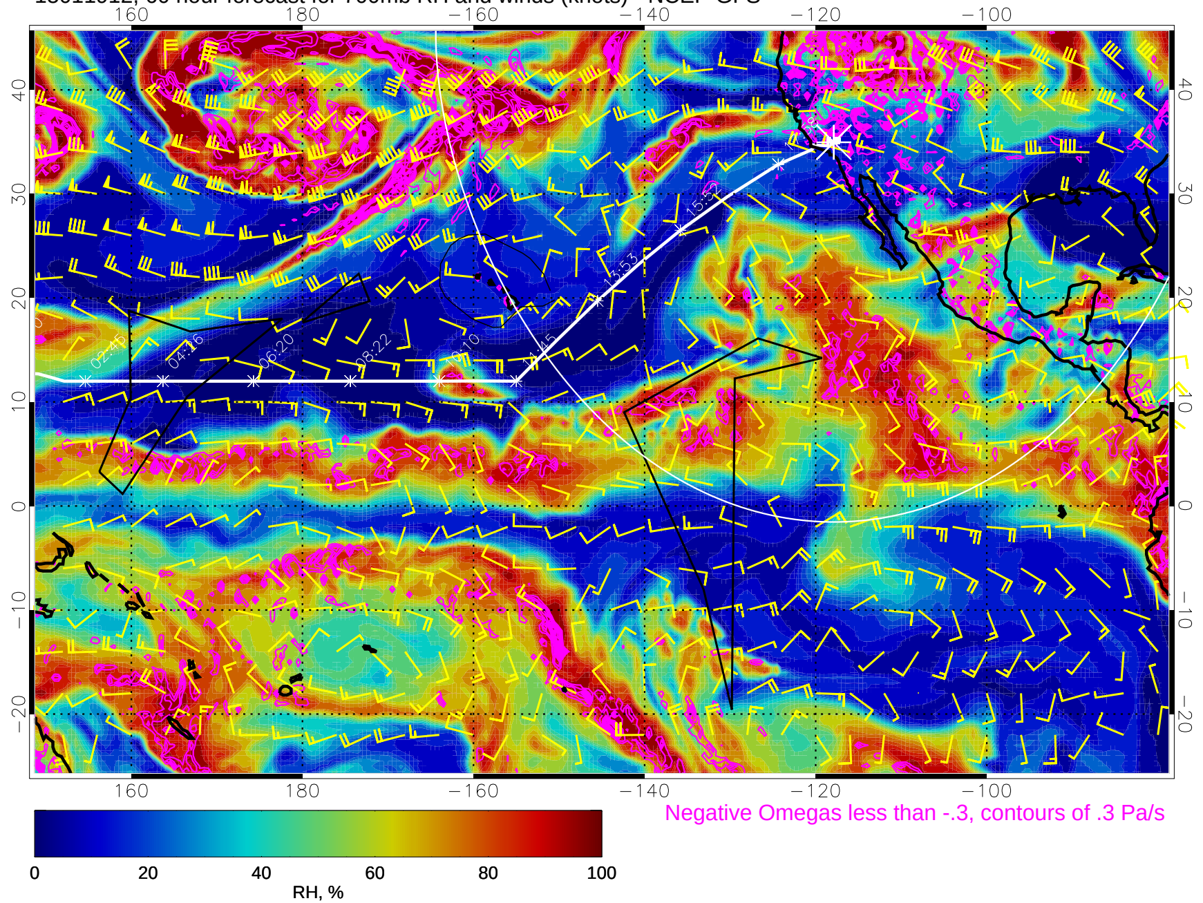
15011912, 60 hour forecast for 700mb RH and winds (knots) - NCEP GFS
