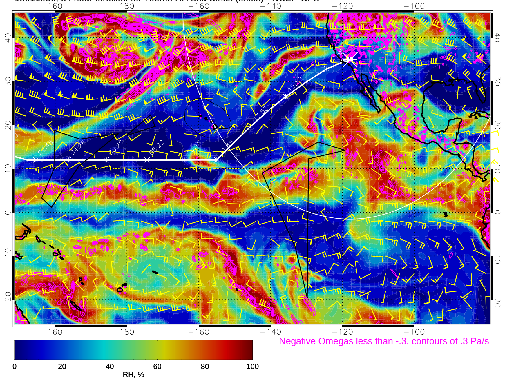
15011906, 54 hour forecast for 700mb RH and winds (knots) - NCEP GFS
