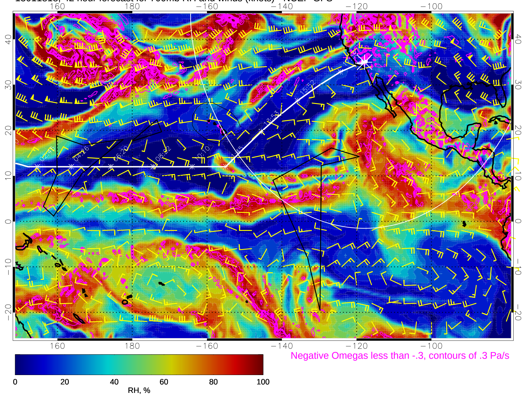
15011818, 42 hour forecast for 700mb RH and winds (knots) - NCEP GFS
