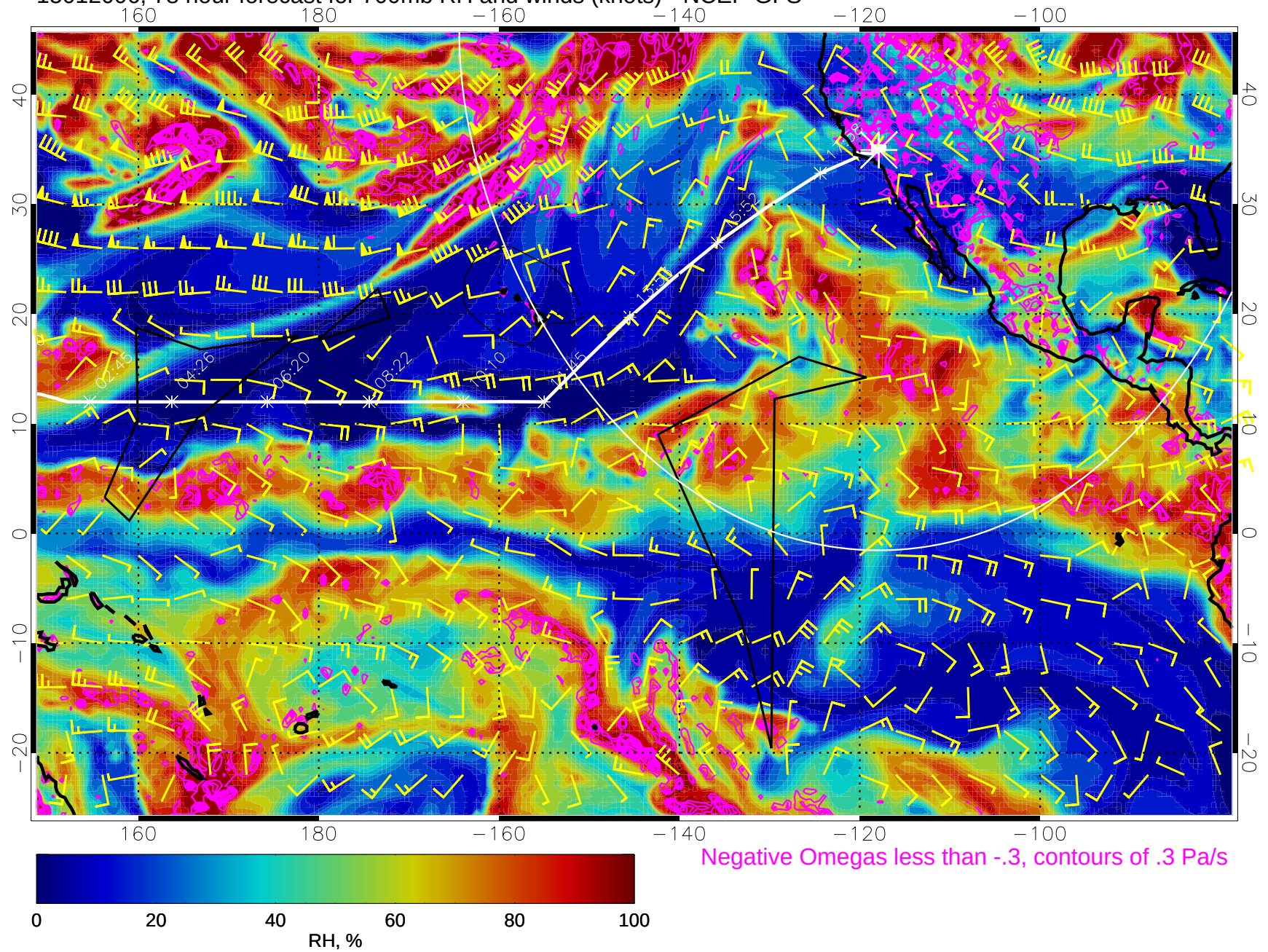
15012006, 78 hour forecast for 700mb RH and winds (knots) - NCEP GFS
