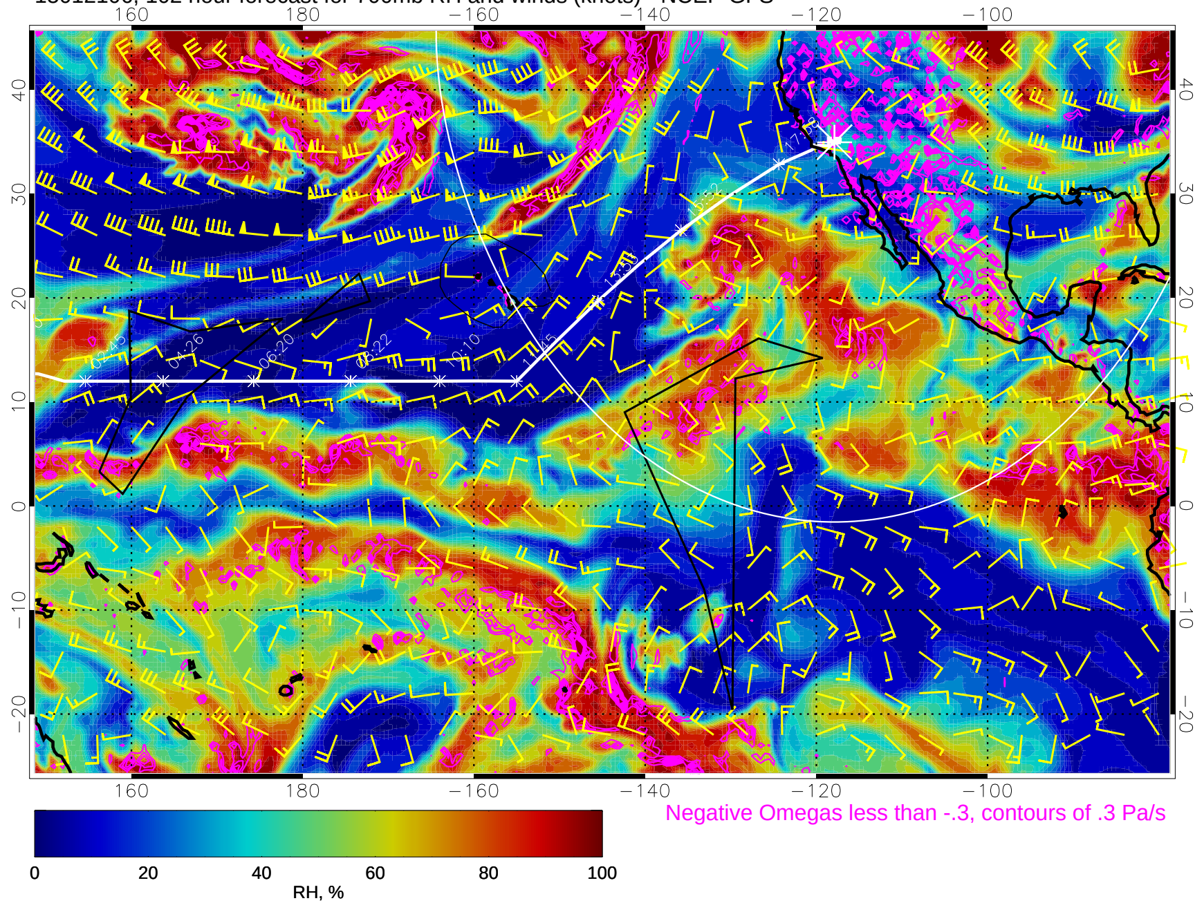
15012106, 102 hour forecast for 700mb RH and winds (knots) - NCEP GFS
