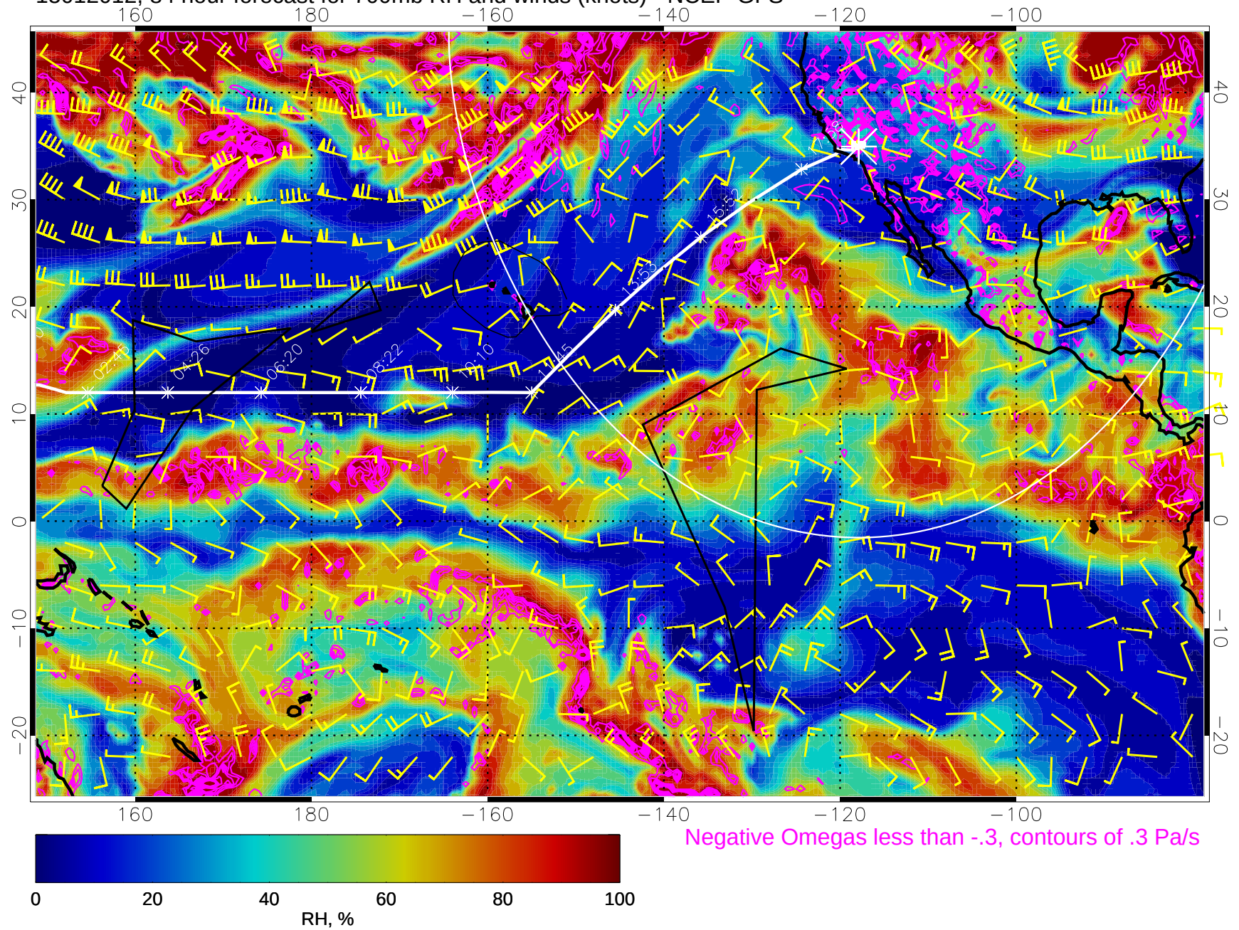
15012012, 84 hour forecast for 700mb RH and winds (knots) - NCEP GFS
