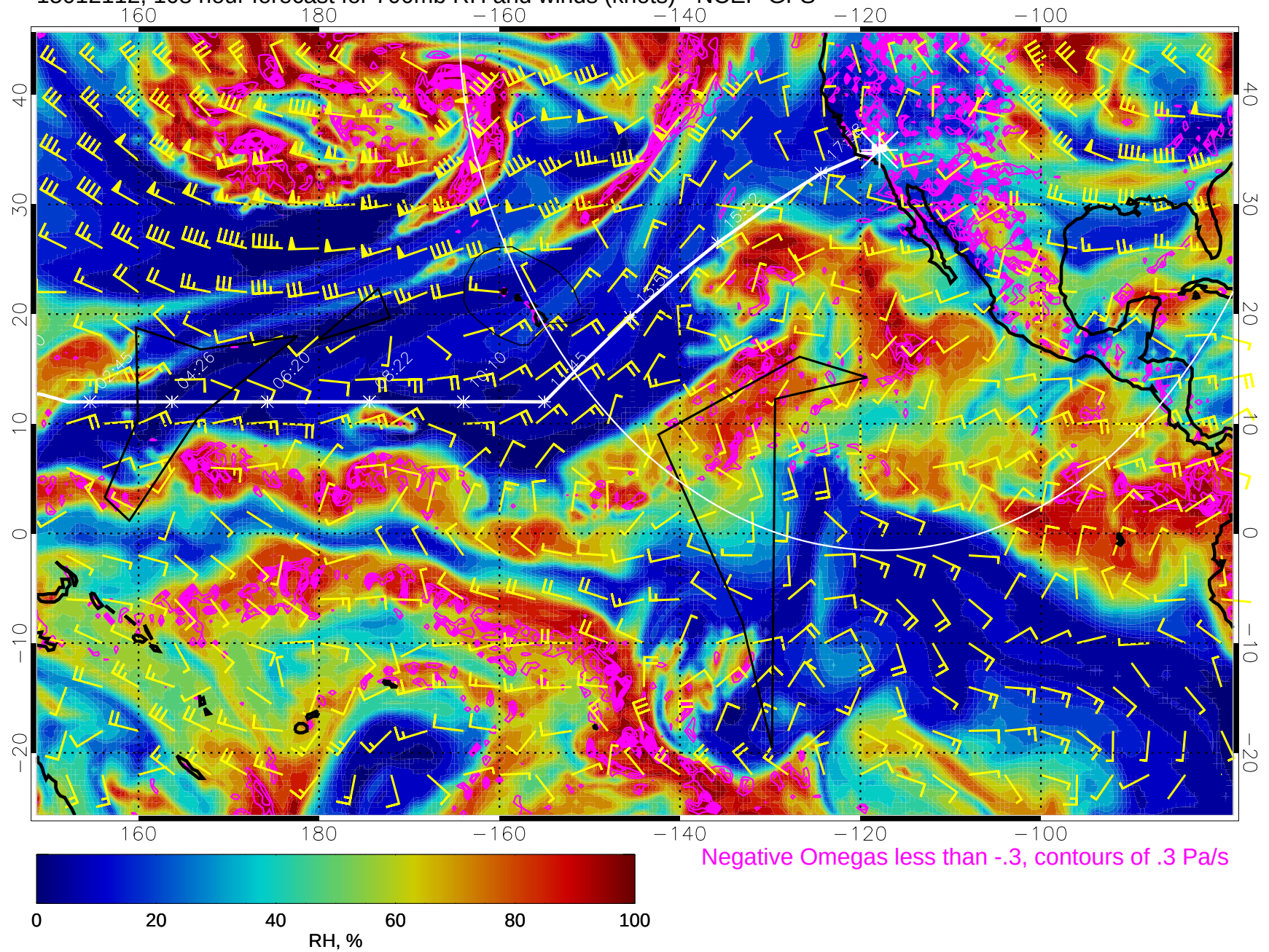
15012112, 108 hour forecast for 700mb RH and winds (knots) - NCEP GFS
