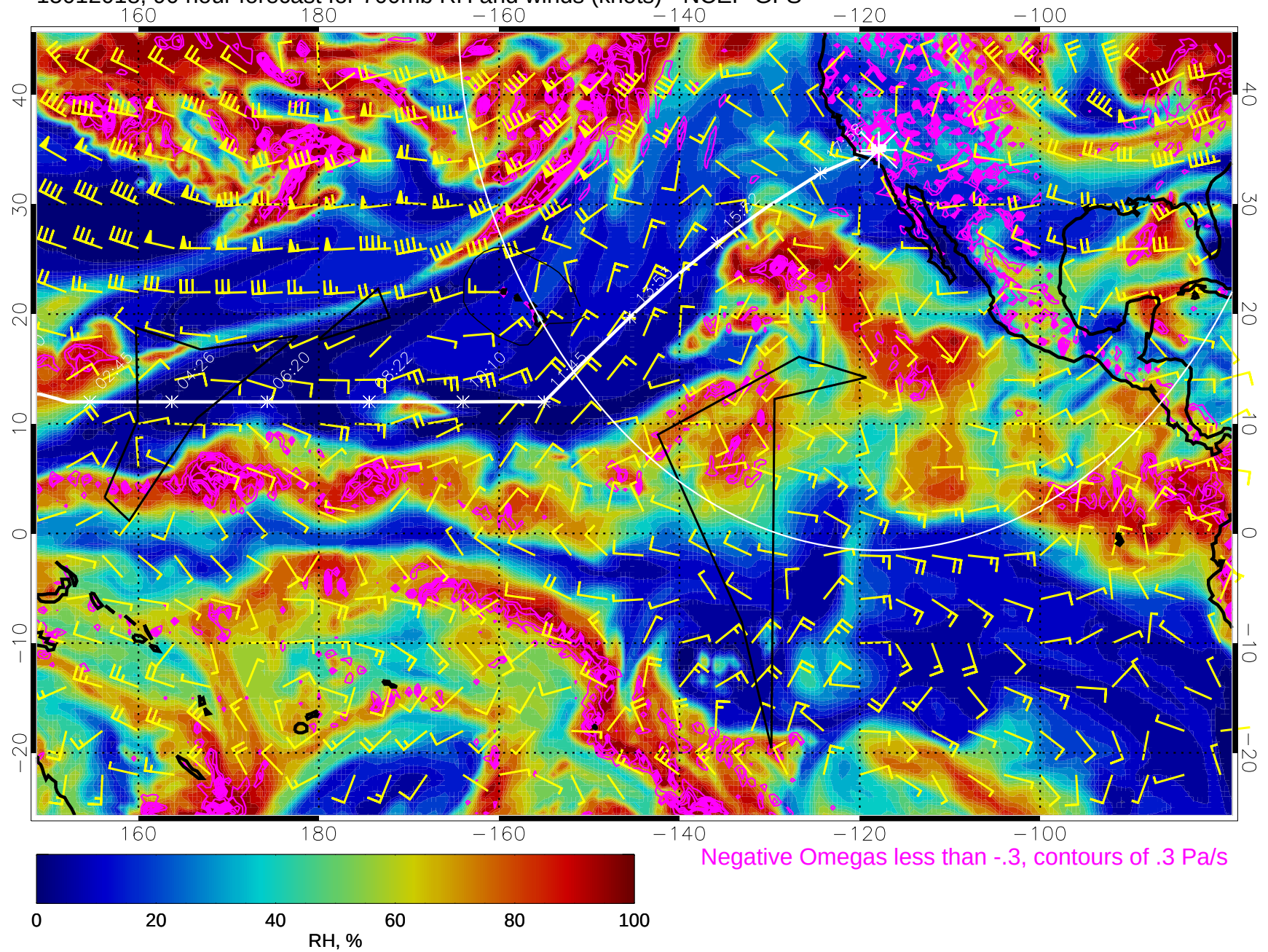
15012018, 90 hour forecast for 700mb RH and winds (knots) - NCEP GFS
