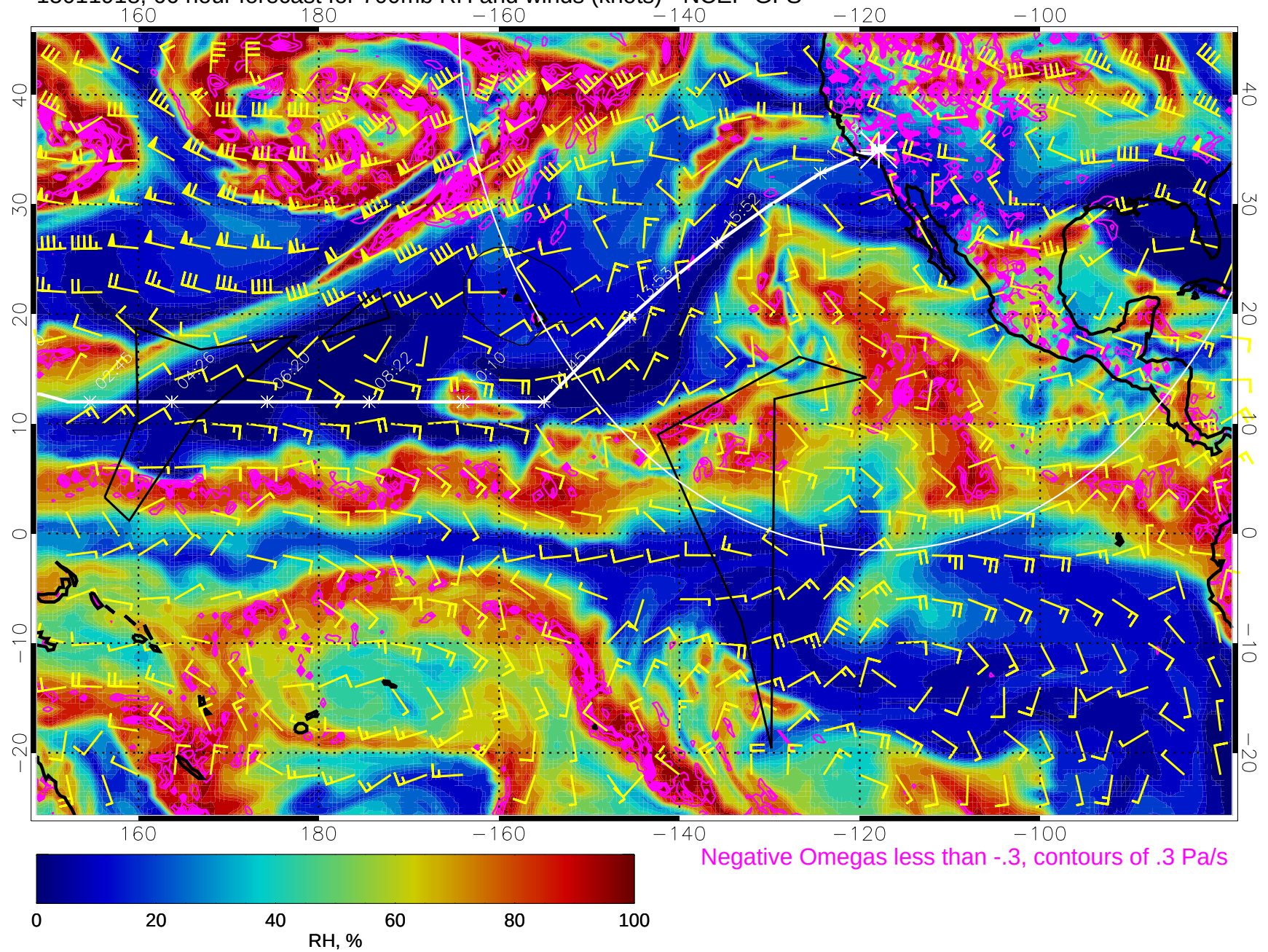
15011918, 66 hour forecast for 700mb RH and winds (knots) - NCEP GFS
