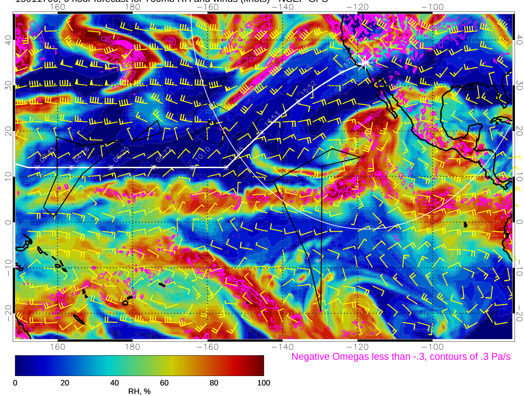
15011706, 6 hour forecast for 700mb RH and winds (knots) - NCEP GFS
