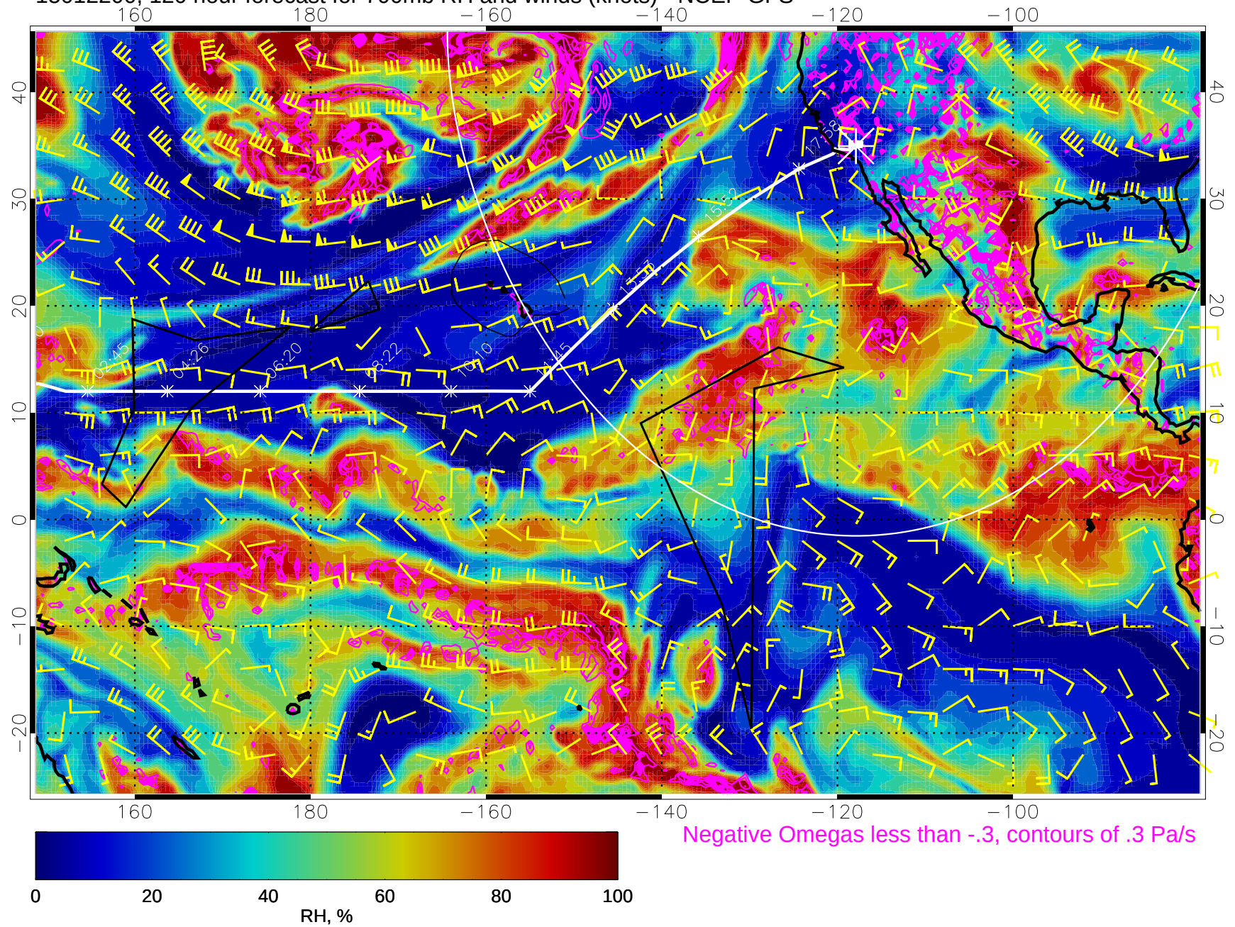
15012200, 120 hour forecast for 700mb RH and winds (knots) - NCEP GFS
