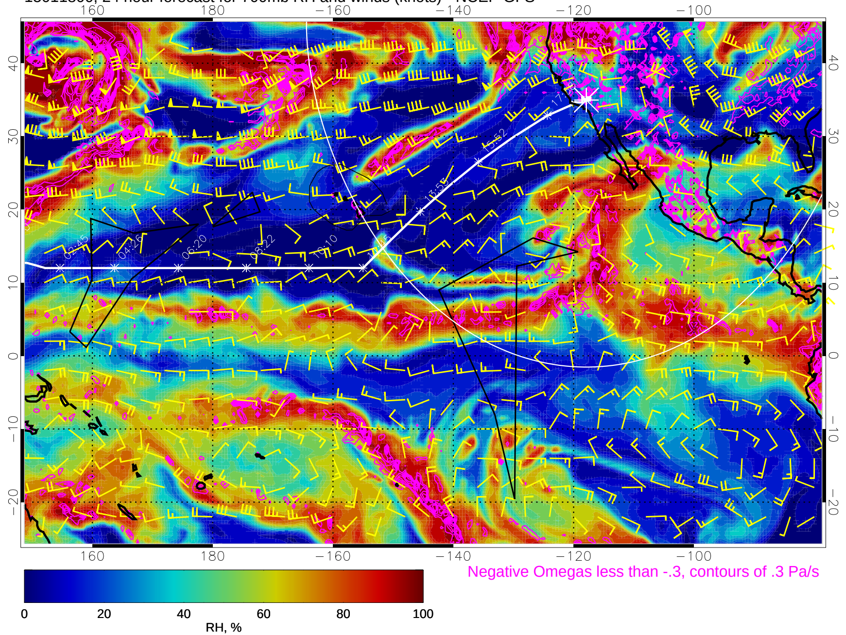
15011800, 24 hour forecast for 700mb RH and winds (knots) - NCEP GFS
