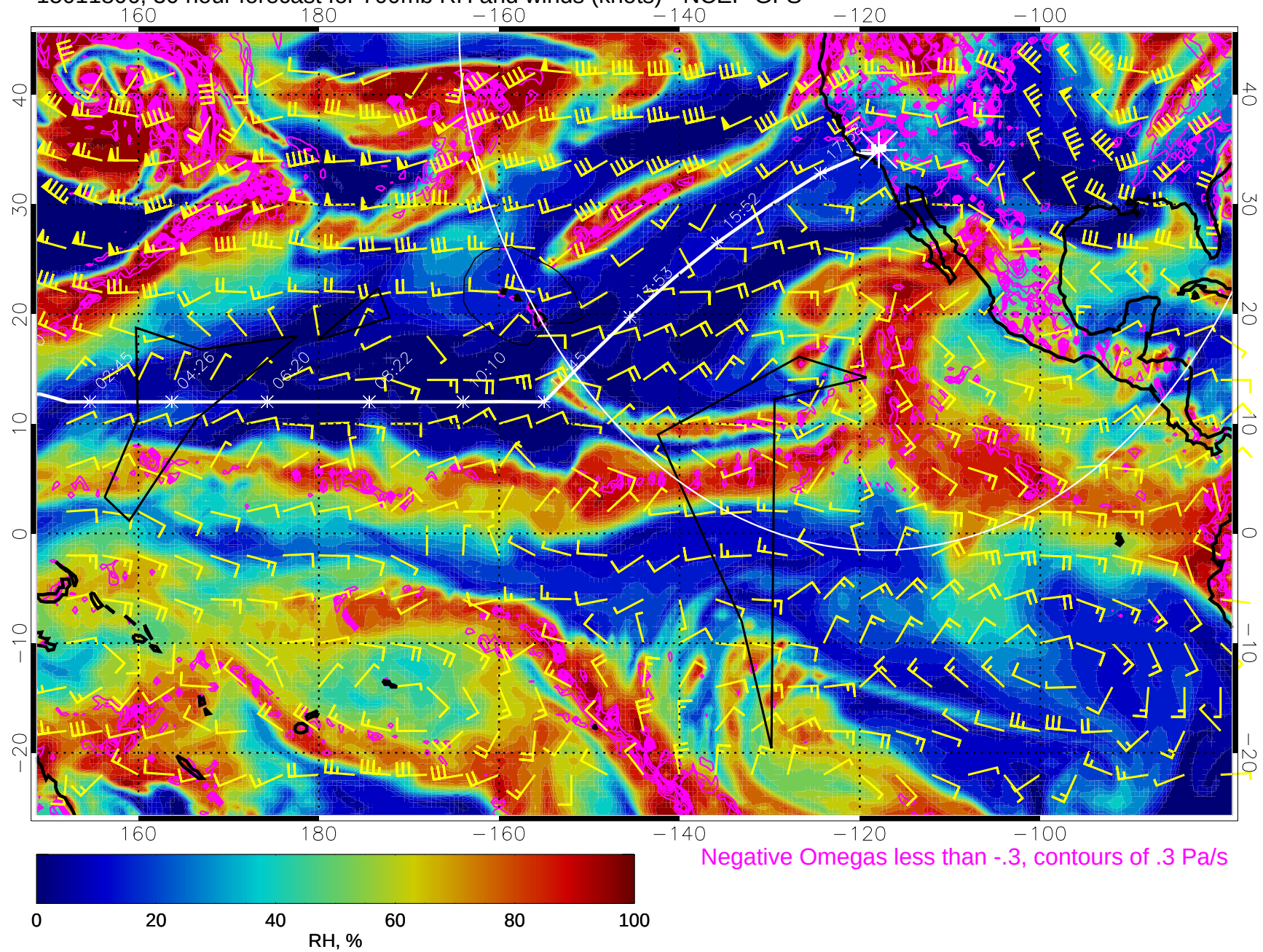
15011806, 30 hour forecast for 700mb RH and winds (knots) - NCEP GFS
