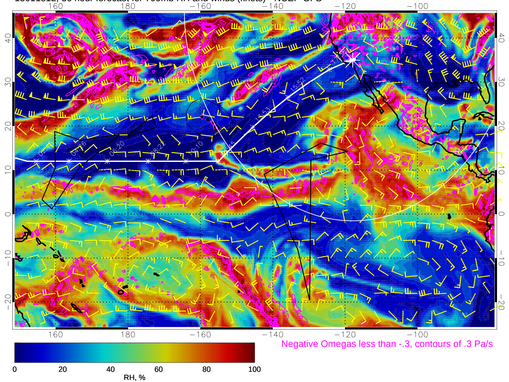
15011812, 36 hour forecast for 700mb RH and winds (knots) - NCEP GFS
