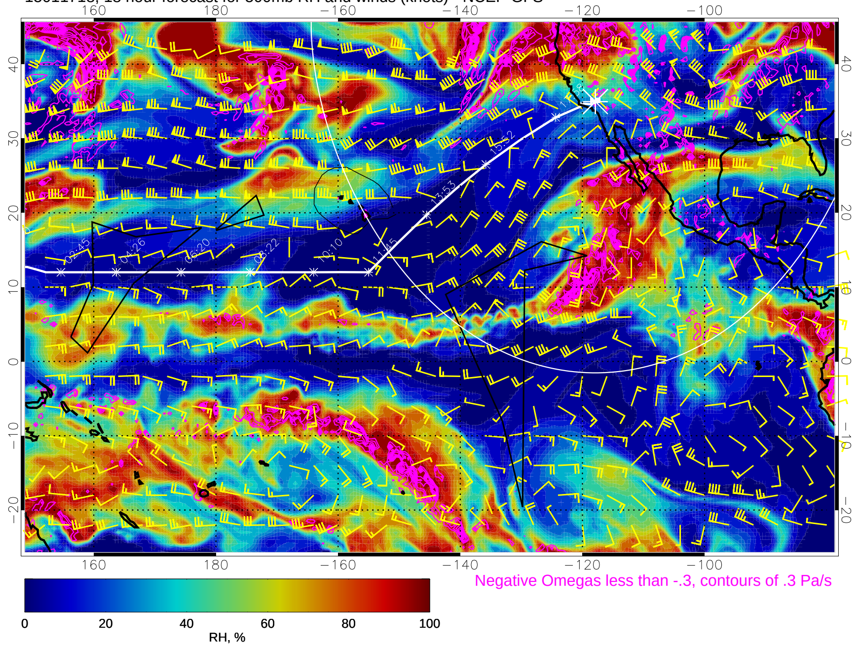
15011718, 18 hour forecast for 500mb RH and winds (knots) - NCEP GFS
