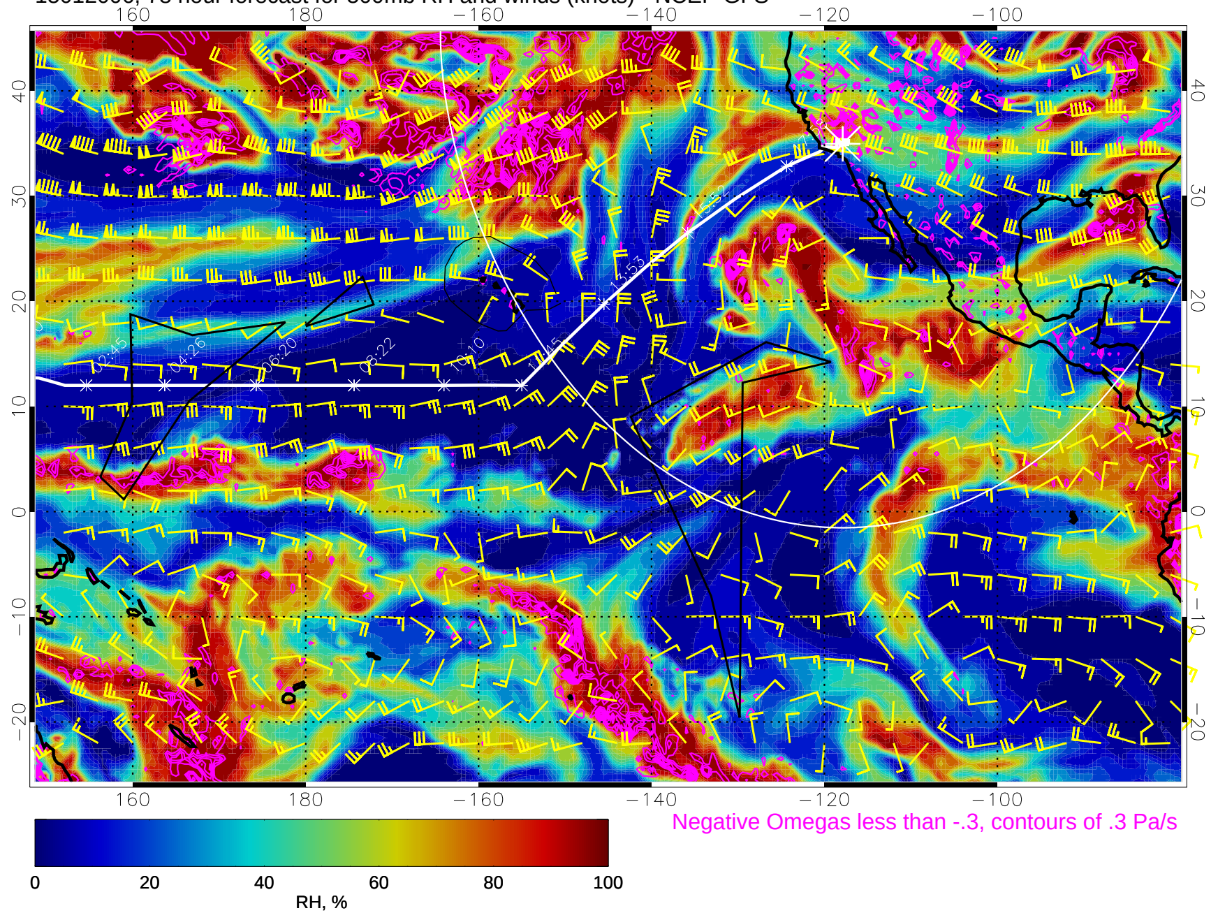
15012006, 78 hour forecast for 500mb RH and winds (knots) - NCEP GFS
