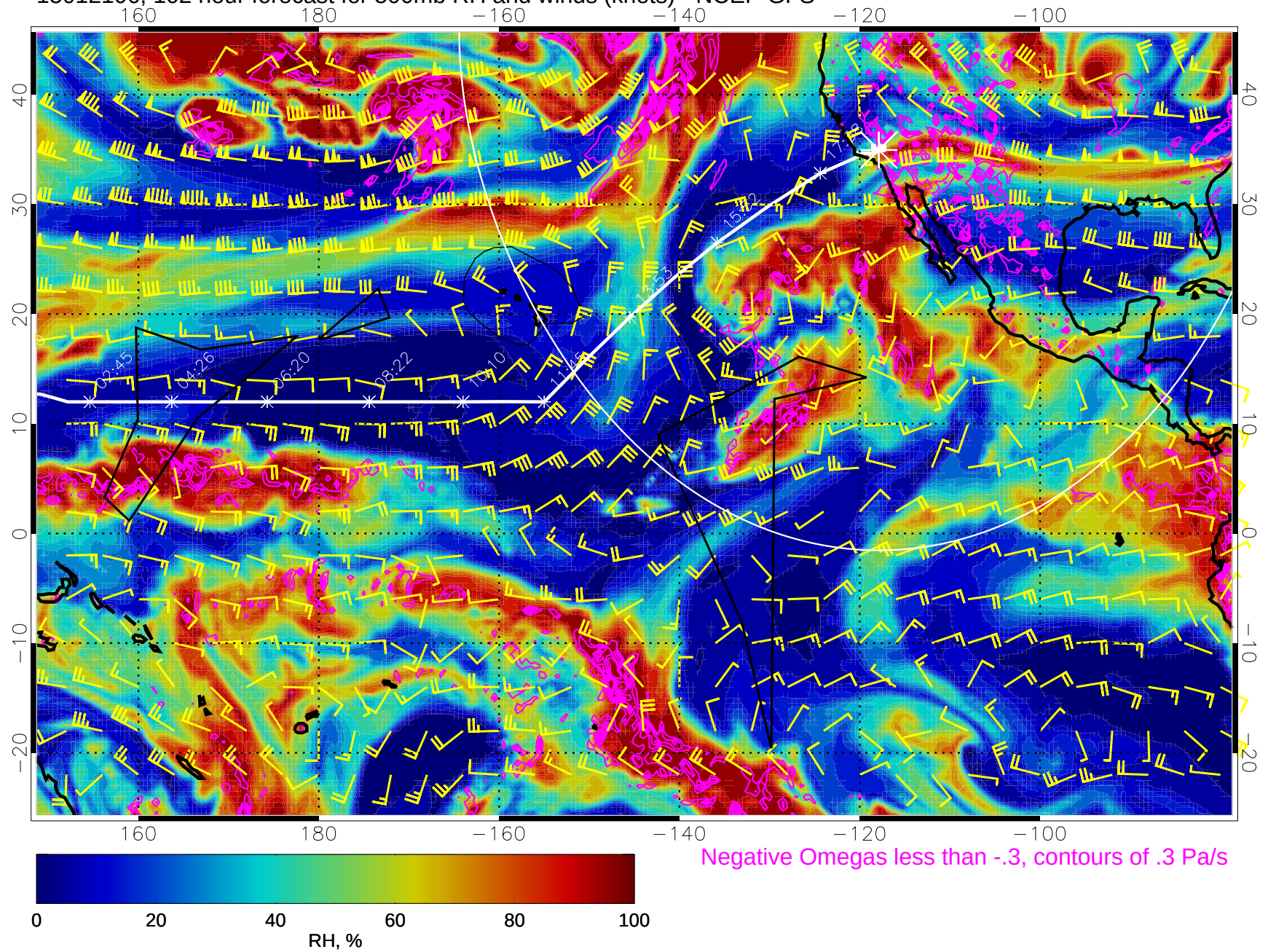
15012106, 102 hour forecast for 500mb RH and winds (knots) - NCEP GFS
