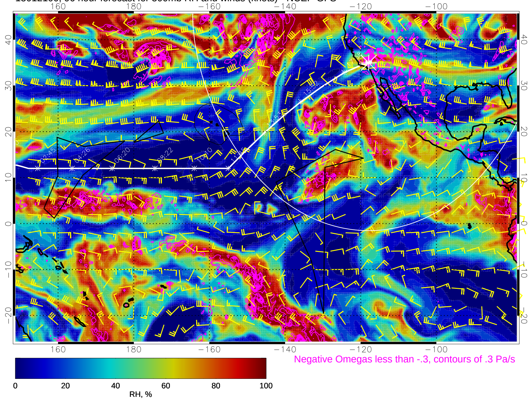
15012100, 96 hour forecast for 500mb RH and winds (knots) - NCEP GFS
