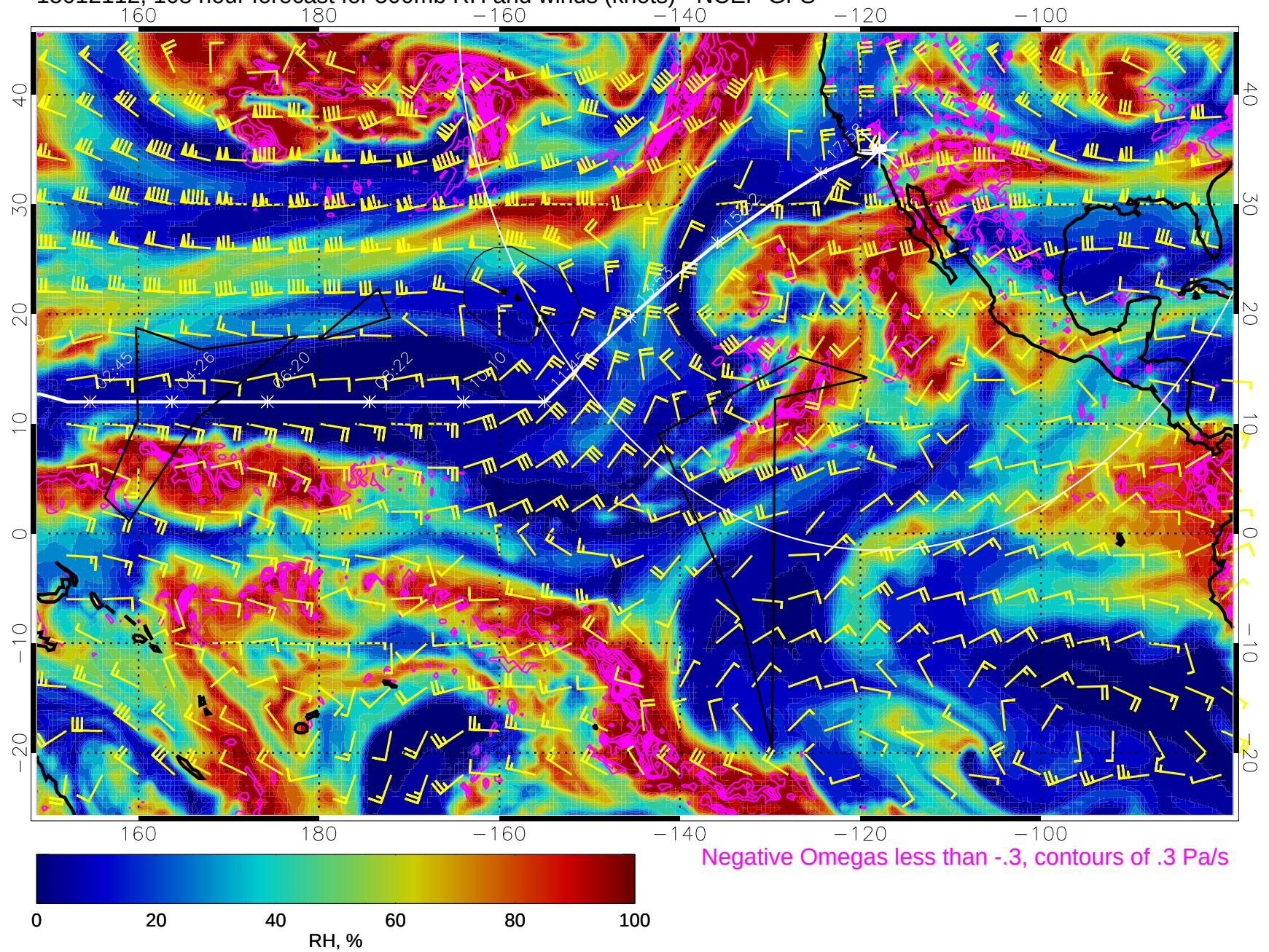
15012112, 108 hour forecast for 500mb RH and winds (knots) - NCEP GFS
