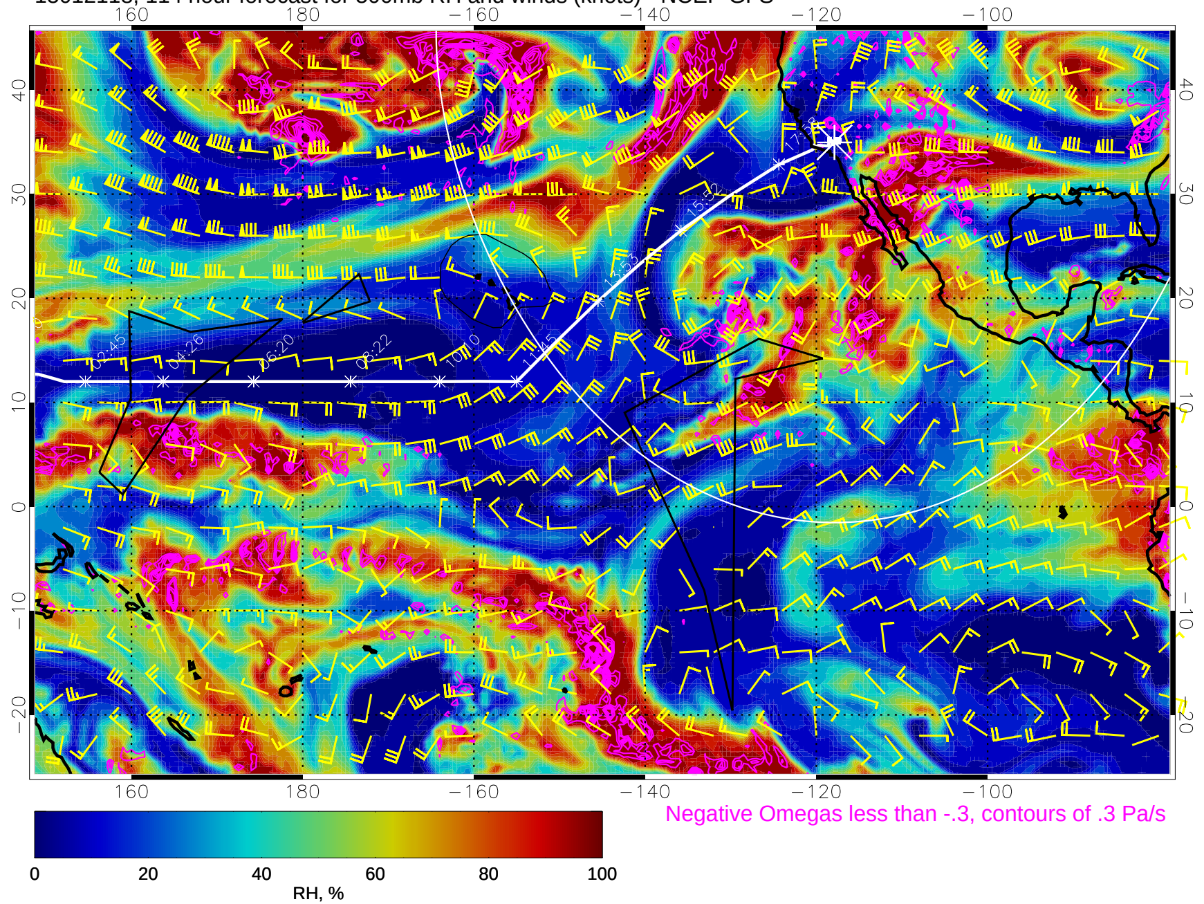
15012118, 114 hour forecast for 500mb RH and winds (knots) - NCEP GFS
