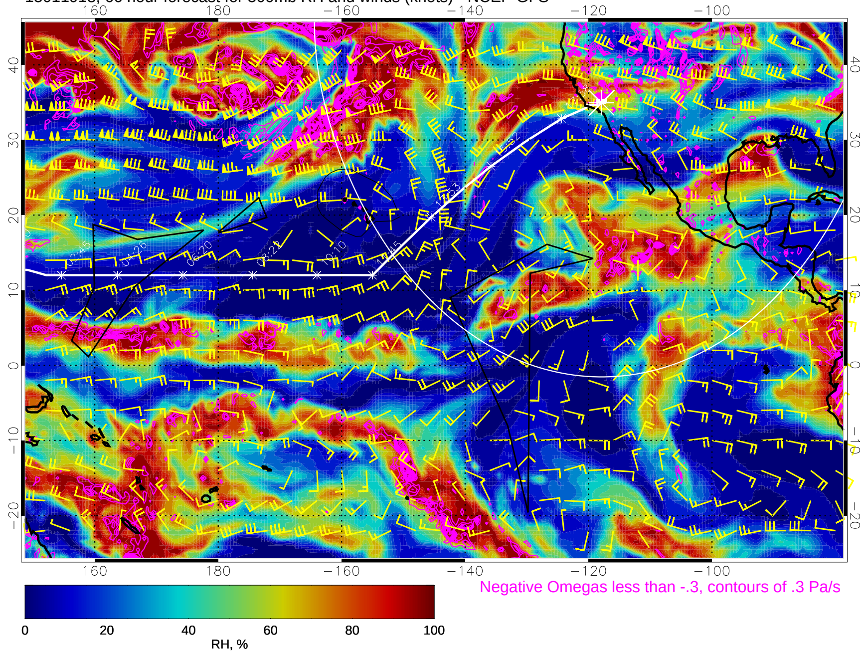
15011918, 66 hour forecast for 500mb RH and winds (knots) - NCEP GFS
