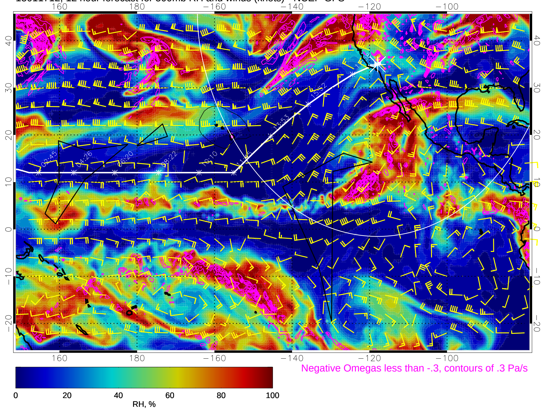
15011712, 12 hour forecast for 500mb RH and winds (knots) - NCEP GFS
