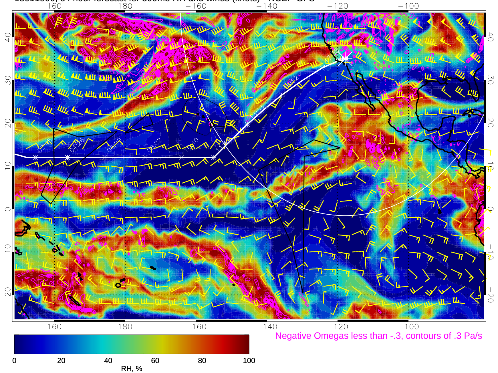
15011906, 54 hour forecast for 500mb RH and winds (knots) - NCEP GFS
