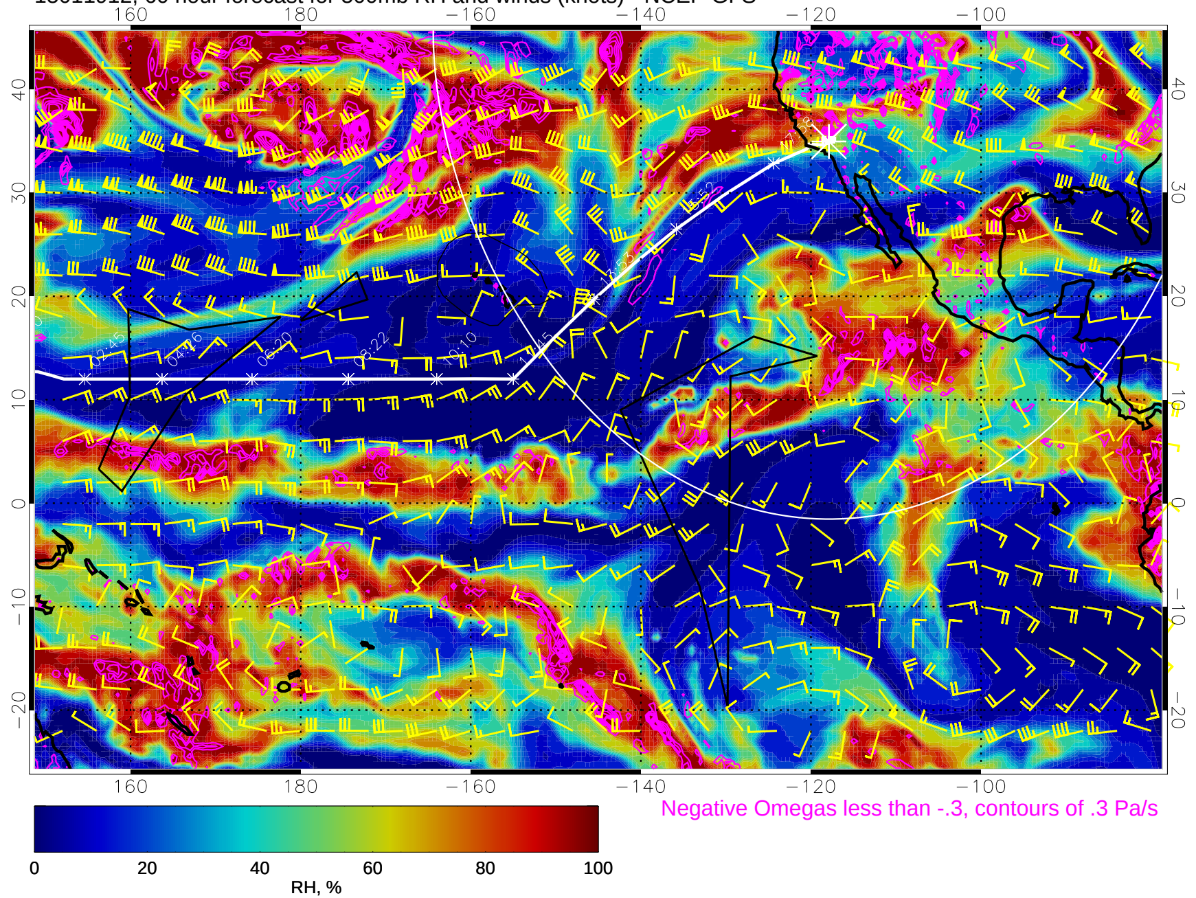
15011912, 60 hour forecast for 500mb RH and winds (knots) - NCEP GFS
