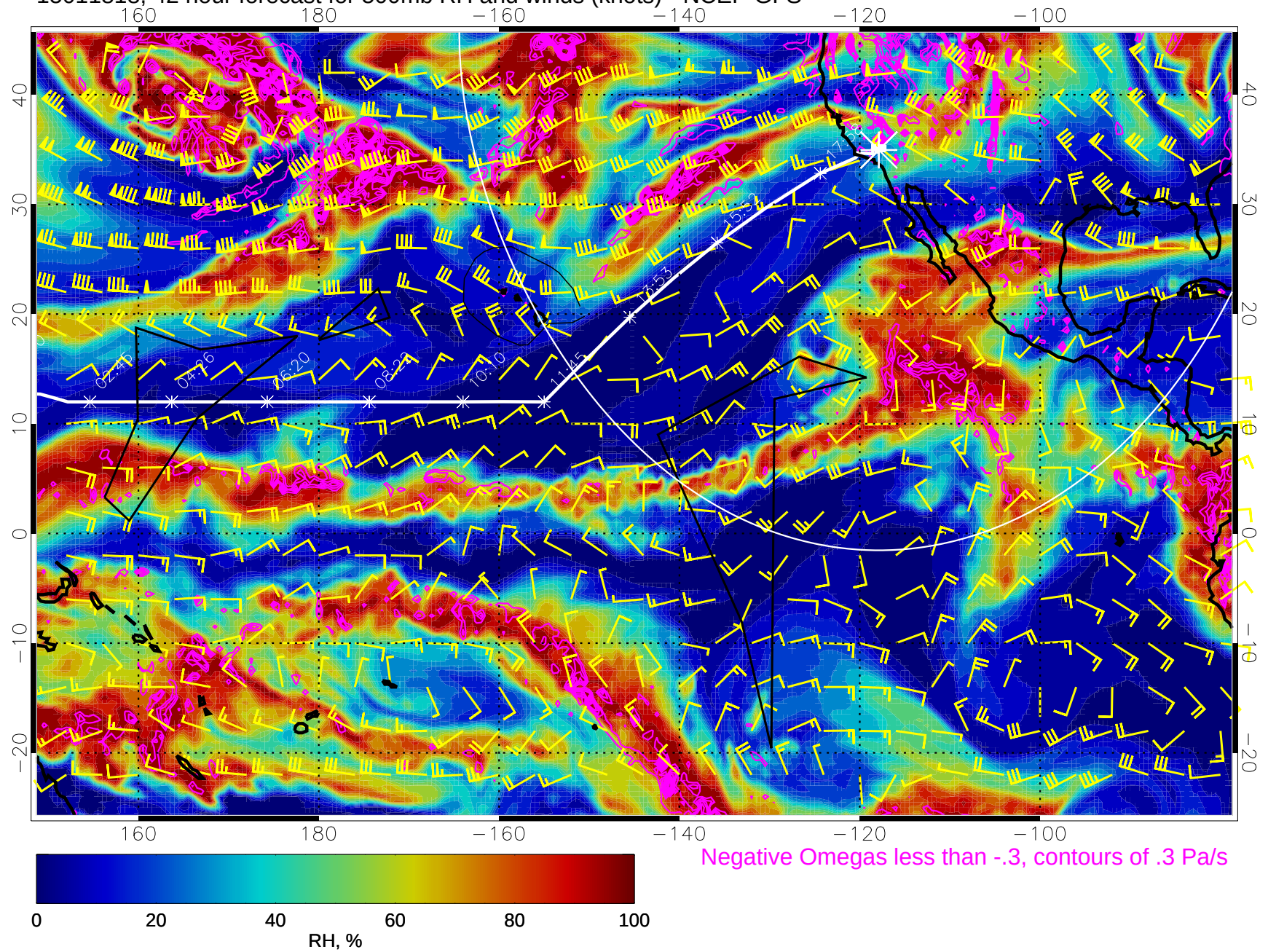
15011818, 42 hour forecast for 500mb RH and winds (knots) - NCEP GFS
