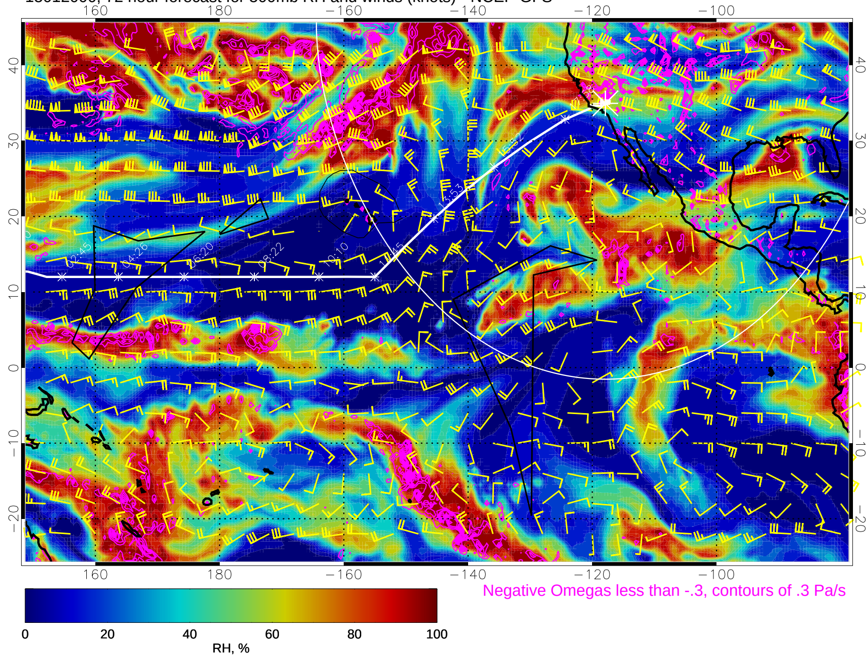
15012000, 72 hour forecast for 500mb RH and winds (knots) - NCEP GFS
