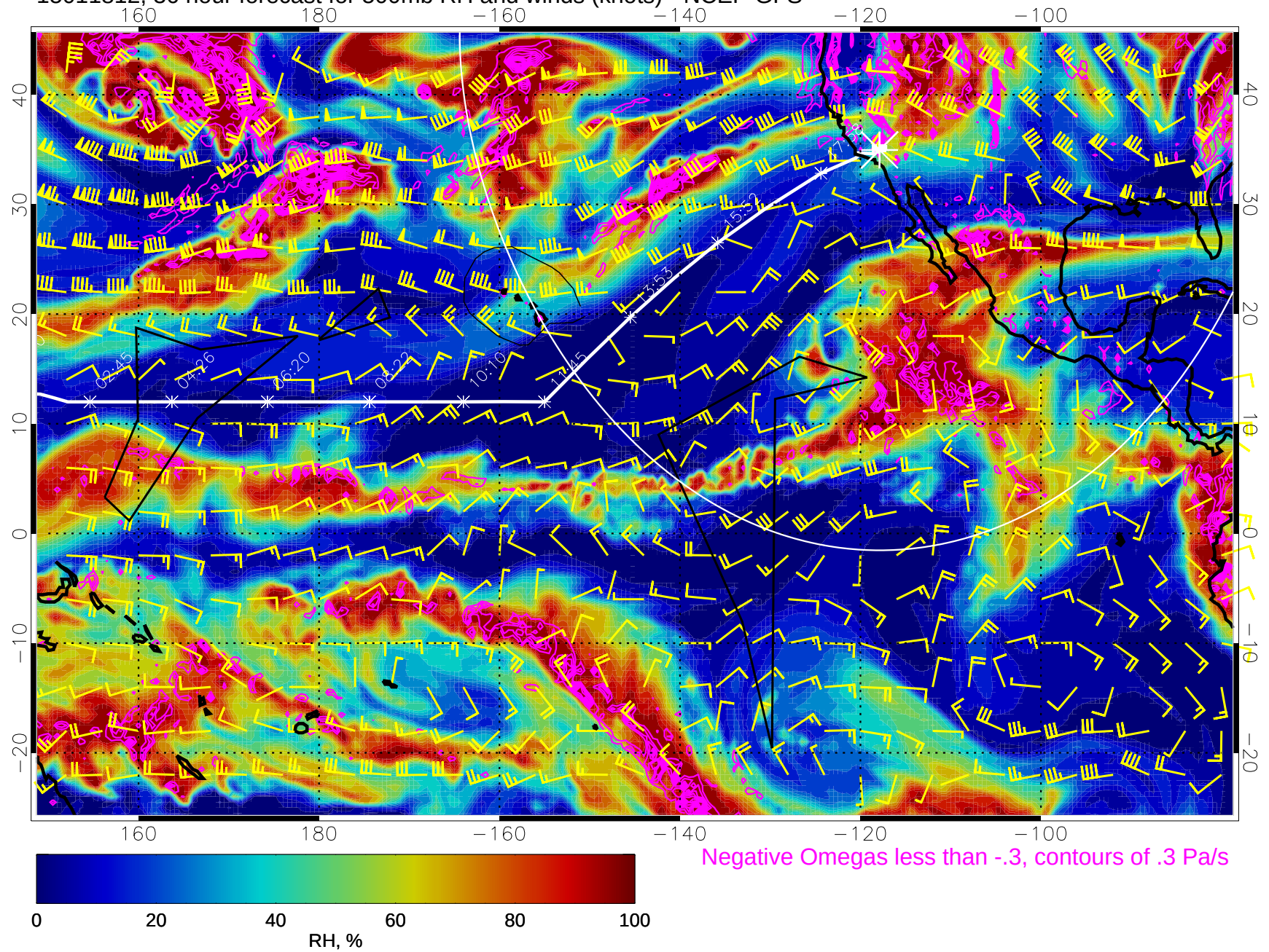
15011812, 36 hour forecast for 500mb RH and winds (knots) - NCEP GFS
