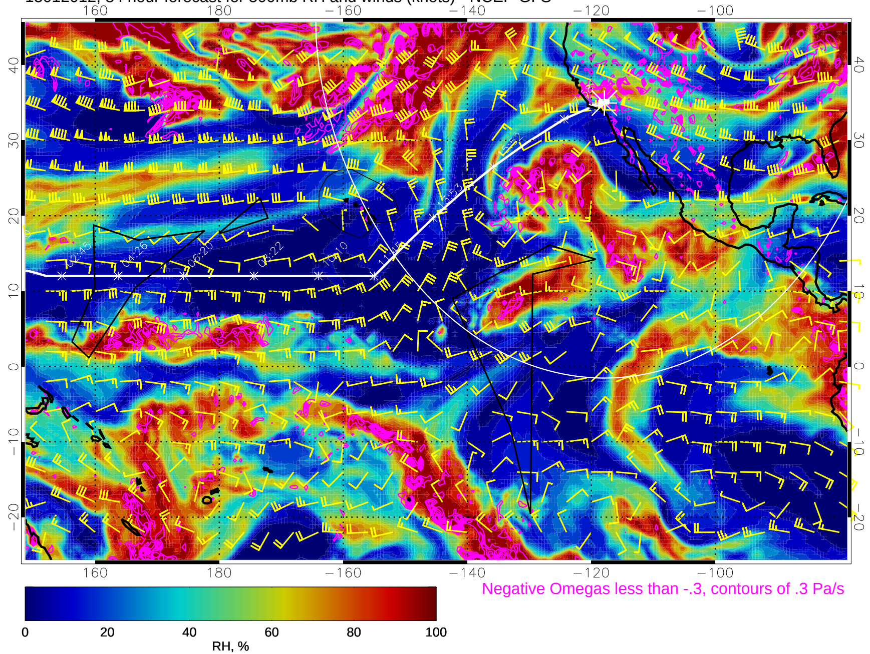
15012012, 84 hour forecast for 500mb RH and winds (knots) - NCEP GFS
