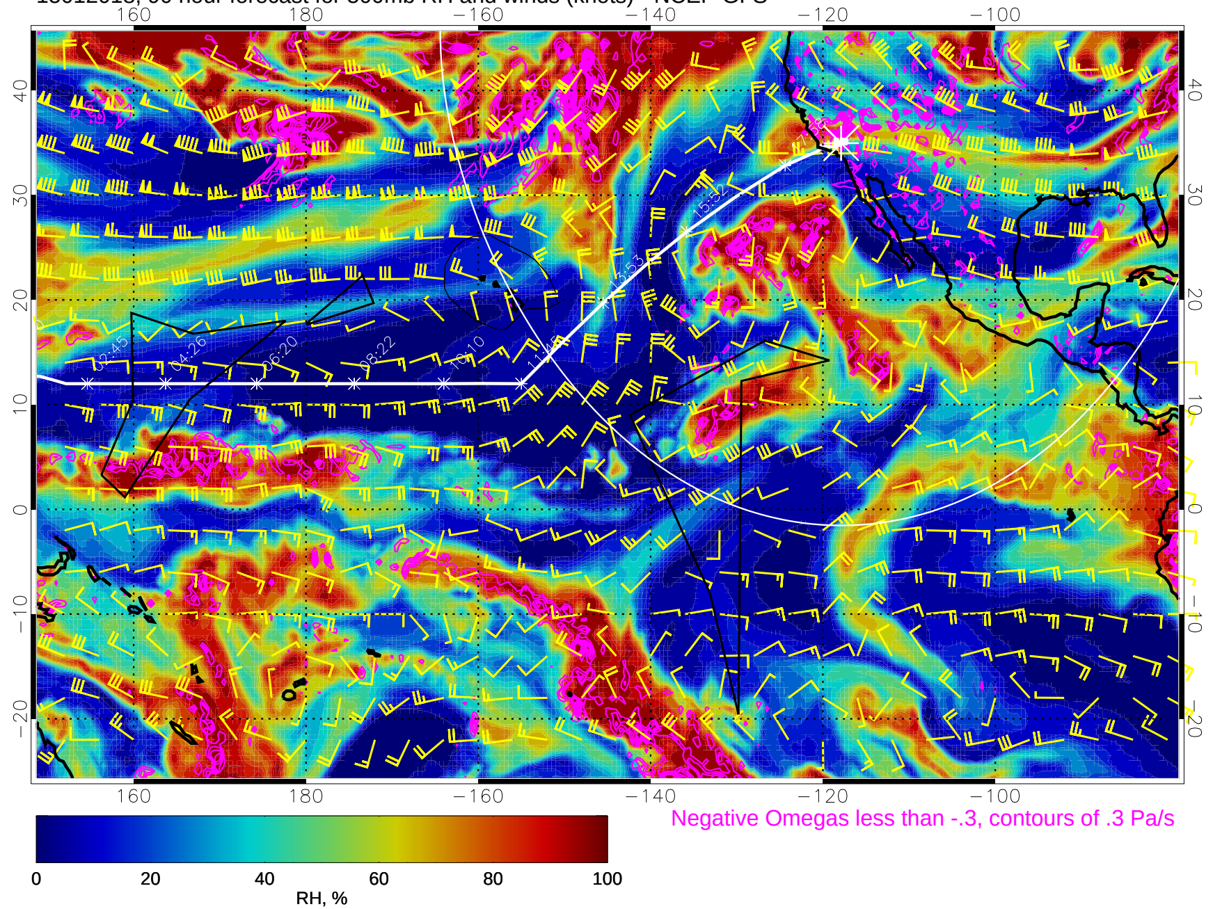
15012018, 90 hour forecast for 500mb RH and winds (knots) - NCEP GFS
