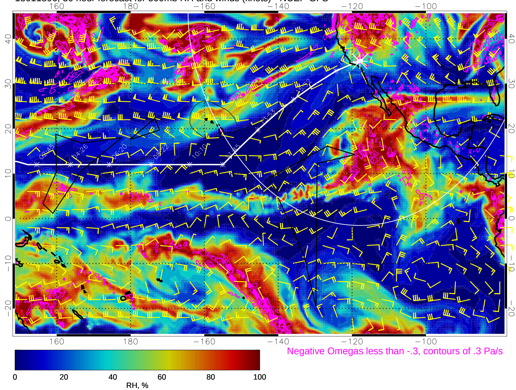
15011806, 30 hour forecast for 500mb RH and winds (knots) - NCEP GFS
