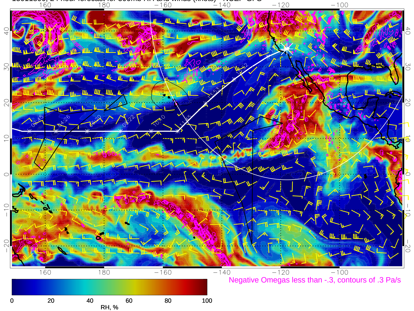
15011800, 24 hour forecast for 500mb RH and winds (knots) - NCEP GFS
