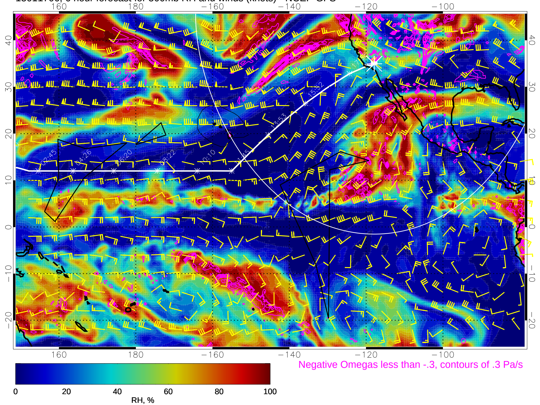
15011706, 6 hour forecast for 500mb RH and winds (knots) - NCEP GFS
