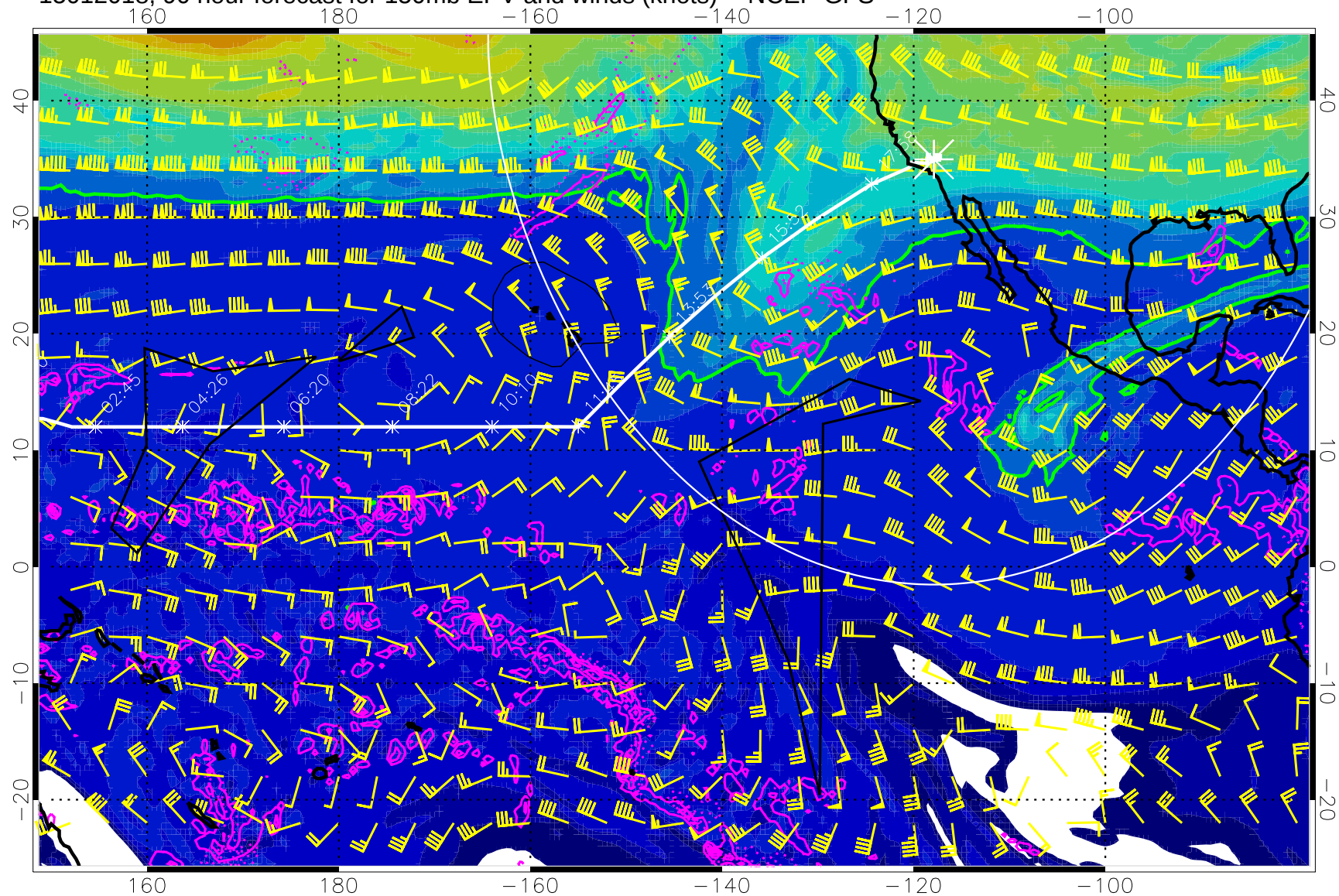
15012018, 90 hour forecast for 150mb EPV and winds (knots) -- NCEP GFS
