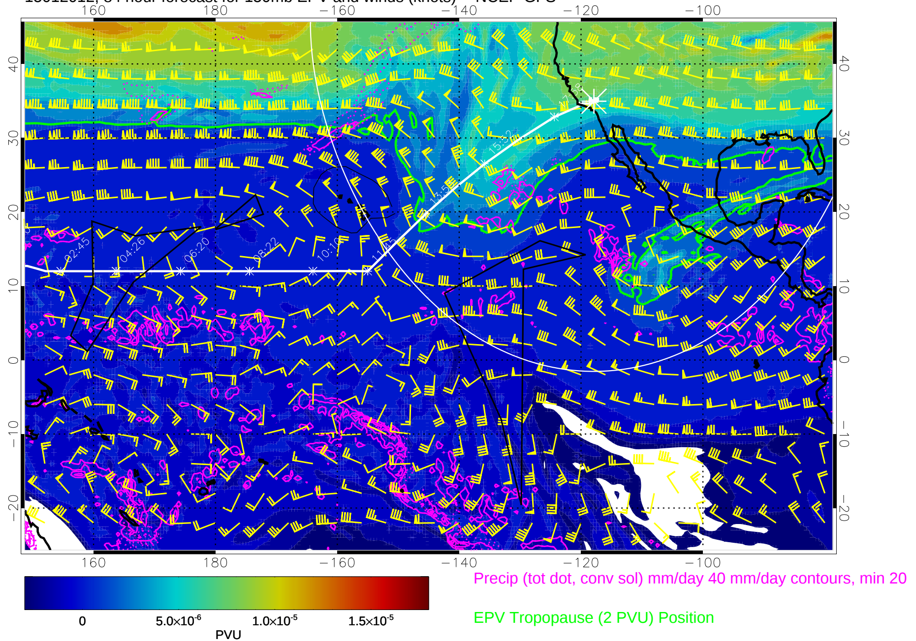
15012012, 84 hour forecast for 150mb EPV and winds (knots) -- NCEP GFS
