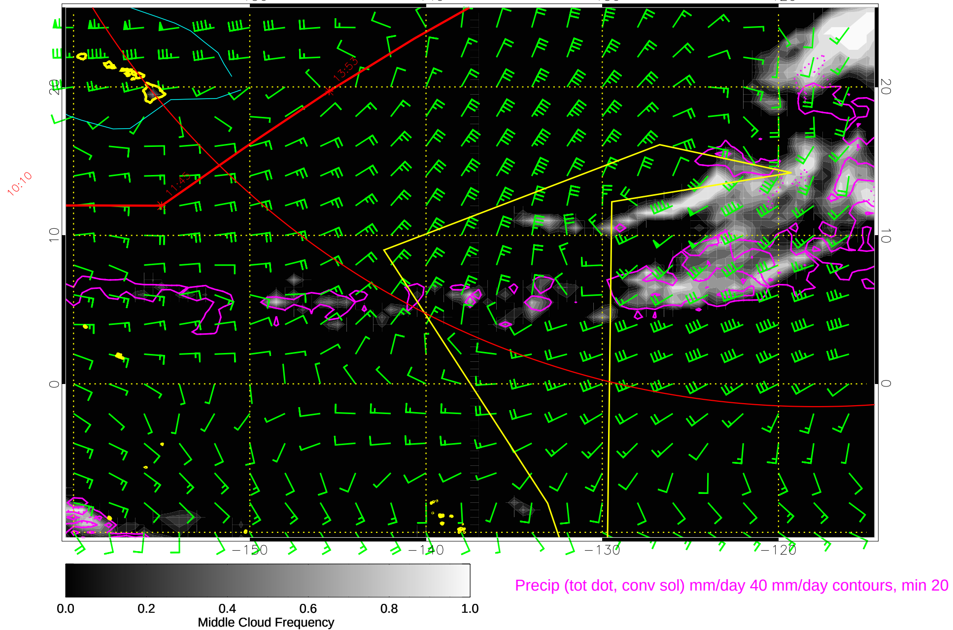
15011706, 6 hour forecast for 500mb winds (knots) and Middle Cloud Frequency -- NCEP GFS
