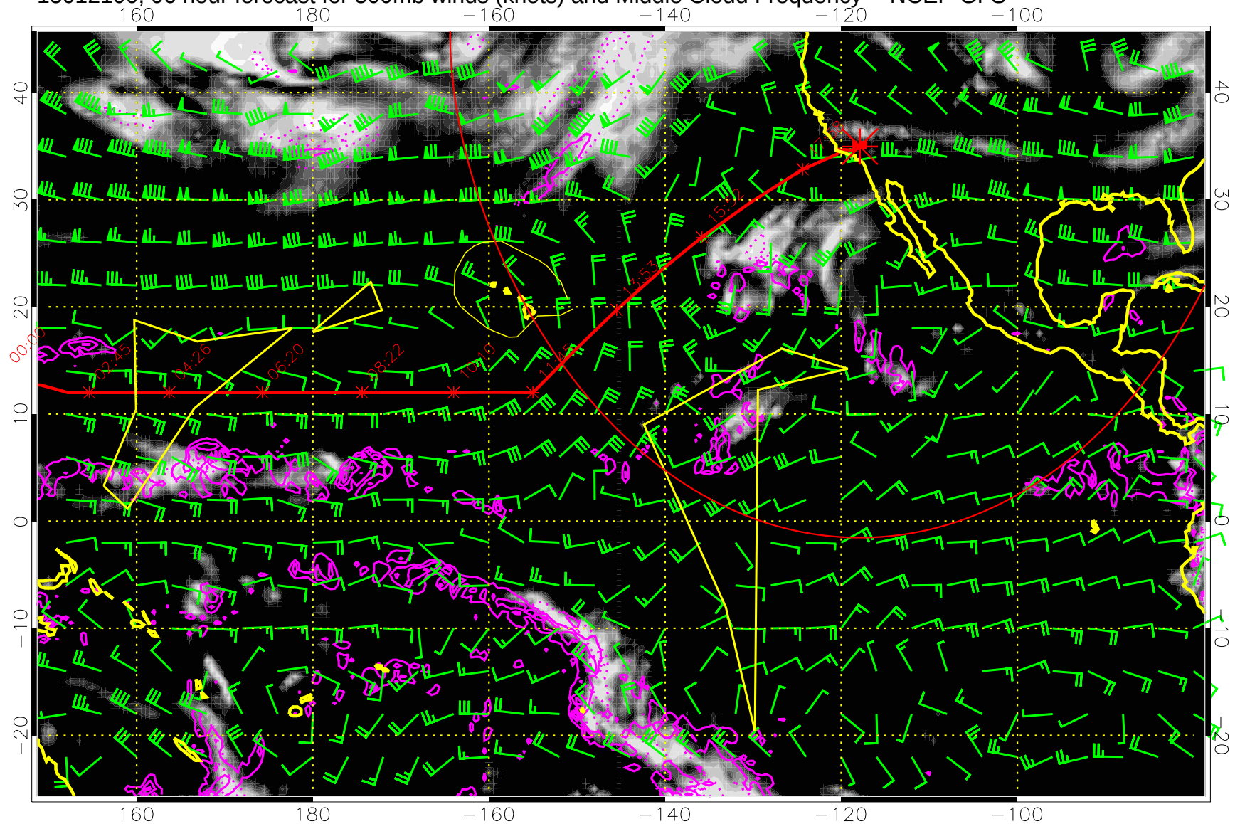
15012100, 96 hour forecast for 500mb winds (knots) and Middle Cloud Frequency -- NCEP GFS
