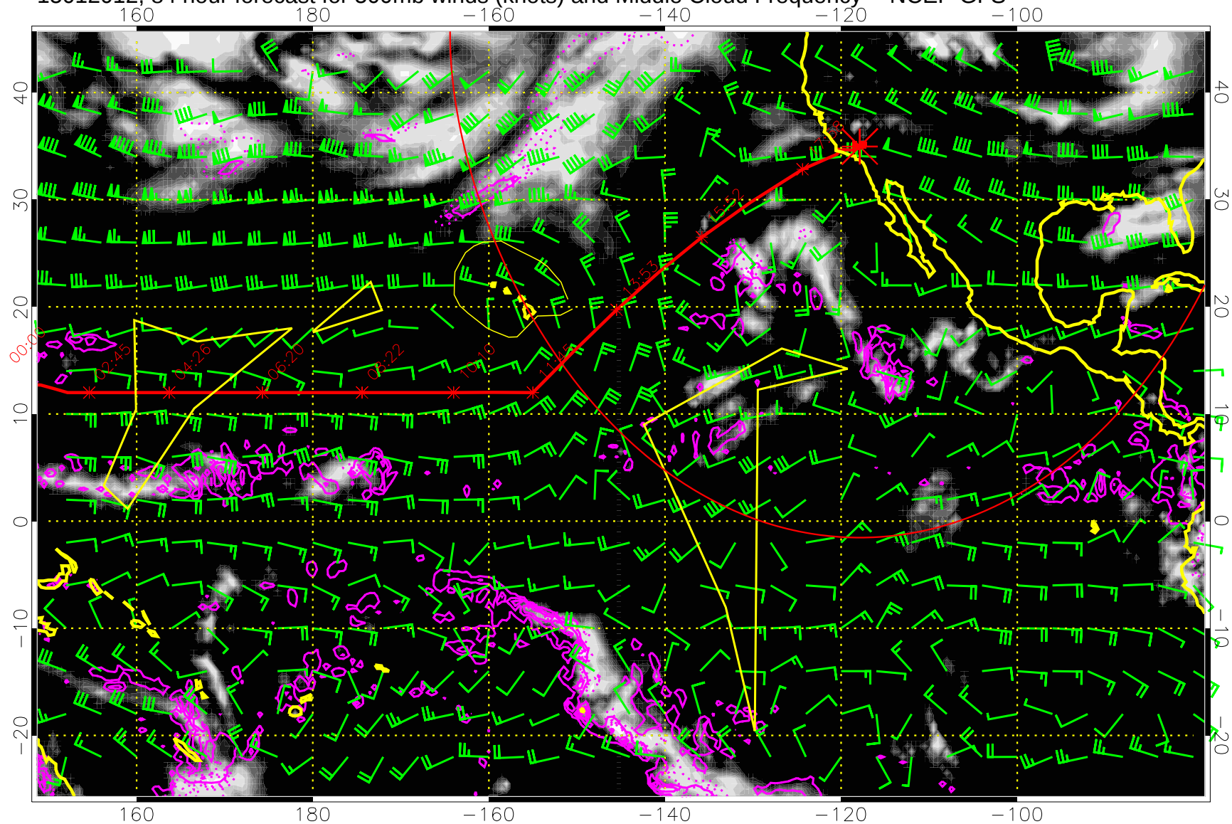
15012012, 84 hour forecast for 500mb winds (knots) and Middle Cloud Frequency -- NCEP GFS
