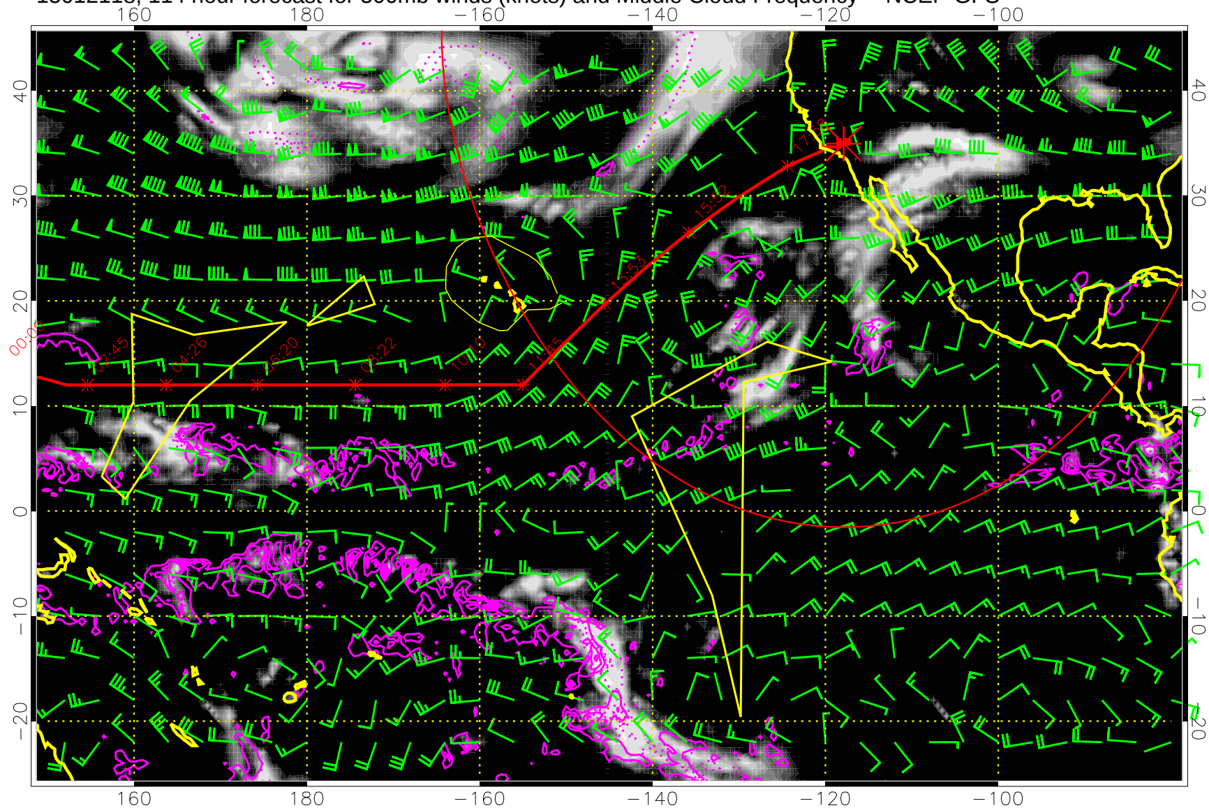
15012118, 114 hour forecast for 500mb winds (knots) and Middle Cloud Frequency -- NCEP GFS
