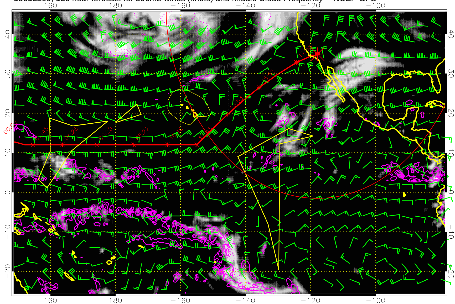
15012200, 120 hour forecast for 500mb winds (knots) and Middle Cloud Frequency -- NCEP GFS
