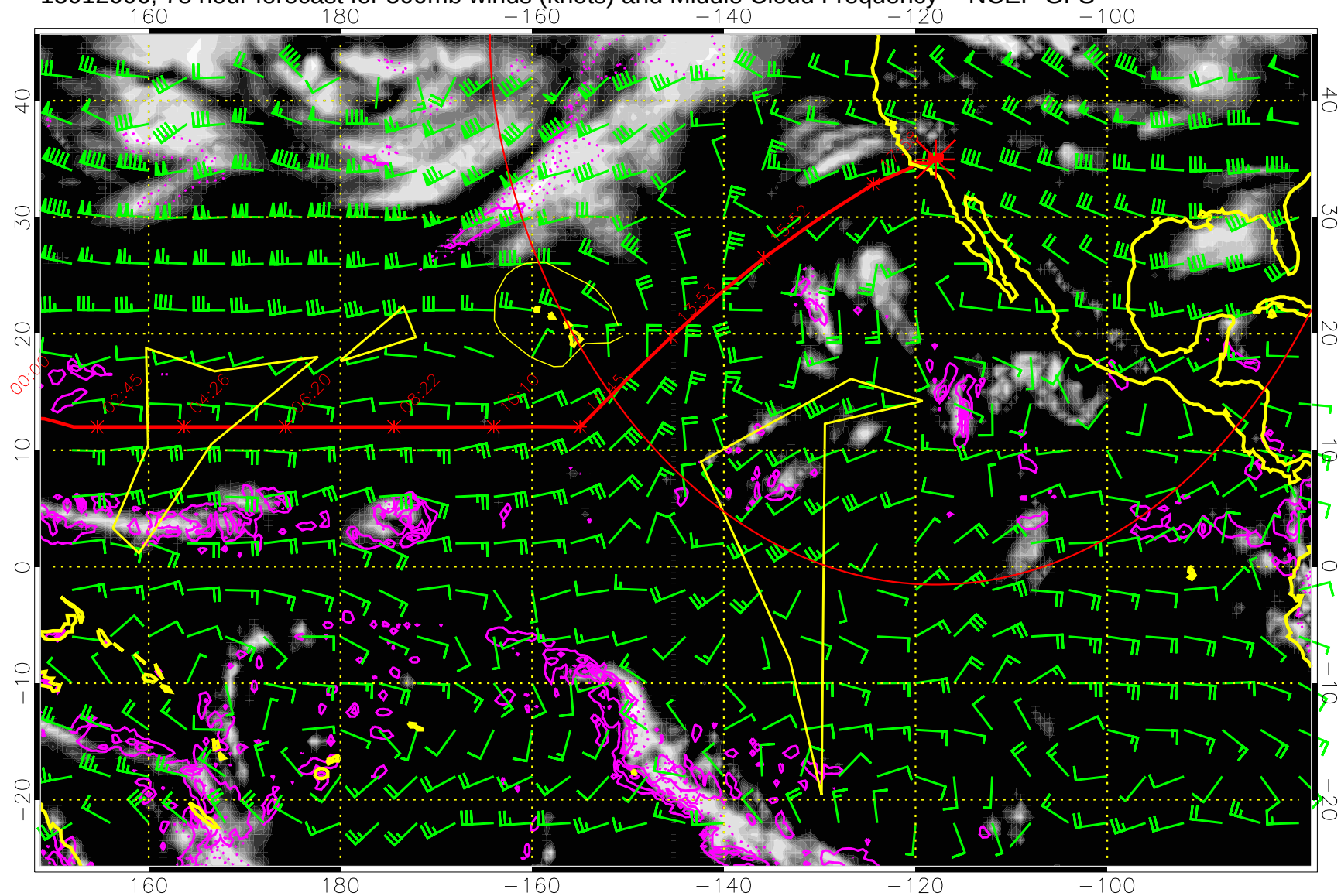
15012006, 78 hour forecast for 500mb winds (knots) and Middle Cloud Frequency -- NCEP GFS
