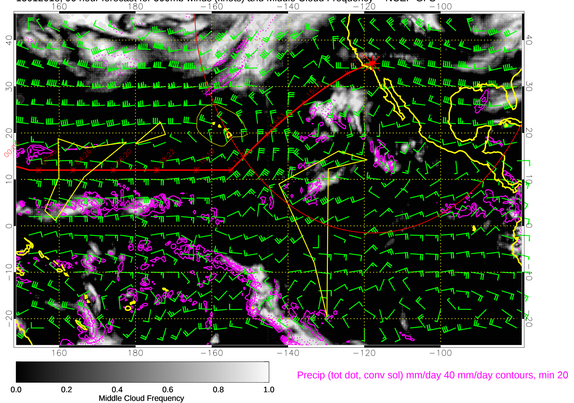
15012018, 90 hour forecast for 500mb winds (knots) and Middle Cloud Frequency -- NCEP GFS
