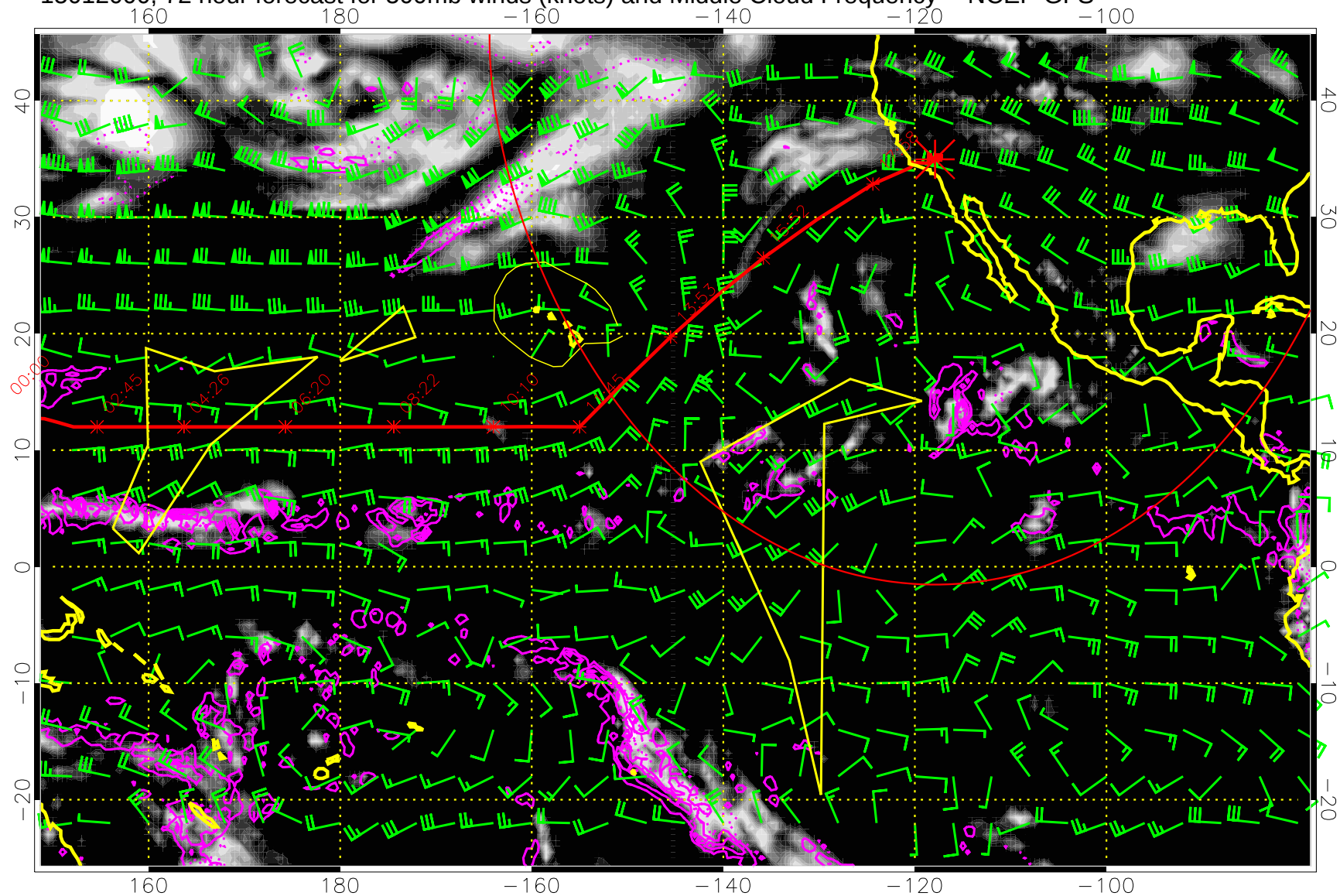
15012000, 72 hour forecast for 500mb winds (knots) and Middle Cloud Frequency -- NCEP GFS
