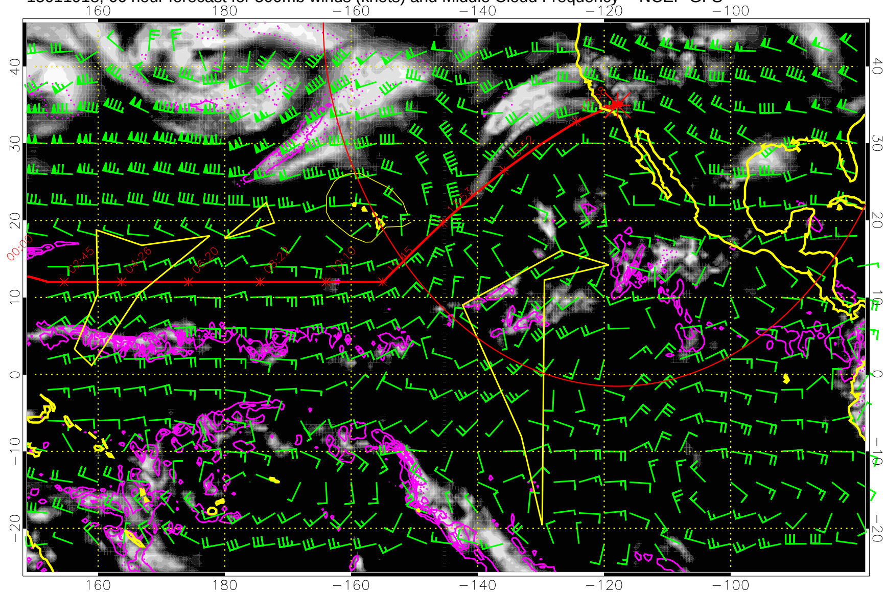
15011918, 66 hour forecast for 500mb winds (knots) and Middle Cloud Frequency -- NCEP GFS
