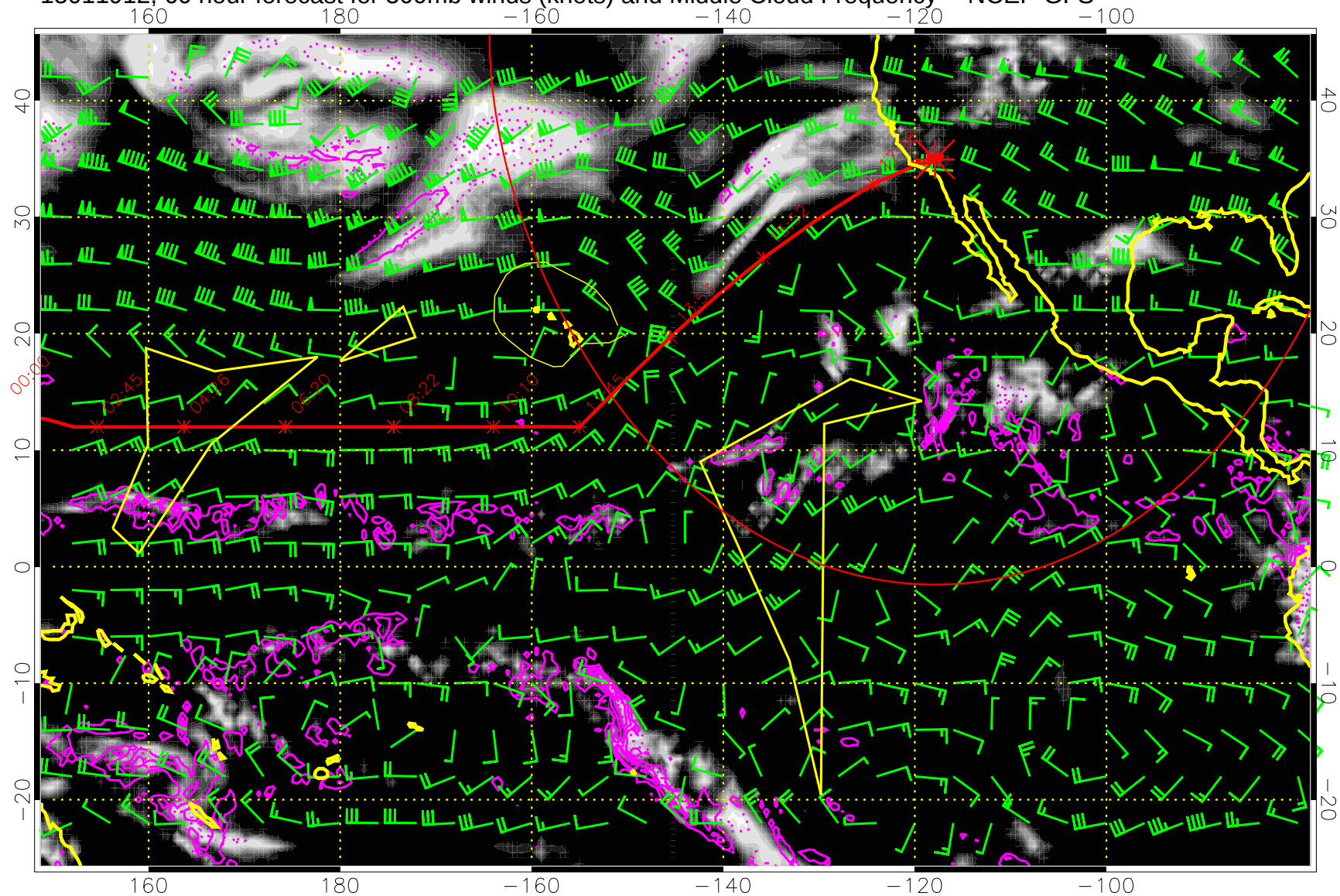
15011912, 60 hour forecast for 500mb winds (knots) and Middle Cloud Frequency -- NCEP GFS
