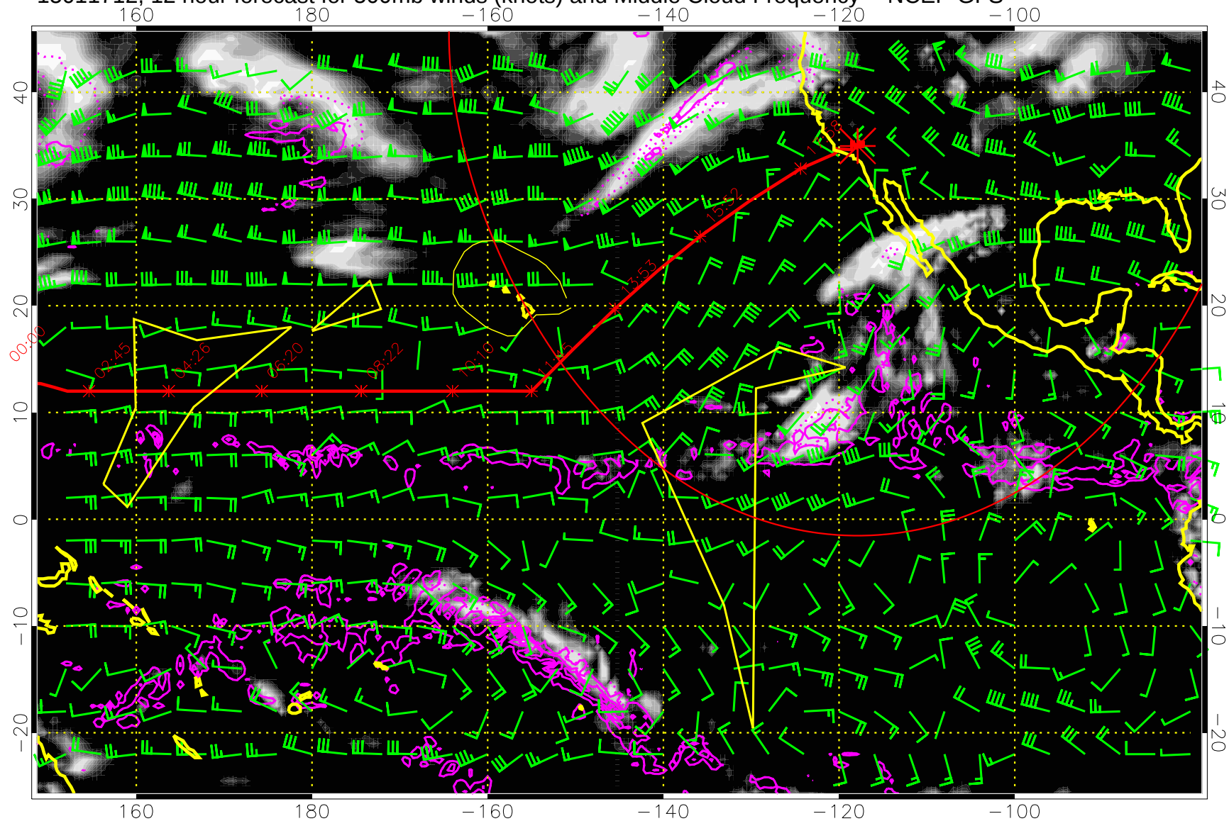
15011712, 12 hour forecast for 500mb winds (knots) and Middle Cloud Frequency -- NCEP GFS
