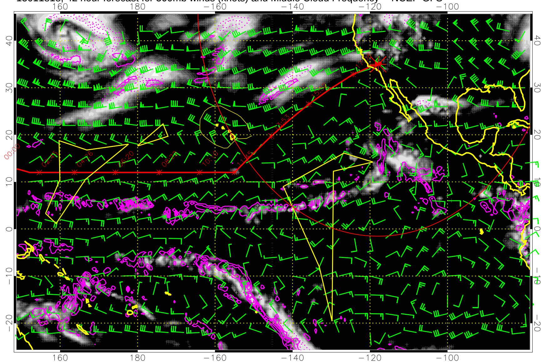
15011818, 42 hour forecast for 500mb winds (knots) and Middle Cloud Frequency -- NCEP GFS
