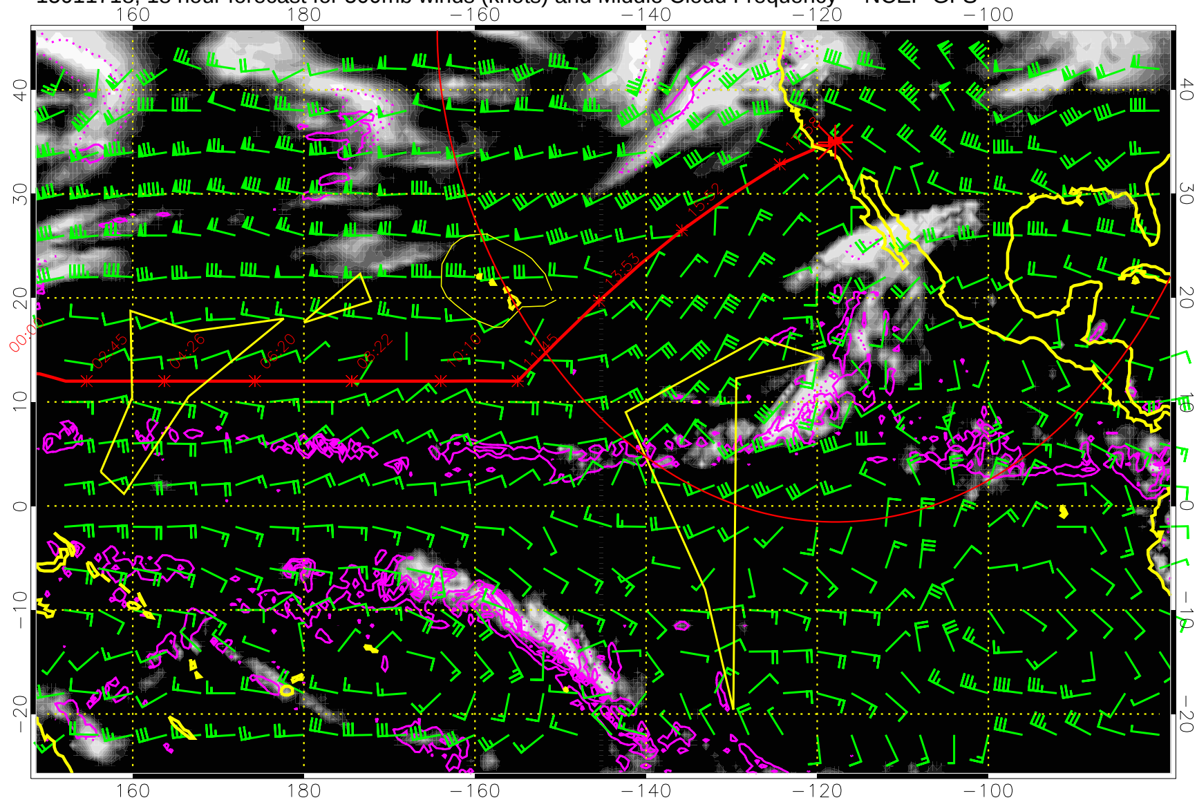
15011718, 18 hour forecast for 500mb winds (knots) and Middle Cloud Frequency -- NCEP GFS
