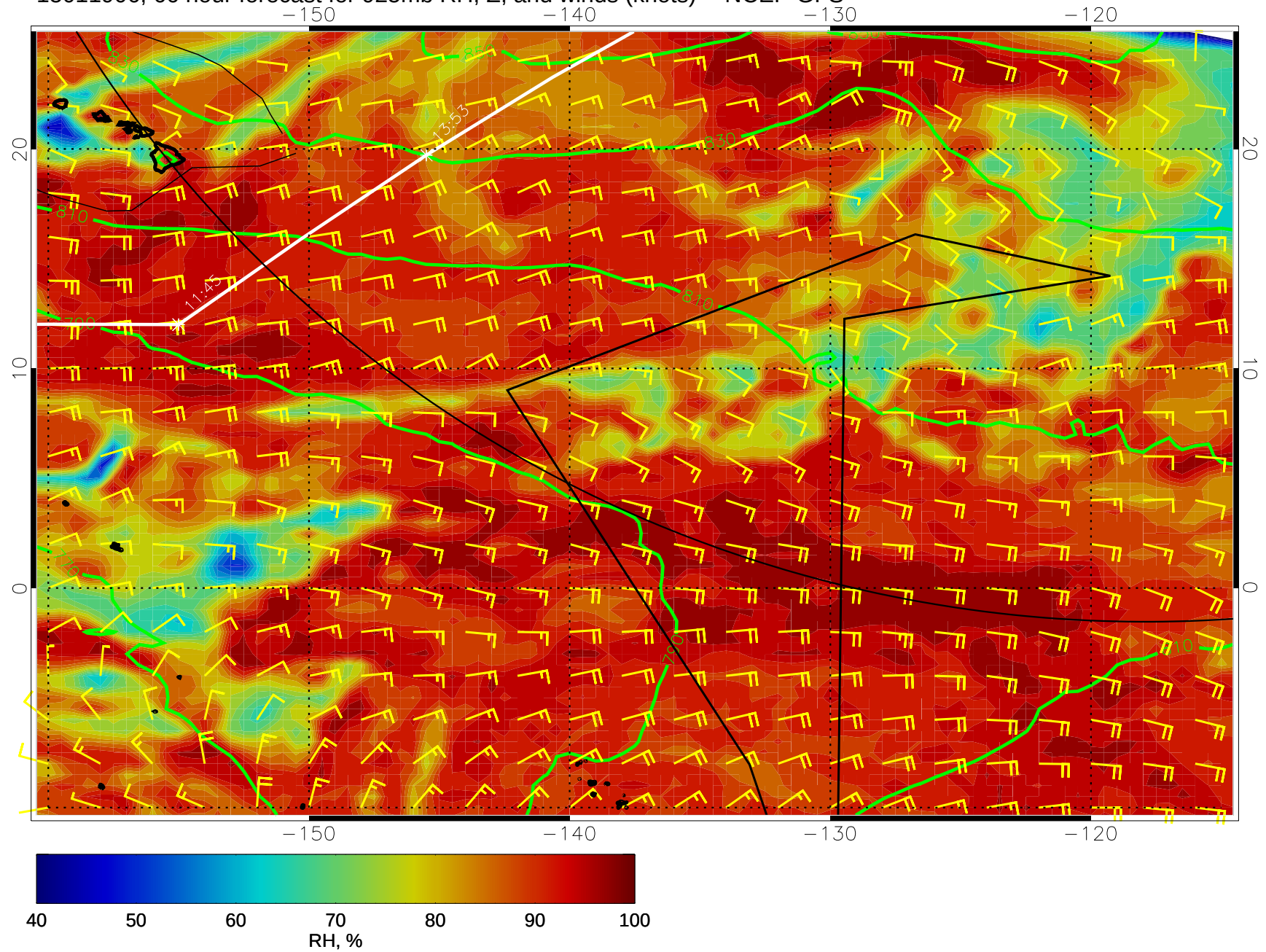
15011906, 66 hour forecast for 925mb RH, Z, and winds (knots) -- NCEP GFS
