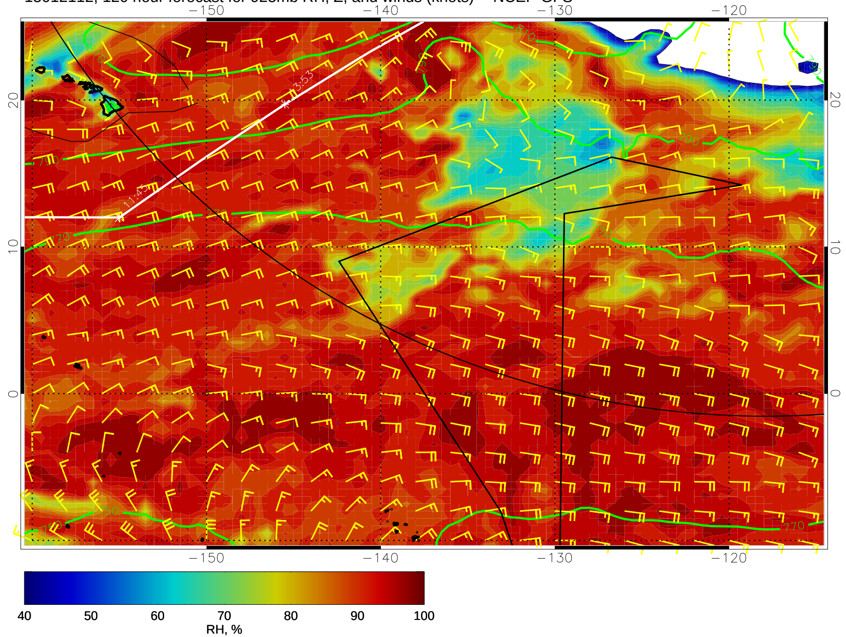
15012112, 120 hour forecast for 925mb RH, Z, and winds (knots) -- NCEP GFS
