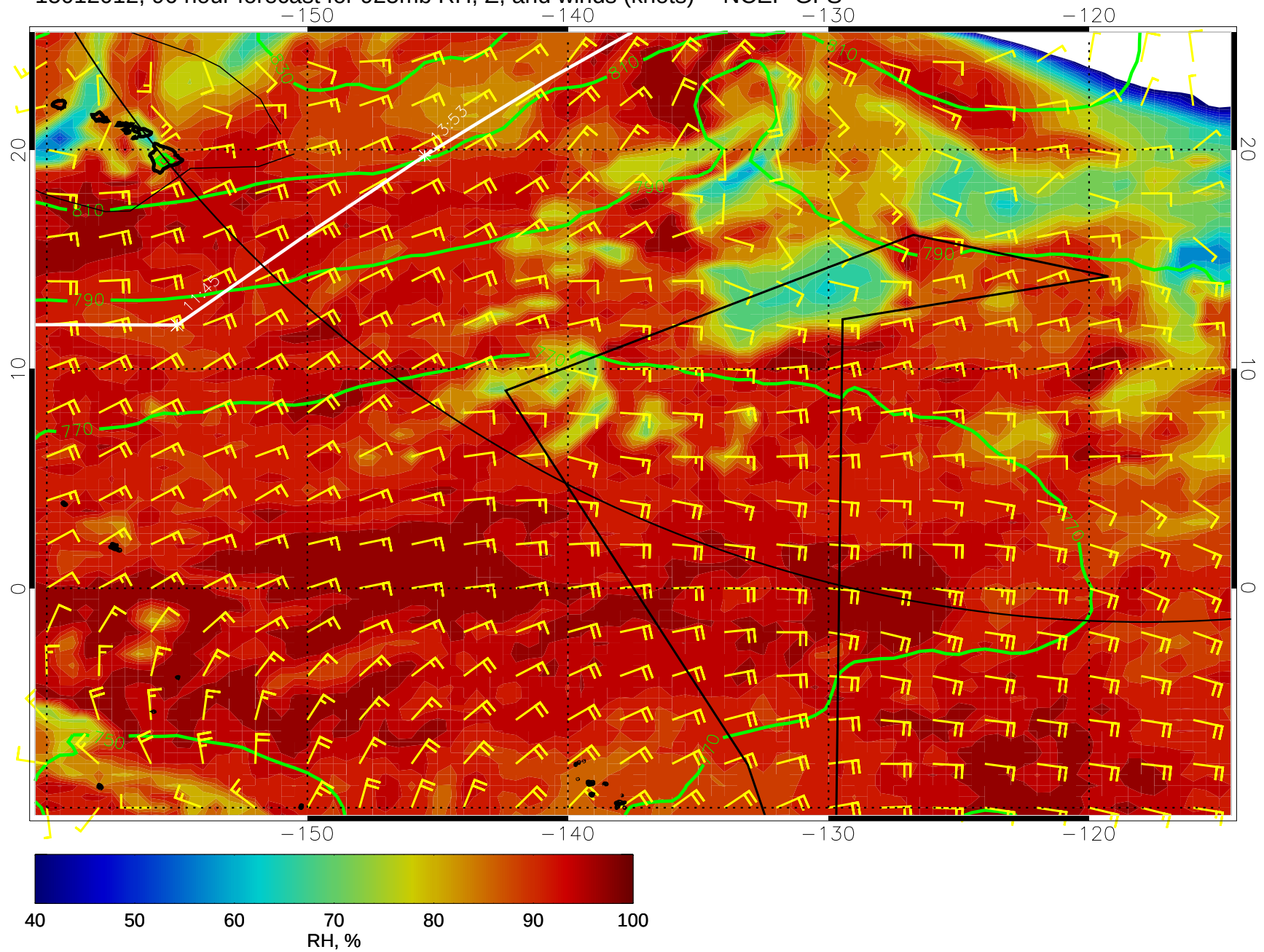
15012012, 96 hour forecast for 925mb RH, Z, and winds (knots) -- NCEP GFS
