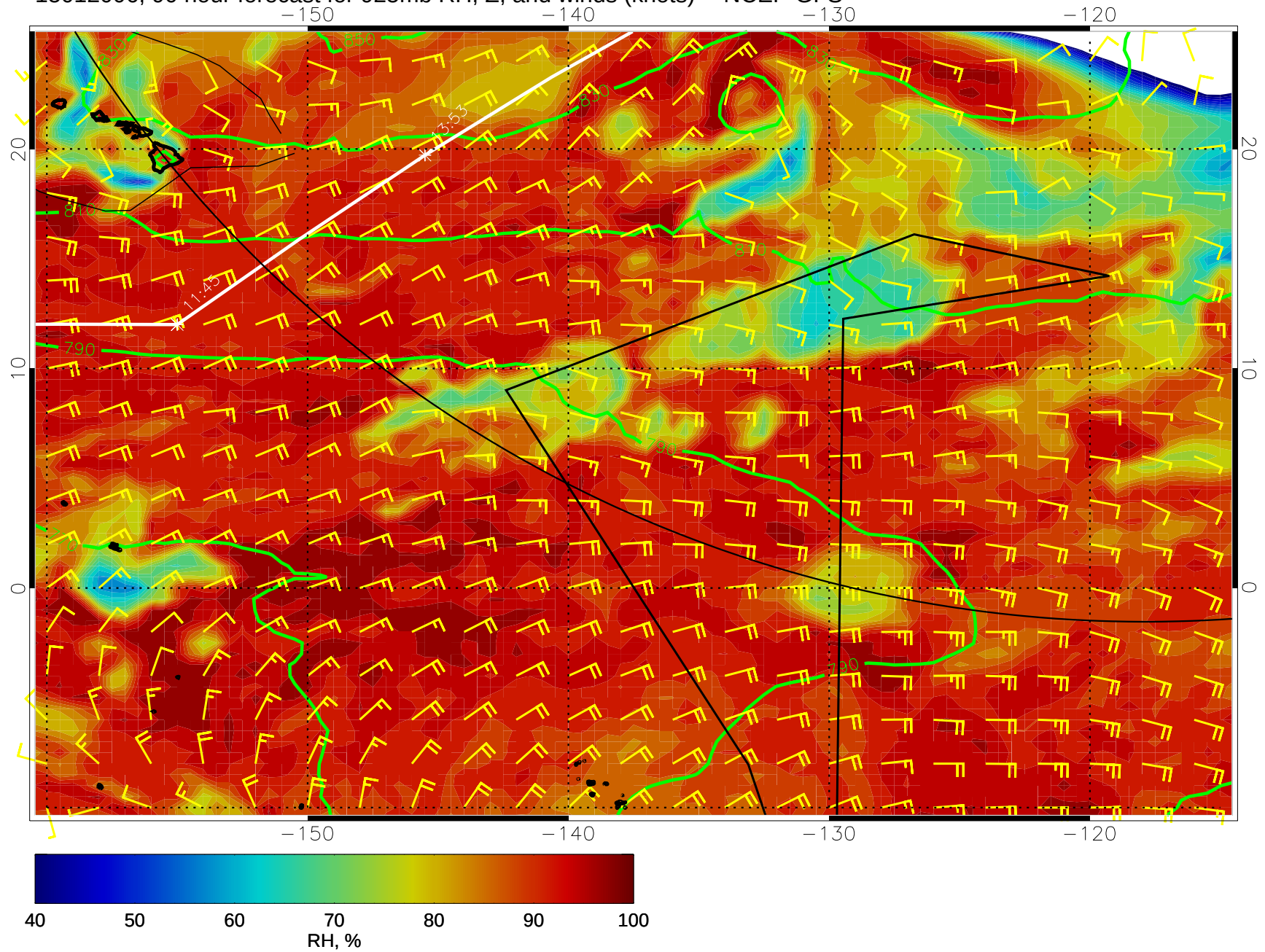
15012006, 90 hour forecast for 925mb RH, Z, and winds (knots) -- NCEP GFS
