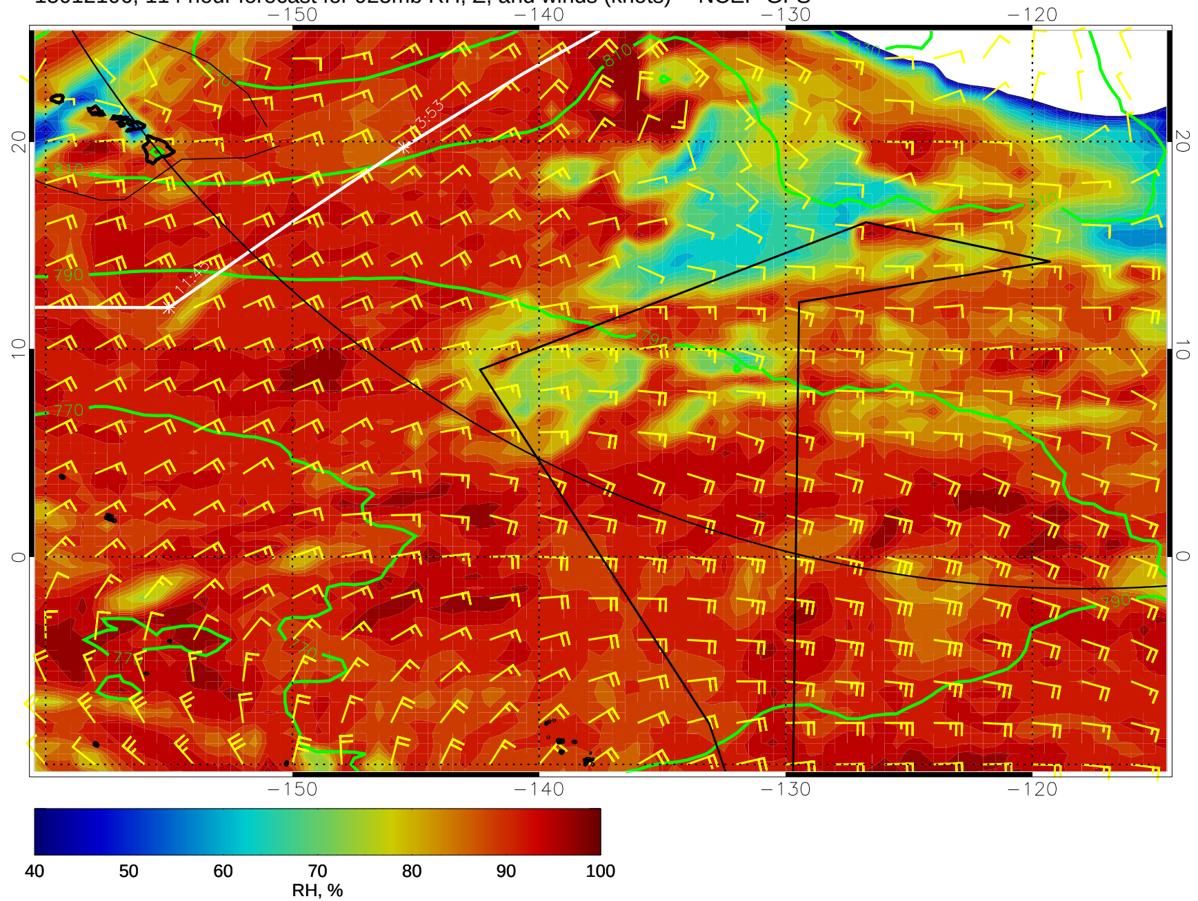
15012106, 114 hour forecast for 925mb RH, Z, and winds (knots) -- NCEP GFS
