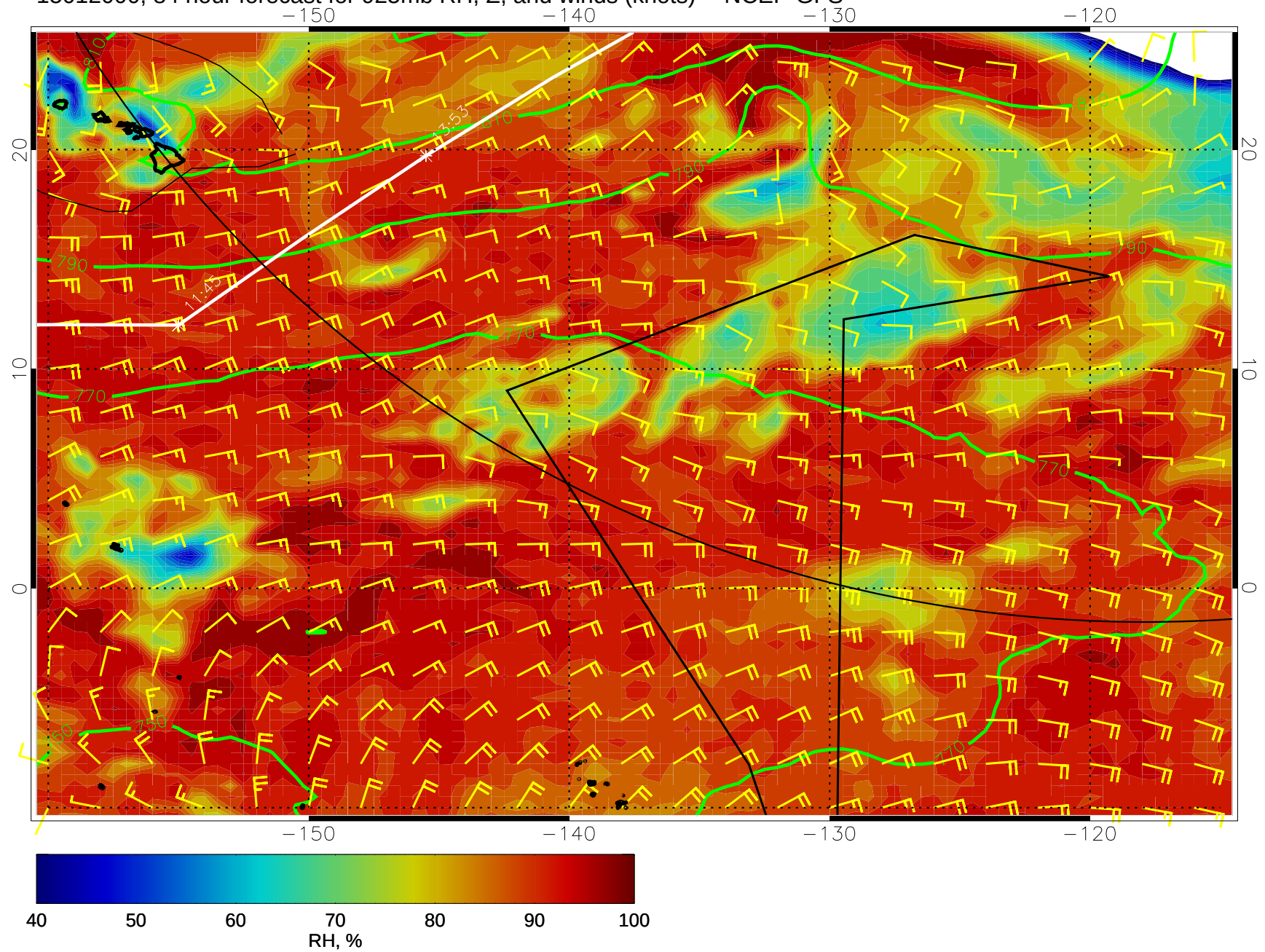
15012000, 84 hour forecast for 925mb RH, Z, and winds (knots) -- NCEP GFS
