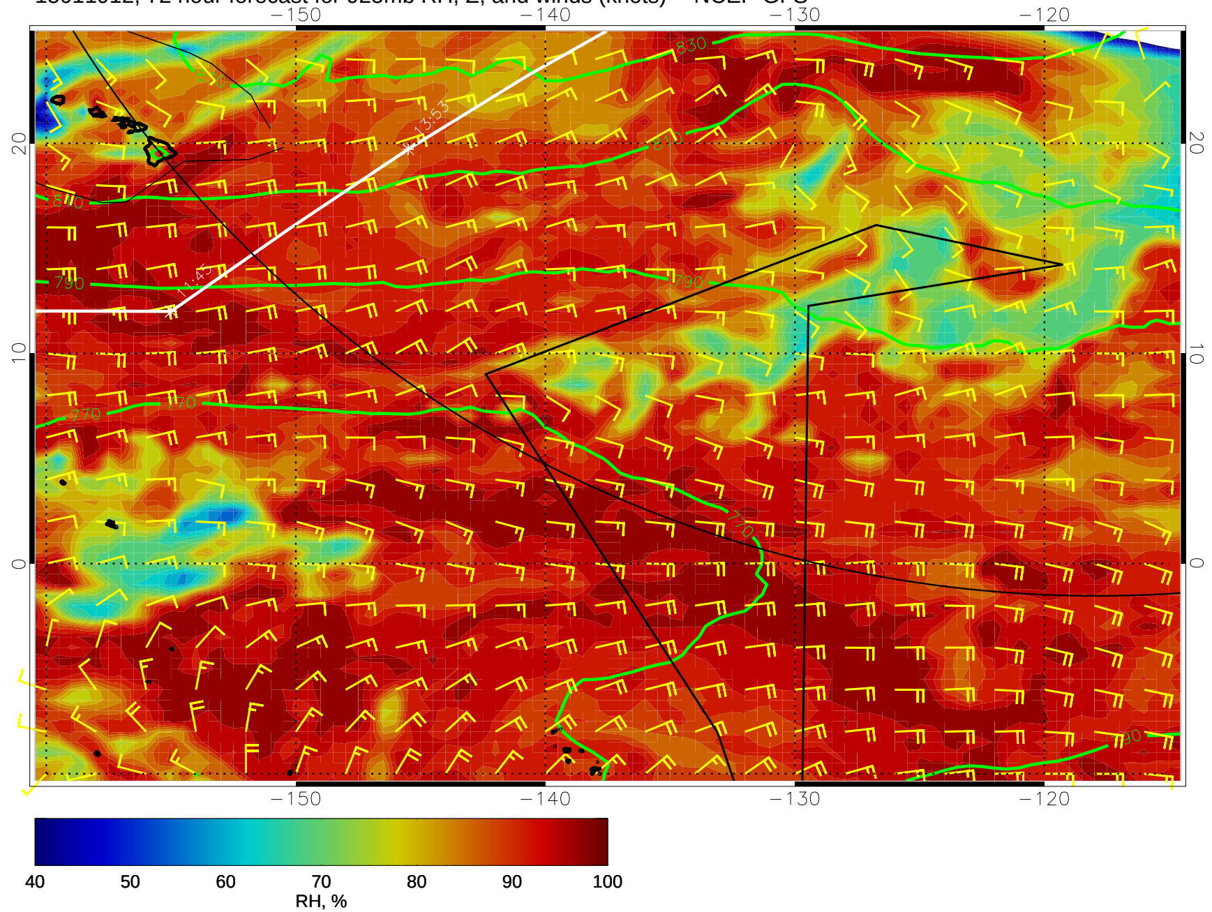
15011912, 72 hour forecast for 925mb RH, Z, and winds (knots) -- NCEP GFS
