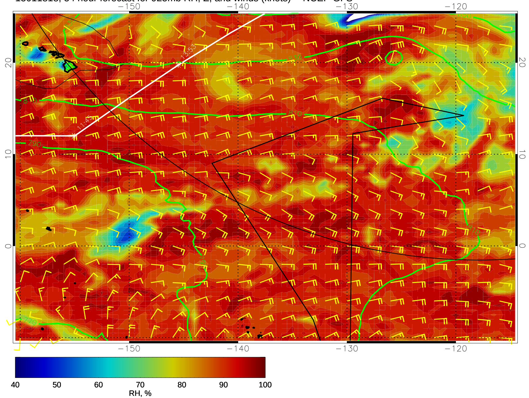
15011818, 54 hour forecast for 925mb RH, Z, and winds (knots) -- NCEP GFS
