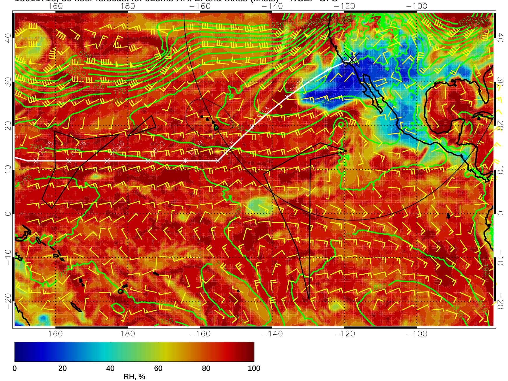
15011718, 30 hour forecast for 925mb RH, Z, and winds (knots) -- NCEP GFS
