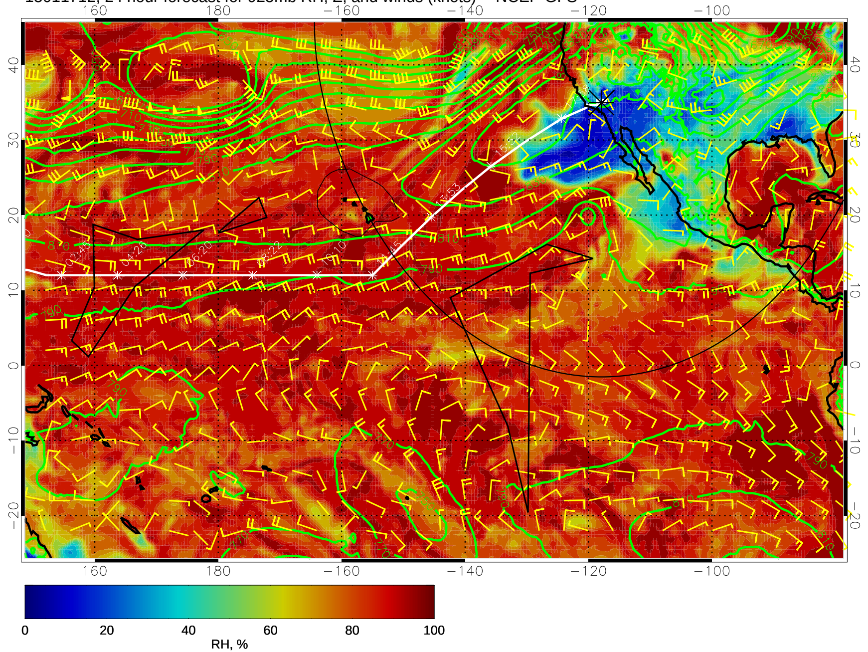
15011712, 24 hour forecast for 925mb RH, Z, and winds (knots) -- NCEP GFS
