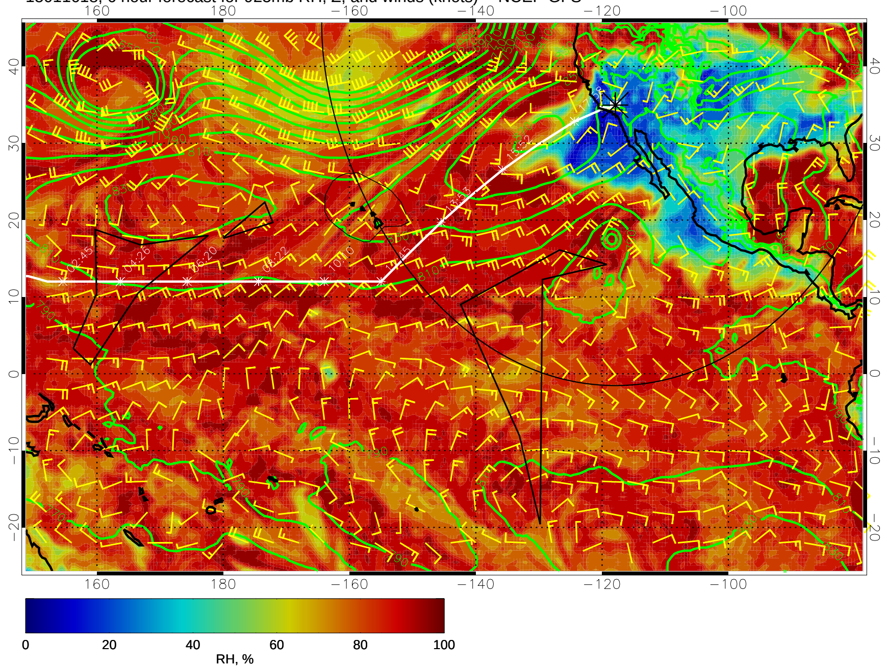
15011618, 6 hour forecast for 925mb RH, Z, and winds (knots) -- NCEP GFS
