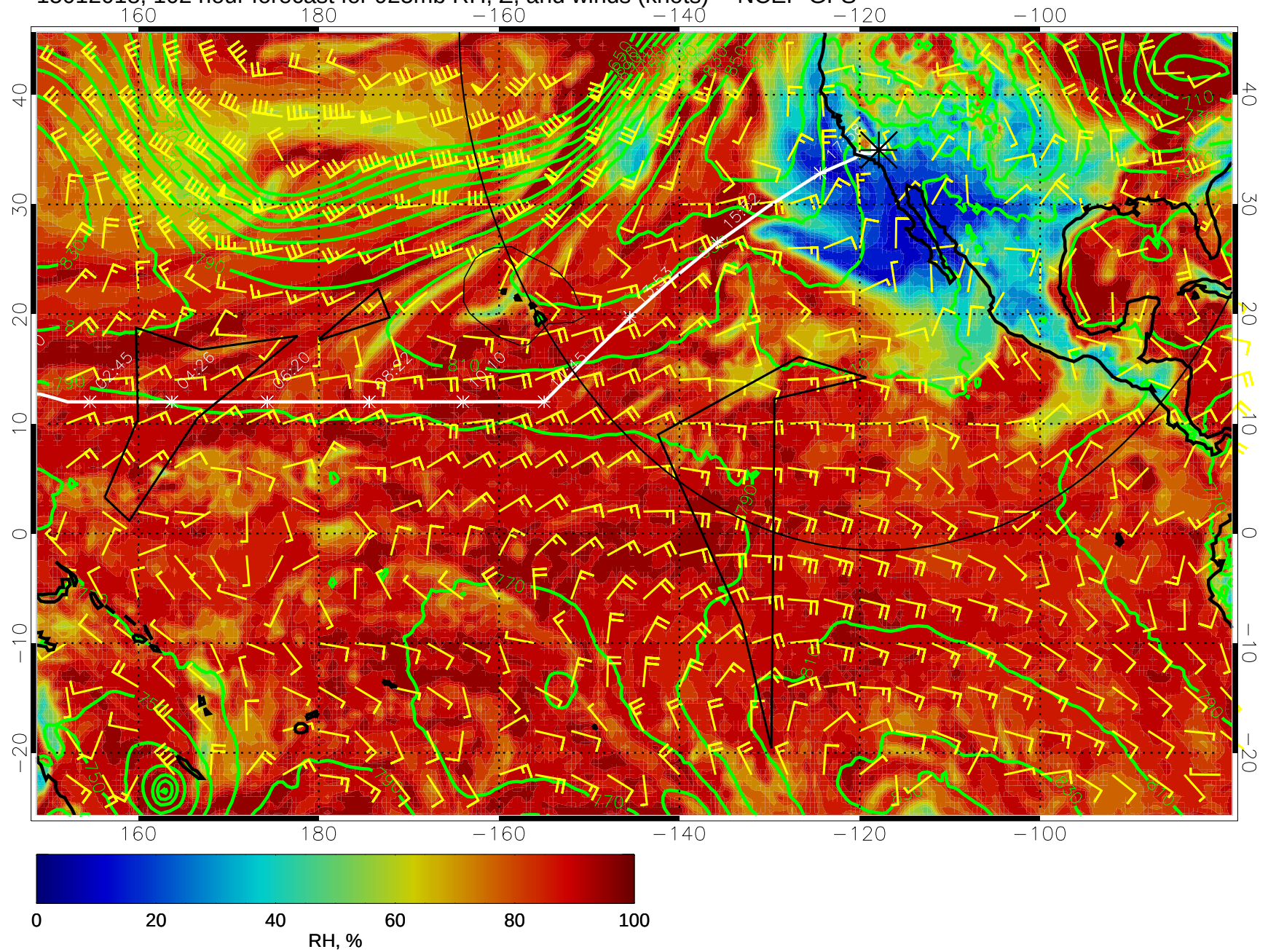
15012018, 102 hour forecast for 925mb RH, Z, and winds (knots) -- NCEP GFS
