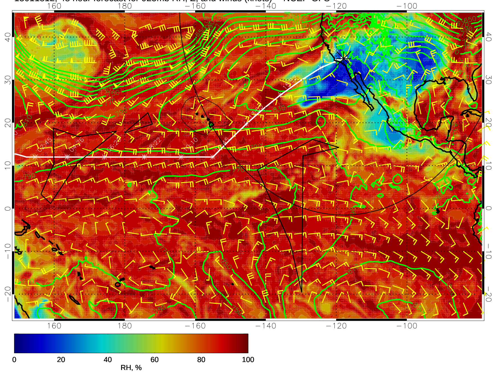
15011812, 48 hour forecast for 925mb RH, Z, and winds (knots) -- NCEP GFS
