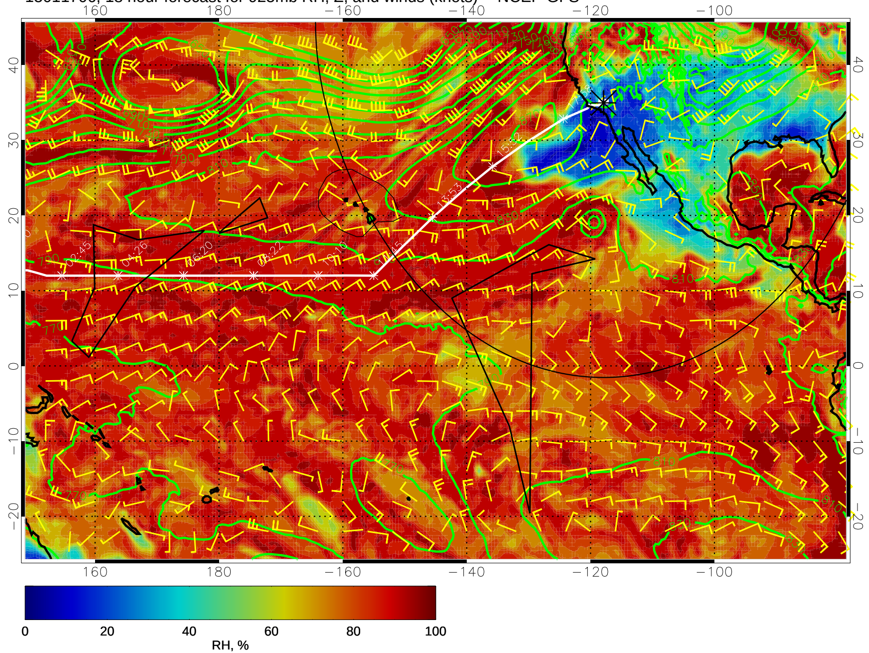
15011706, 18 hour forecast for 925mb RH, Z, and winds (knots) -- NCEP GFS
