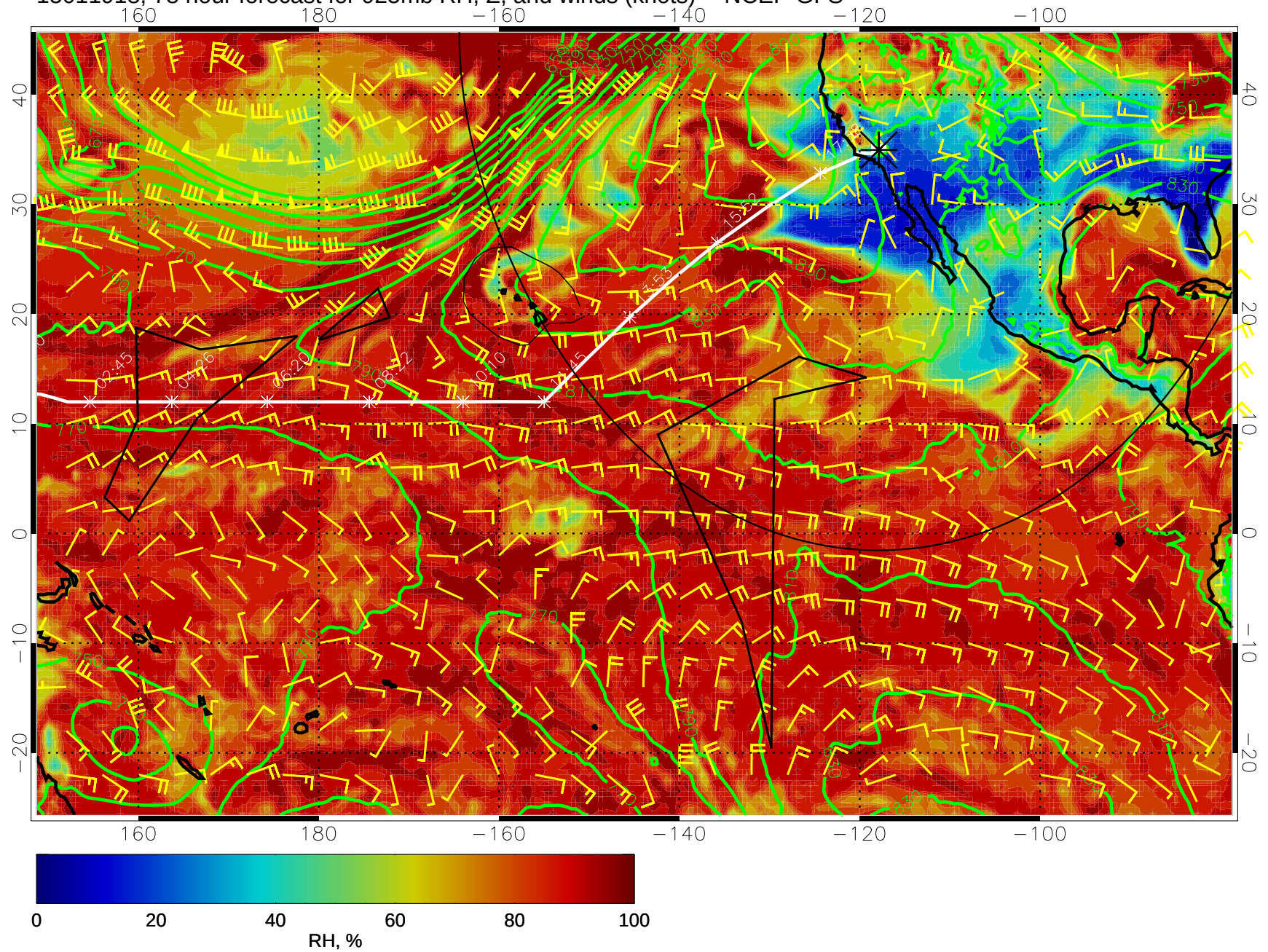
15011918, 78 hour forecast for 925mb RH, Z, and winds (knots) -- NCEP GFS
