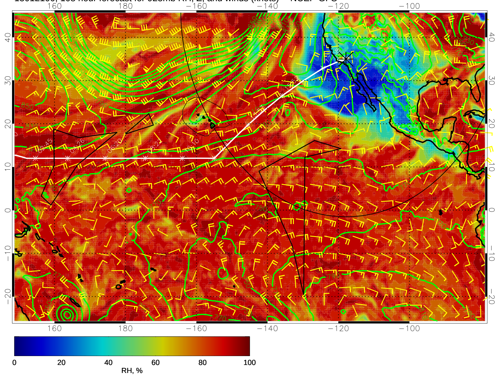
15012100, 108 hour forecast for 925mb RH, Z, and winds (knots) -- NCEP GFS
