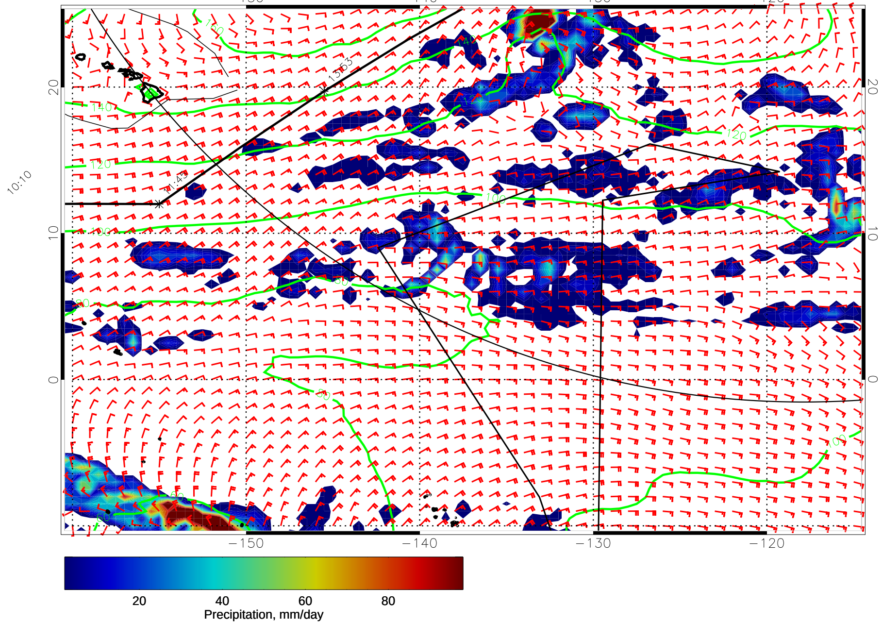
15012012, 96 hour forecast for precip, 1000mb Z, and winds (knots) -- NCEP GFS
