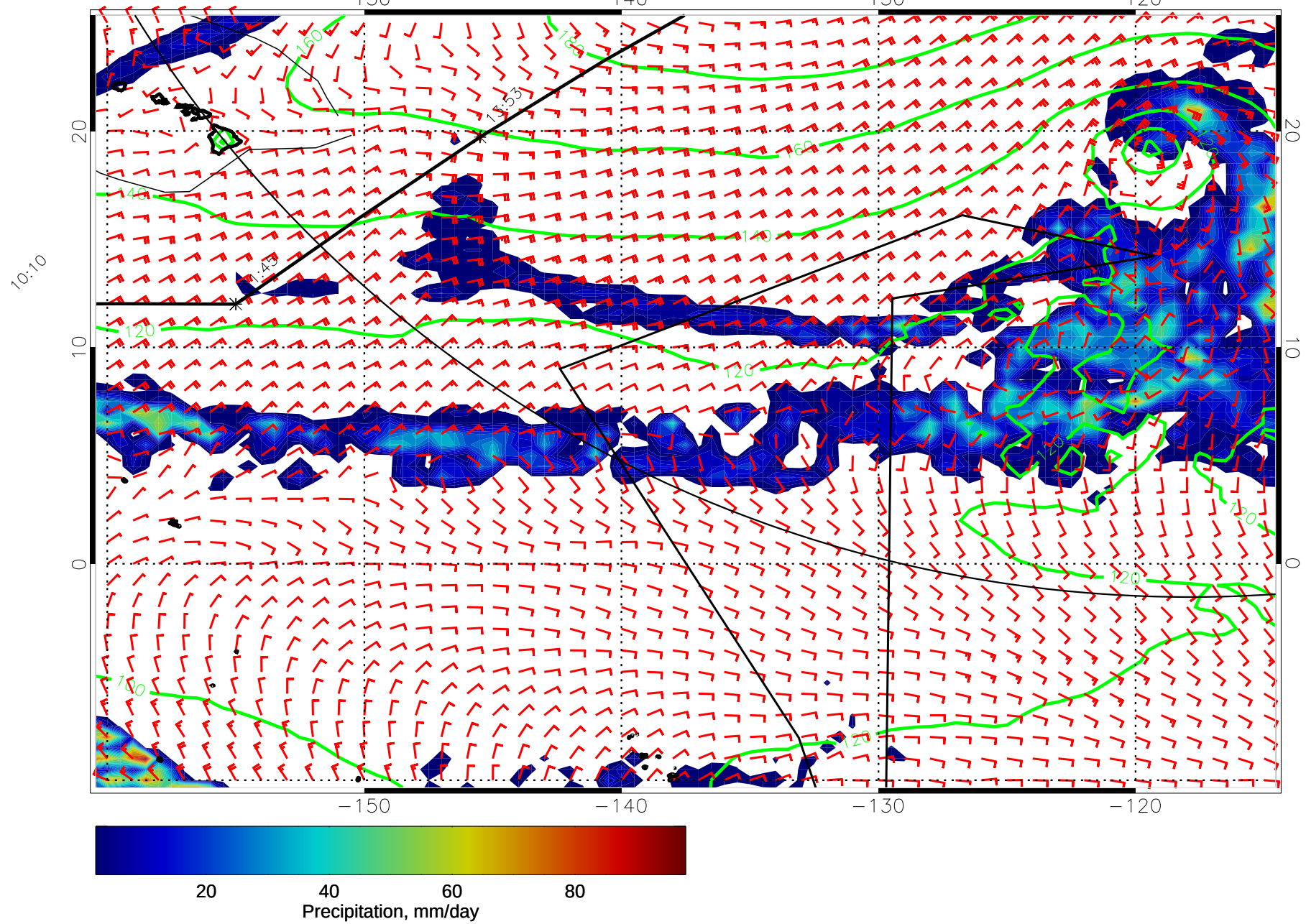
15011706, 18 hour forecast for precip, 1000mb Z, and winds (knots) -- NCEP GFS
