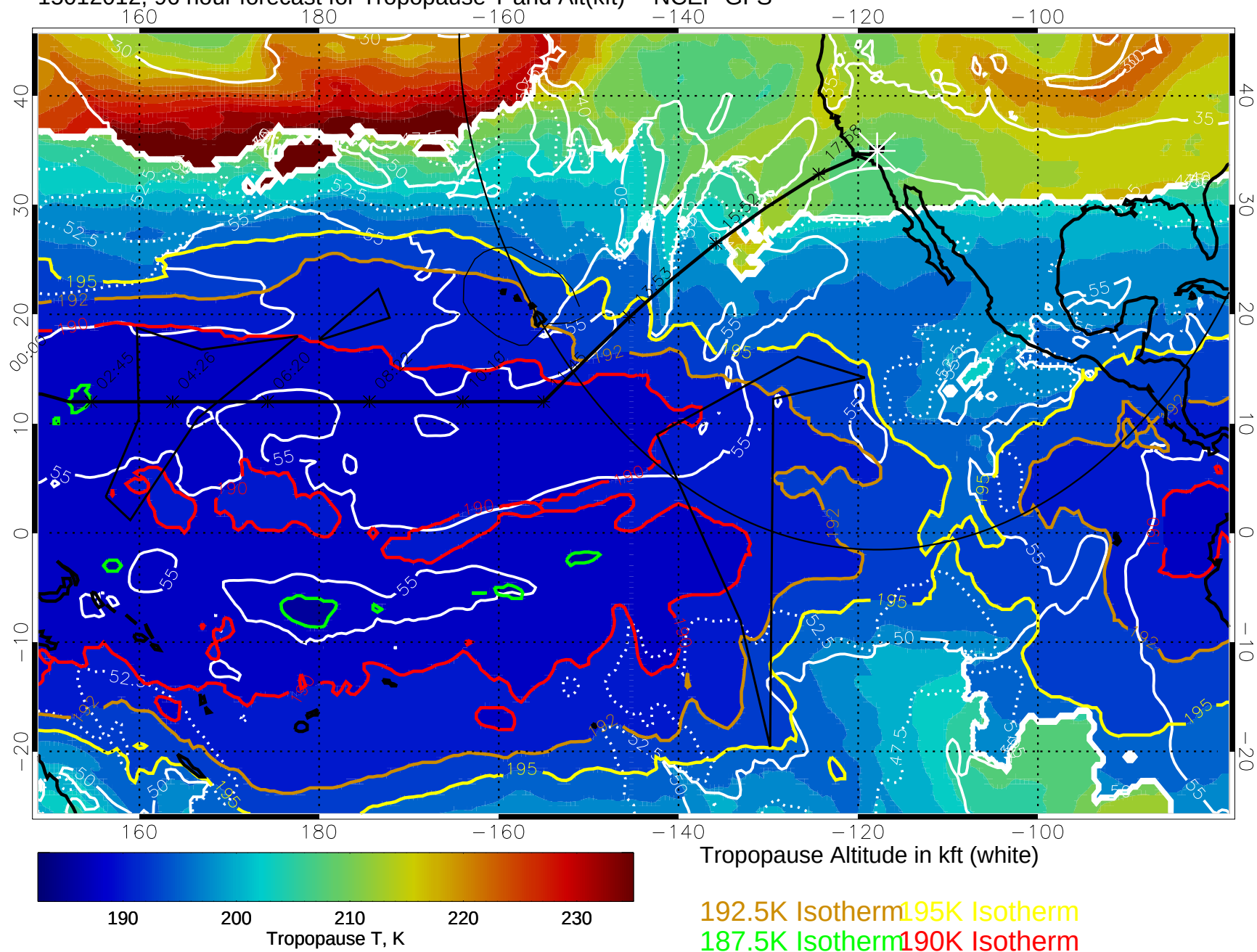
15012012, 96 hour forecast for Tropopause T and Alt(kft) -- NCEP GFS
