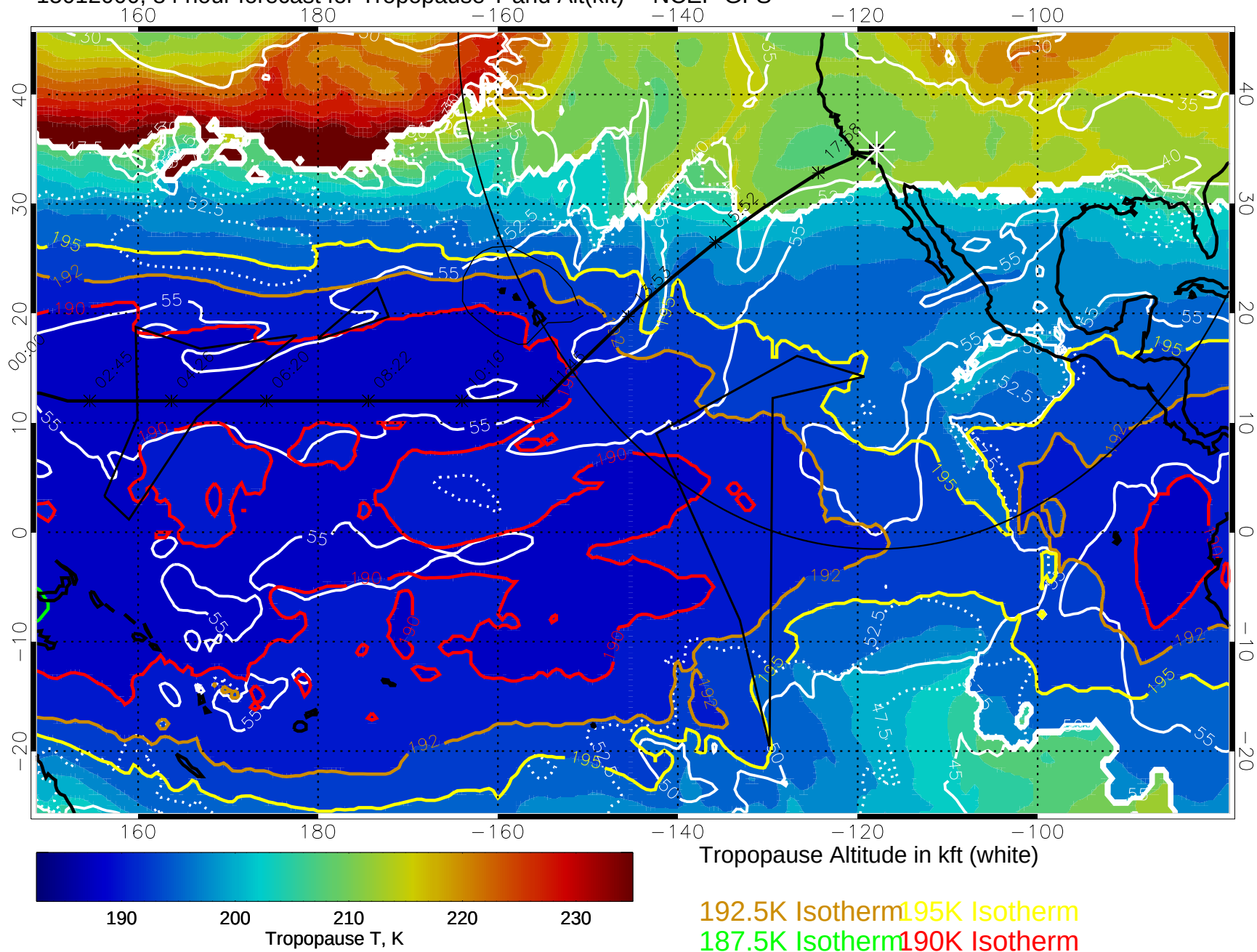
15012000, 84 hour forecast for Tropopause T and Alt(kft) -- NCEP GFS
