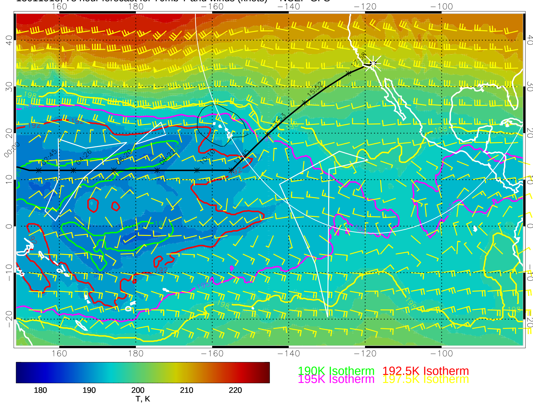
15011918, 78 hour forecast for 70mb T and winds (knots) -- NCEP GFS
