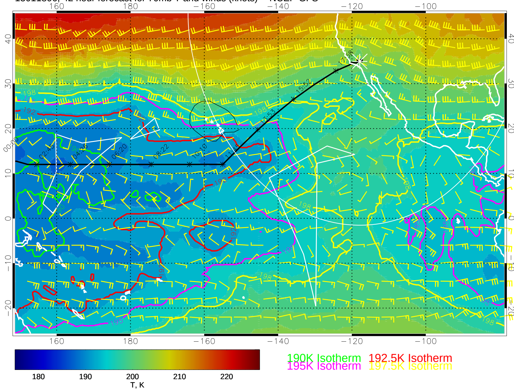
15011806, 42 hour forecast for 70mb T and winds (knots) -- NCEP GFS
