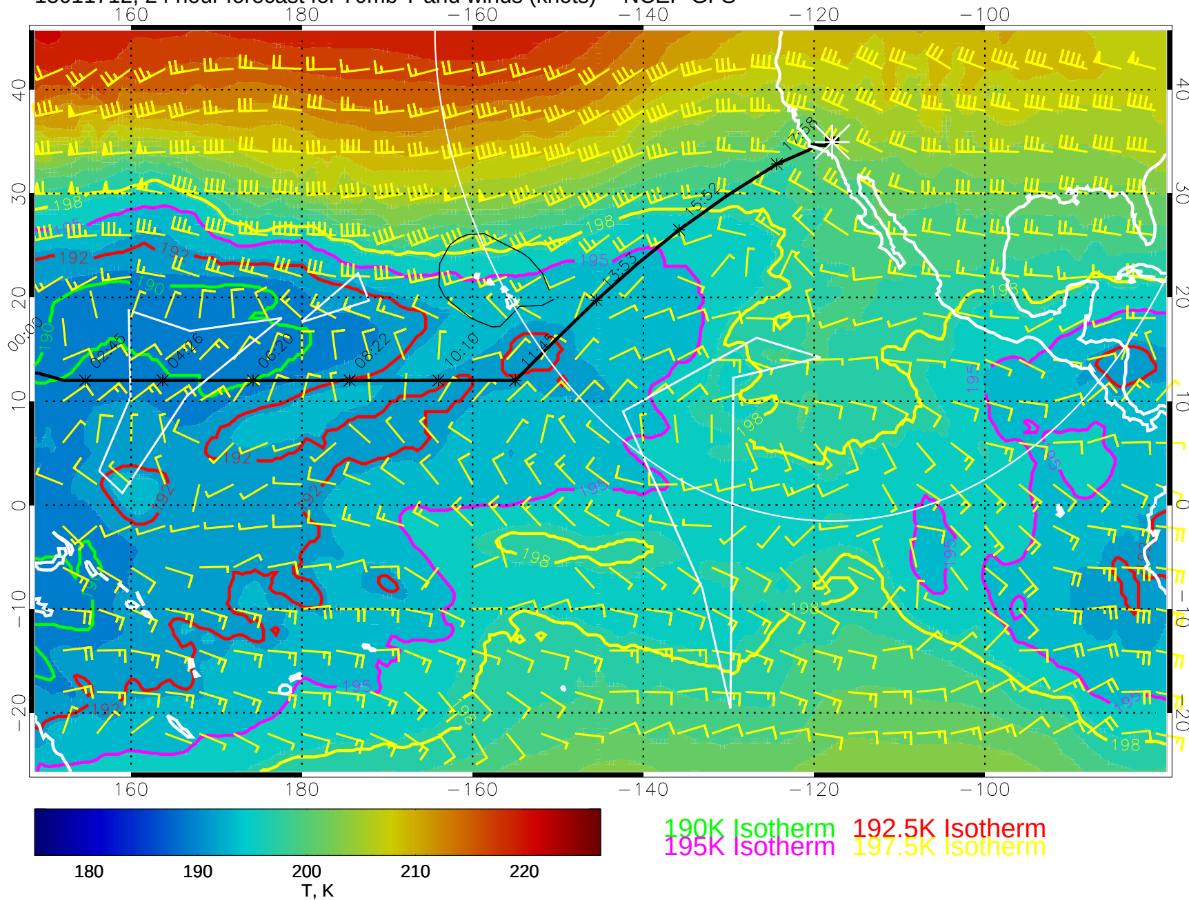
15011712, 24 hour forecast for 70mb T and winds (knots) -- NCEP GFS
