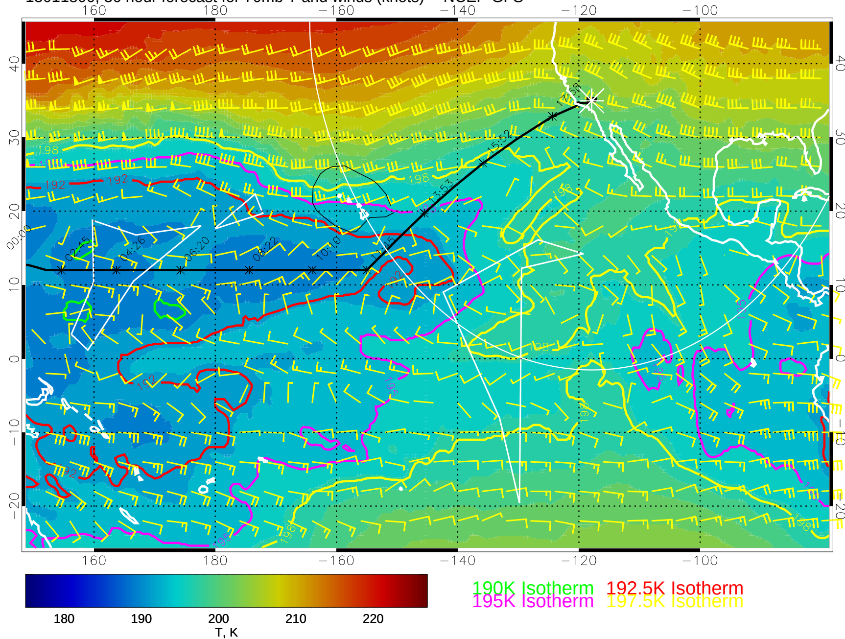
15011800, 36 hour forecast for 70mb T and winds (knots) -- NCEP GFS
