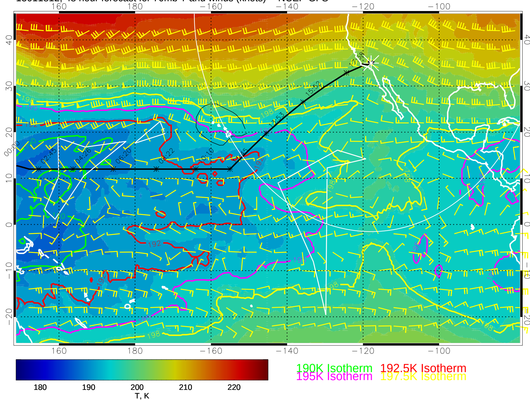
15011812, 48 hour forecast for 70mb T and winds (knots) -- NCEP GFS
