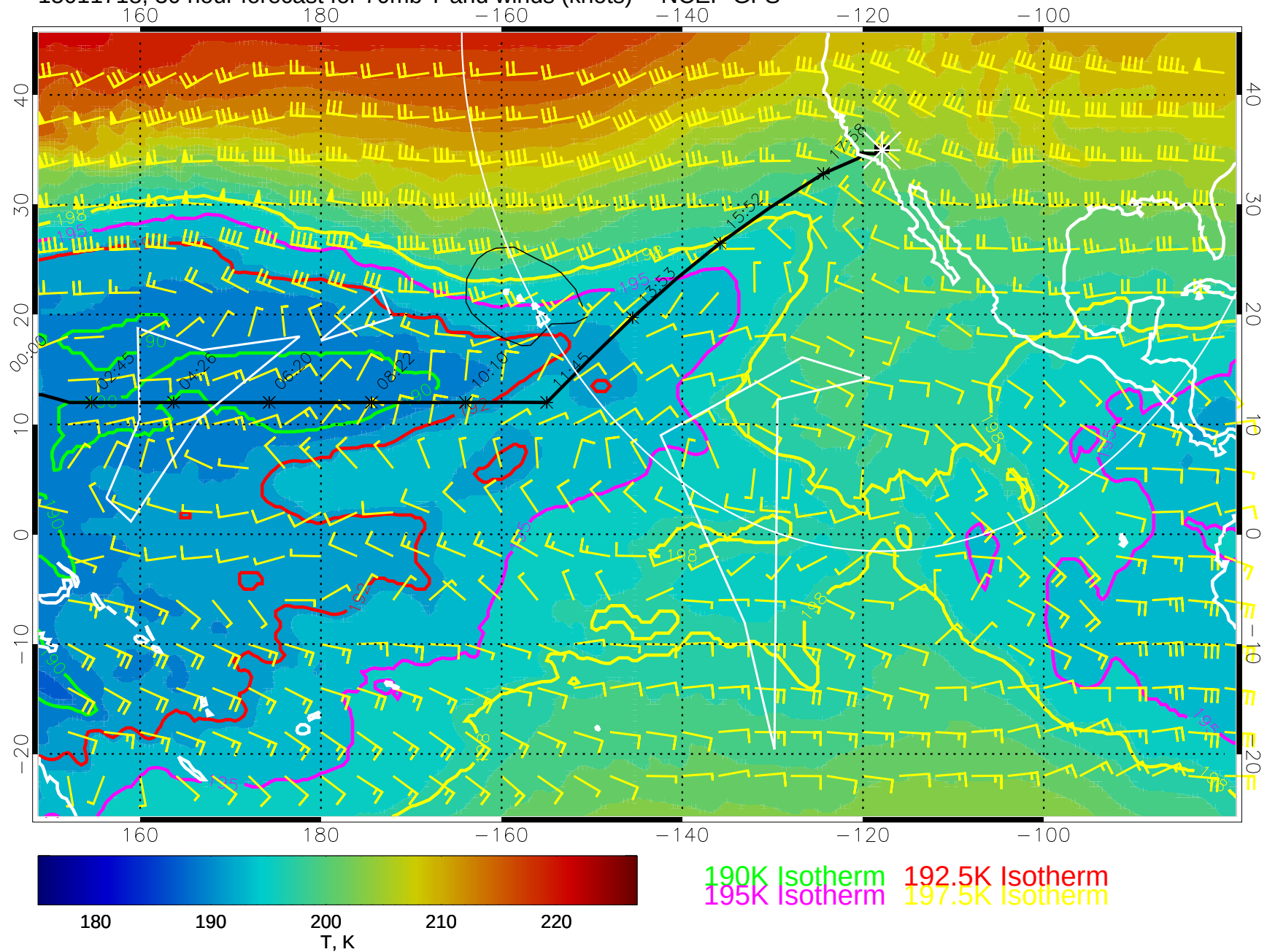
15011718, 30 hour forecast for 70mb T and winds (knots) -- NCEP GFS
