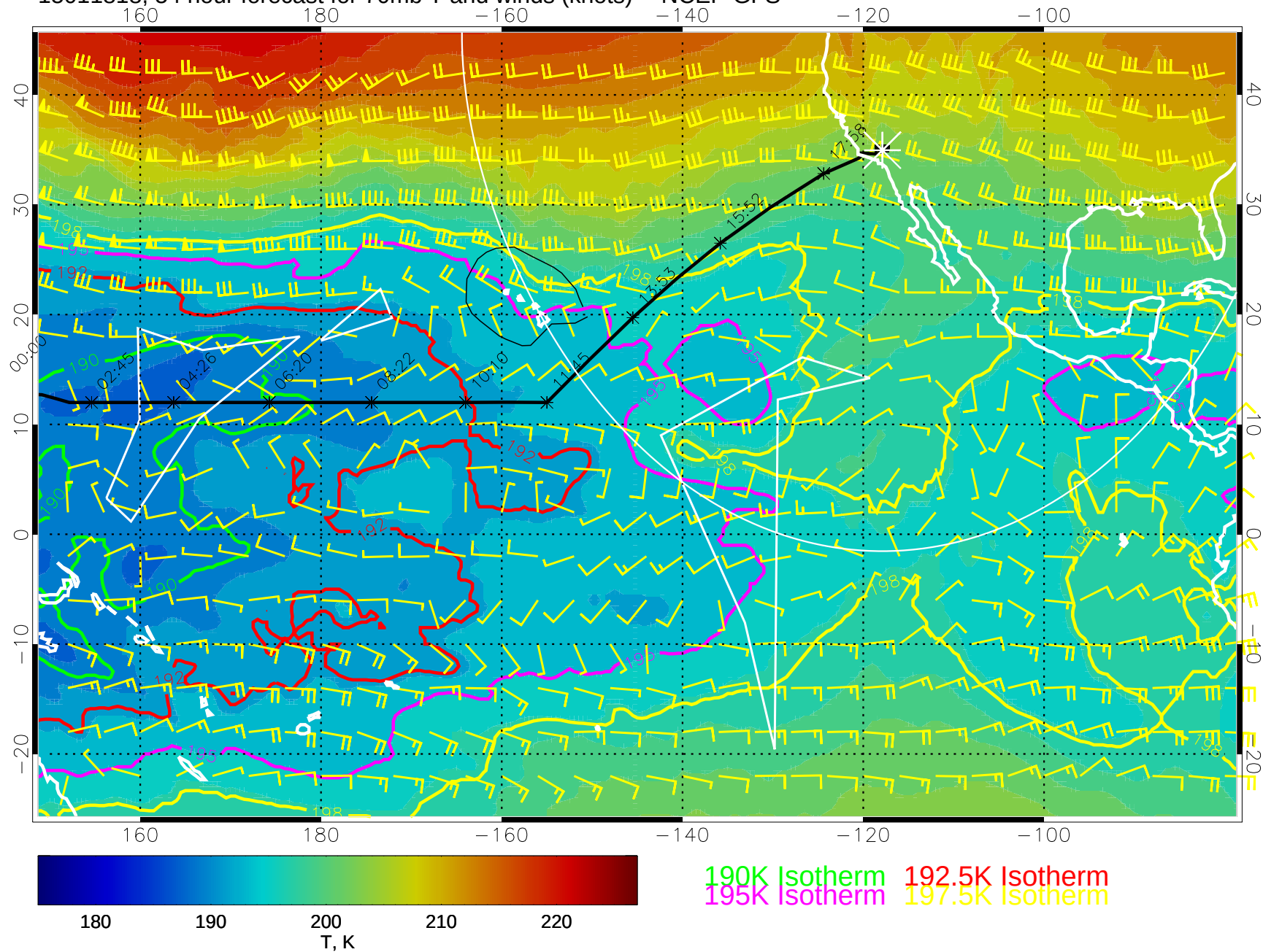
15011818, 54 hour forecast for 70mb T and winds (knots) -- NCEP GFS
