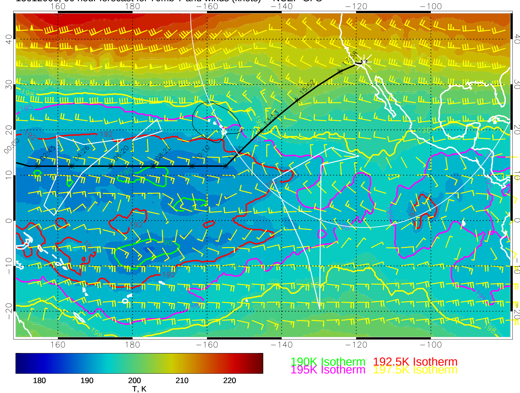
15012006, 90 hour forecast for 70mb T and winds (knots) -- NCEP GFS
