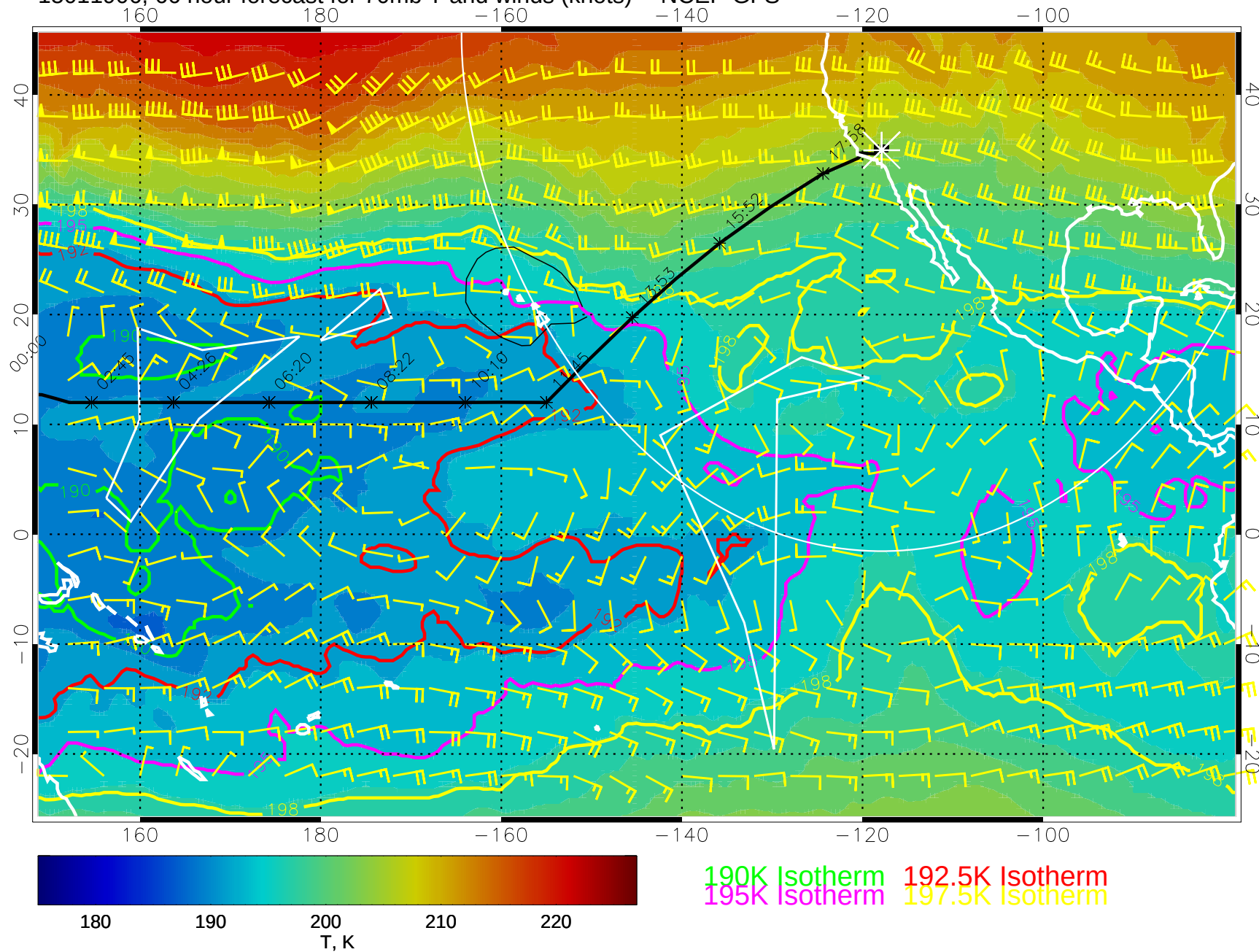
15011906, 66 hour forecast for 70mb T and winds (knots) -- NCEP GFS
