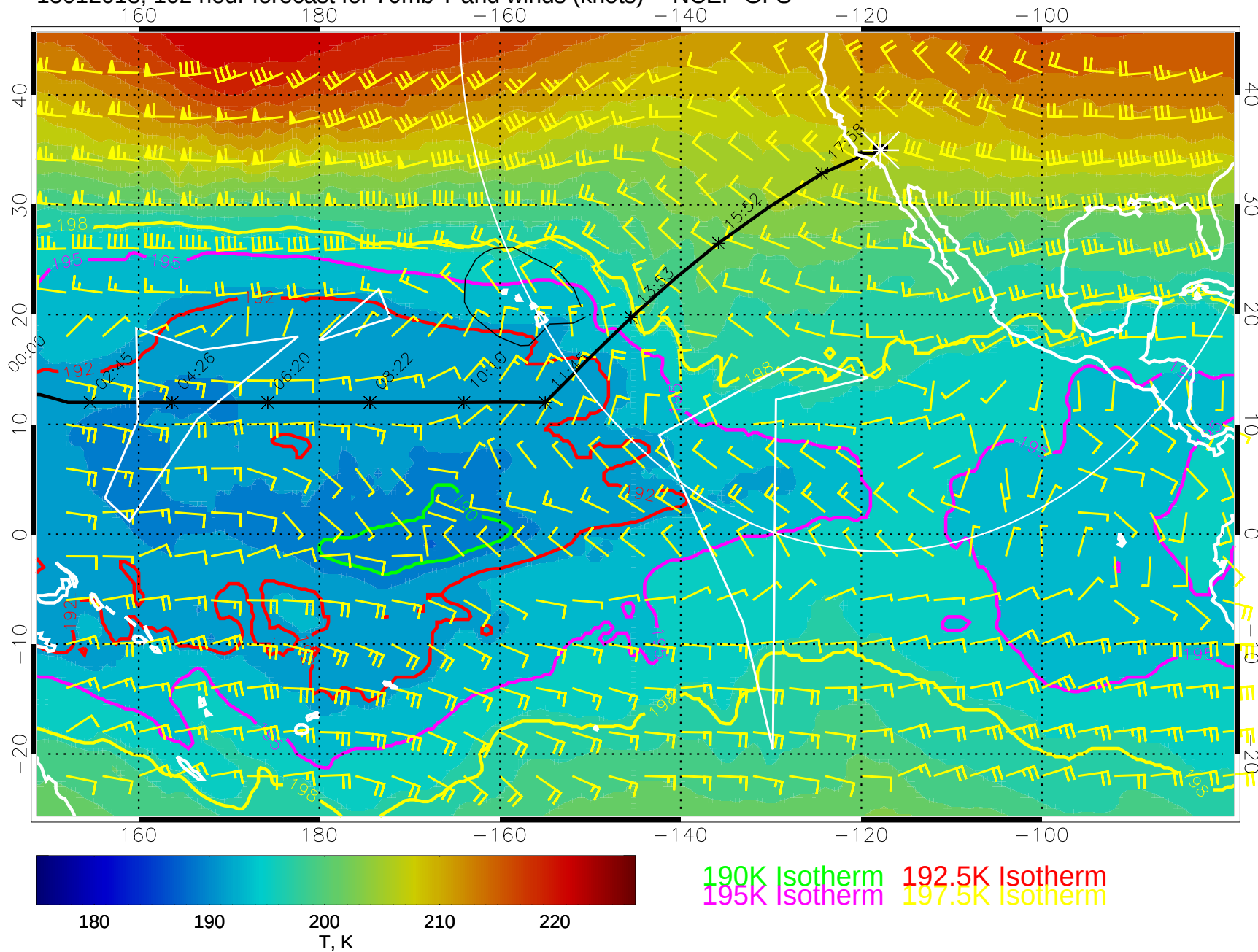
15012018, 102 hour forecast for 70mb T and winds (knots) -- NCEP GFS
