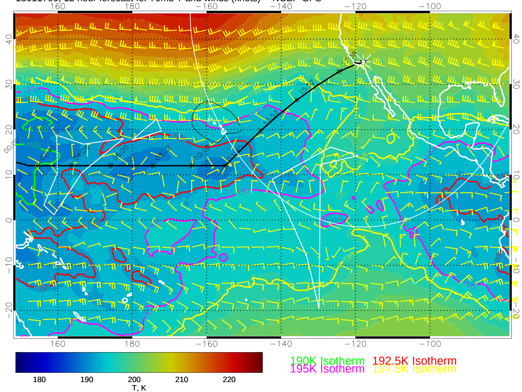
15011700, 12 hour forecast for 70mb T and winds (knots) -- NCEP GFS
