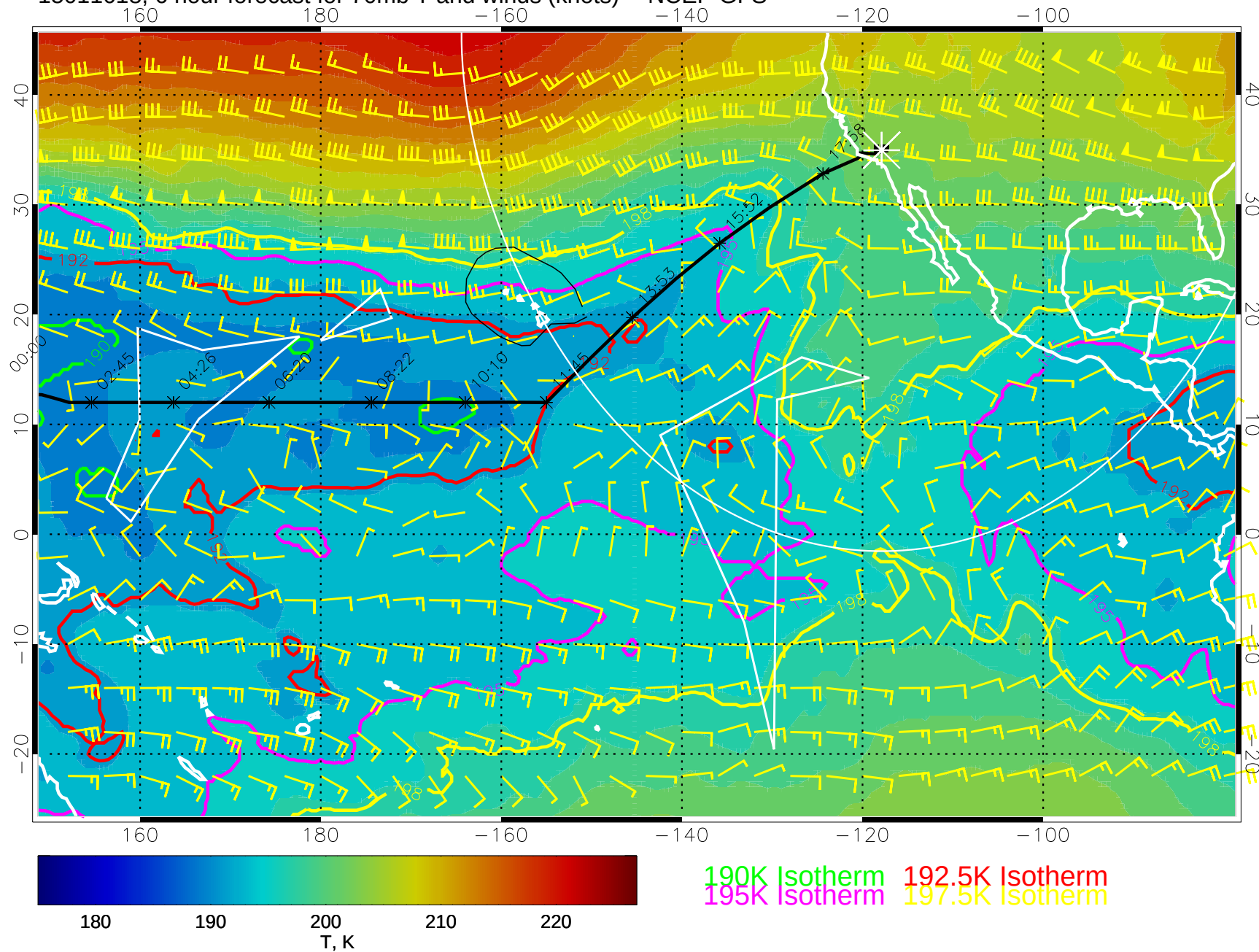
15011618, 6 hour forecast for 70mb T and winds (knots) -- NCEP GFS
