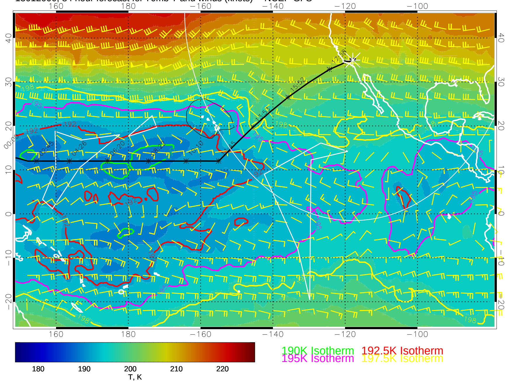
15012000, 84 hour forecast for 70mb T and winds (knots) -- NCEP GFS
