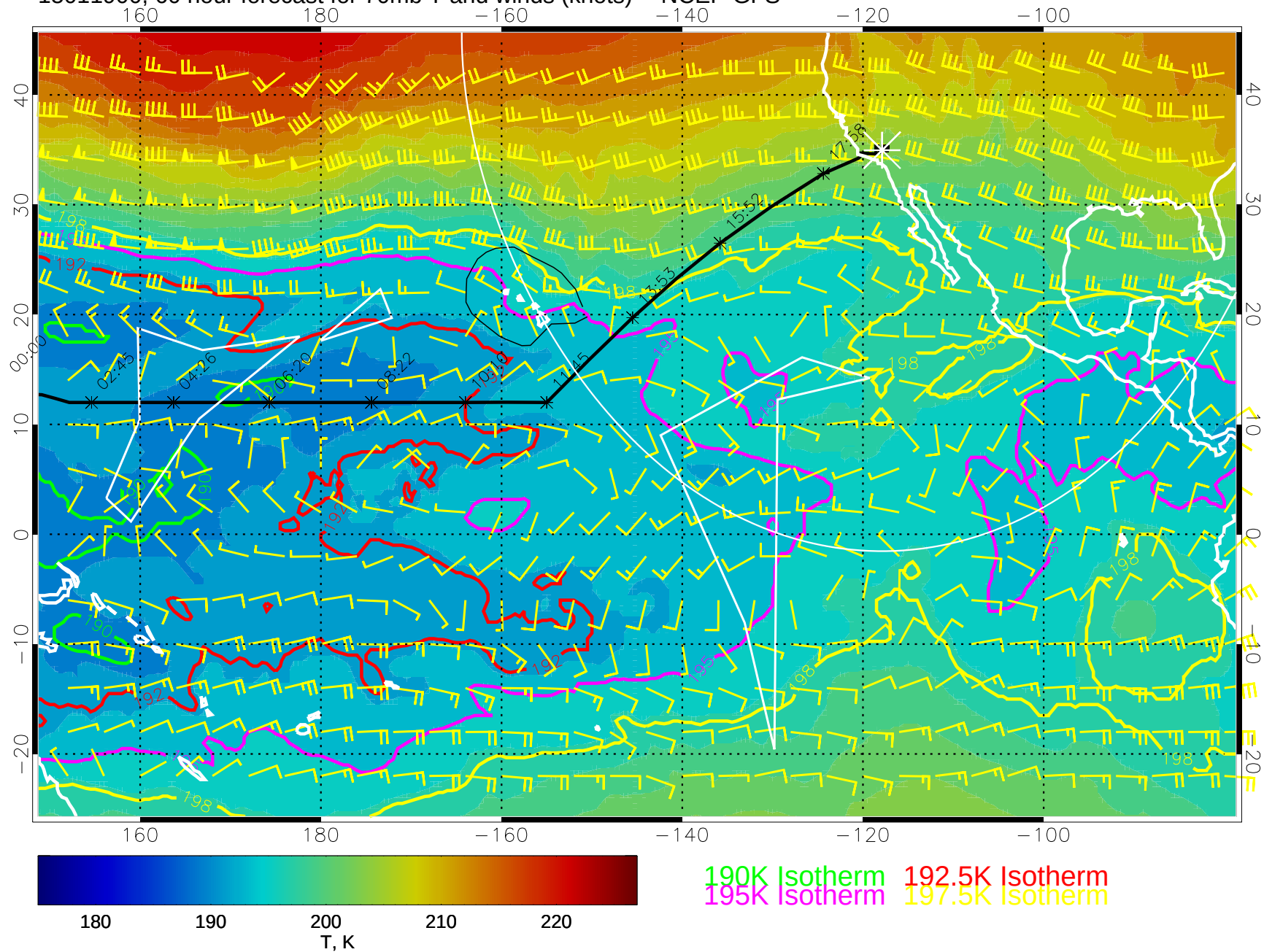
15011900, 60 hour forecast for 70mb T and winds (knots) -- NCEP GFS
