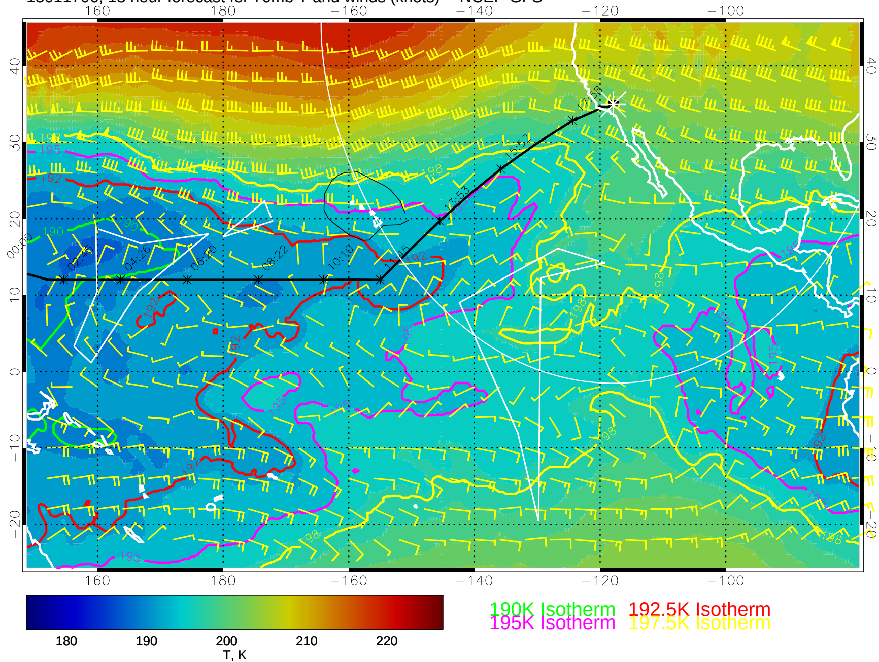
15011706, 18 hour forecast for 70mb T and winds (knots) -- NCEP GFS
