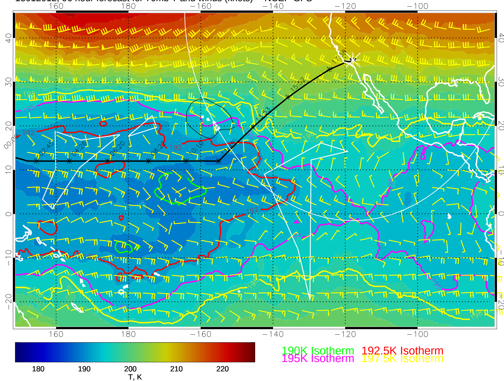
15012012, 96 hour forecast for 70mb T and winds (knots) -- NCEP GFS
