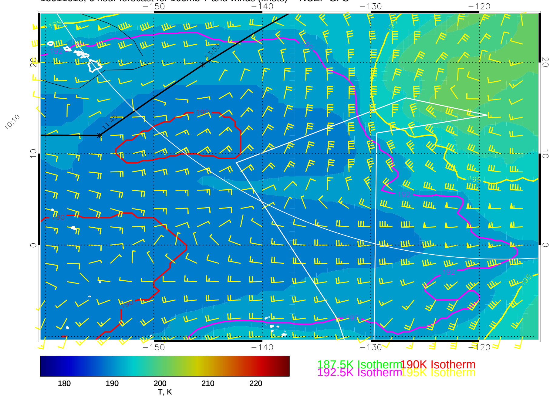
15011618, 6 hour forecast for 100mb T and winds (knots) -- NCEP GFS
