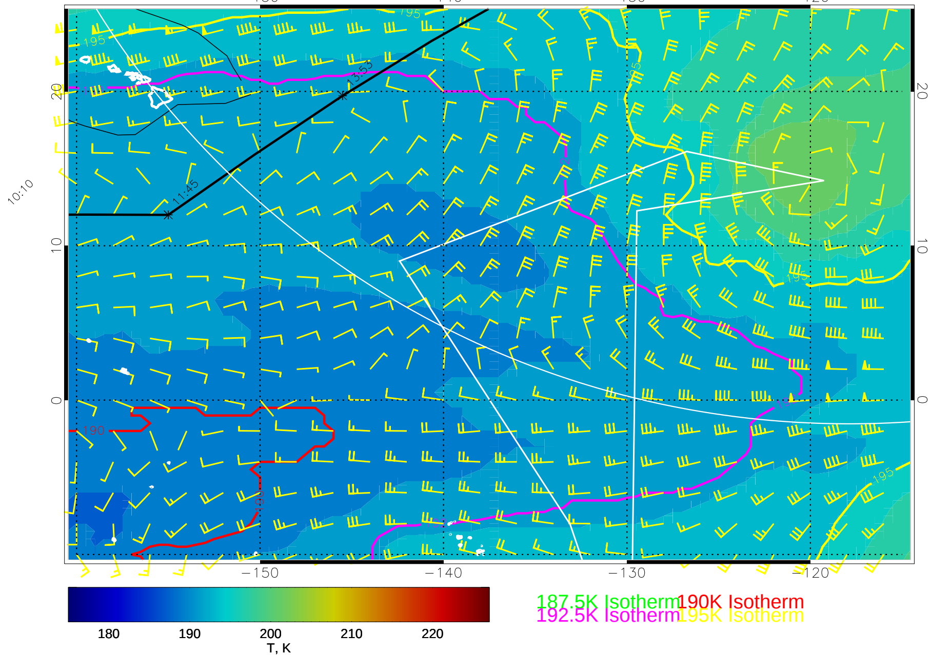
15011706, 18 hour forecast for 100mb T and winds (knots) -- NCEP GFS
