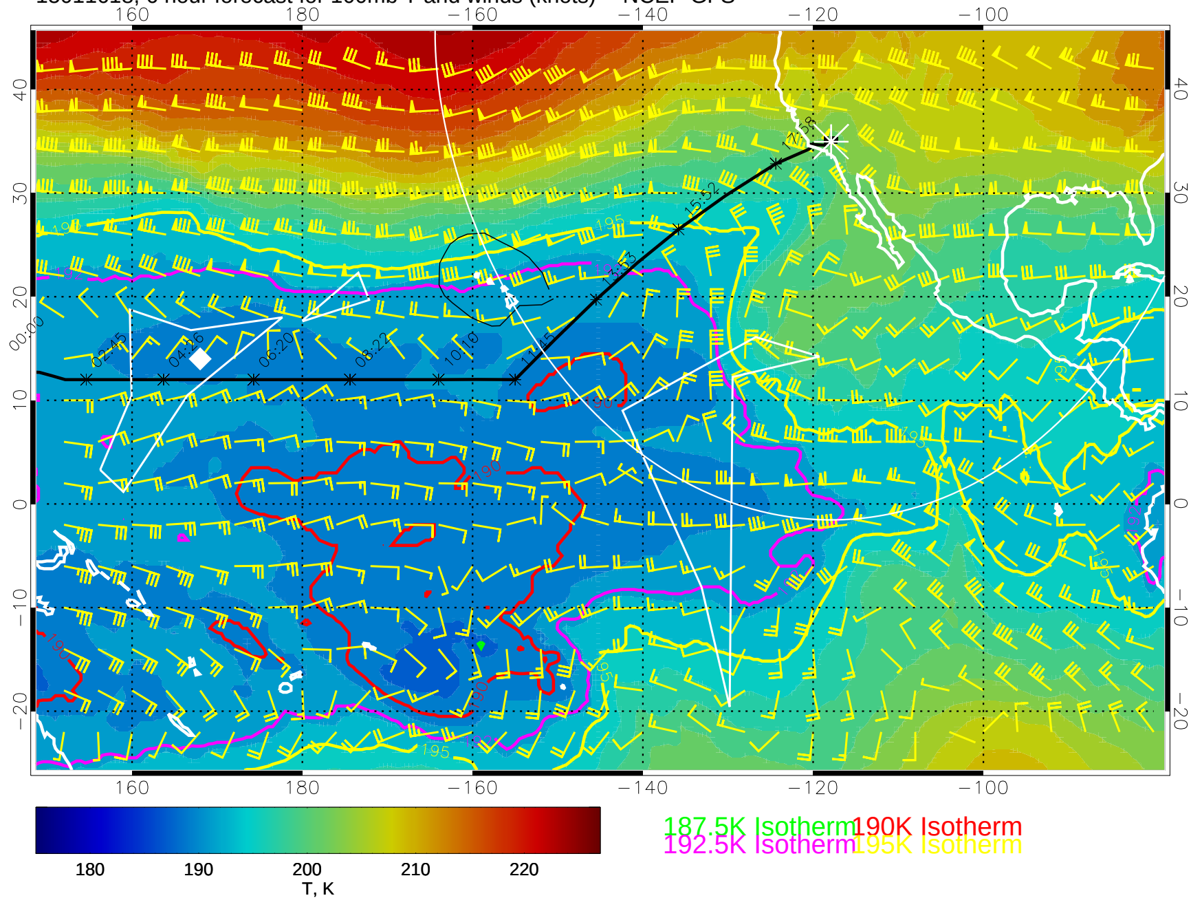
15011618, 6 hour forecast for 100mb T and winds (knots) -- NCEP GFS
