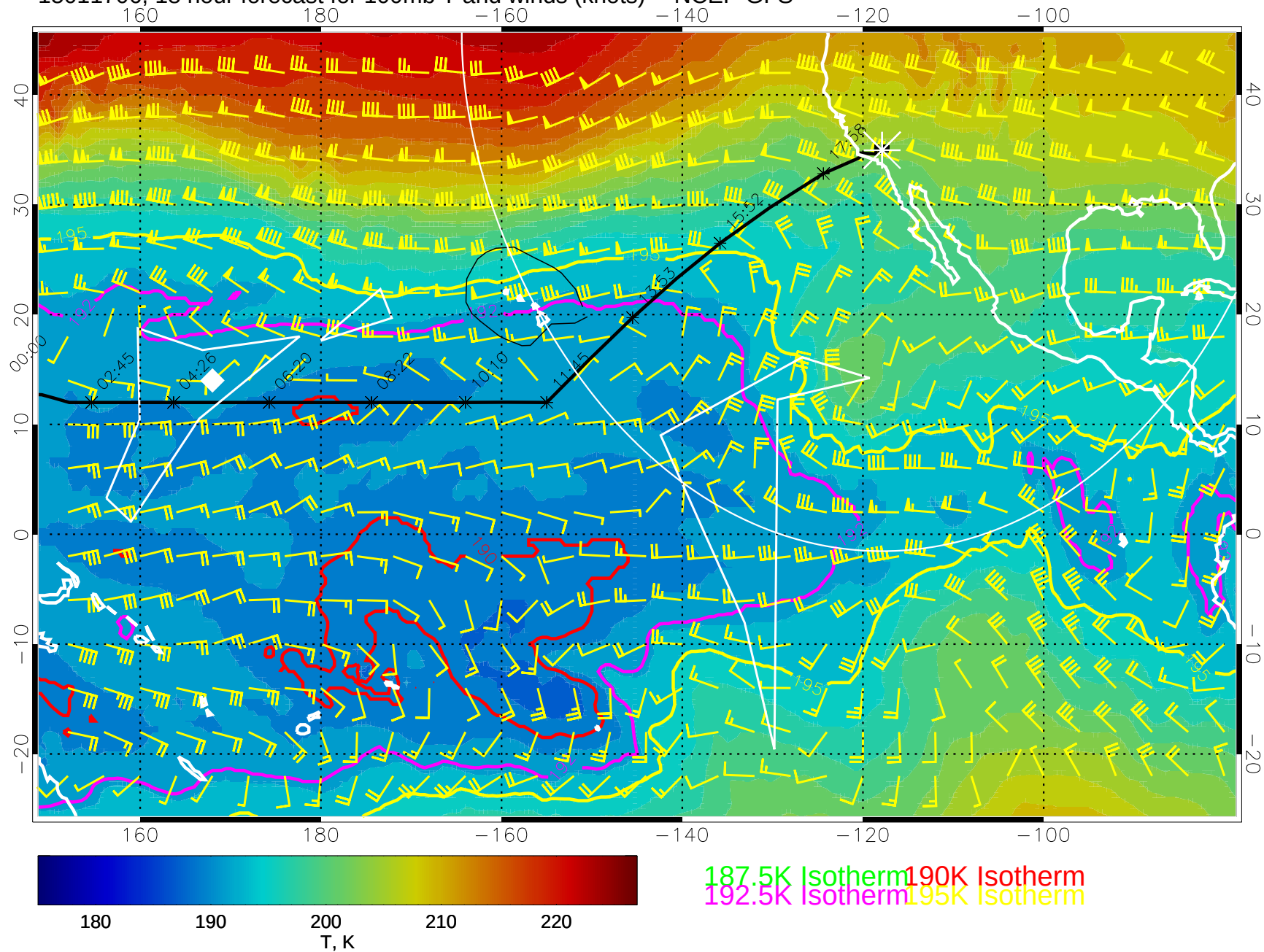
15011706, 18 hour forecast for 100mb T and winds (knots) -- NCEP GFS
