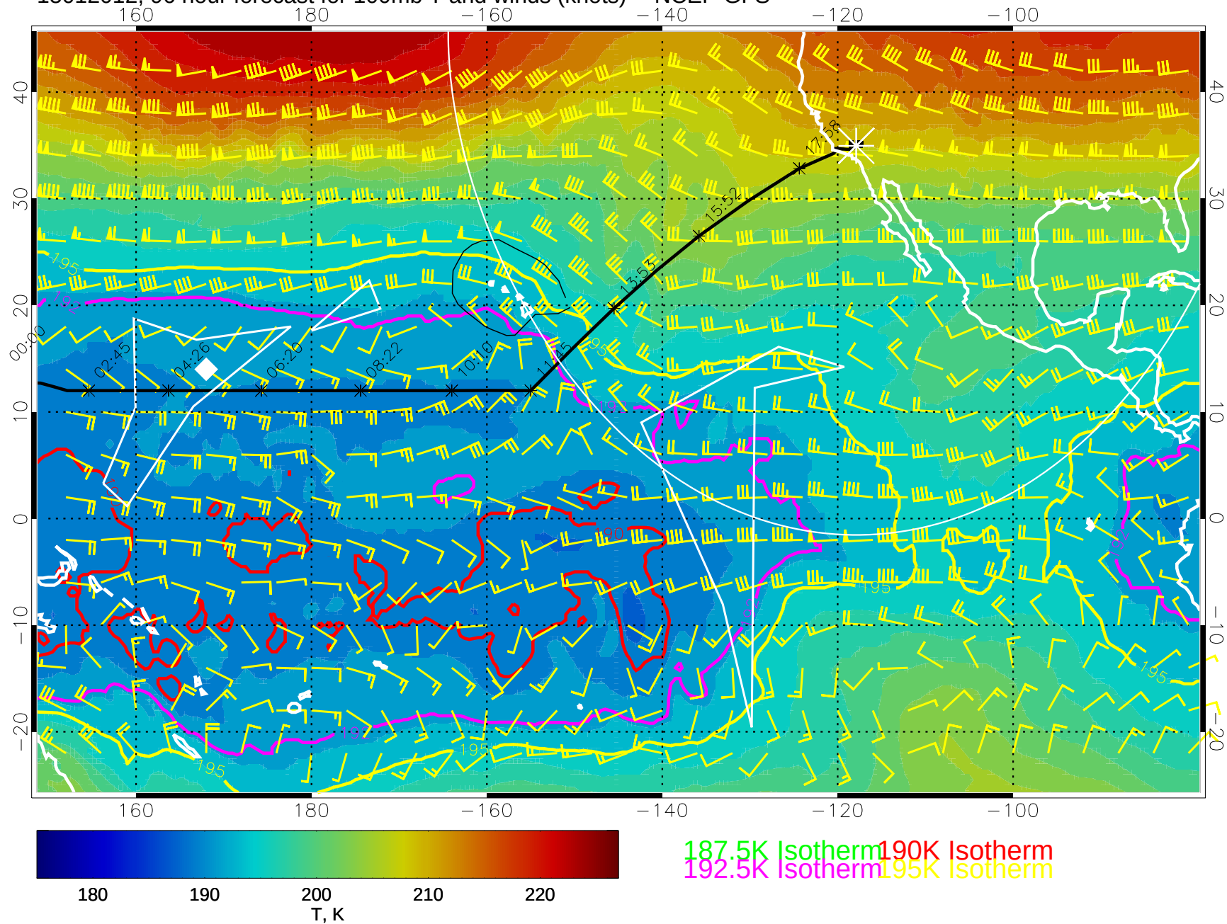
15012012, 96 hour forecast for 100mb T and winds (knots) -- NCEP GFS
