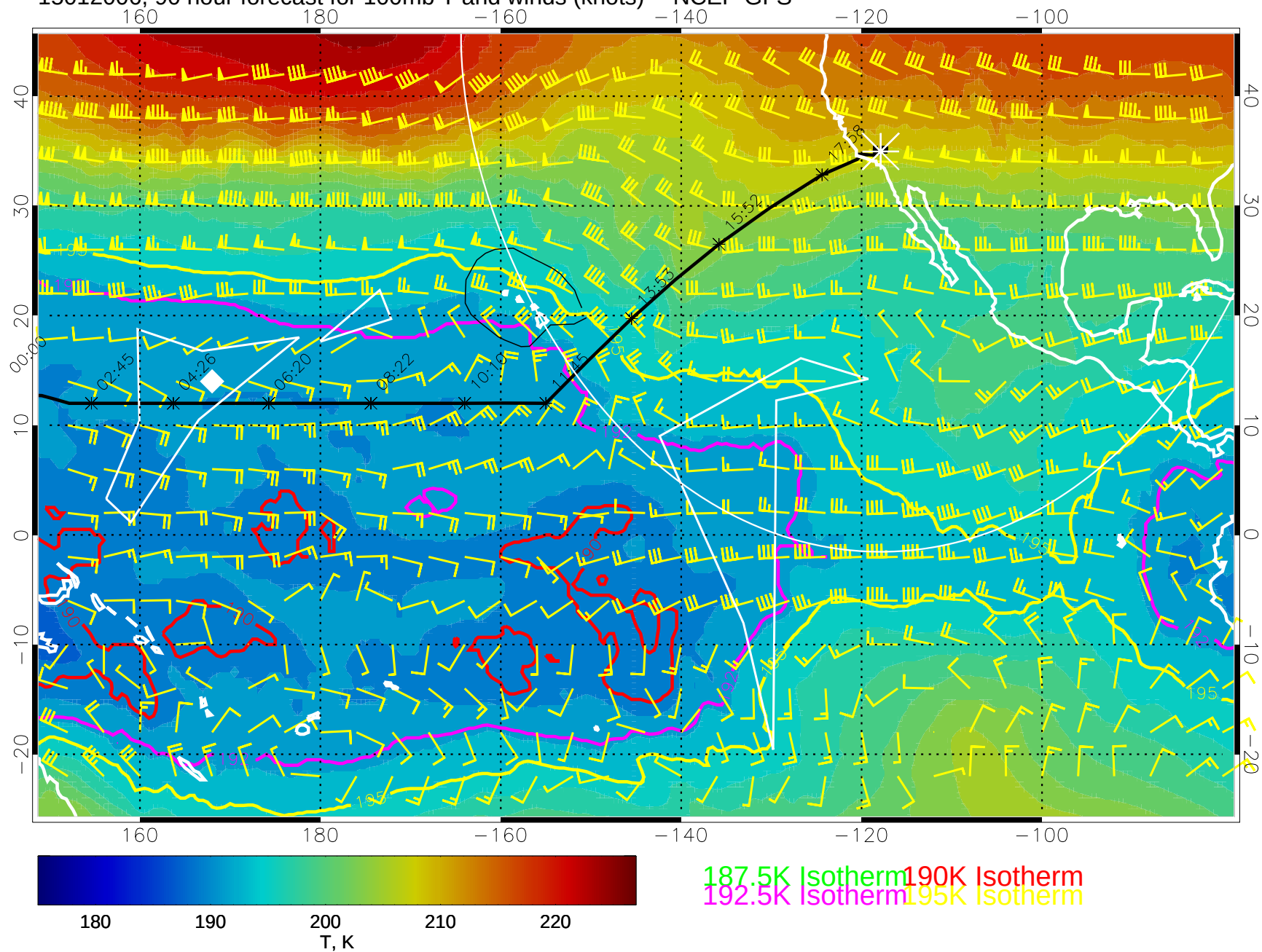
15012006, 90 hour forecast for 100mb T and winds (knots) -- NCEP GFS
