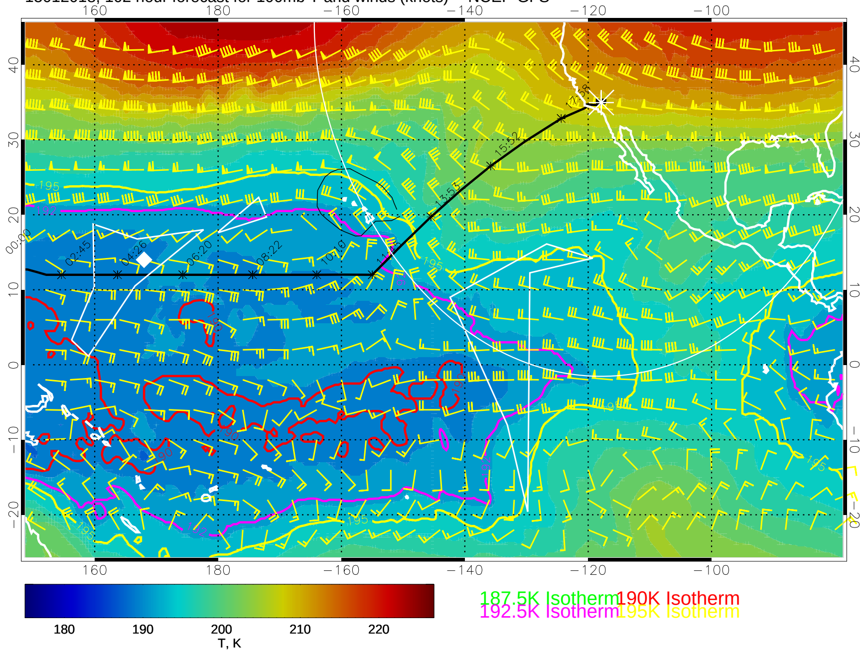
15012018, 102 hour forecast for 100mb T and winds (knots) -- NCEP GFS
