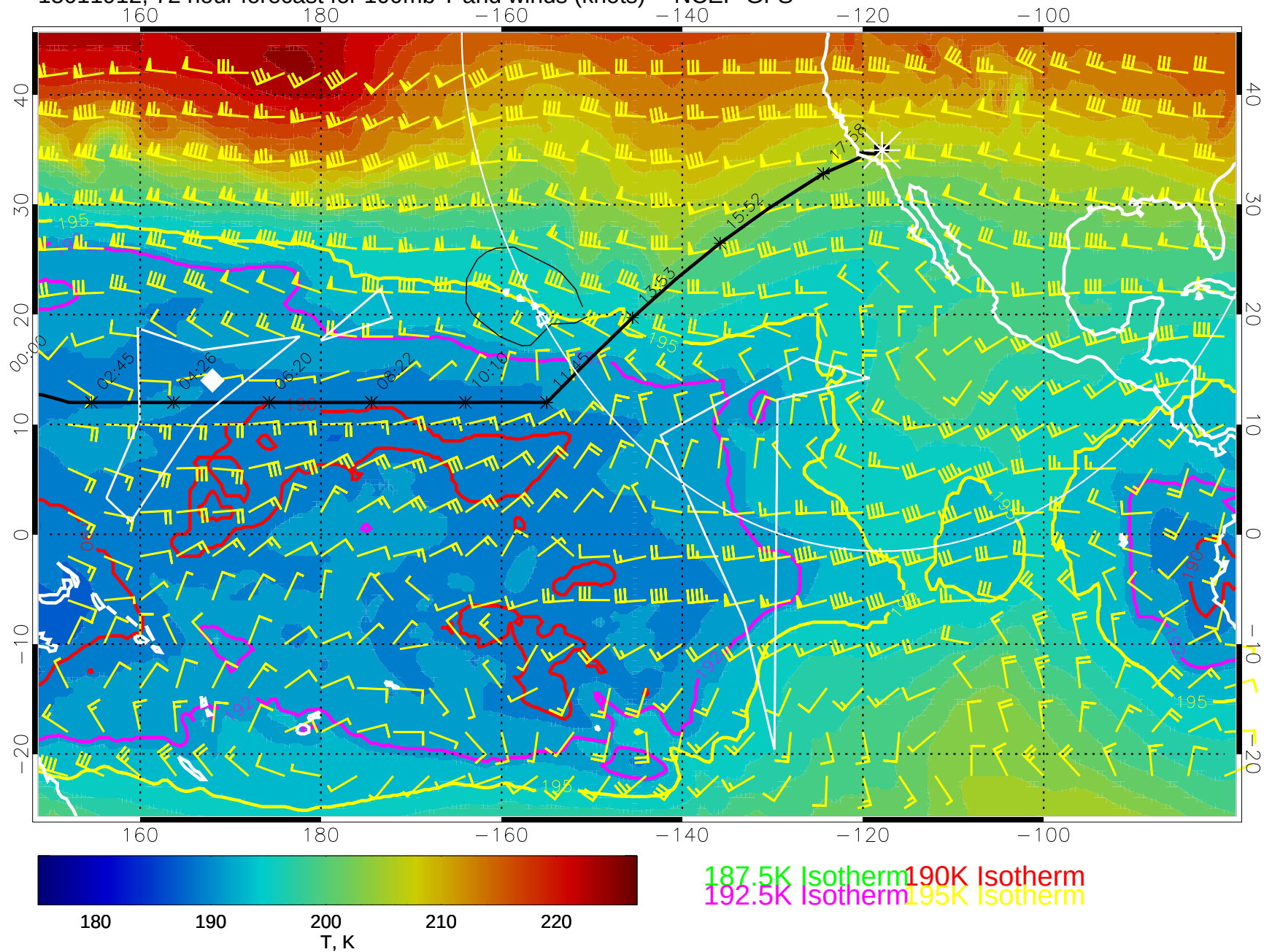
15011912, 72 hour forecast for 100mb T and winds (knots) -- NCEP GFS
