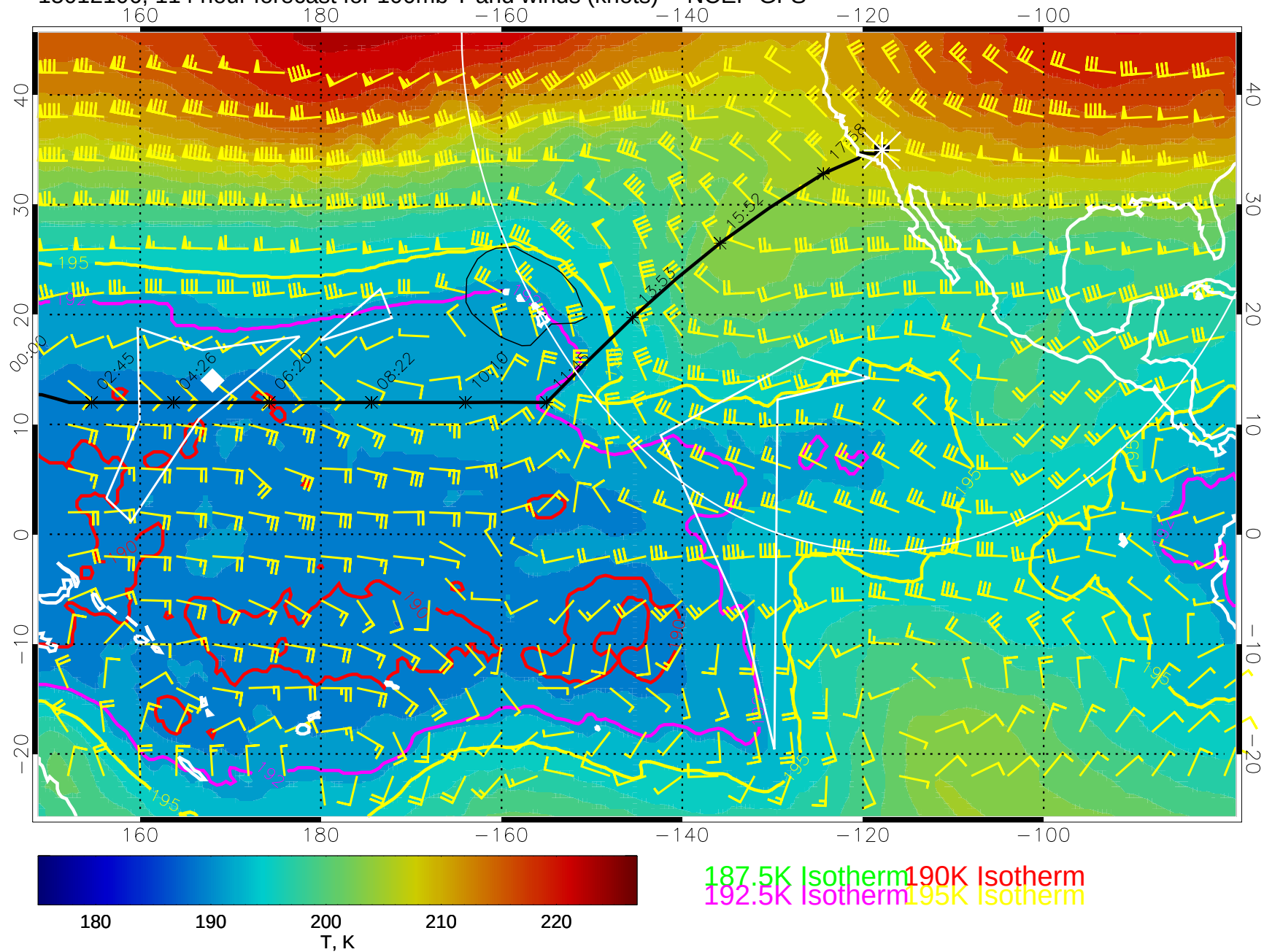
15012106, 114 hour forecast for 100mb T and winds (knots) -- NCEP GFS
