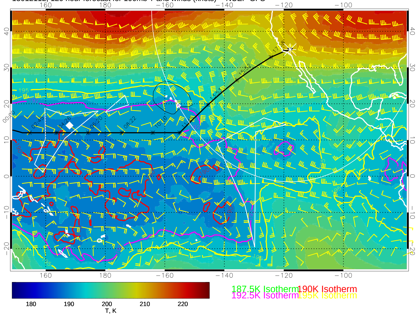
15012112, 120 hour forecast for 100mb T and winds (knots) -- NCEP GFS
