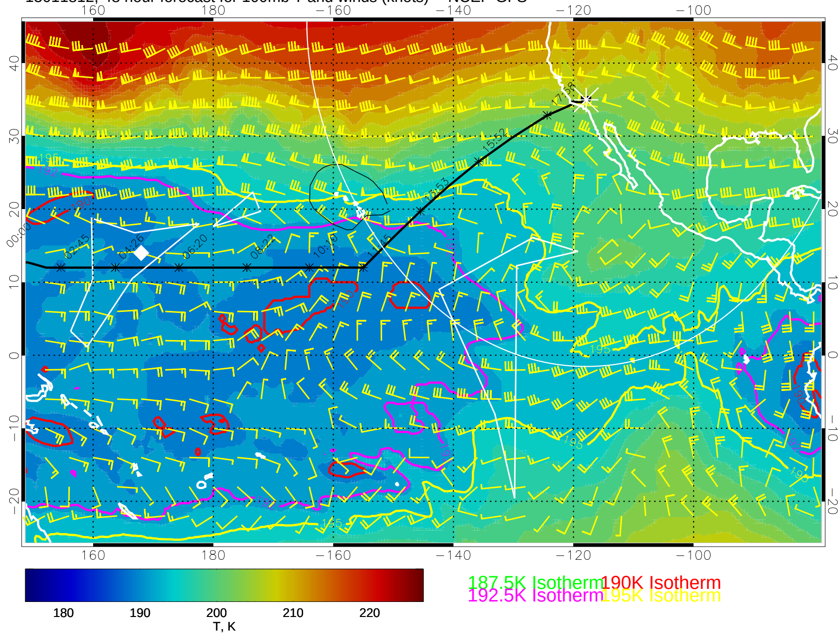
15011812, 48 hour forecast for 100mb T and winds (knots) -- NCEP GFS
