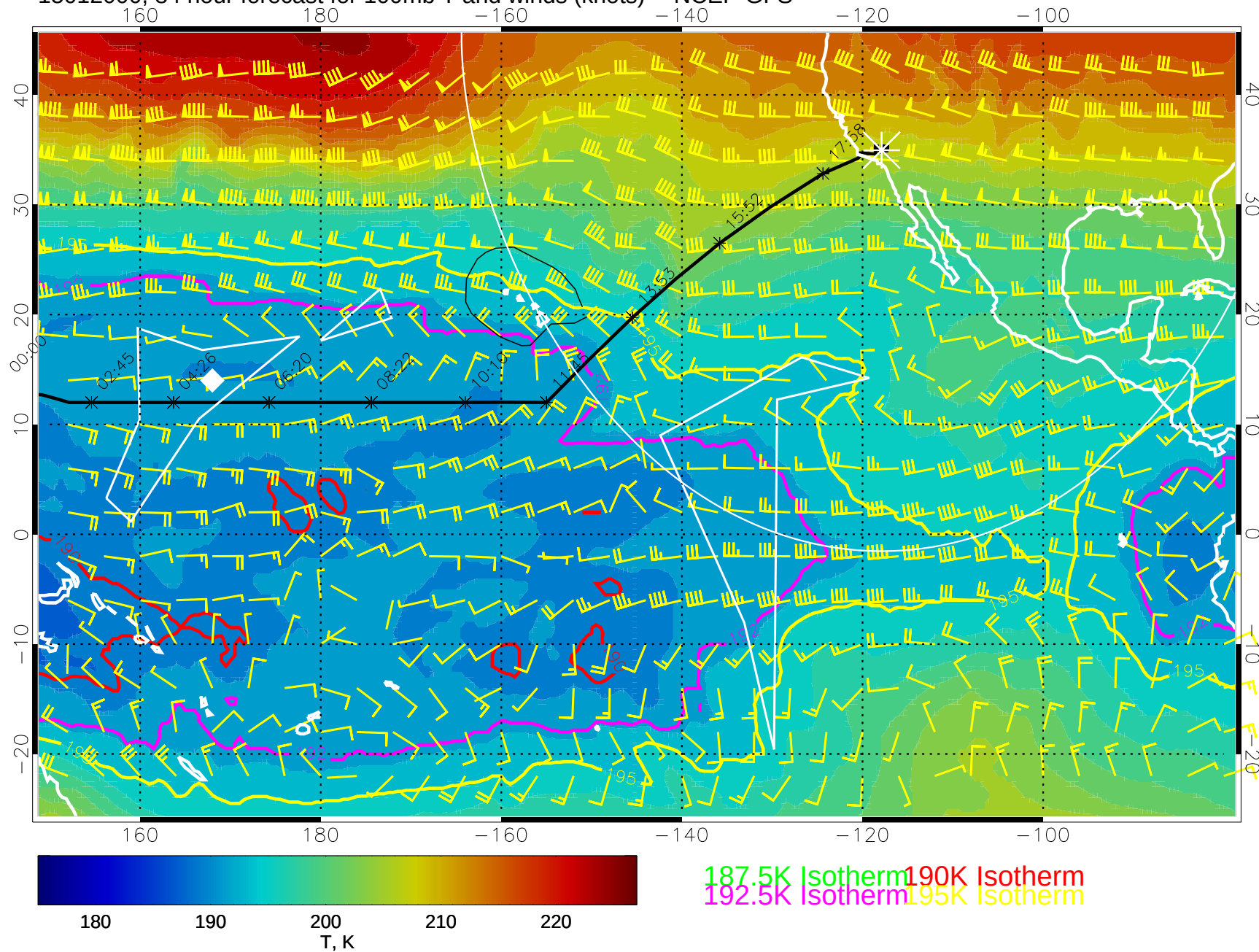
15012000, 84 hour forecast for 100mb T and winds (knots) -- NCEP GFS
