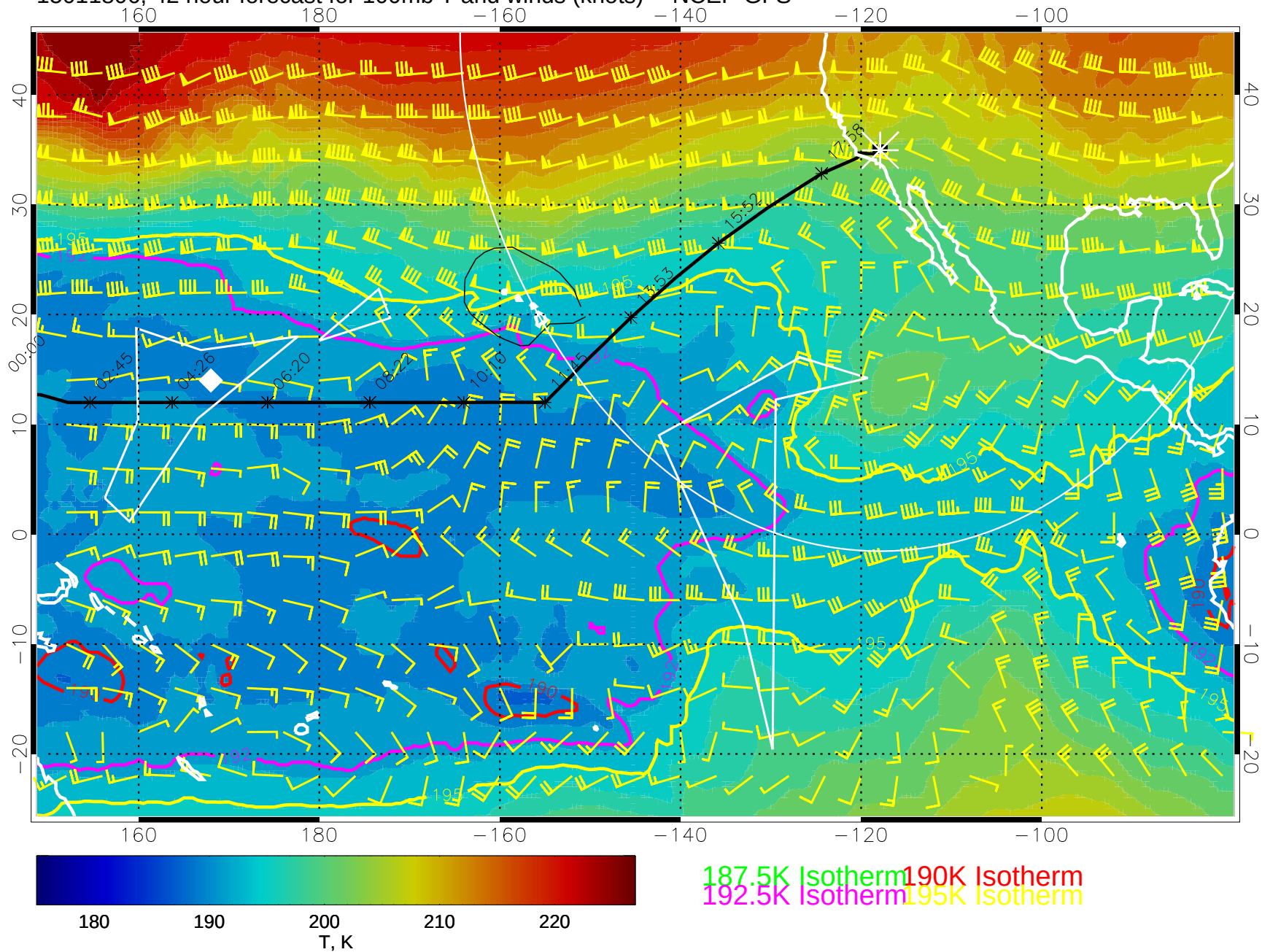
15011806, 42 hour forecast for 100mb T and winds (knots) -- NCEP GFS
