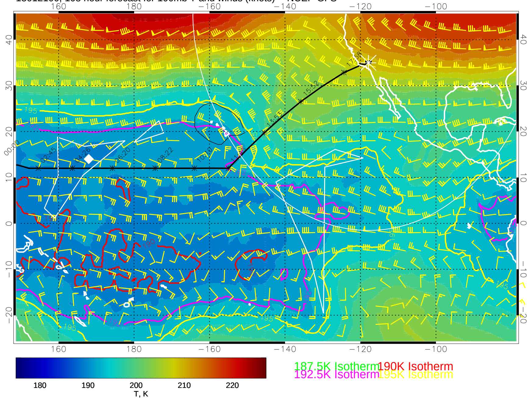
15012100, 108 hour forecast for 100mb T and winds (knots) -- NCEP GFS
