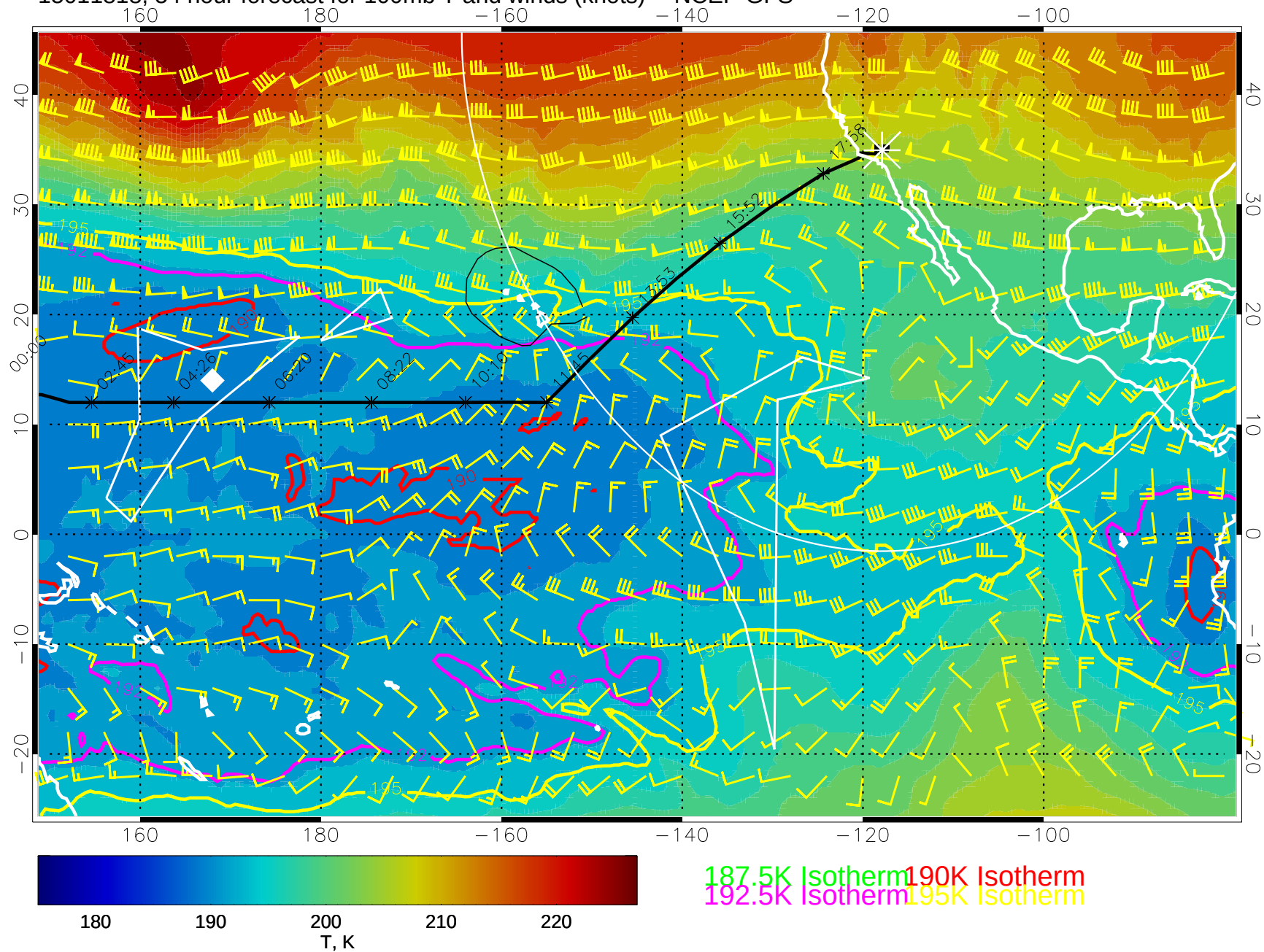
15011818, 54 hour forecast for 100mb T and winds (knots) -- NCEP GFS
