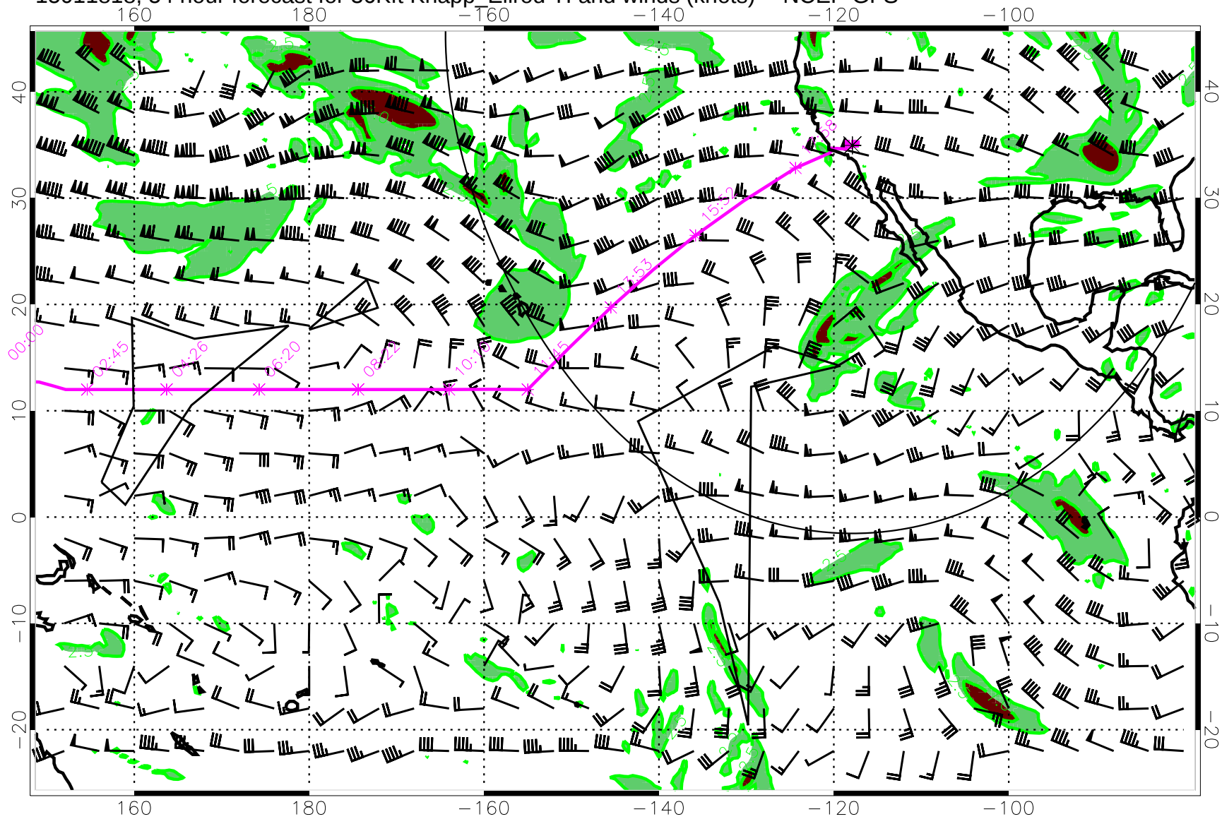
15011818, 54 hour forecast for 36Kft Knapp_Ellrod TI and winds (knots) -- NCEP GFS
