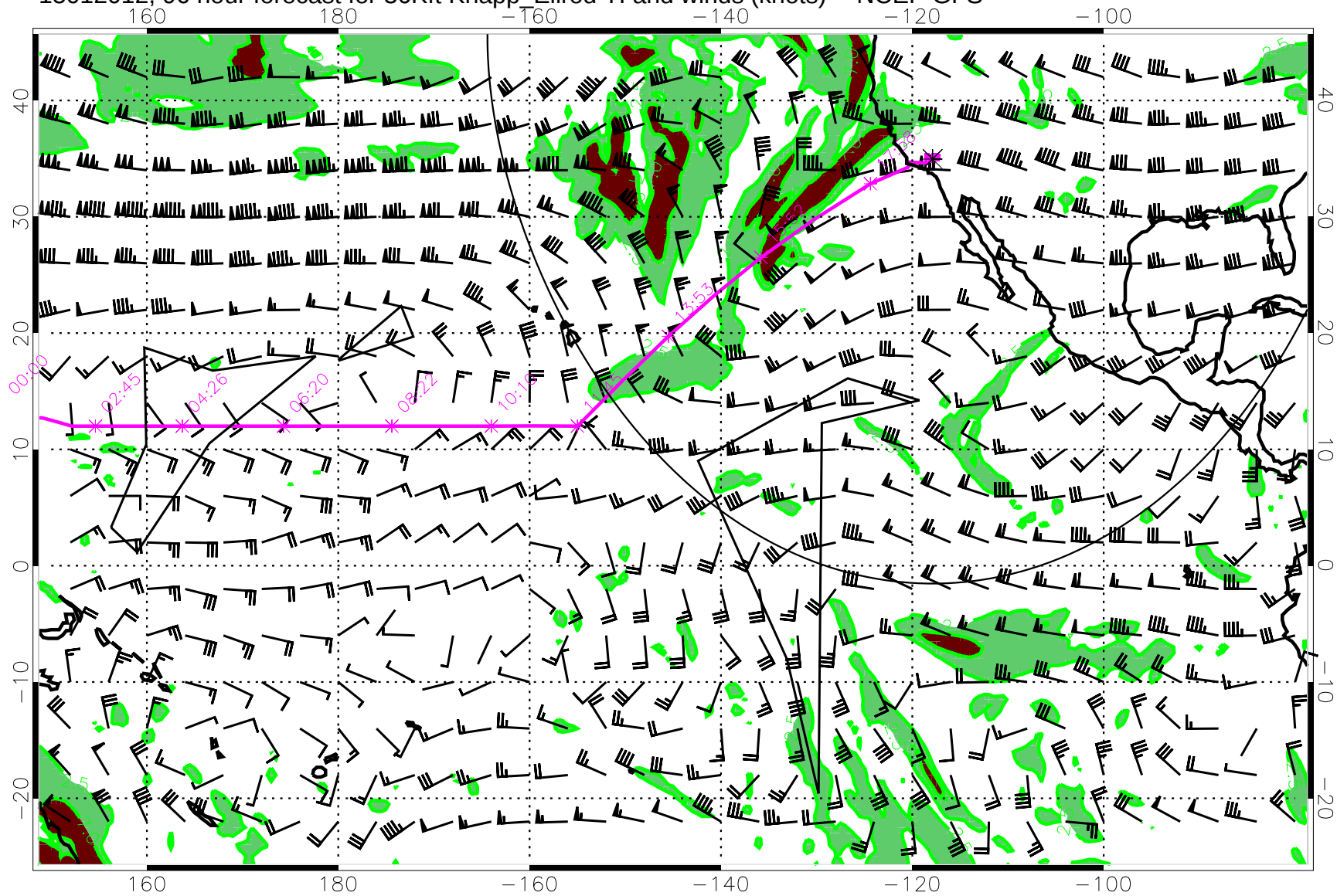
15012012, 96 hour forecast for 36Kft Knapp_Ellrod TI and winds (knots) -- NCEP GFS
