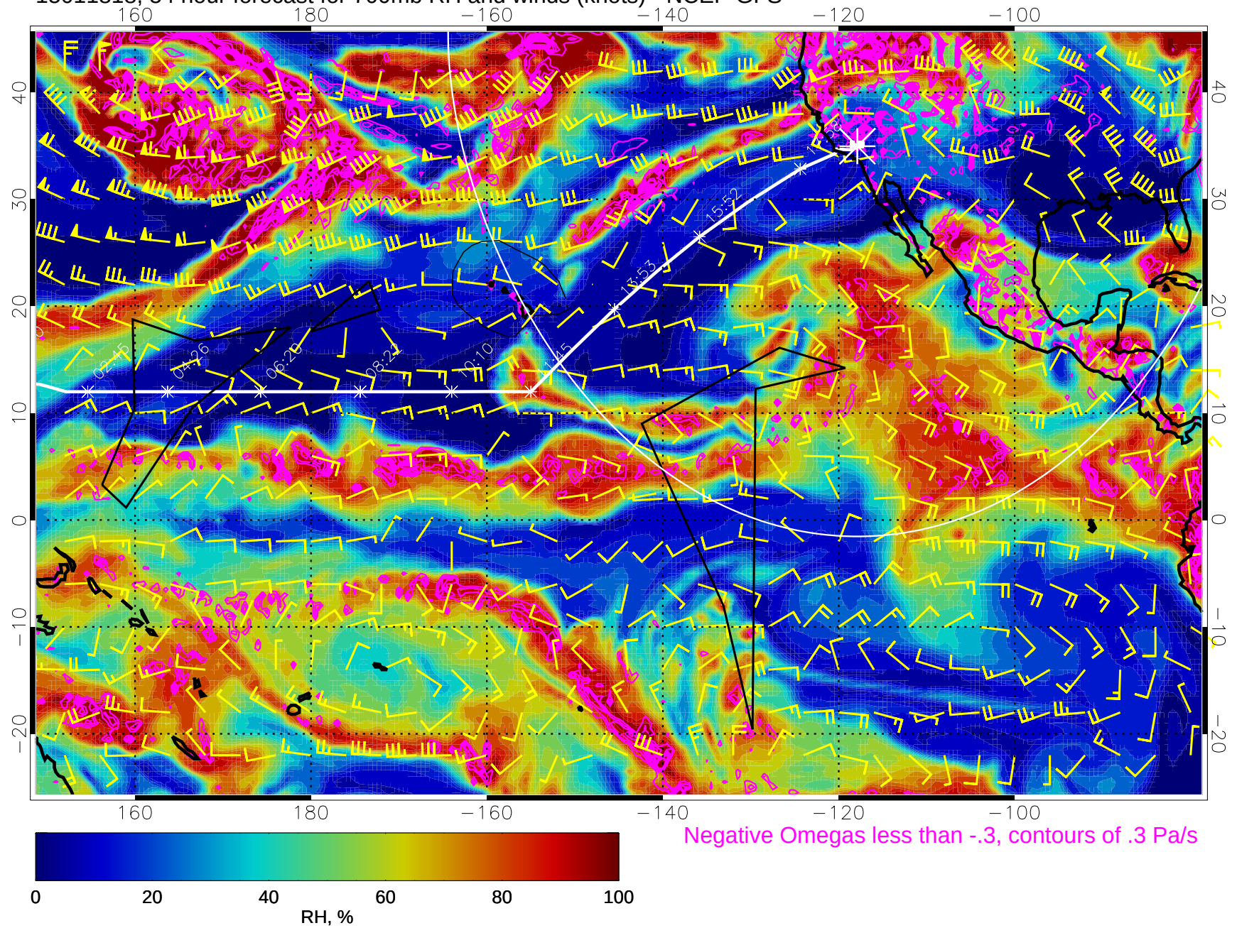
15011818, 54 hour forecast for 700mb RH and winds (knots) - NCEP GFS
