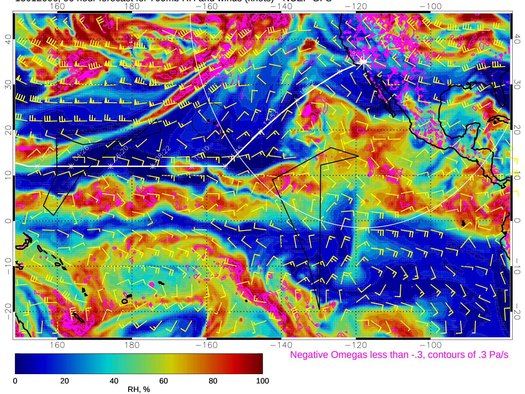
15012006, 90 hour forecast for 700mb RH and winds (knots) - NCEP GFS
