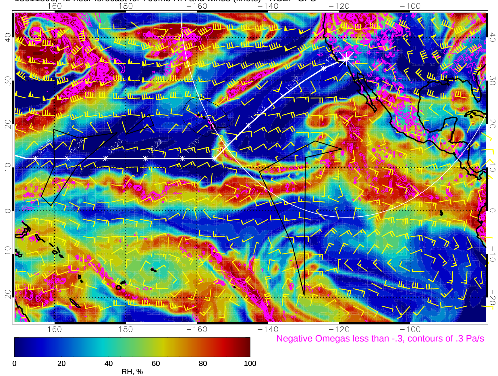
15011806, 42 hour forecast for 700mb RH and winds (knots) - NCEP GFS
