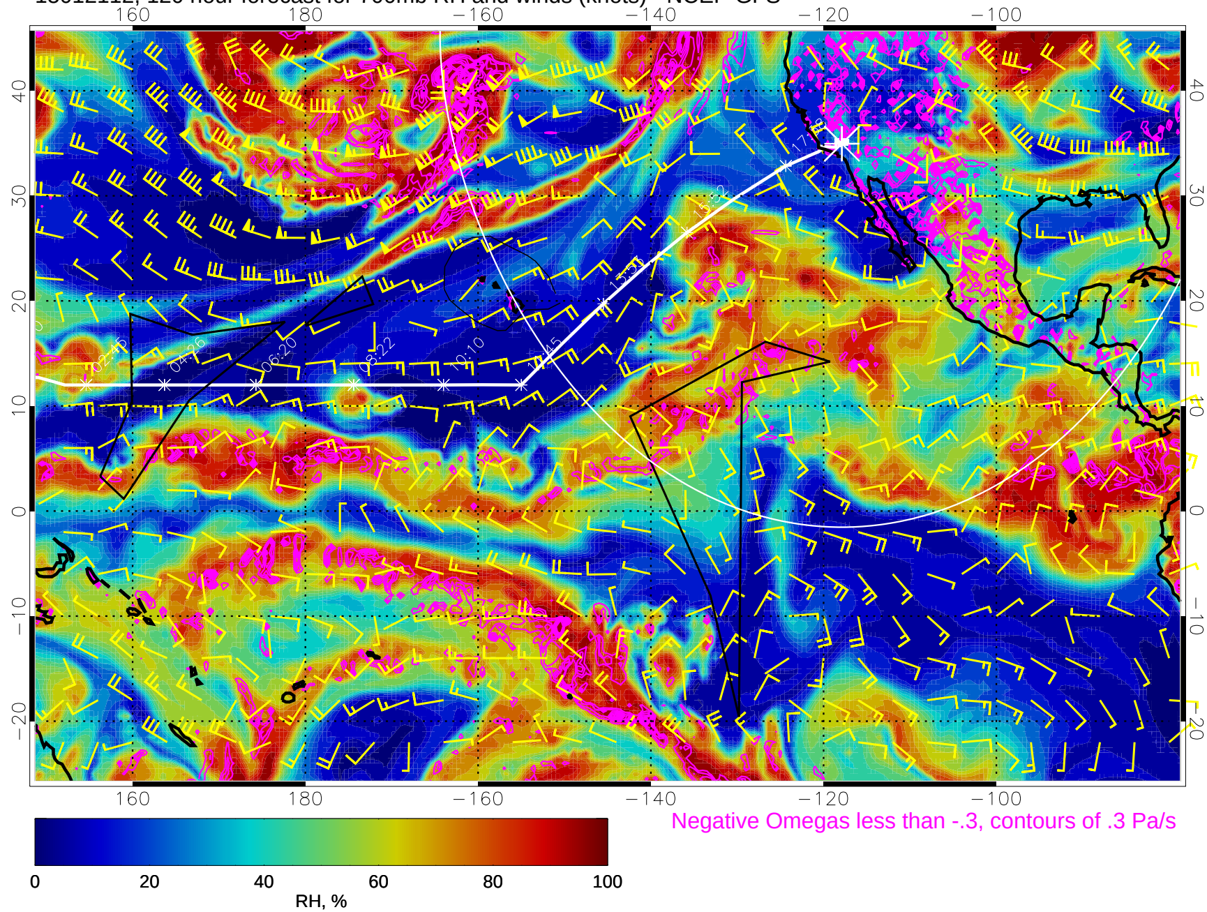
15012112, 120 hour forecast for 700mb RH and winds (knots) - NCEP GFS
