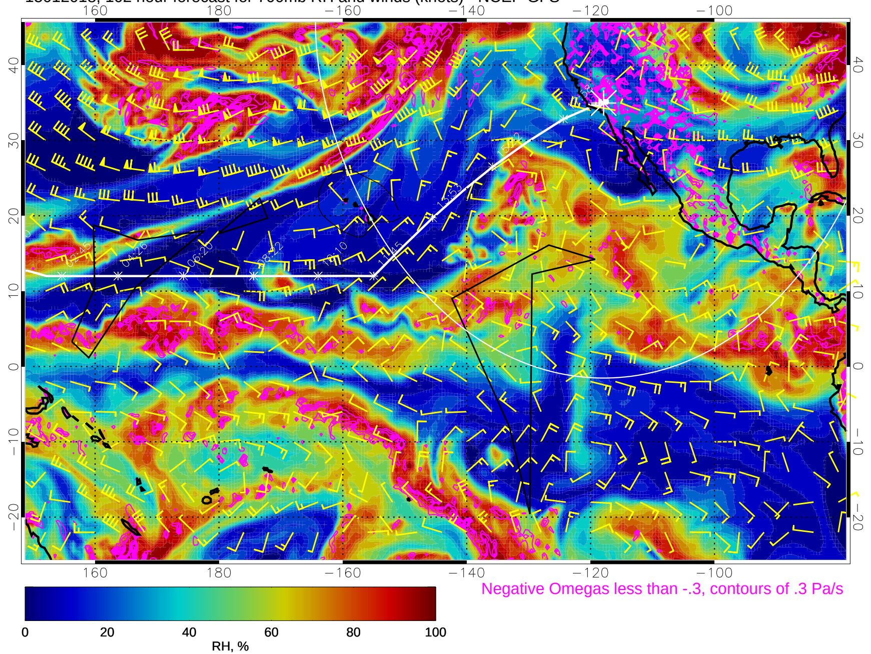
15012018, 102 hour forecast for 700mb RH and winds (knots) - NCEP GFS
