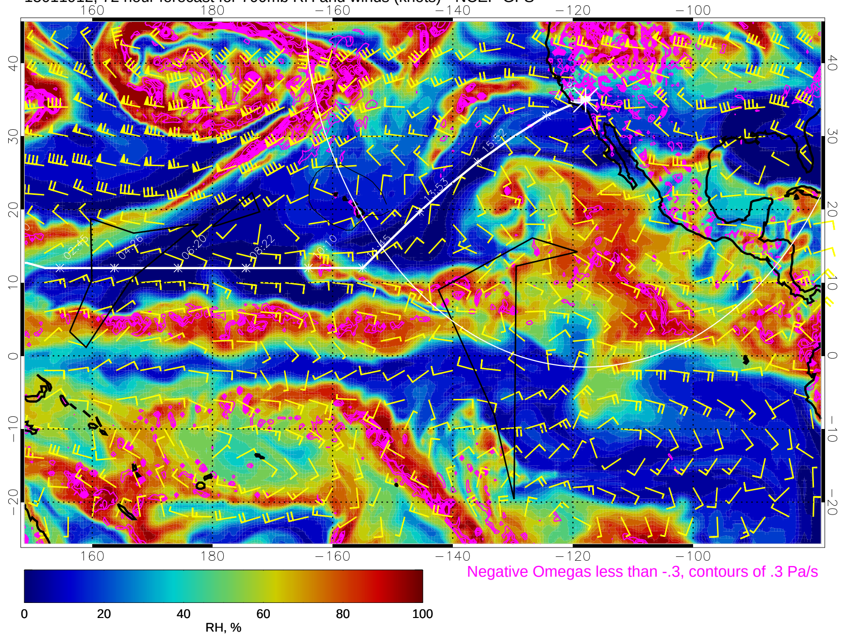
15011912, 72 hour forecast for 700mb RH and winds (knots) - NCEP GFS
