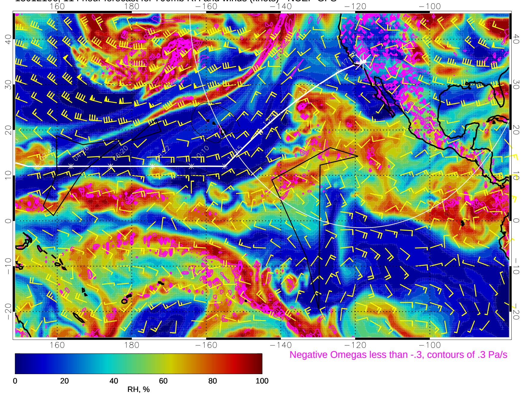
15012106, 114 hour forecast for 700mb RH and winds (knots) - NCEP GFS
