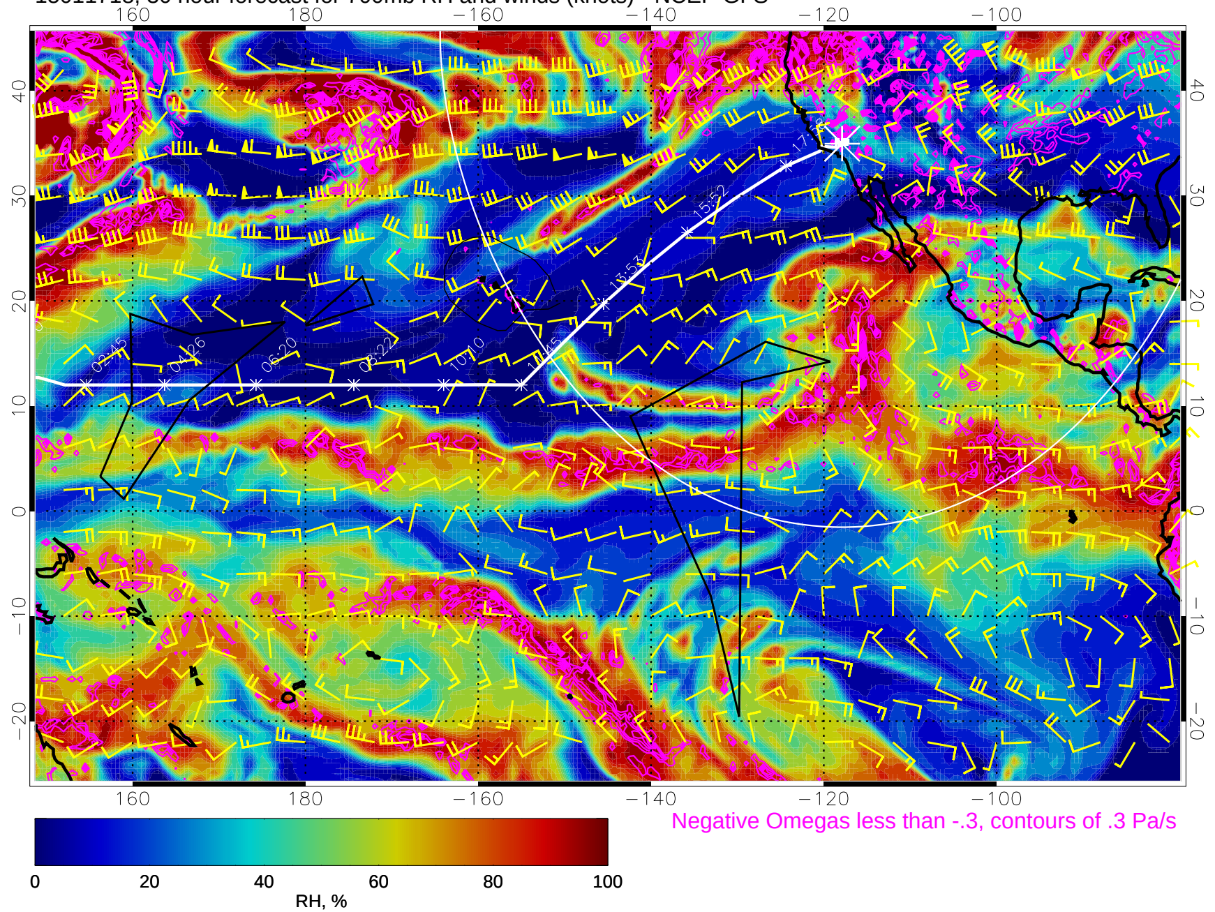
15011718, 30 hour forecast for 700mb RH and winds (knots) - NCEP GFS
