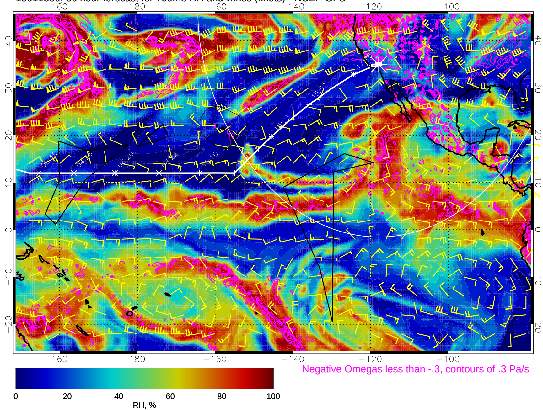
15011800, 36 hour forecast for 700mb RH and winds (knots) - NCEP GFS
