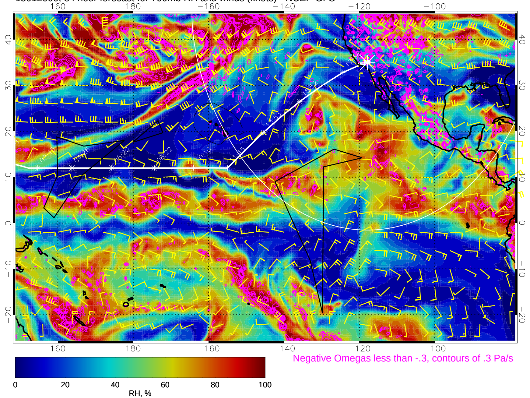
15012000, 84 hour forecast for 700mb RH and winds (knots) - NCEP GFS
