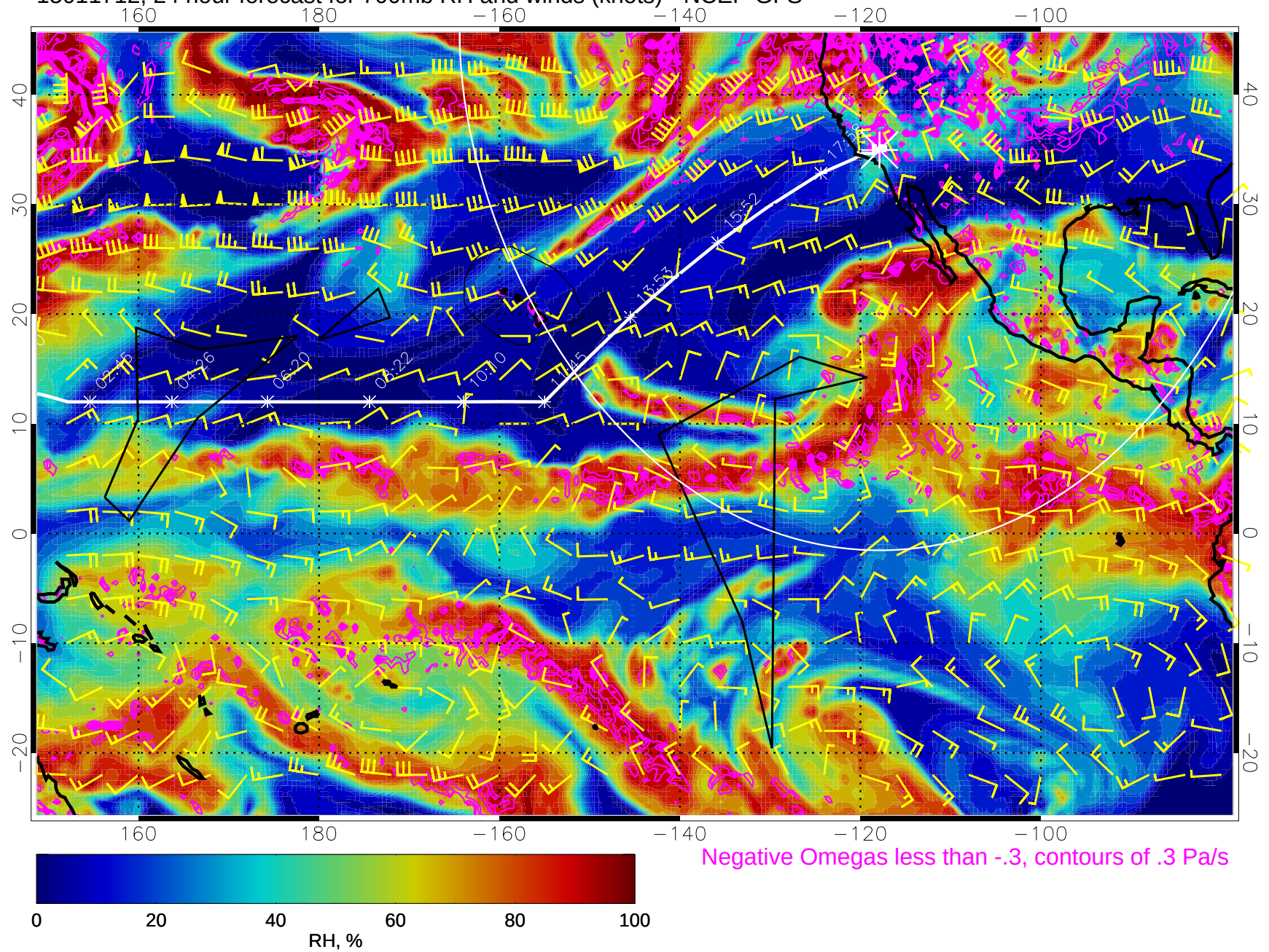
15011712, 24 hour forecast for 700mb RH and winds (knots) - NCEP GFS
