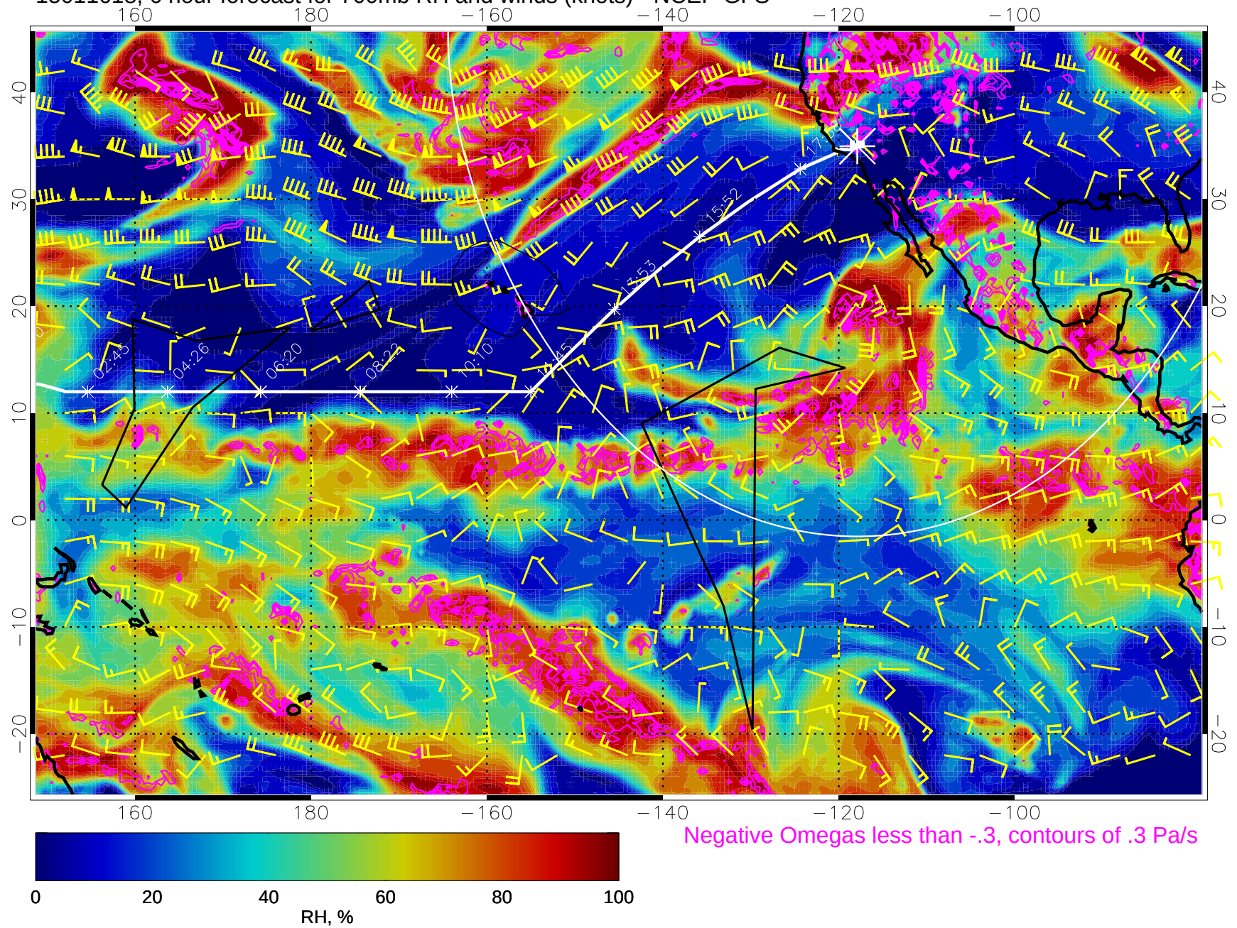
15011618, 6 hour forecast for 700mb RH and winds (knots) - NCEP GFS
