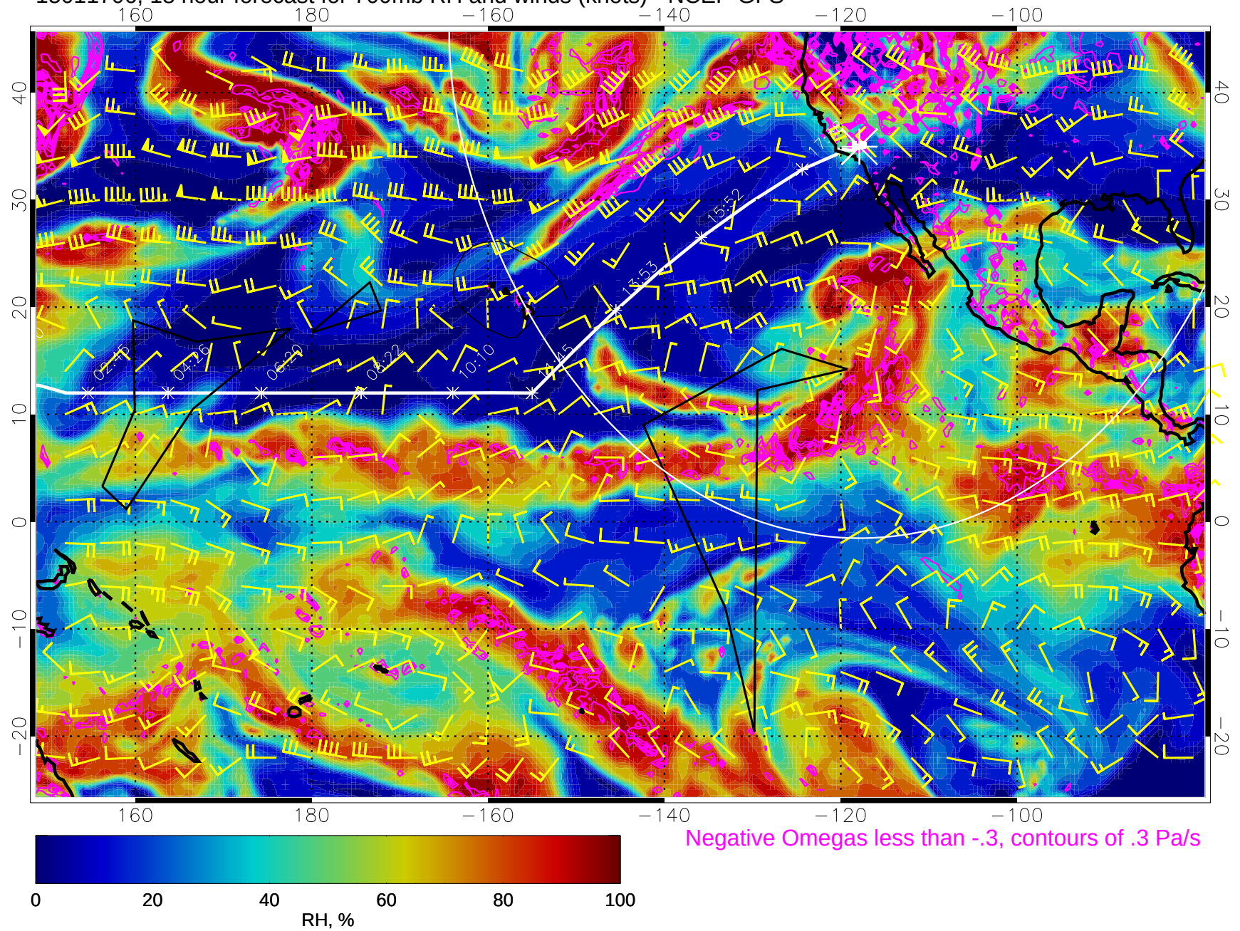
15011706, 18 hour forecast for 700mb RH and winds (knots) - NCEP GFS
