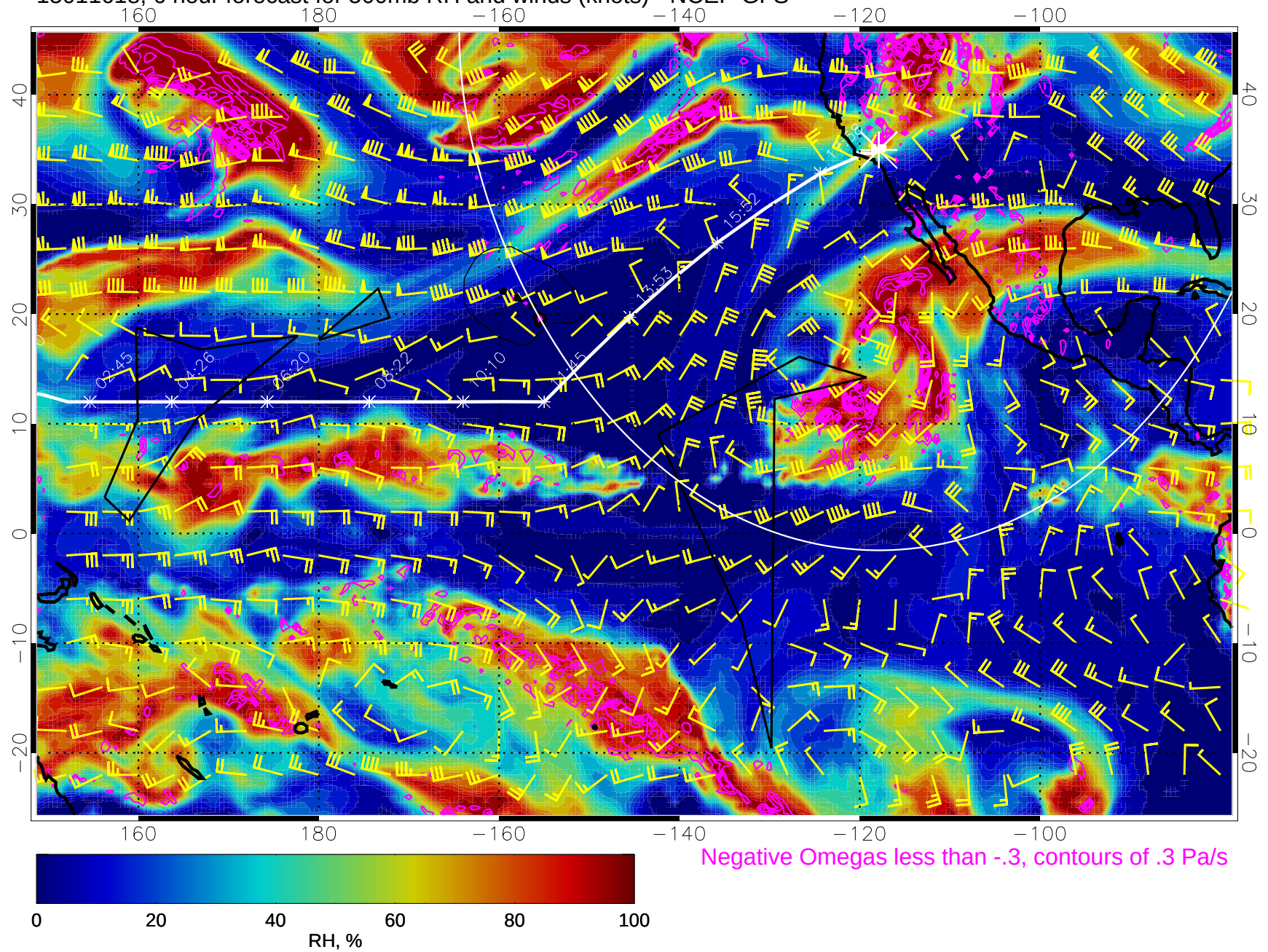
15011618, 6 hour forecast for 500mb RH and winds (knots) - NCEP GFS
