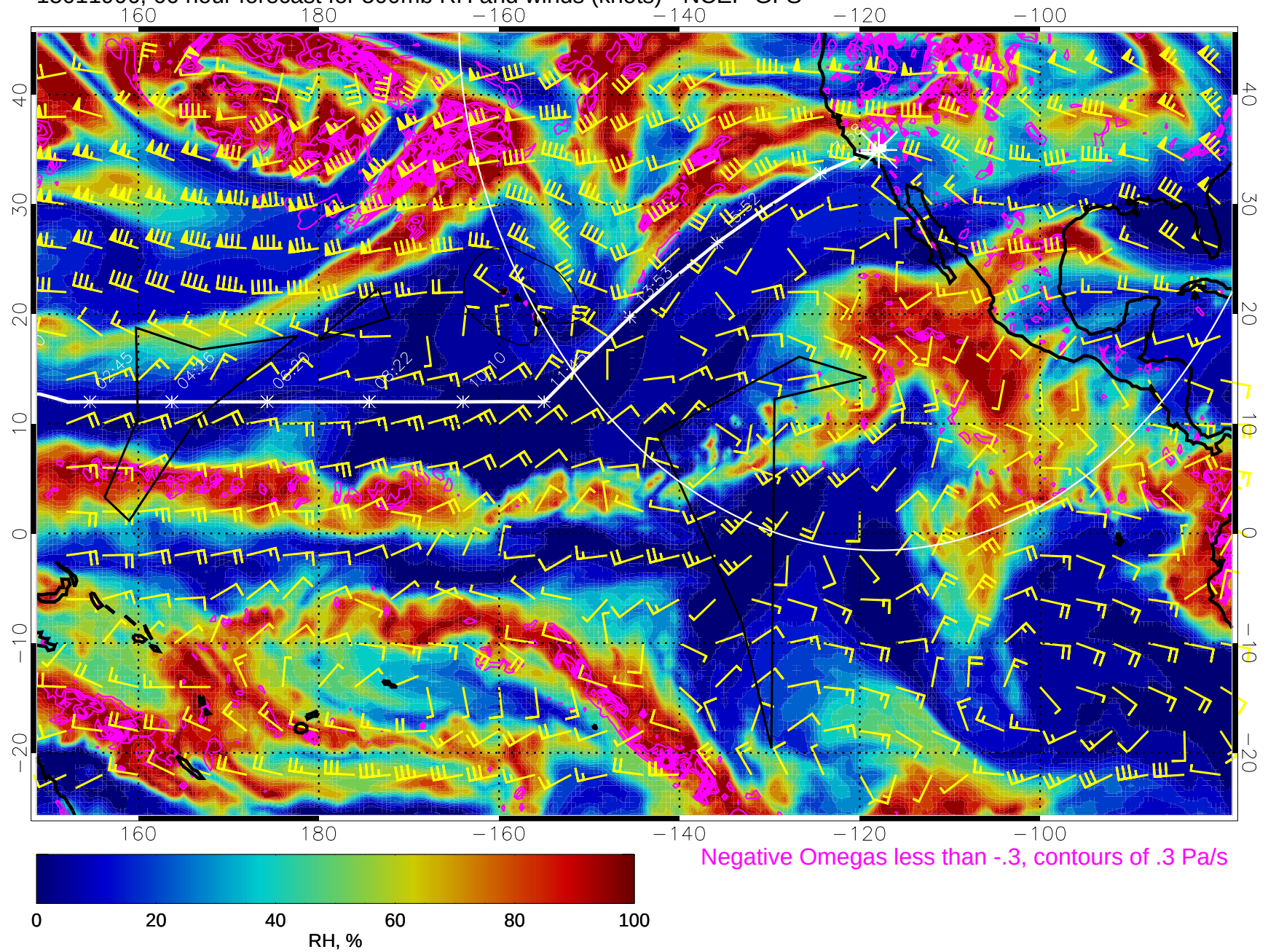
15011906, 66 hour forecast for 500mb RH and winds (knots) - NCEP GFS
