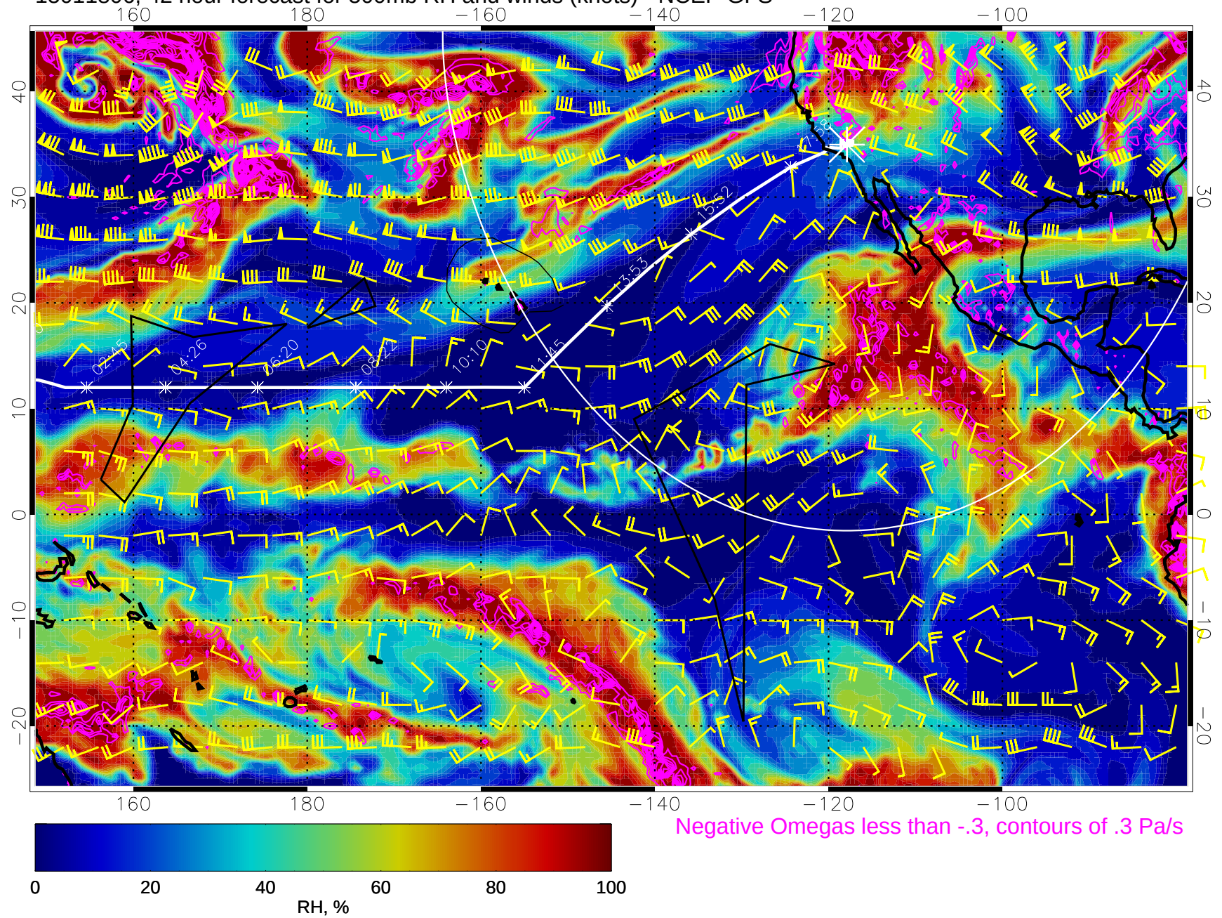
15011806, 42 hour forecast for 500mb RH and winds (knots) - NCEP GFS
