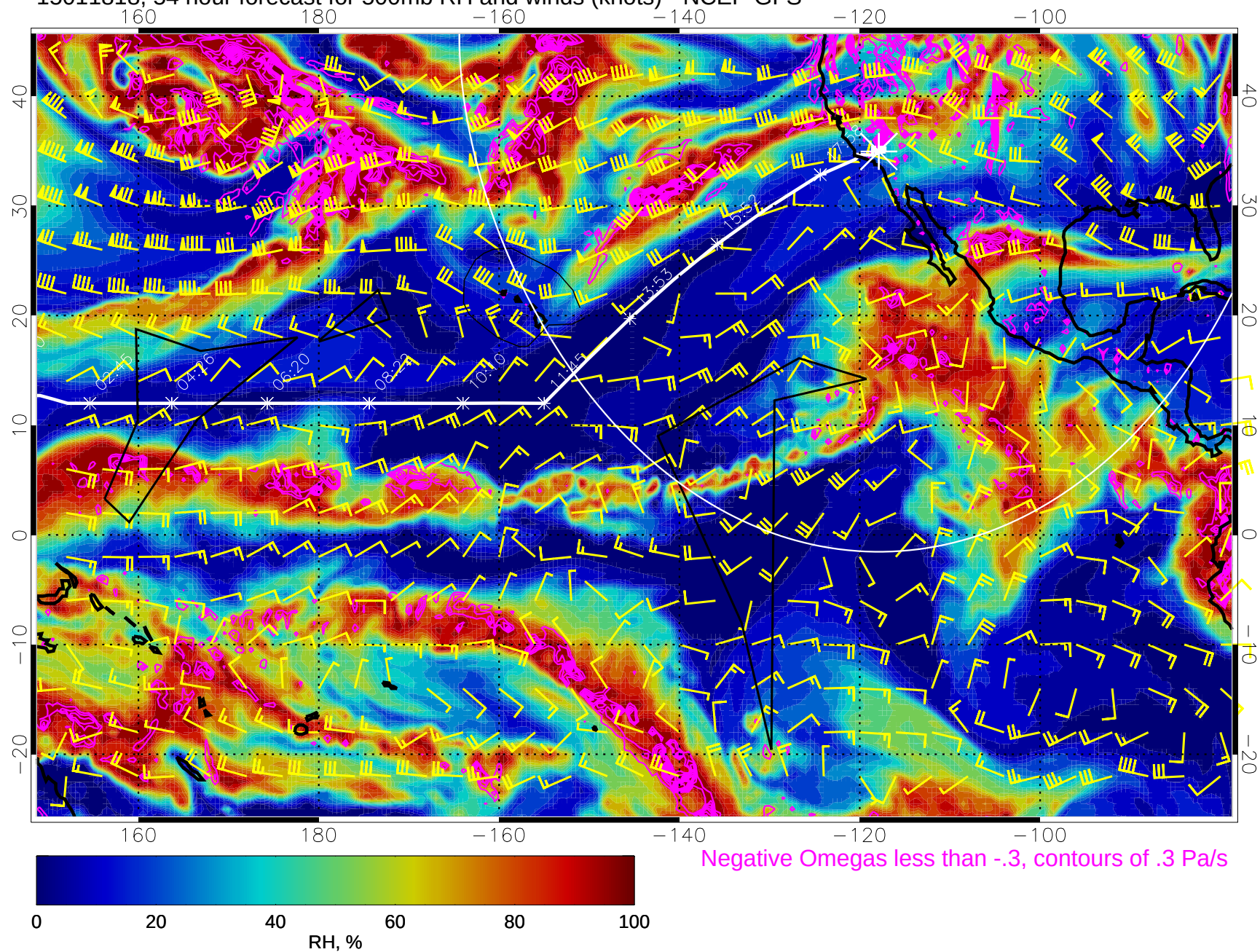
15011818, 54 hour forecast for 500mb RH and winds (knots) - NCEP GFS
