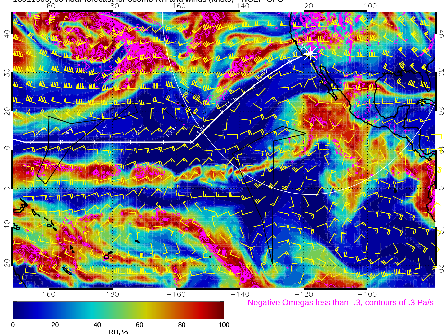
15011900, 60 hour forecast for 500mb RH and winds (knots) - NCEP GFS
