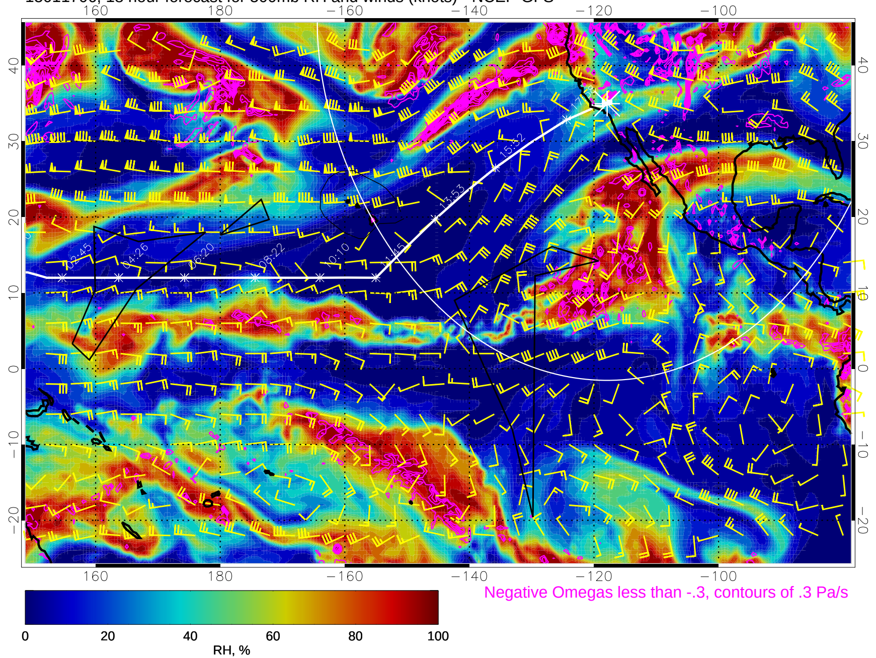
15011706, 18 hour forecast for 500mb RH and winds (knots) - NCEP GFS
