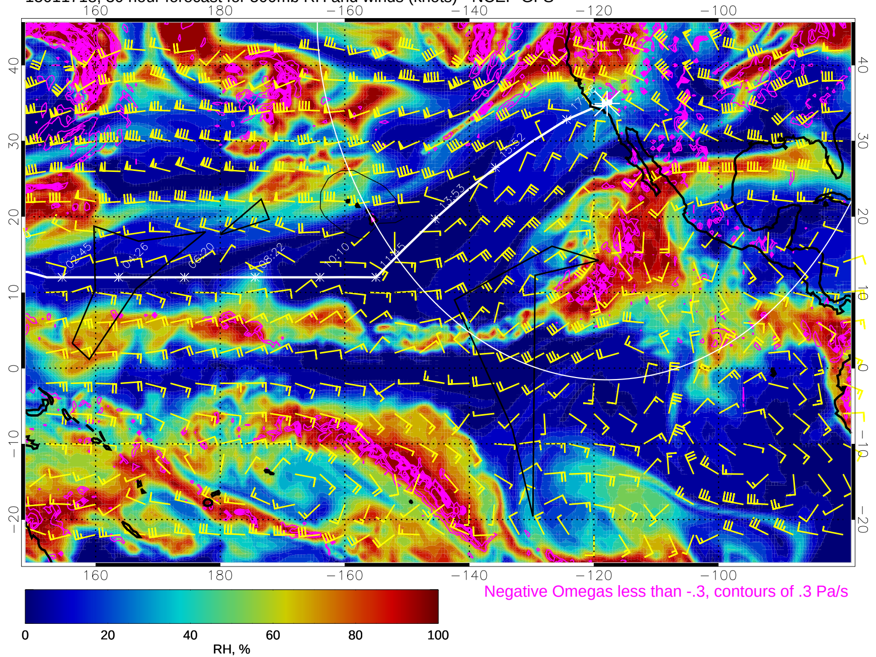
15011718, 30 hour forecast for 500mb RH and winds (knots) - NCEP GFS
