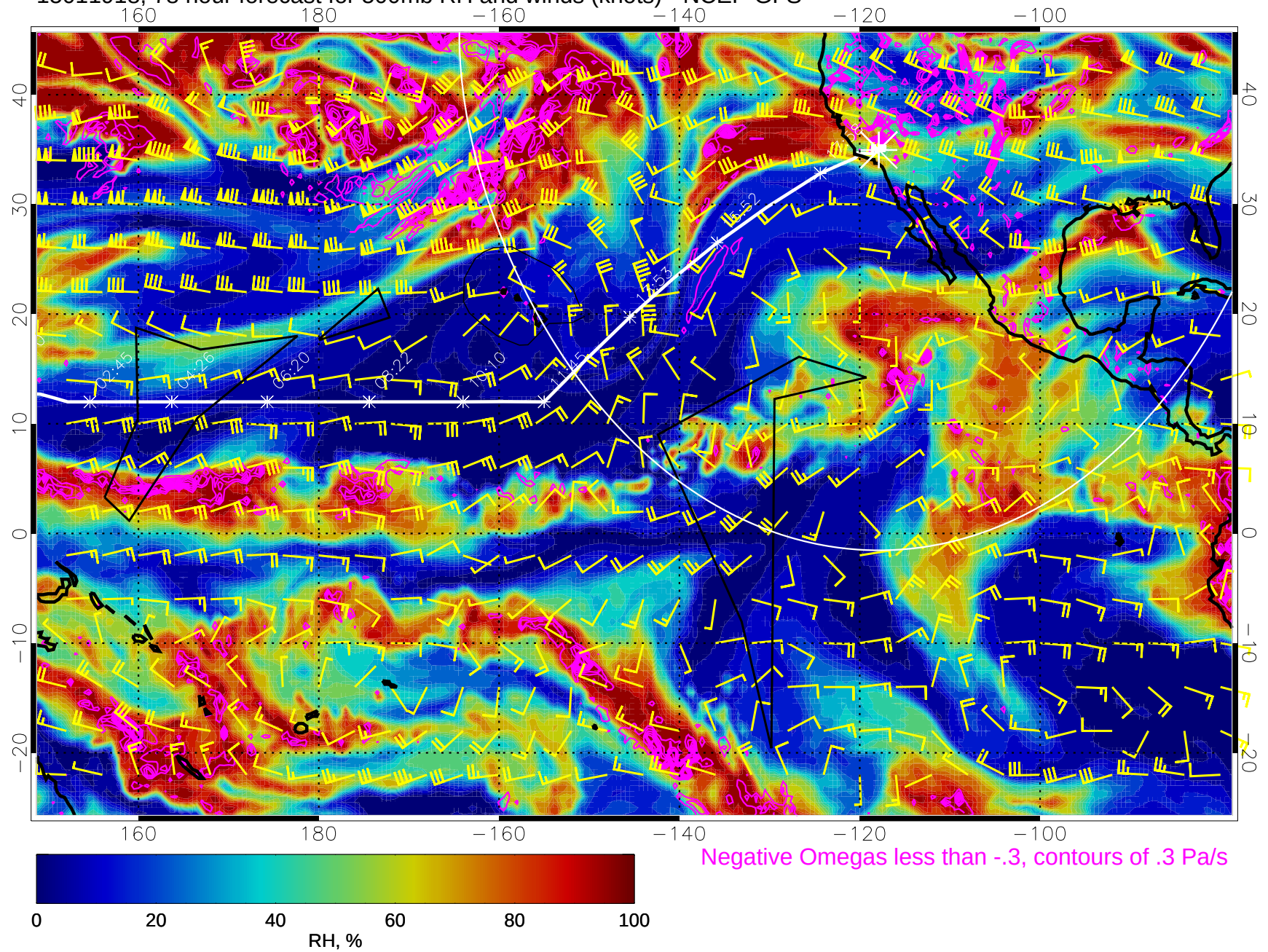
15011918, 78 hour forecast for 500mb RH and winds (knots) - NCEP GFS
