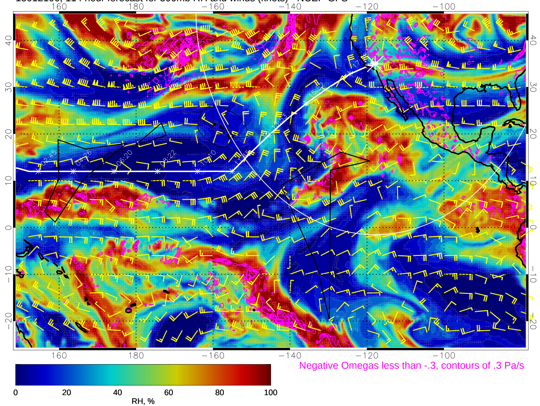
15012106, 114 hour forecast for 500mb RH and winds (knots) - NCEP GFS
