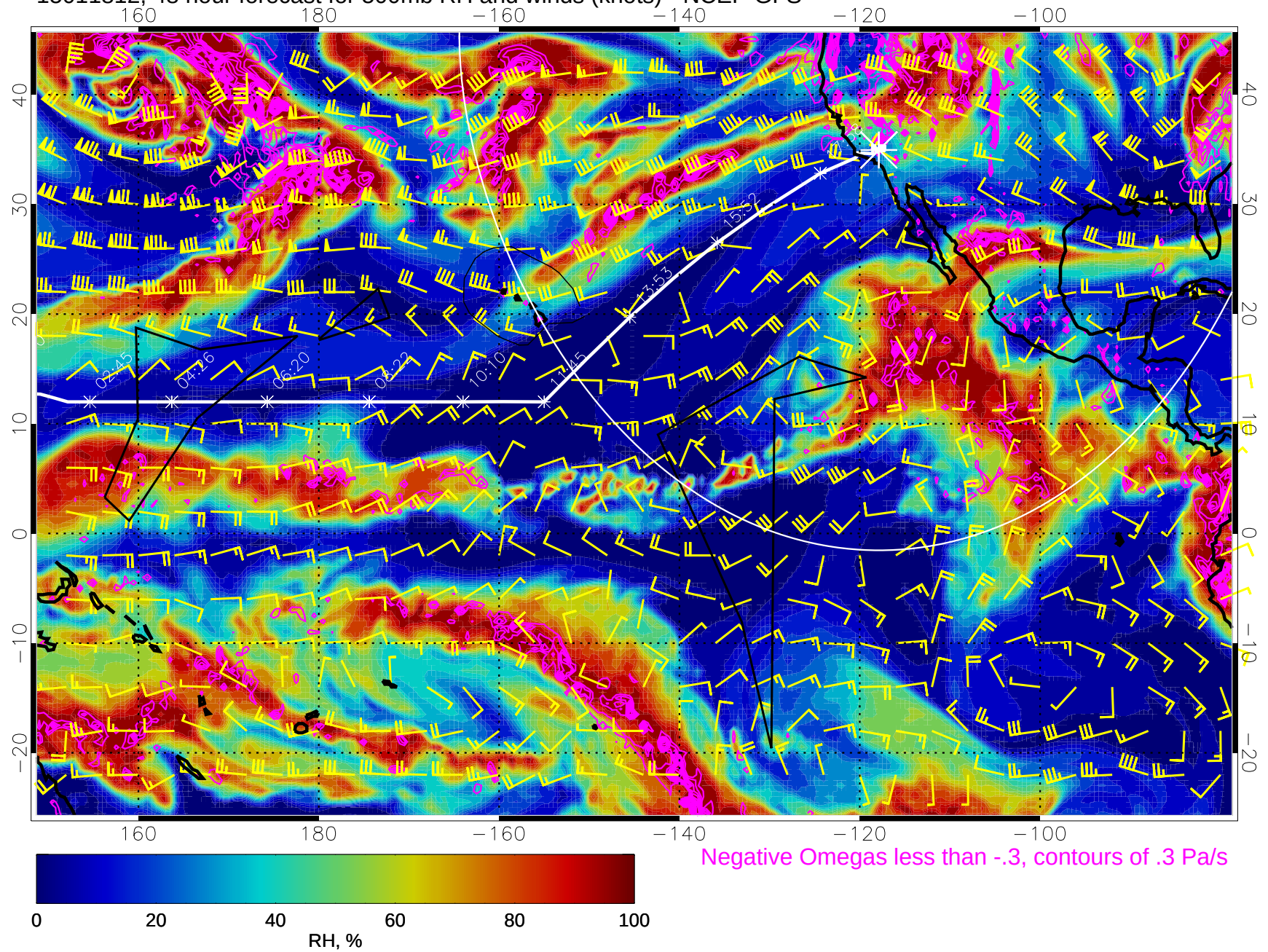
15011812, 48 hour forecast for 500mb RH and winds (knots) - NCEP GFS
