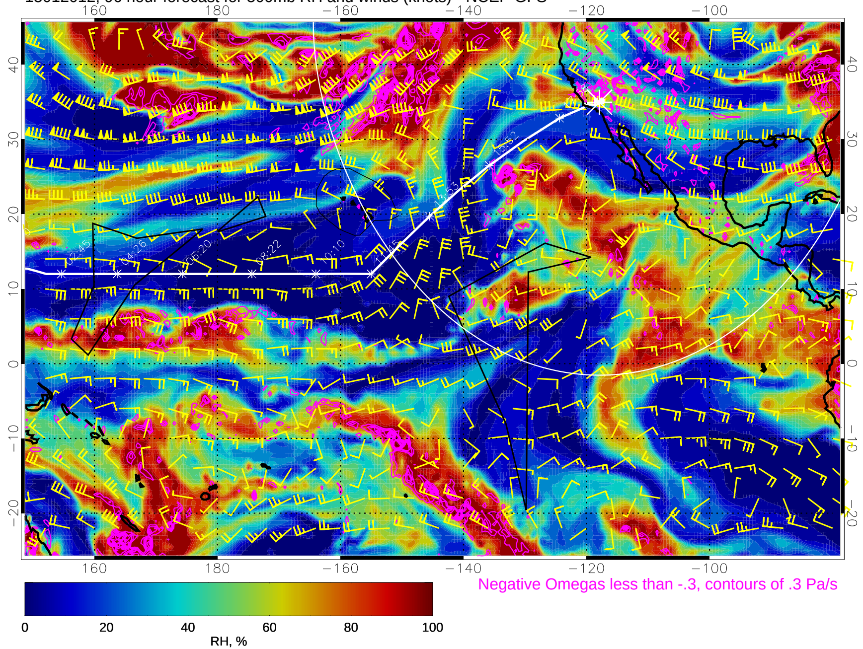
15012012, 96 hour forecast for 500mb RH and winds (knots) - NCEP GFS
