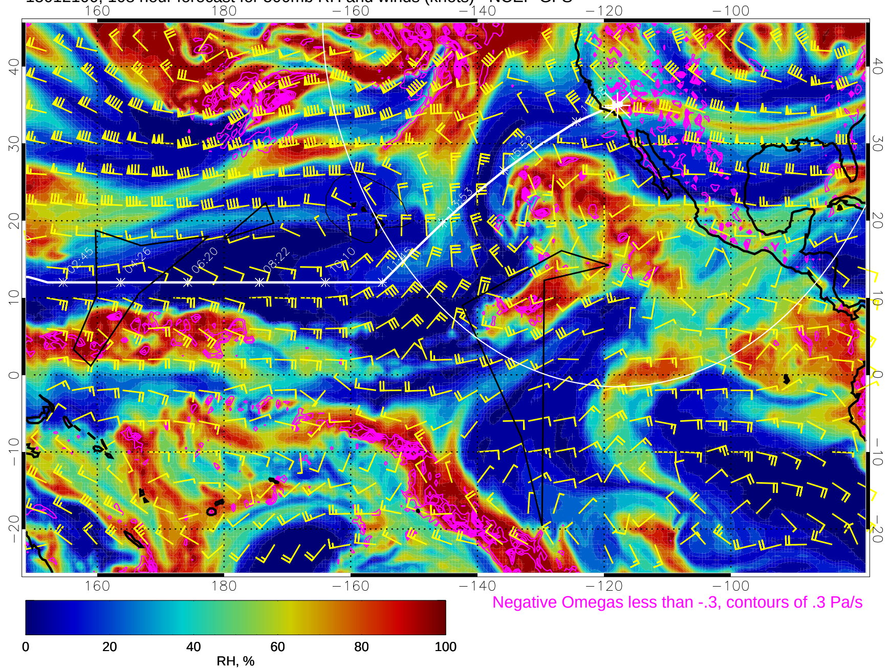
15012100, 108 hour forecast for 500mb RH and winds (knots) - NCEP GFS
