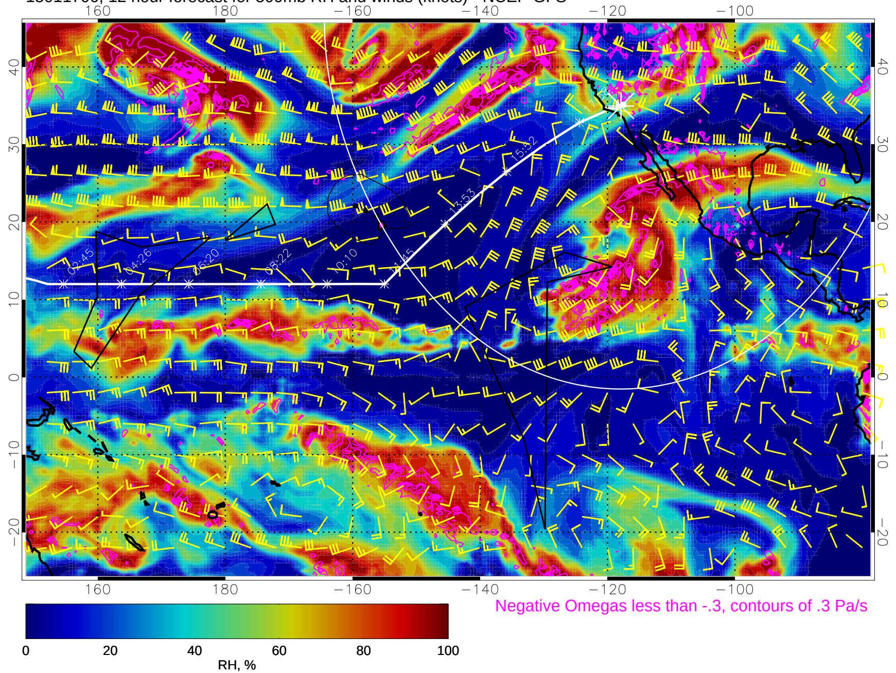
15011700, 12 hour forecast for 500mb RH and winds (knots) - NCEP GFS
