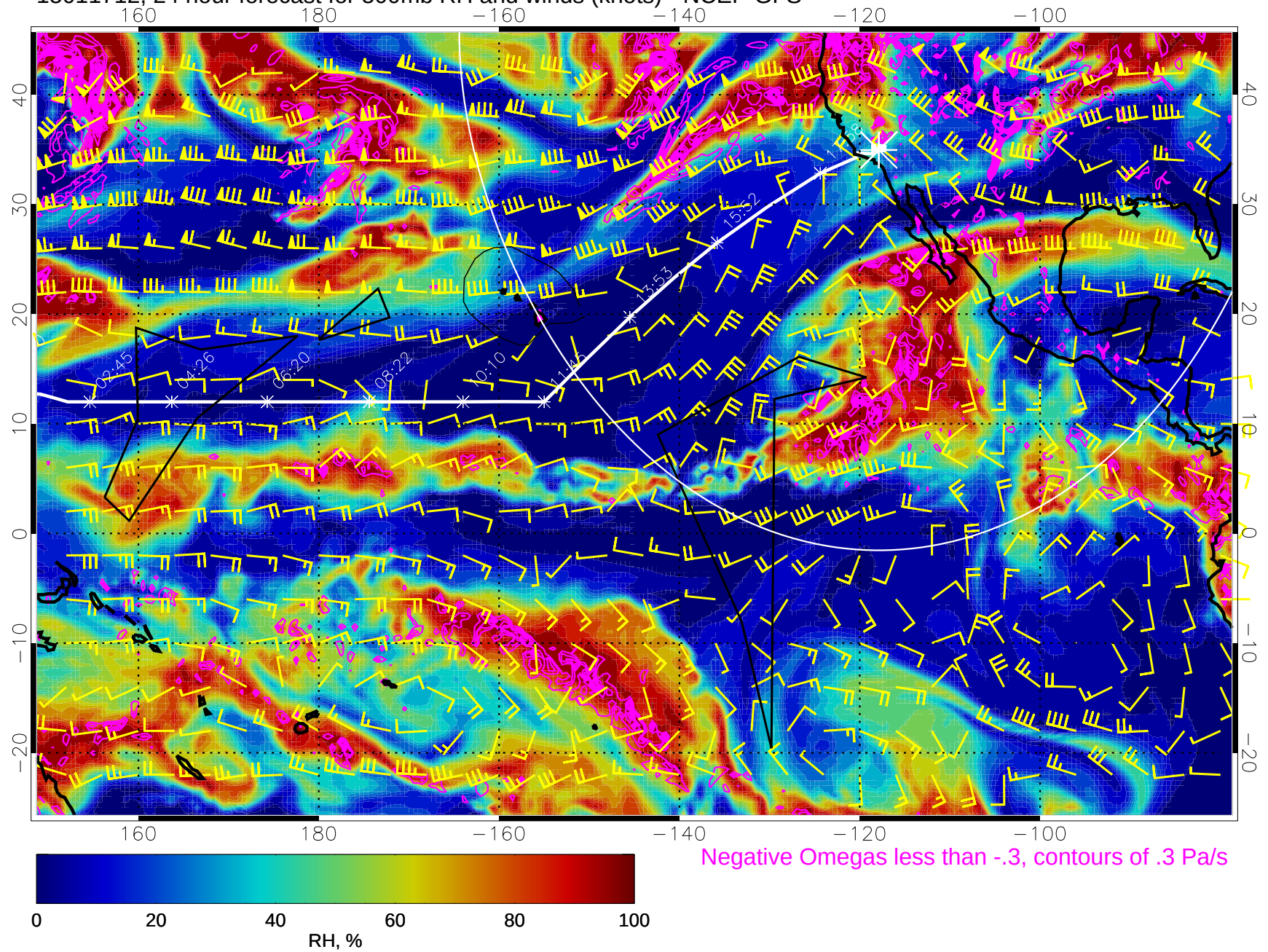
15011712, 24 hour forecast for 500mb RH and winds (knots) - NCEP GFS
