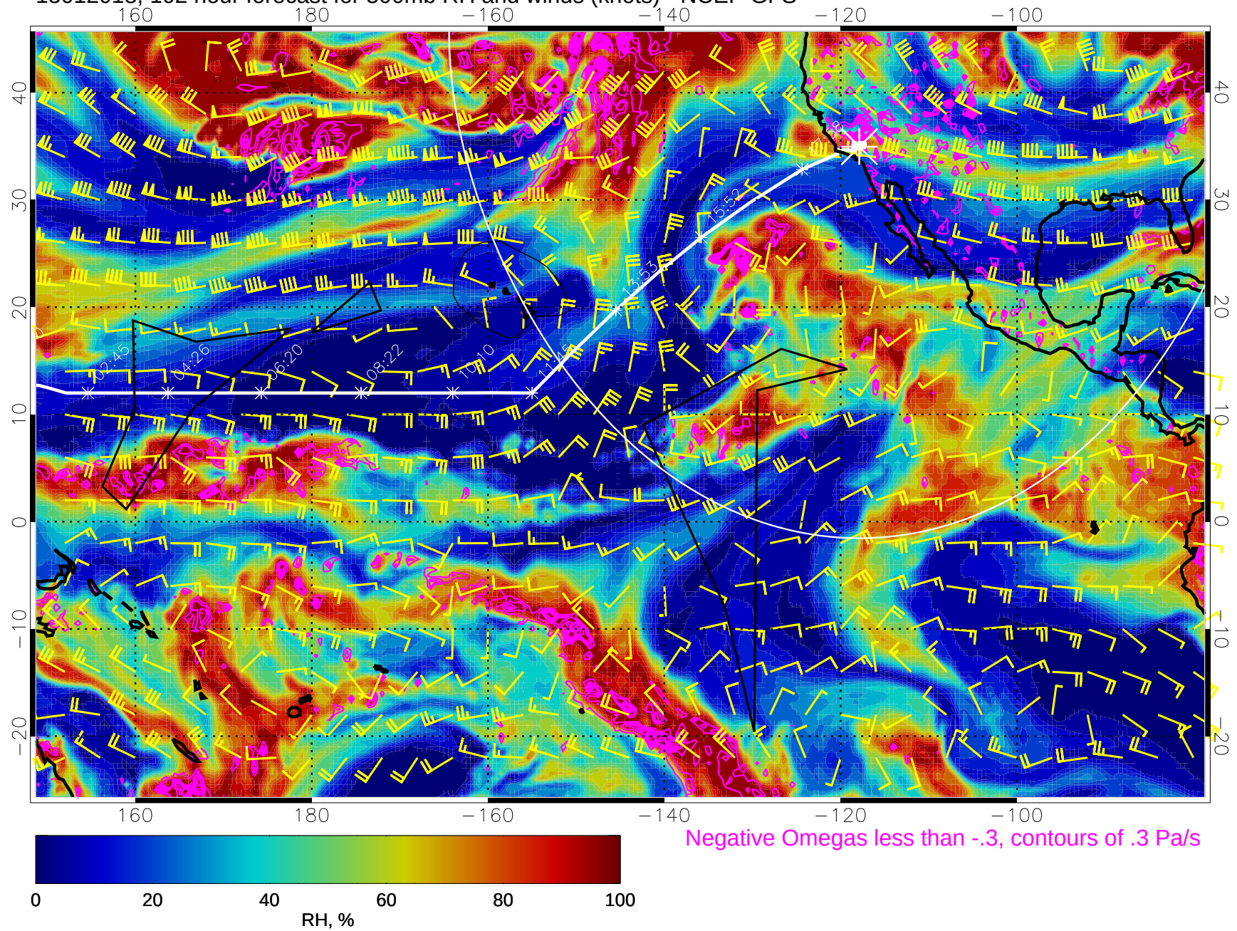
15012018, 102 hour forecast for 500mb RH and winds (knots) - NCEP GFS
