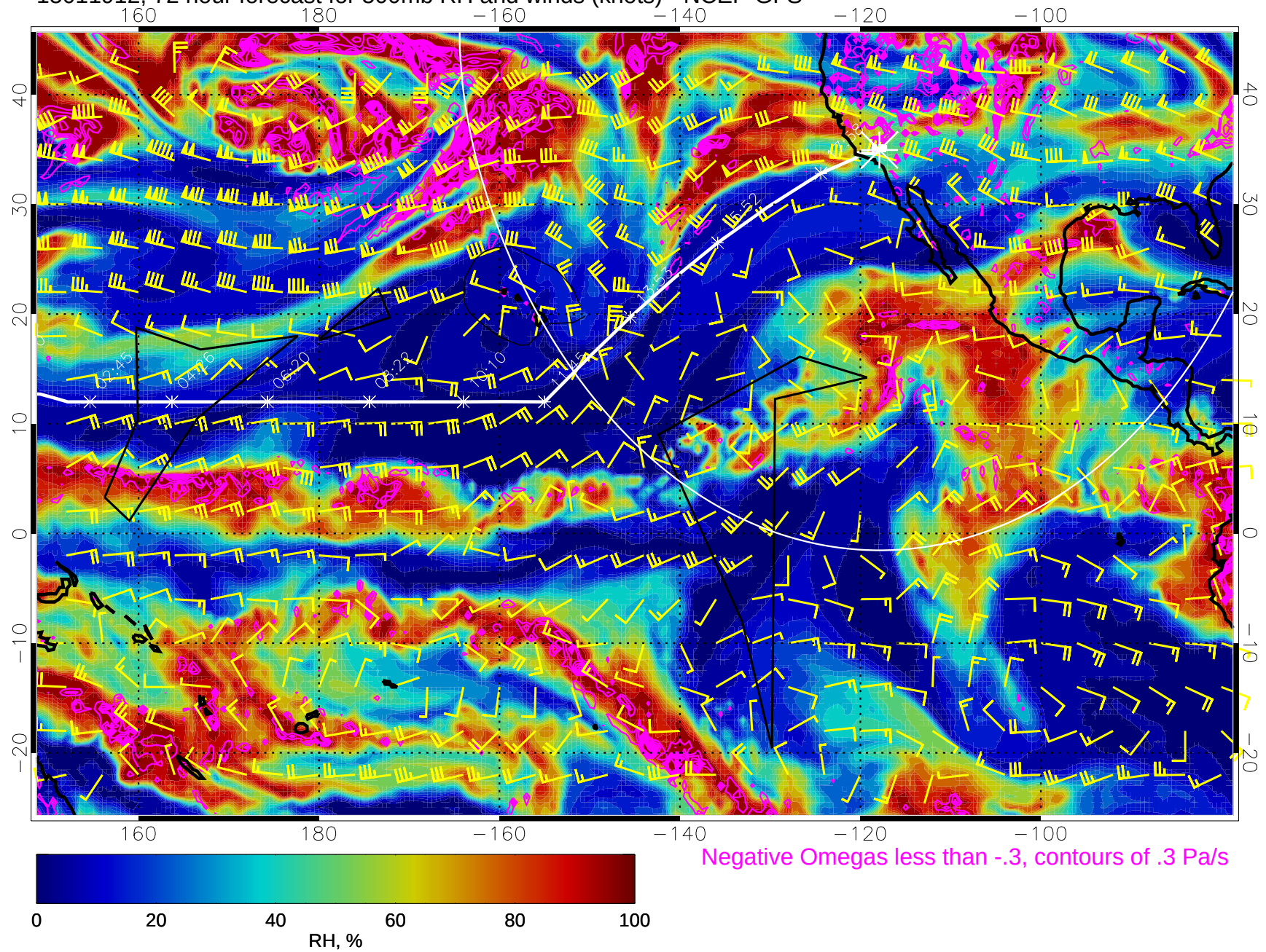
15011912, 72 hour forecast for 500mb RH and winds (knots) - NCEP GFS
