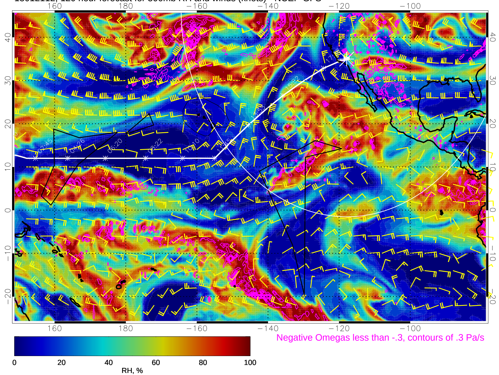
15012112, 120 hour forecast for 500mb RH and winds (knots) - NCEP GFS
