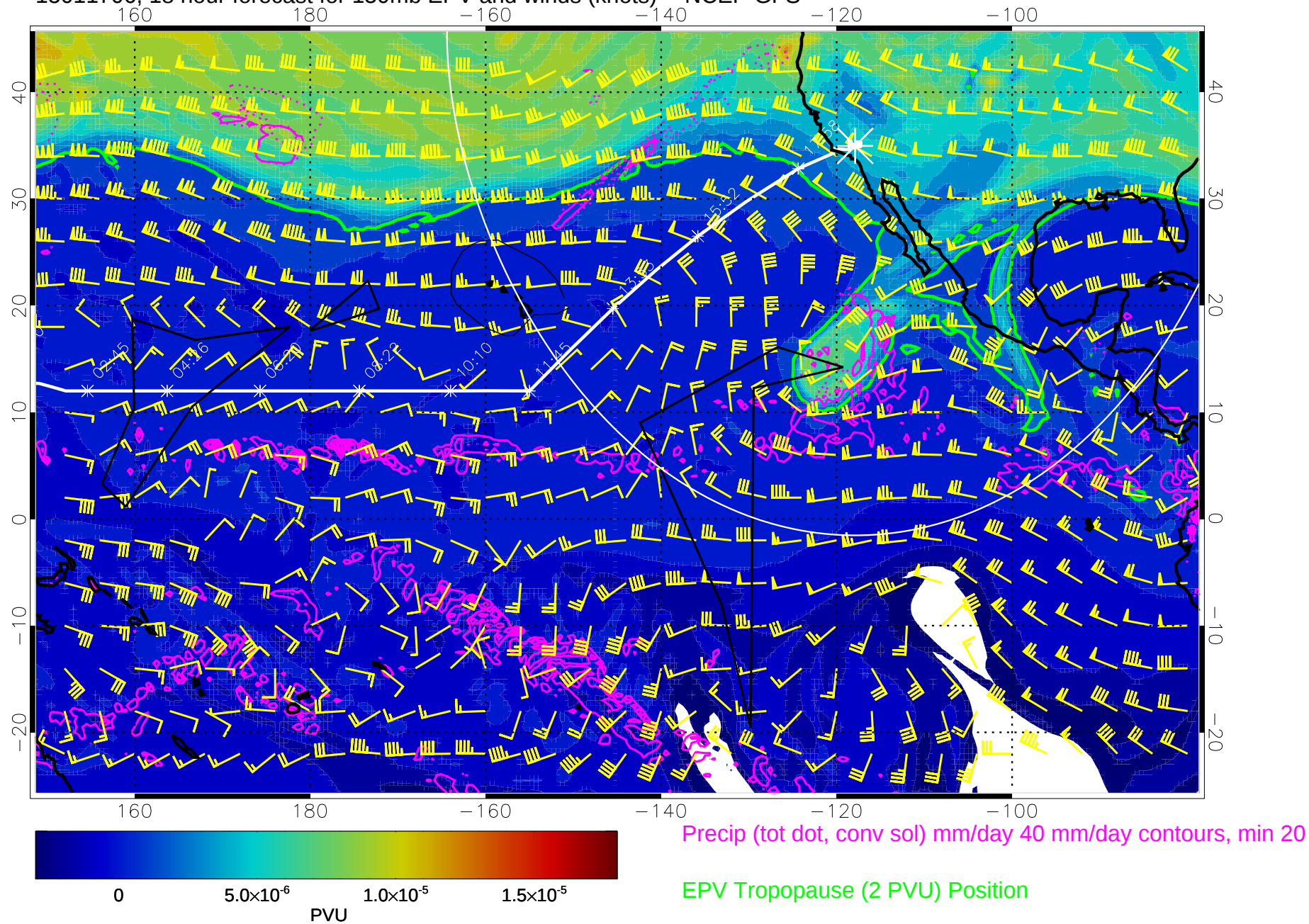
15011706, 18 hour forecast for 150mb EPV and winds (knots) -- NCEP GFS
