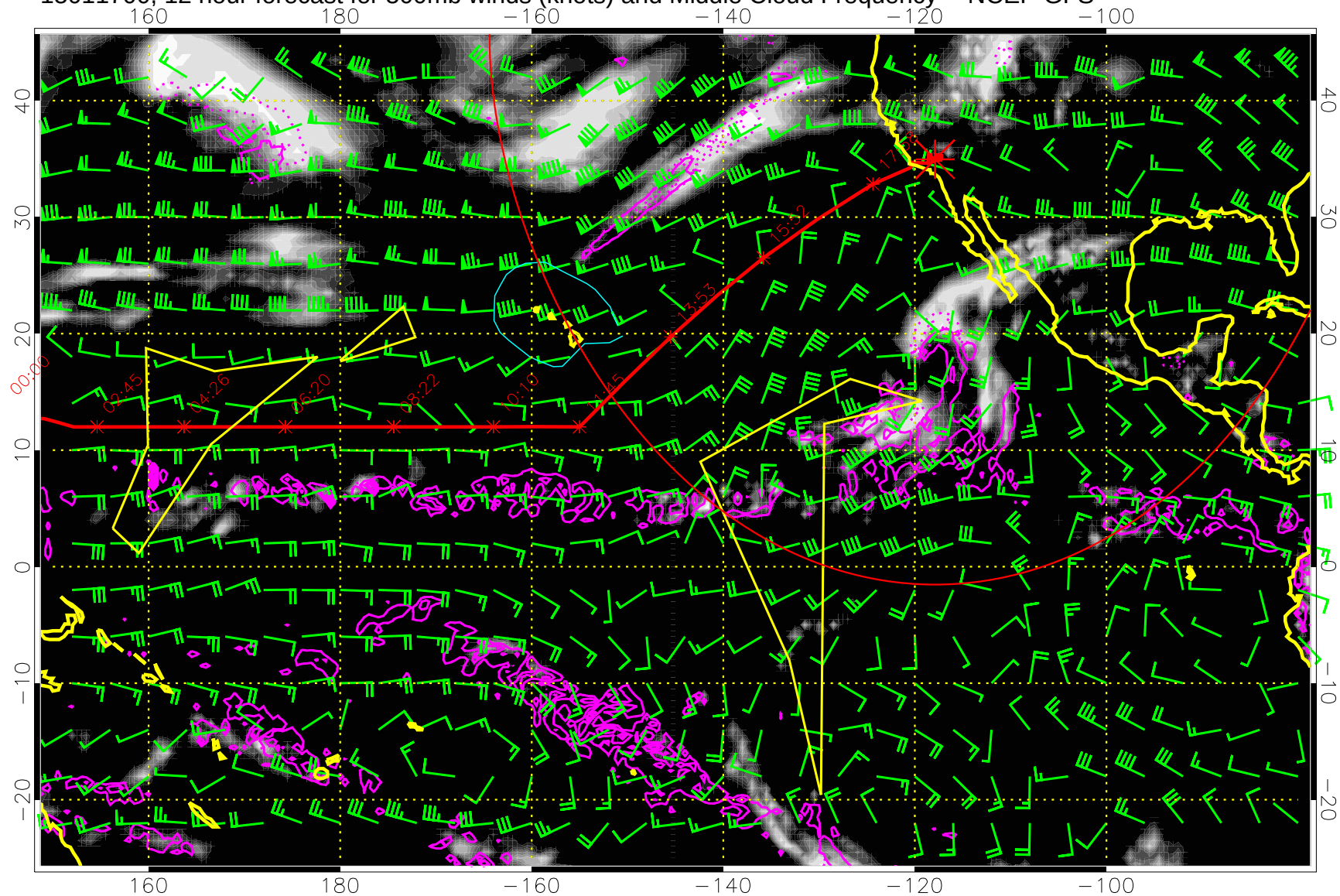
15011700, 12 hour forecast for 500mb winds (knots) and Middle Cloud Frequency -- NCEP GFS
