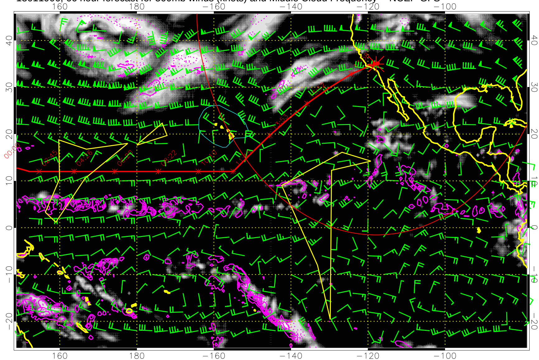
15011906, 66 hour forecast for 500mb winds (knots) and Middle Cloud Frequency -- NCEP GFS
