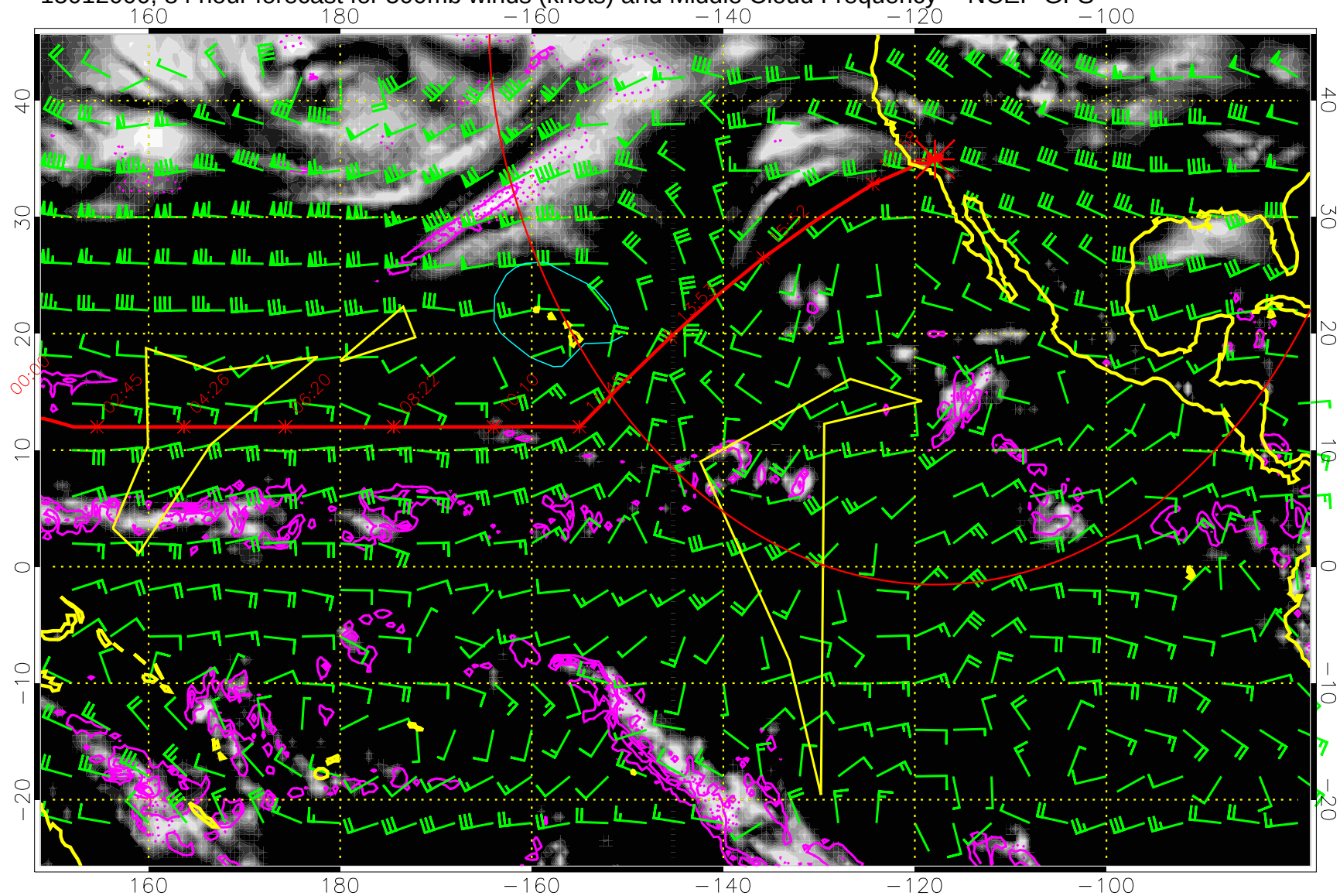
15012000, 84 hour forecast for 500mb winds (knots) and Middle Cloud Frequency -- NCEP GFS
