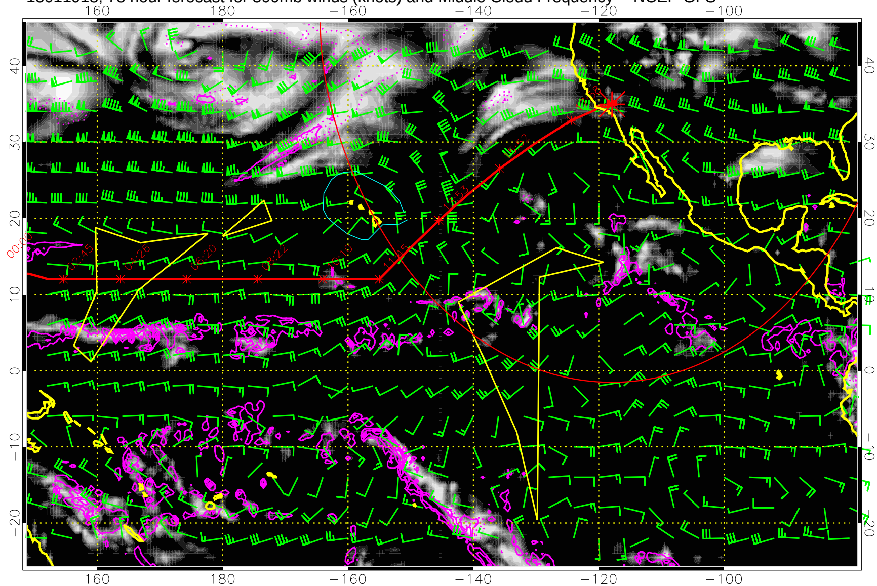
15011918, 78 hour forecast for 500mb winds (knots) and Middle Cloud Frequency -- NCEP GFS
