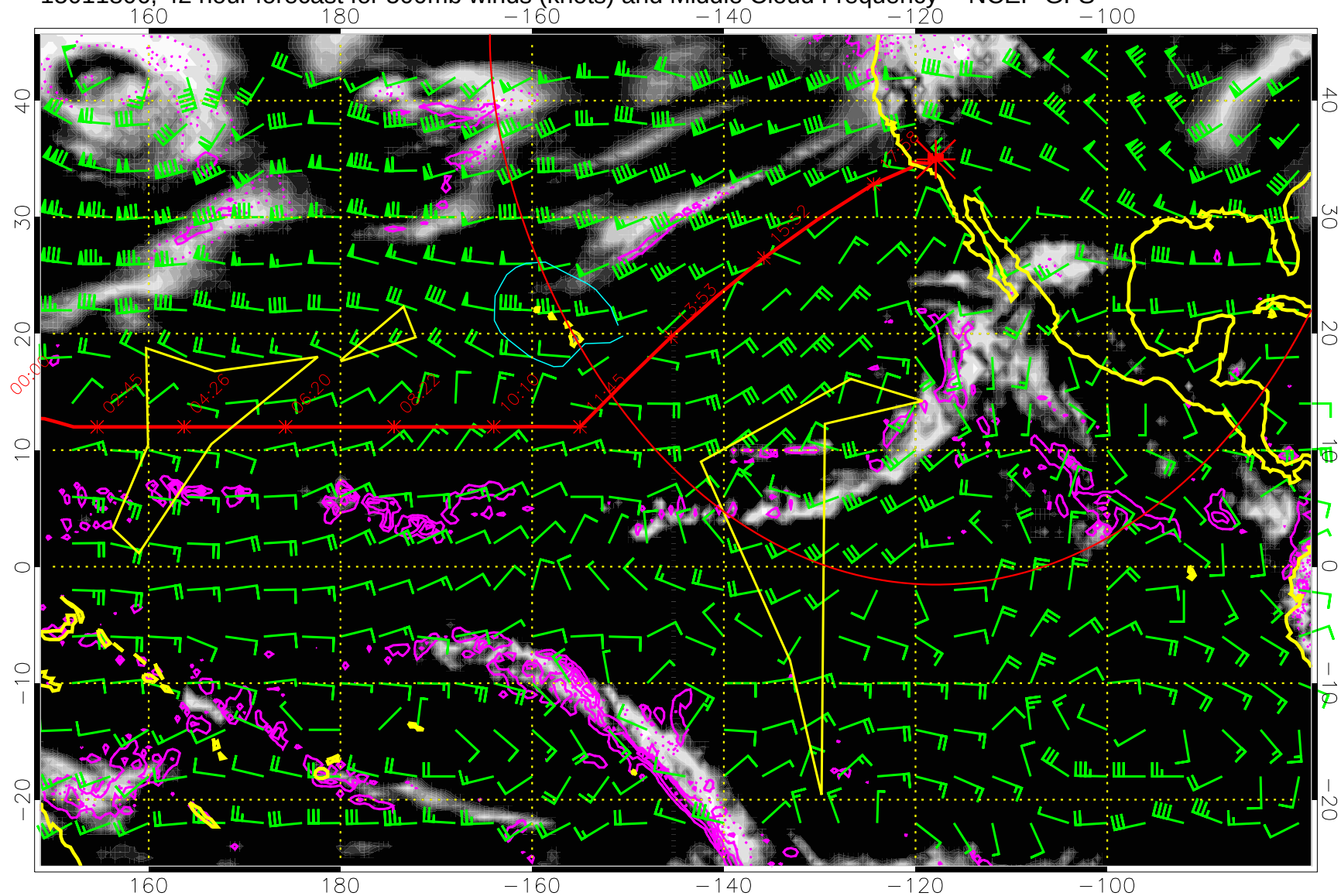
15011806, 42 hour forecast for 500mb winds (knots) and Middle Cloud Frequency -- NCEP GFS
