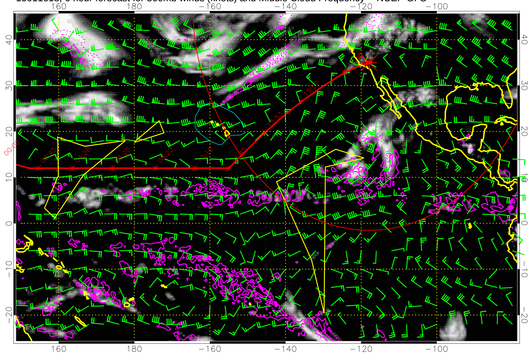
15011618, 6 hour forecast for 500mb winds (knots) and Middle Cloud Frequency -- NCEP GFS
