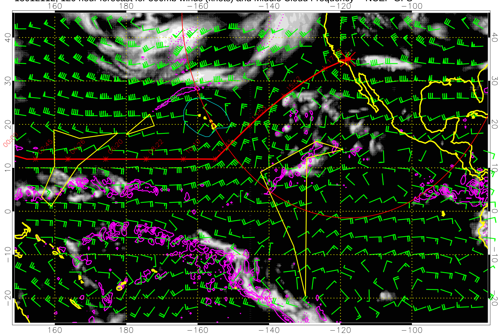
15012112, 120 hour forecast for 500mb winds (knots) and Middle Cloud Frequency -- NCEP GFS
