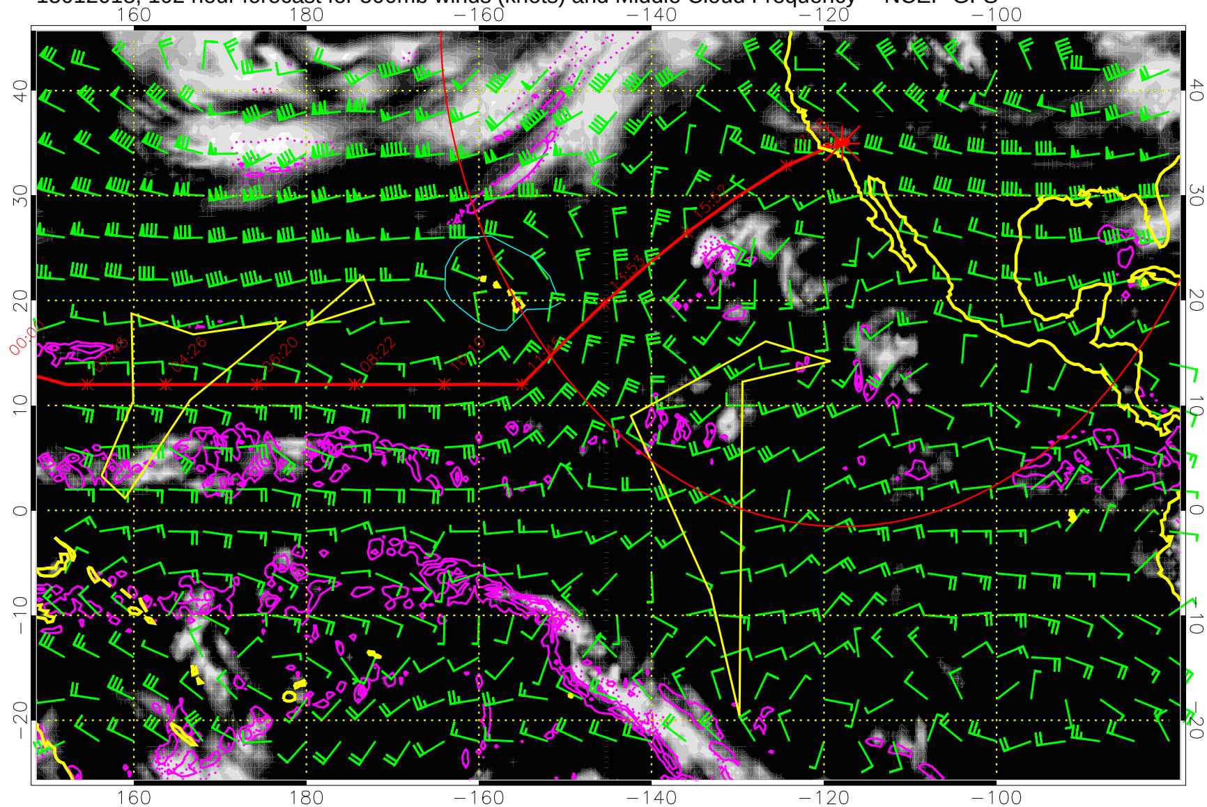
15012018, 102 hour forecast for 500mb winds (knots) and Middle Cloud Frequency -- NCEP GFS
