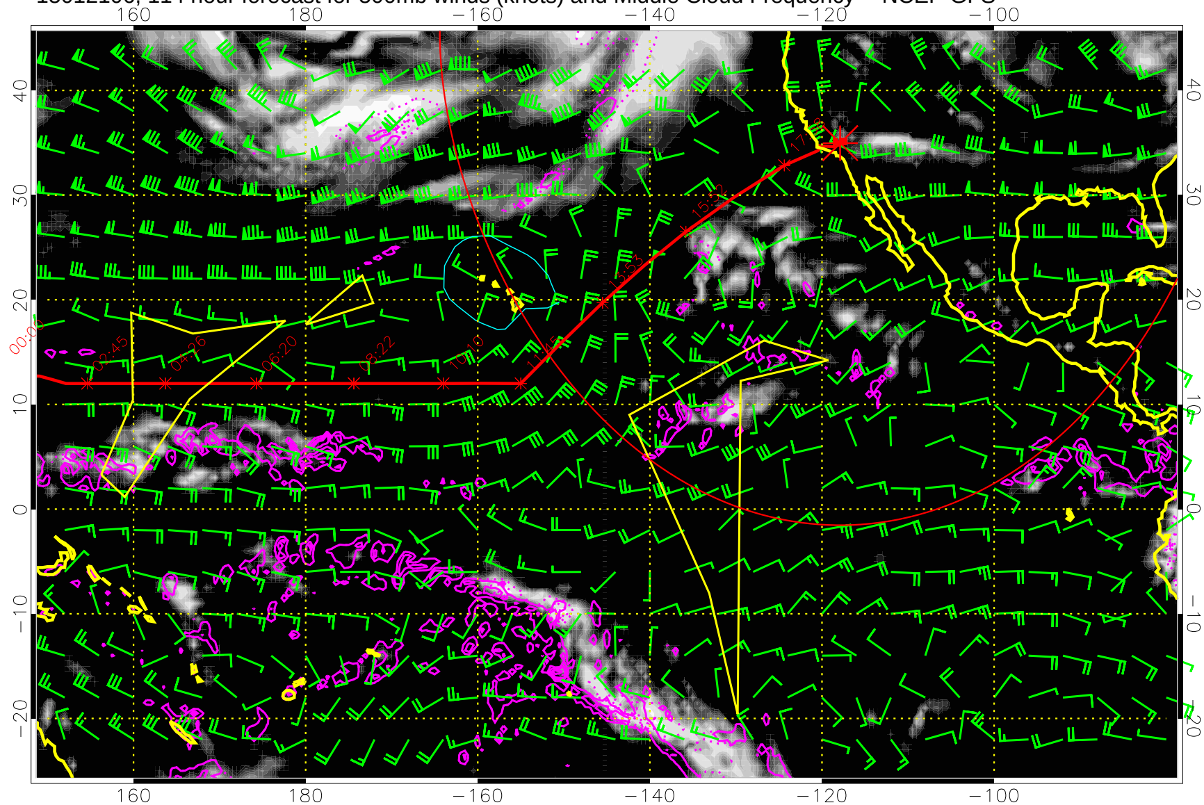
15012106, 114 hour forecast for 500mb winds (knots) and Middle Cloud Frequency -- NCEP GFS
