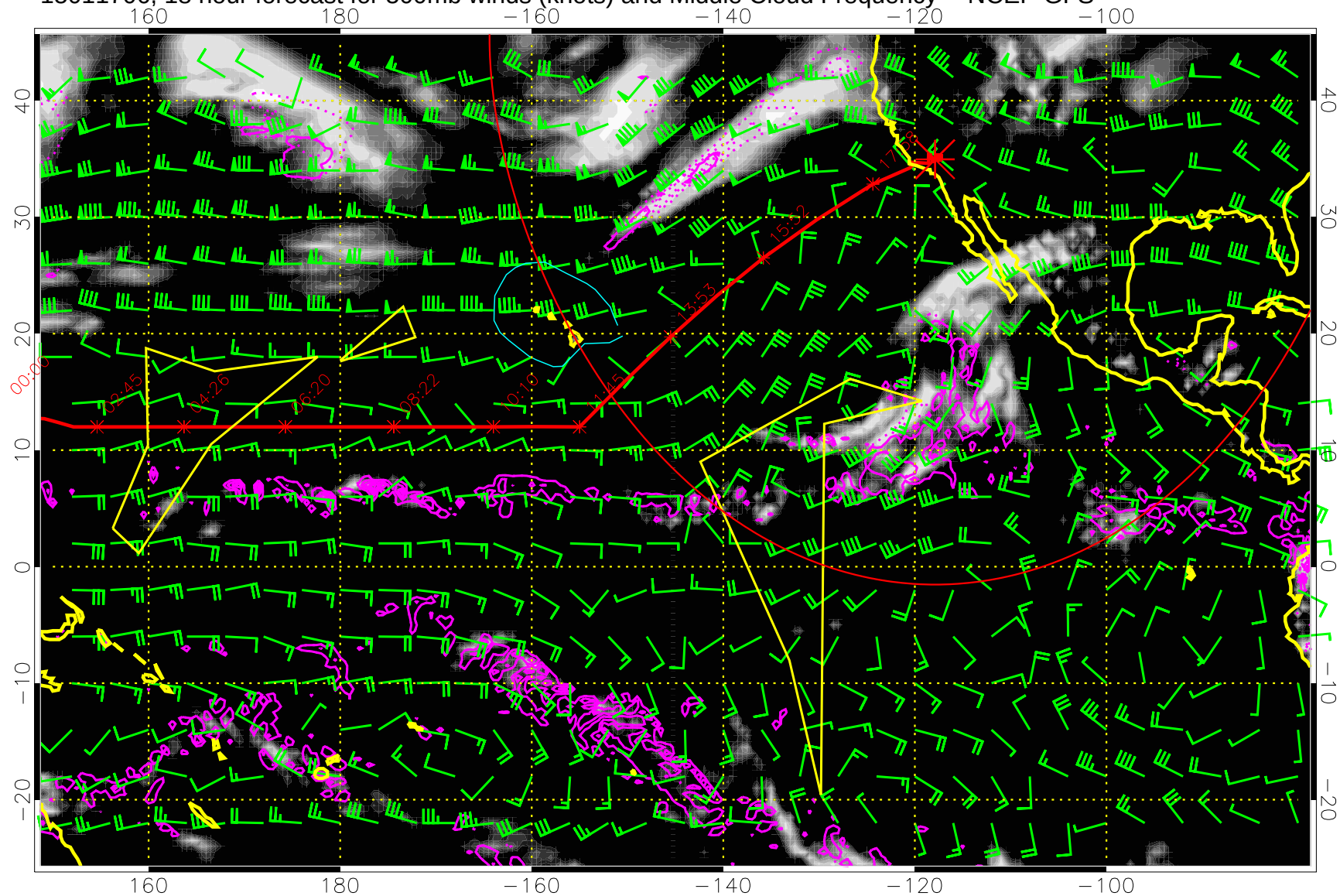
15011706, 18 hour forecast for 500mb winds (knots) and Middle Cloud Frequency -- NCEP GFS
