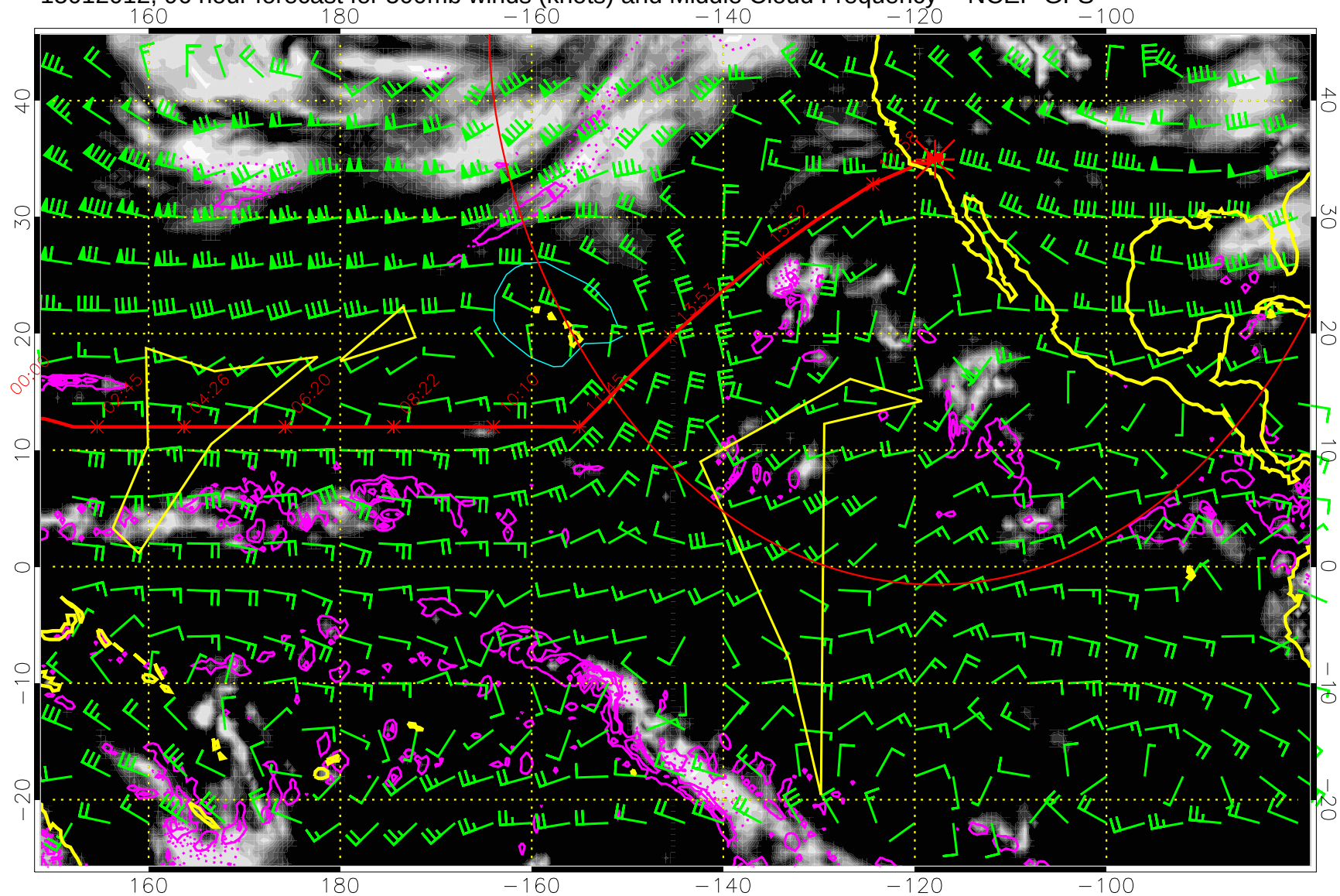
15012012, 96 hour forecast for 500mb winds (knots) and Middle Cloud Frequency -- NCEP GFS
