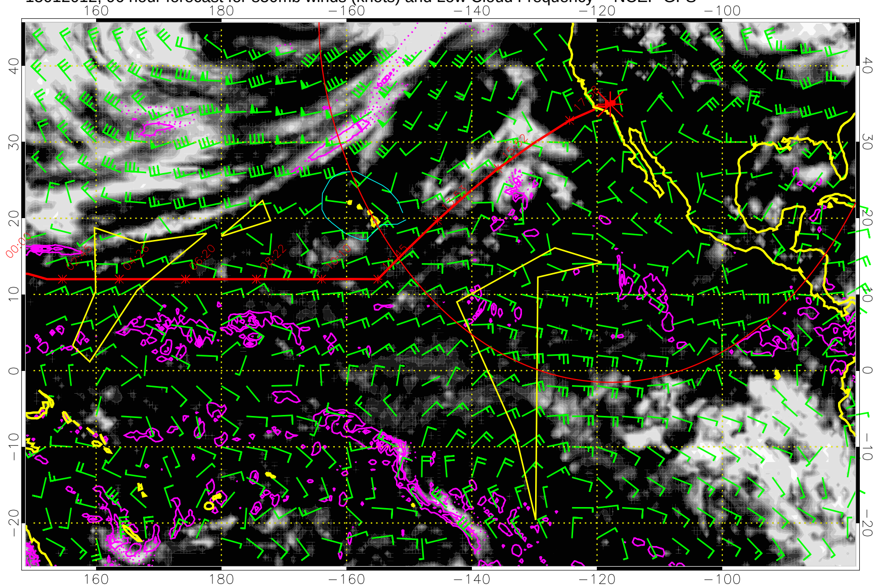
15012012, 96 hour forecast for 850mb winds (knots) and Low Cloud Frequency -- NCEP GFS
