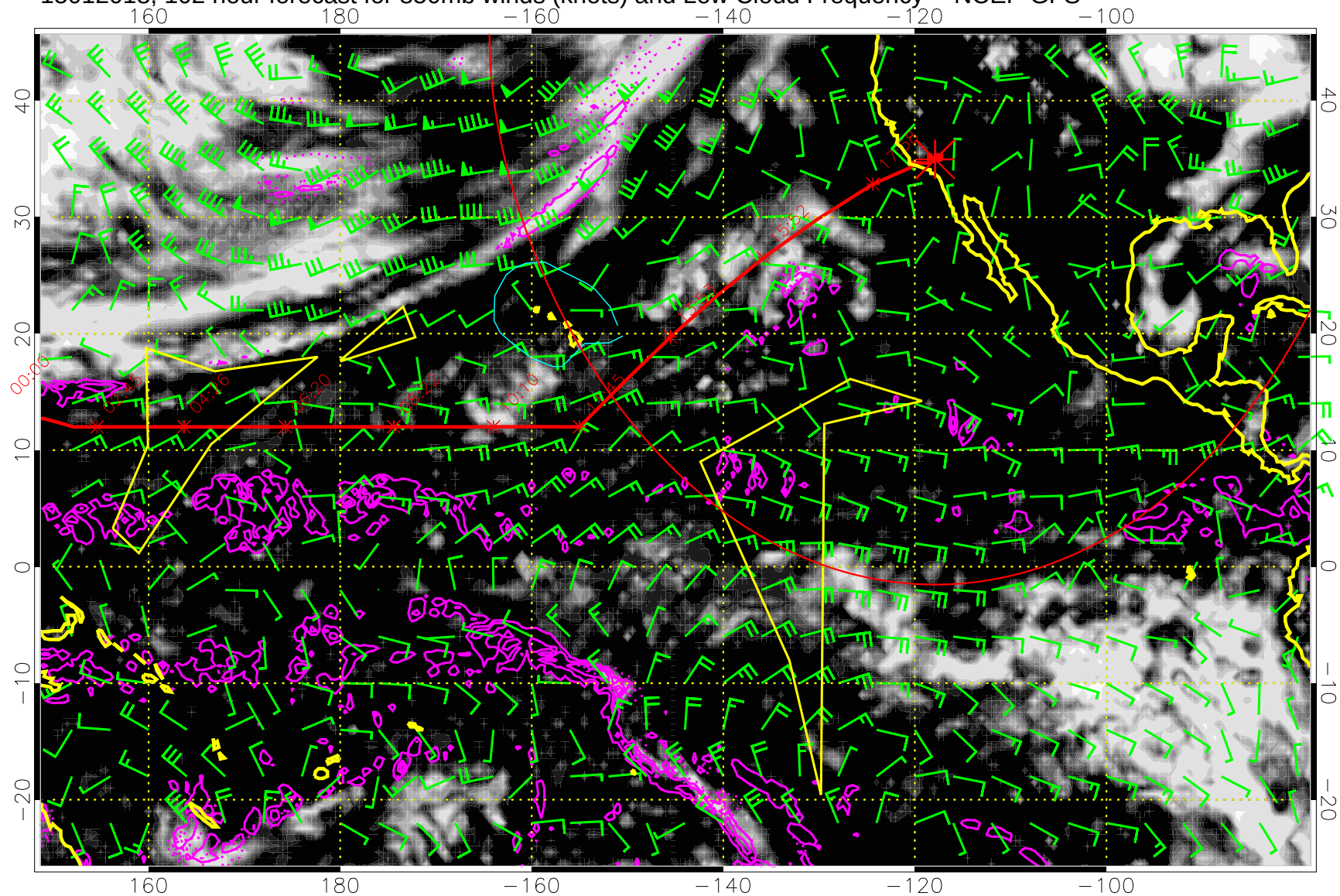
15012018, 102 hour forecast for 850mb winds (knots) and Low Cloud Frequency -- NCEP GFS
