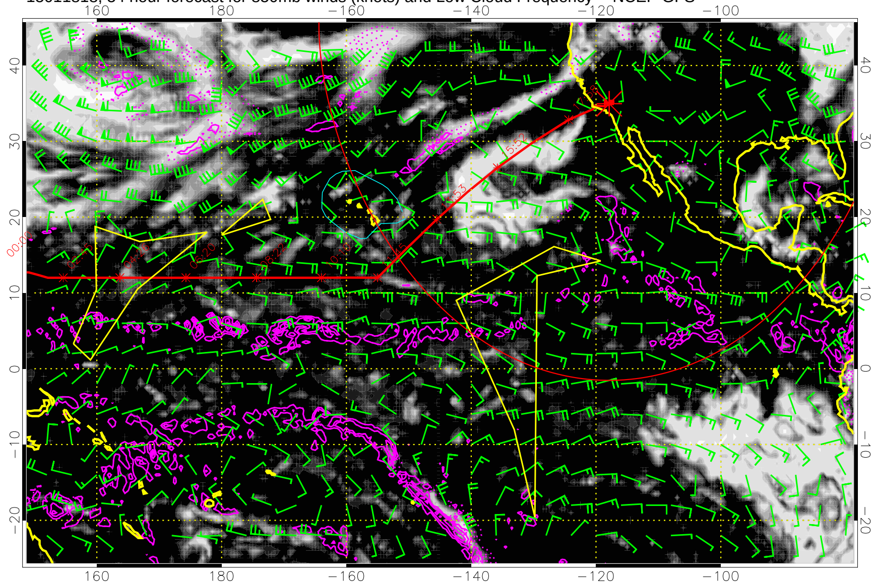
15011818, 54 hour forecast for 850mb winds (knots) and Low Cloud Frequency -- NCEP GFS
