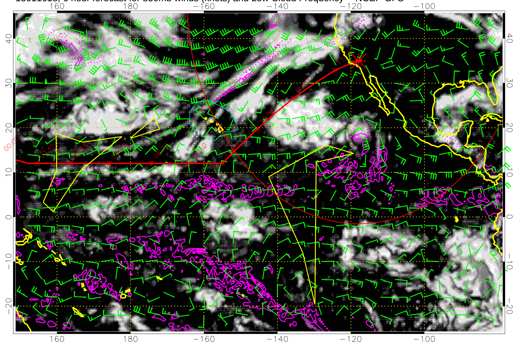
15011618, 6 hour forecast for 850mb winds (knots) and Low Cloud Frequency -- NCEP GFS
