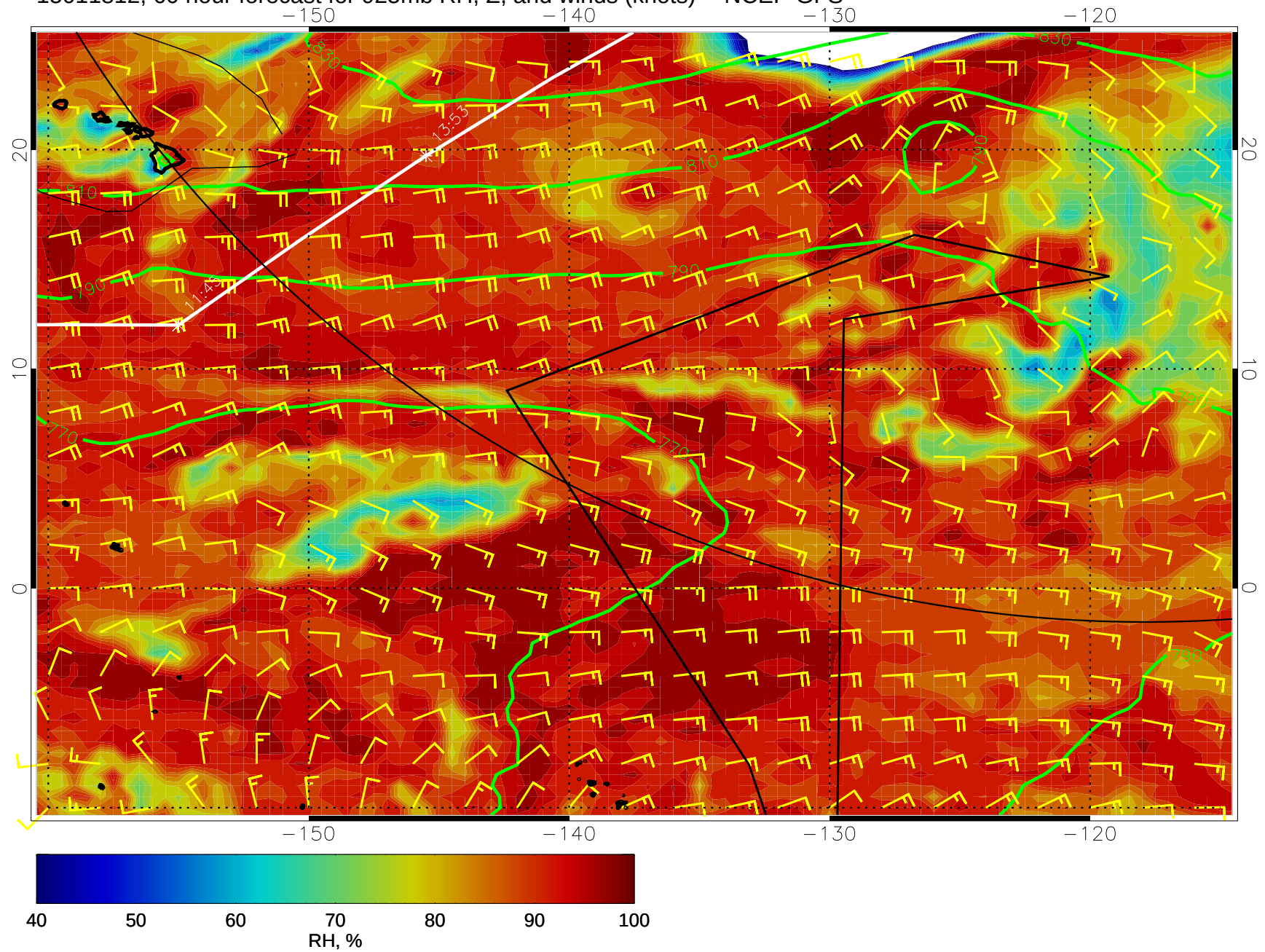
15011812, 60 hour forecast for 925mb RH, Z, and winds (knots) -- NCEP GFS
