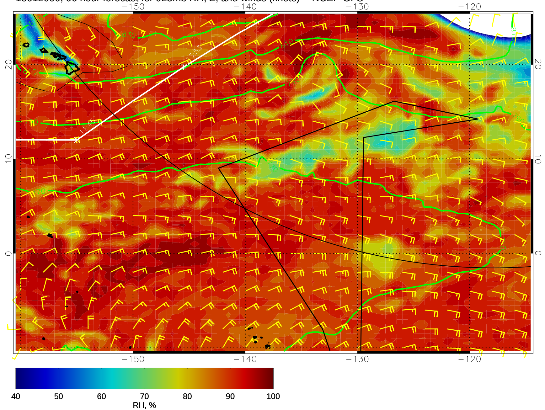
15012000, 96 hour forecast for 925mb RH, Z, and winds (knots) -- NCEP GFS
