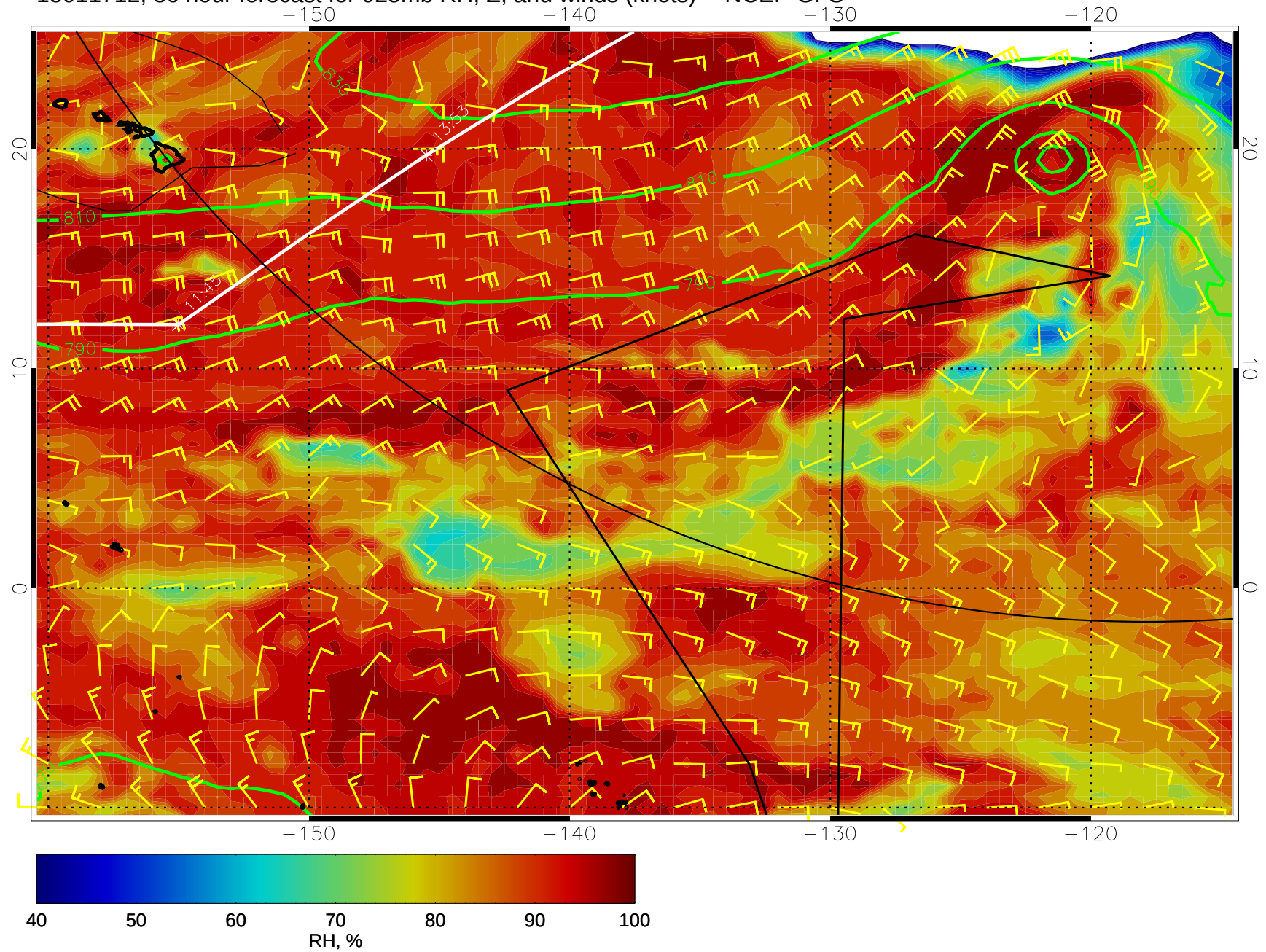
15011712, 36 hour forecast for 925mb RH, Z, and winds (knots) -- NCEP GFS
