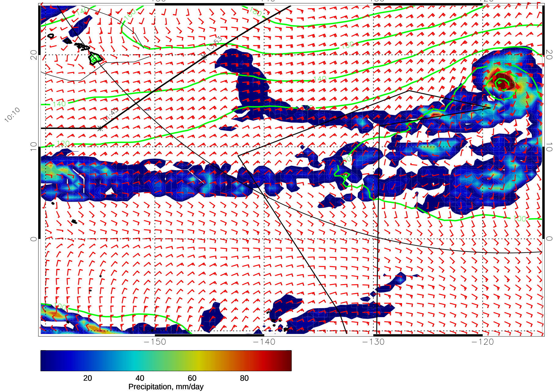
15011612, 12 hour forecast for precip, 1000mb Z, and winds (knots) -- NCEP GFS
