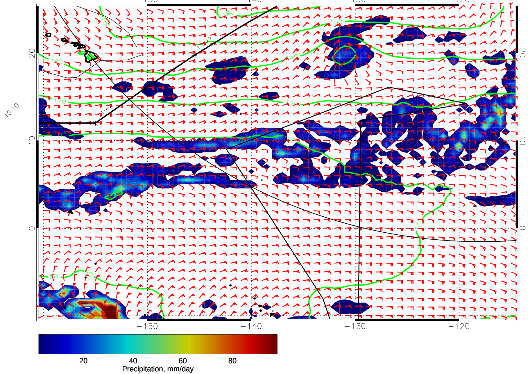
15011912, 84 hour forecast for precip, 1000mb Z, and winds (knots) -- NCEP GFS
