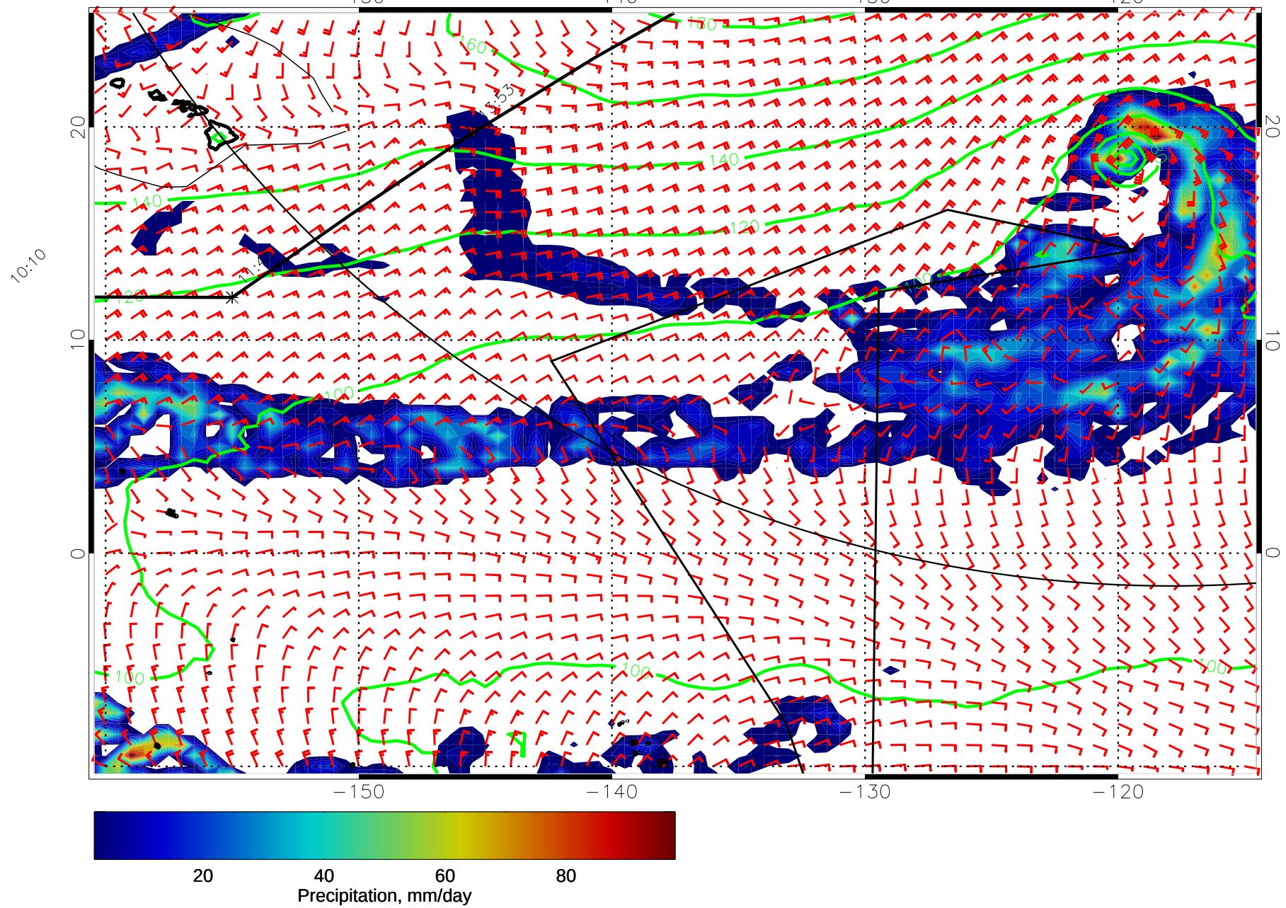
15011700, 24 hour forecast for precip, 1000mb Z, and winds (knots) -- NCEP GFS
