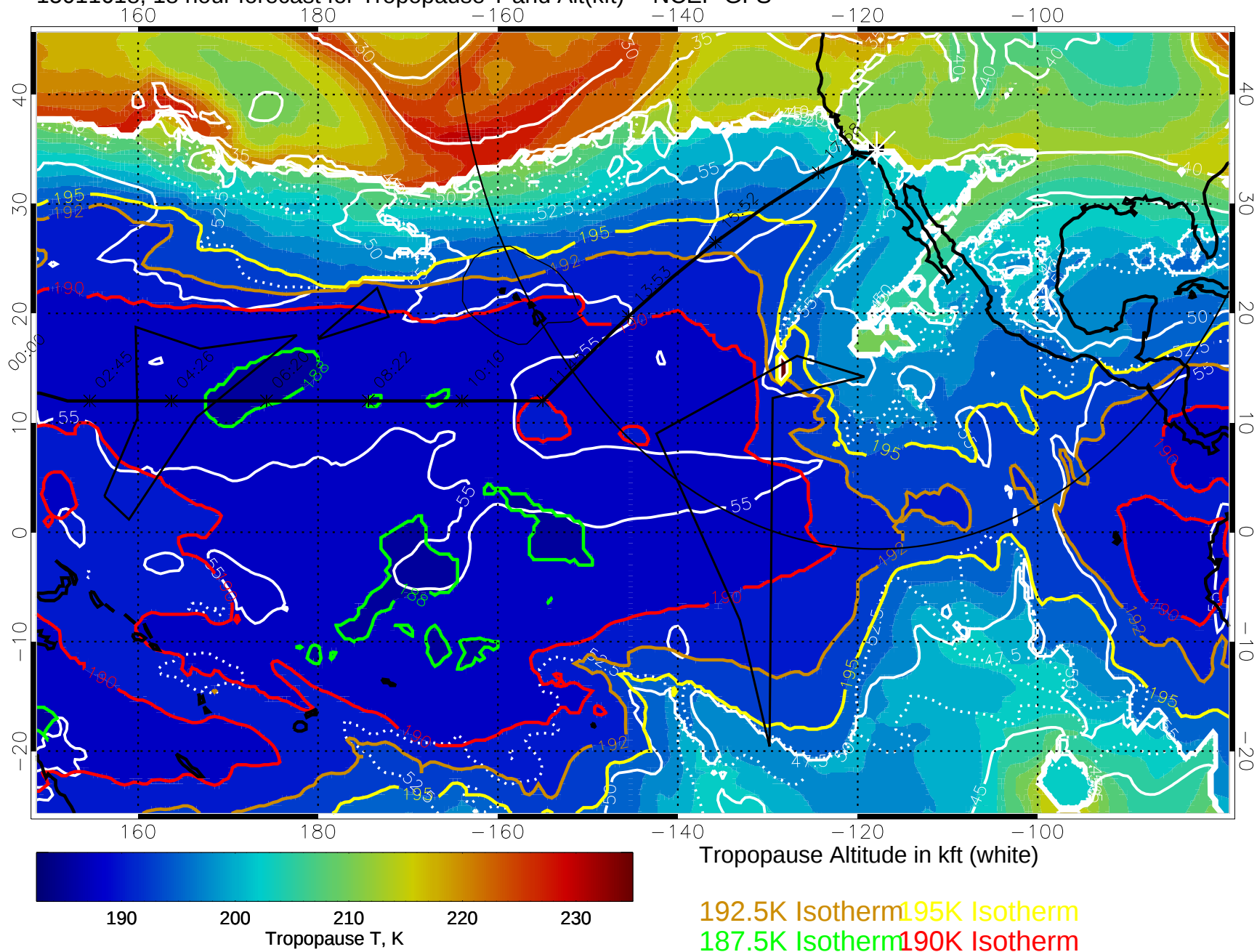
15011618, 18 hour forecast for Tropopause T and Alt(kft) -- NCEP GFS
