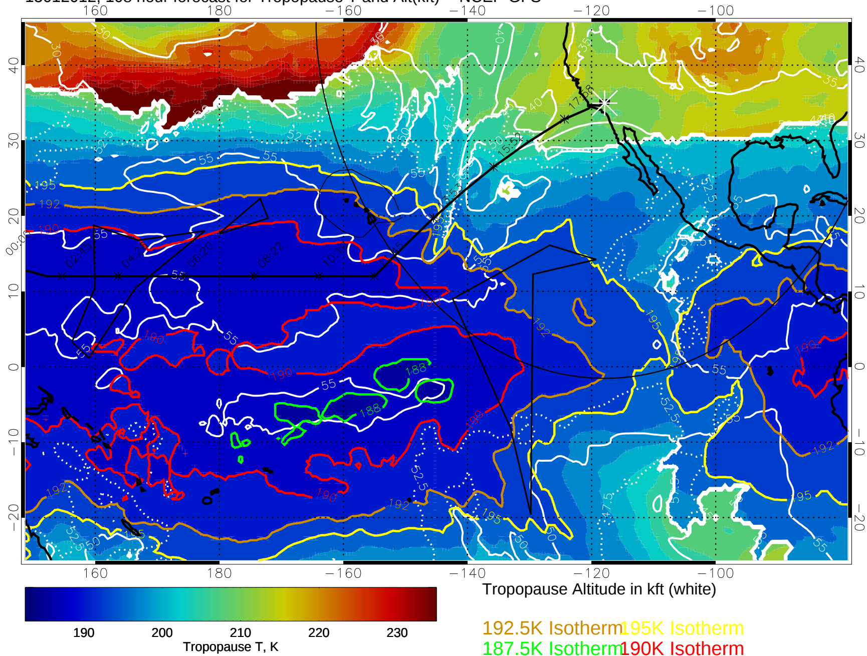
15012012, 108 hour forecast for Tropopause T and Alt(kft) -- NCEP GFS
