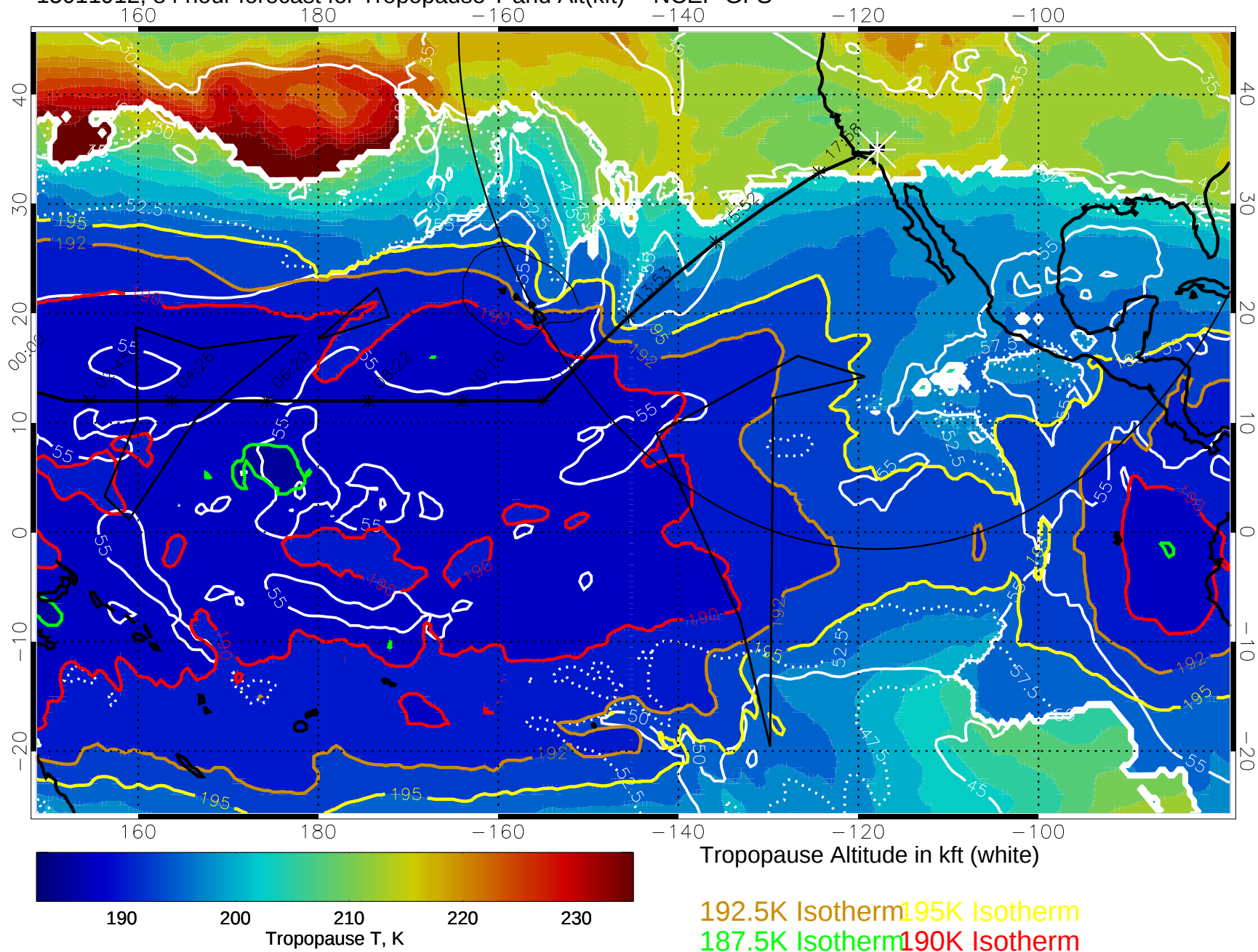
15011912, 84 hour forecast for Tropopause T and Alt(kft) -- NCEP GFS
