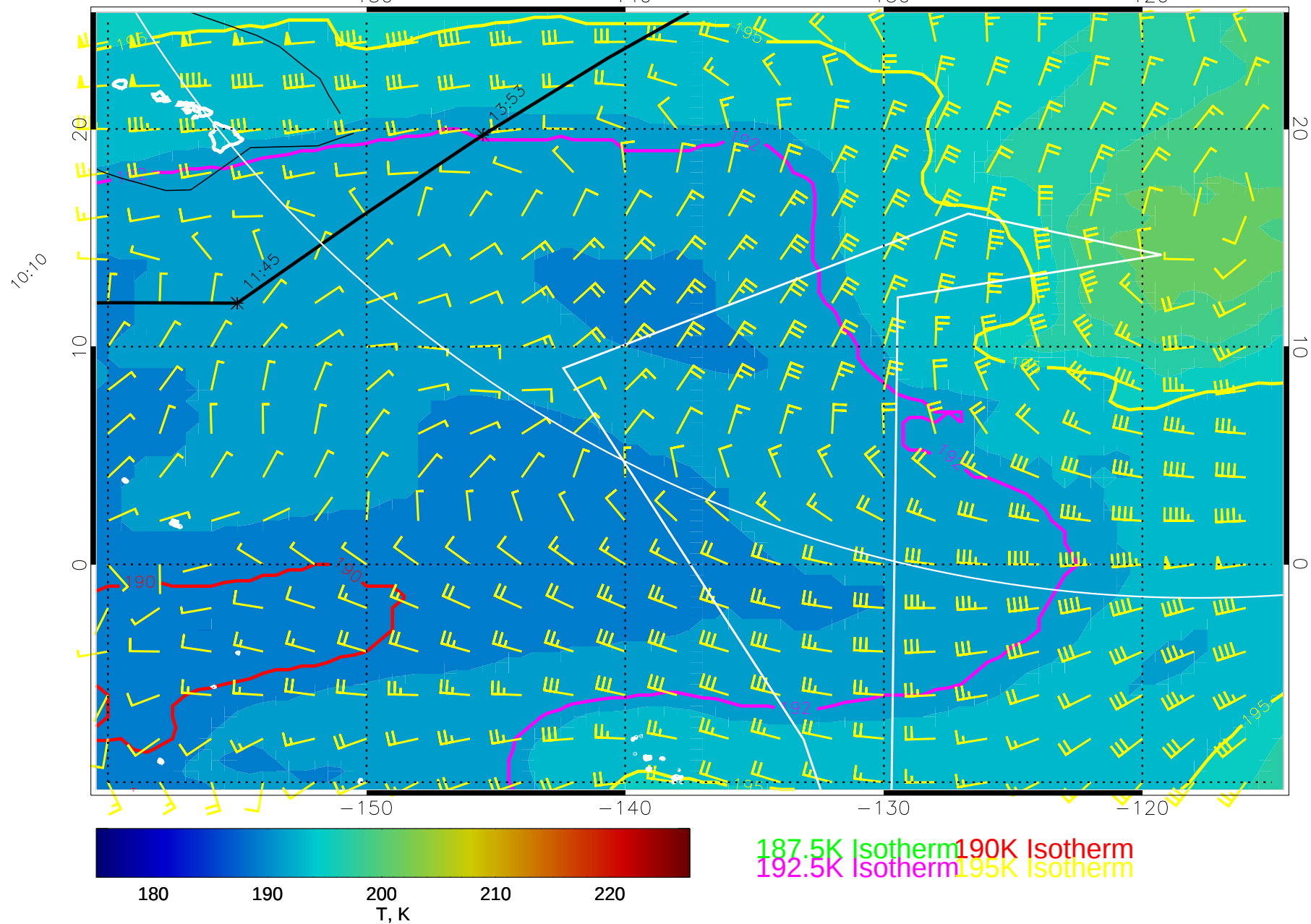
15011712, 36 hour forecast for 100mb T and winds (knots) -- NCEP GFS
