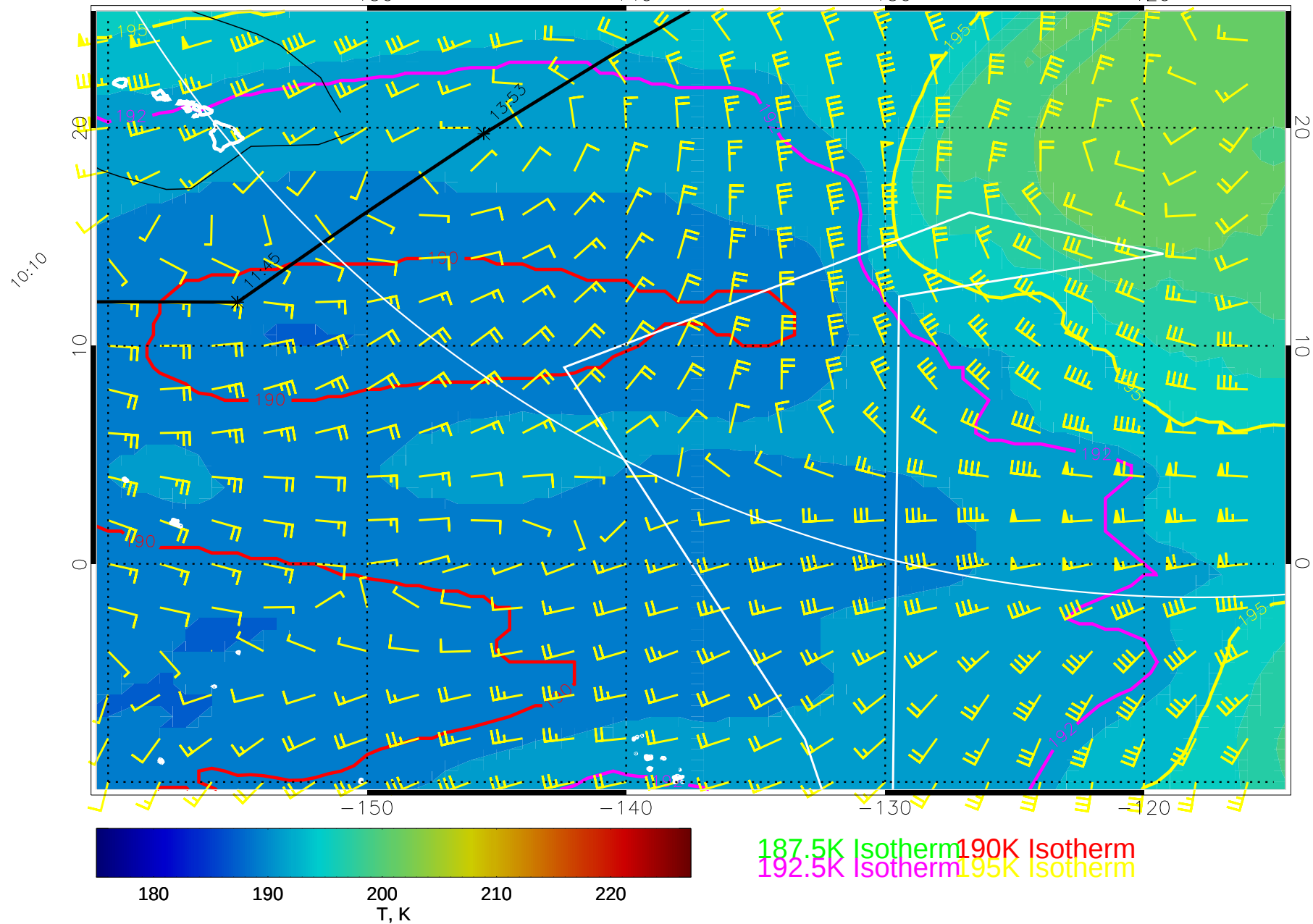
15011612, 12 hour forecast for 100mb T and winds (knots) -- NCEP GFS
