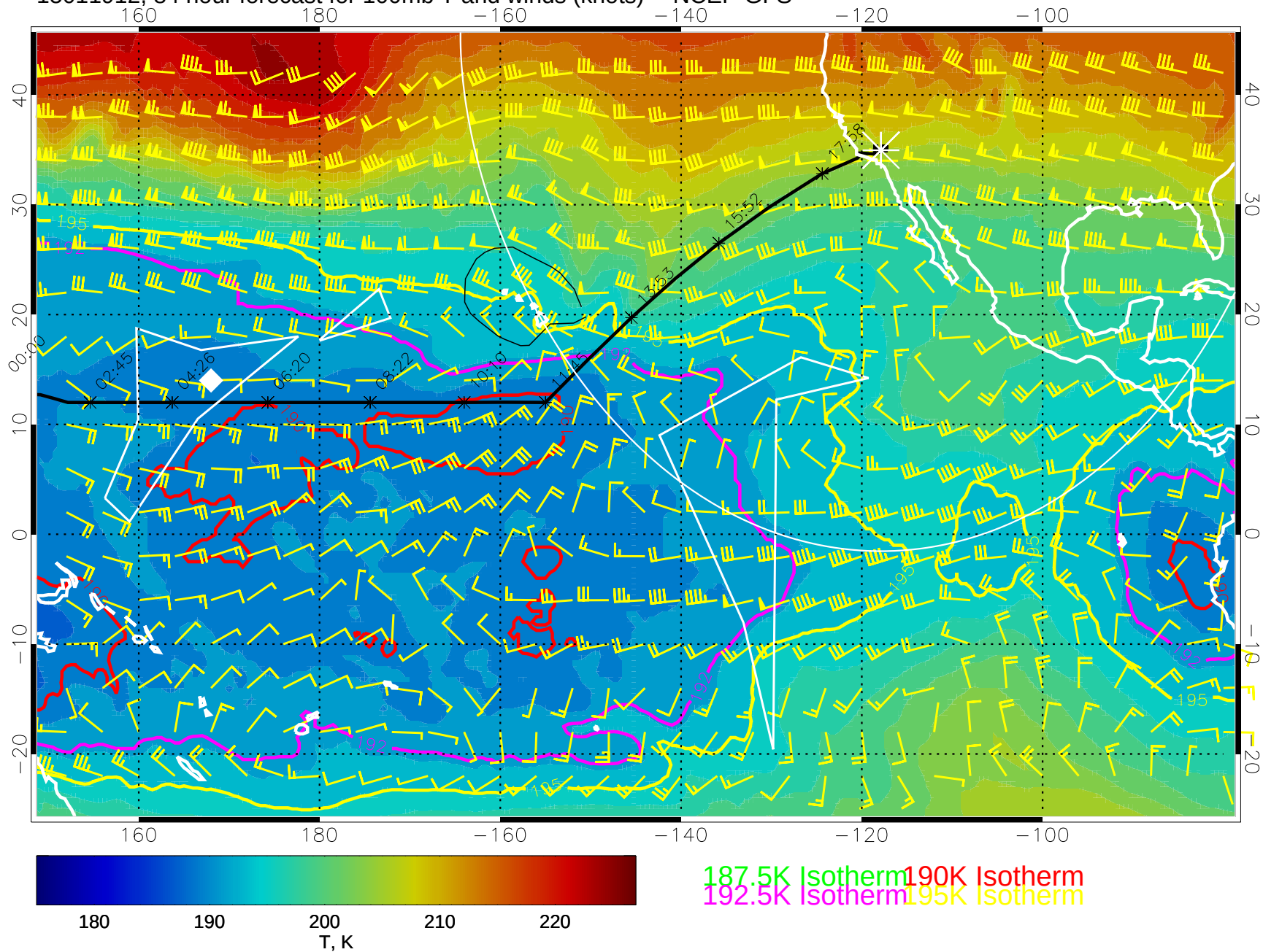
15011912, 84 hour forecast for 100mb T and winds (knots) -- NCEP GFS
