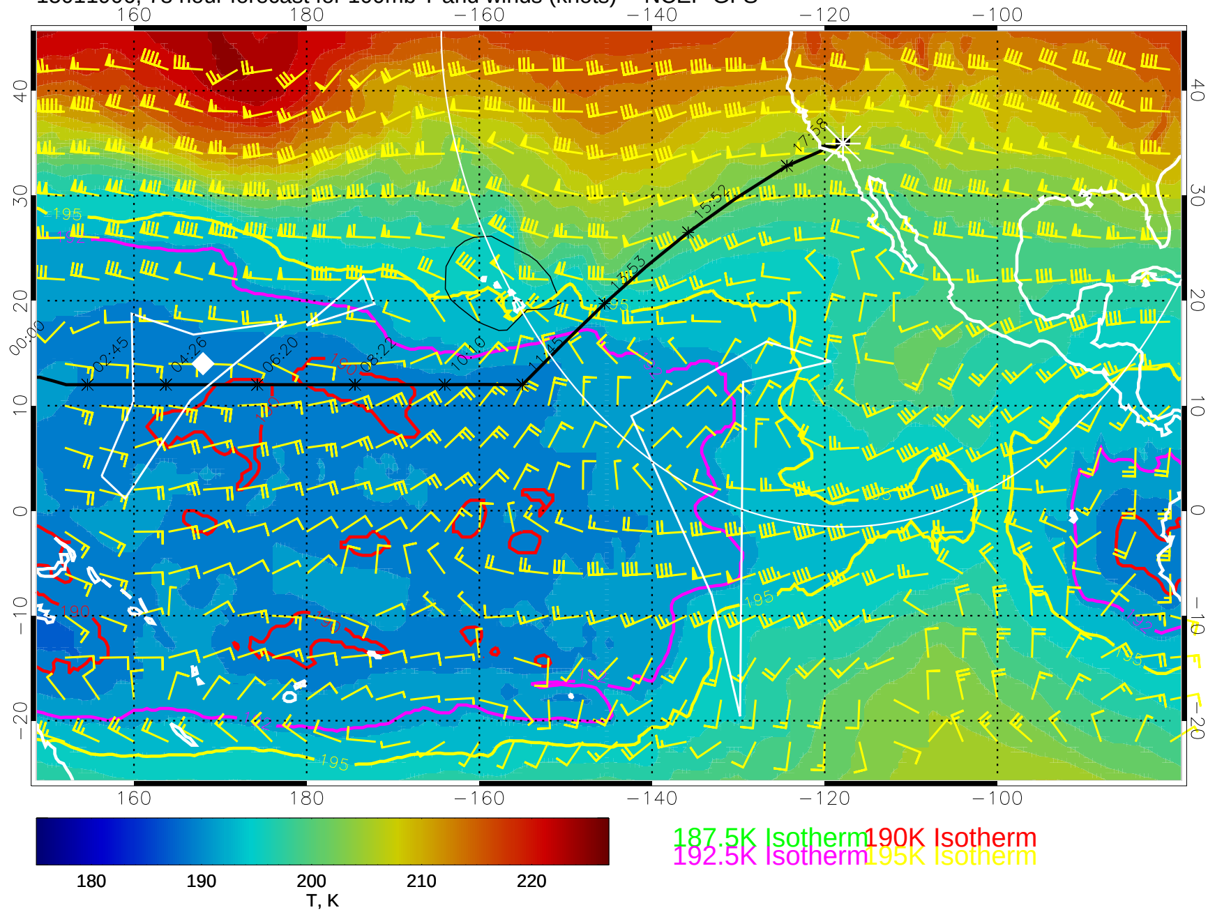
15011906, 78 hour forecast for 100mb T and winds (knots) -- NCEP GFS
