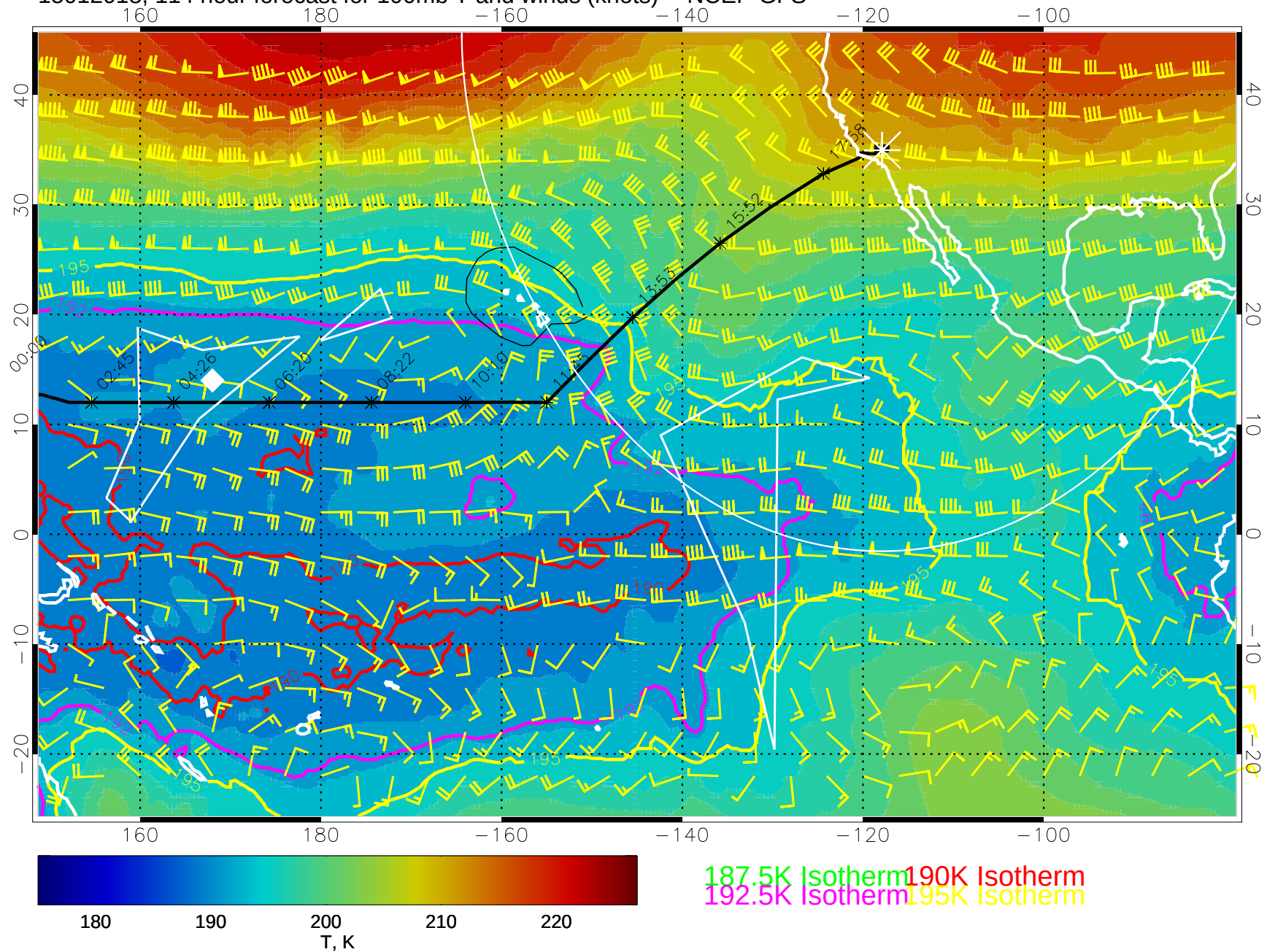
15012018, 114 hour forecast for 100mb T and winds (knots) -- NCEP GFS
