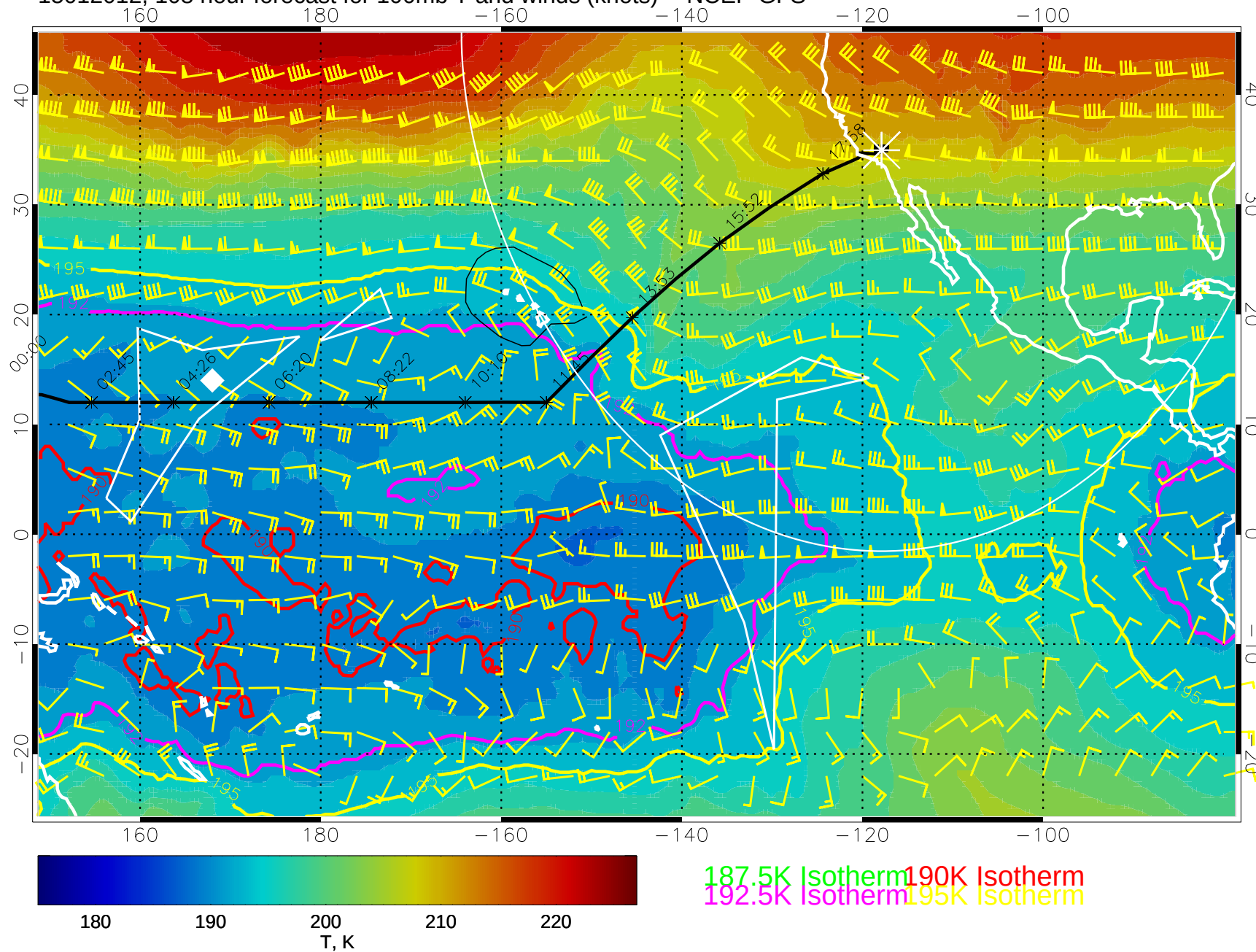
15012012, 108 hour forecast for 100mb T and winds (knots) -- NCEP GFS
