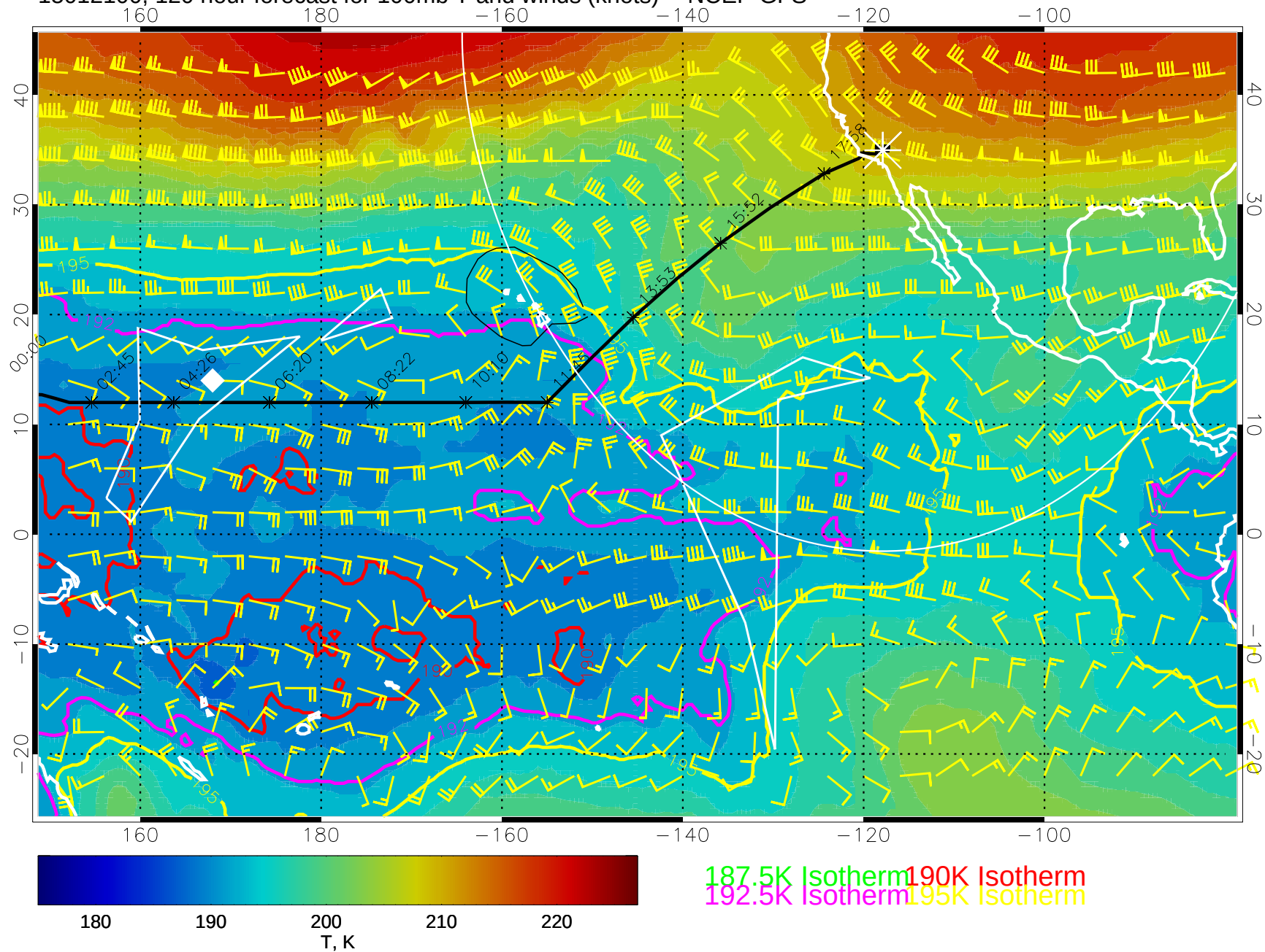
15012100, 120 hour forecast for 100mb T and winds (knots) -- NCEP GFS
