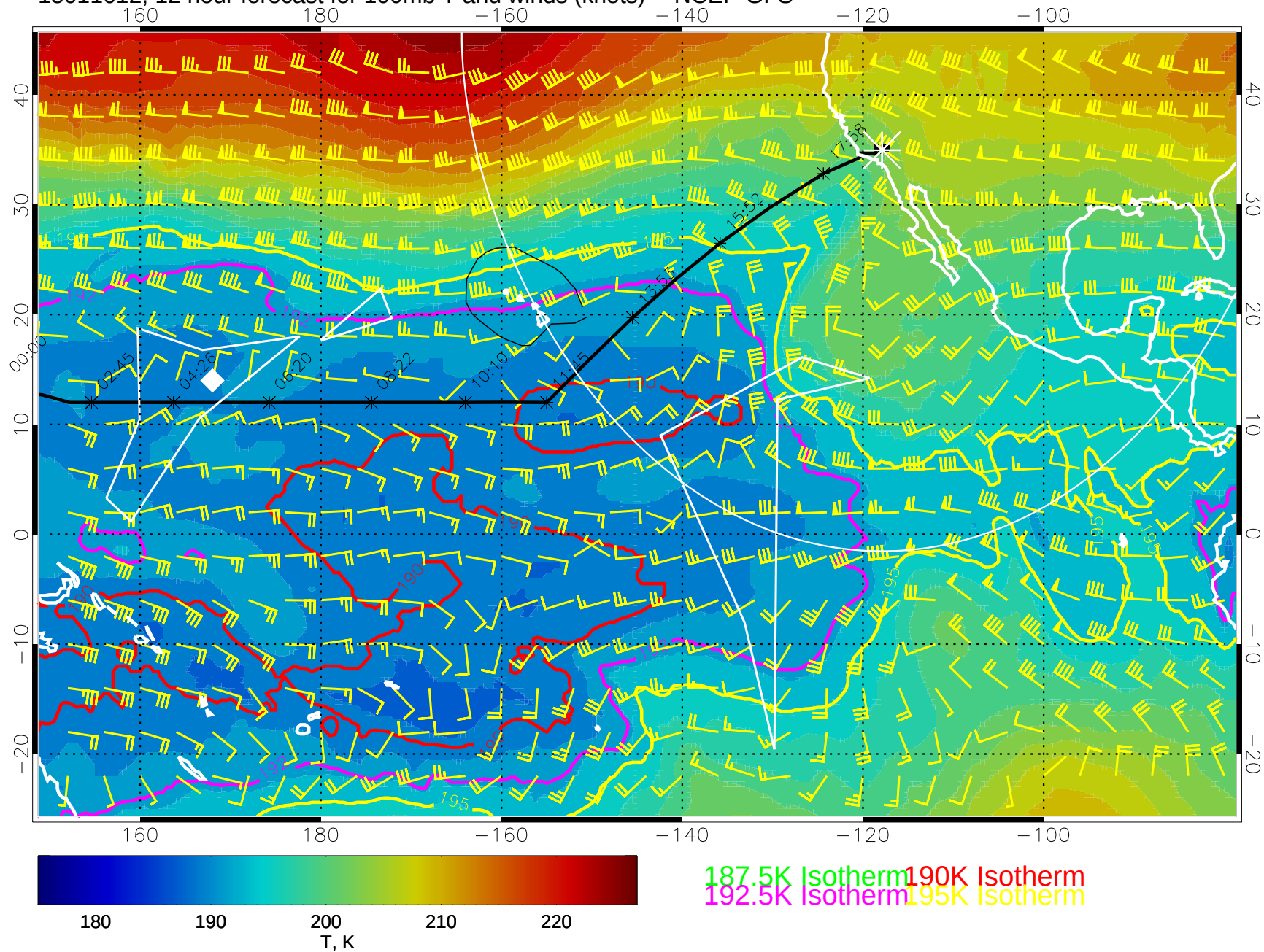
15011612, 12 hour forecast for 100mb T and winds (knots) -- NCEP GFS
