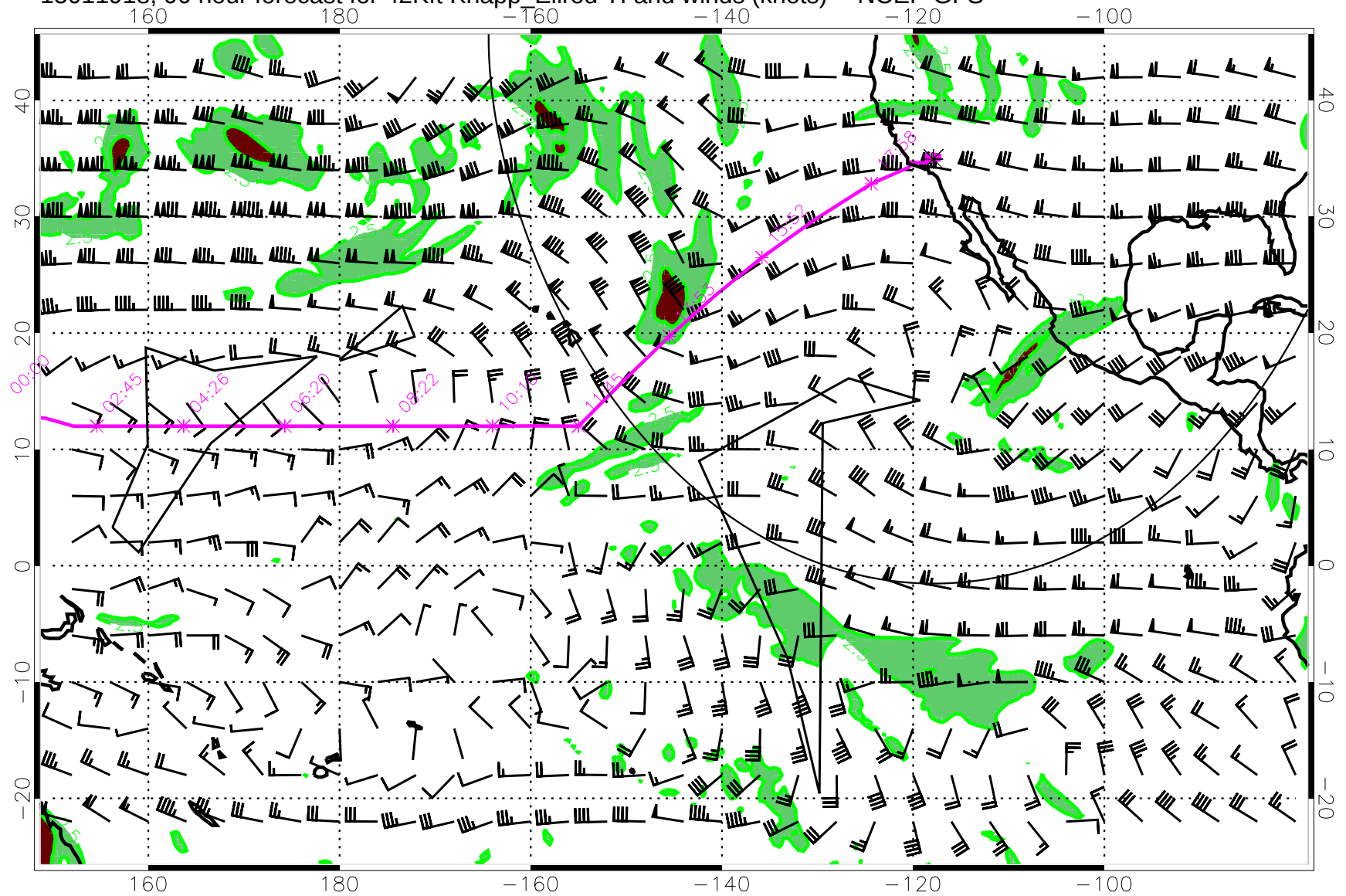
15011918, 90 hour forecast for 42Kft Knapp_Ellrod TI and winds (knots) -- NCEP GFS
