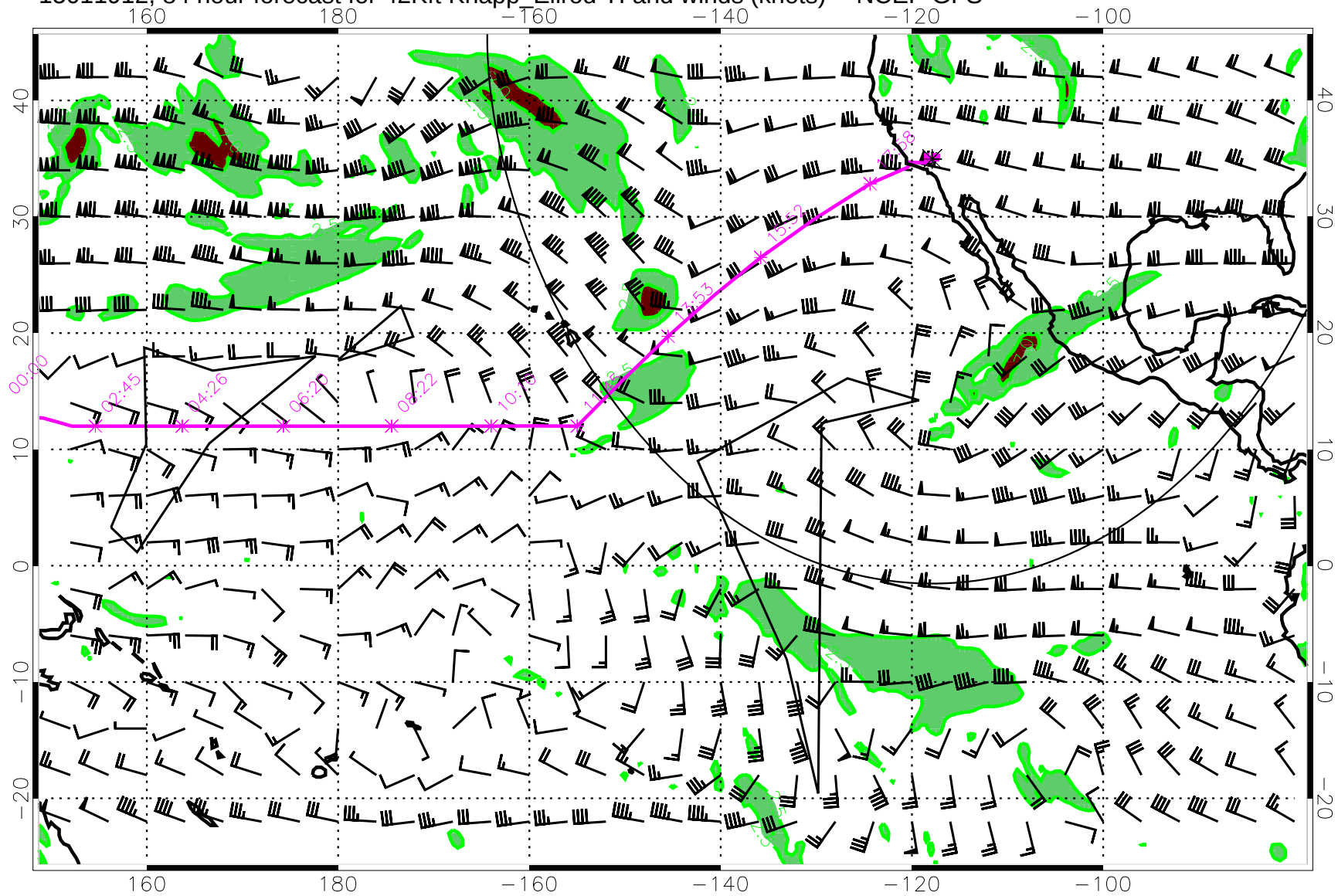
15011912, 84 hour forecast for 42Kft Knapp_Ellrod TI and winds (knots) -- NCEP GFS
