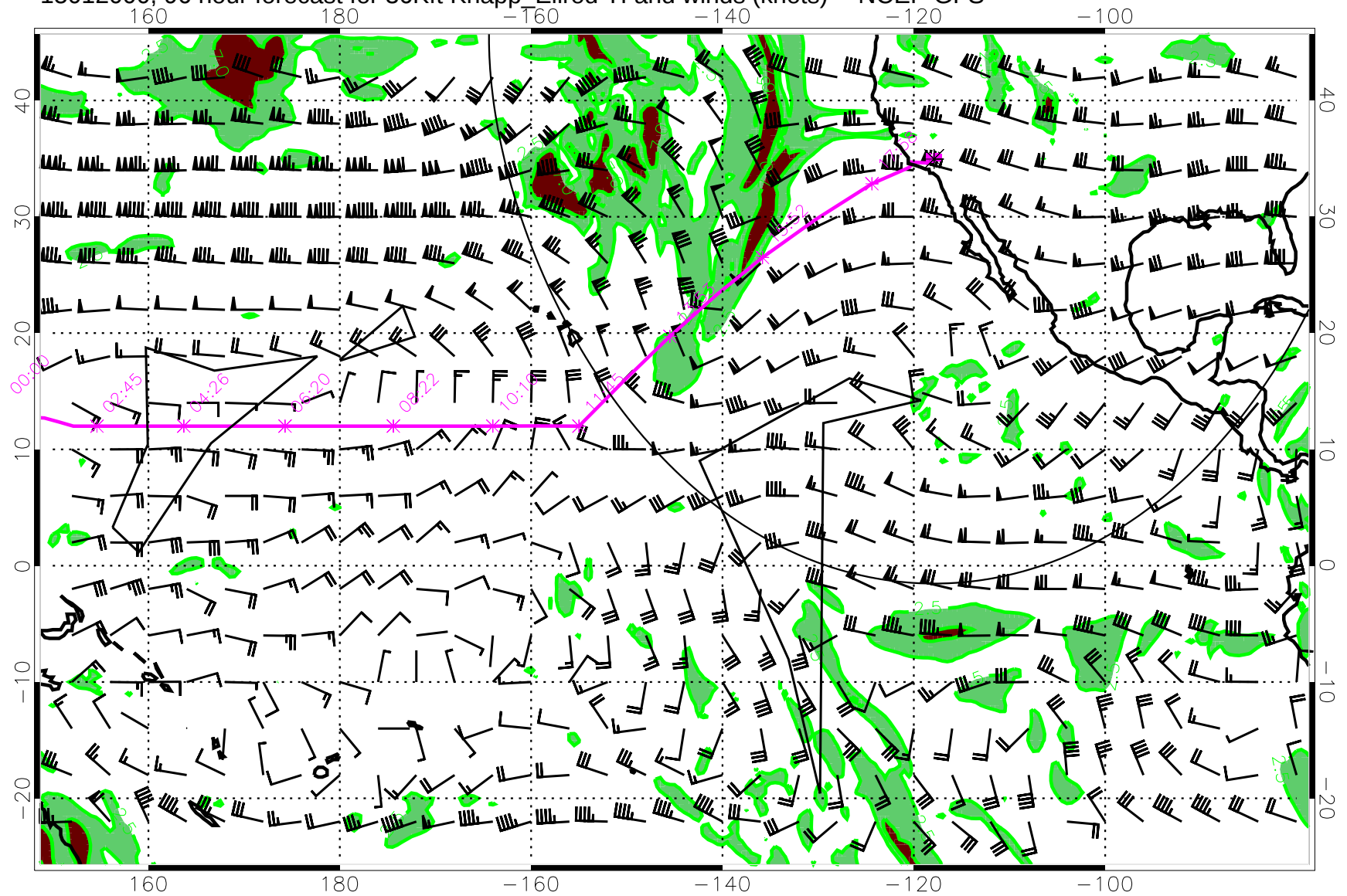
15012000, 96 hour forecast for 36Kft Knapp_Ellrod TI and winds (knots) -- NCEP GFS
