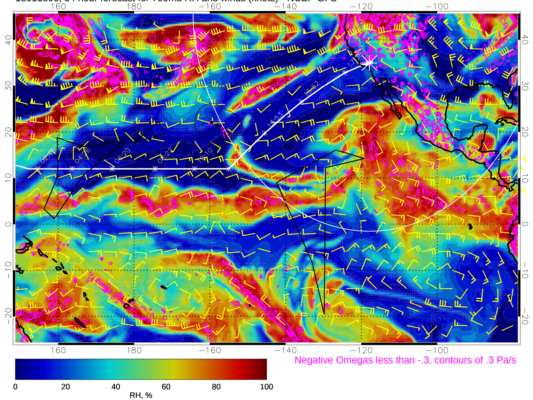
15011806, 54 hour forecast for 700mb RH and winds (knots) - NCEP GFS
