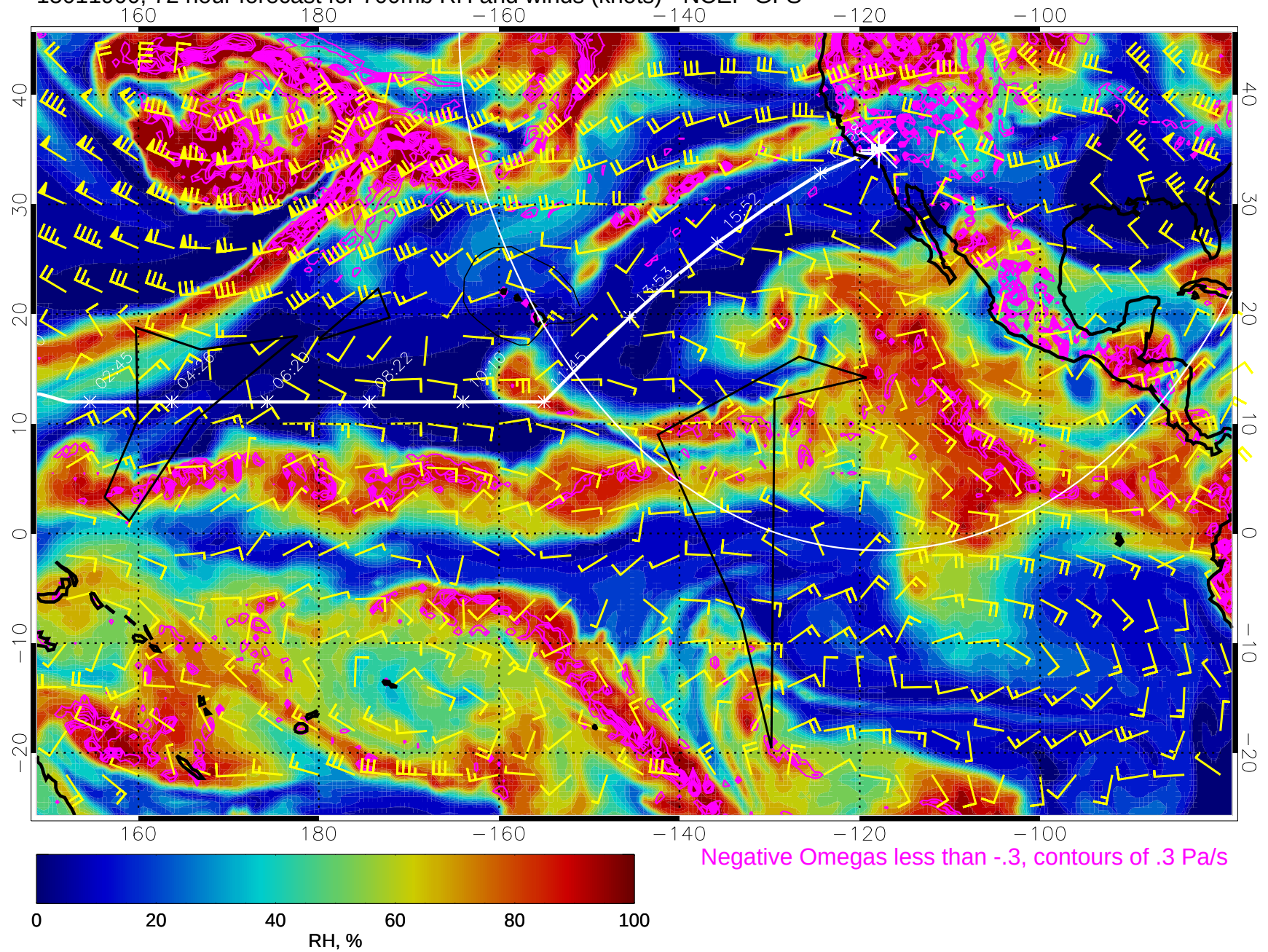
15011900, 72 hour forecast for 700mb RH and winds (knots) - NCEP GFS
