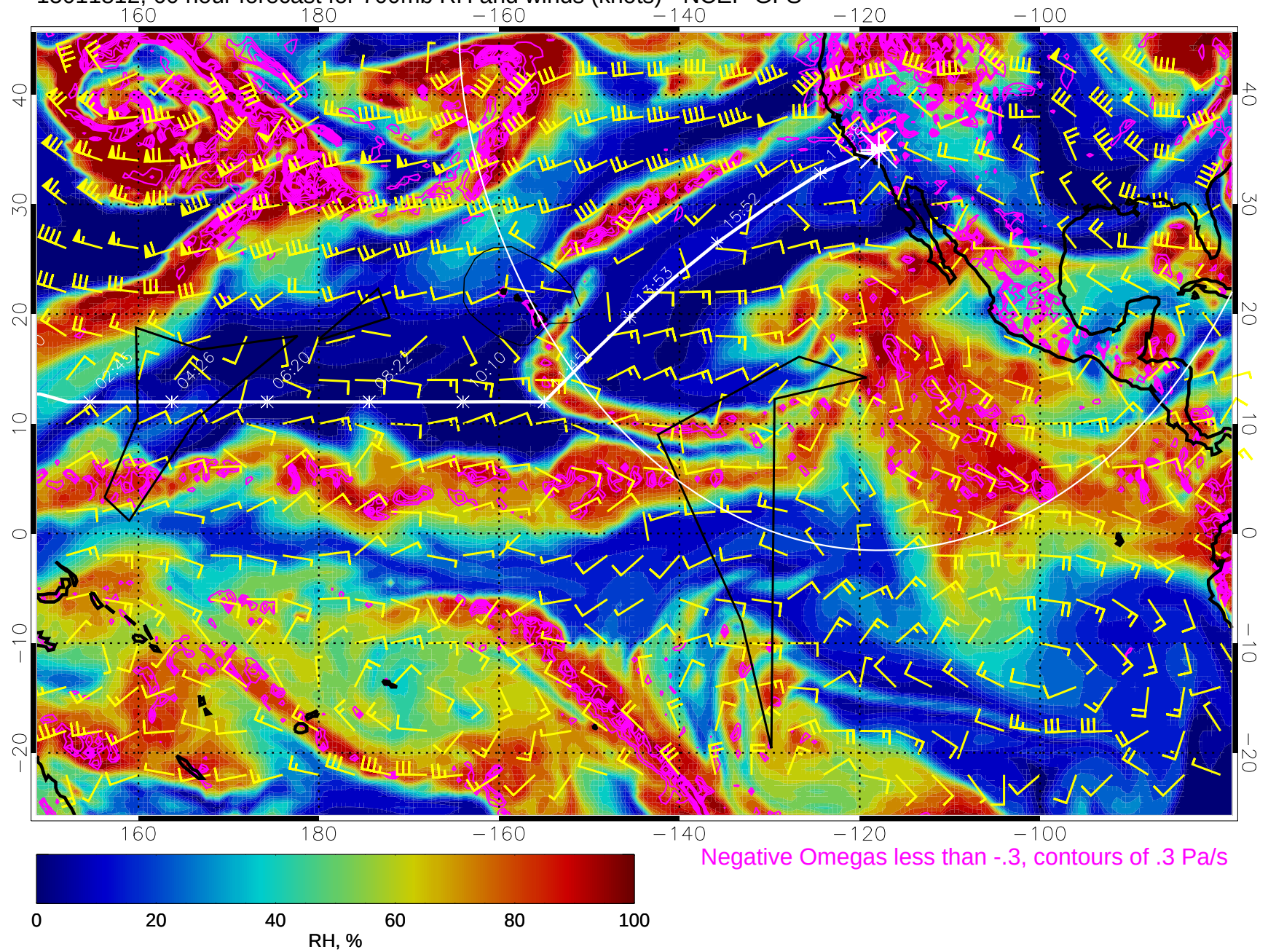
15011812, 60 hour forecast for 700mb RH and winds (knots) - NCEP GFS
