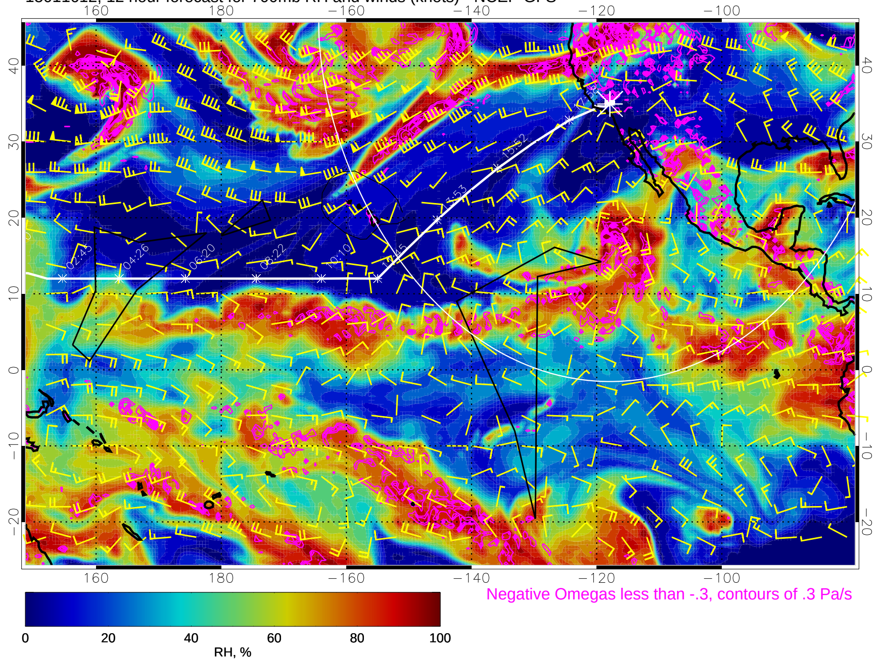
15011612, 12 hour forecast for 700mb RH and winds (knots) - NCEP GFS
