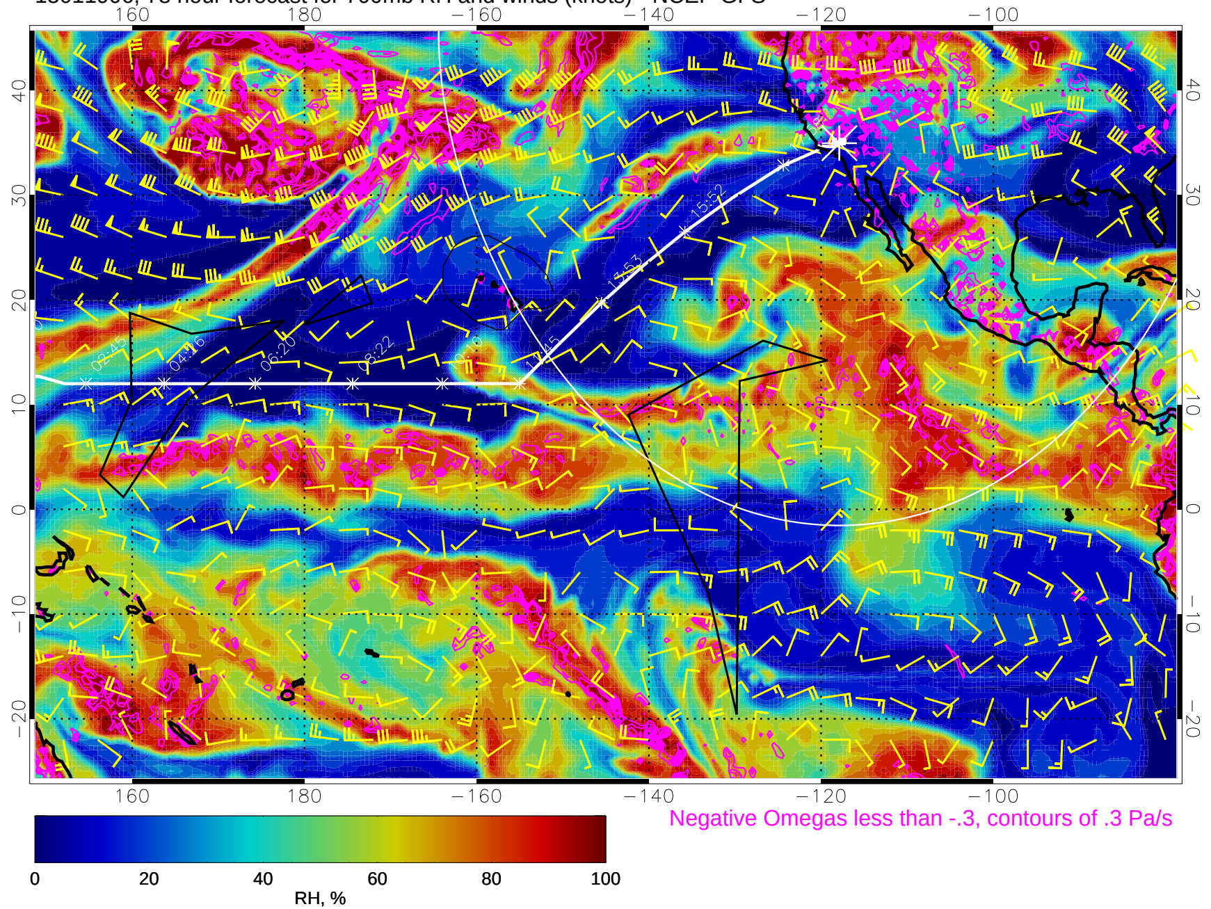
15011906, 78 hour forecast for 700mb RH and winds (knots) - NCEP GFS
