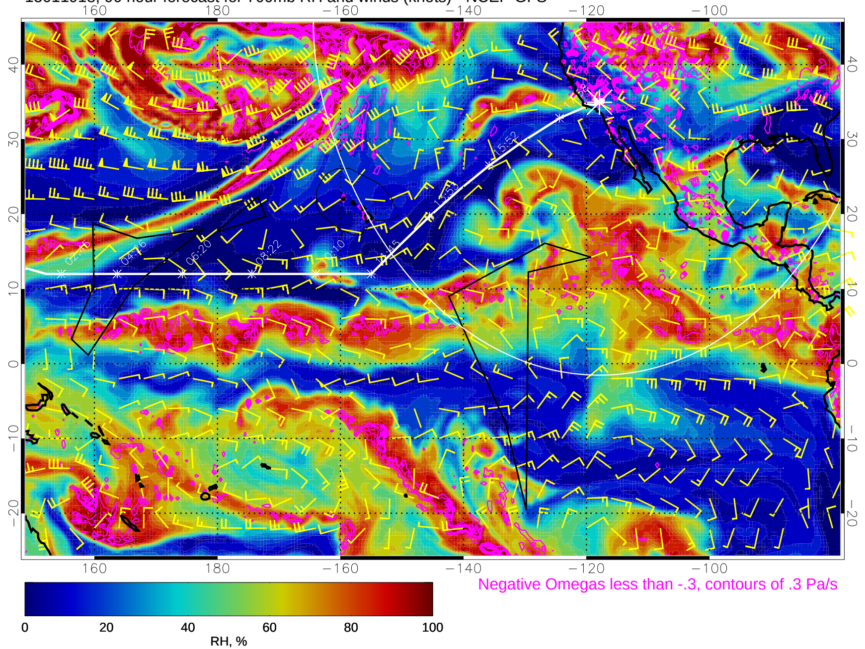
15011918, 90 hour forecast for 700mb RH and winds (knots) - NCEP GFS
