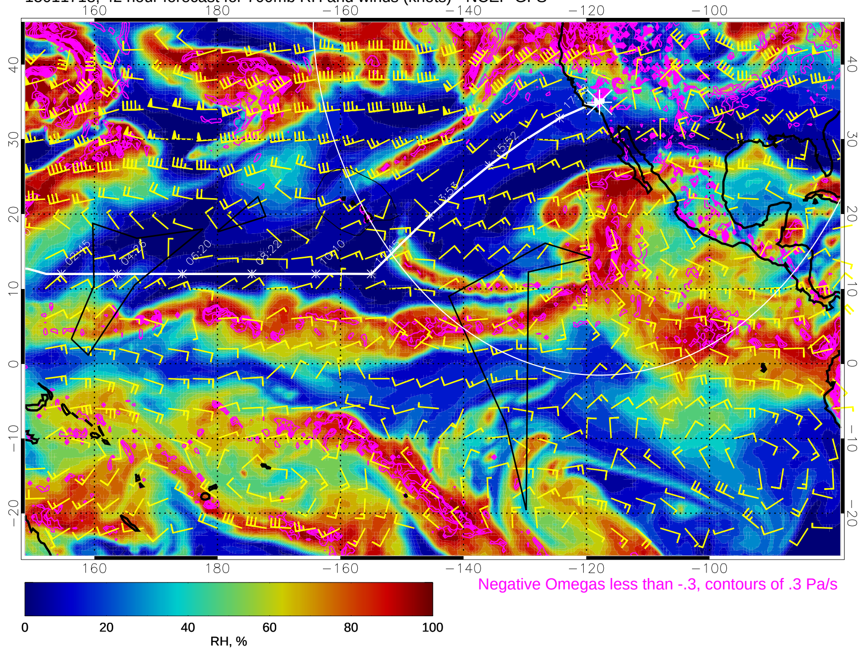
15011718, 42 hour forecast for 700mb RH and winds (knots) - NCEP GFS
