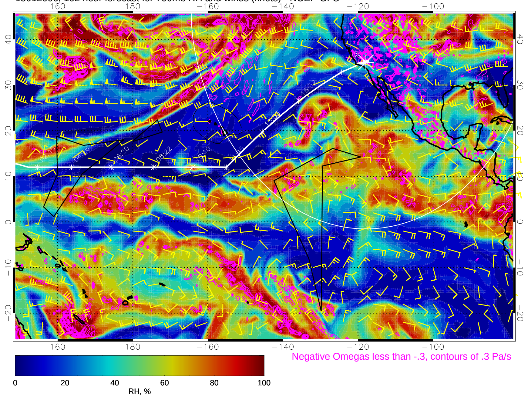
15012006, 102 hour forecast for 700mb RH and winds (knots) - NCEP GFS
