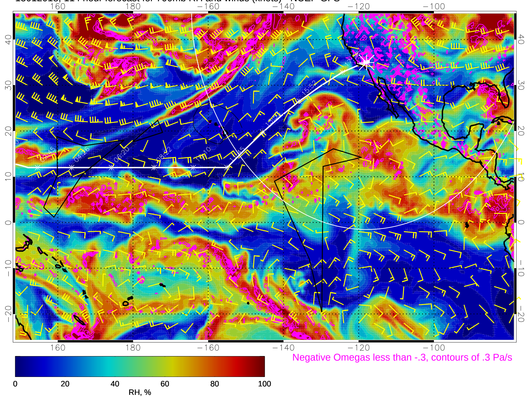
15012018, 114 hour forecast for 700mb RH and winds (knots) - NCEP GFS
