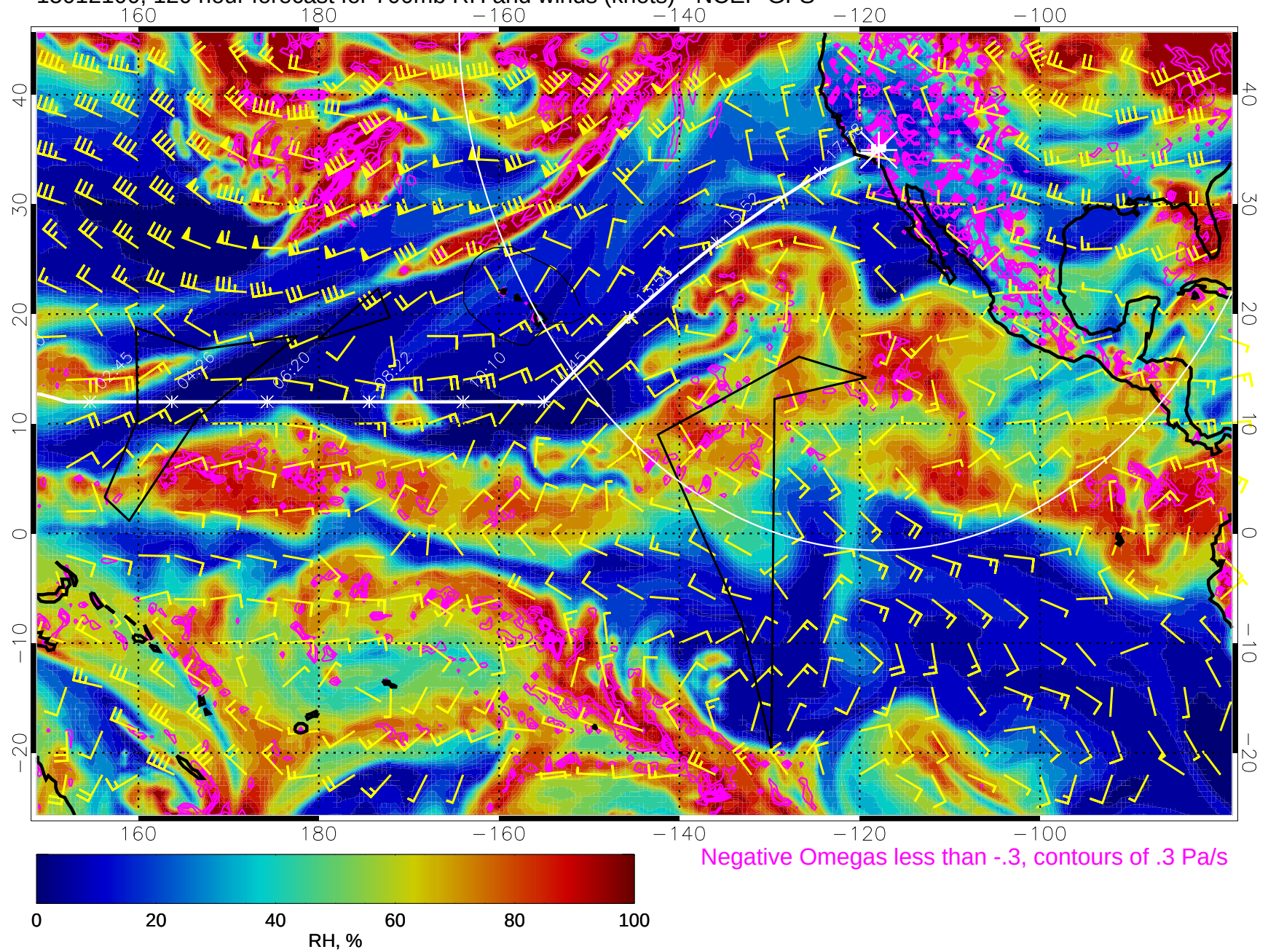
15012100, 120 hour forecast for 700mb RH and winds (knots) - NCEP GFS
