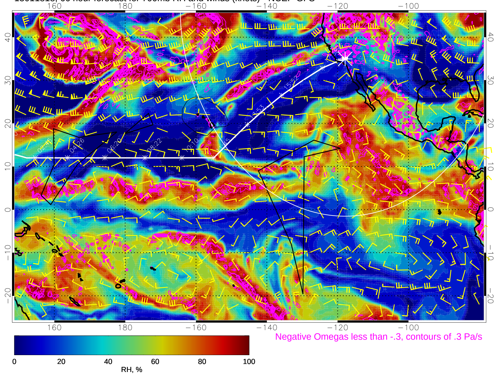
15011818, 66 hour forecast for 700mb RH and winds (knots) - NCEP GFS
