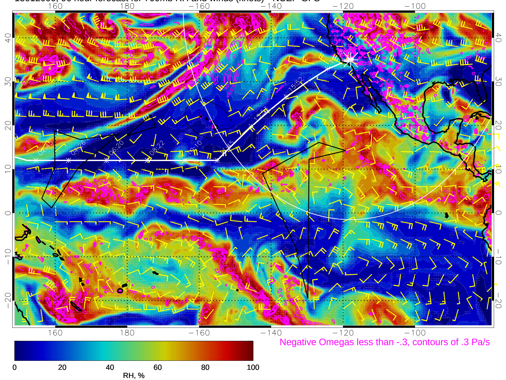
15012000, 96 hour forecast for 700mb RH and winds (knots) - NCEP GFS
