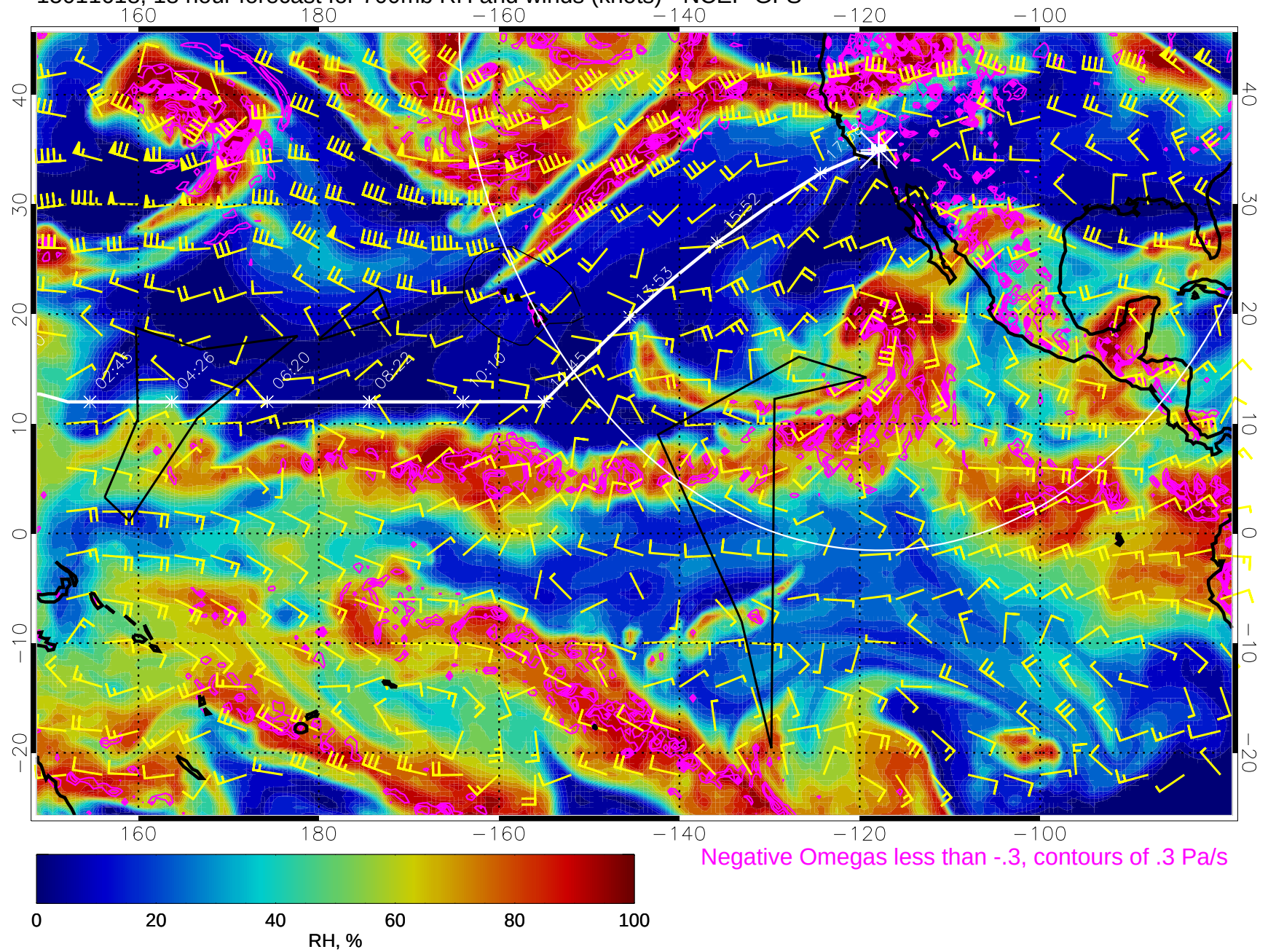
15011618, 18 hour forecast for 700mb RH and winds (knots) - NCEP GFS
