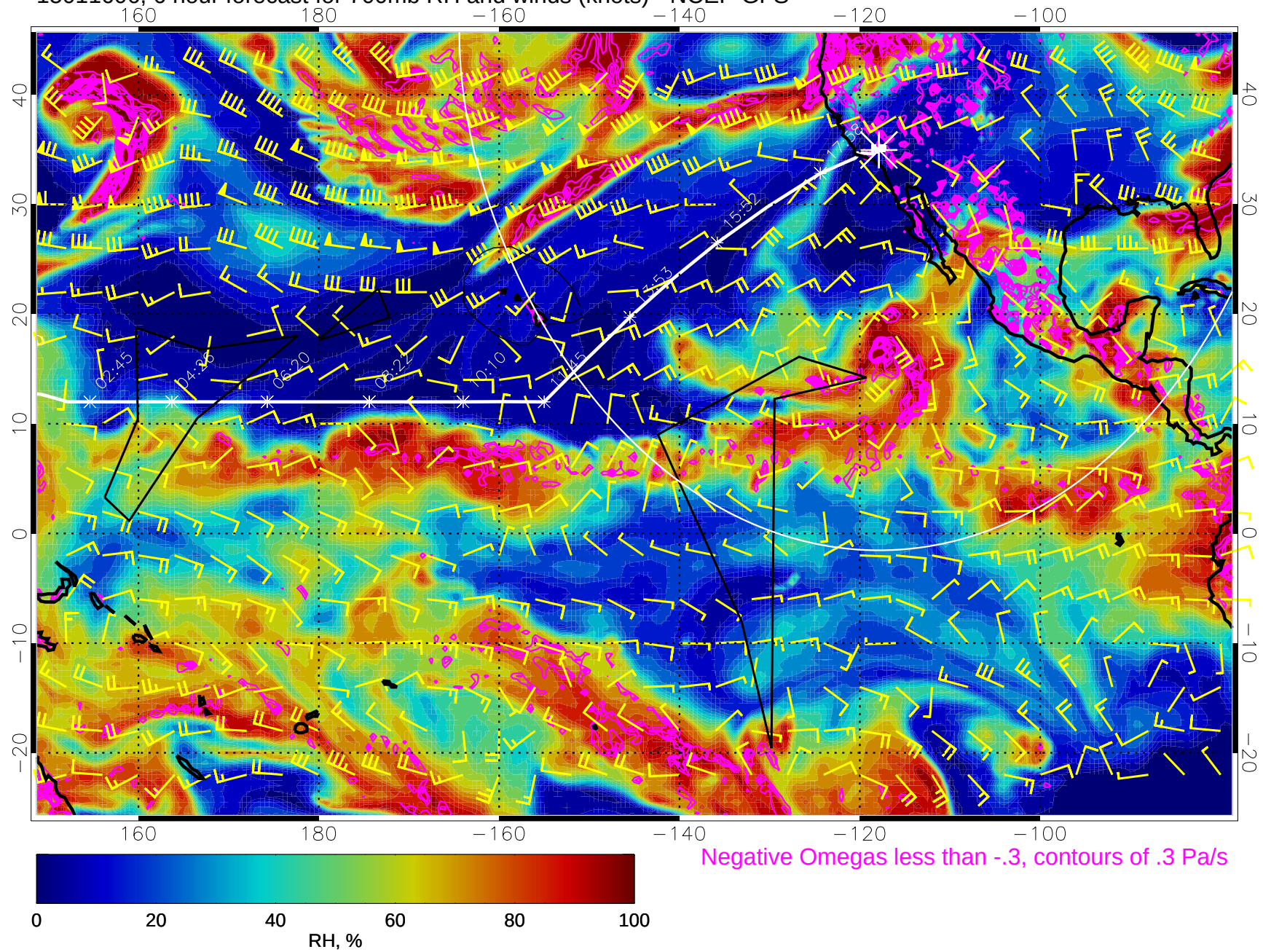
15011606, 6 hour forecast for 700mb RH and winds (knots) - NCEP GFS
