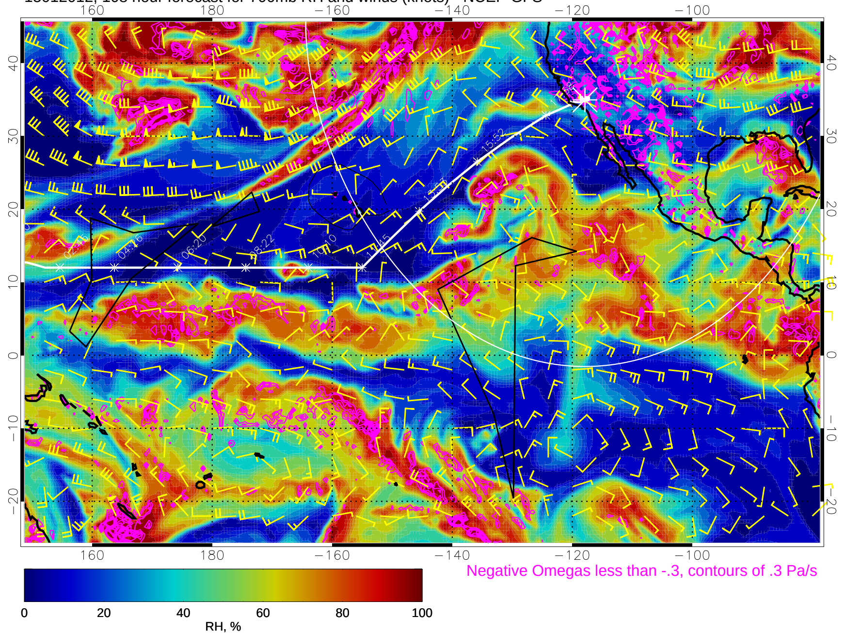
15012012, 108 hour forecast for 700mb RH and winds (knots) - NCEP GFS
