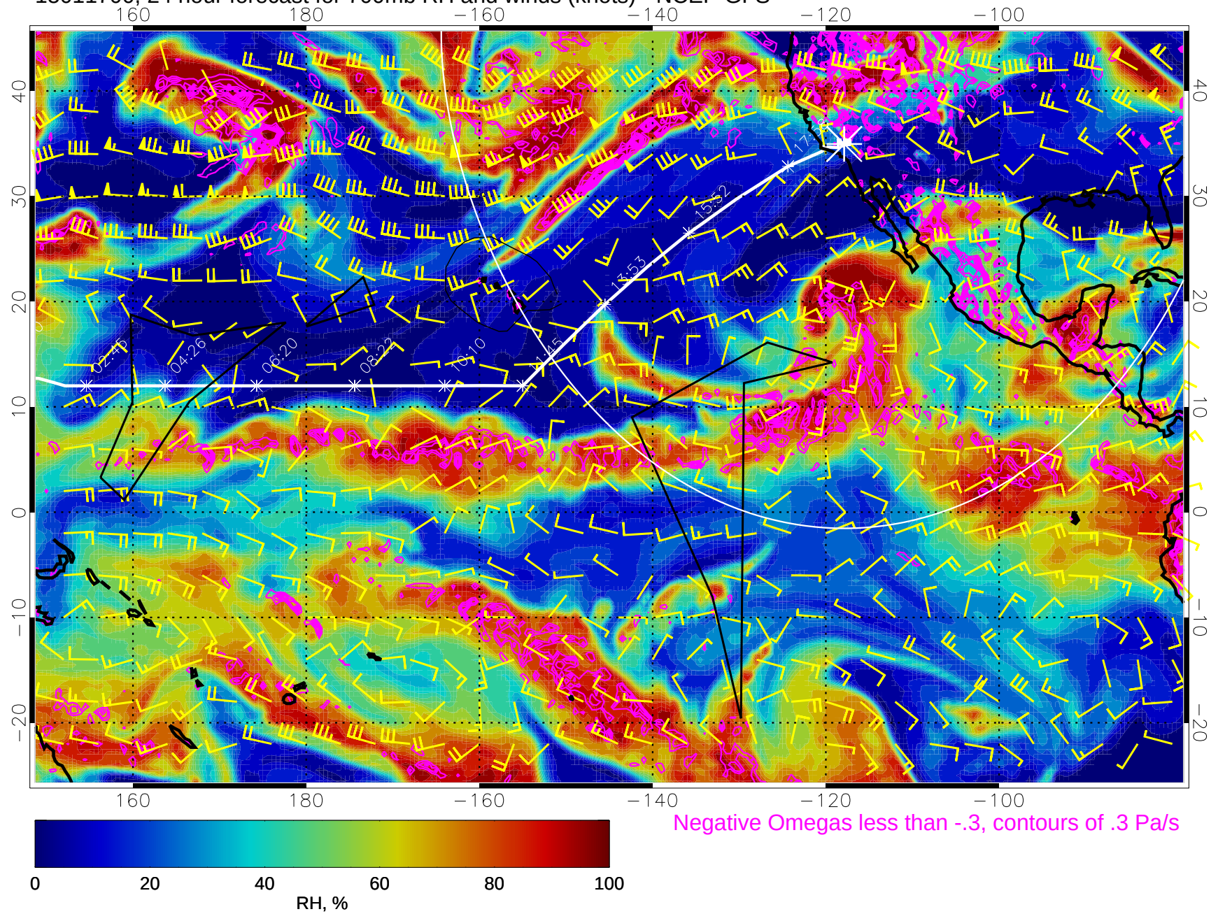
15011700, 24 hour forecast for 700mb RH and winds (knots) - NCEP GFS
