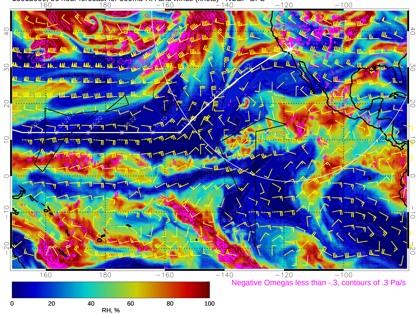
15012000, 96 hour forecast for 500mb RH and winds (knots) - NCEP GFS
