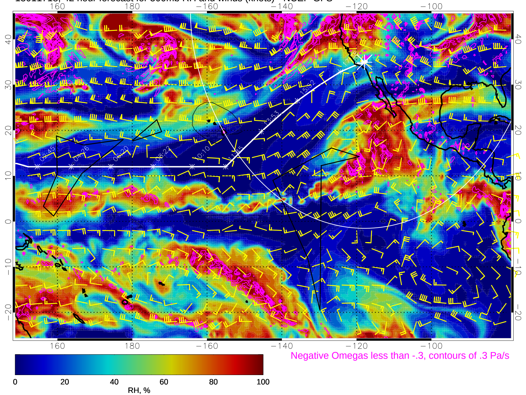
15011718, 42 hour forecast for 500mb RH and winds (knots) - NCEP GFS
