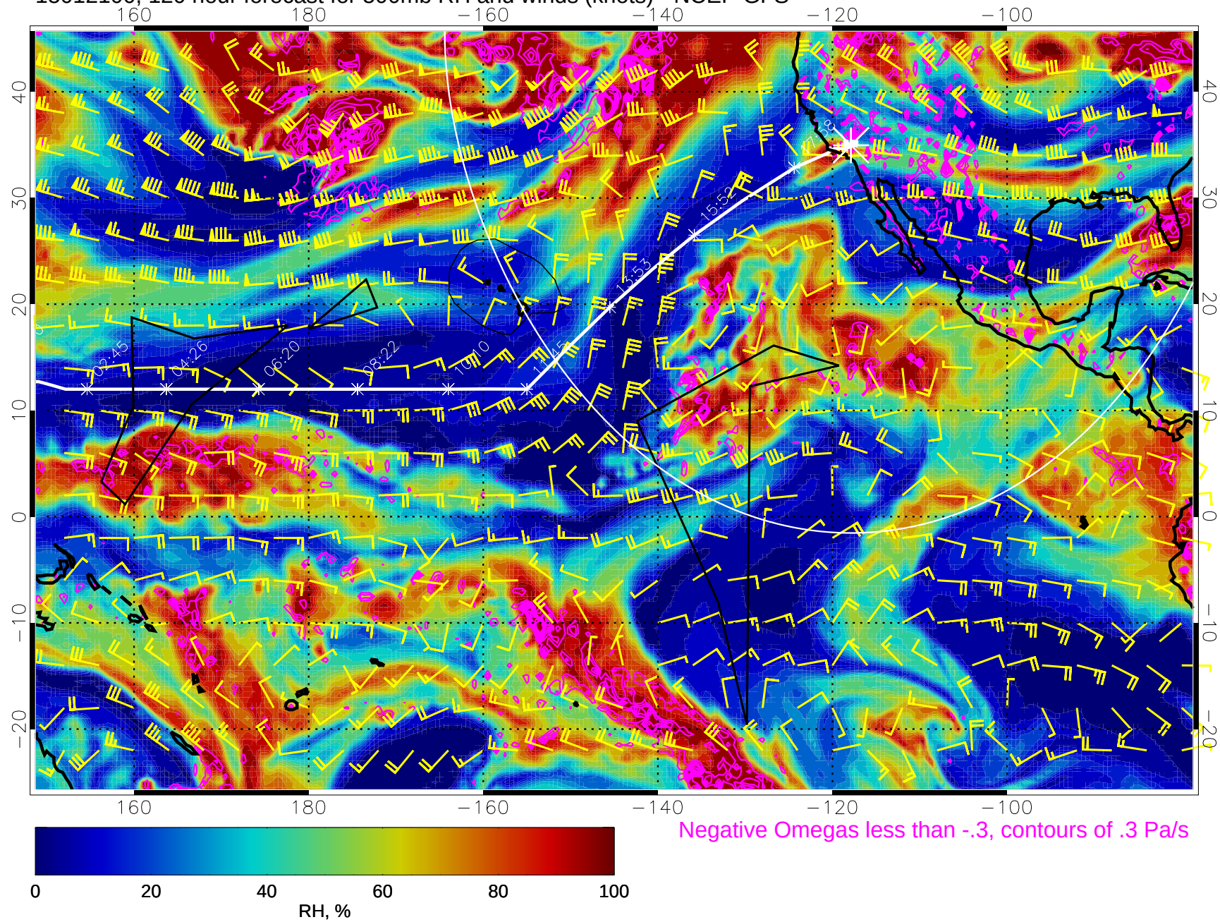
15012100, 120 hour forecast for 500mb RH and winds (knots) - NCEP GFS
