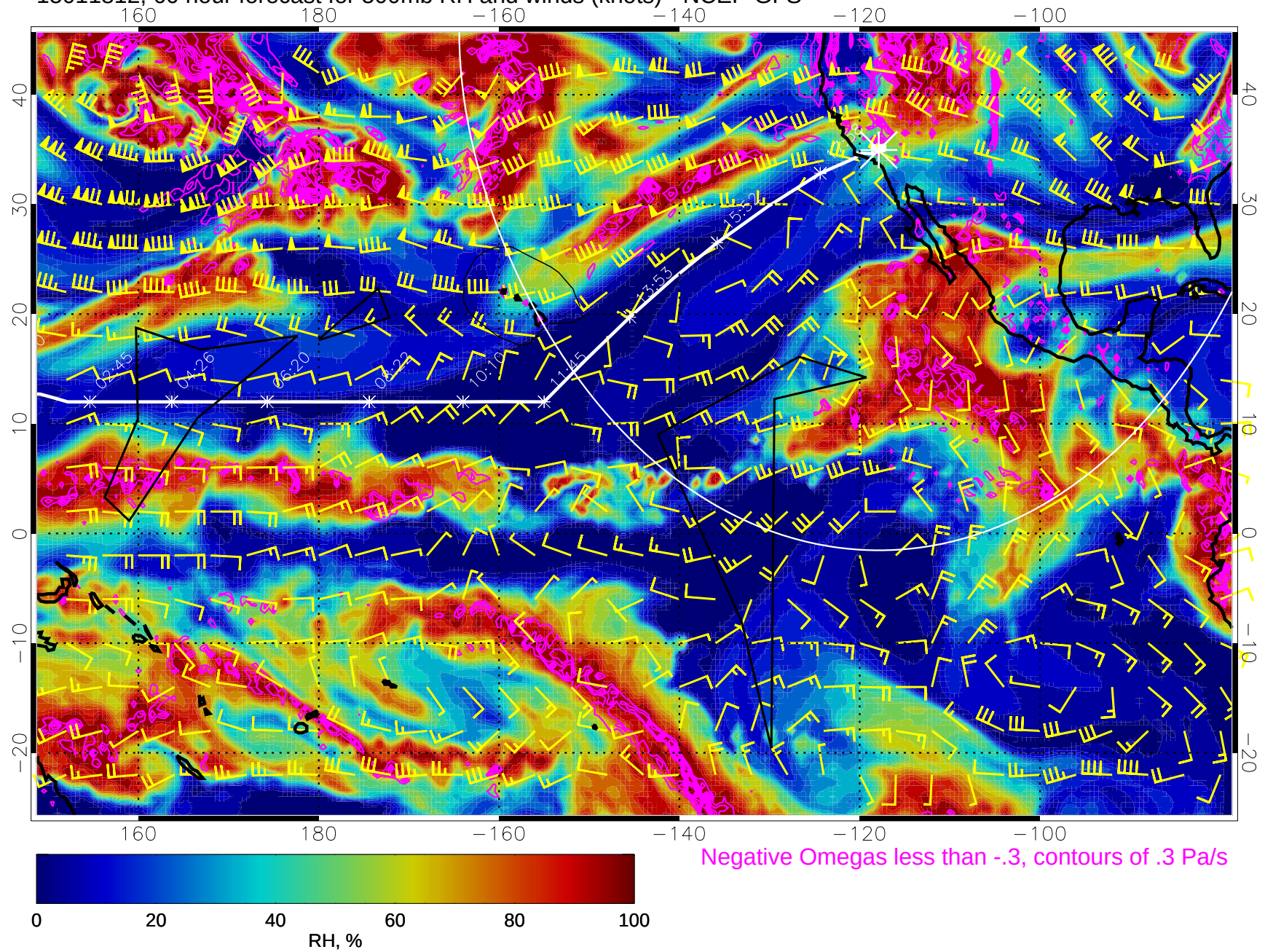
15011812, 60 hour forecast for 500mb RH and winds (knots) - NCEP GFS
