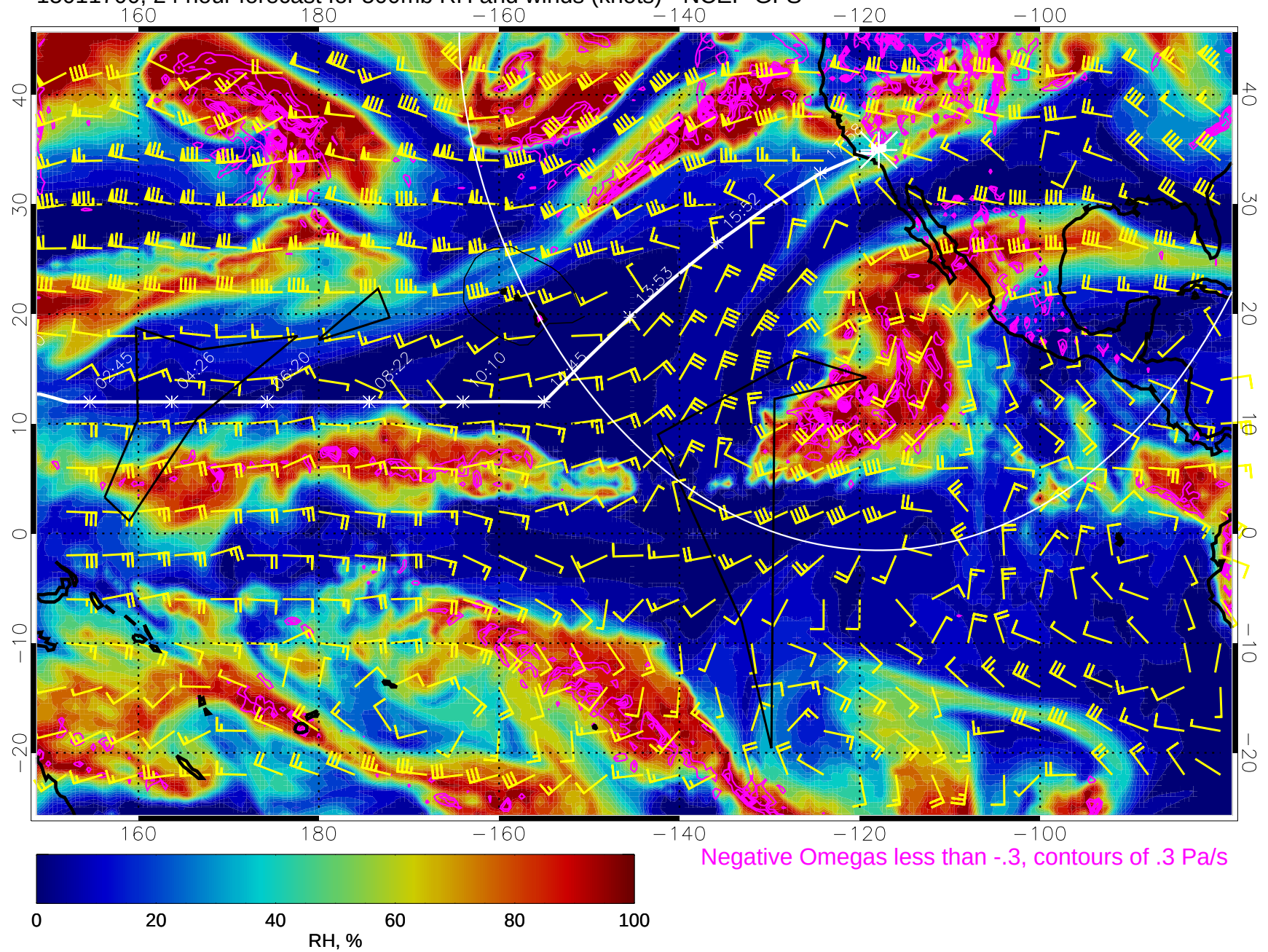
15011700, 24 hour forecast for 500mb RH and winds (knots) - NCEP GFS
