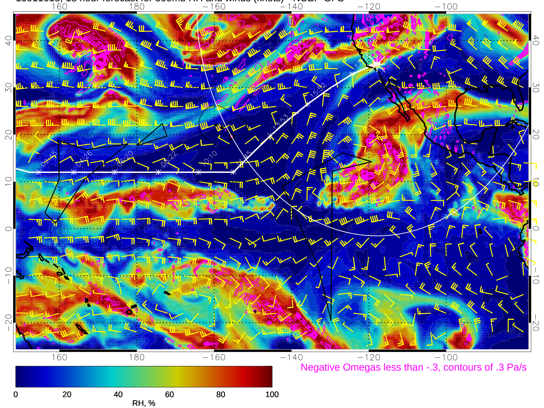
15011618, 18 hour forecast for 500mb RH and winds (knots) - NCEP GFS
