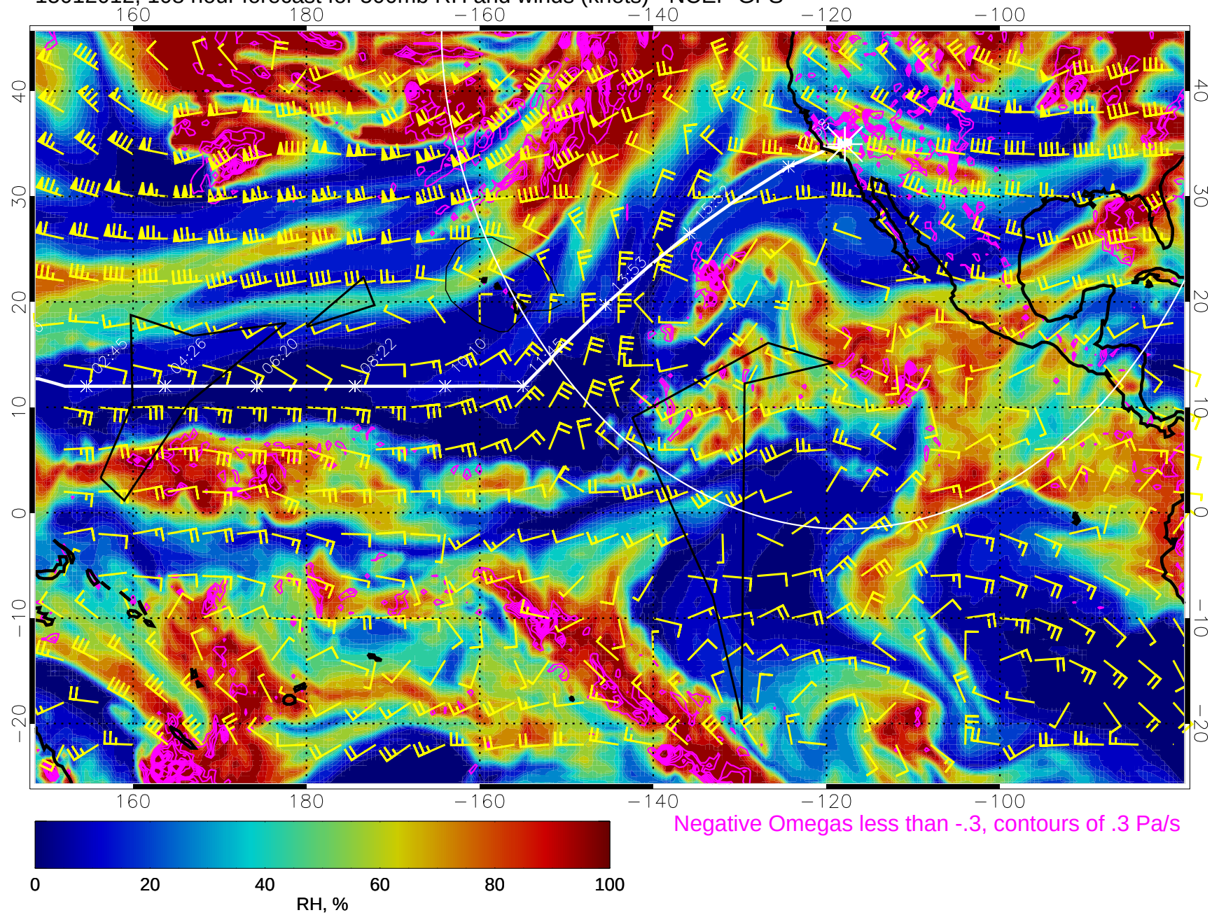
15012012, 108 hour forecast for 500mb RH and winds (knots) - NCEP GFS
