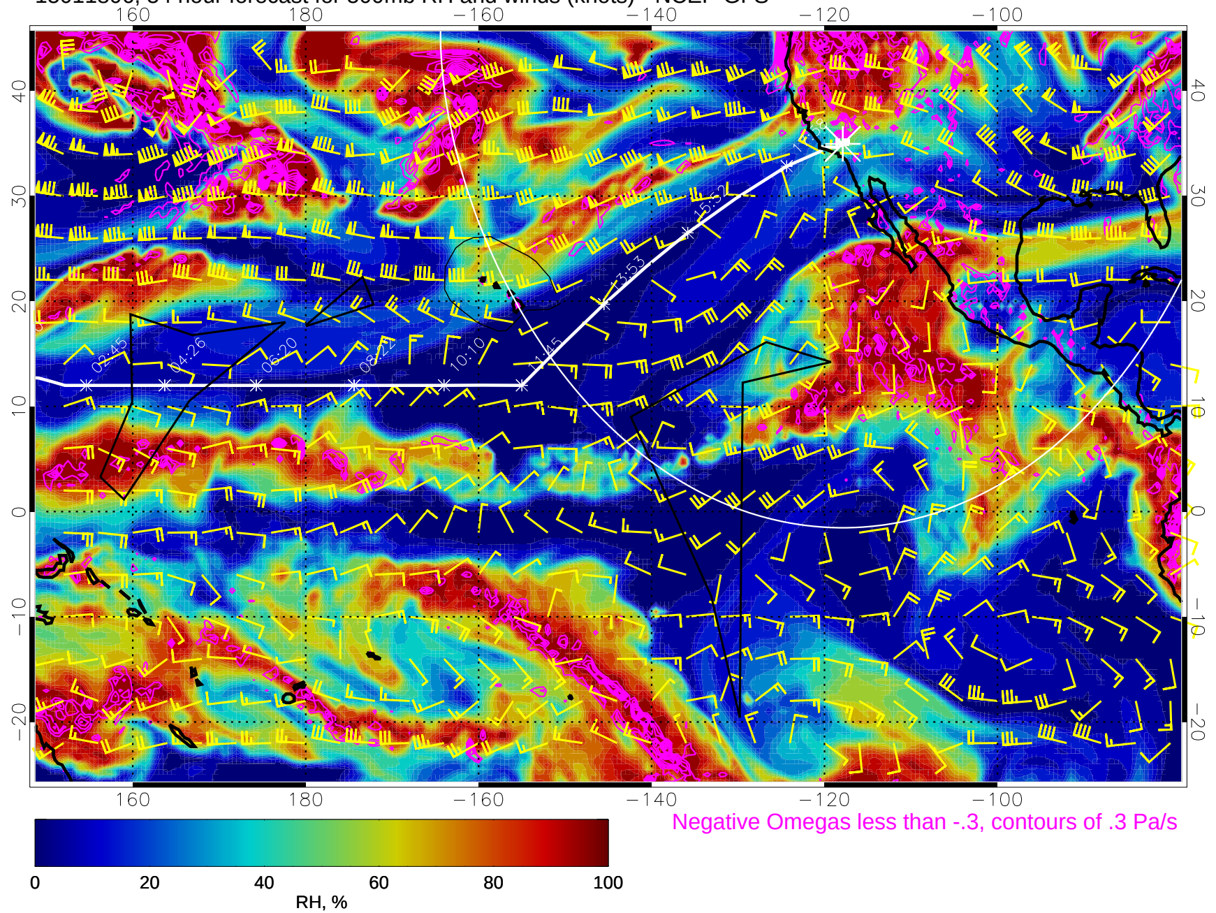
15011806, 54 hour forecast for 500mb RH and winds (knots) - NCEP GFS
