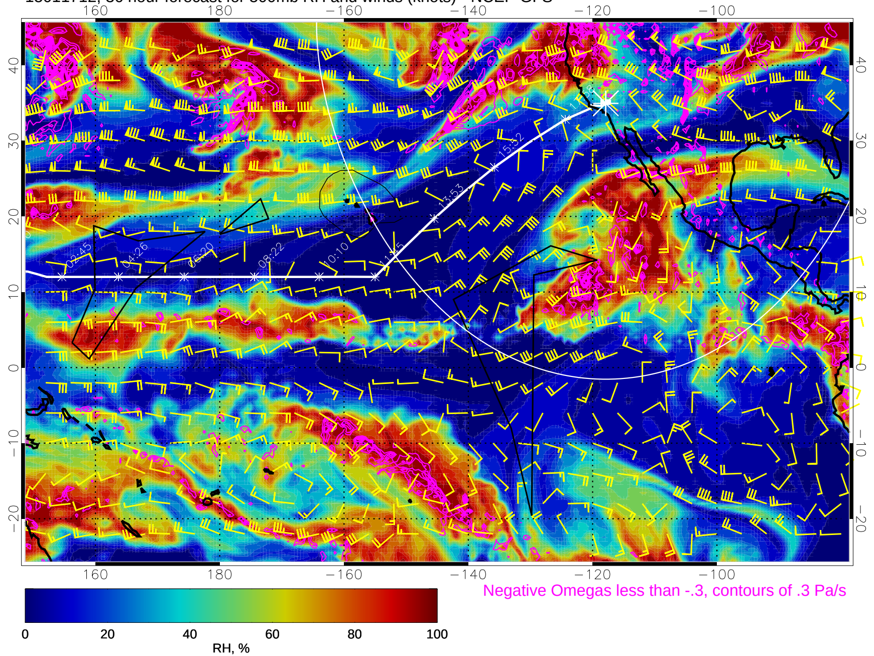
15011712, 36 hour forecast for 500mb RH and winds (knots) - NCEP GFS
