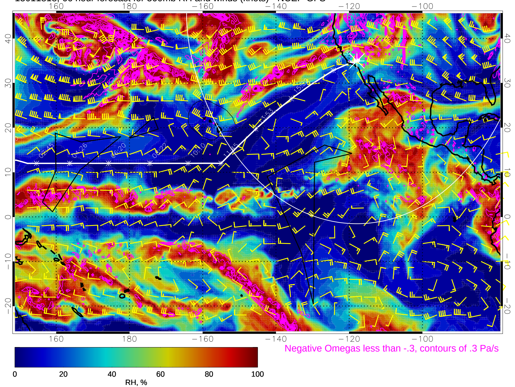
15011818, 66 hour forecast for 500mb RH and winds (knots) - NCEP GFS
