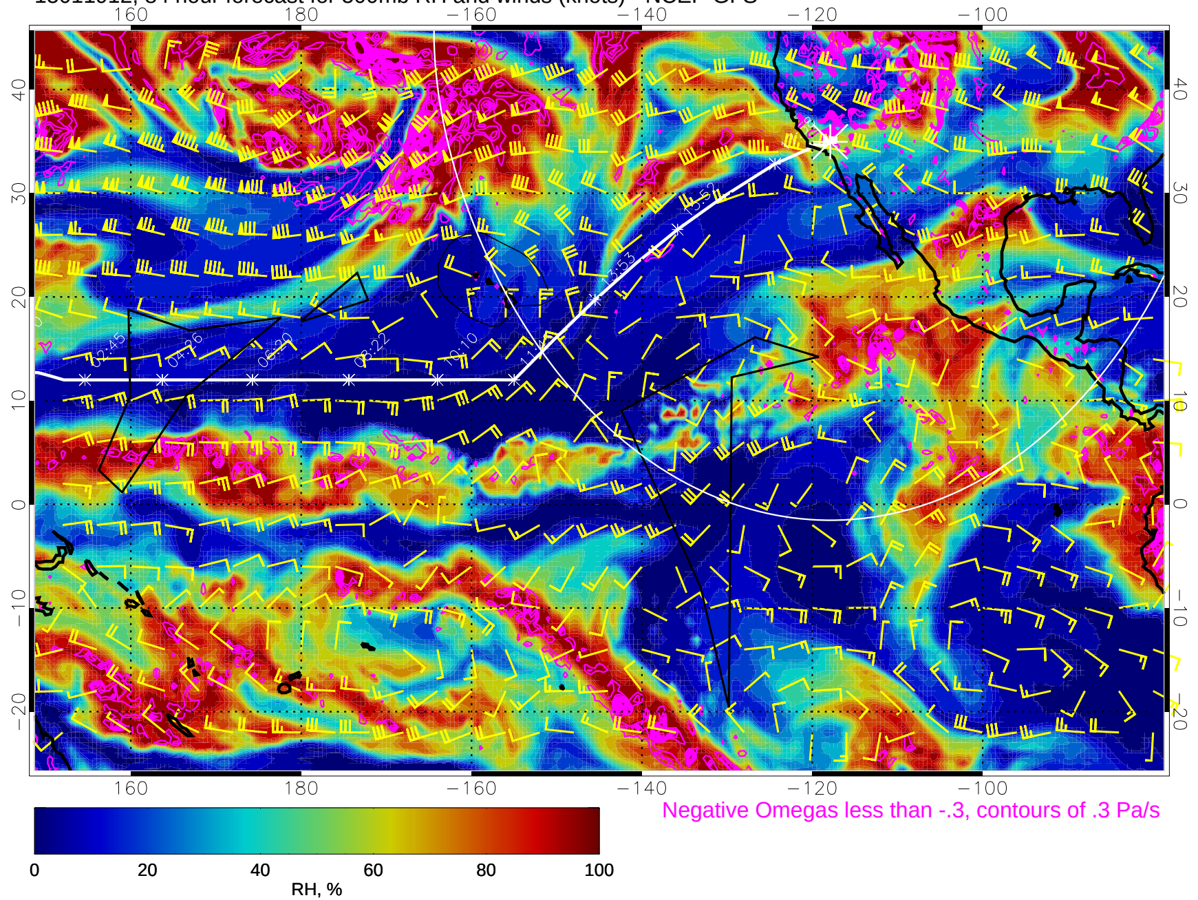
15011912, 84 hour forecast for 500mb RH and winds (knots) - NCEP GFS
