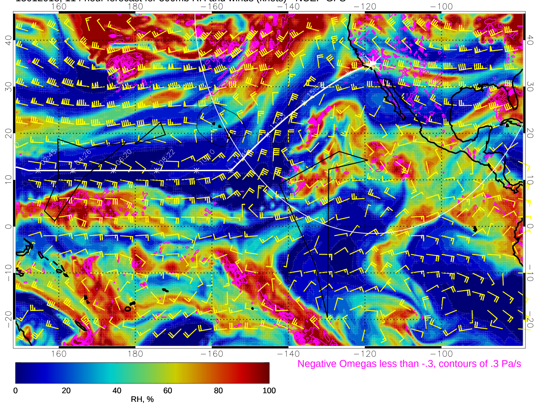
15012018, 114 hour forecast for 500mb RH and winds (knots) - NCEP GFS
