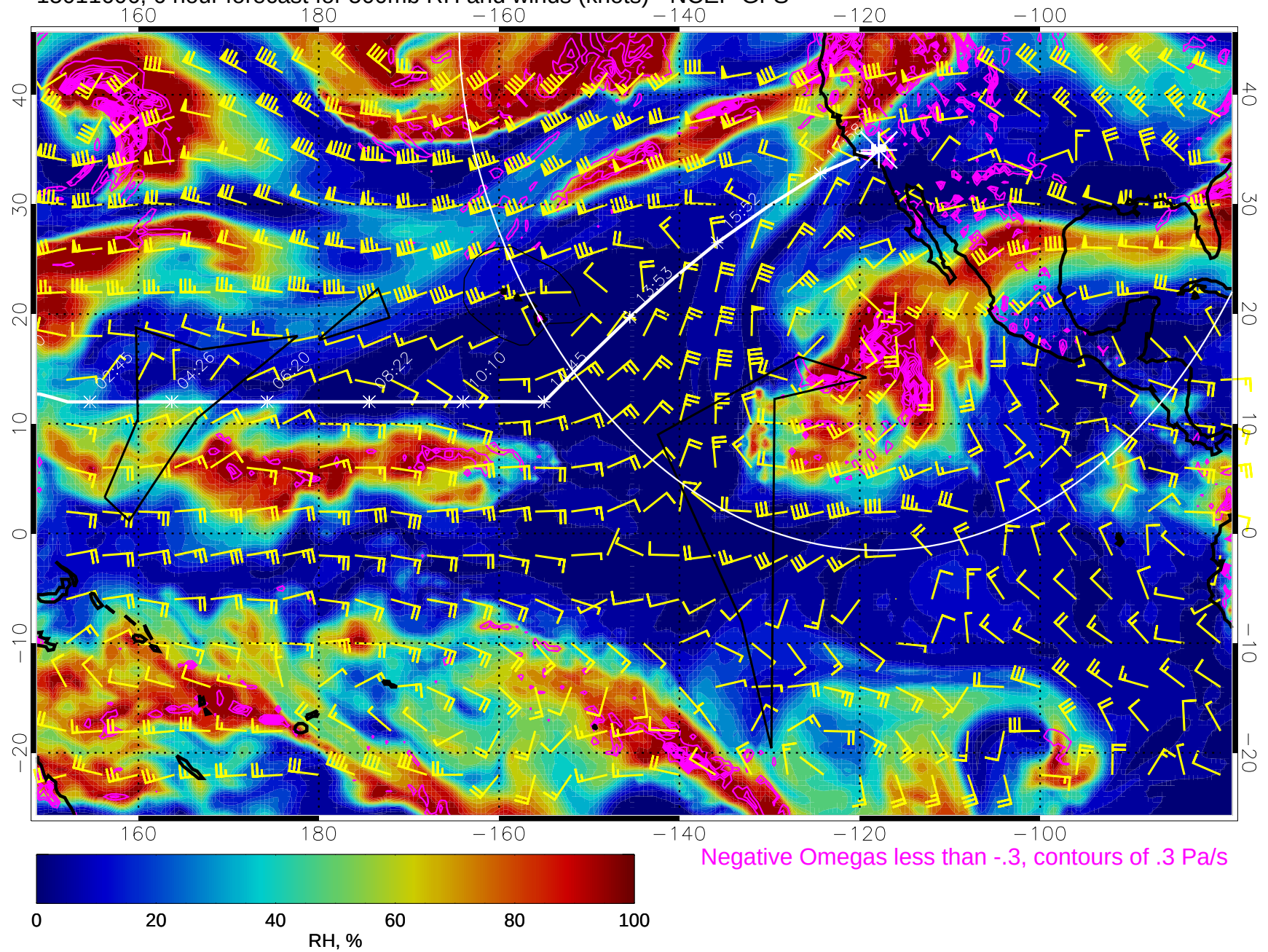
15011606, 6 hour forecast for 500mb RH and winds (knots) - NCEP GFS
