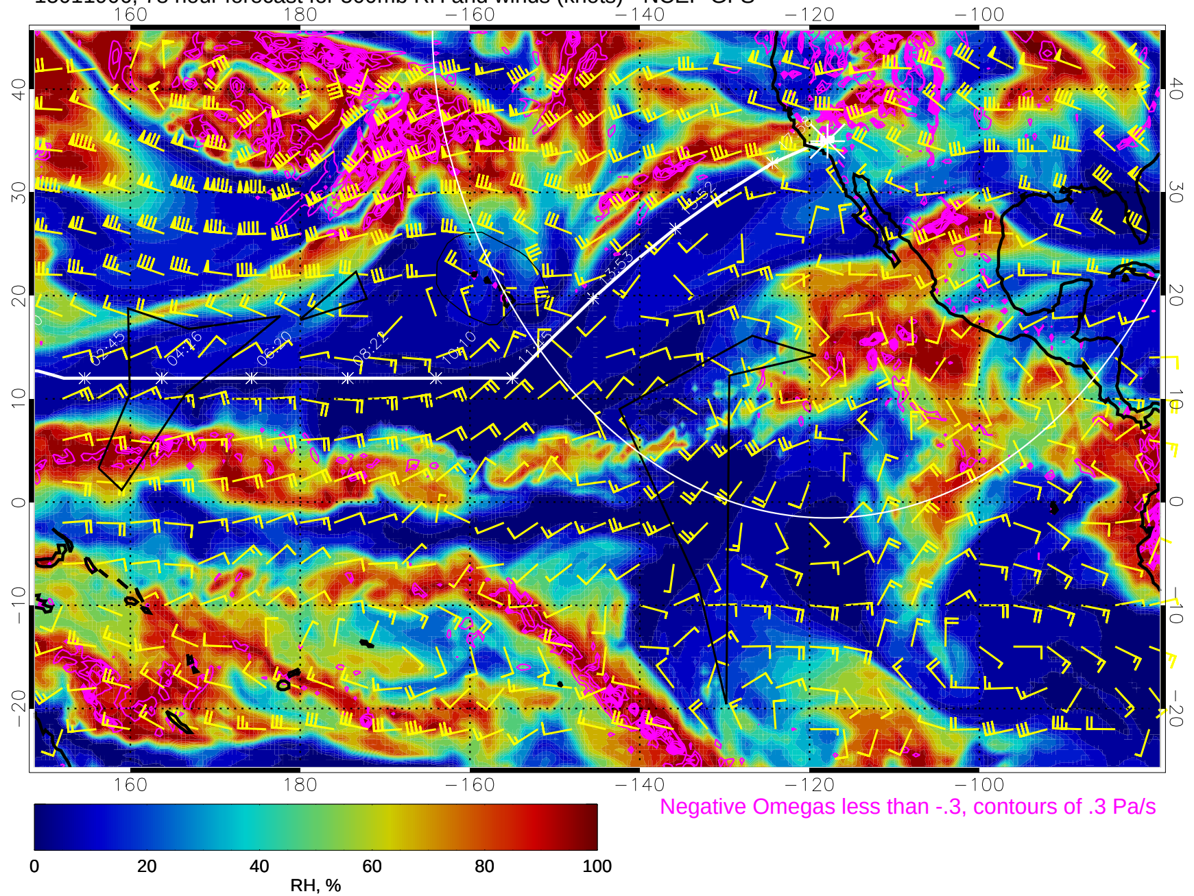
15011906, 78 hour forecast for 500mb RH and winds (knots) - NCEP GFS
