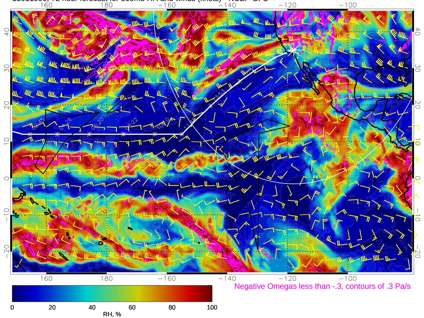
15011900, 72 hour forecast for 500mb RH and winds (knots) - NCEP GFS
