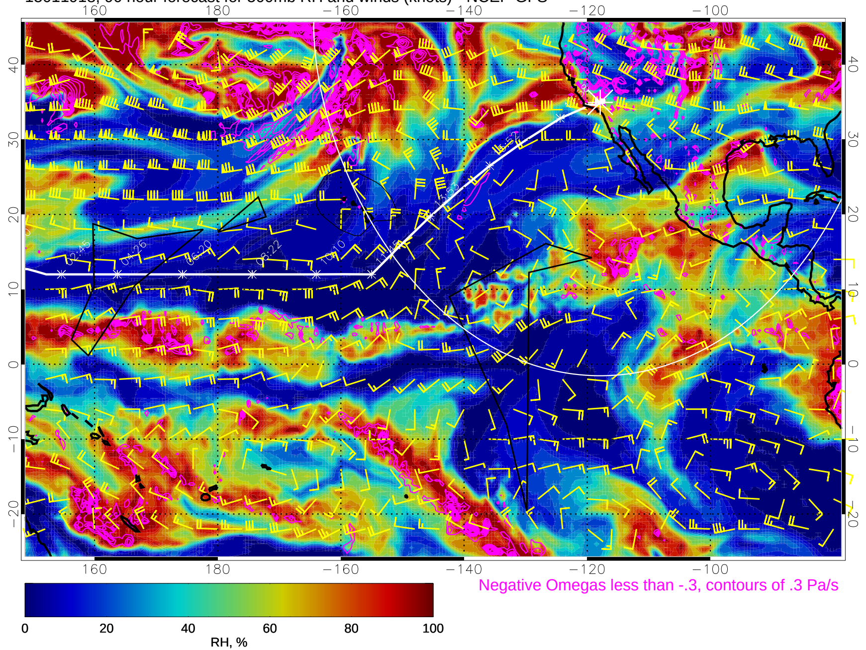
15011918, 90 hour forecast for 500mb RH and winds (knots) - NCEP GFS
