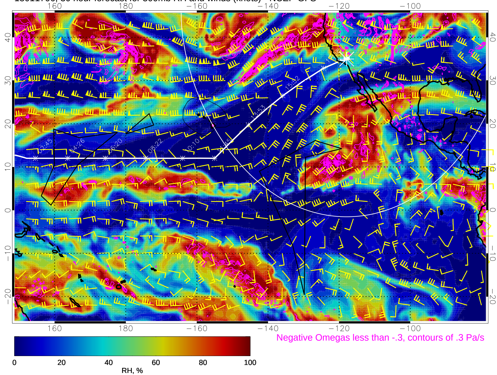
15011706, 30 hour forecast for 500mb RH and winds (knots) - NCEP GFS
