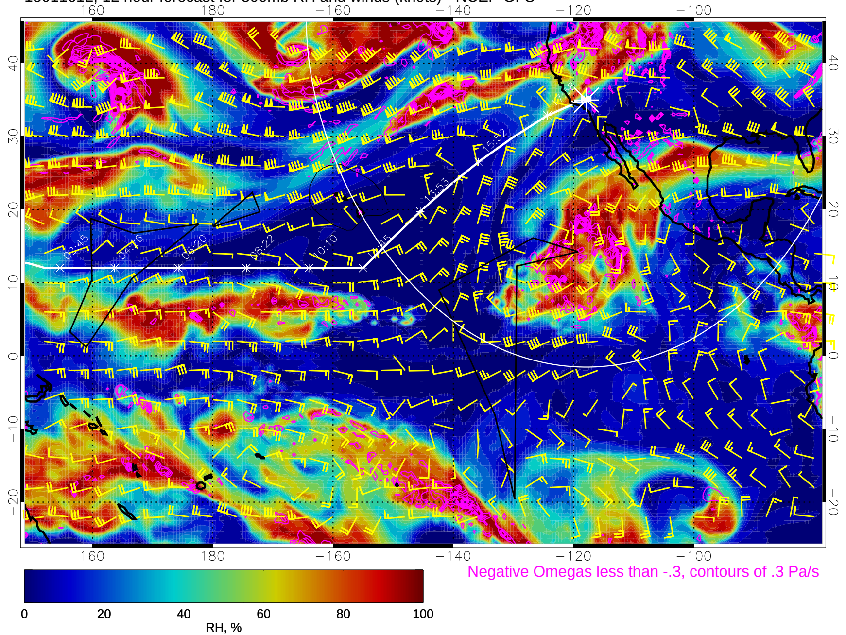
15011612, 12 hour forecast for 500mb RH and winds (knots) - NCEP GFS
