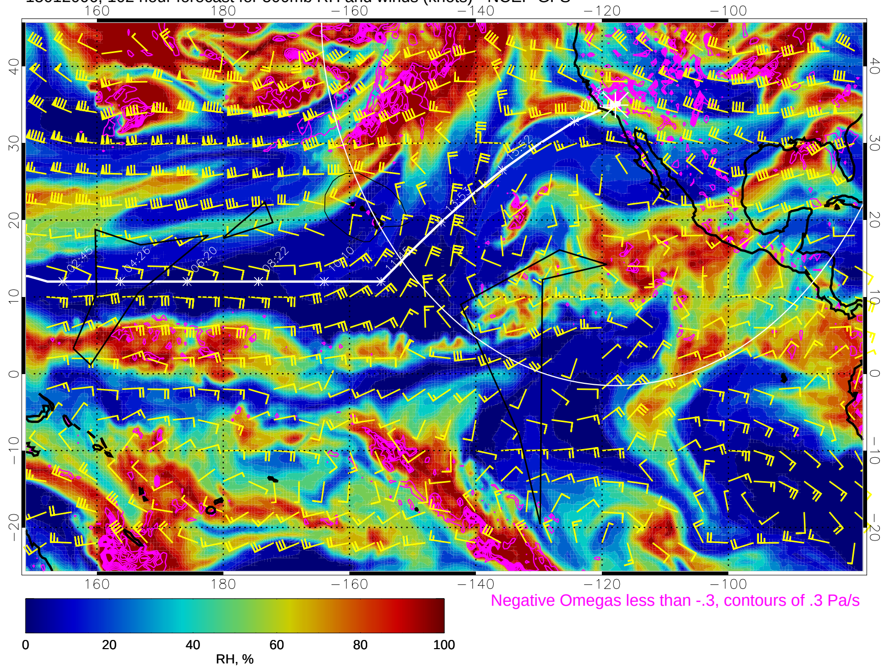
15012006, 102 hour forecast for 500mb RH and winds (knots) - NCEP GFS
