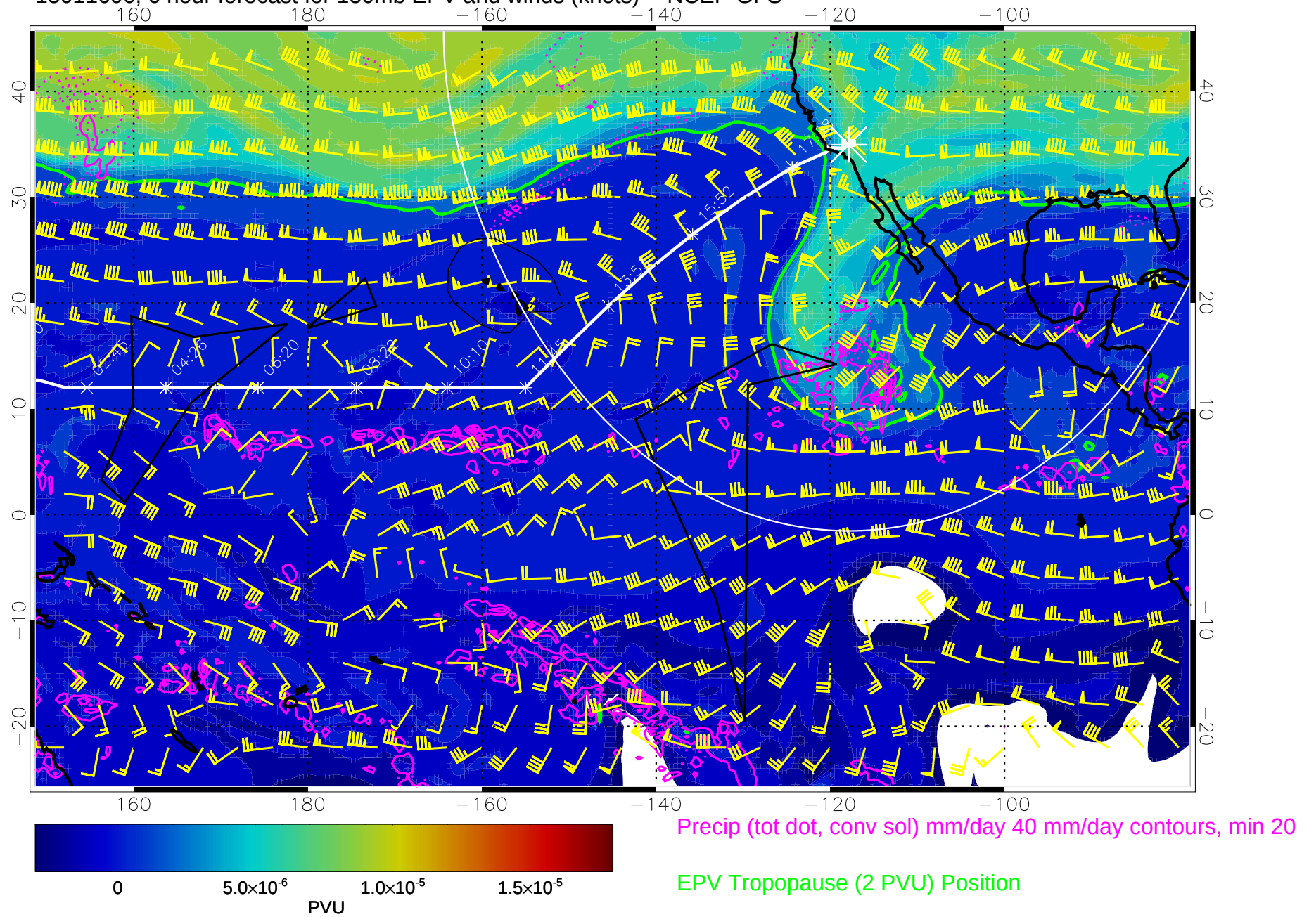
15011606, 6 hour forecast for 150mb EPV and winds (knots) -- NCEP GFS
