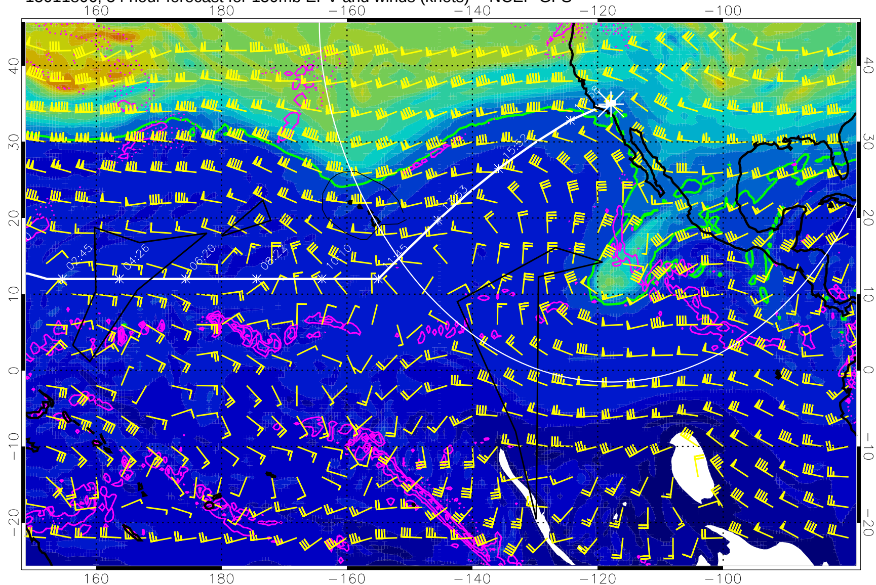
15011806, 54 hour forecast for 150mb EPV and winds (knots) -- NCEP GFS
