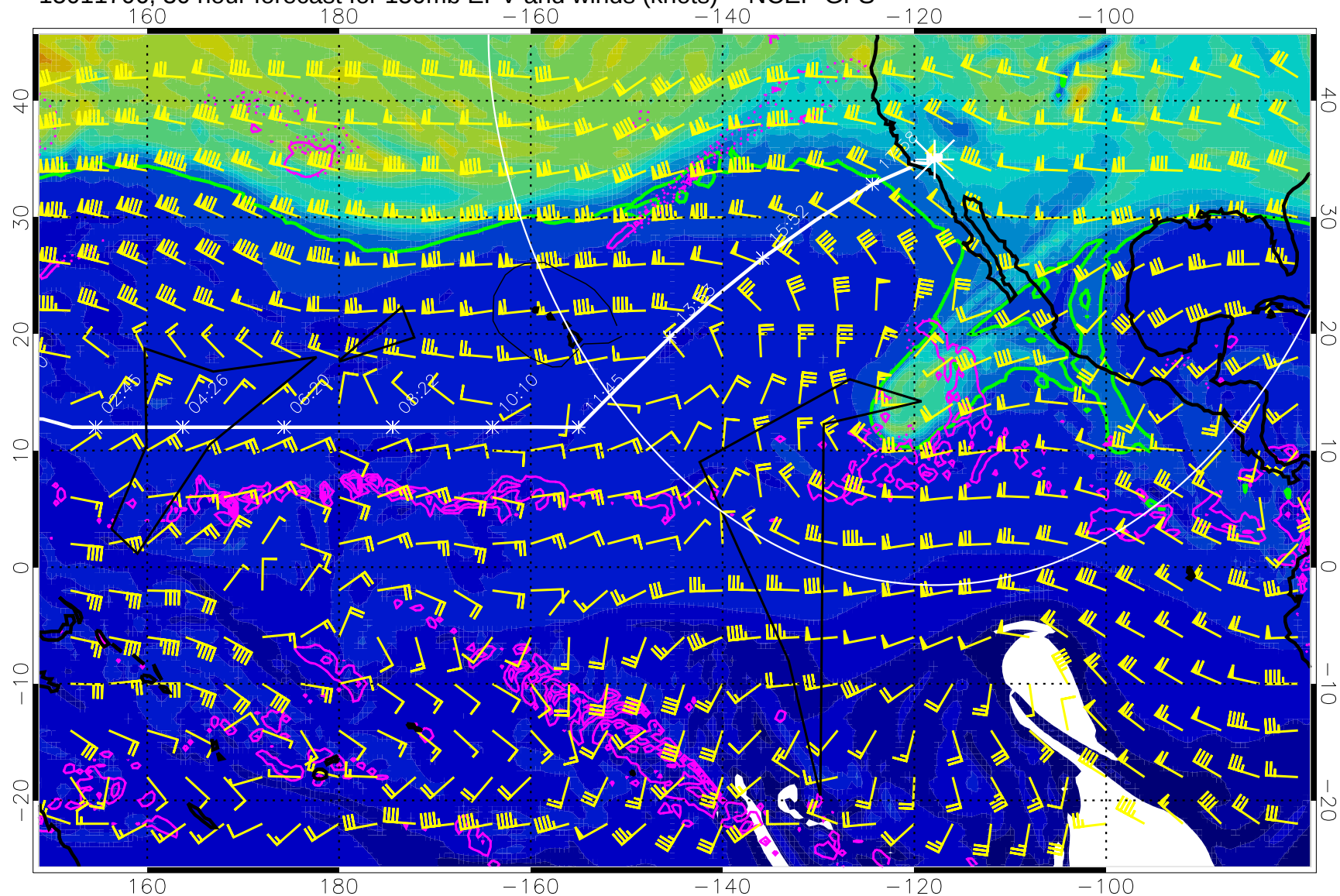
15011706, 30 hour forecast for 150mb EPV and winds (knots) -- NCEP GFS
