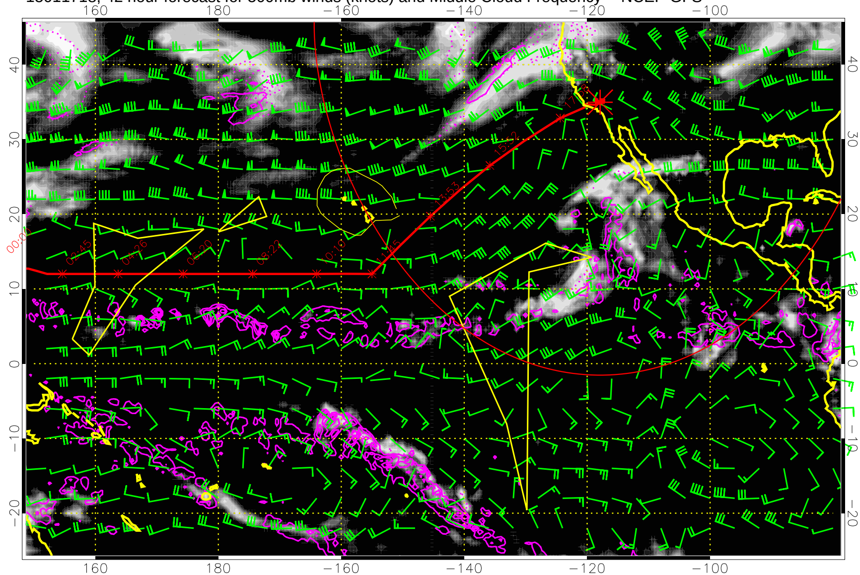
15011718, 42 hour forecast for 500mb winds (knots) and Middle Cloud Frequency -- NCEP GFS
