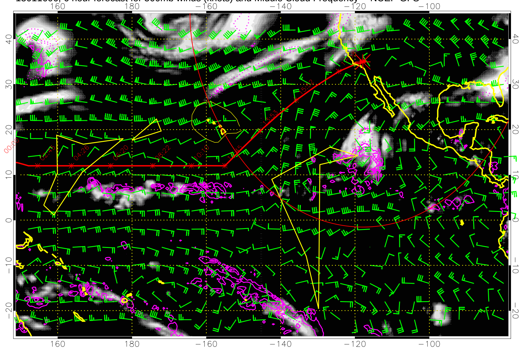
15011606, 6 hour forecast for 500mb winds (knots) and Middle Cloud Frequency -- NCEP GFS
