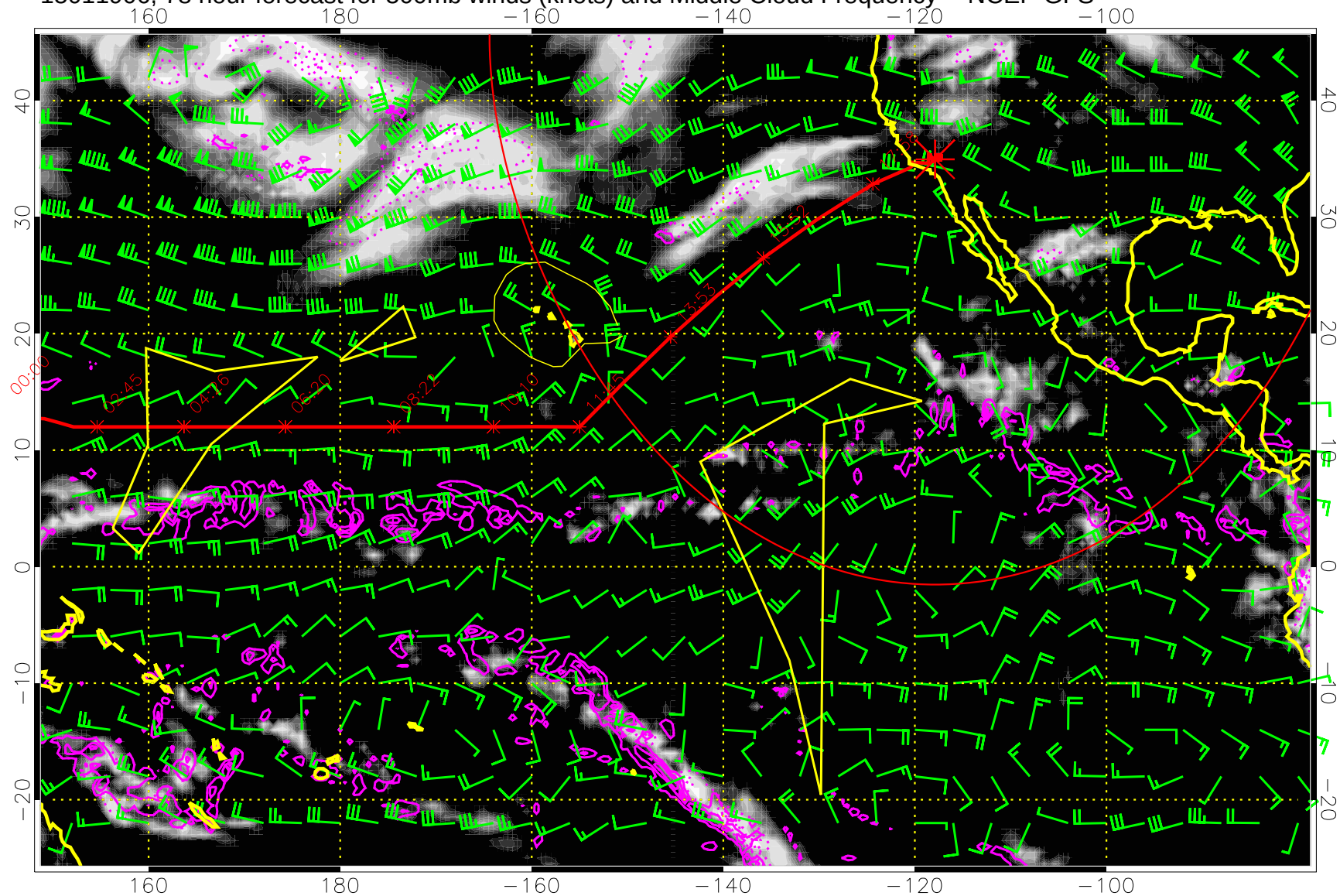
15011906, 78 hour forecast for 500mb winds (knots) and Middle Cloud Frequency -- NCEP GFS
