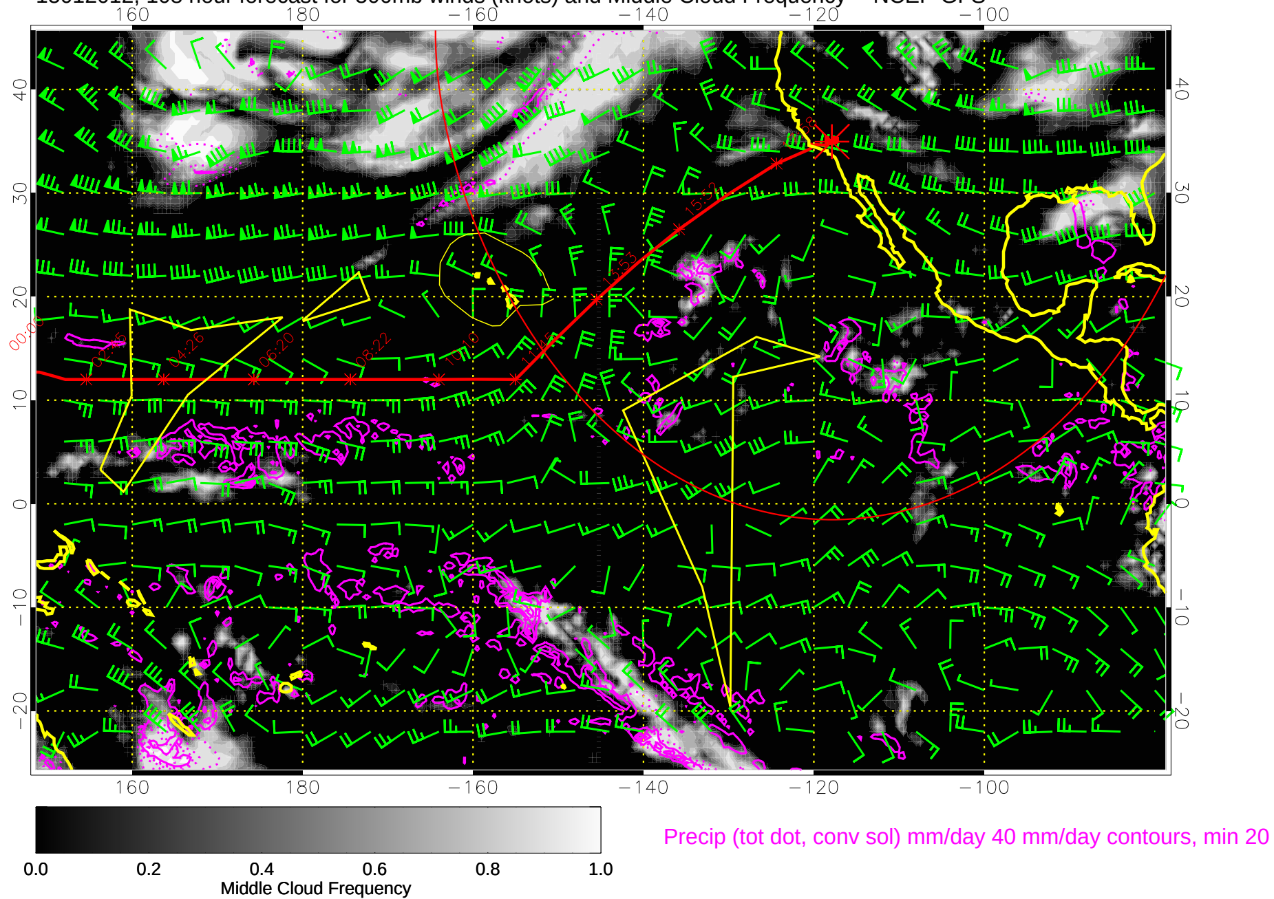
15012012, 108 hour forecast for 500mb winds (knots) and Middle Cloud Frequency -- NCEP GFS
