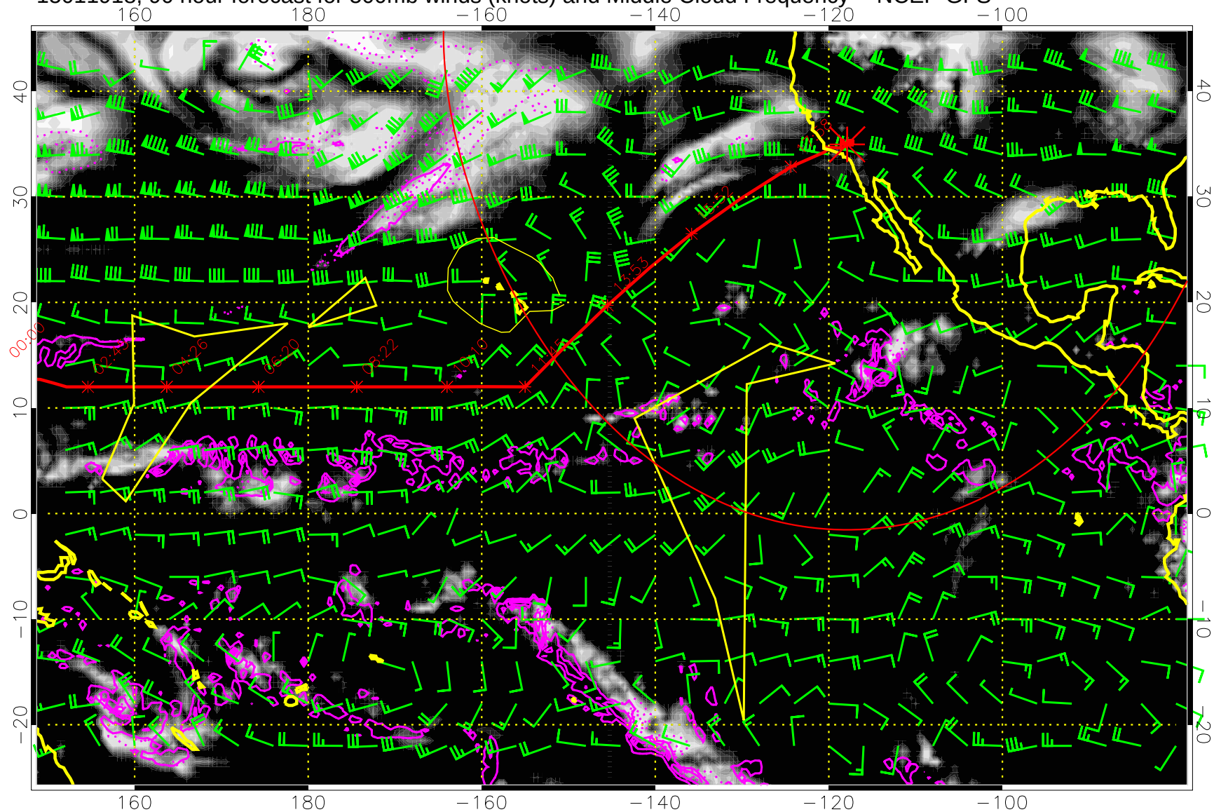
15011918, 90 hour forecast for 500mb winds (knots) and Middle Cloud Frequency -- NCEP GFS
