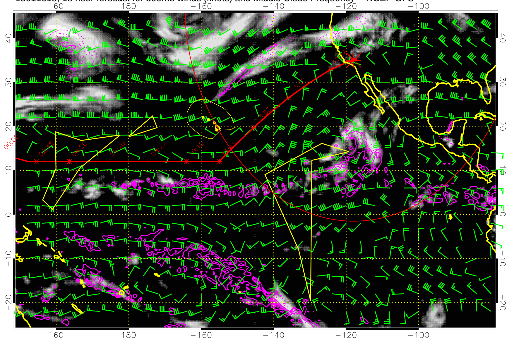
15011618, 18 hour forecast for 500mb winds (knots) and Middle Cloud Frequency -- NCEP GFS
