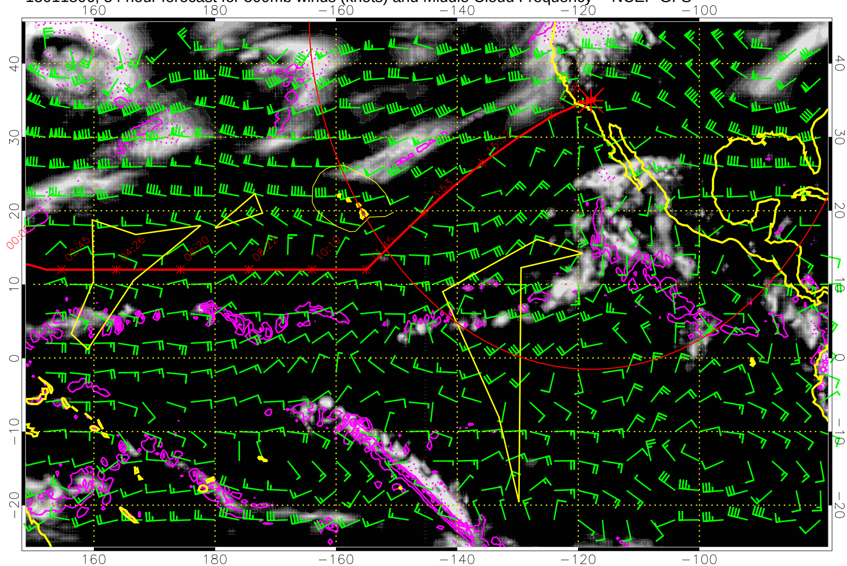
15011806, 54 hour forecast for 500mb winds (knots) and Middle Cloud Frequency -- NCEP GFS
