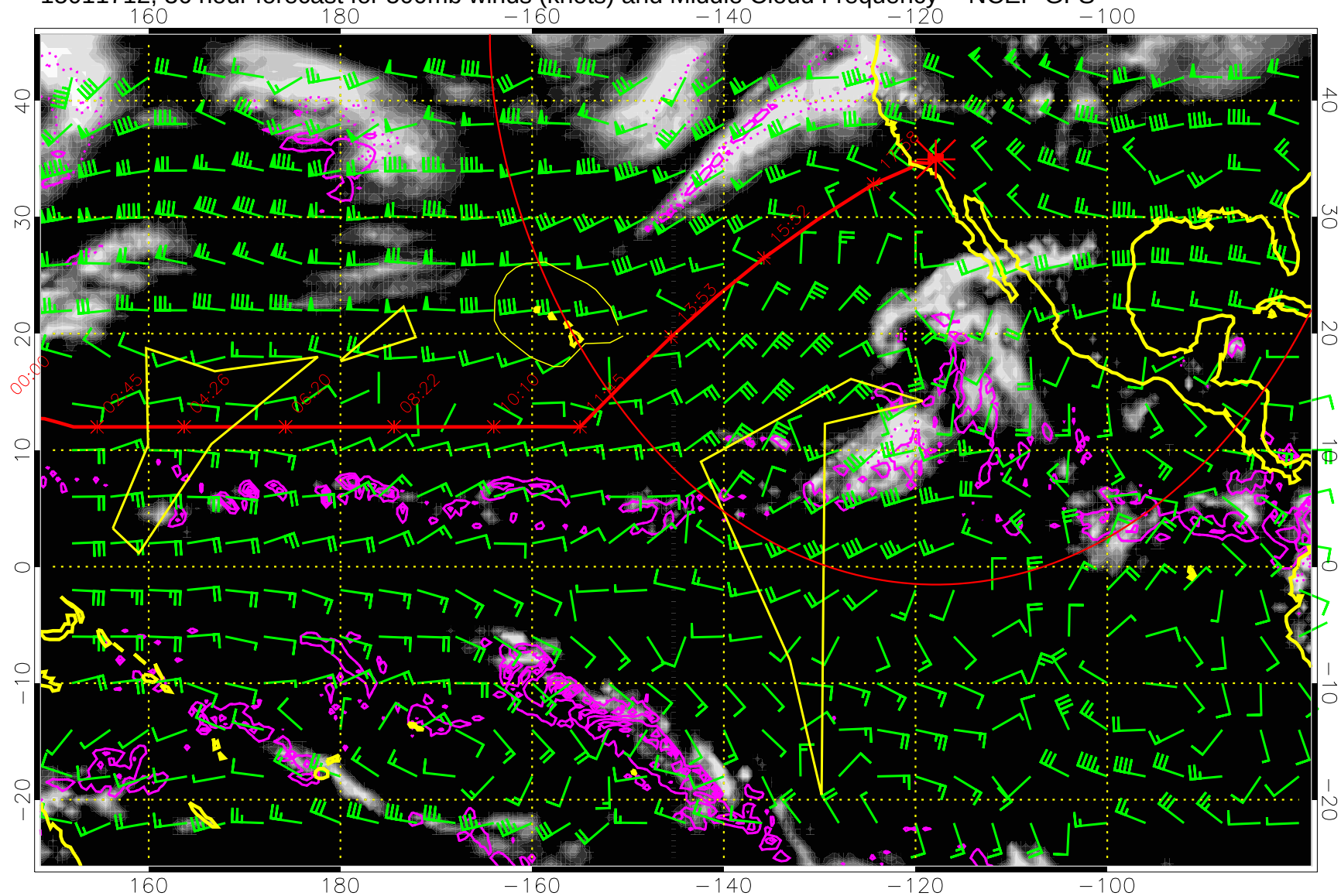
15011712, 36 hour forecast for 500mb winds (knots) and Middle Cloud Frequency -- NCEP GFS
