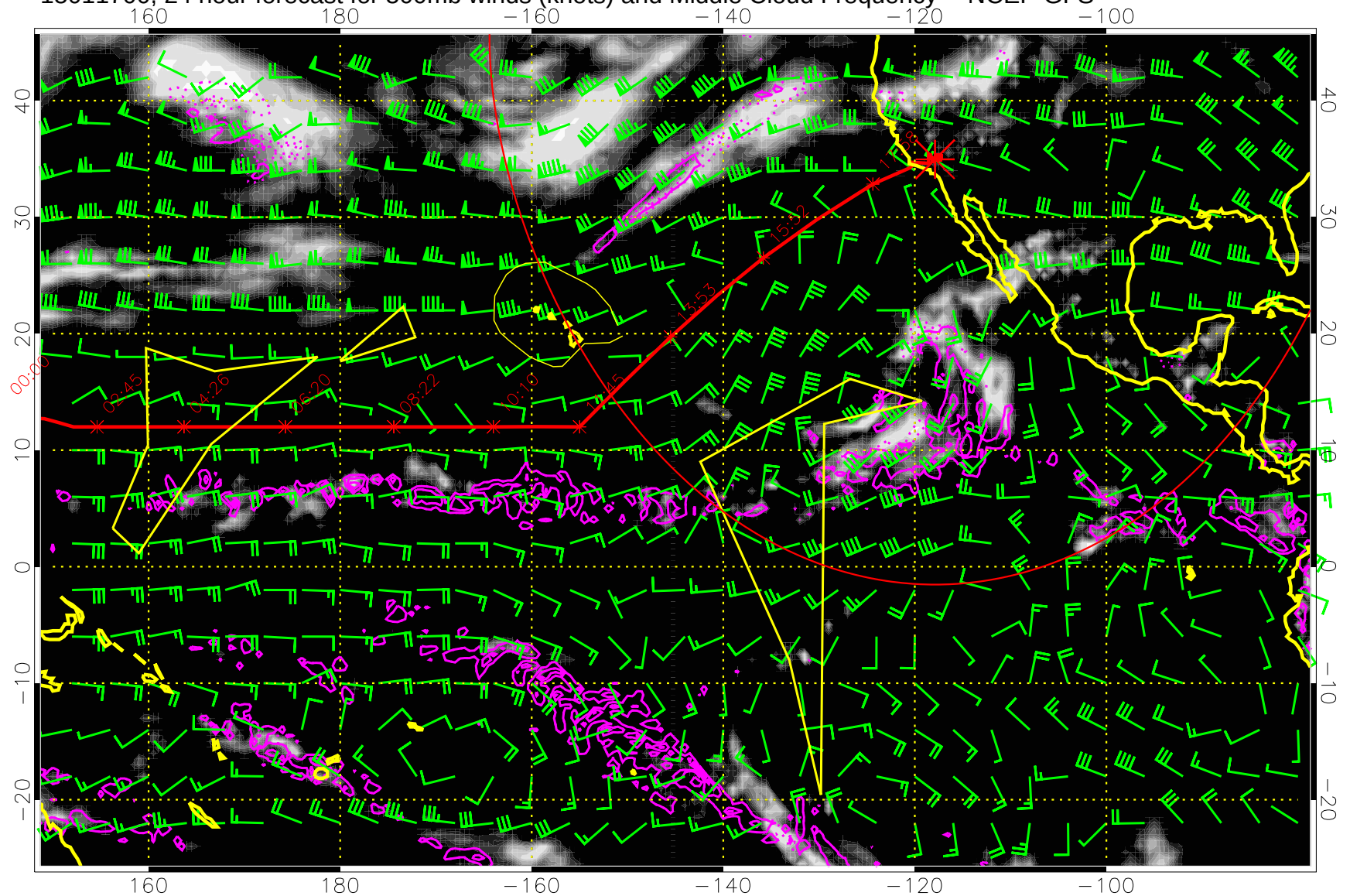
15011700, 24 hour forecast for 500mb winds (knots) and Middle Cloud Frequency -- NCEP GFS
