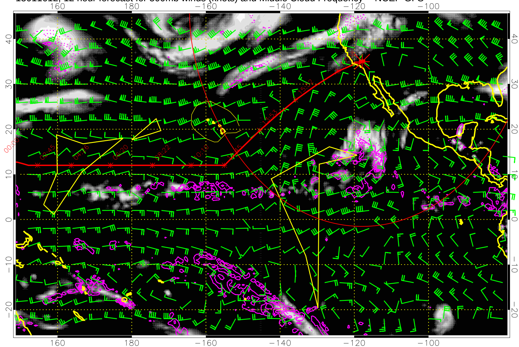
15011612, 12 hour forecast for 500mb winds (knots) and Middle Cloud Frequency -- NCEP GFS
