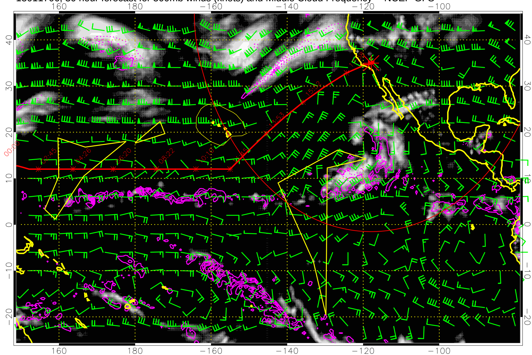
15011706, 30 hour forecast for 500mb winds (knots) and Middle Cloud Frequency -- NCEP GFS
