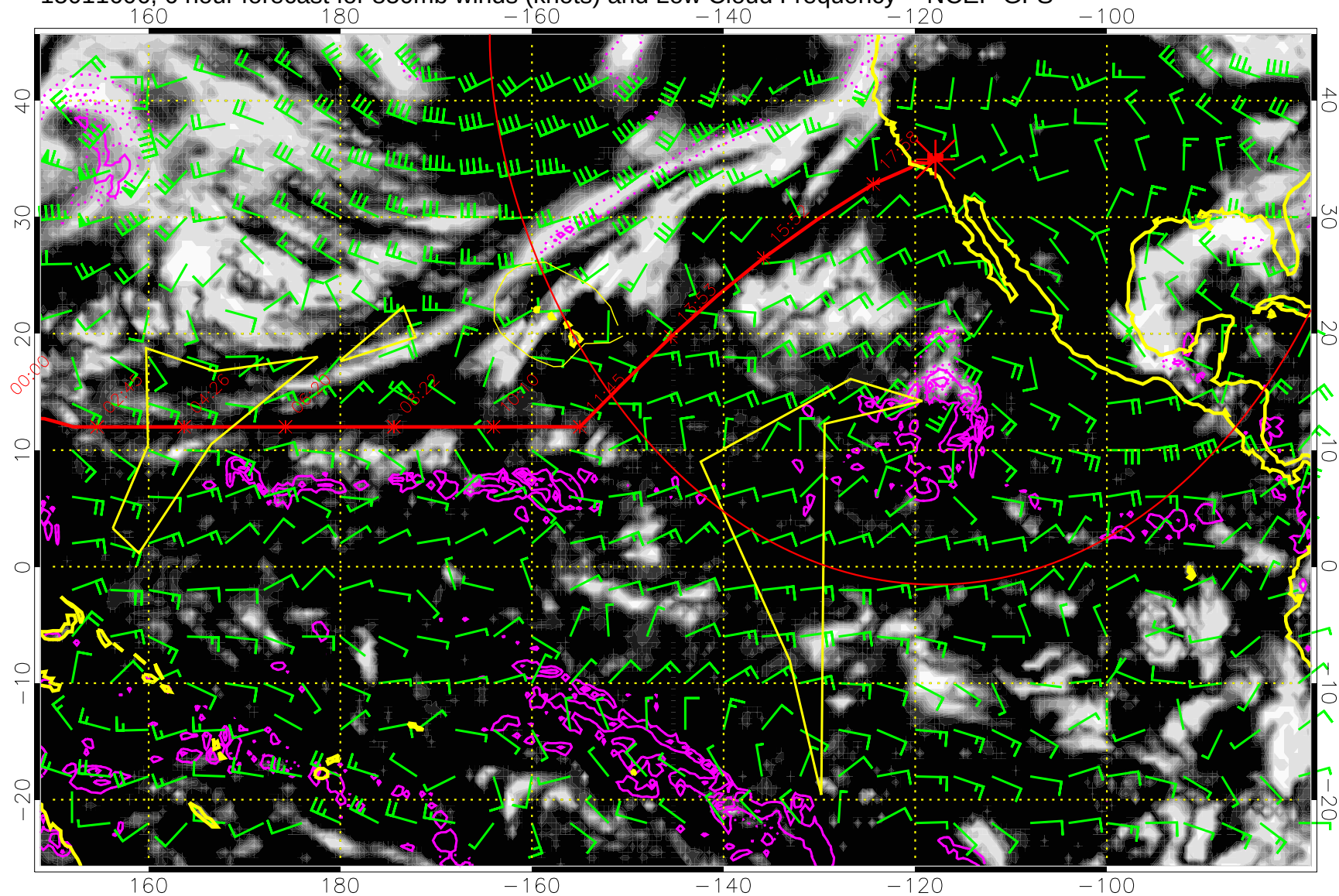
15011606, 6 hour forecast for 850mb winds (knots) and Low Cloud Frequency -- NCEP GFS
