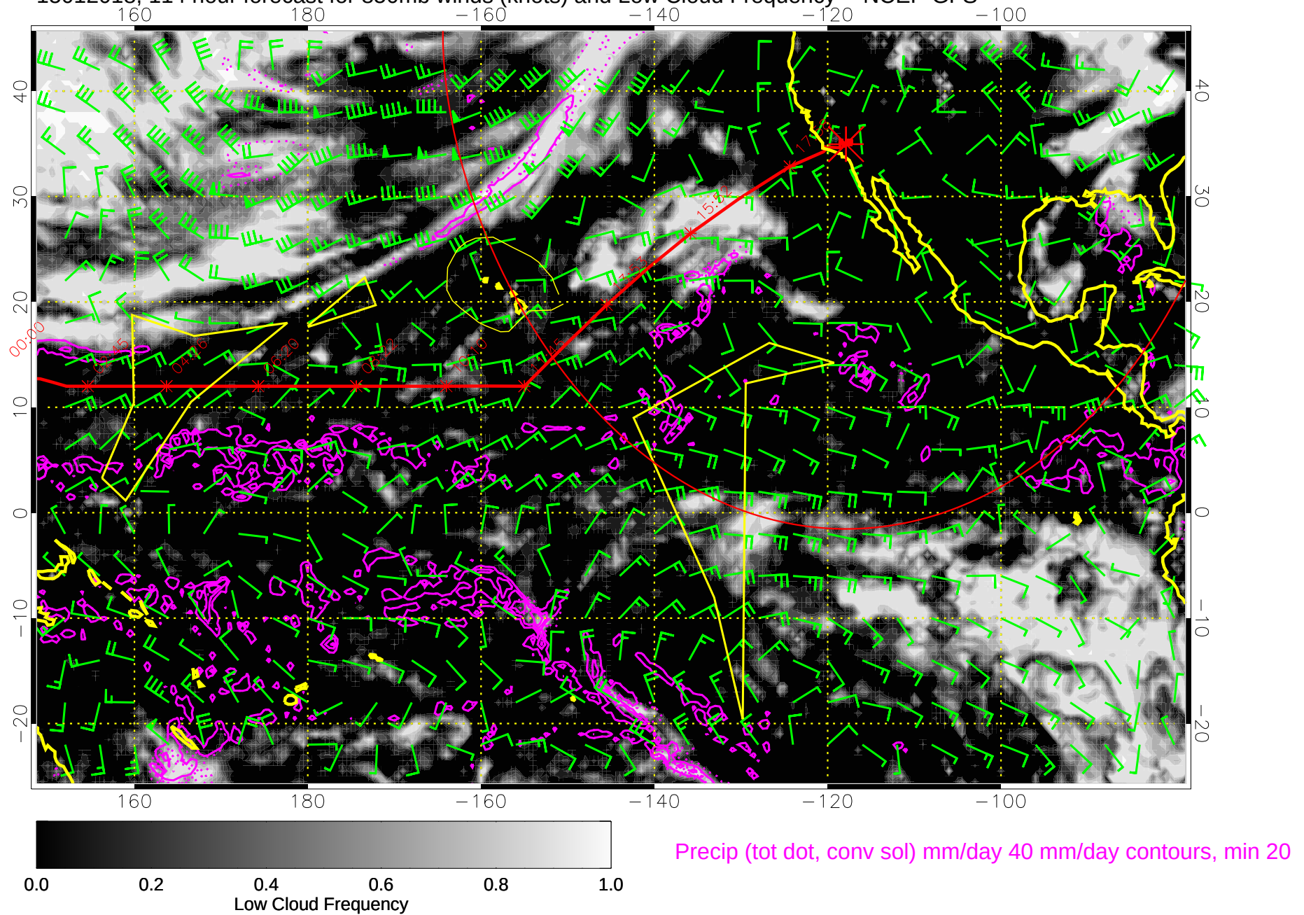
15012018, 114 hour forecast for 850mb winds (knots) and Low Cloud Frequency -- NCEP GFS
