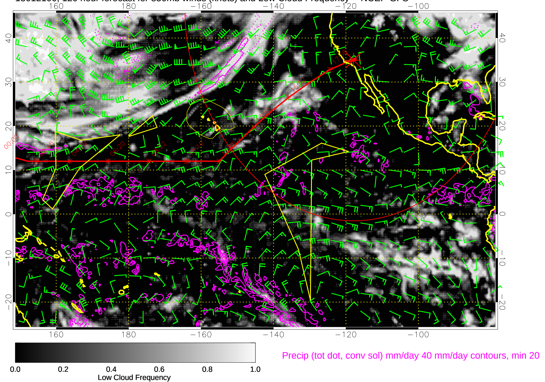
15012100, 120 hour forecast for 850mb winds (knots) and Low Cloud Frequency -- NCEP GFS
