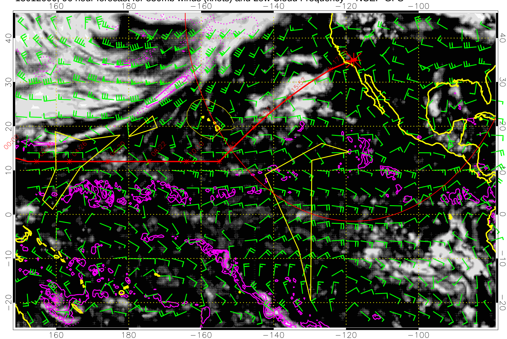
15012000, 96 hour forecast for 850mb winds (knots) and Low Cloud Frequency -- NCEP GFS
