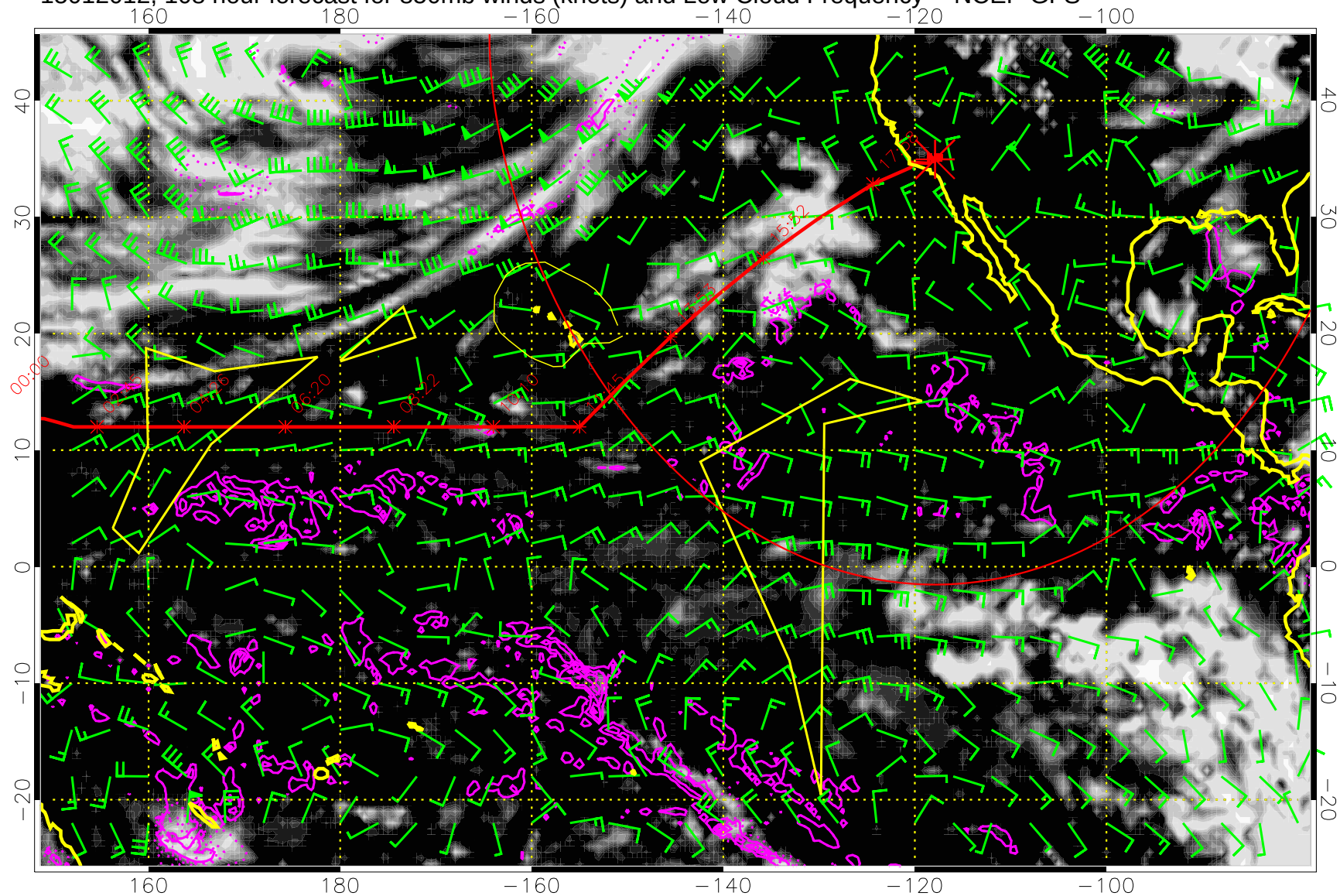
15012012, 108 hour forecast for 850mb winds (knots) and Low Cloud Frequency -- NCEP GFS
