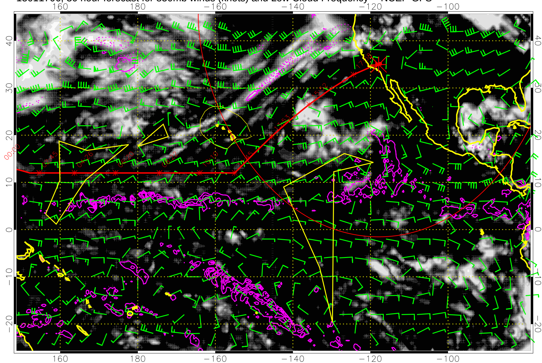
15011706, 30 hour forecast for 850mb winds (knots) and Low Cloud Frequency -- NCEP GFS
