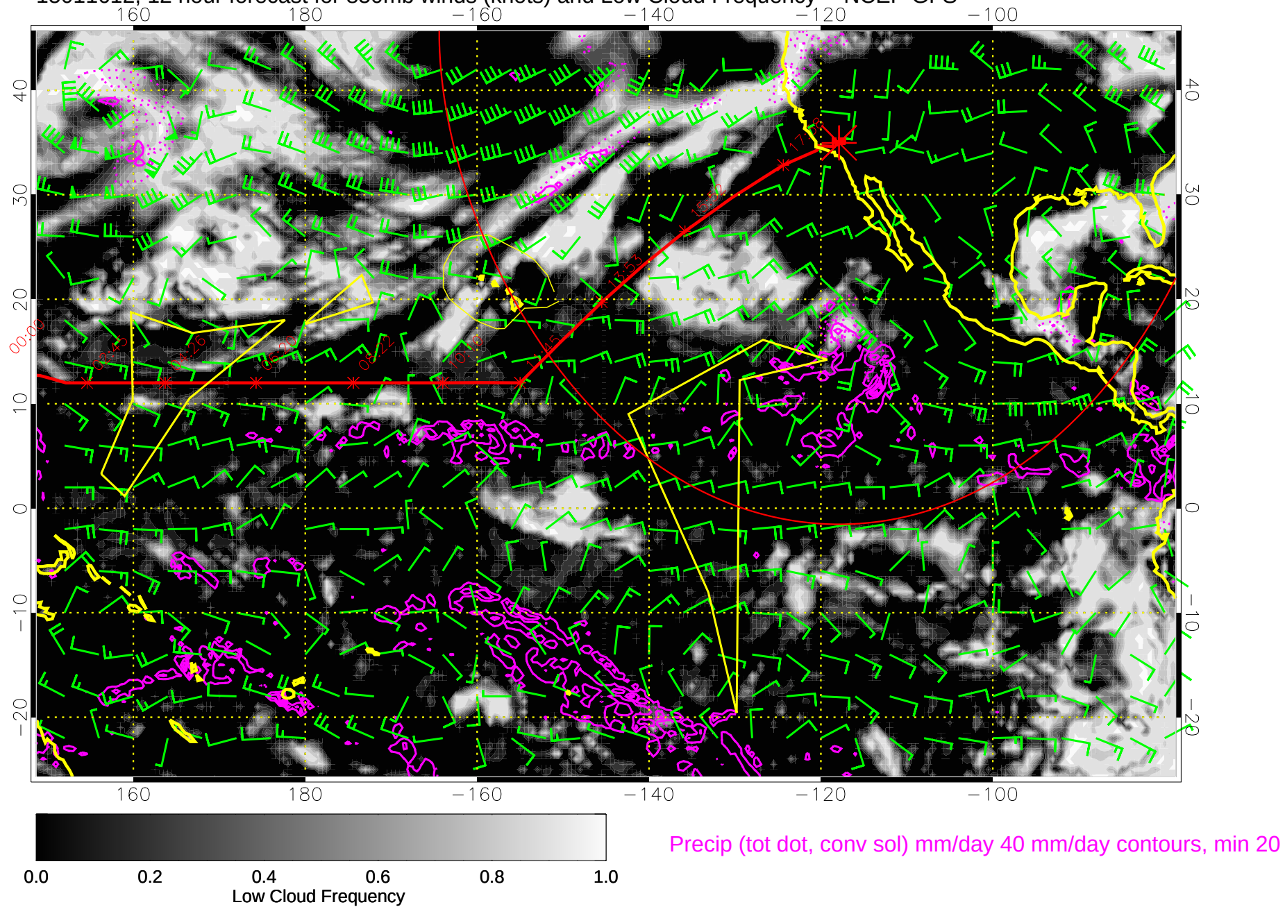
15011612, 12 hour forecast for 850mb winds (knots) and Low Cloud Frequency -- NCEP GFS
