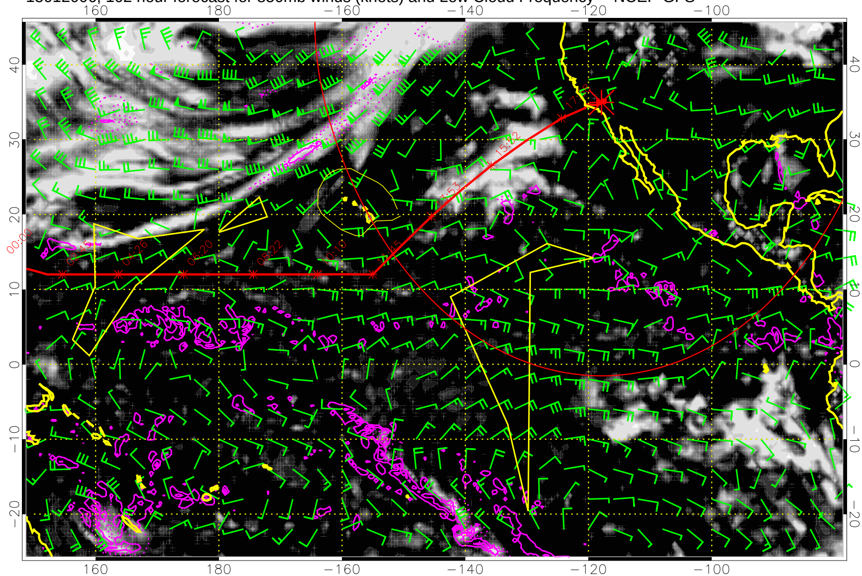
15012006, 102 hour forecast for 850mb winds (knots) and Low Cloud Frequency -- NCEP GFS
