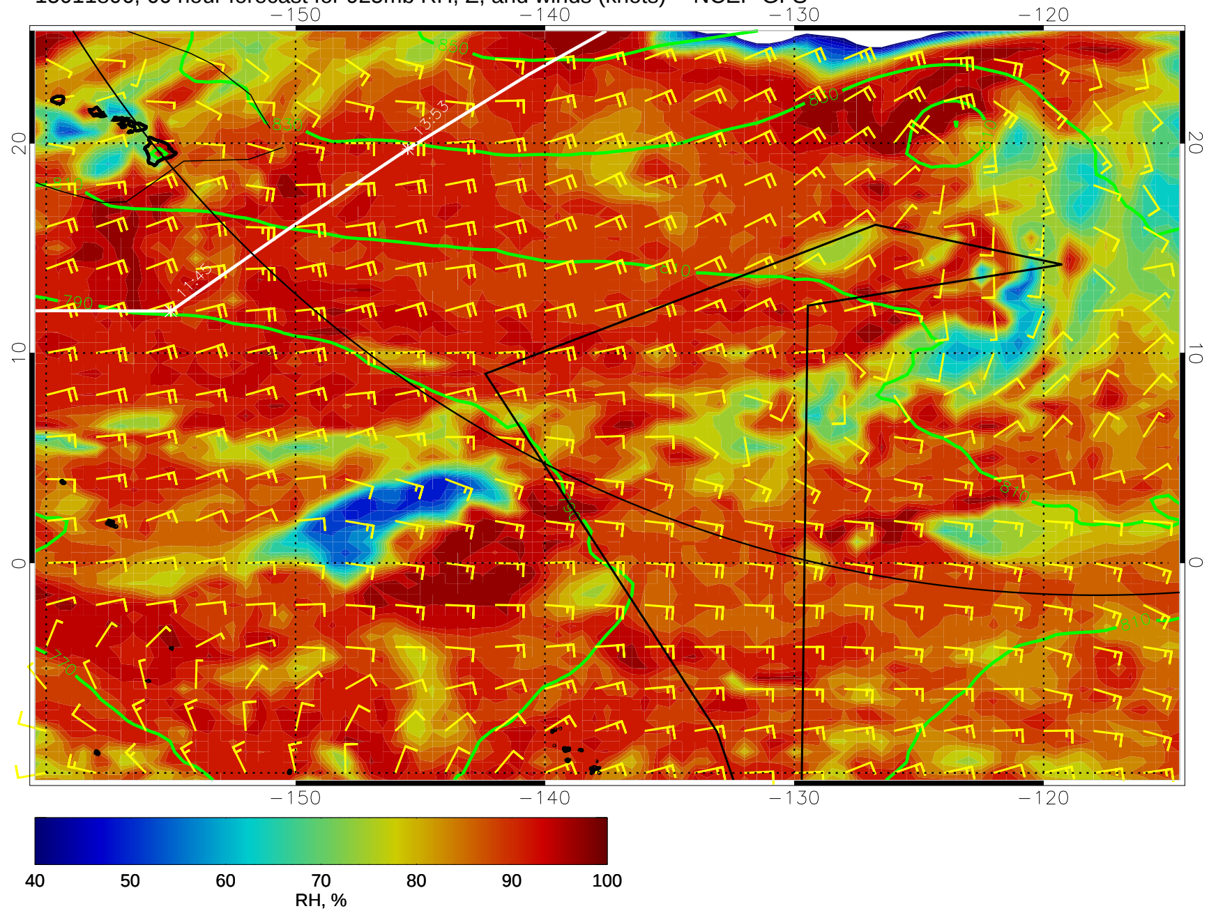
15011806, 66 hour forecast for 925mb RH, Z, and winds (knots) -- NCEP GFS
