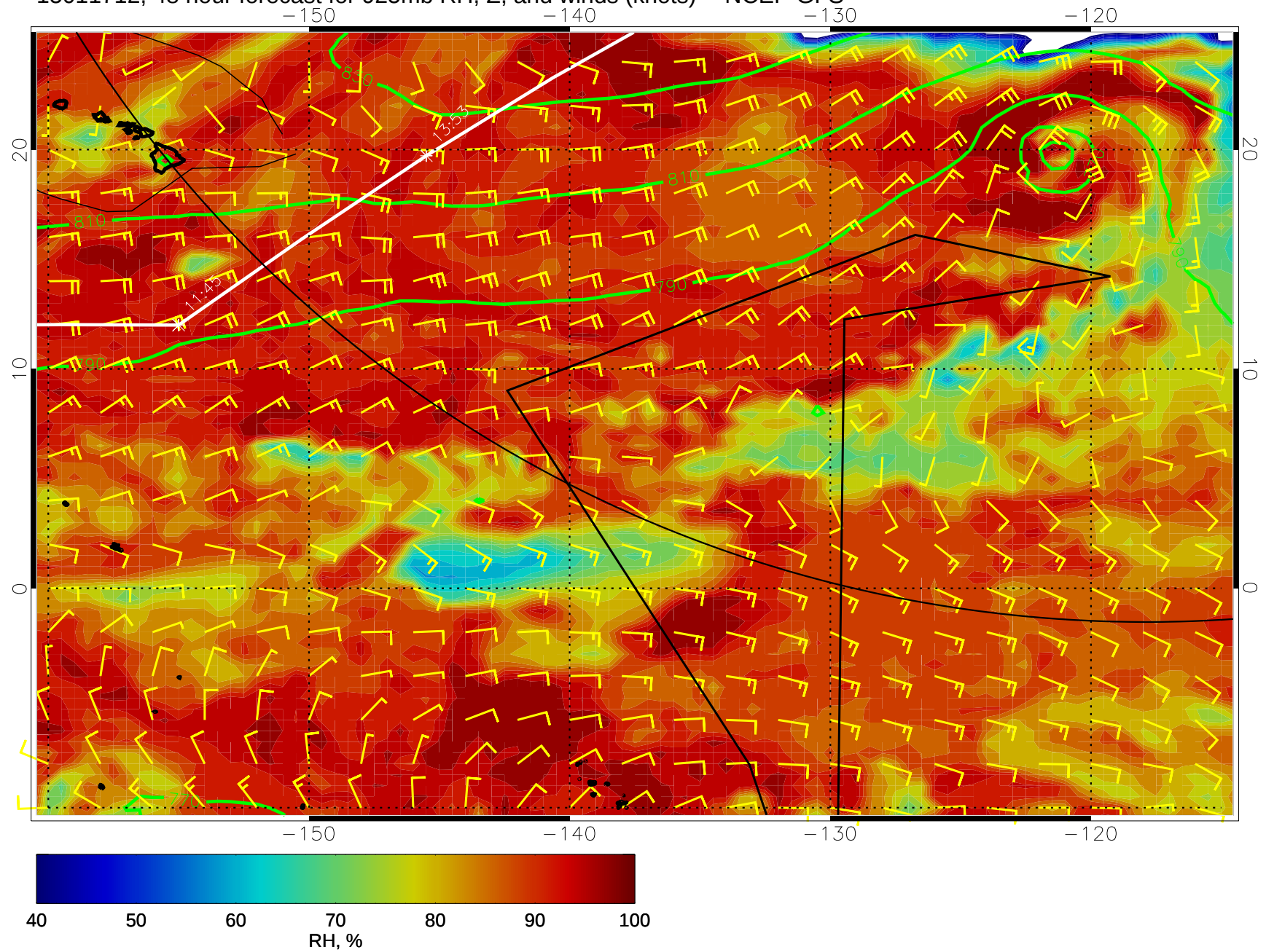
15011712, 48 hour forecast for 925mb RH, Z, and winds (knots) -- NCEP GFS
