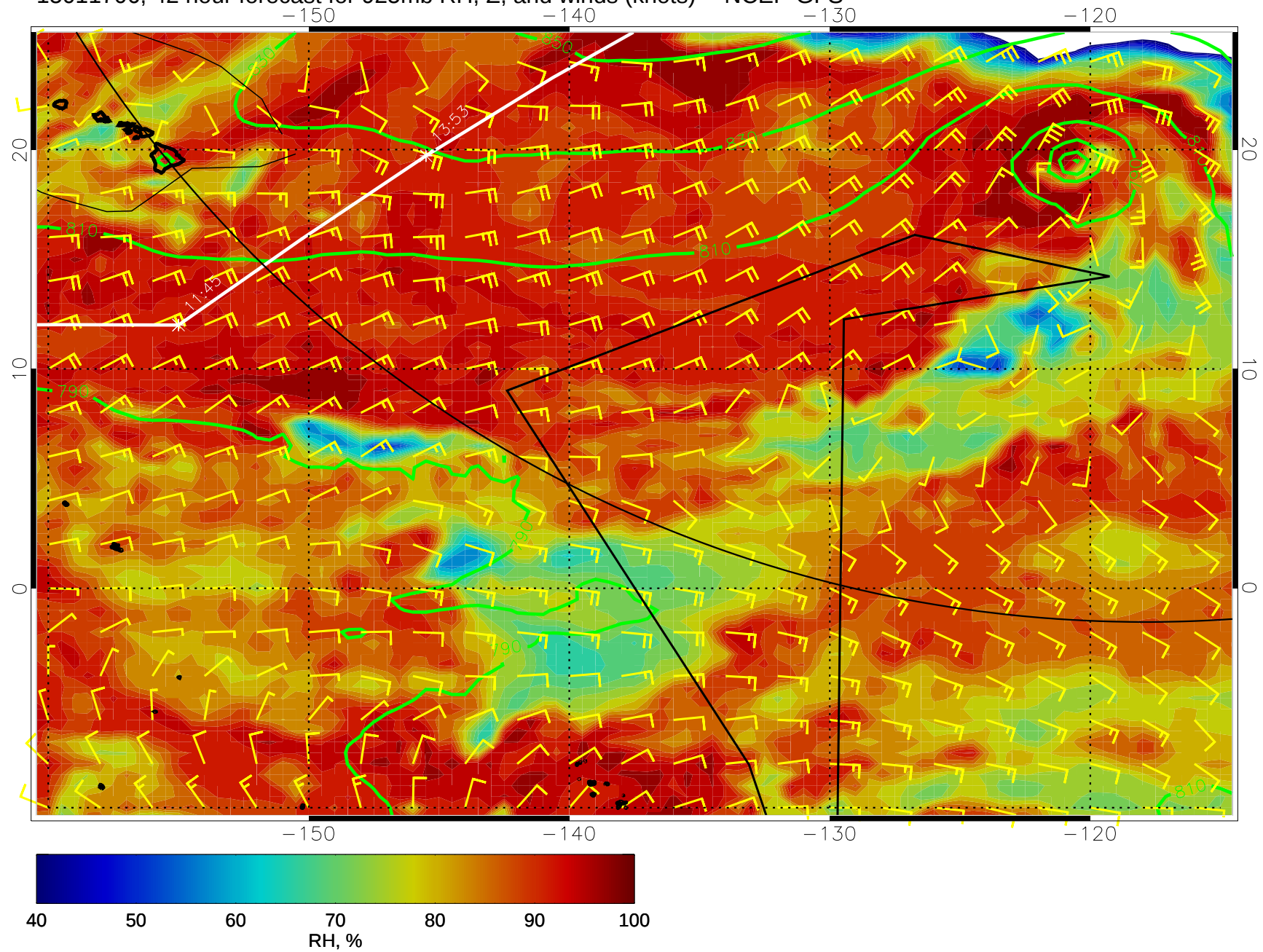
15011706, 42 hour forecast for 925mb RH, Z, and winds (knots) -- NCEP GFS
