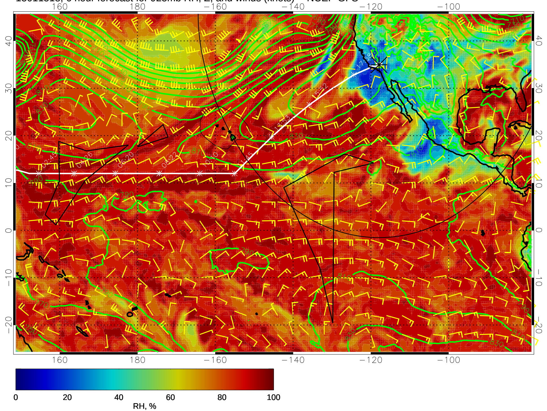
15011518, 6 hour forecast for 925mb RH, Z, and winds (knots) -- NCEP GFS
