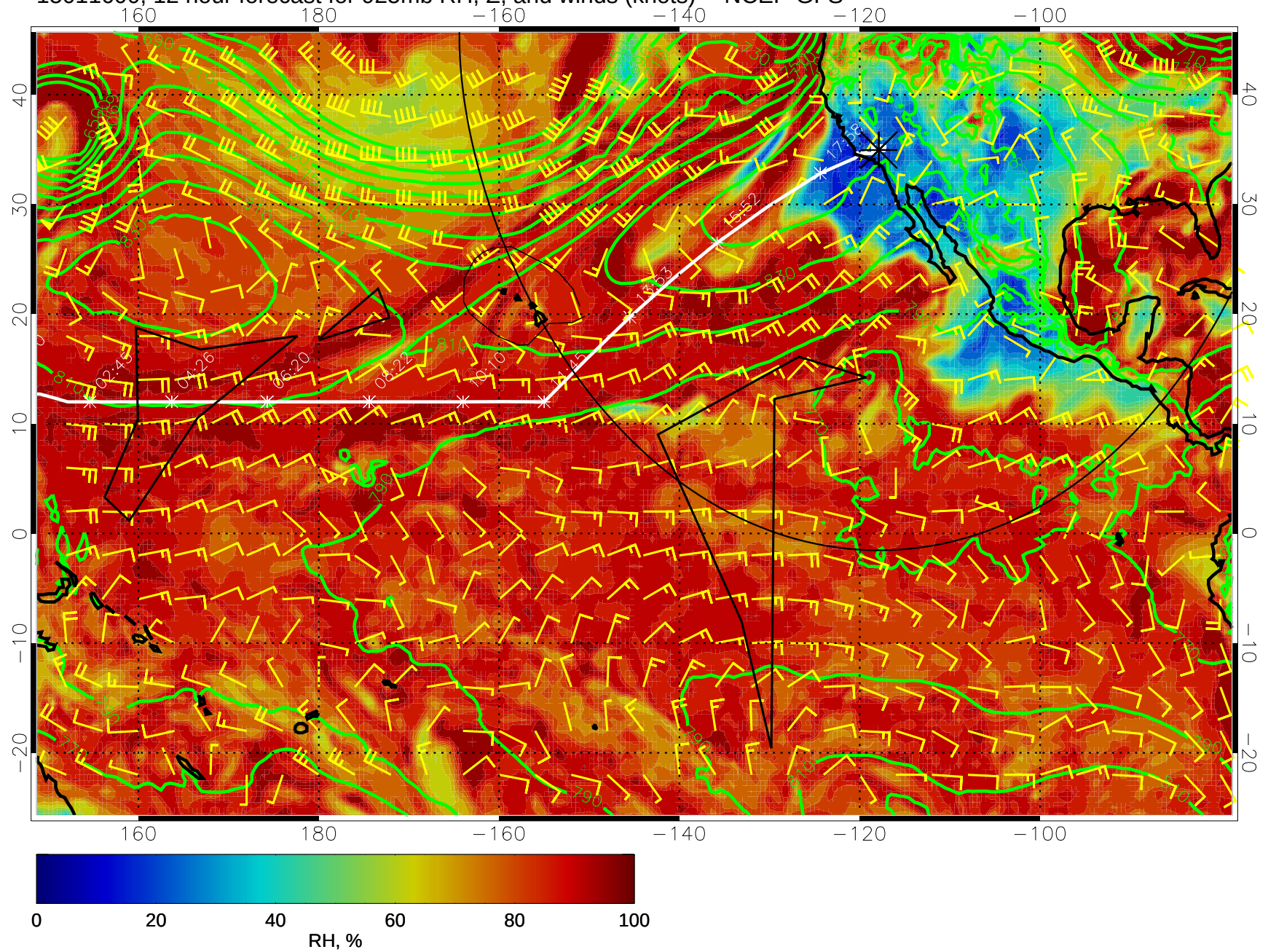
15011600, 12 hour forecast for 925mb RH, Z, and winds (knots) -- NCEP GFS
