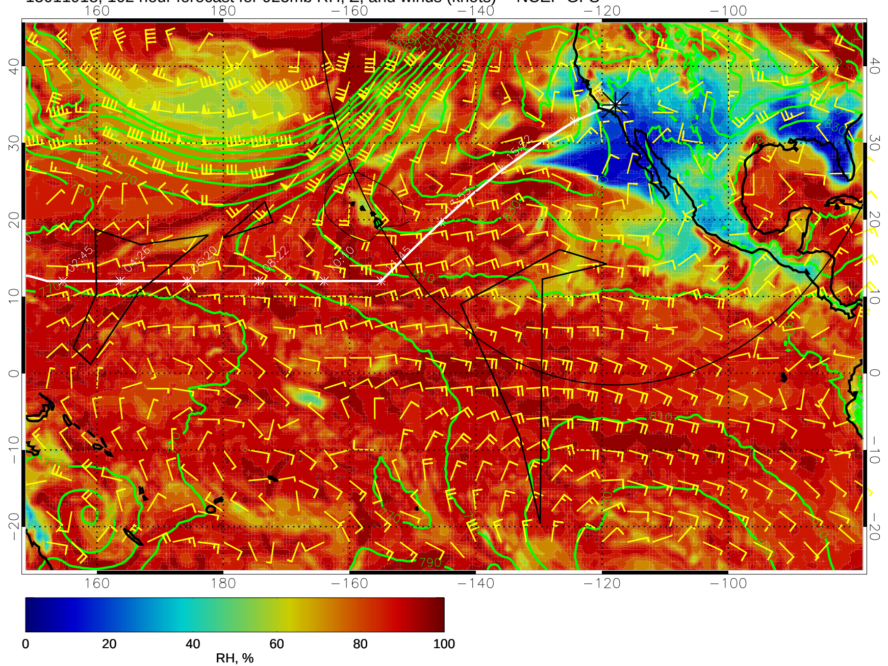
15011918, 102 hour forecast for 925mb RH, Z, and winds (knots) -- NCEP GFS
