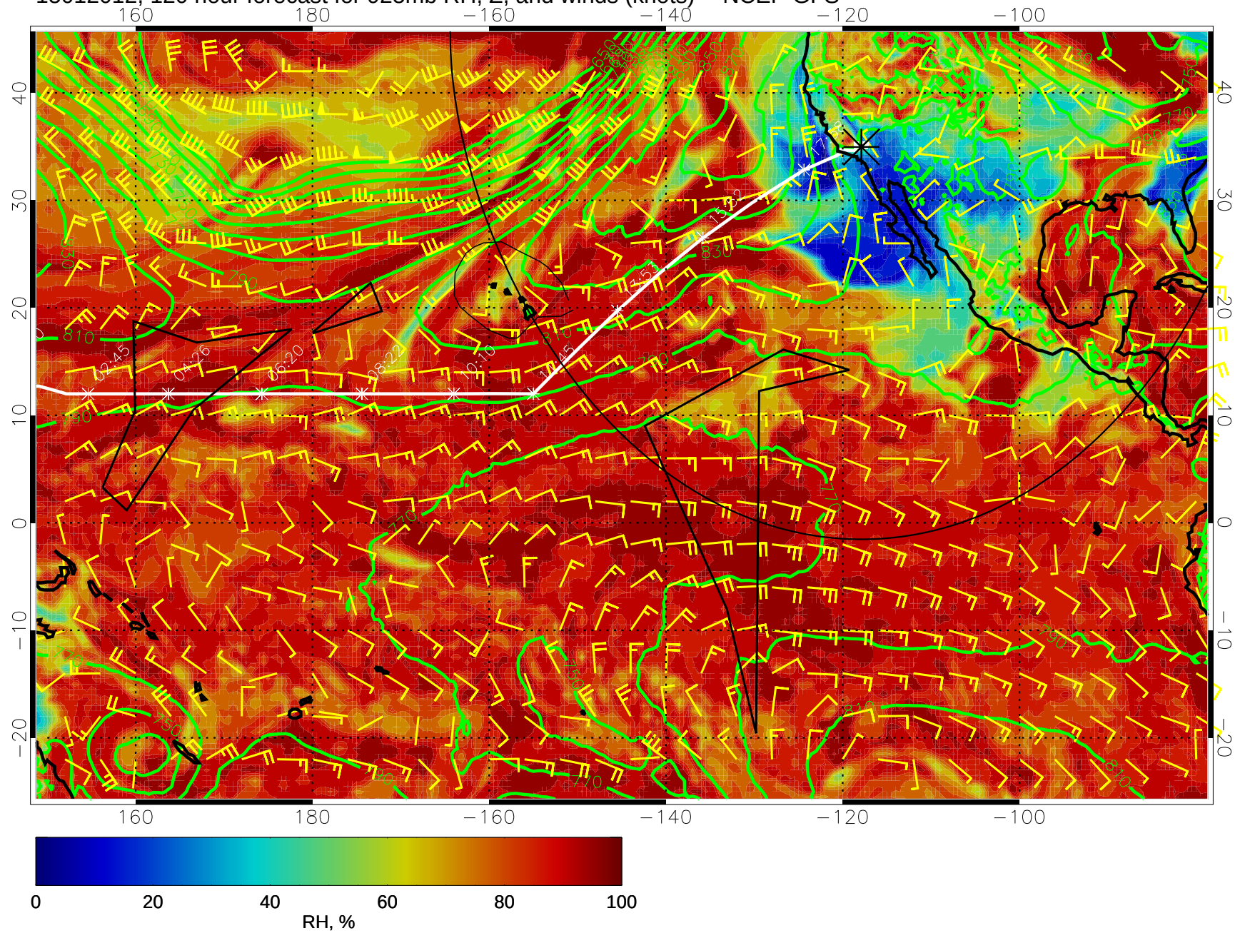
15012012, 120 hour forecast for 925mb RH, Z, and winds (knots) -- NCEP GFS
