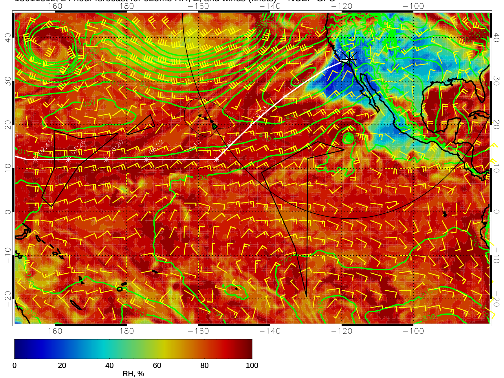
15011612, 24 hour forecast for 925mb RH, Z, and winds (knots) -- NCEP GFS
