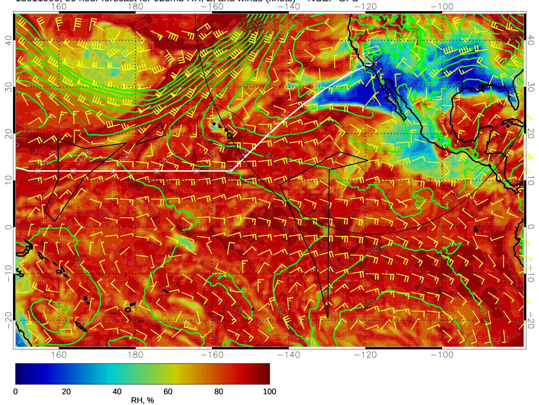
15011906, 90 hour forecast for 925mb RH, Z, and winds (knots) -- NCEP GFS
