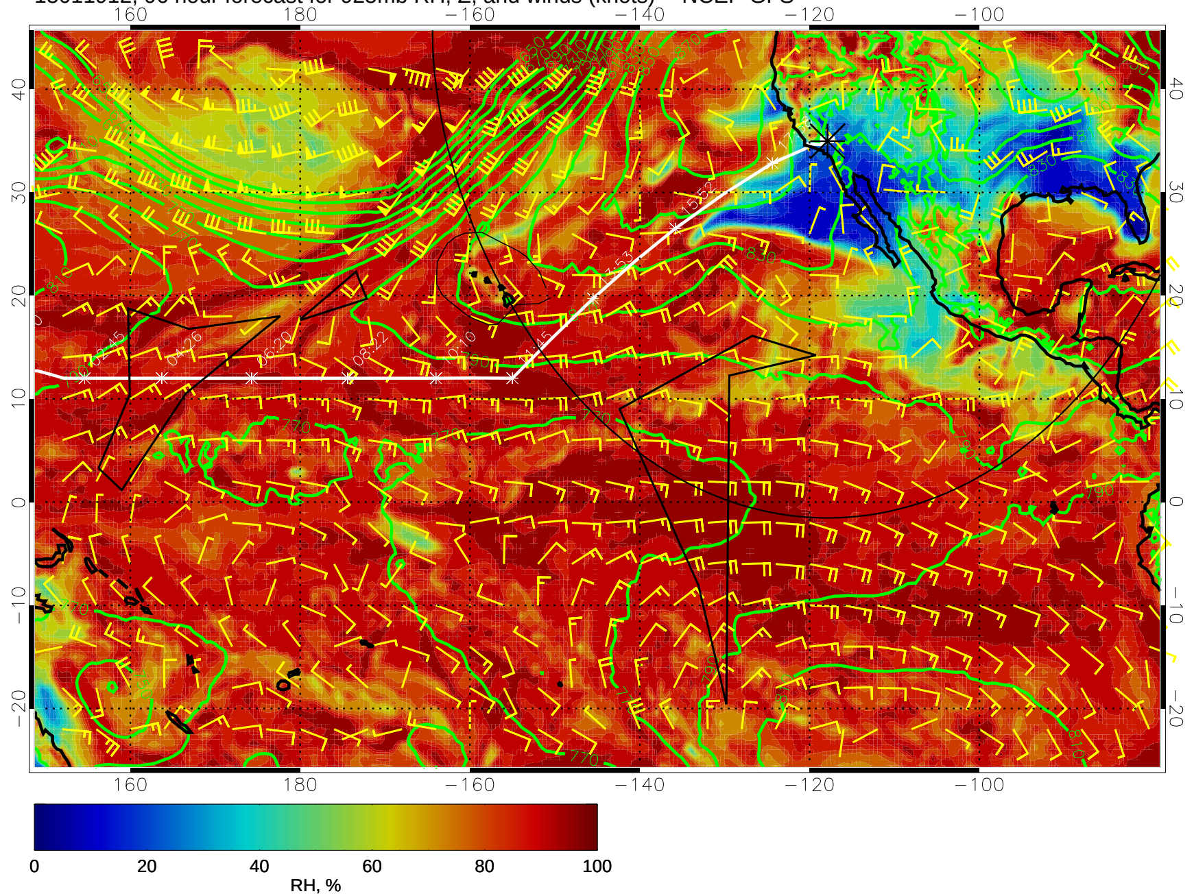
15011912, 96 hour forecast for 925mb RH, Z, and winds (knots) -- NCEP GFS
