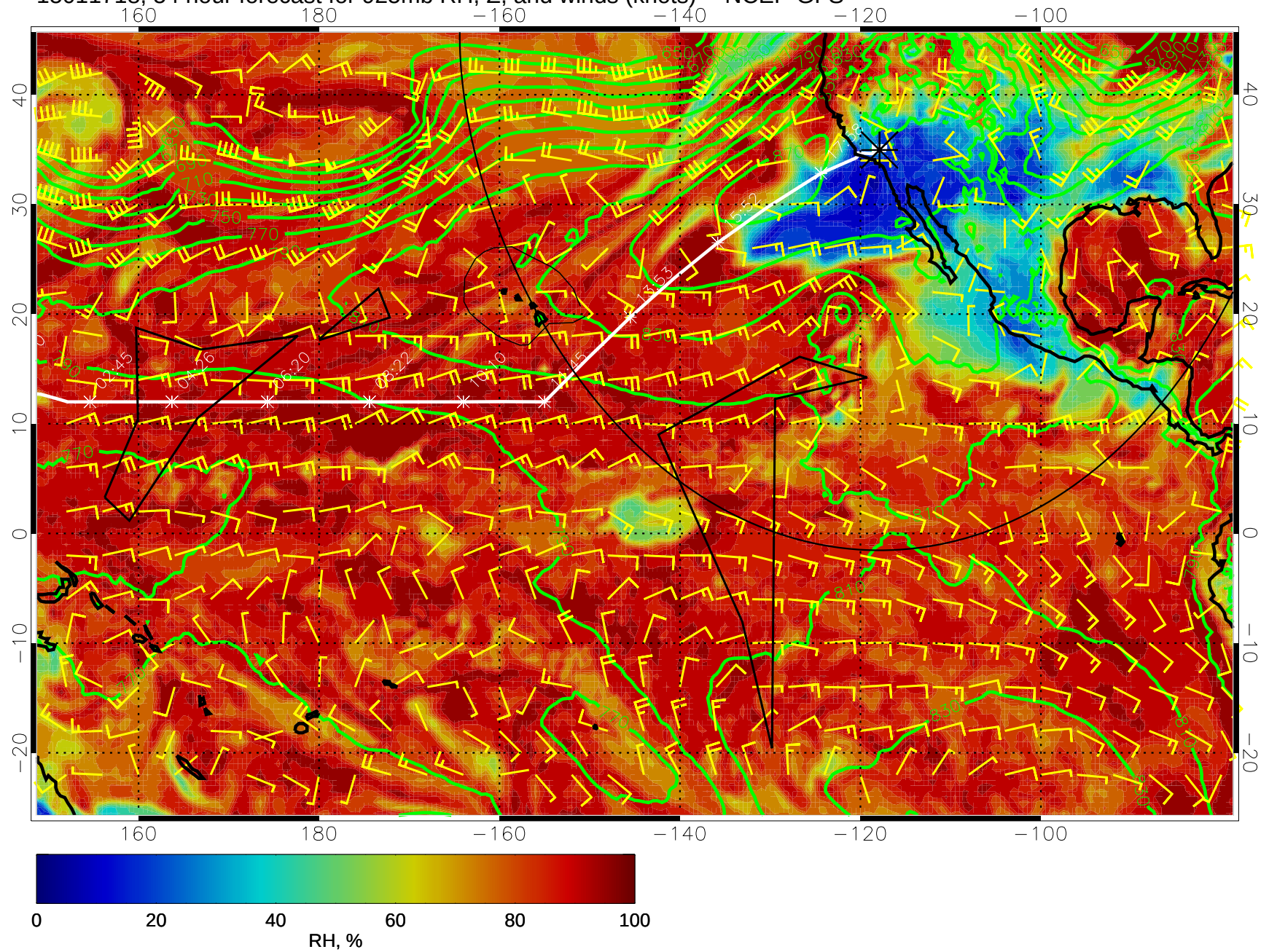
15011718, 54 hour forecast for 925mb RH, Z, and winds (knots) -- NCEP GFS
