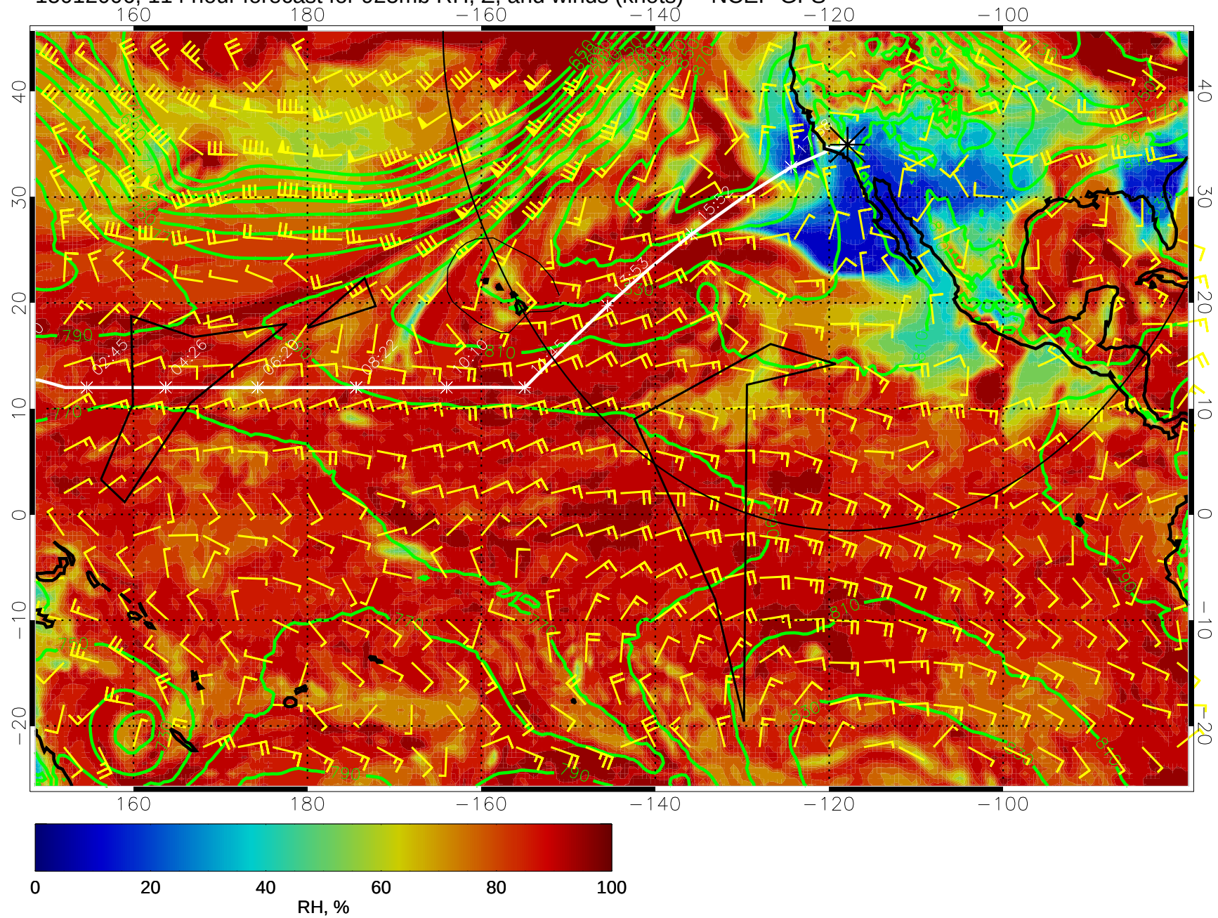
15012006, 114 hour forecast for 925mb RH, Z, and winds (knots) -- NCEP GFS
