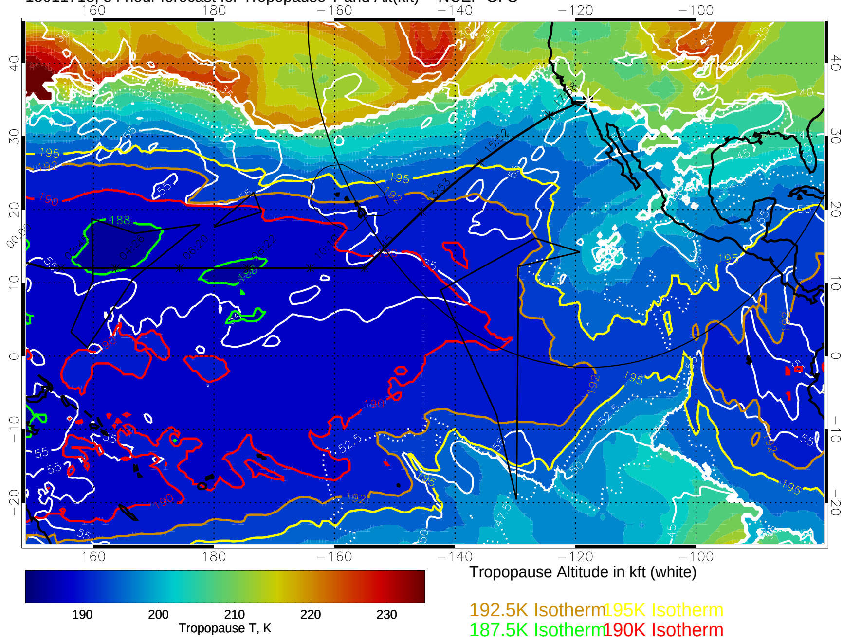
15011718, 54 hour forecast for Tropopause T and Alt(kft) -- NCEP GFS
