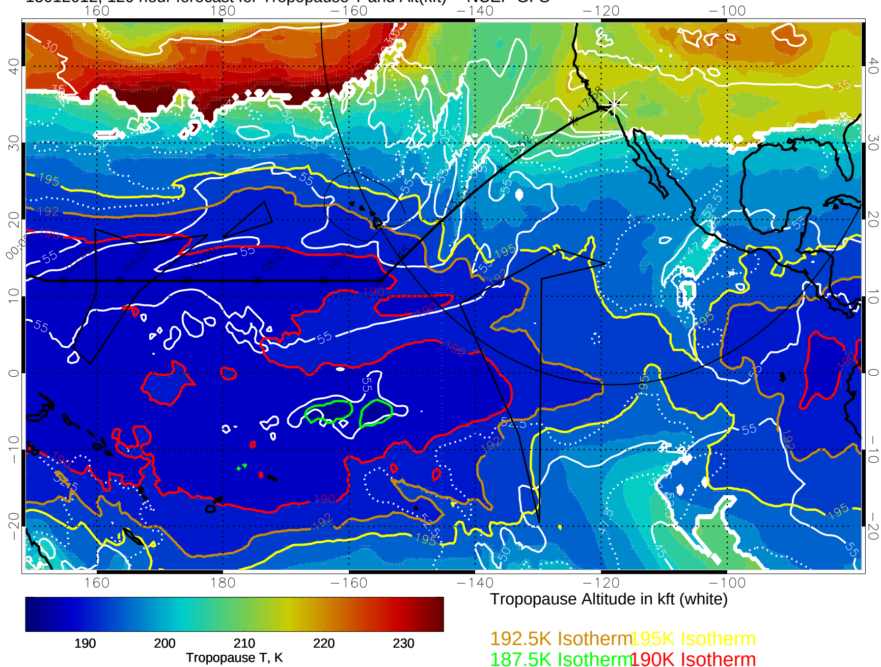
15012012, 120 hour forecast for Tropopause T and Alt(kft) -- NCEP GFS
