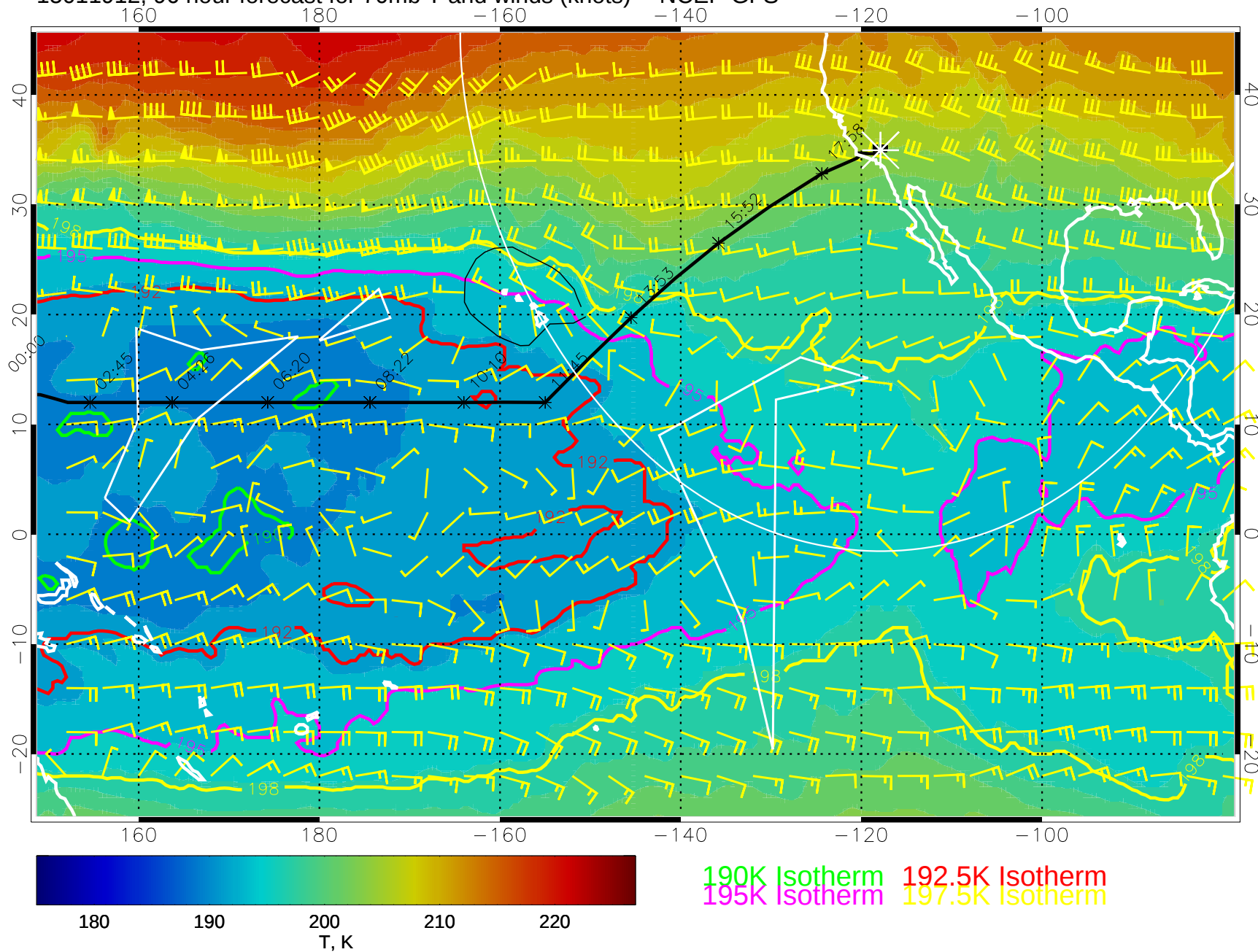
15011912, 96 hour forecast for 70mb T and winds (knots) -- NCEP GFS
