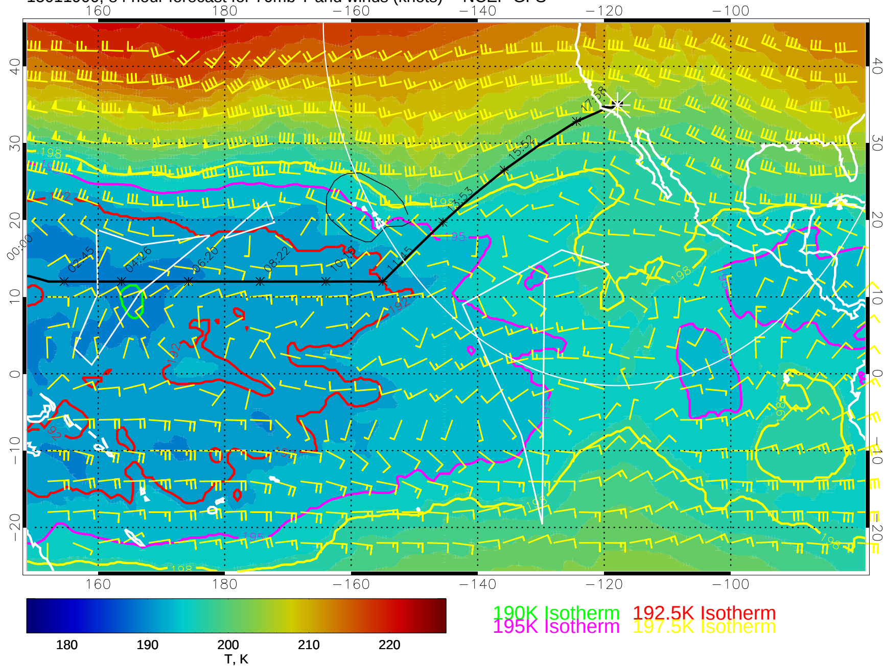
15011900, 84 hour forecast for 70mb T and winds (knots) -- NCEP GFS
