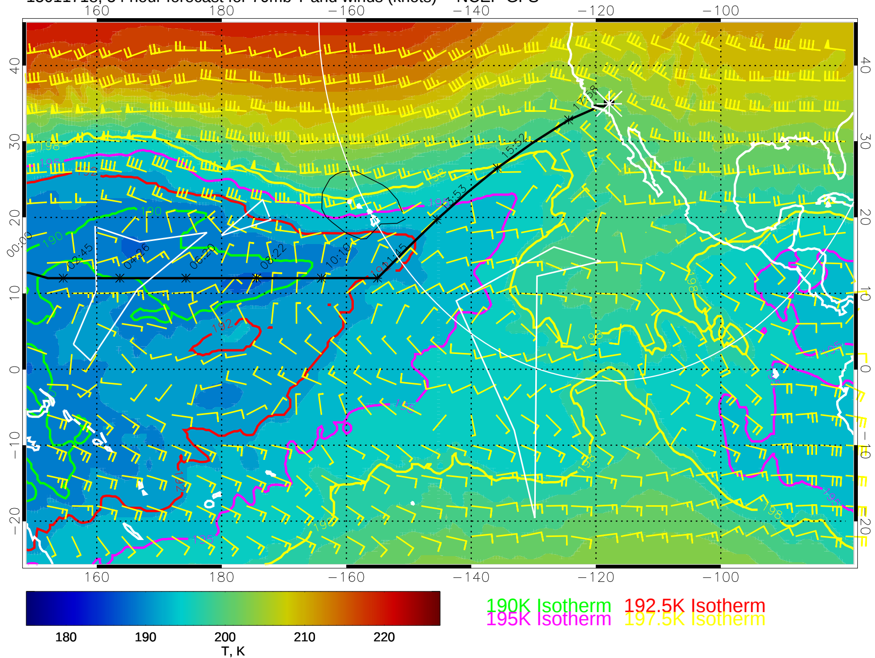
15011718, 54 hour forecast for 70mb T and winds (knots) -- NCEP GFS
