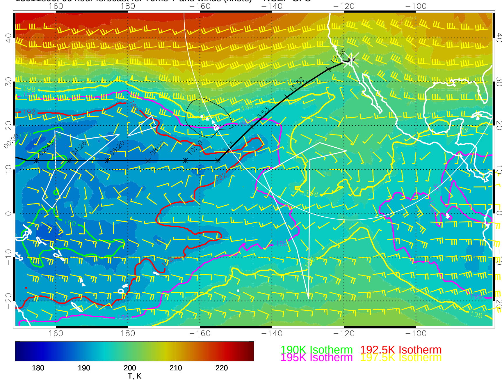
15011806, 66 hour forecast for 70mb T and winds (knots) -- NCEP GFS
