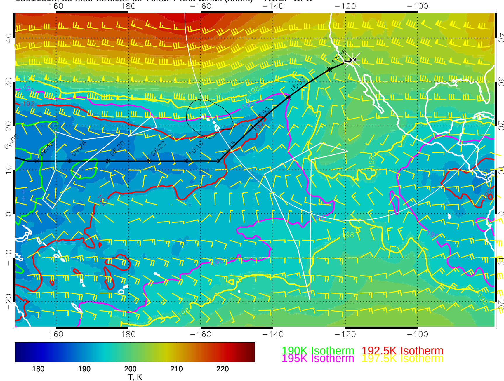
15011618, 30 hour forecast for 70mb T and winds (knots) -- NCEP GFS
