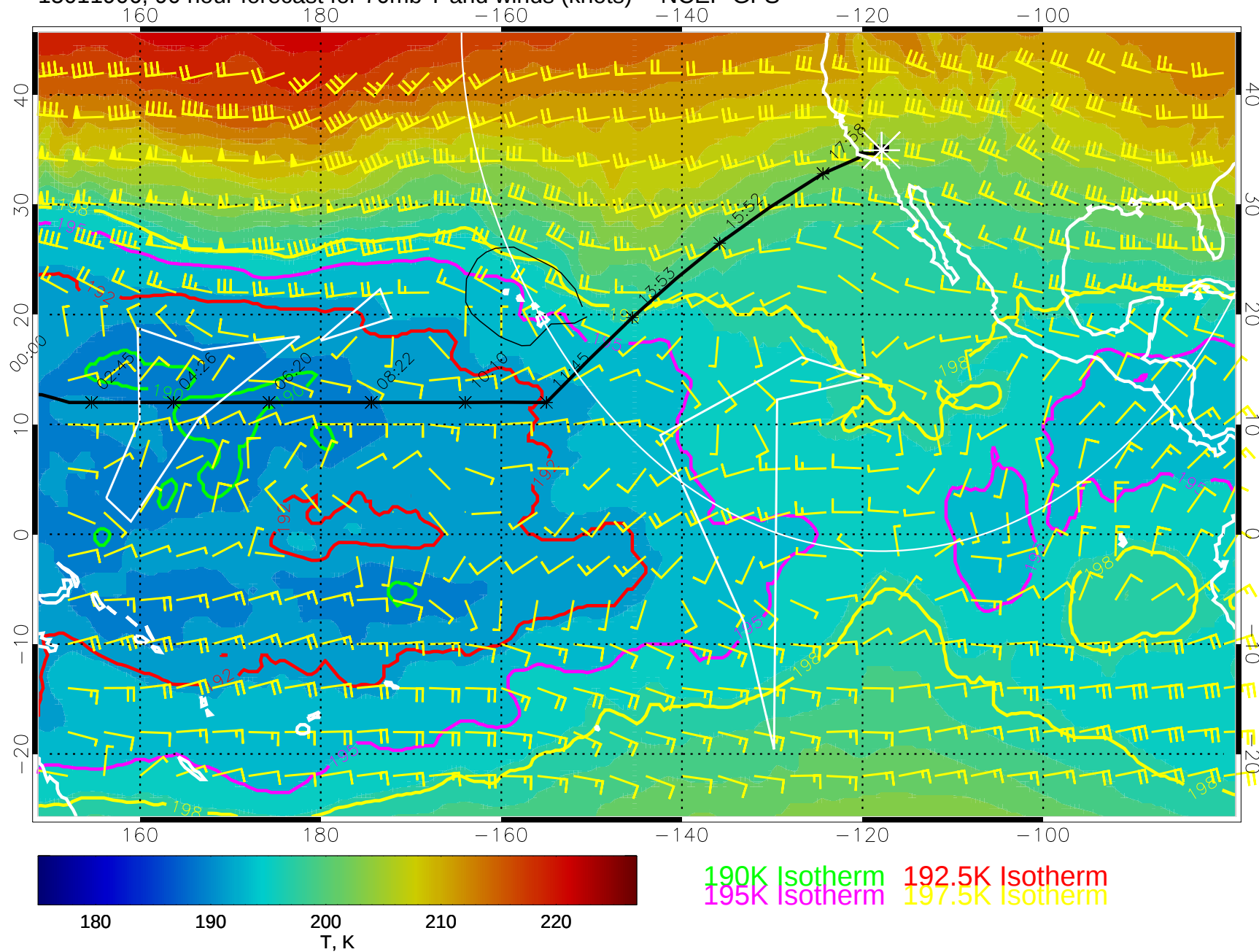
15011906, 90 hour forecast for 70mb T and winds (knots) -- NCEP GFS
