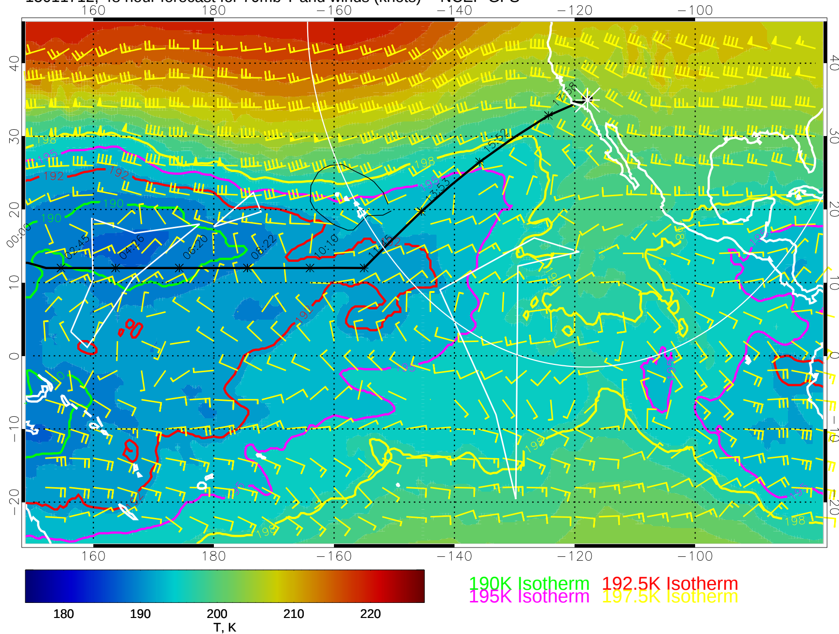
15011712, 48 hour forecast for 70mb T and winds (knots) -- NCEP GFS
