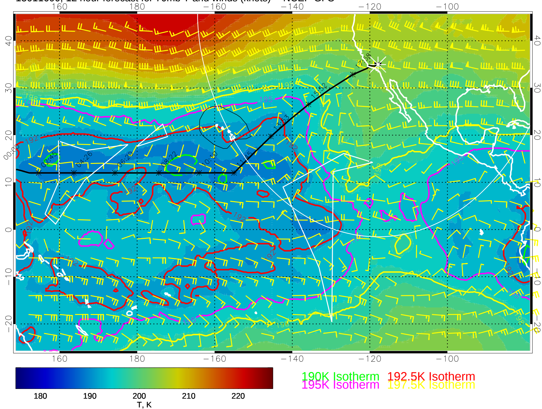
15011600, 12 hour forecast for 70mb T and winds (knots) -- NCEP GFS
