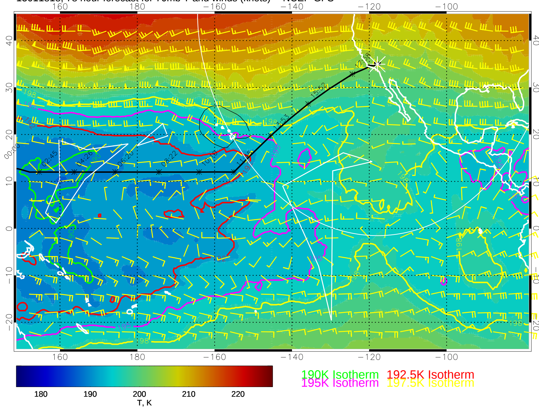
15011818, 78 hour forecast for 70mb T and winds (knots) -- NCEP GFS
