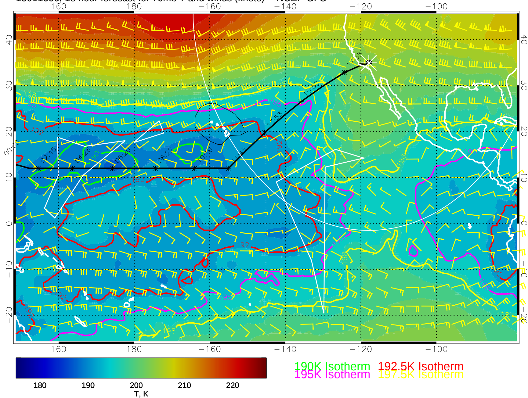
15011606, 18 hour forecast for 70mb T and winds (knots) -- NCEP GFS
