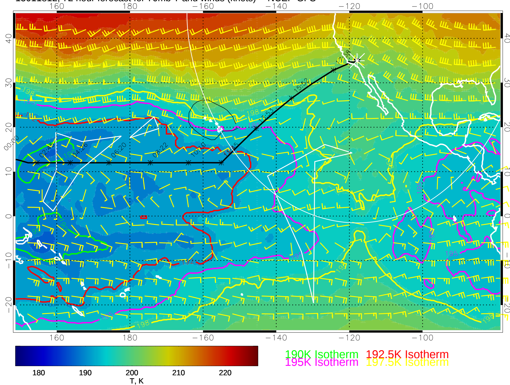
15011812, 72 hour forecast for 70mb T and winds (knots) -- NCEP GFS
