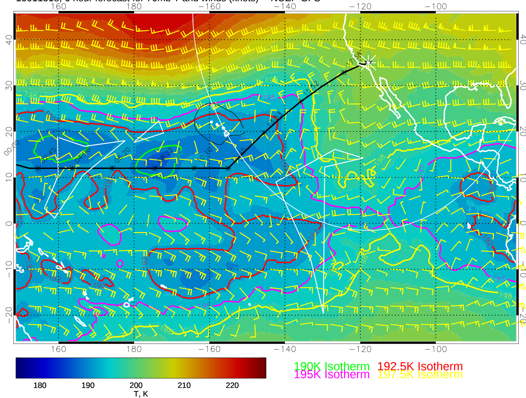
15011518, 6 hour forecast for 70mb T and winds (knots) -- NCEP GFS
