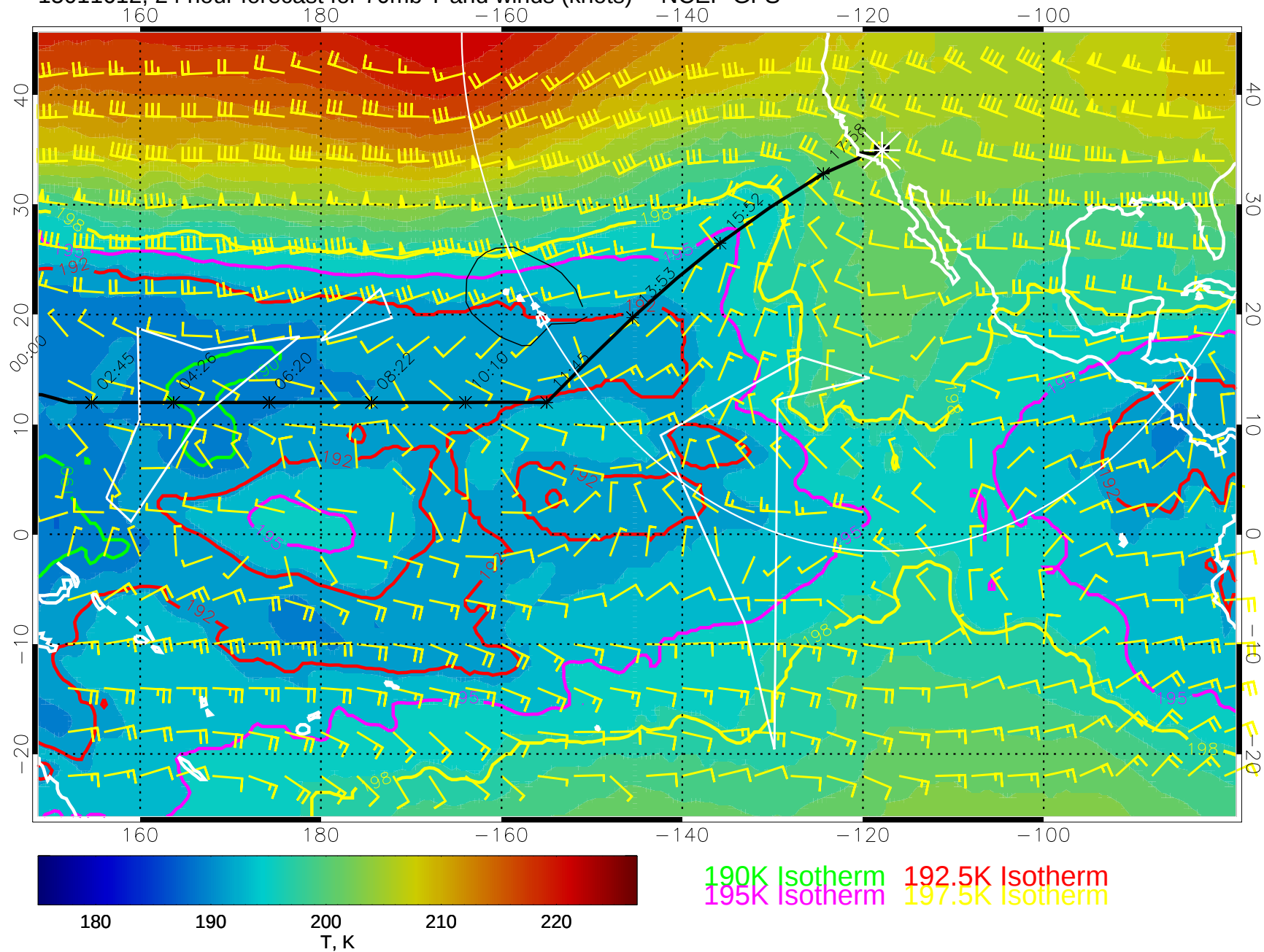
15011612, 24 hour forecast for 70mb T and winds (knots) -- NCEP GFS
