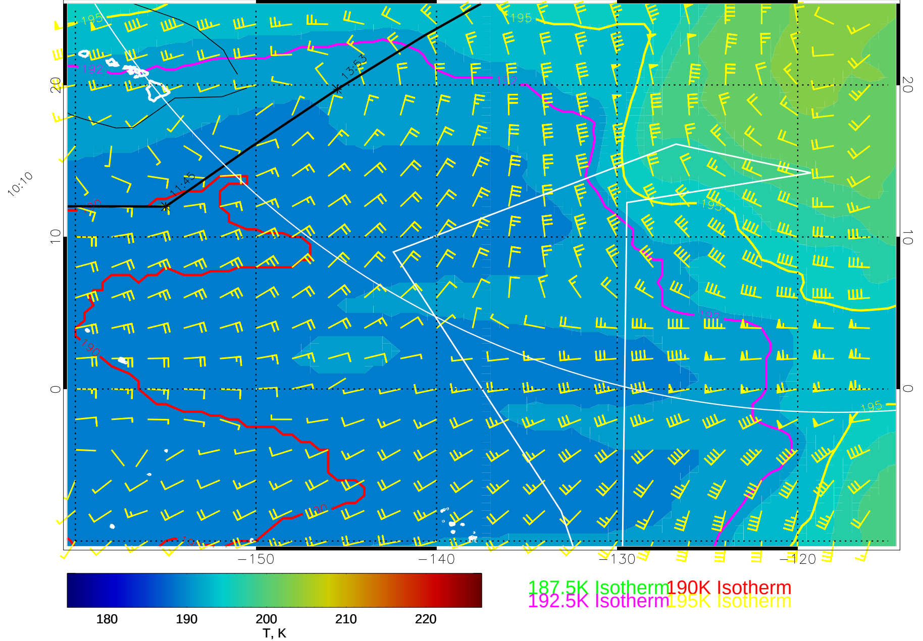
15011606, 18 hour forecast for 100mb T and winds (knots) -- NCEP GFS
