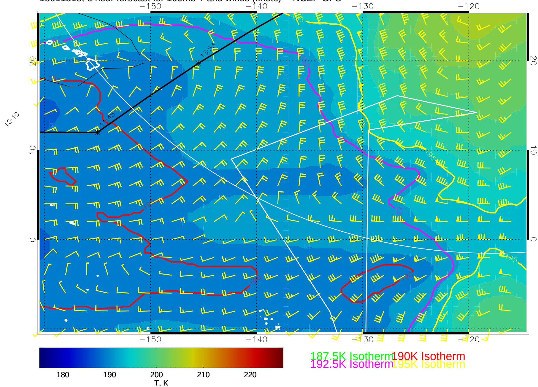
15011518, 6 hour forecast for 100mb T and winds (knots) -- NCEP GFS
