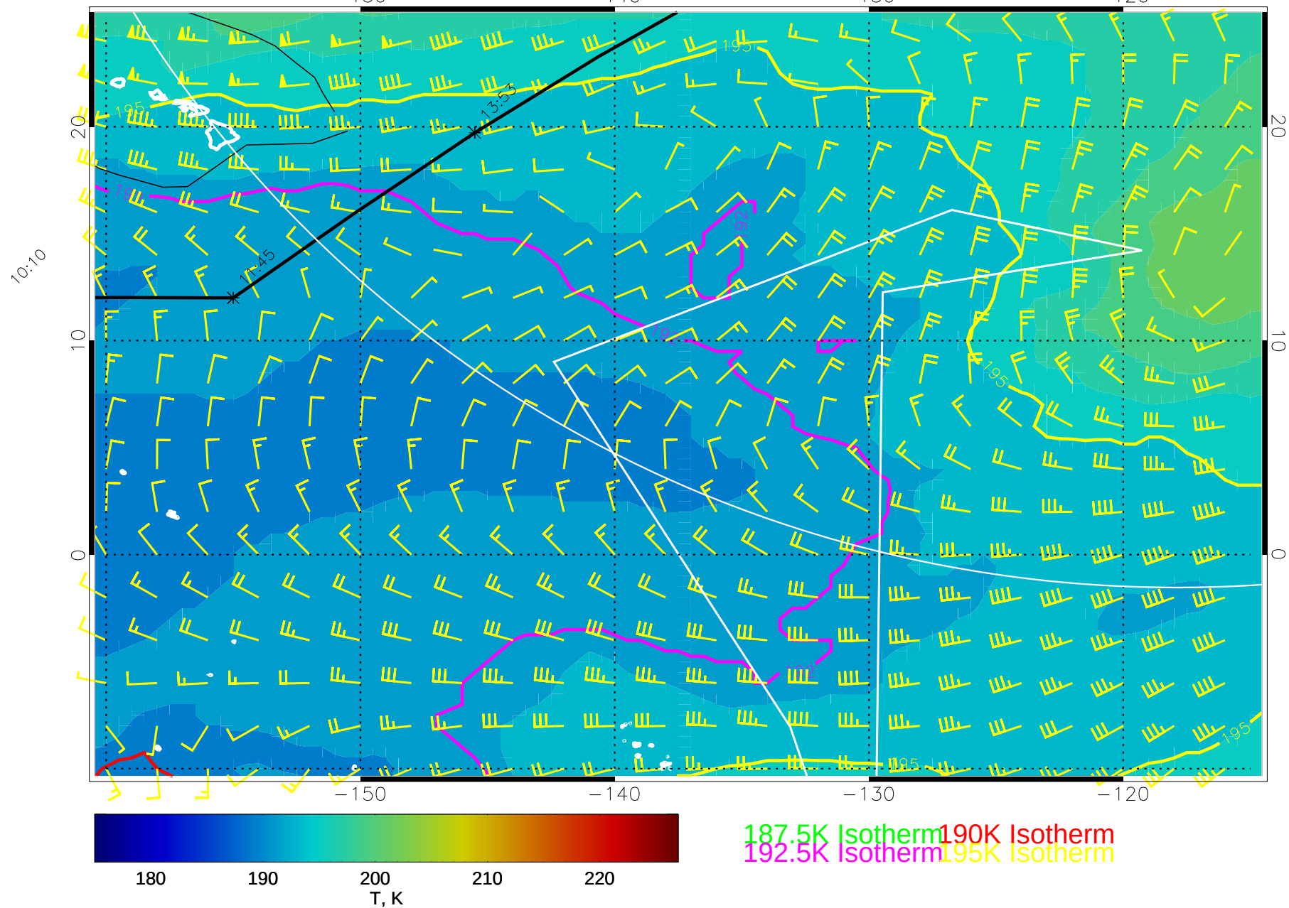
15011806, 66 hour forecast for 100mb T and winds (knots) -- NCEP GFS
