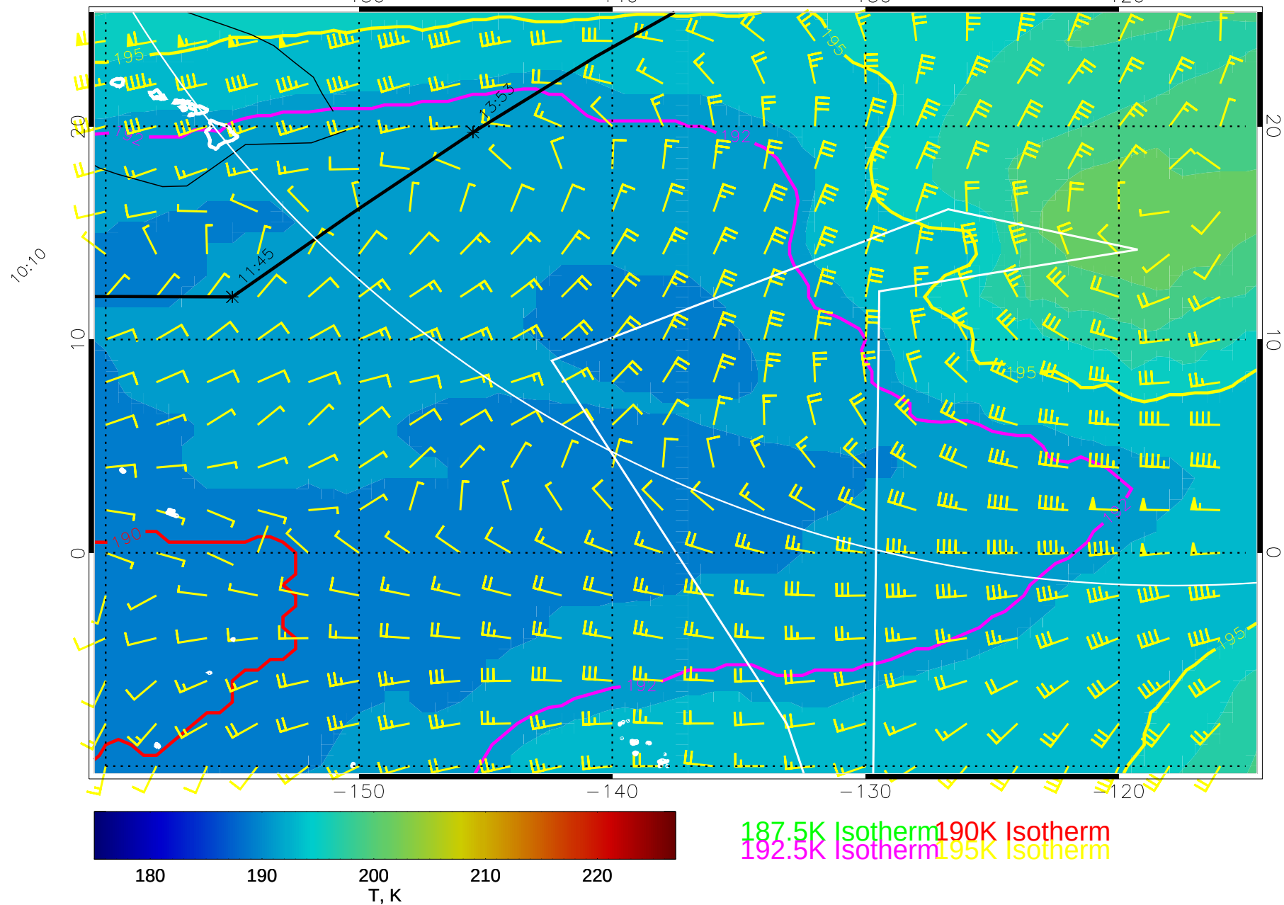
15011706, 42 hour forecast for 100mb T and winds (knots) -- NCEP GFS
