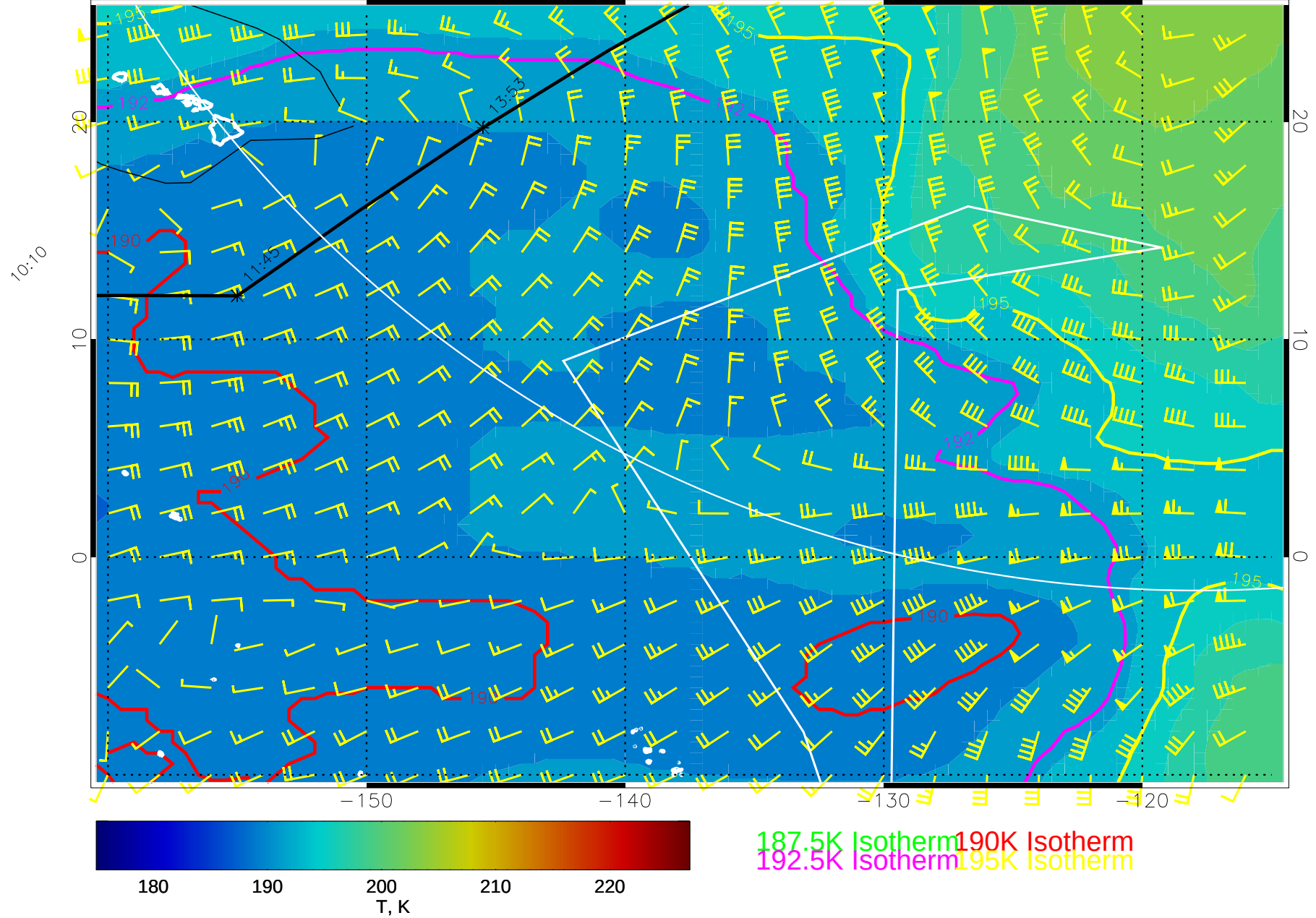
15011600, 12 hour forecast for 100mb T and winds (knots) -- NCEP GFS
