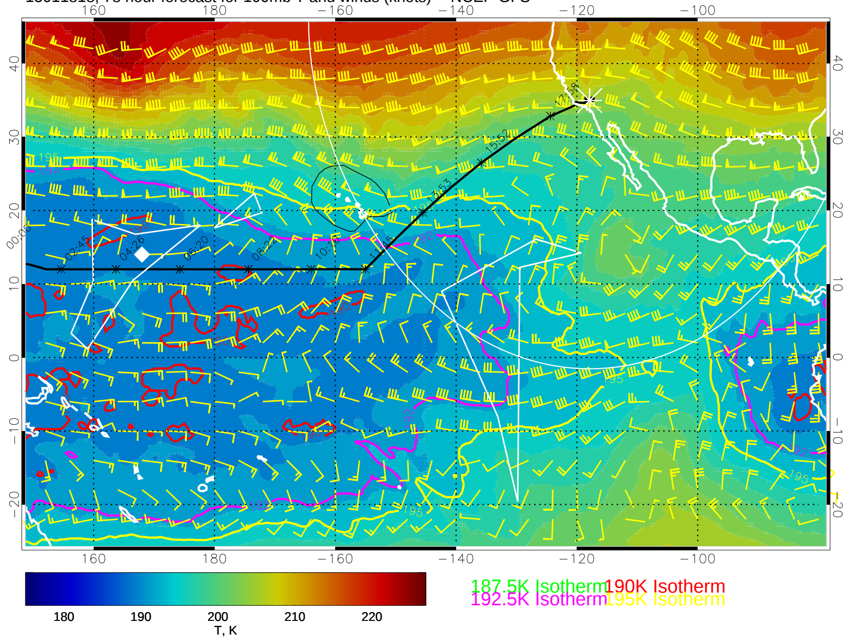
15011818, 78 hour forecast for 100mb T and winds (knots) -- NCEP GFS
