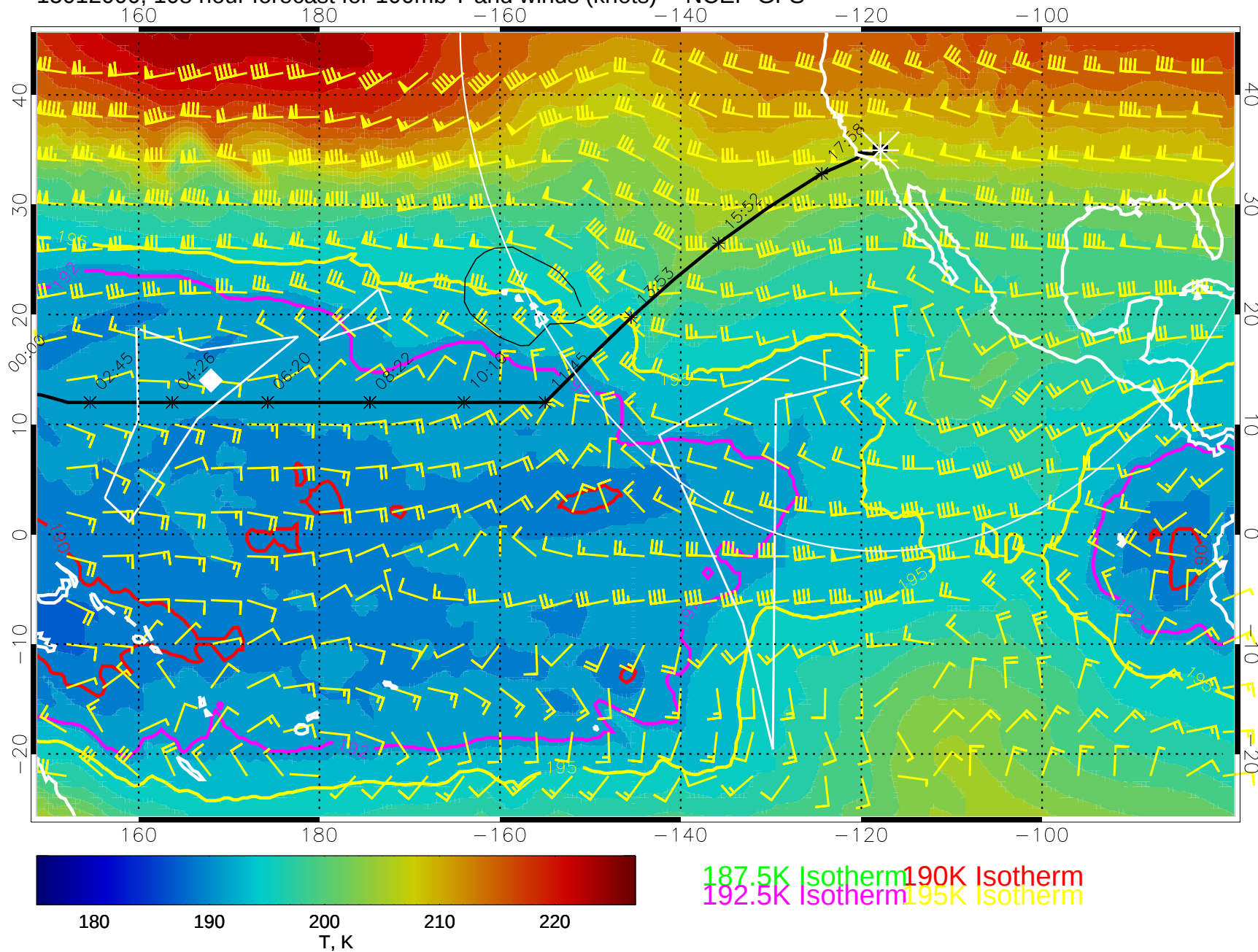
15012000, 108 hour forecast for 100mb T and winds (knots) -- NCEP GFS
