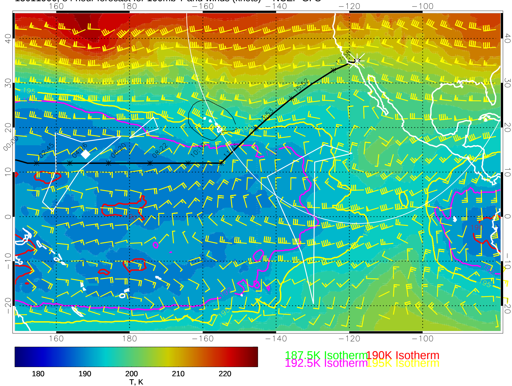
15011900, 84 hour forecast for 100mb T and winds (knots) -- NCEP GFS
