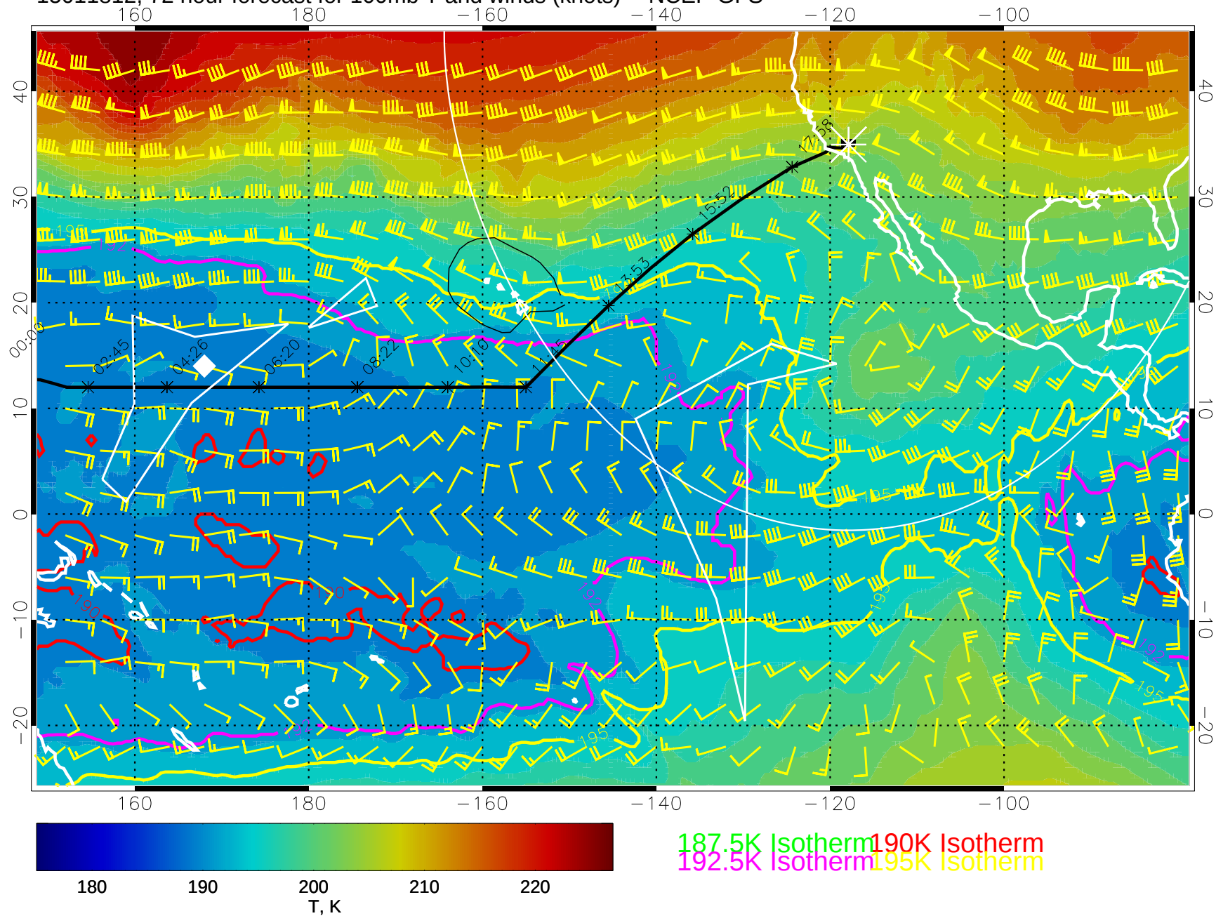
15011812, 72 hour forecast for 100mb T and winds (knots) -- NCEP GFS
