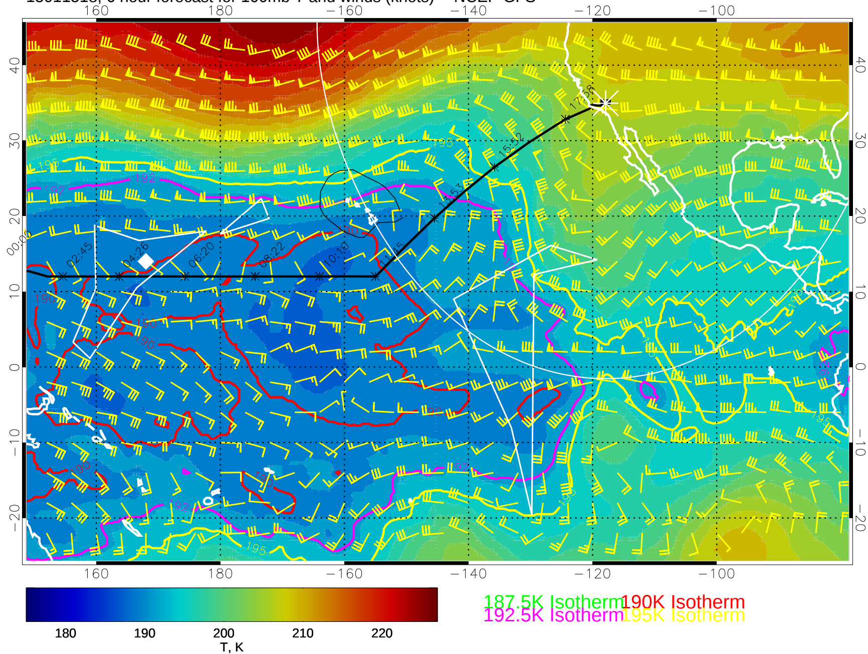
15011518, 6 hour forecast for 100mb T and winds (knots) -- NCEP GFS
