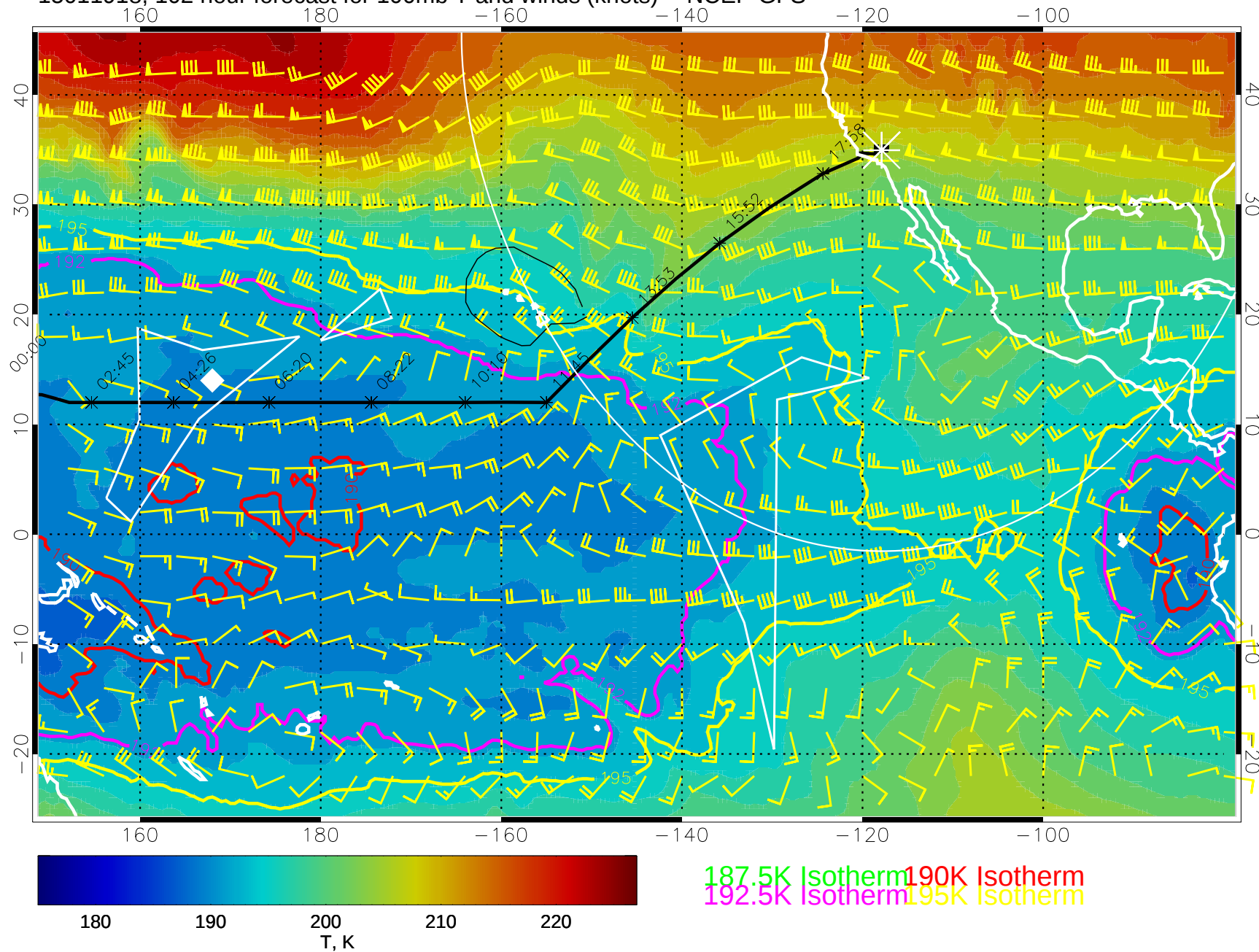
15011918, 102 hour forecast for 100mb T and winds (knots) -- NCEP GFS
