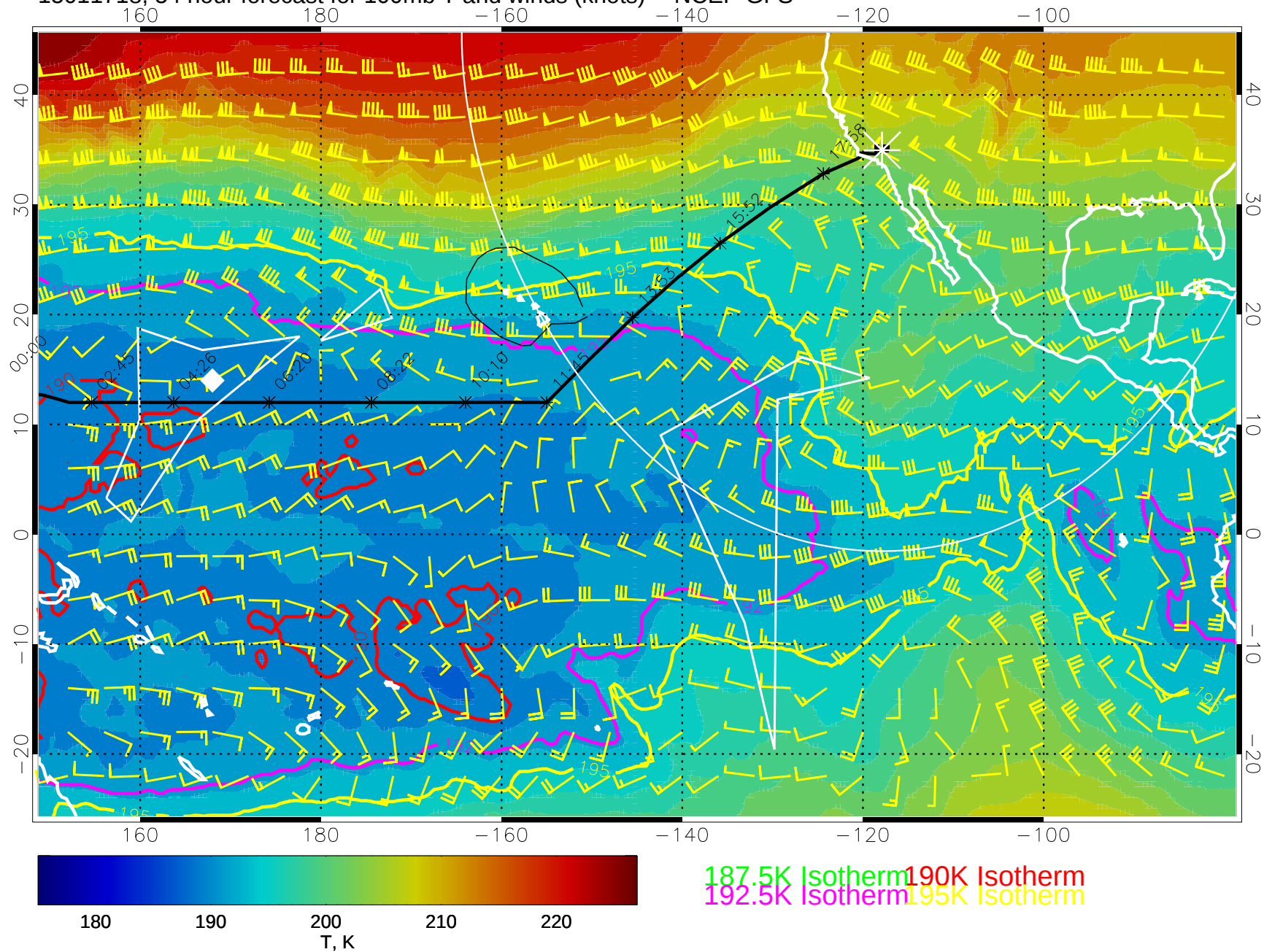
15011718, 54 hour forecast for 100mb T and winds (knots) -- NCEP GFS
