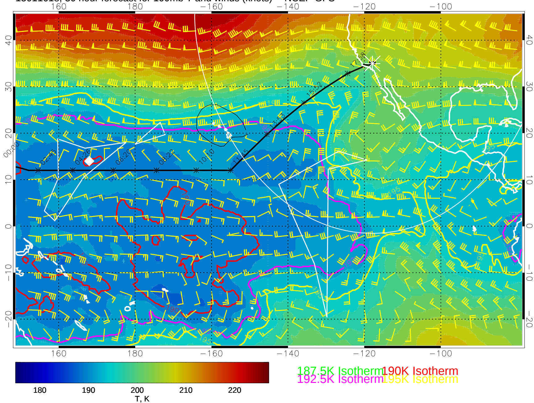
15011618, 30 hour forecast for 100mb T and winds (knots) -- NCEP GFS
