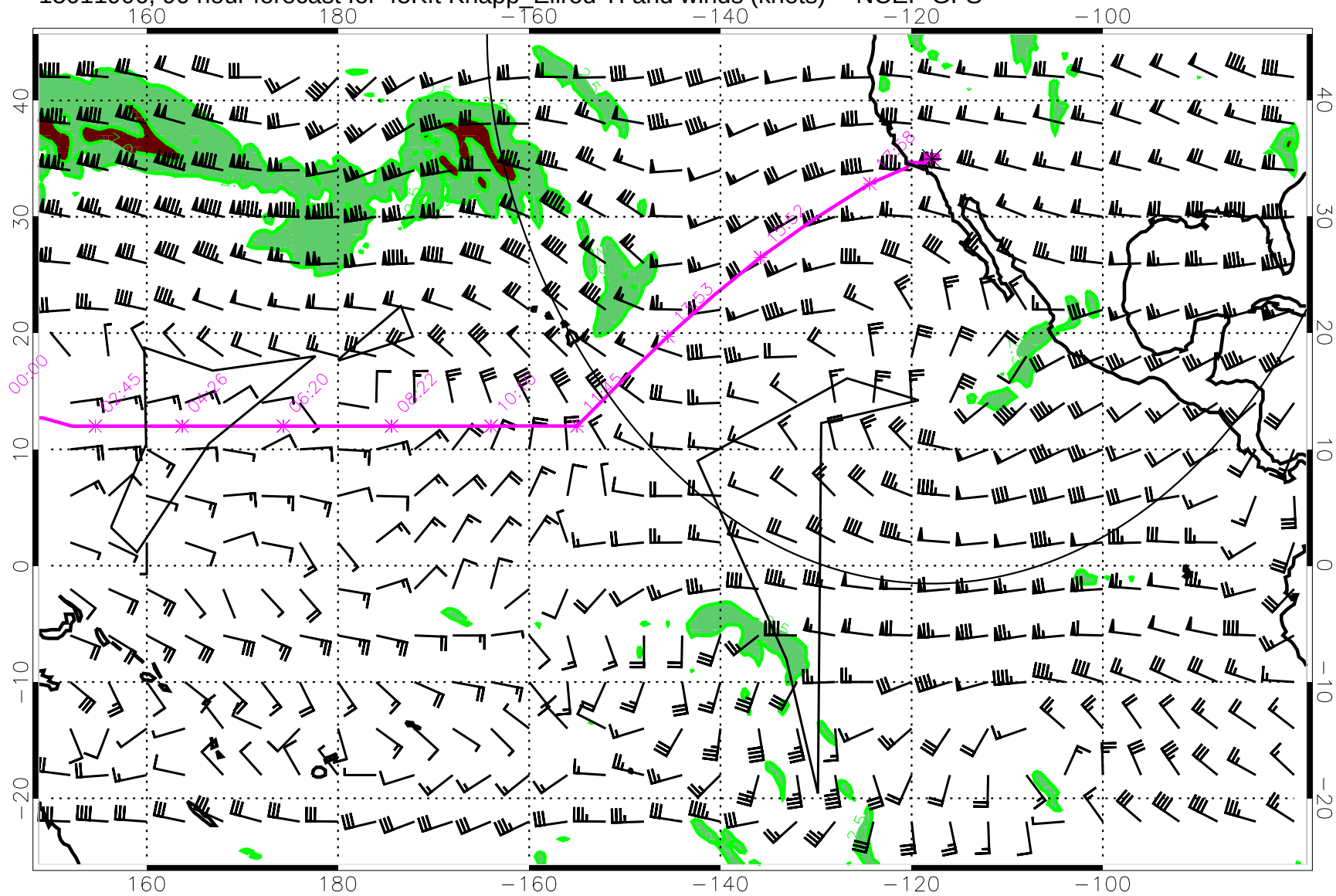
15011906, 90 hour forecast for 45Kft Knapp_Ellrod TI and winds (knots) -- NCEP GFS
